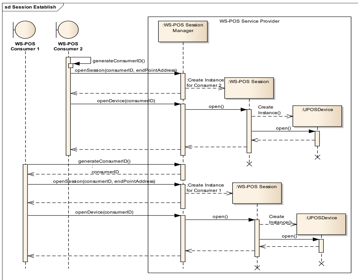
Figure 9: Establish Session
