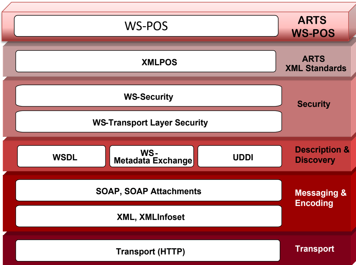
Figure 2: WS-POS Stack
