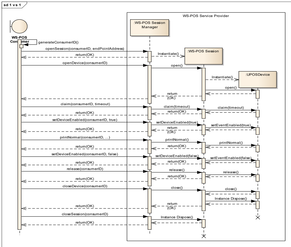
Figure 10: POS Printer - Print Normal example
