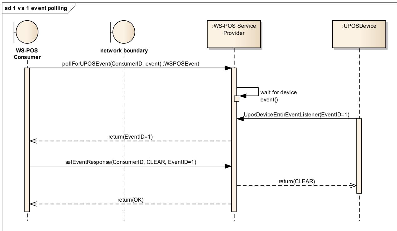
Figure 17: Event Polling
