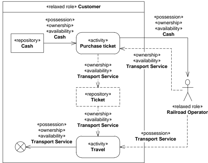
Figure 102 - Example of a POA Model Figure 102—Example of a POA Model
