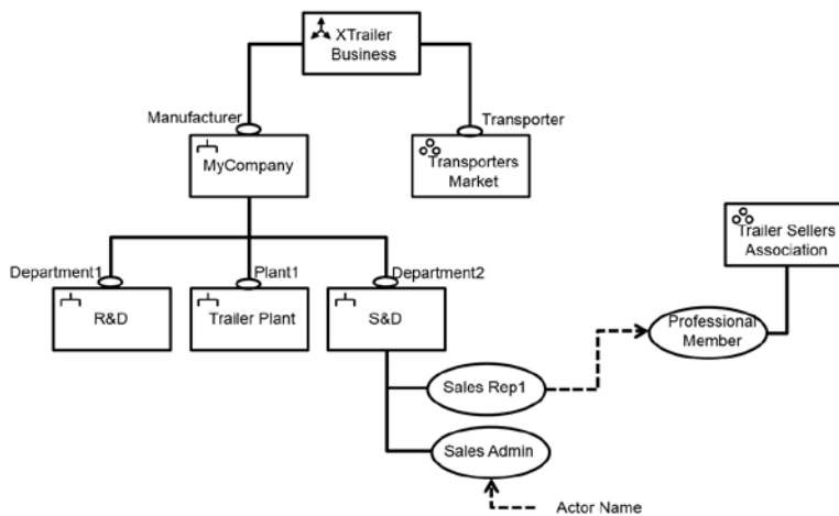
Figure 76 - Collaboration Structure diagram (example)
