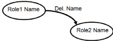
Figure 34 - DeliverableFlow for Tangible, connecting two Roles
