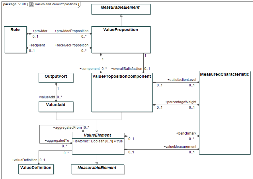
Figure 7.12 - Values and ValuePropositions
