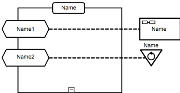
Figure 88 - CapabilityOffers of OrgUnit with capabilityResource and method from other OrgUnit (not shown) Figure 88 - CapabilityOffers of OrgUnit with capabilityResource and method from other OrgUnit (not shown)
