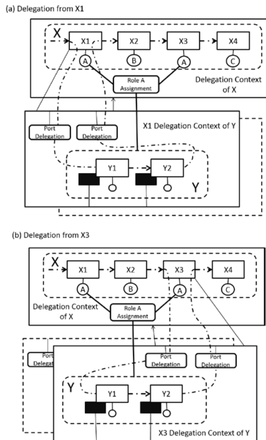
Figure 7.4 - Two uses of a collaboration
