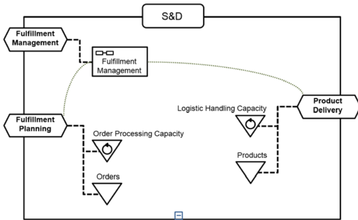
Figure 91 - Capability Management diagram (example)
