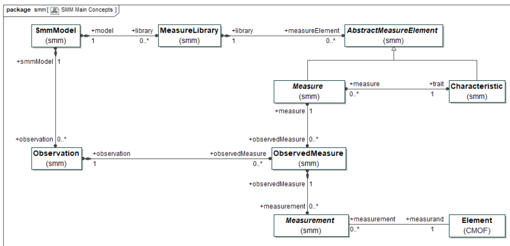
Figure 7.29 - SMM main concepts
