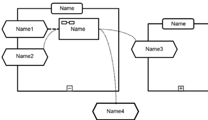
Figure 90 - Dependencies of CapabilityMethod on CapabilityOffers of methodOwner and other OrgUnits Figure 90 - Dependencies of CapabilityMethod on CapabilityOffers of methodOwner and other OrgUnits
