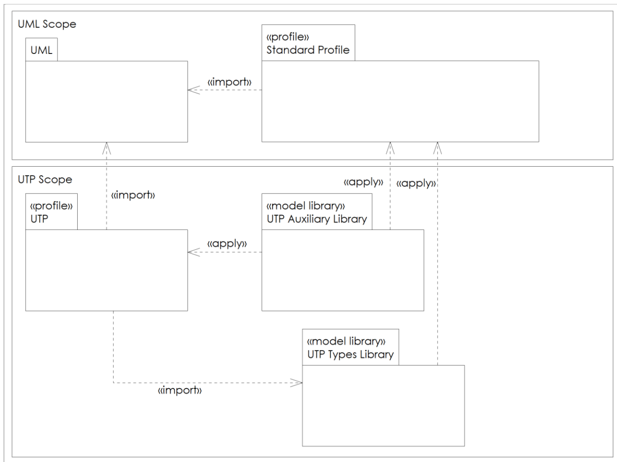
Figure 8.1 - Language Architecture
