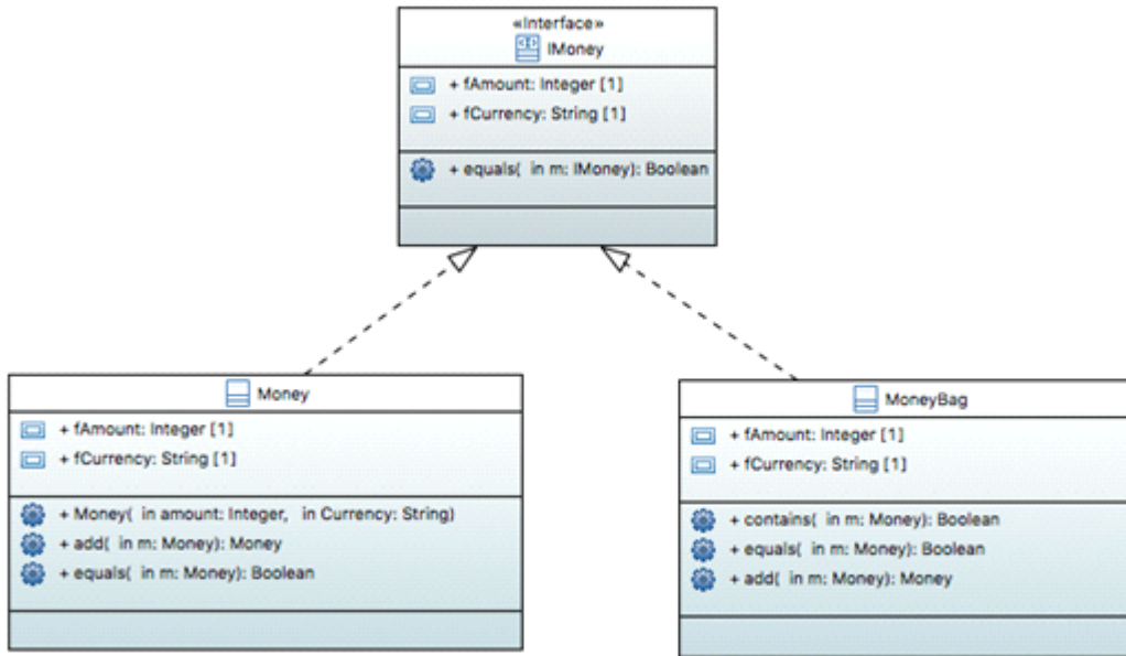
Figure A.4 - Classes in Package Money in IBEN ModelI
