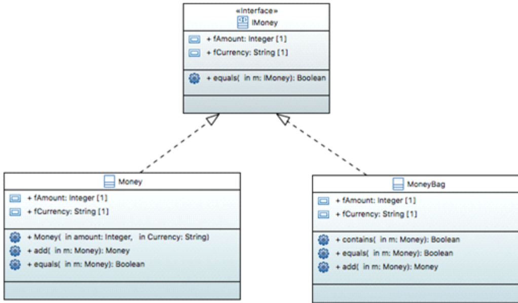
Figure A.4 - Classes in Package Money in IBEN Model
