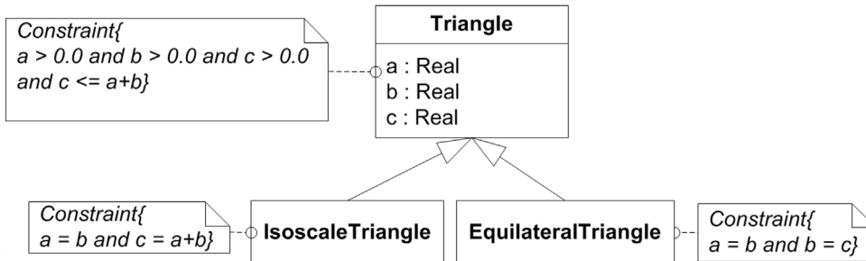
Figure 10.4 - Triangle classes
