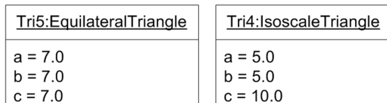
Figure 10.8 - Semantically equivalent InstanceSpecifications Figure 10.7
