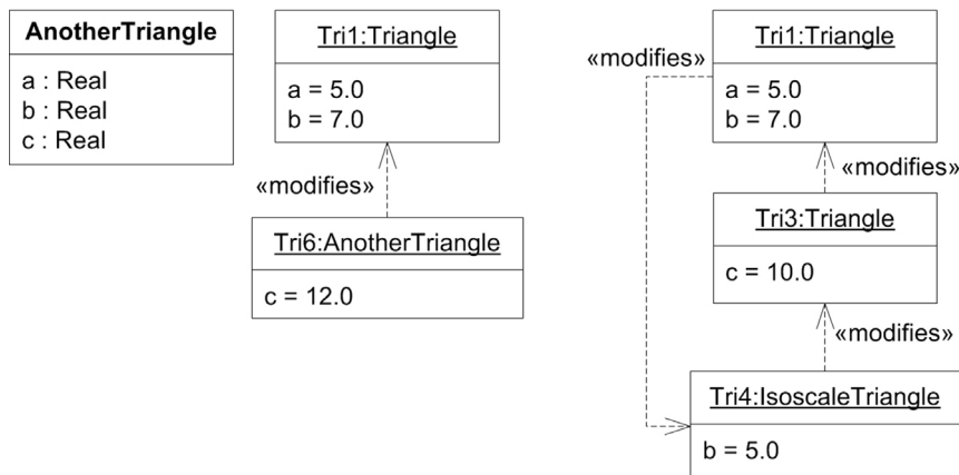
Figure 10.9 - Erroneous use of Modification
