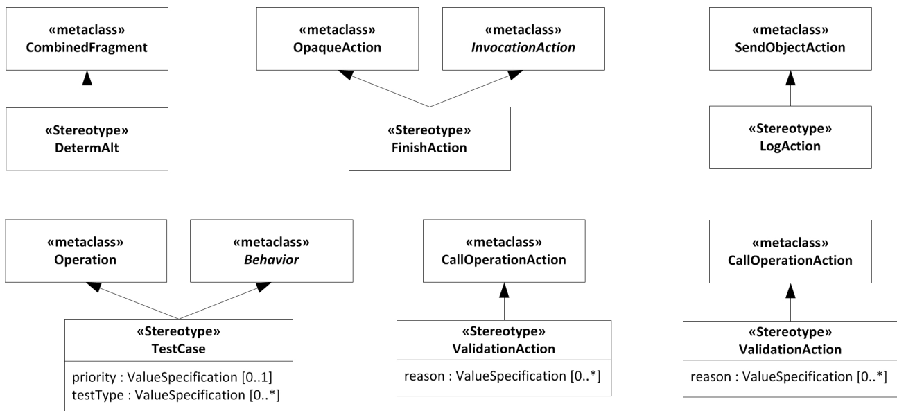
Figure 9.1 - Test Behavior Foundation
