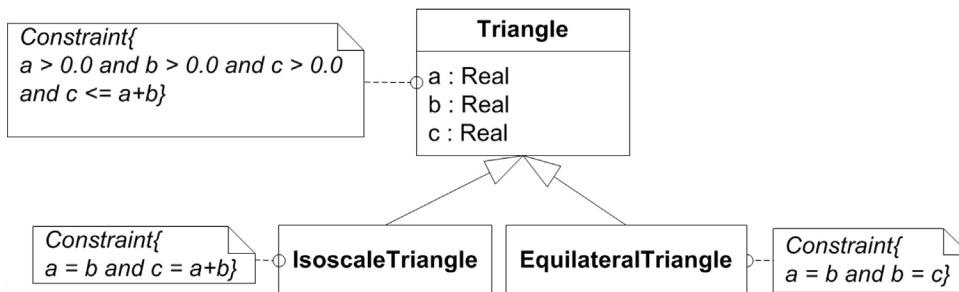
Figure 10.4 - Triangle classes
