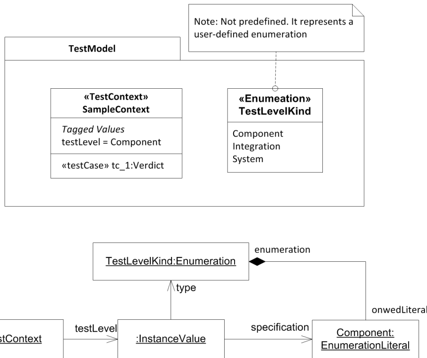
Figure 8.3 - User-defined test level values and corresponding object model
