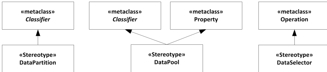
Figure 10.1 - Test Data Specification
