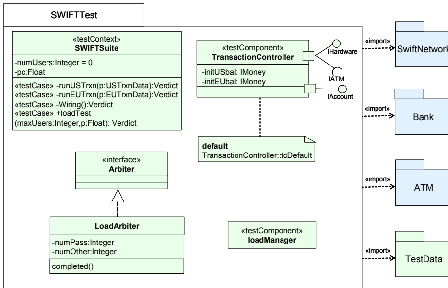
Figure 38. SWIFTTest package
