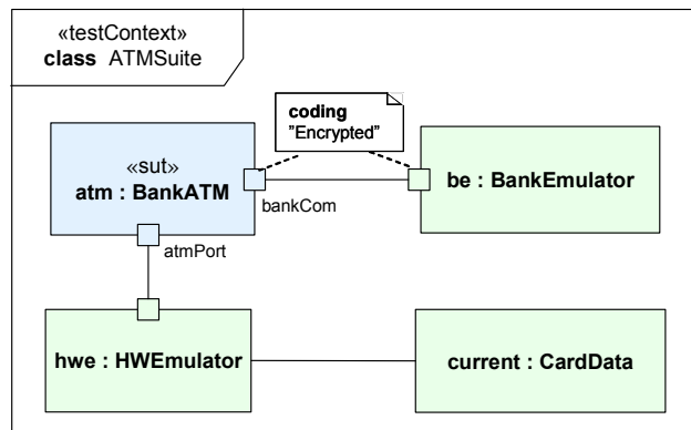
Figure 26. The composite structure of the ATMSuite test context
