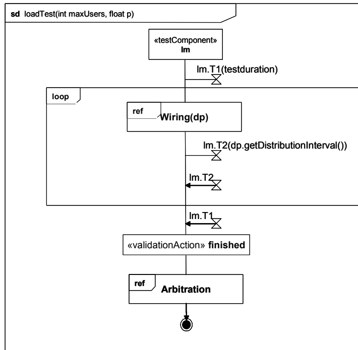
Figure 41. Main test behavior
