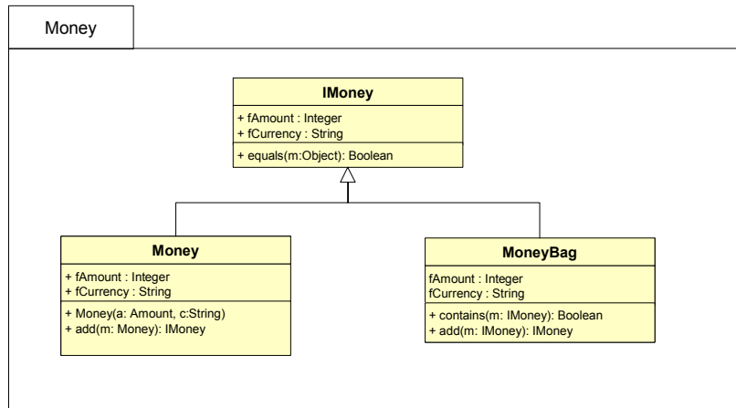
Figure 19. Money structure
