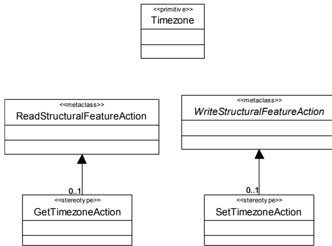
Figure 55. Timezone concepts
