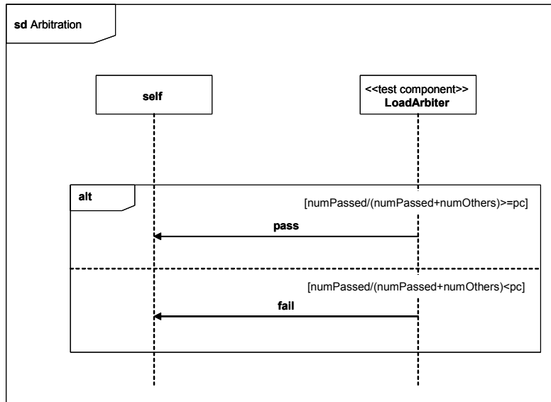
Figure 43. Arbitration behavior
