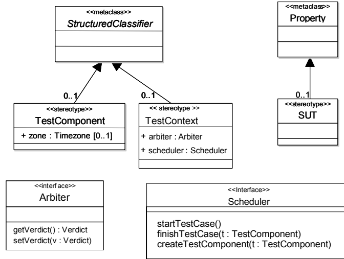
Figure 47. Test Architecture
