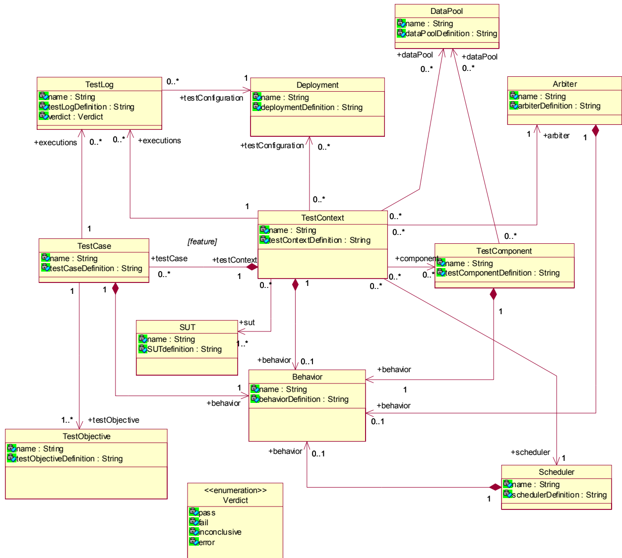
Figure 13. Test architecture and test behavior portion of the MOF-based metamodel
