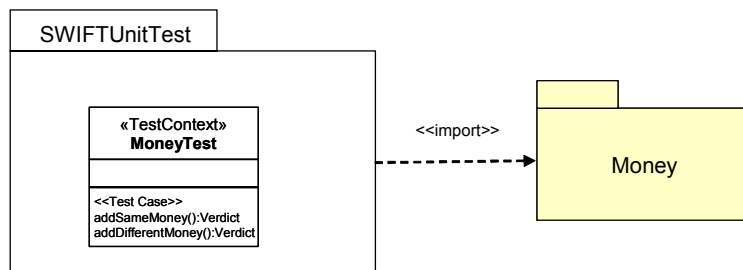
Figure 20. SWIFTUnitTest package
