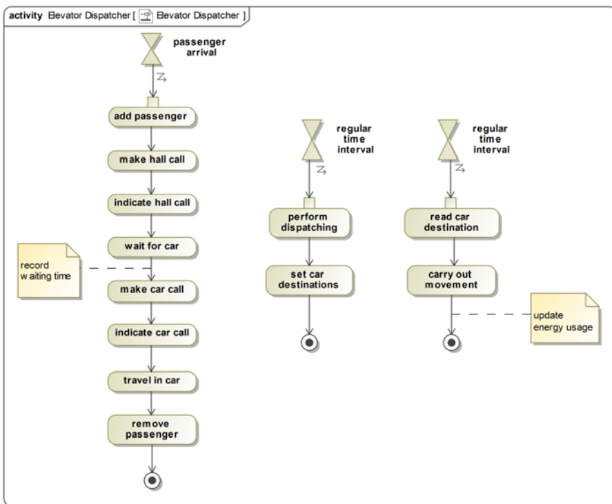
Figure A-2 Elevator Dispatcher Activity Diagram
