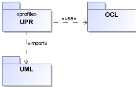
Figure 6-3 UPR Language Architecture
