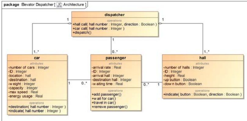
Figure A-3 Elevator Dispatcher Class Diagram
