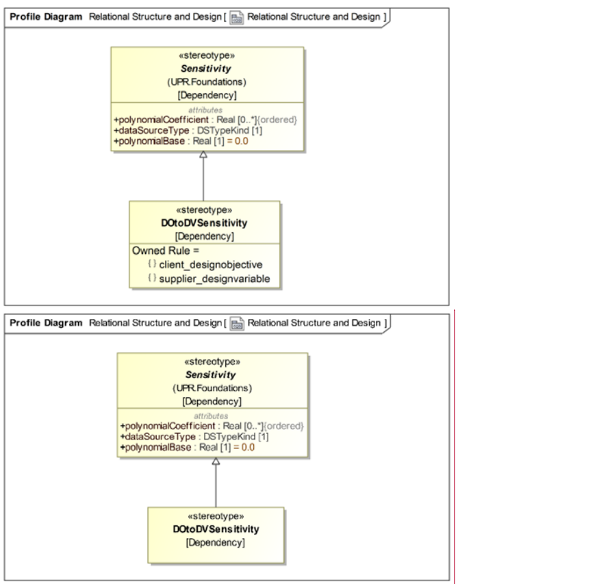
Figure 11-2 Relational Structure and Design Profile Diagram
