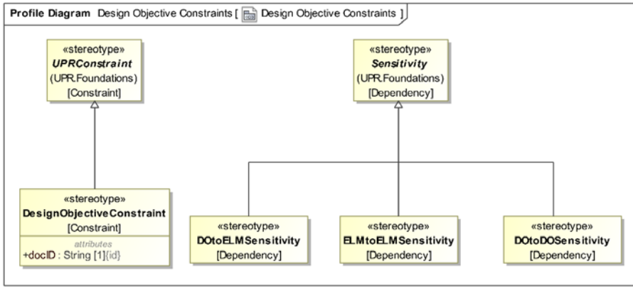
Figure 9-2 Design Objective Constraints Profile Diagram
