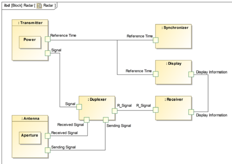
Figure 11-5 Radar system component architecture
