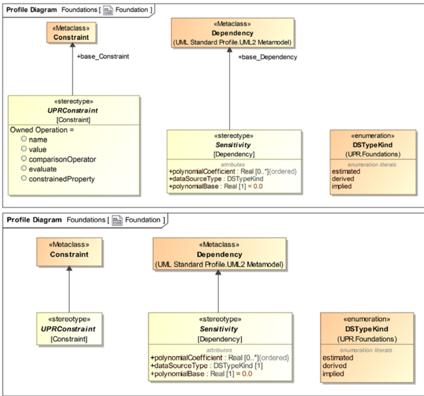
Figure 7-2 Foundations Profile Diagram 5
