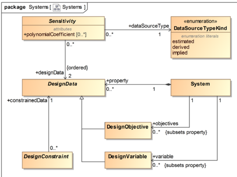
Figure 7-1 Systems (UPR Foundations) Domain Model
