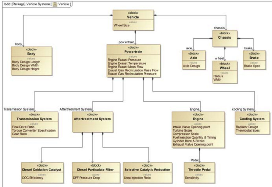
Figure B-1 Vehicle subsystems and properties
