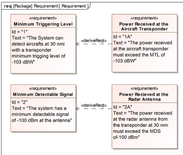
Figure 11-3 Design Objectives (Requirements) for a Radar System
