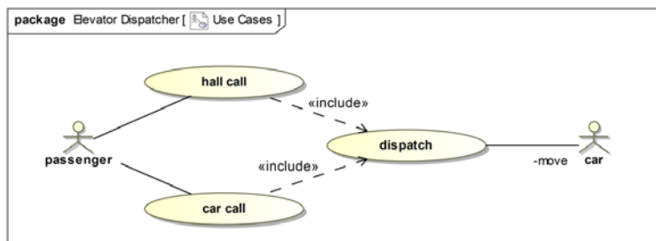
Figure A-1 Elevator Dispatcher Use Case Diagram
