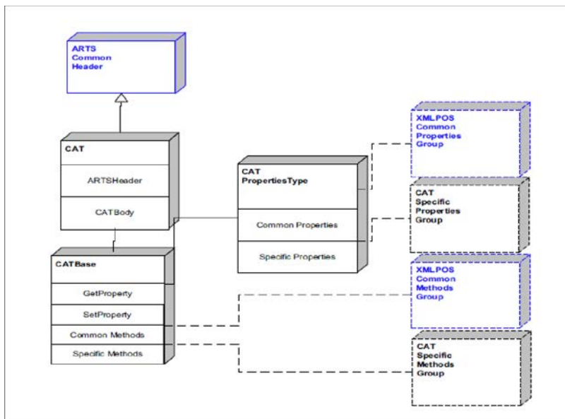
Figure 39: CAT Domain View
