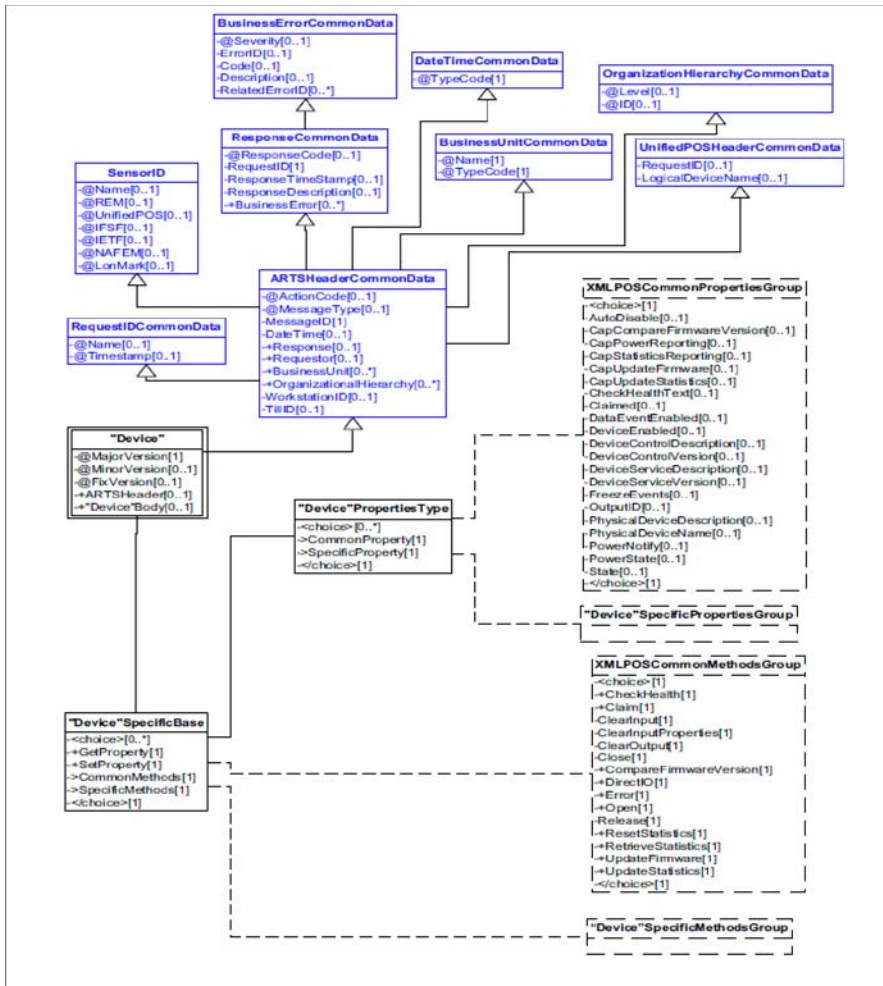
Figure 75: Image Scanner Domain View
