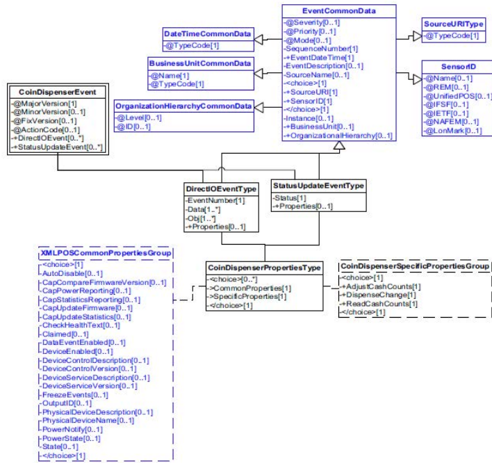
Figure 54: Coin Dispenser Events Domain View
