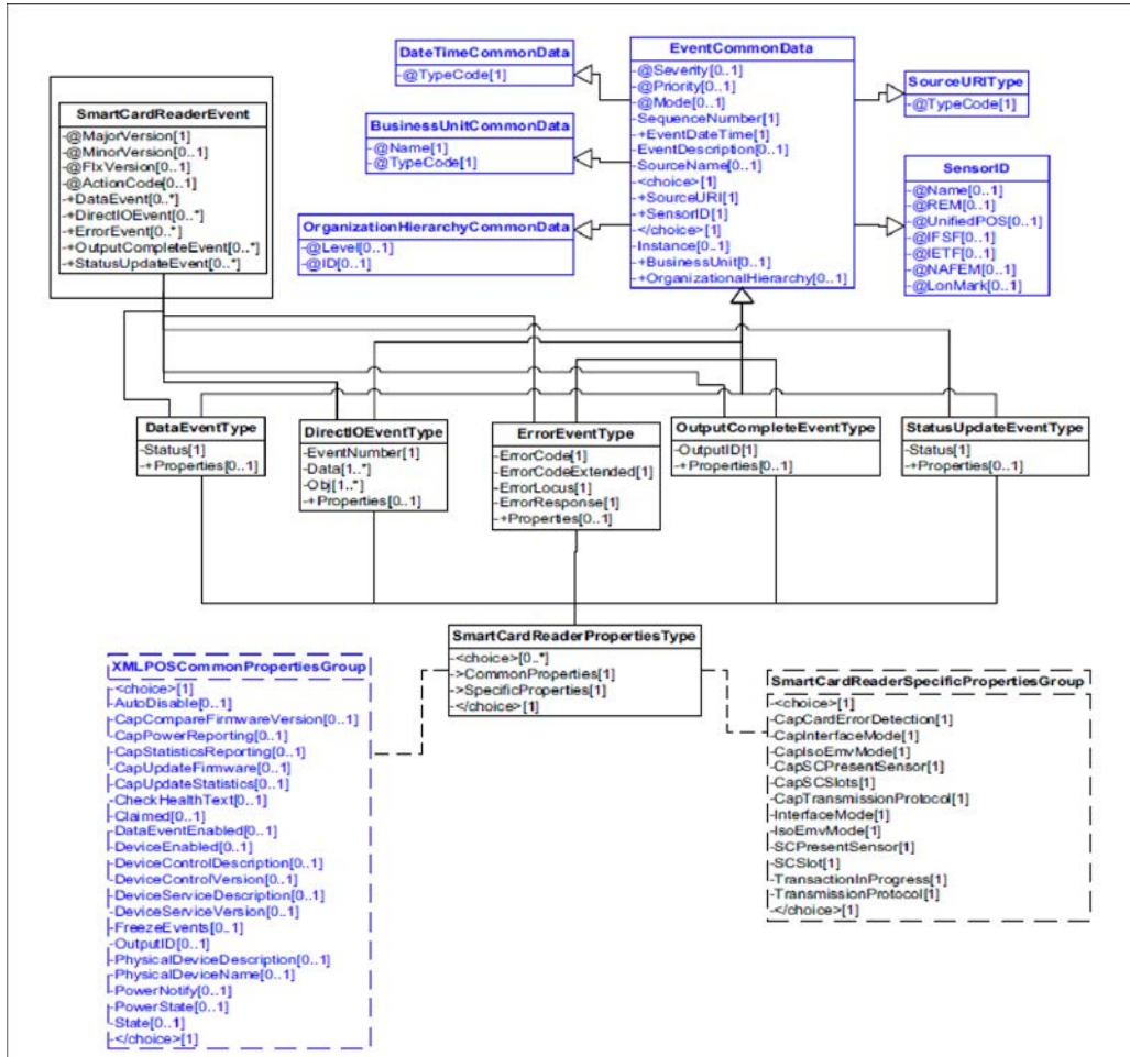
Figure 150: Smart Card Reader Events Domain View
