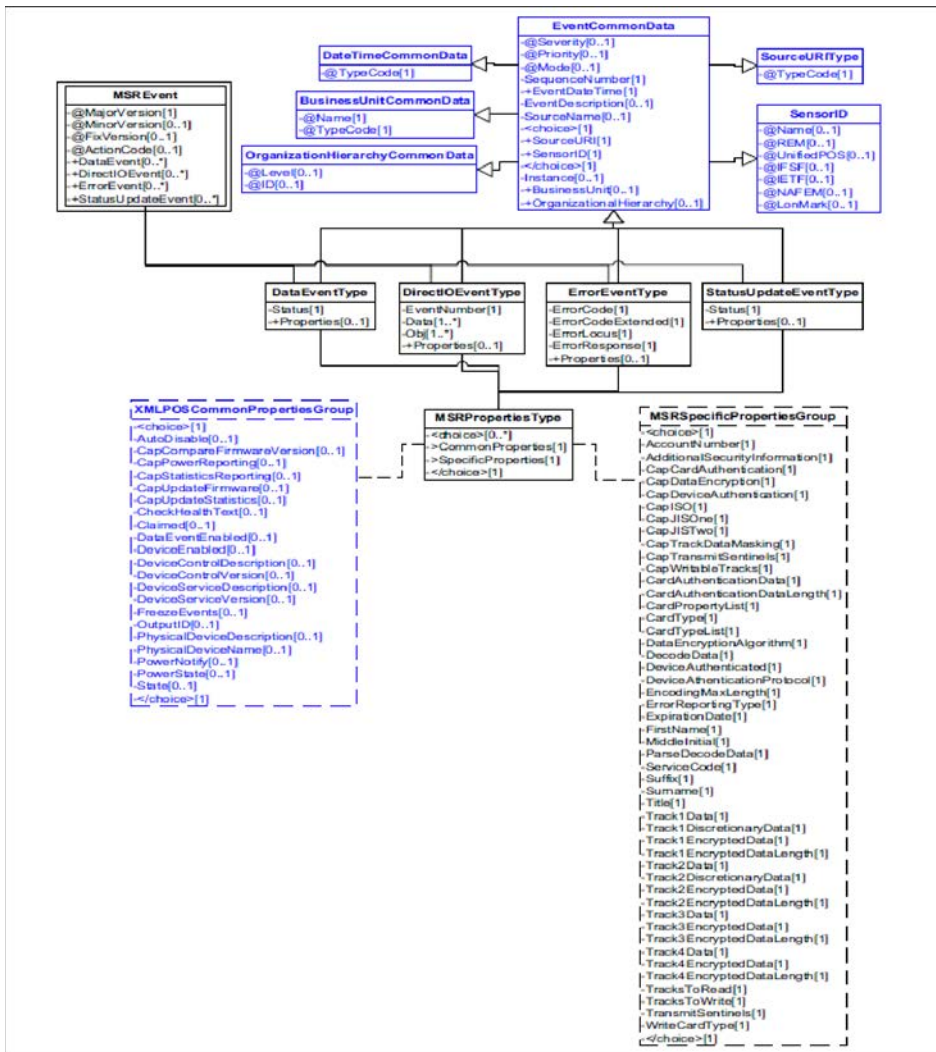
Figure 106: MSR Events Domain View
