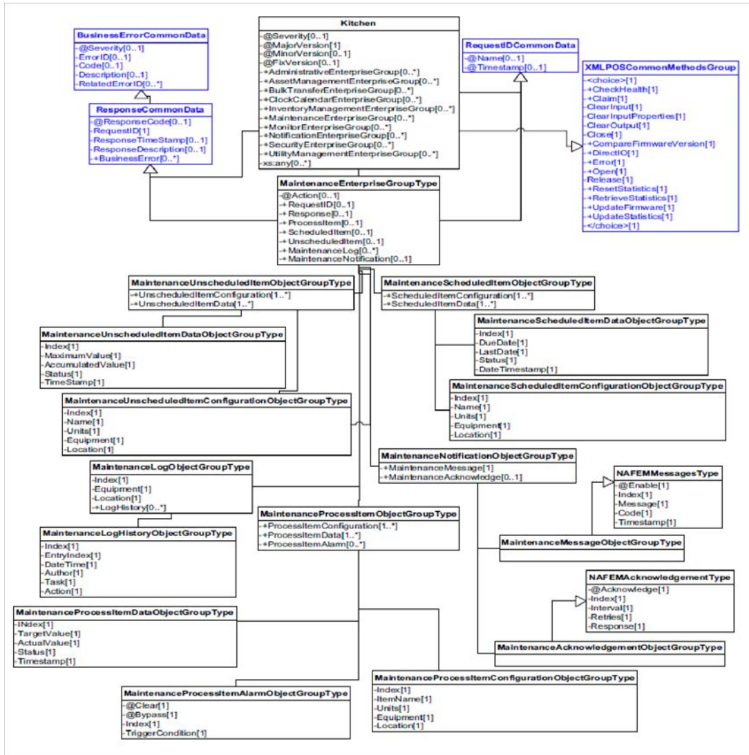
Figure 160: Maintenance Enterprise Group Domain View
