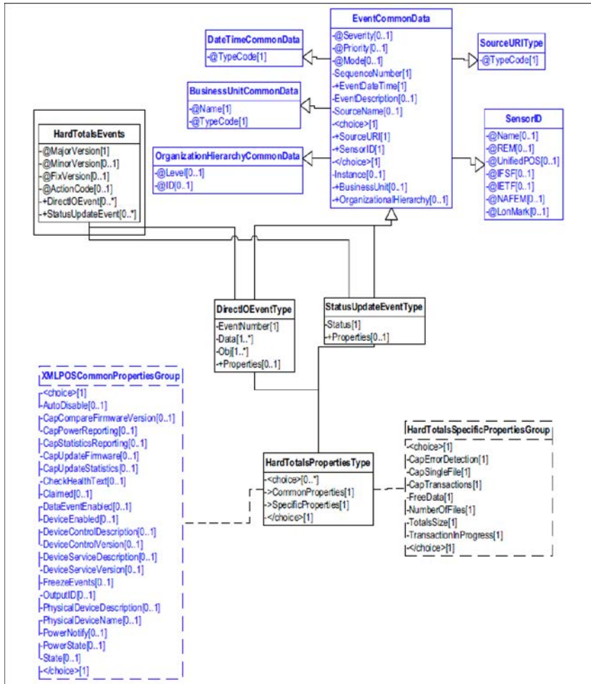
Figure 74: Hard Totals Events Domain View
