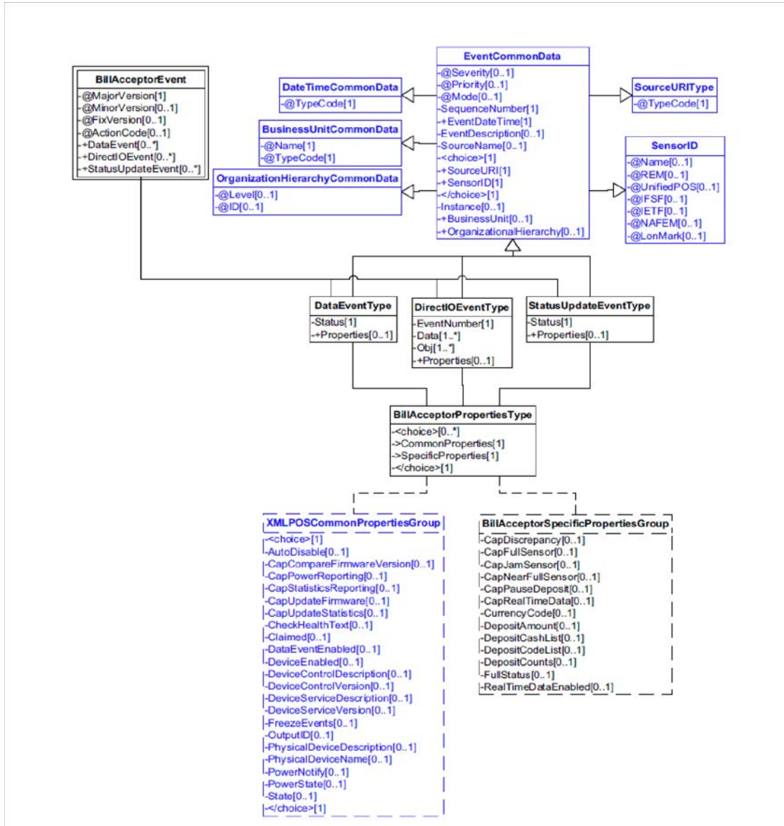
Figure 18: Bill Acceptor Events Domain View
