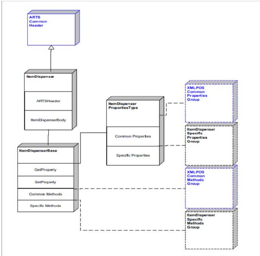
Figure 79: Item Dispenser Domain View
