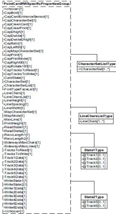
Figure 112: Point Card RW Properties Domain View
