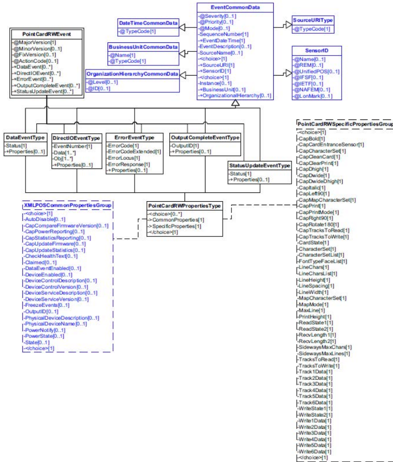
Figure 114: Point Card RW Events Domain View
