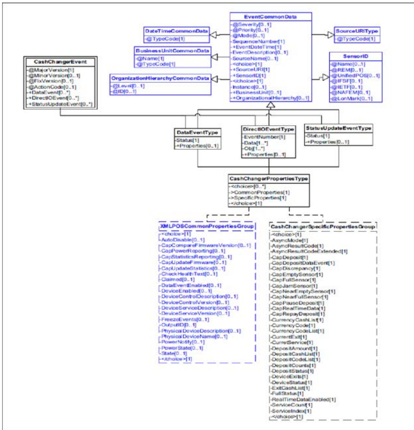
Figure 34: Cash Changer Events Domain View
