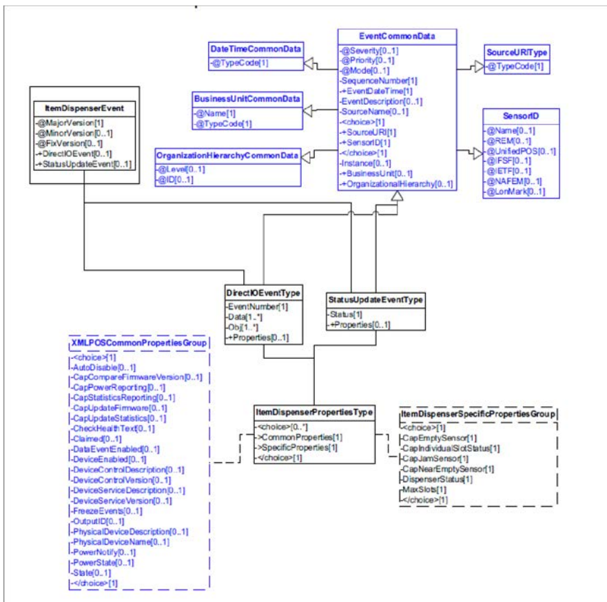
Figure 82: Item Dispenser Events Domain View
