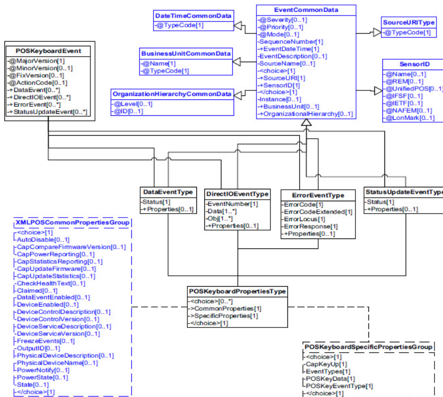
Figure 118: POS Keyboard Events Domain View
