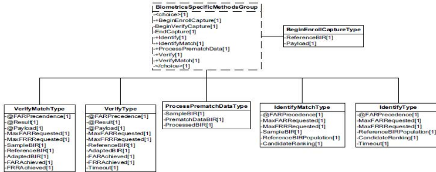
Figure 25: Biometric Methods Domain View
