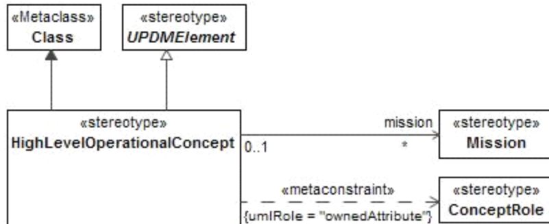
Figure 8.55 - HighLevelOperationalConcept
