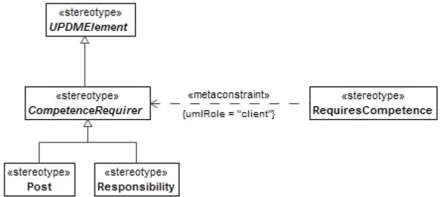
Figure 8.75 - CompetenceRequirer
