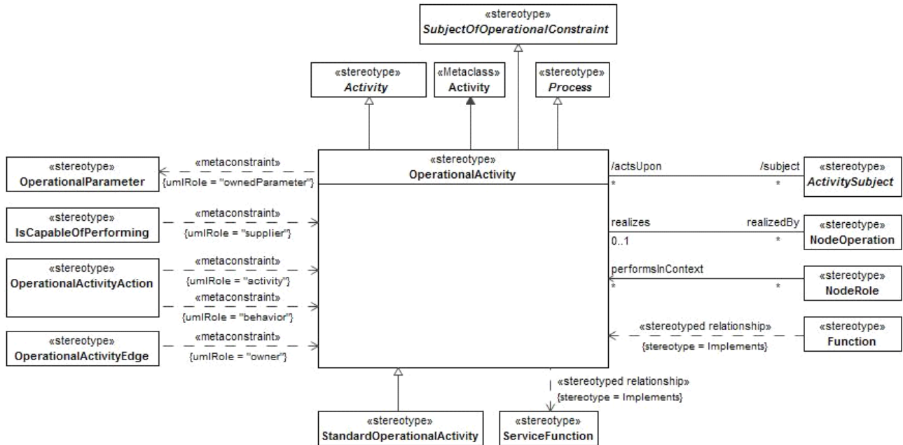
Figure 8.38 - OperationalActivity
