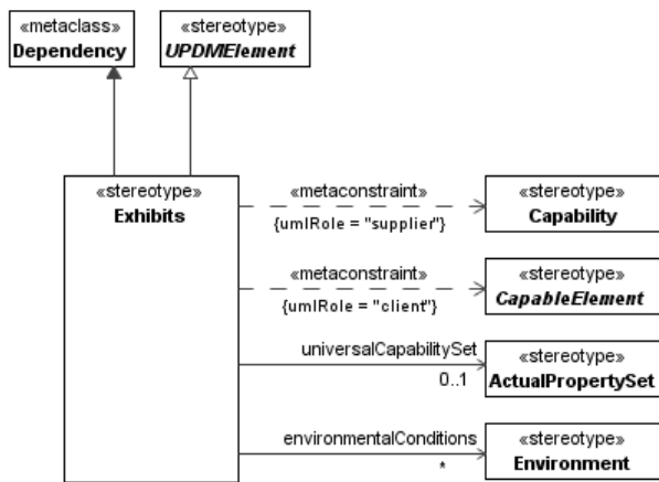
Figure 7.6 - “Exhibits” extends the UML Dependency metaclass
