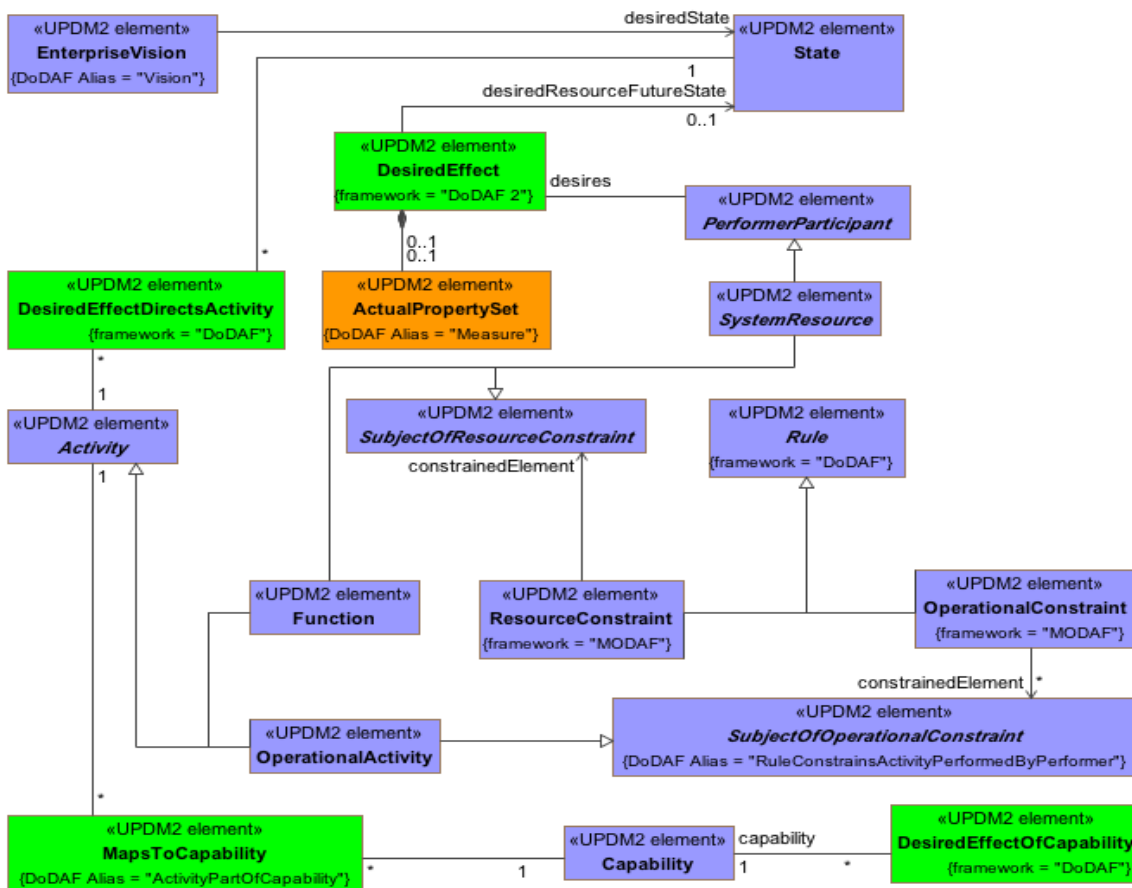
Figure A.50 - Goals - DM2
