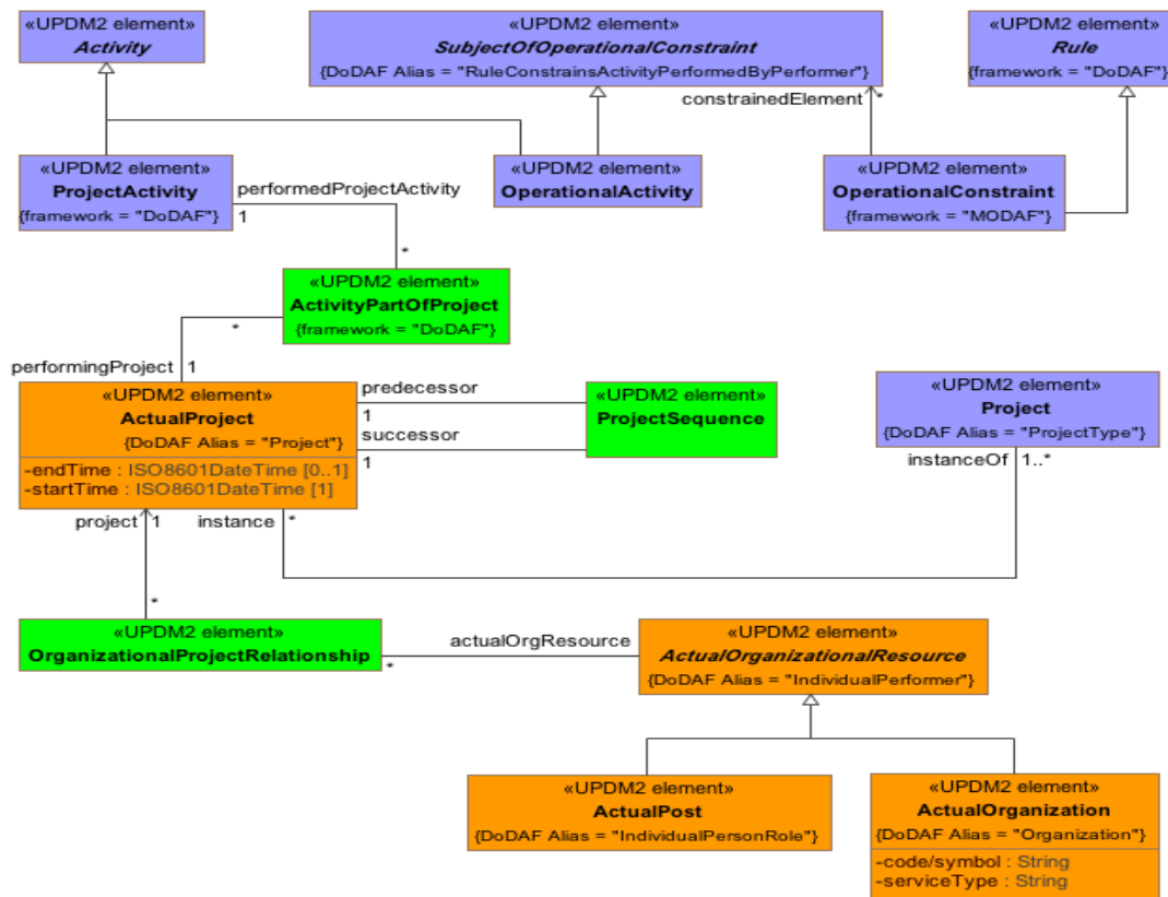
Figure A.57 - Project - DM2
