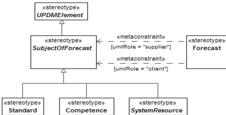
Figure 8.139 - SubjectOfForecast
