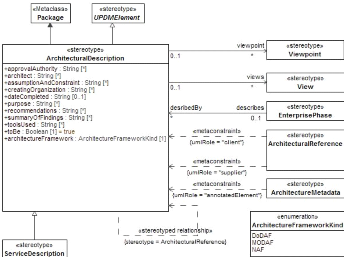
Figure 8.30 - ArchitecturalDescription
