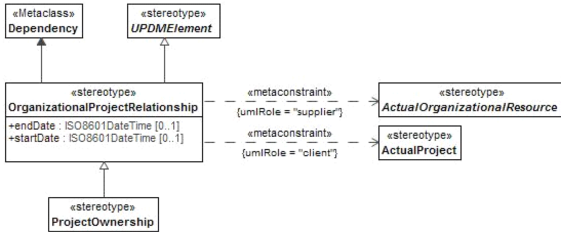
Figure 8.4 - OrganizationalProjectRelationship
