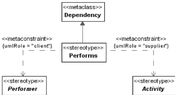
Figure 7.2 - Performs Hierarchy
