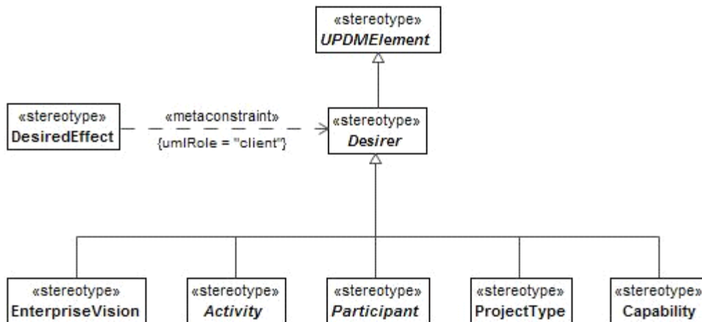
Figure 8.105 - Desirer
