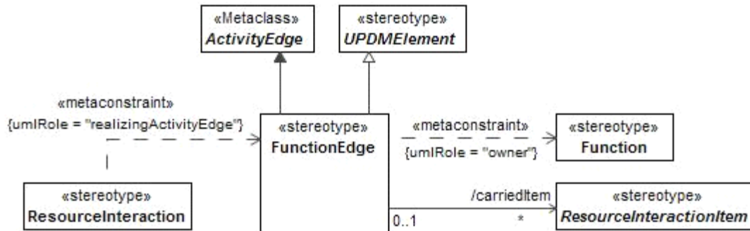
Figure 8.116 - FunctionEdge
