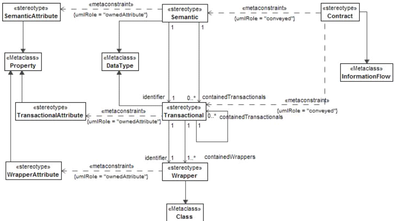
Figure 8.216 - SOPES Elements
