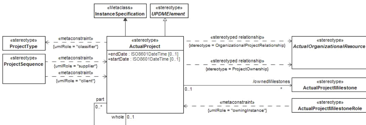
Figure 8.2 - ActualProject
