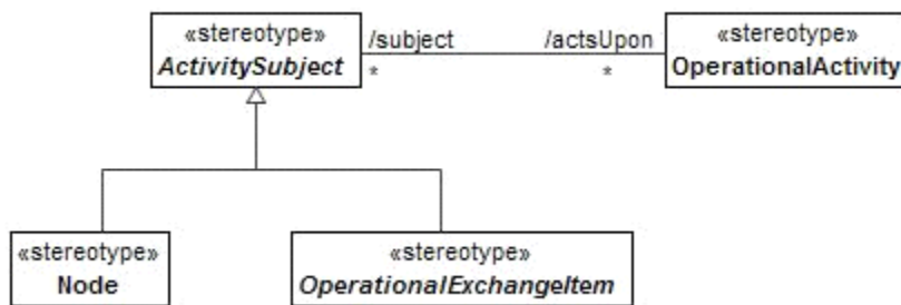
Figure 8.202 - ActivitySubject
