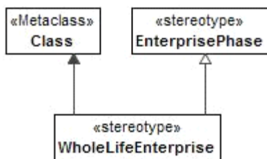
Figure 8.214 - WholeLifeEnterprise
