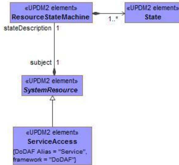
Figure A:33 - SV-10b/SvcV-10b DMM
