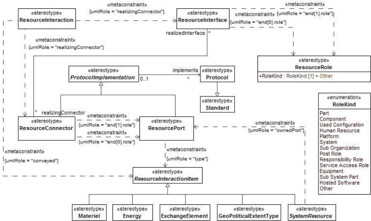
Figure B:39 - SV-2/SvcV-2
