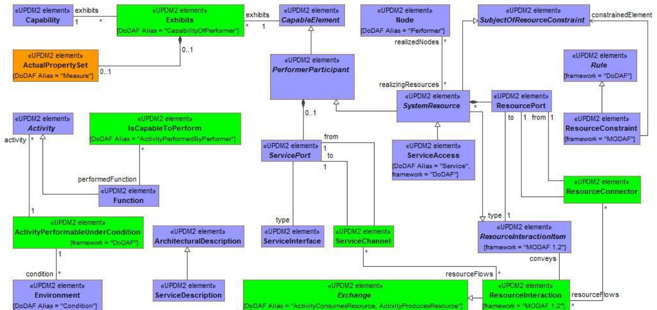
Figure A:60 - Services - DM2
