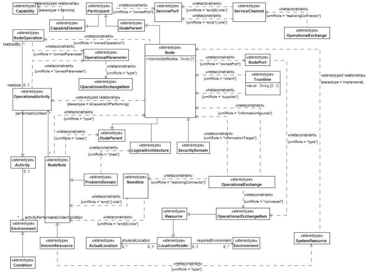
Figure B:10 - OV-2
