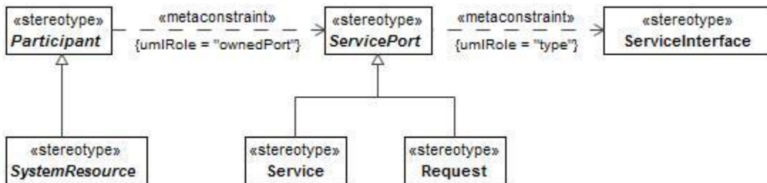
Figure B:38 - SV-12
