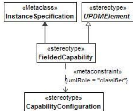
Figure 8:128 - FieldedCapability
