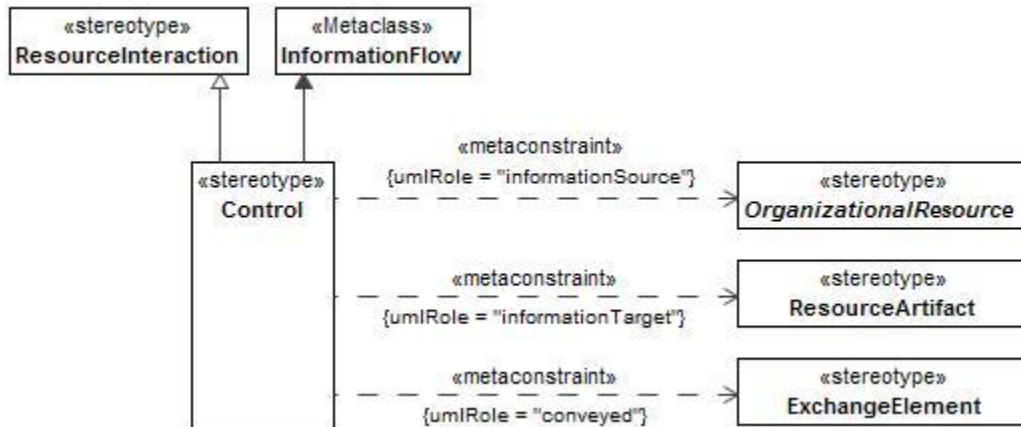
Figure 8:206 - Control
