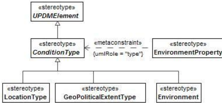
Figure 8:14 - ConditionType
