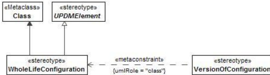
Figure 8:143 - WholeLifeConfiguration
