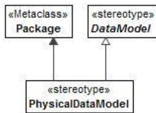
Figure 8:124 - PhysicalDataModel
