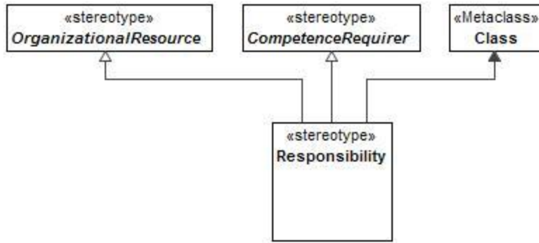
Figure 8:82 - Responsibility
