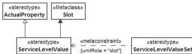
Figure 8:98 - ServiceLevelValue
