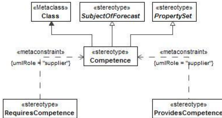
Figure 8:52 - Competence
