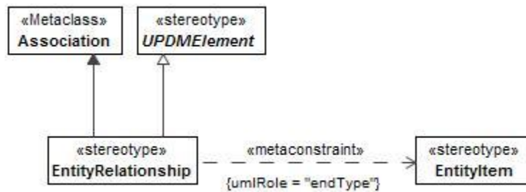
Figure 8:151 - EntityRelationship
