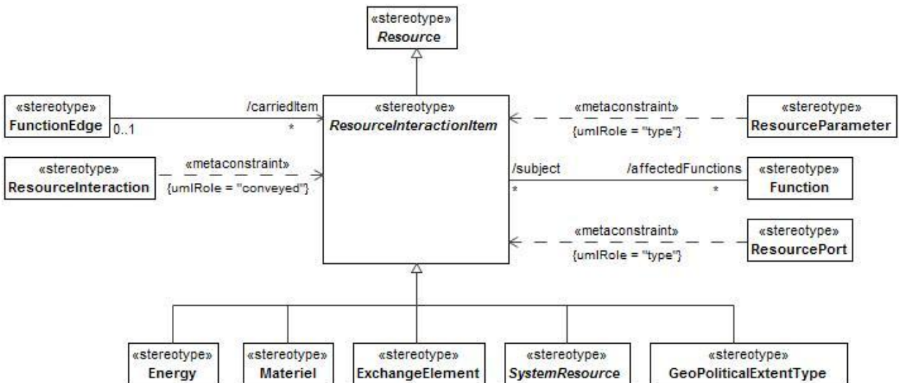
Figure 8:126 - ResourceInteractionItem
