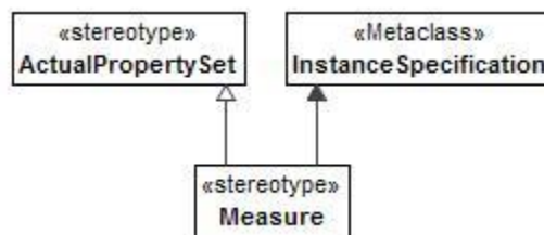
Figure 8:164 - Measure
