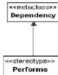
Figure 7:1 - Performs Stereotype
