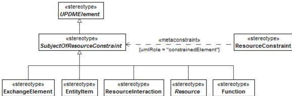
Figure 8:140 - SubjectOfResourceConstraint
