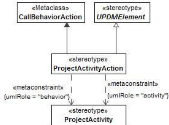
Figure 8:155 - ProjectActivityAction
