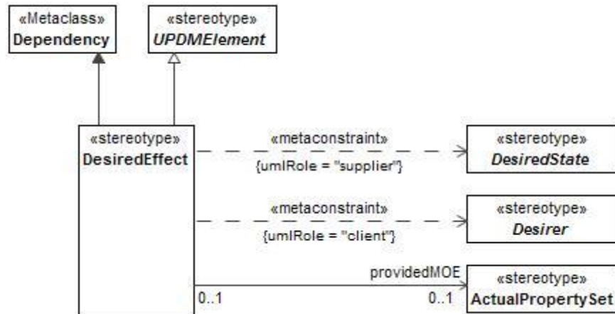
Figure 8:176 - DesiredEffect
