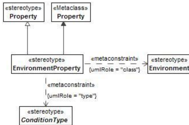
Figure 8:16 - EnvironmentProperty
