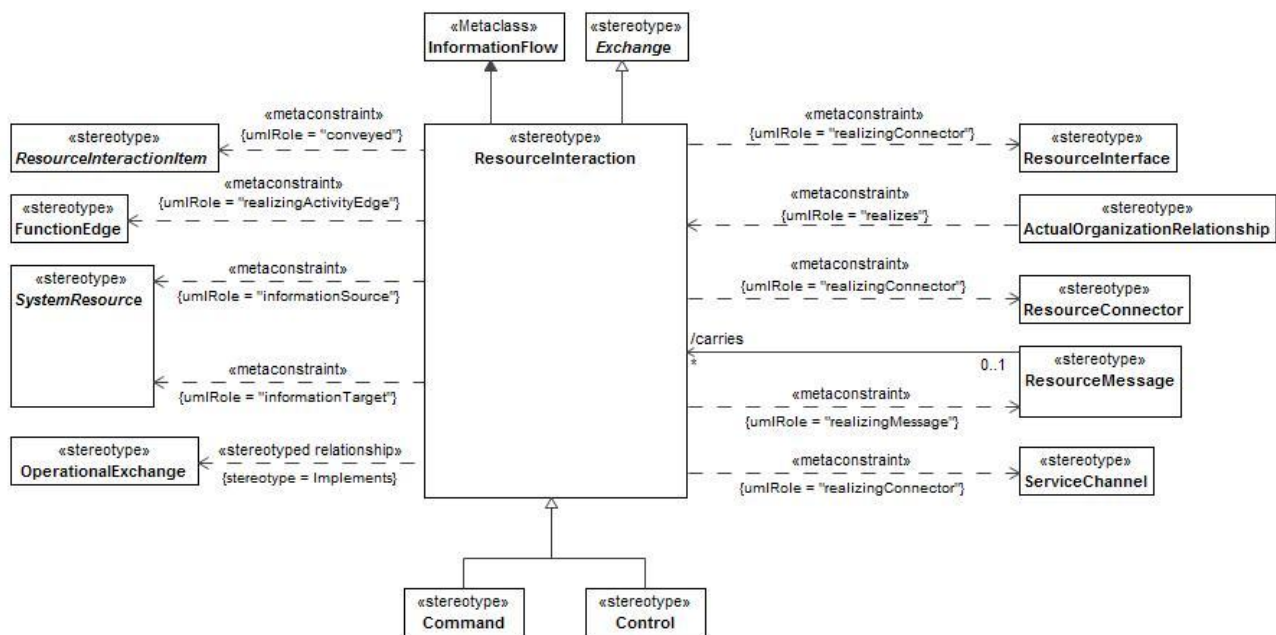
Figure 8:125 - ResourceInteraction
