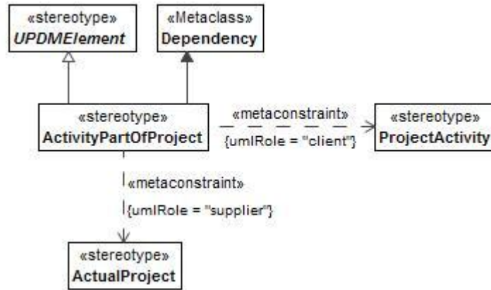
Figure 8:152 - ActivityPartOfProject
