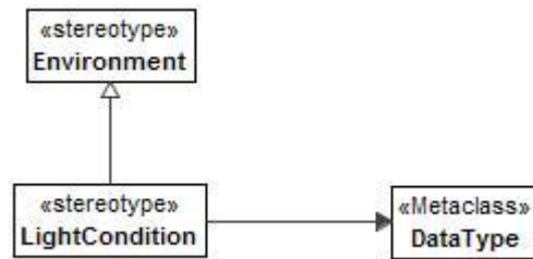
Figure 8:194 - LightCondition
