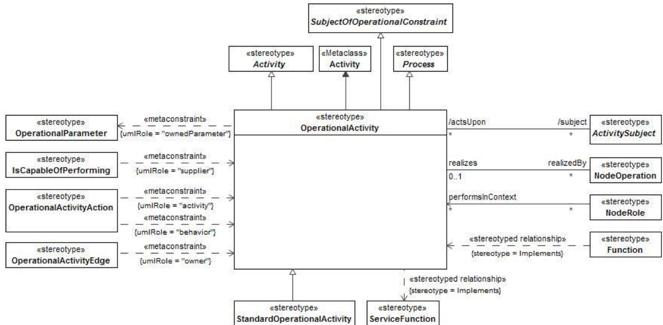
Figure 8:38 - OperationalActivity
