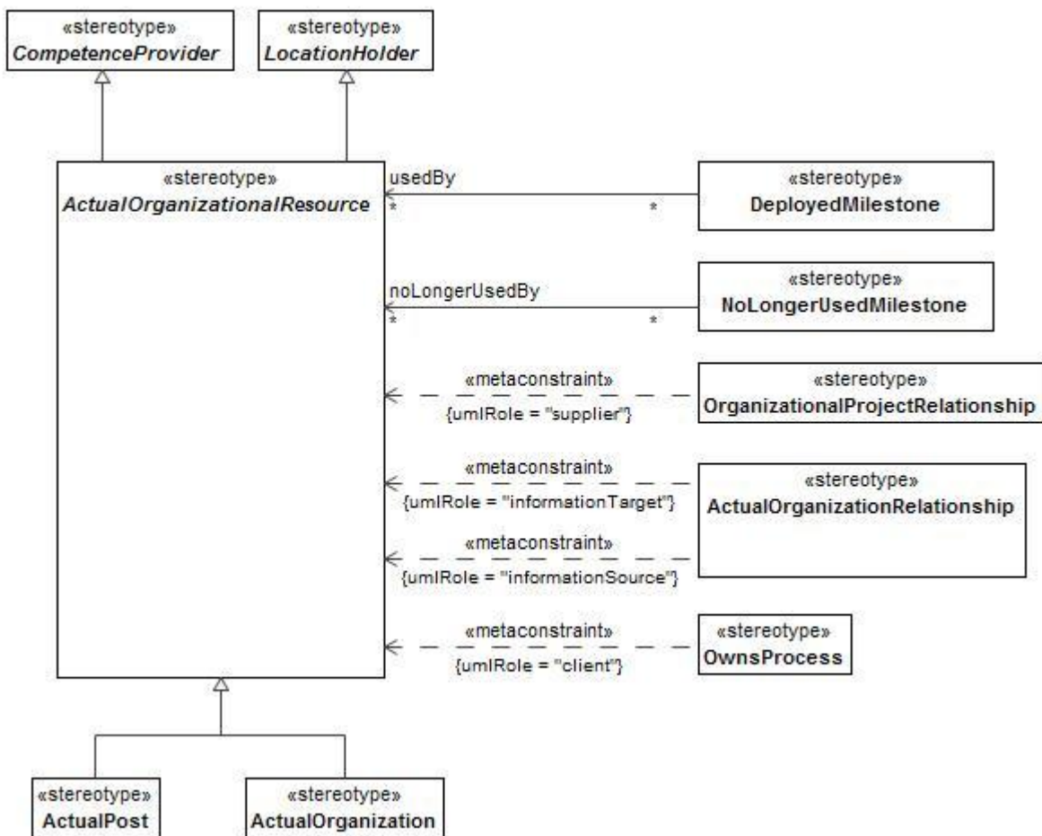
Figure 8:68 - ActualOrganizationalResource
