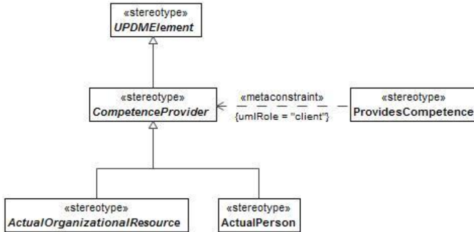
Figure 8:73 - CompetenceProvider
