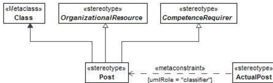
Figure 8:79 - Post
