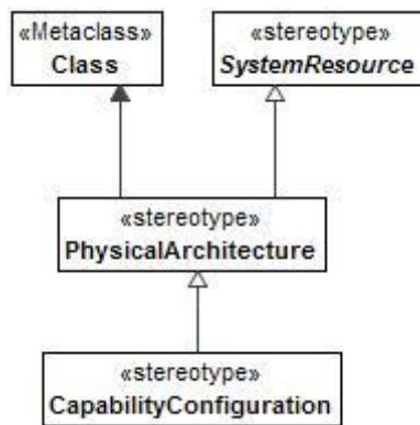
Figure 8:130 - PhysicalArchitecture
