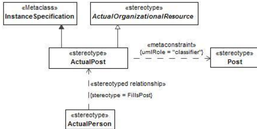
Figure 8:72 - ActualPost
