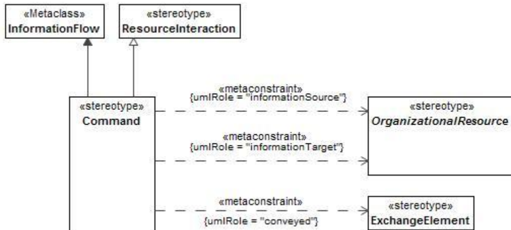
Figure 8:48 - Command
