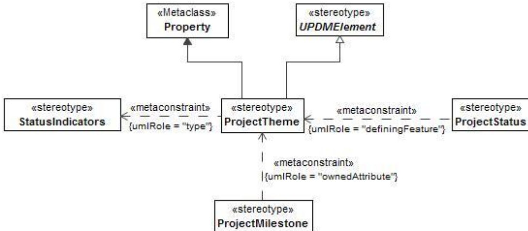
Figure 8:191 - ProjectTheme
