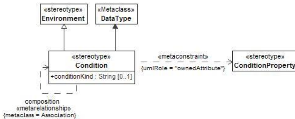
Figure 8:159 - Condition
