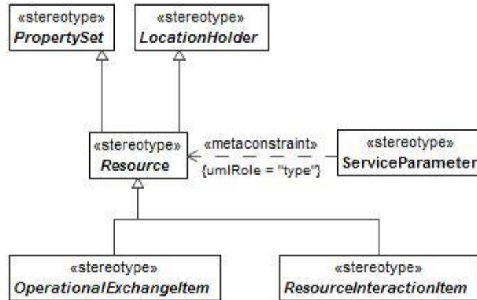
Figure 8:28 - Resource
