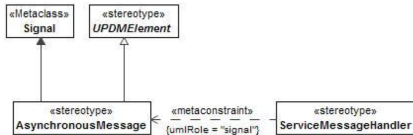
Figure 8:93 - AsynchronousMessage
