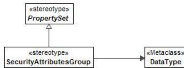
Figure 8:182 - SecurityAttributesGroup
