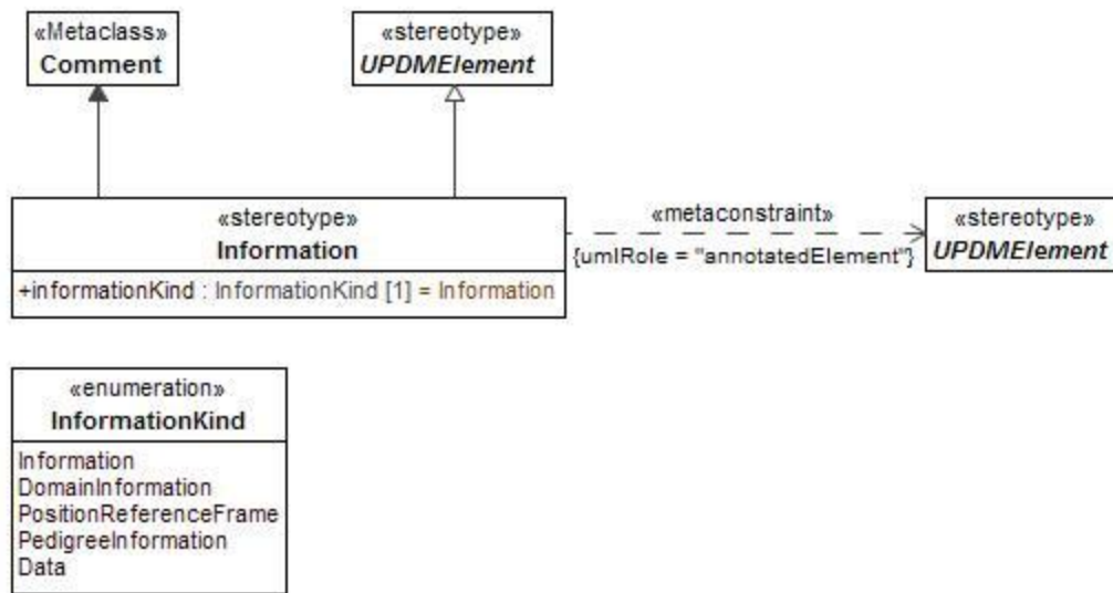
Figure 8:157 - Information
