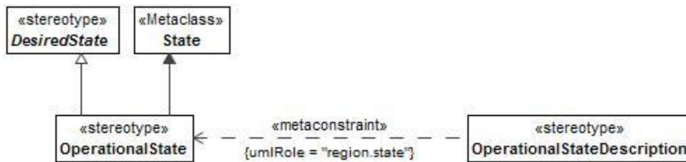
Figure 8:44 - OperationalState
