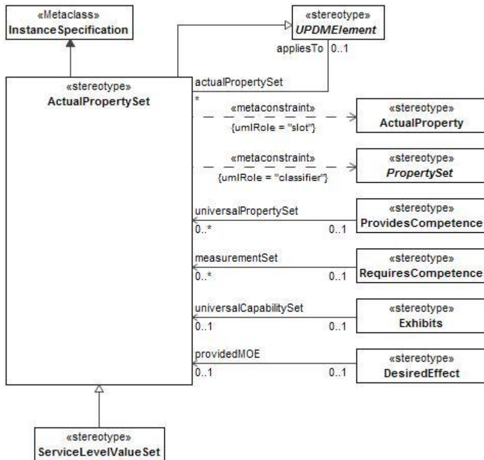
Figure 8:21 - ActualPropertySet
