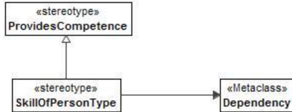
Figure 8:171 - SkillOfPersonType
