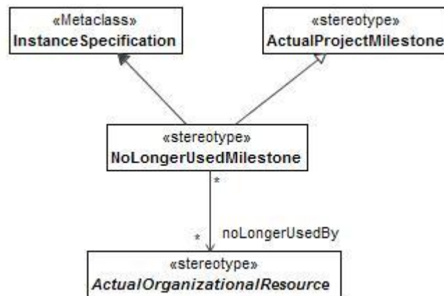
Figure 8:212 - NoLongerUsedMilestone
