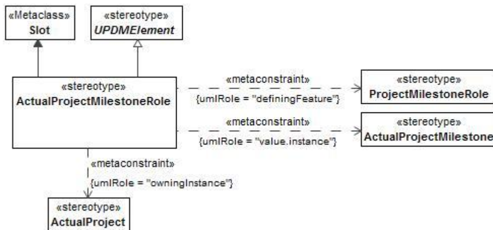
Figure 8:3 - ActualProjectMilestoneRole
