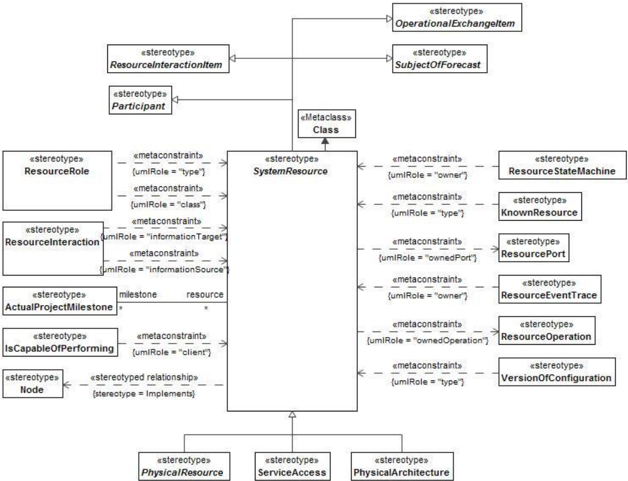
Figure 8:141 - SystemResource
