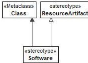
Figure 8:138 - Software
