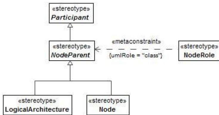
Figure 8:61 - NodeParent
