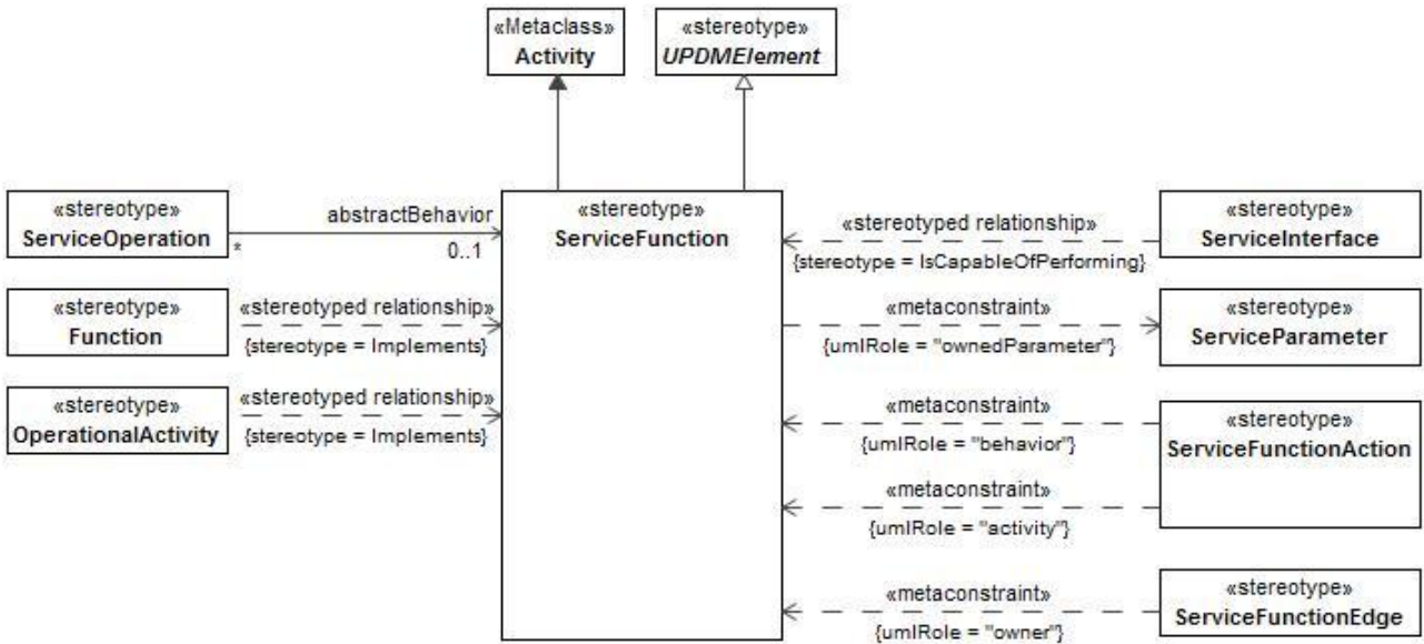
Figure 8:84 - ServiceFunction
