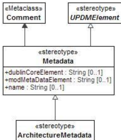
Figure 8:33 - Metadata
