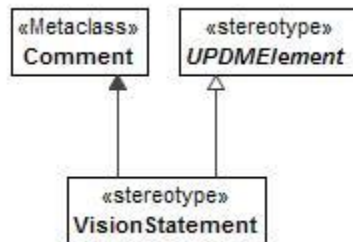
Figure 8:113 - VisionStatement
