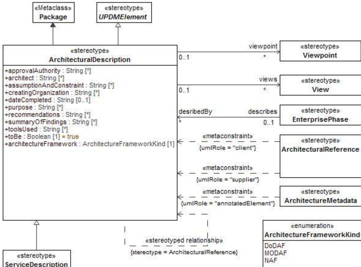
Figure 8:30 - ArchitecturalDescription
