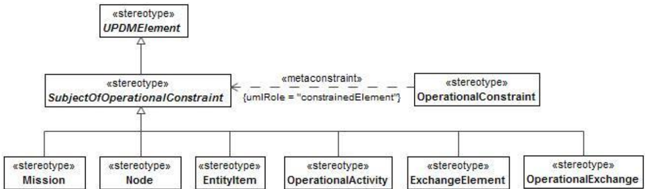
Figure 8:66 - SubjectOfOperationalConstraint
