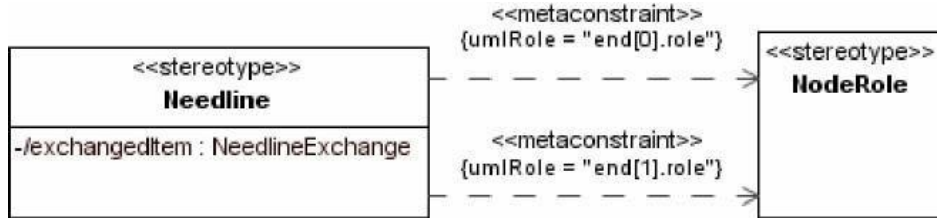
Figure 7:3 - Connector Extension
