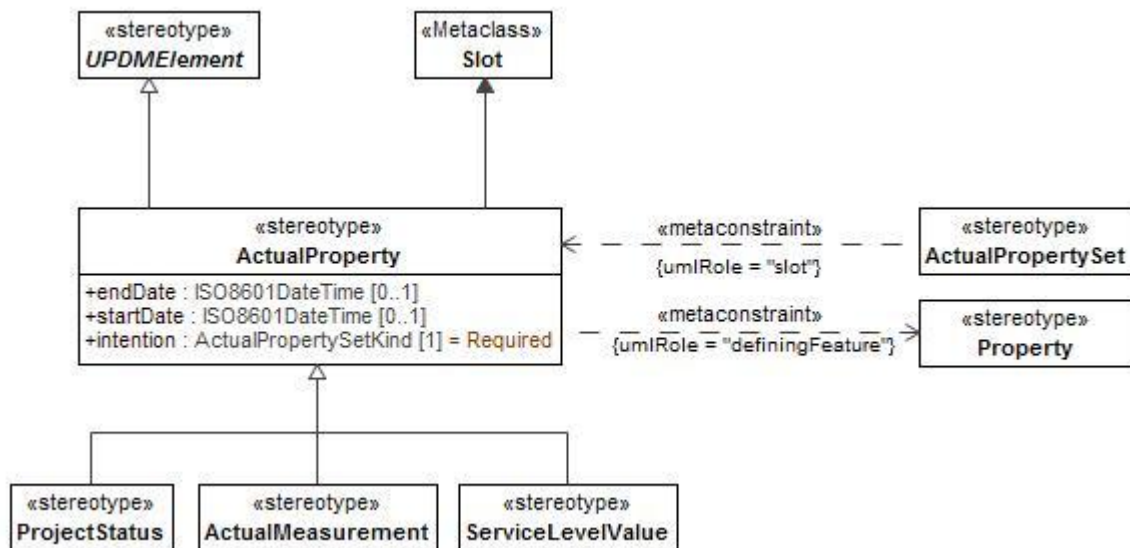
Figure 8:20 - ActualProperty
