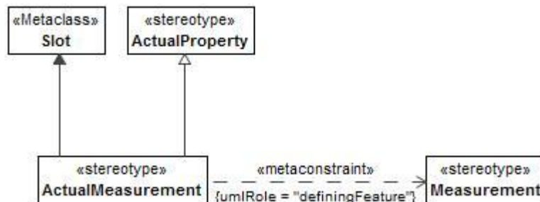
Figure 8:19 - ActualMeasurement
