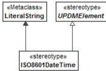
Figure 8:36 - ISO8601DateTime
