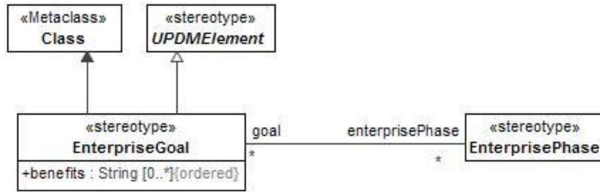
Figure 8:106 - EnterpriseGoal
