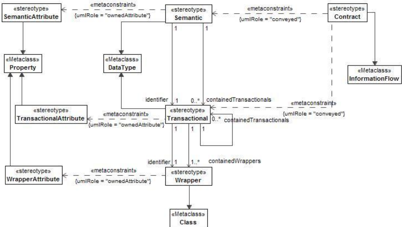
Figure 8:216 - SOPES Elements
