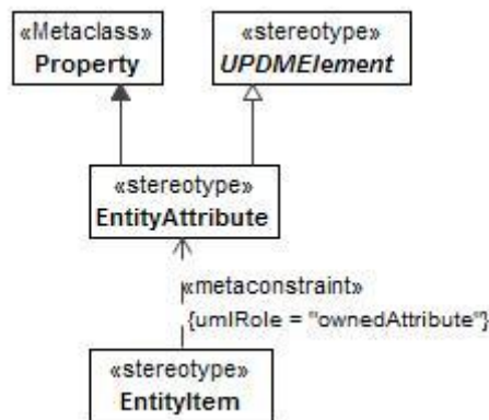
Figure 8:149 - EntityAttribute
