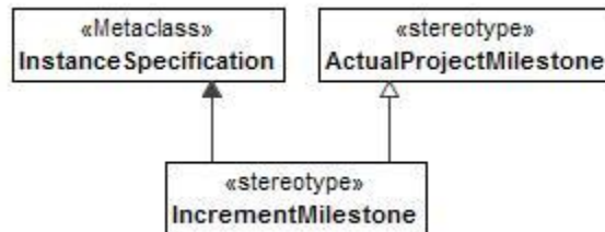
Figure 8:184 - IncrementMilestone
