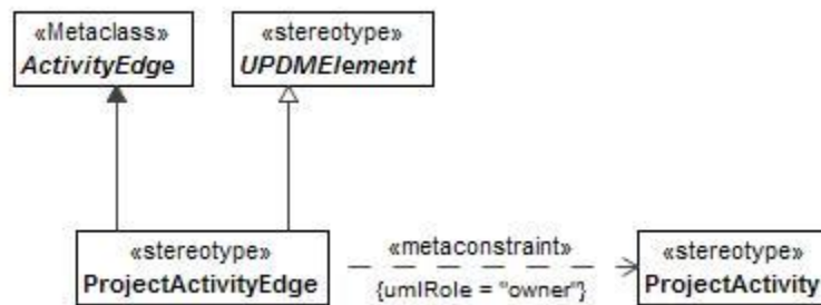
Figure 8:156 - ProjectActivityEdge
