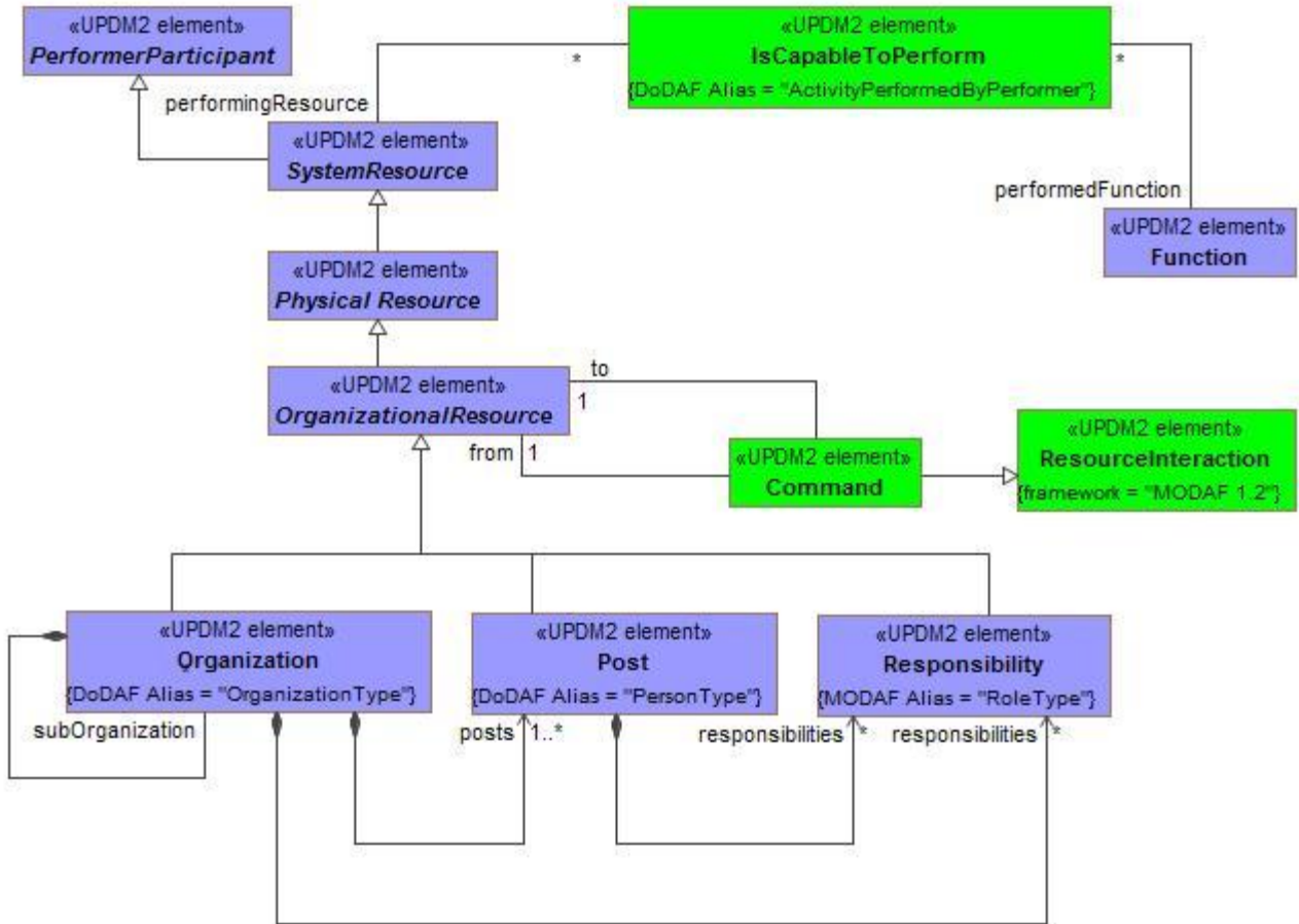
Figure A:11 - OV-4 Typical - DMM
