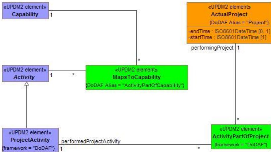
Figure A:3 - PV-3 Derived from Project Activity - DMM
