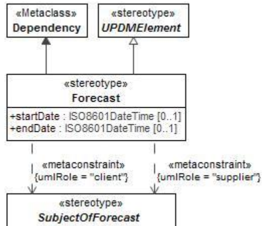
Figure 8:129 - Forecast
