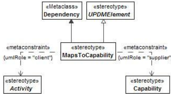
Figure 8:110 - MapsToCapability
