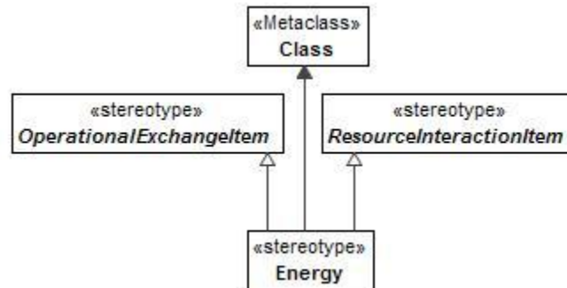
Figure 8:207 - Energy
