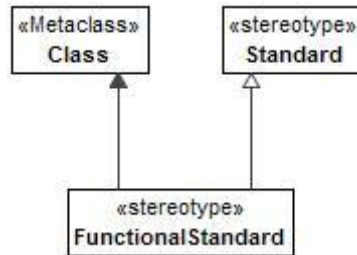
Figure 8:179 - FunctionalStandard
