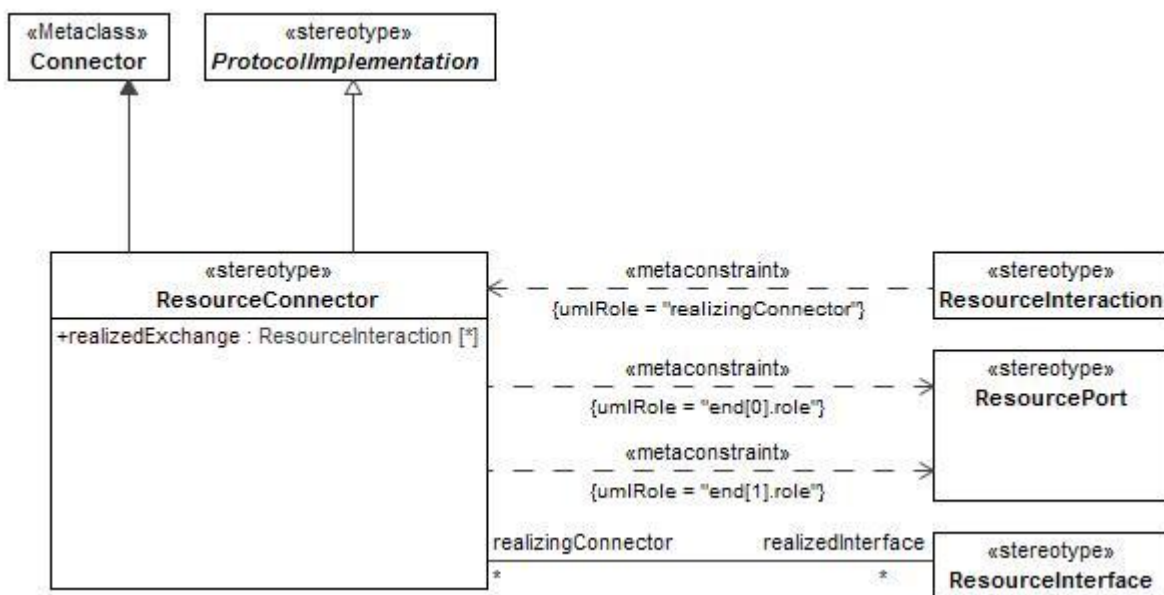
Figure 8:133 - ResourceConnector
