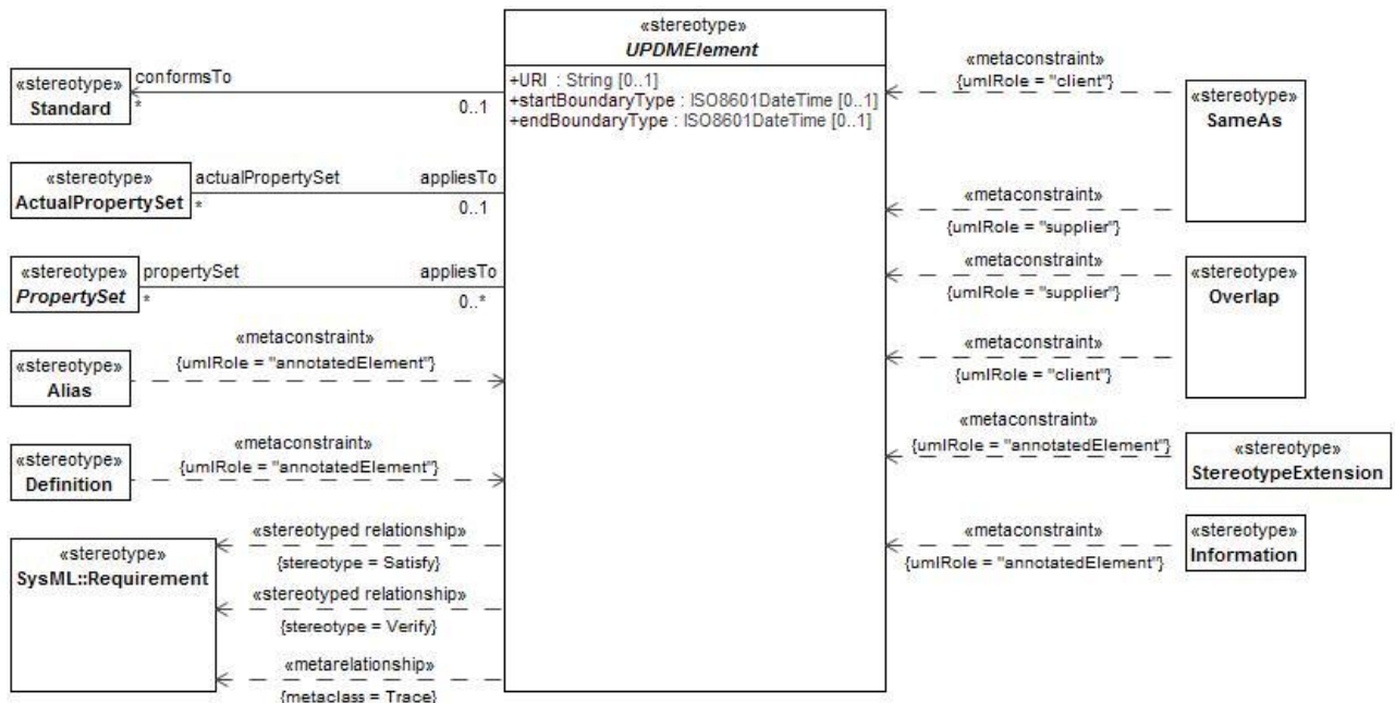
Figure 8:8 - UPDMElement
