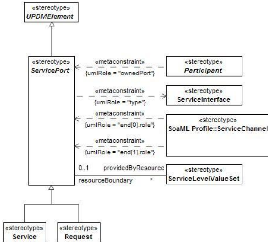
Figure 8:101 - ServicePort
