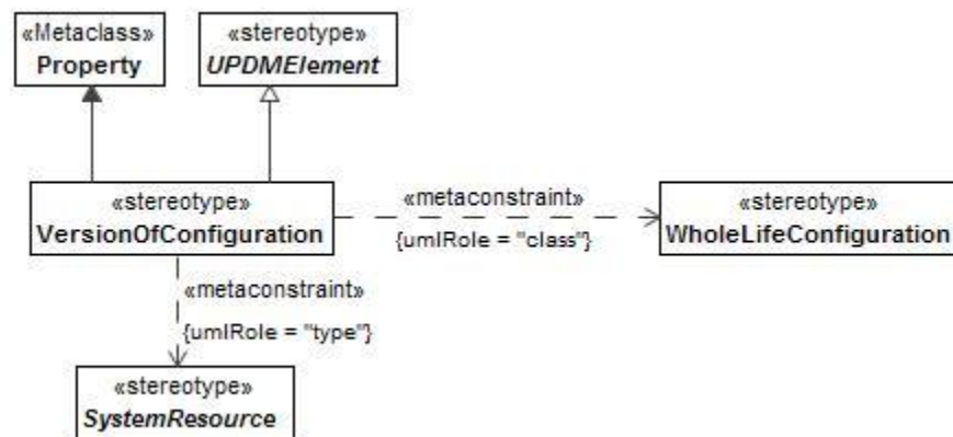
Figure 8:142 - VersionOfConfiguration
