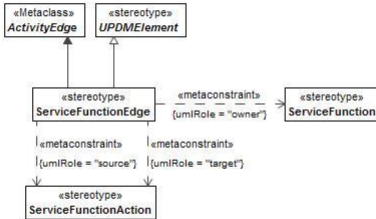
Figure 8:86 - ServiceFunctionEdge
