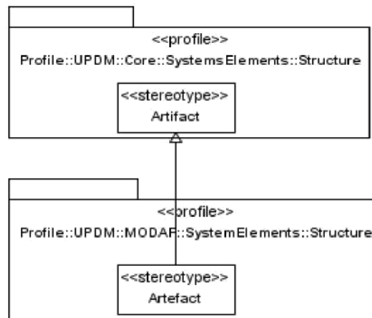
Figure 7:8 - Aliases
