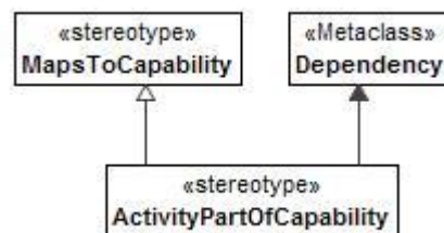
Figure 8:174 - ActivityPartOfCapability
