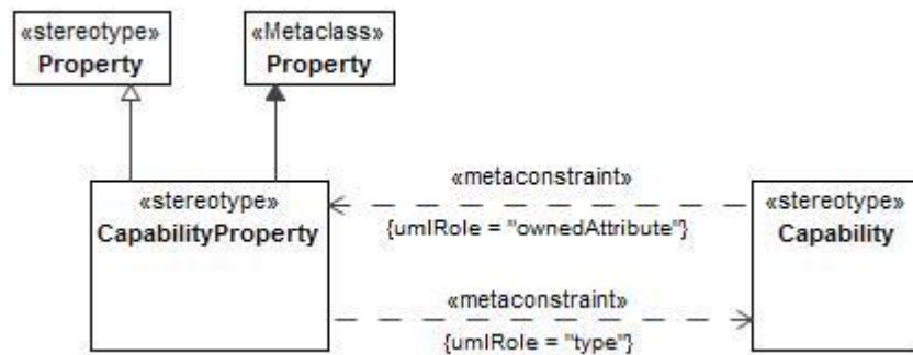
Figure 8:103 - CapabilityProperty
