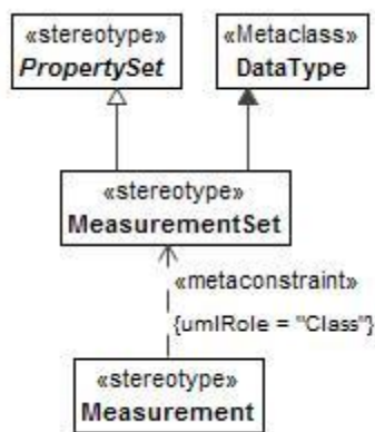
Figure 8:23 - MeasurementSet
