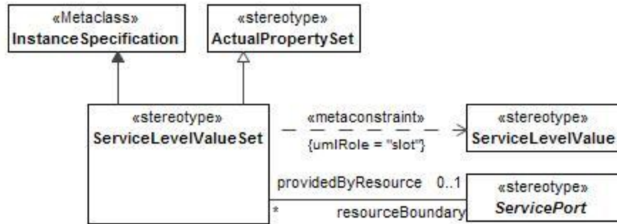
Figure 8:99 - ServiceLevelValueSet
