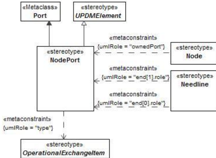
Figure 8:62 - NodePort
