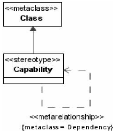
Figure 7:5 - Visualizing <metarelationship>
