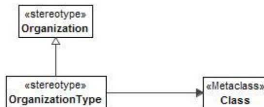
Figure 8:168 - OrganizationType
