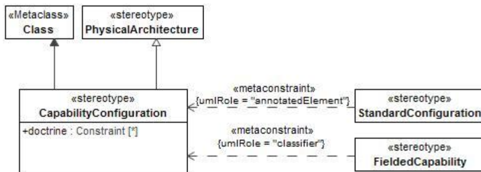
Figure 8:127 - CapabilityConfiguration
