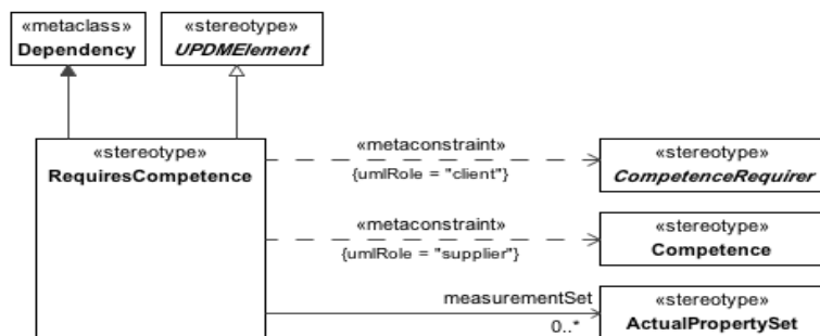
Figure 8.84 - RequiresCompetence
