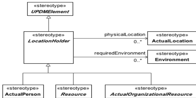
Figure 8.15 - LocationHolder
