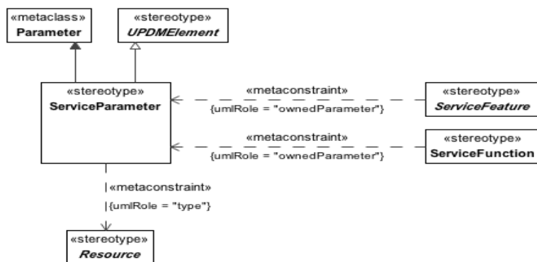
Figure 8.94 - ServiceParameter
