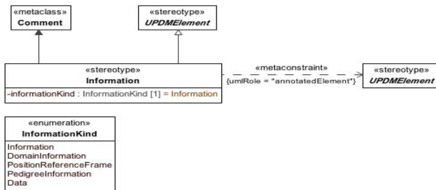
Figure 8.155 - Information
