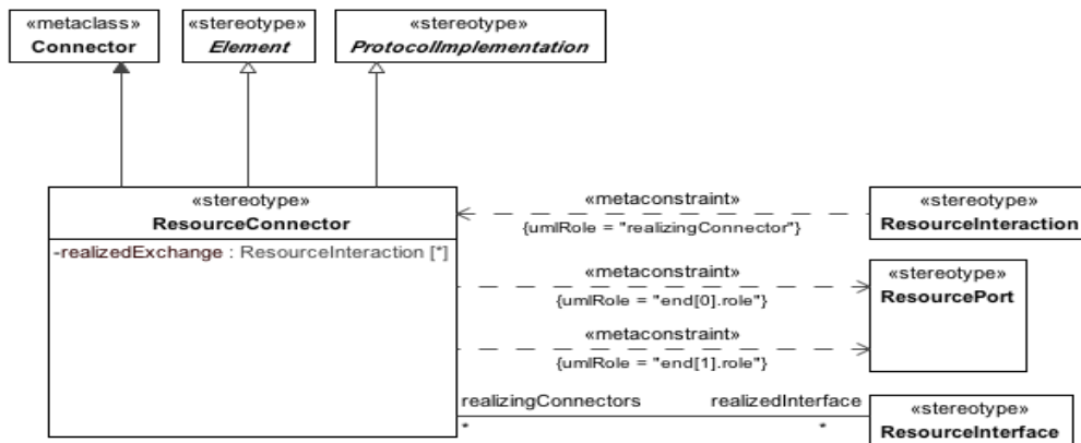
Figure 8.134 - ResourceConnector
