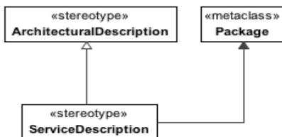
Figure 8.185 - ServiceDescription
