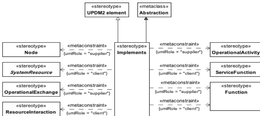
Figure 8.12 - Implements
