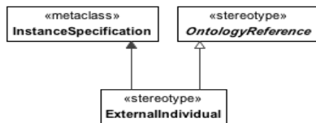
Figure 8.200 - ExternalIndividual
