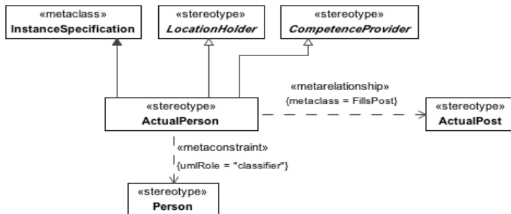
Figure 8.74 - ActualPerson
