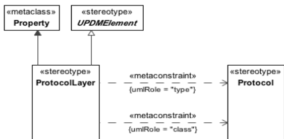
Figure 8.218 - ProtocolLayer
