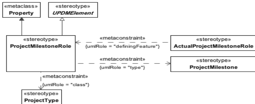
Figure 8.7 - ProjectMilestoneRole
