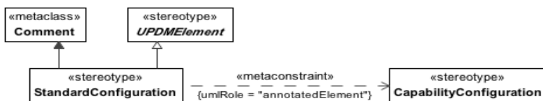
Figure 8.148 - StandardConfiguration
