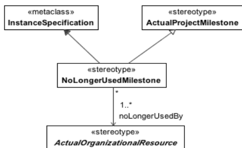
Figure 8.215 - NoLongerUsedMilestone
