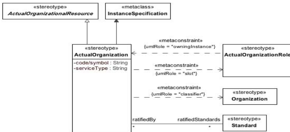
Figure 8.70 - ActualOrganization
