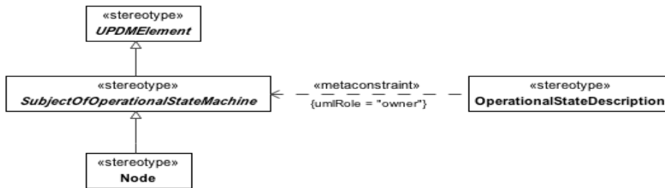
Figure 8.48 - SubjectOfOperationalStateMachine
