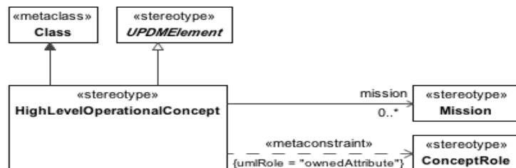
Figure 8.58 - HighLevelOperationalConcept
