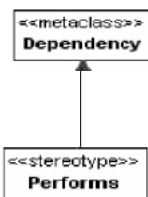
Figure 7.3 - Performs Stereotype
