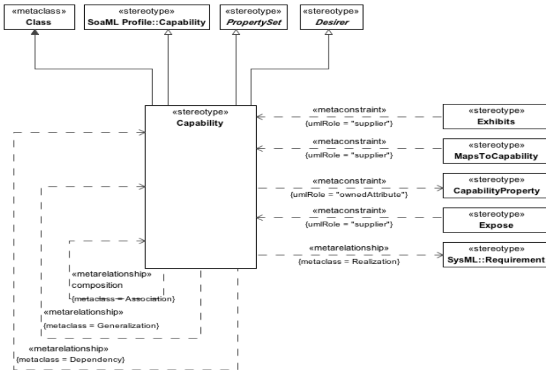
Figure 8.105 - Capability
