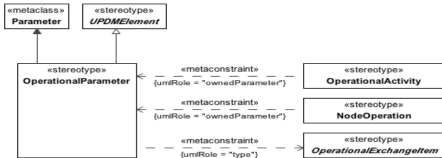
Figure 8.46 - OperationalParameter
