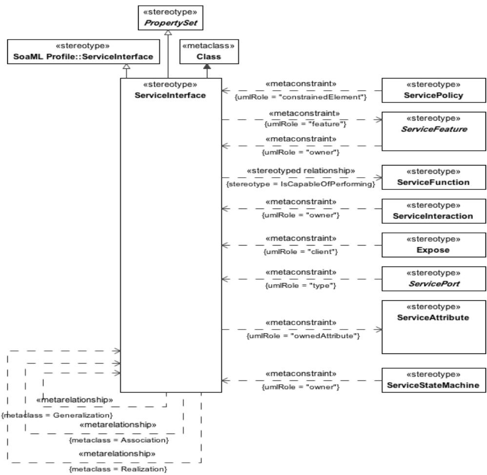
Figure 8.100 - ServiceInterface
