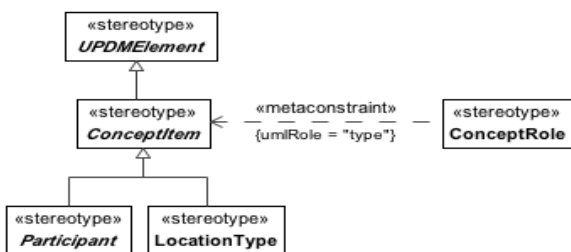
Figure 8.56 - ConceptItem
