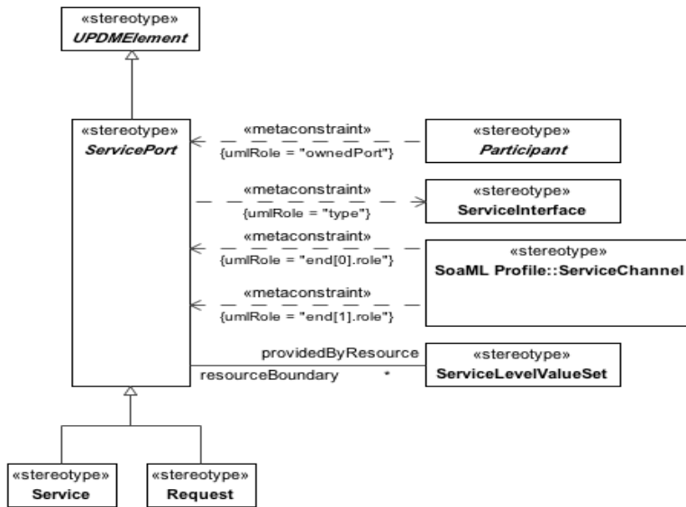
Figure 8.104 - ServicePort
