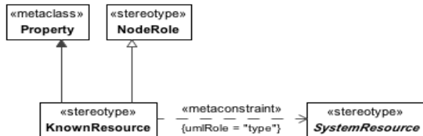
Figure 8.59 - KnownResource
