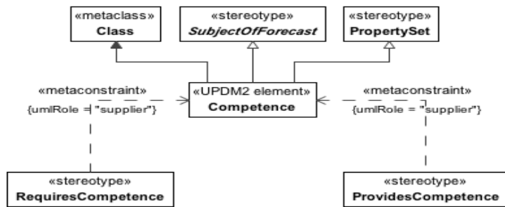
Figure 8.55 - Competence
