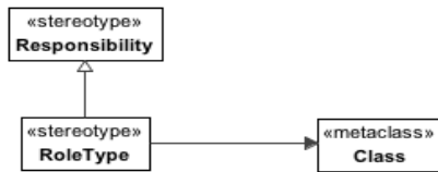
Figure 8.213 - RoleType
