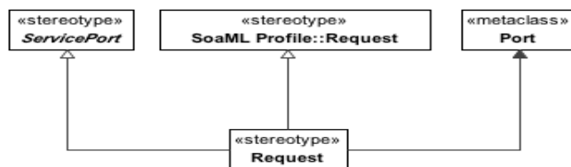
Figure 8.97 - Request
