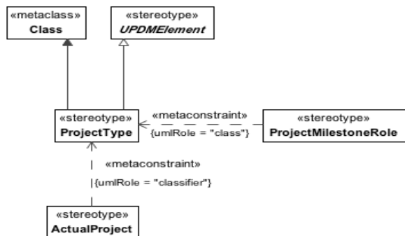
Figure 8.5 - ProjectType
