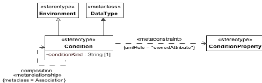
Figure 8.157 - Condition
