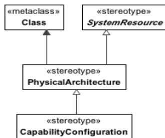
Figure 8.131 - PhysicalArchitecture
