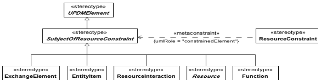
Figure 8.141 - SubjectOfResourceConstraint
