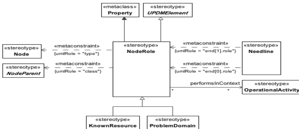
Figure 8.66 - NodeRole
