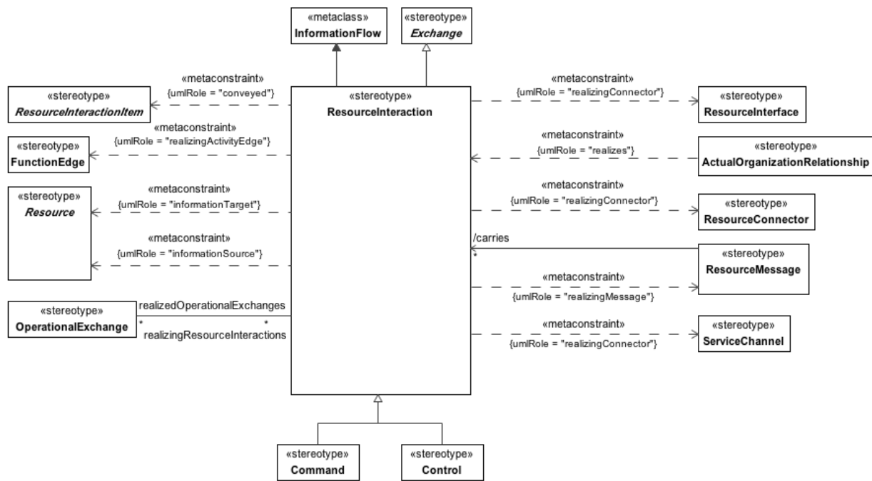
Figure 8.126 - ResourceInteraction
