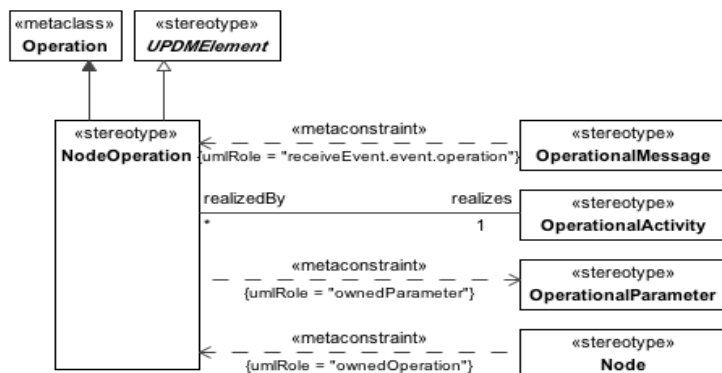
Figure 8.40 - NodeOperation
