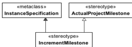
Figure 8.187 - IncrementMilestone
