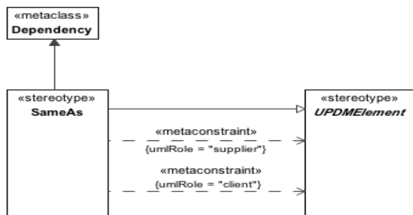
Figure 8.203 - SameAs
