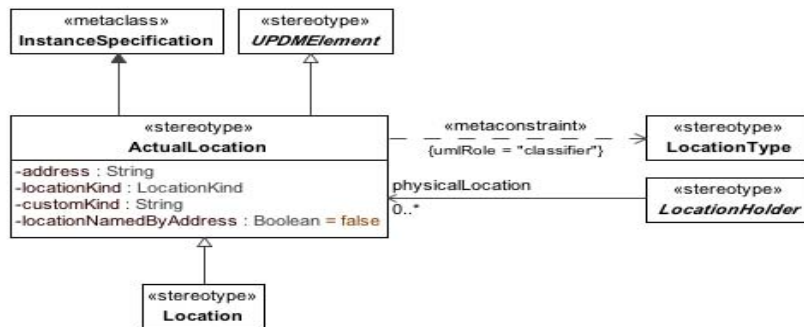
Figure 8.16 - ActualLocation
