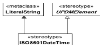
Figure 8.39 - ISO8601DateTime
