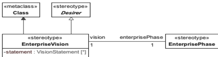
Figure 8.109 - EnterpriseVision
