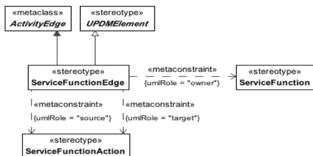
Figure 8.89 - ServiceFunctionEdge
