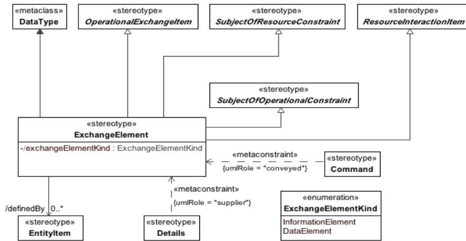
Figure 8.29 - ExchangeElement
