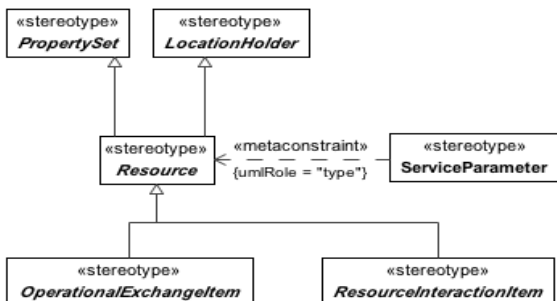
Figure 8.31 - Resource
