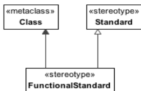
Figure 8.180 - FunctionalStandard
