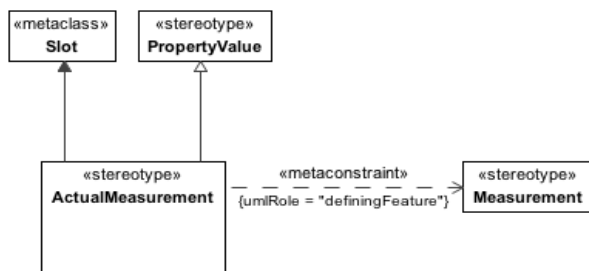
Figure 8.22 - ActualMeasurement
