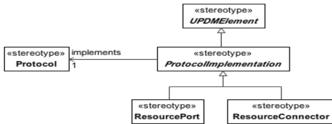
Figure 8.146 - ProtocolImplementation
