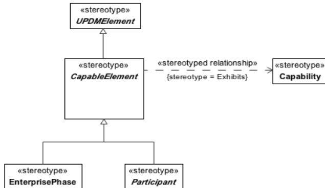
Figure 8.14 - CapableElement
