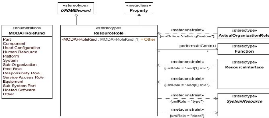
Figure 8.138 - ResourceRole
