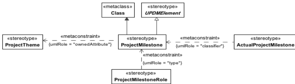
Figure 8.190 - ProjectMilestone
