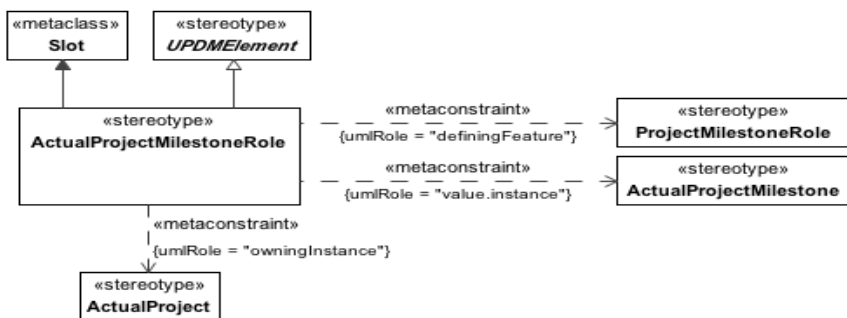
Figure 8.6 - ActualProjectMilestoneRole
