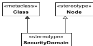
Figure 8.68 - SecurityDomain
