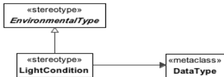
Figure 8.197 - LightCondition
