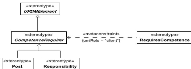
Figure 8.78 - CompetenceRequirer
