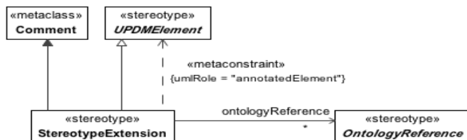
Figure 8.204 - StereotypeExtension
