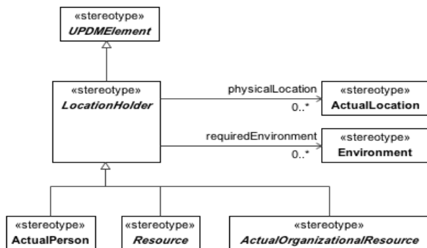
Figure 8.20 - LocationHolder
