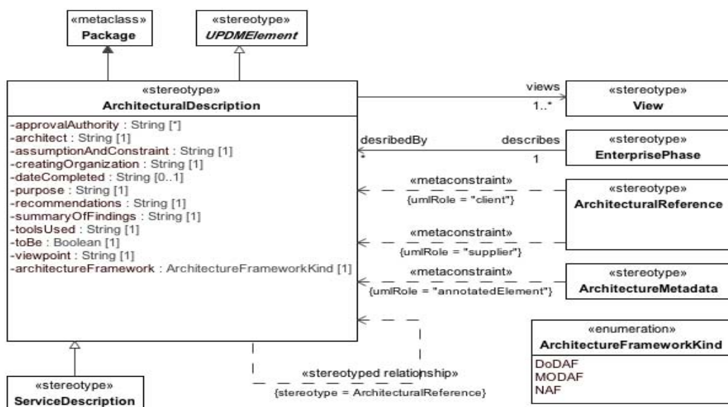
Figure 8.33 - ArchitecturalDescription
