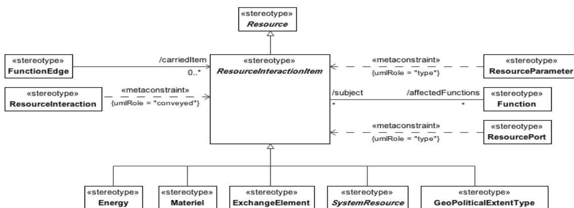
Figure 8.127 - ResourceInteractionItem
