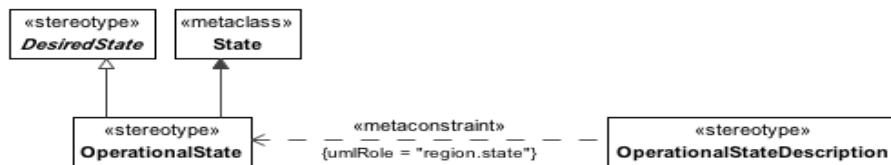
Figure 8.49 - OperationalState
