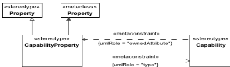
Figure 8.106 - CapabilityProperty
