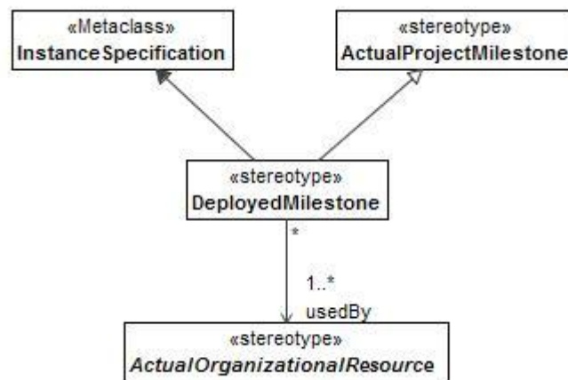
Figure 8:209 - DeployedMilestone
