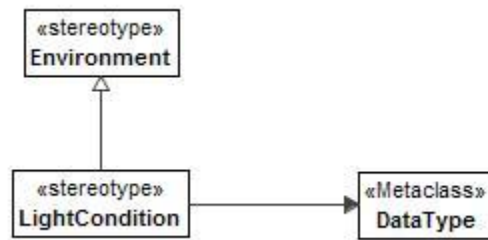
Figure 8:192 - LightCondition
