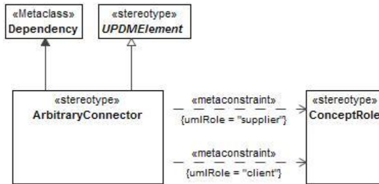
Figure 8:51 - ArbitraryConnector
