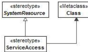
Figure 8:170 - ServiceAccess
