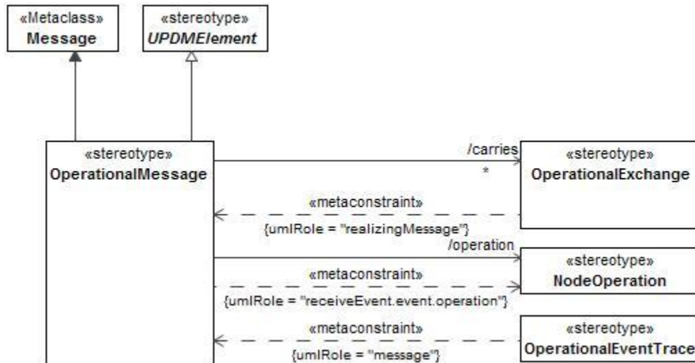
Figure 8:42 - OperationalMessage
