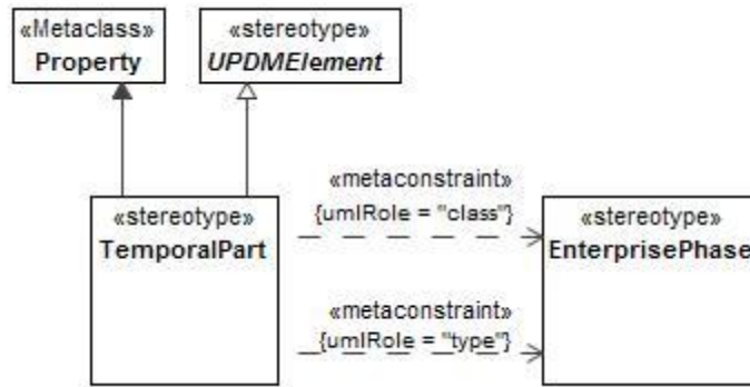
Figure 8:112 - TemporalPart
