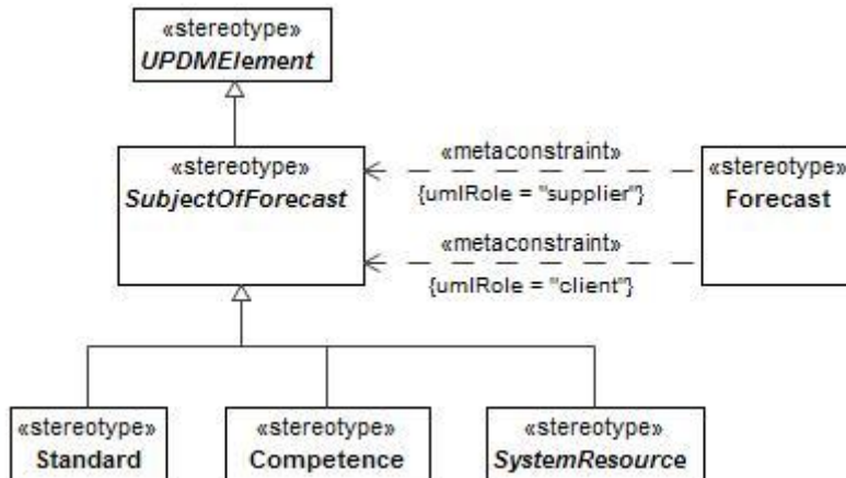
Figure 8:139 - SubjectOfForecast
