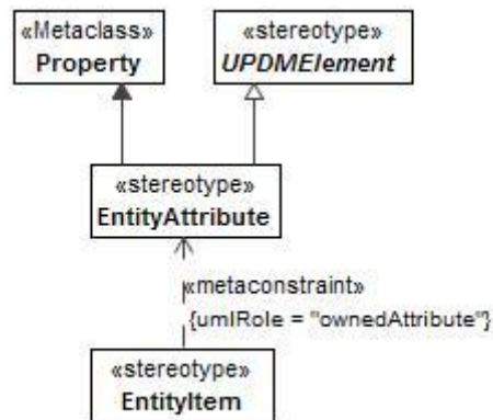
Figure 8:149 - EntityAttribute
