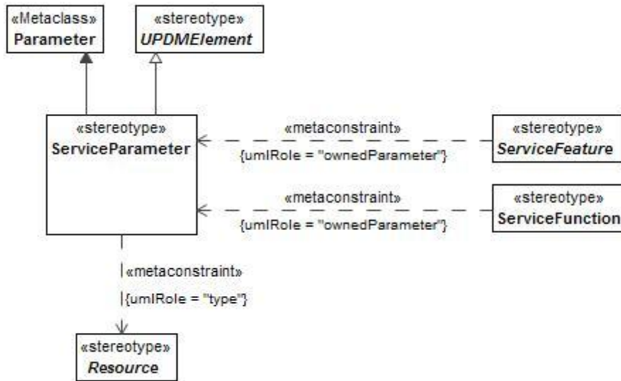
Figure 8:91 - ServiceParameter
