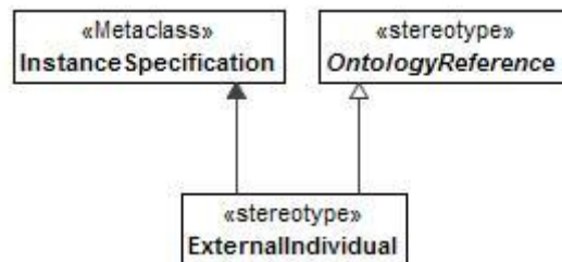
Figure 8:195 - ExternalIndividual
