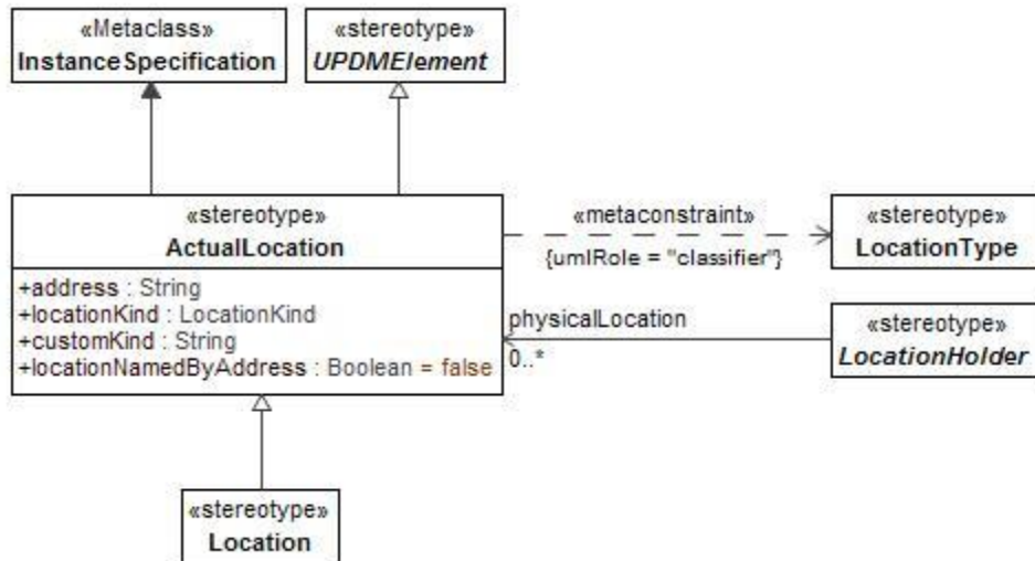
Figure 8:13 - ActualLocation
