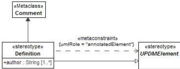
Figure 8:194 - Definition
