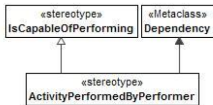
Figure 8:156 - ActivityPerformedByPerformer
