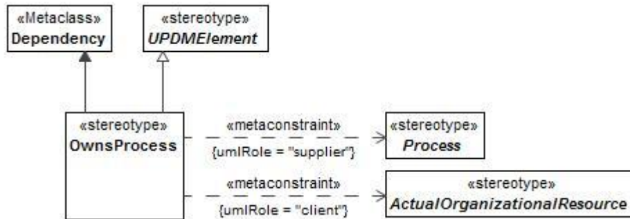
Figure 8:201 - OwnsProcess
