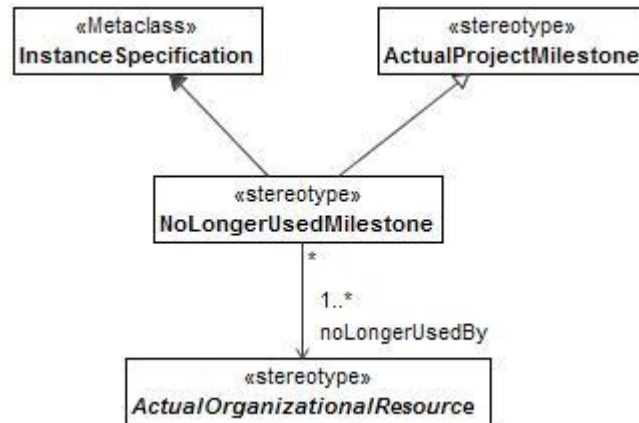
Figure 8:210 - NoLongerUsedMilestone
