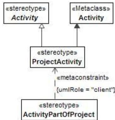
Figure 8:154 - ProjectActivity
