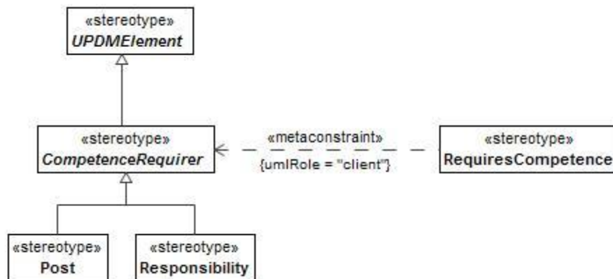
Figure 8:75 - CompetenceRequirer
