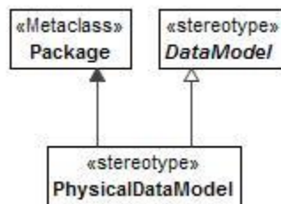
Figure 8:124 - PhysicalDataModel
