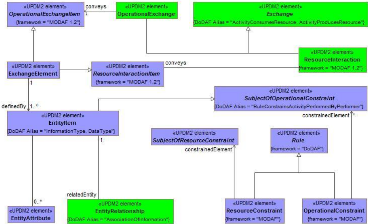
Figure A:50 - Information and Data - DM2
