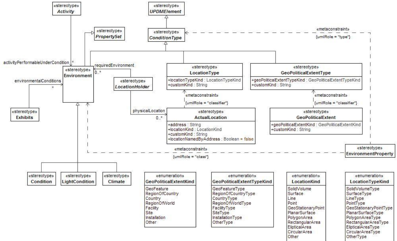
Figure B:6 - Environment Elements
