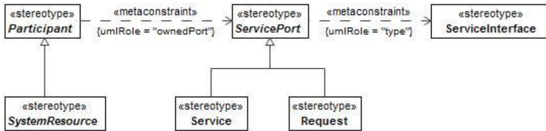
Figure B:37 - SV-12
