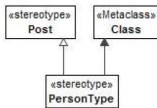
Figure 8:167 - PersonType
