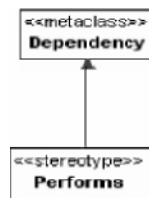
Figure 7:3 - Performs Stereotype
