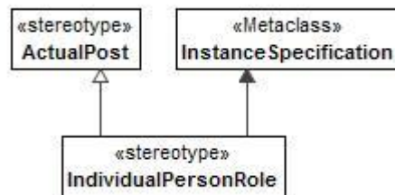
Figure 8:165 - IndividualPersonRole
