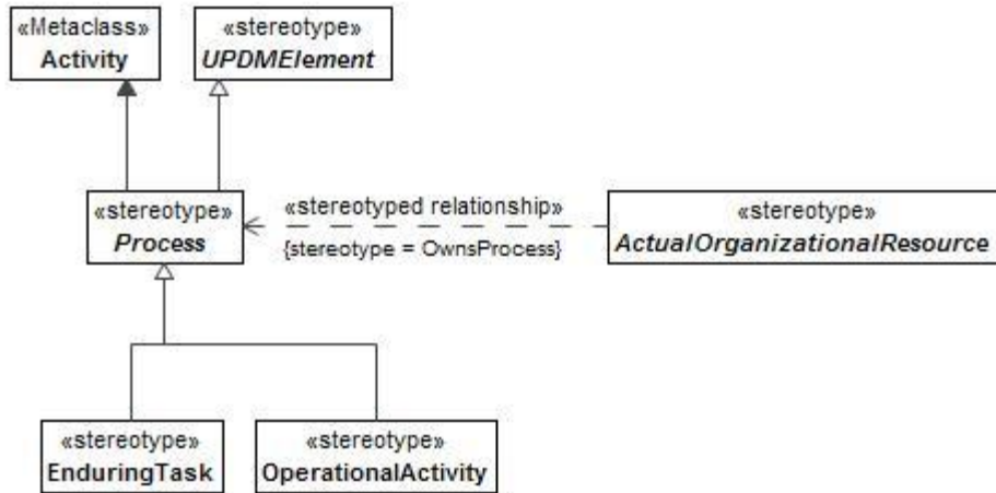
Figure 8:202 - Process
