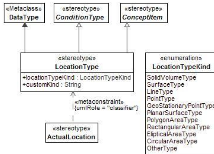
Figure 8:18 - LocationType
