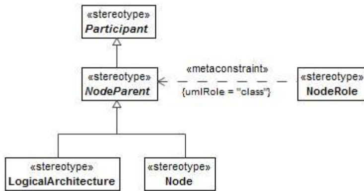
Figure 8:61 - NodeParent
