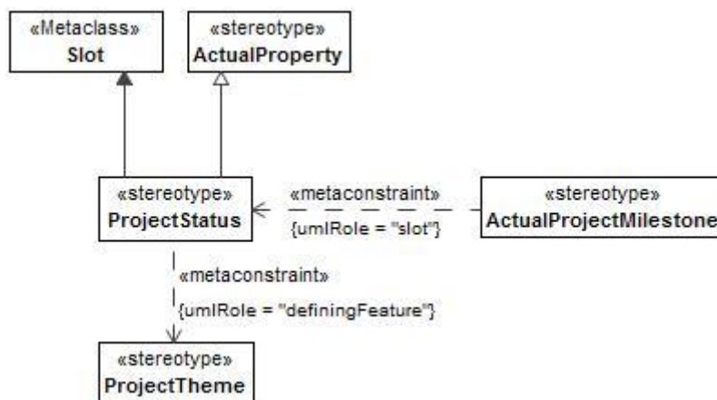
Figure 8:188 - ProjectStatus
