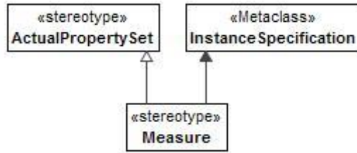
Figure 8:162 - Measure
