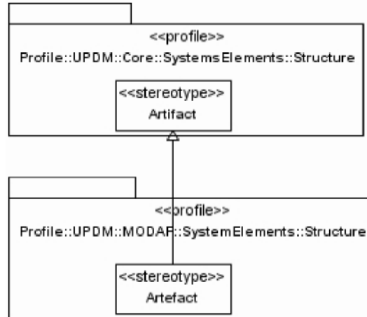
Figure 7:10 - Aliases
