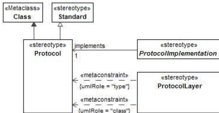
Figure 8:144 - Protocol
