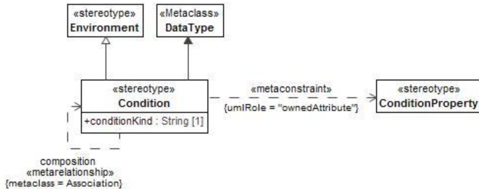
Figure 8:157 - Condition
