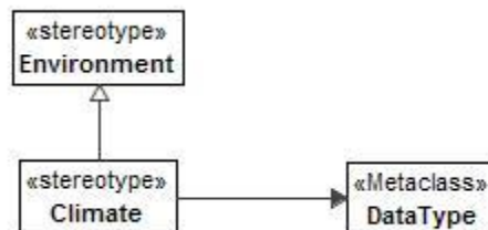
Figure 8:191 - Climate
