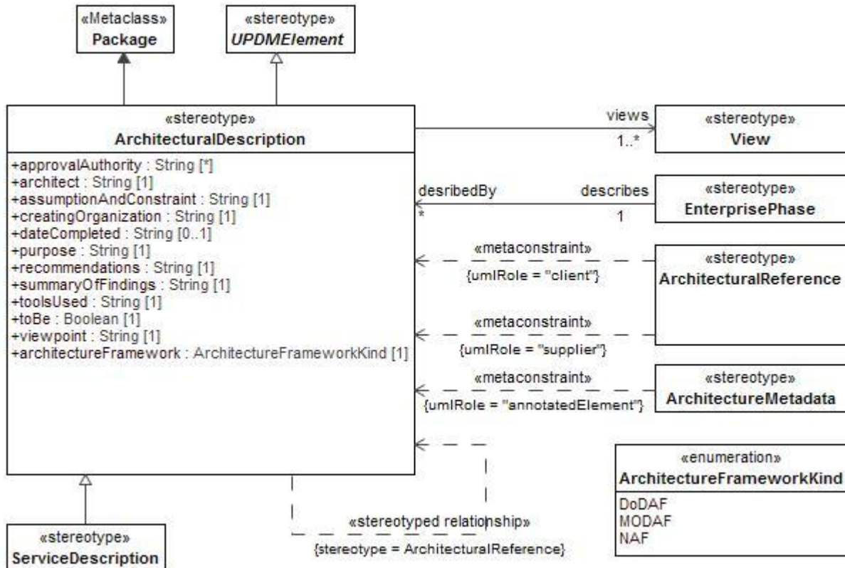
Figure 8:30 - ArchitecturalDescription
