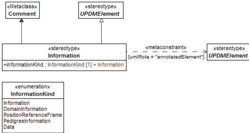
Figure 8:155 - Information
