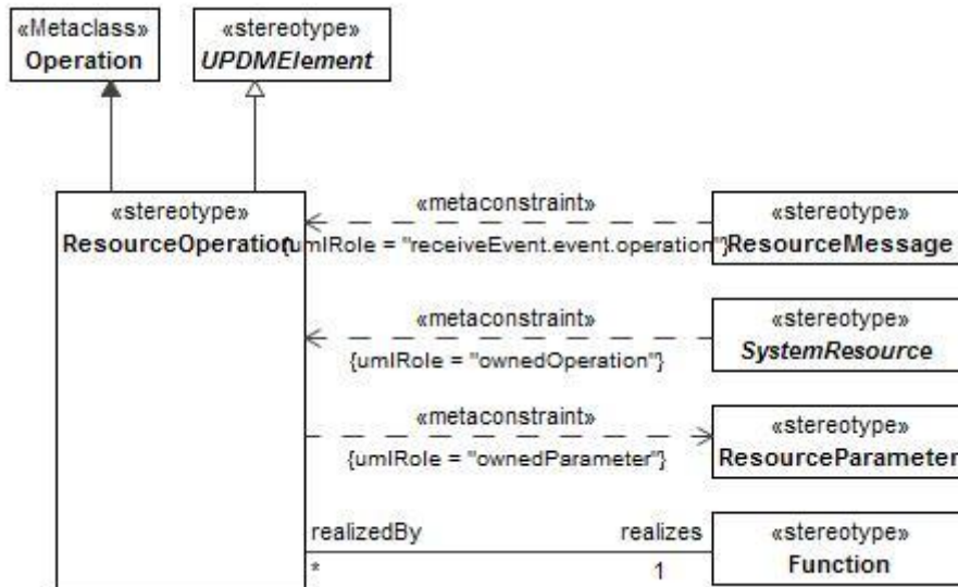
Figure 8:119 - ResourceOperation
