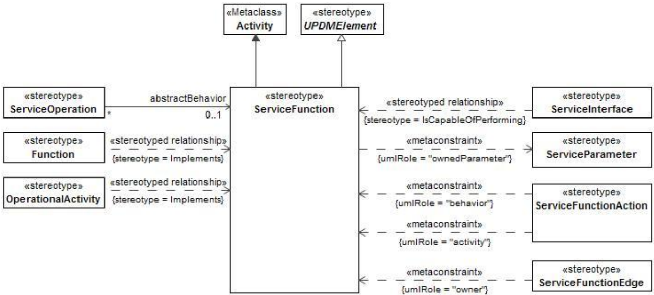
Figure 8:84 - ServiceFunction
