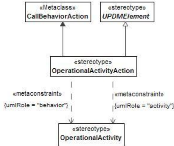
Figure 8:39 - OperationalActivityAction
