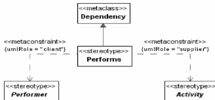
Figure 7:4 - Performs Hierarchy
