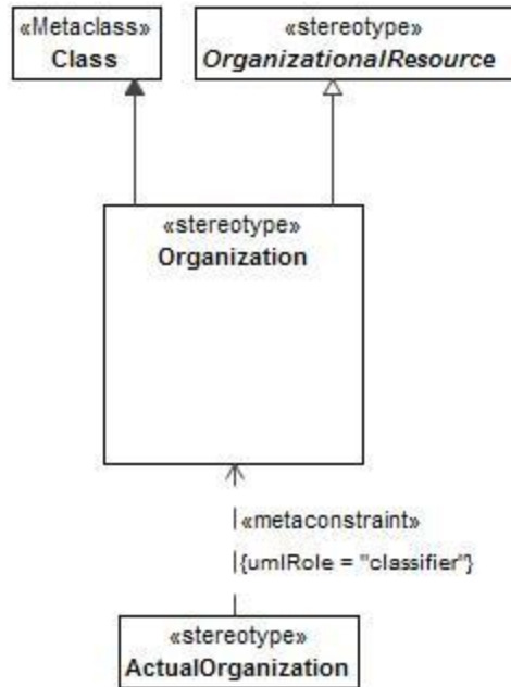
Figure 8:76 - Organization
