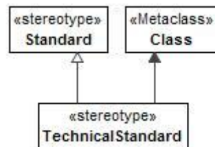
Figure 8:178 - TechnicalStandard
