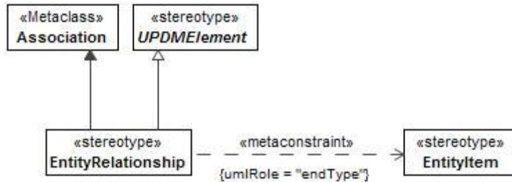
Figure 8:151 - EntityRelationship
