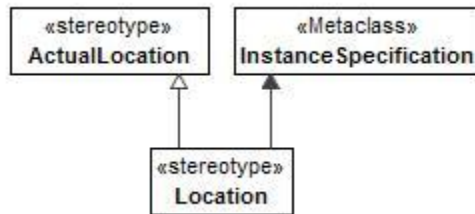
Figure 8:161 - Location
