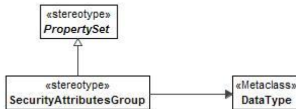
Figure 8:180 - SecurityAttributesGroup
