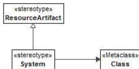
Figure 8:176 - System
