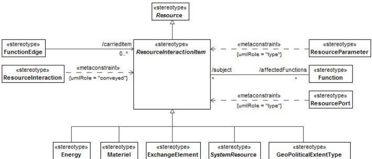
Figure 8:126 - ResourceInteractionItem
