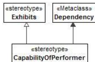
Figure 8:173 - CapabilityOfPerformer
