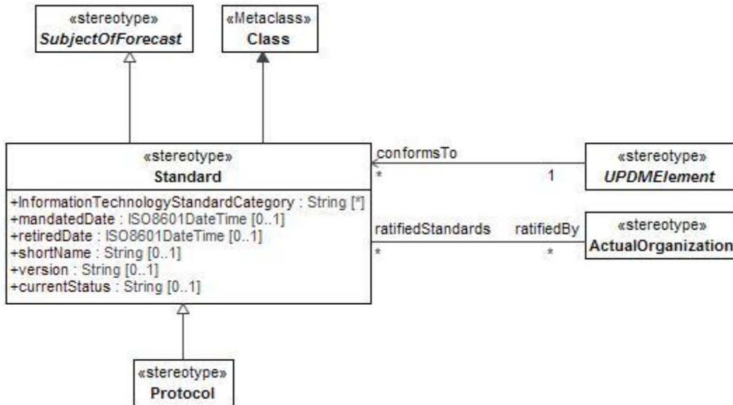
Figure 8:146 - Standard
