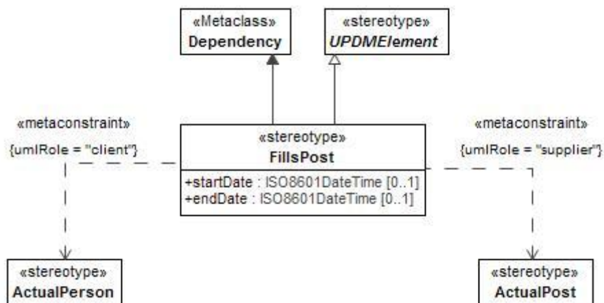
Figure 8:74 - FillsPost
