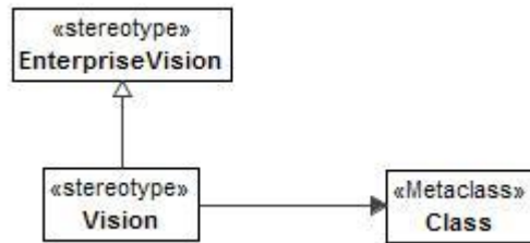
Figure 8:175 - Vision
