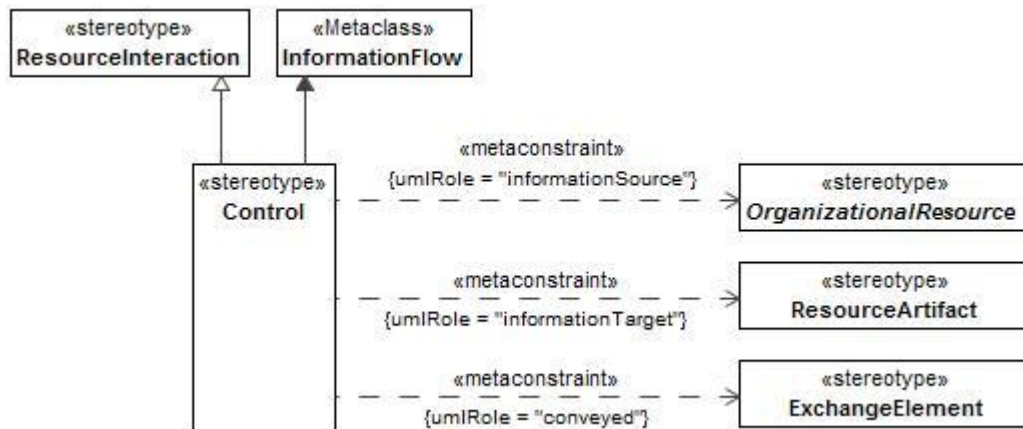
Figure 8:204 - Control
