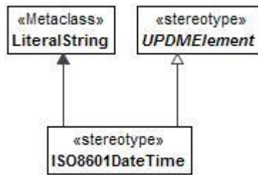
Figure 8:36 - ISO8601DateTime
