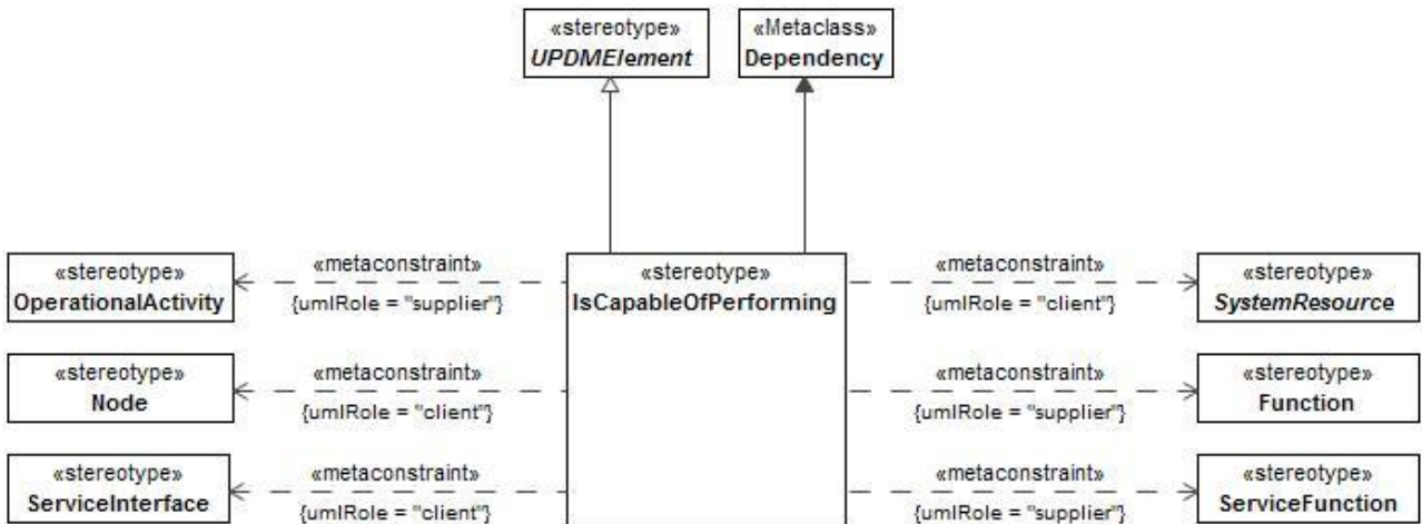
Figure 8:12 - IsCapableOfPerforming
