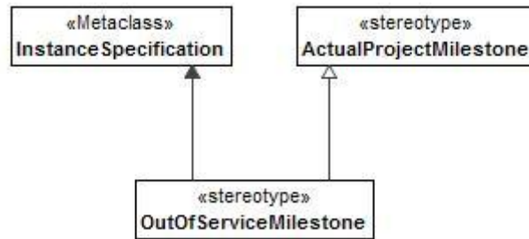
Figure 8:184 - OutOfServiceMilestone
