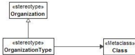
Figure 8:166 - OrganizationType
