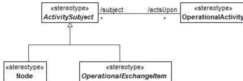
Figure 8:200 - ActivitySubject
