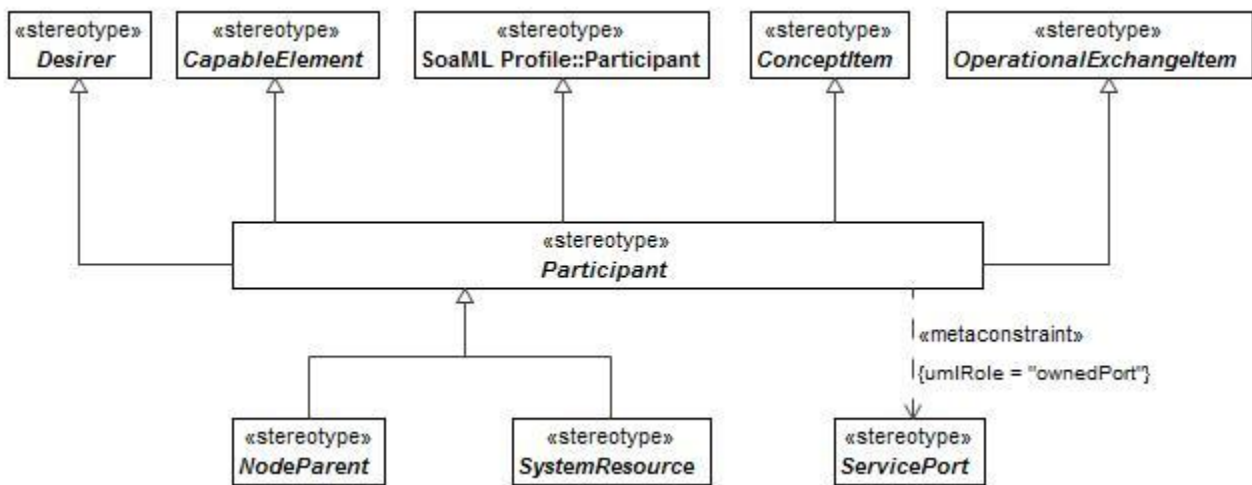
Figure 8:27 - Participant
