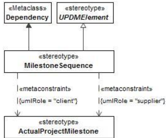
Figure 8:183 - MilestoneSequence
