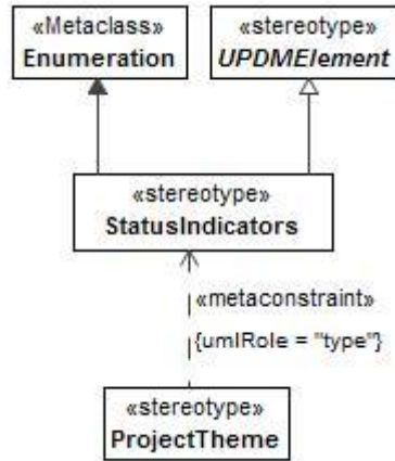
Figure 8:190 - StatusIndicators
