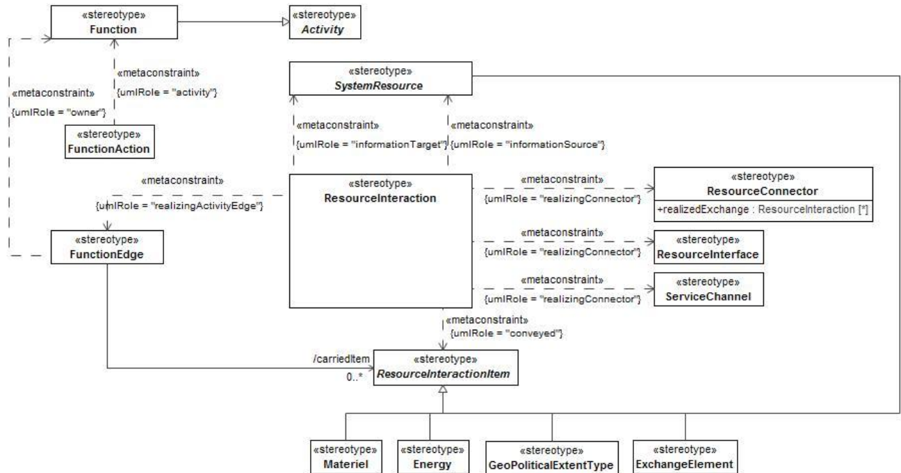
Figure B:42 - SV-6/SvcV-6
