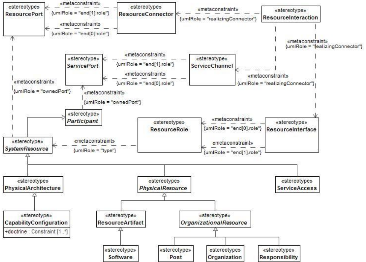
Figure B:39 - SV-3/SvcV-3a/SvcV-3b
