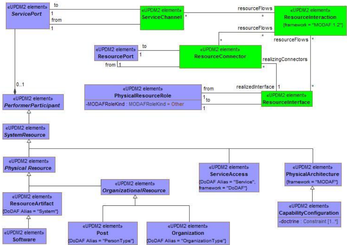
Figure A:37 - SV-3/SvcV-3a/SvcV-3b - DMM
