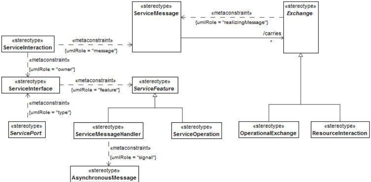
Figure B:23 - SOV-4c
