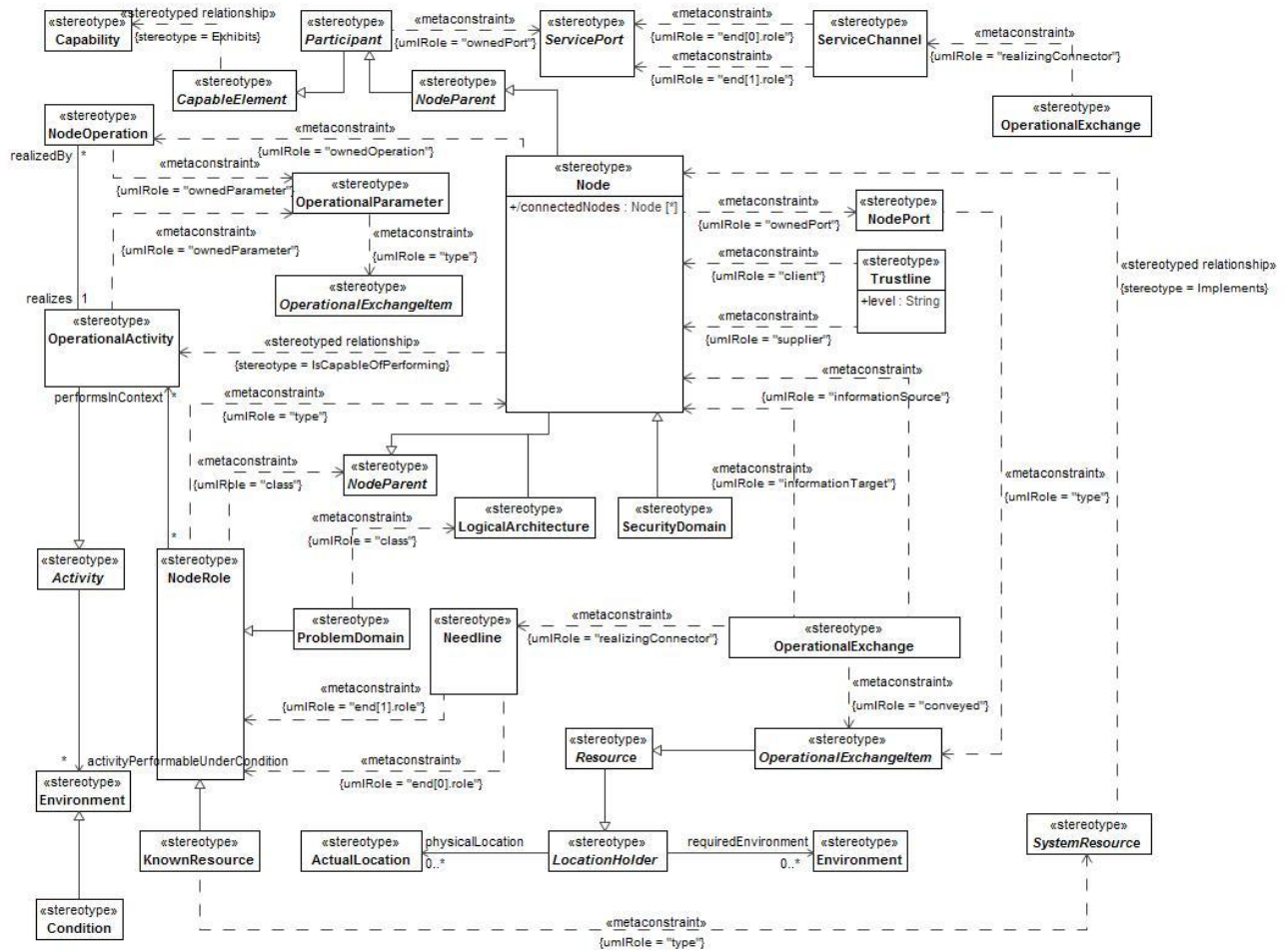
Figure B:9 - OV-2
