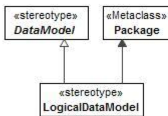
Figure 8:47 - LogicalDataModel
