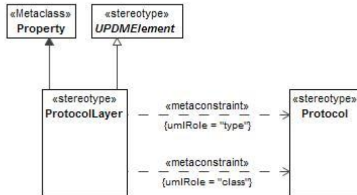
Figure 8:213 - ProtocolLayer
