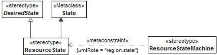
Figure 8:121 - ResourceState
