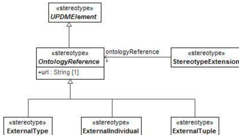
Figure 8:197 - OntologyReference
