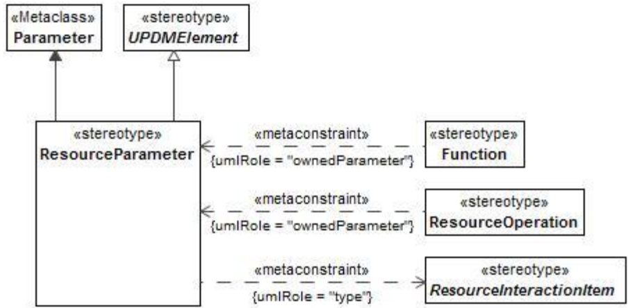
Figure 8:120 - ResourceParameter
