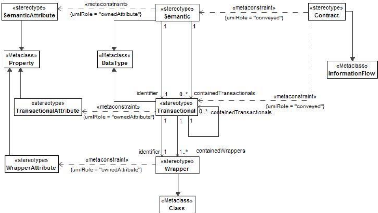
Figure 8:214 - SOPES Elements
