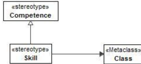
Figure 8:168 - Skill
