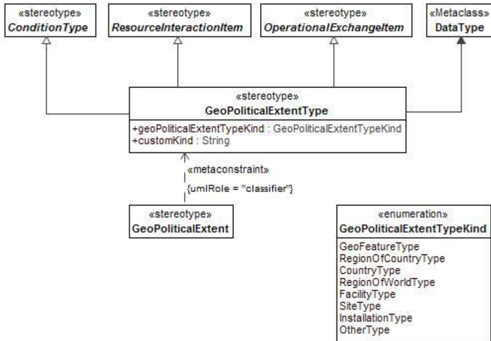
Figure 8:160 - GeoPoliticalExtentType
