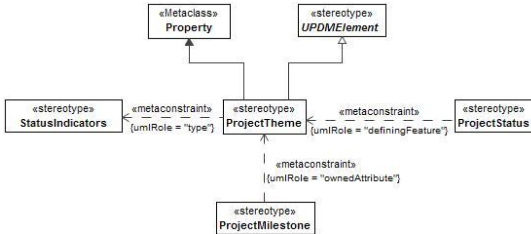
Figure 8:189 - ProjectTheme
