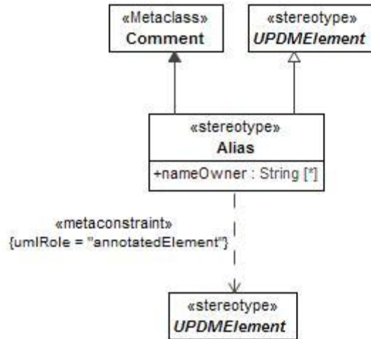
Figure 8:193 - Alias
