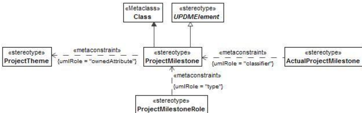
Figure 8:185 - ProjectMilestone
