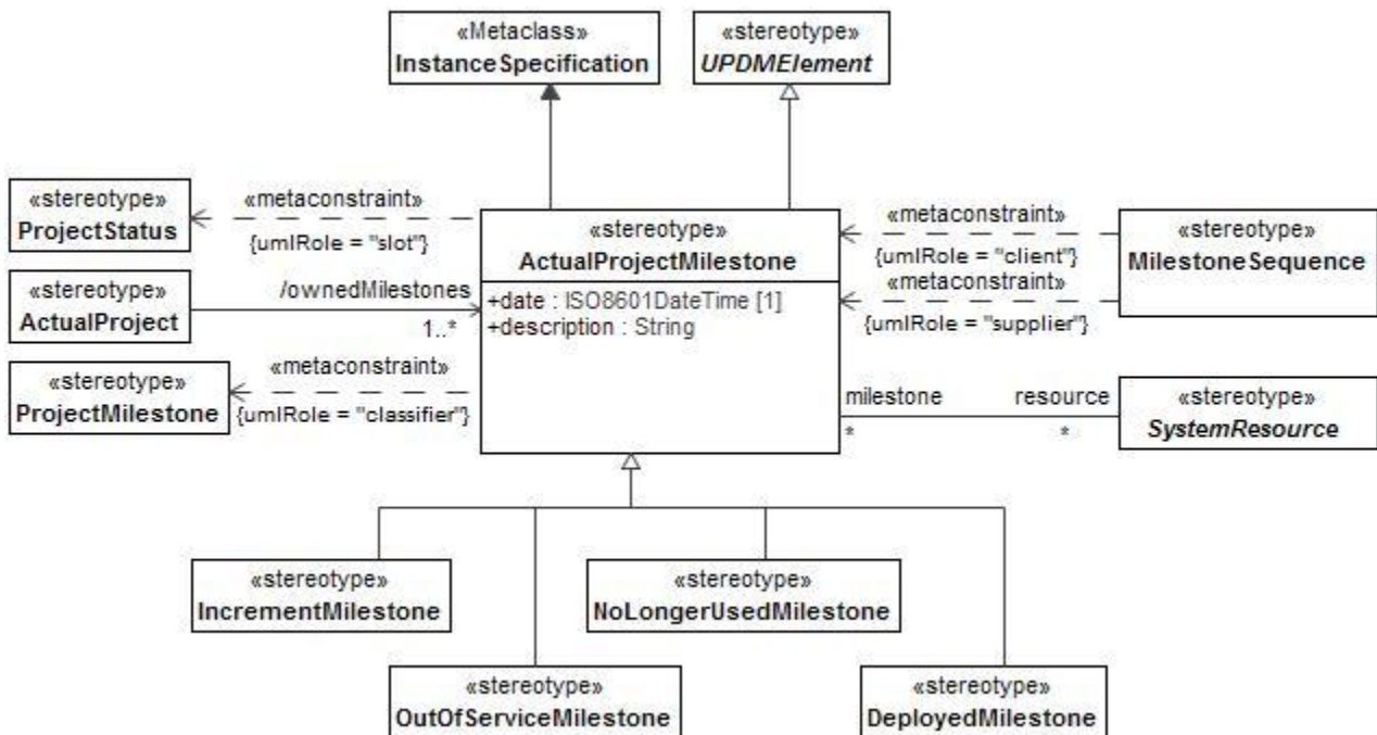
Figure 8:181 - ActualProjectMilestone
