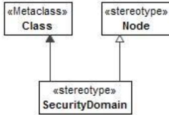
Figure 8:65 - SecurityDomain
