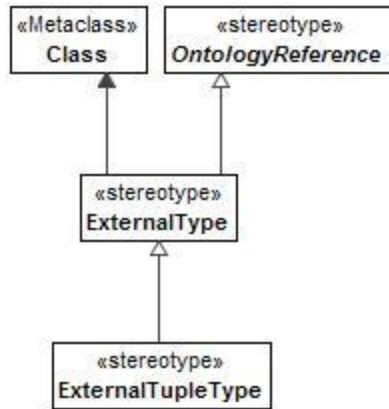
Figure 8:196 - ExternalType
