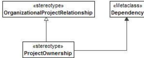
Figure 8:186 - ProjectOwnership
