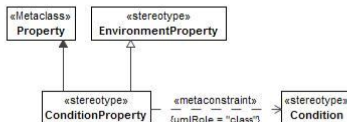
Figure 8:158 - ConditionProperty
