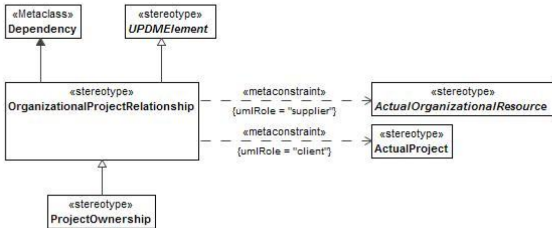
Figure 8:4 - OrganizationalProjectRelationship
