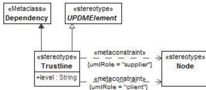
Figure 8:207 - Trustline
