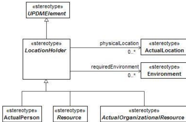
Figure 8:17 - LocationHolder
