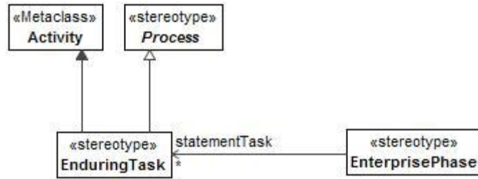
Figure 8:211 - EnduringTask
