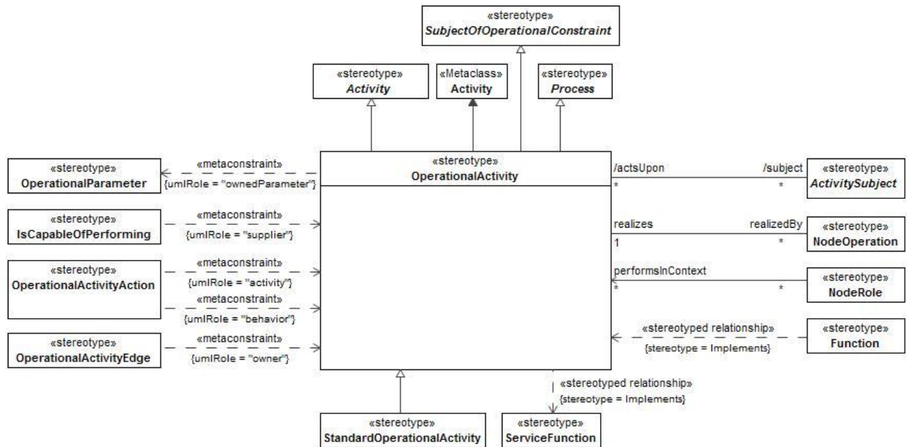
Figure 8:38 - OperationalActivity
