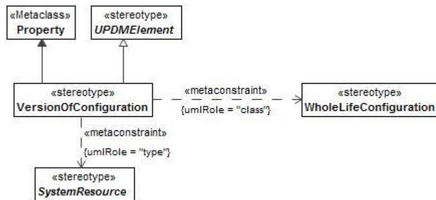
Figure 8:142 - VersionOfConfiguration
