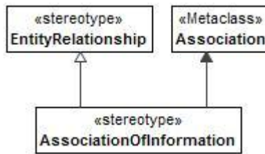
Figure 8:179 - AssociationOfInformation
