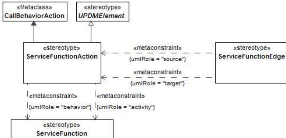
Figure 8:85 - ServiceFunctionAction
