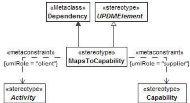
Figure 8:110 - MapsToCapability
