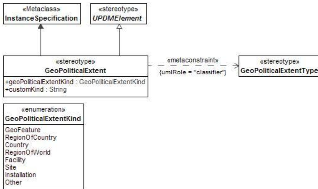
Figure 8:159 - GeoPoliticalExtent
