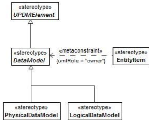
Figure 8:123 - DataModel
