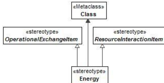
Figure 8:205 - Energy
