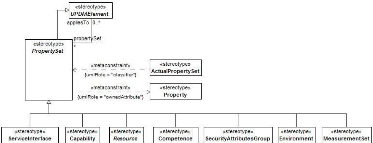
Figure 8:25 - PropertySet
