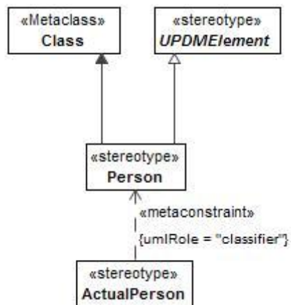
Figure 8:78 - Person
