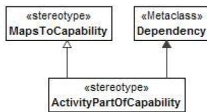
Figure 8:172 - ActivityPartOfCapability
