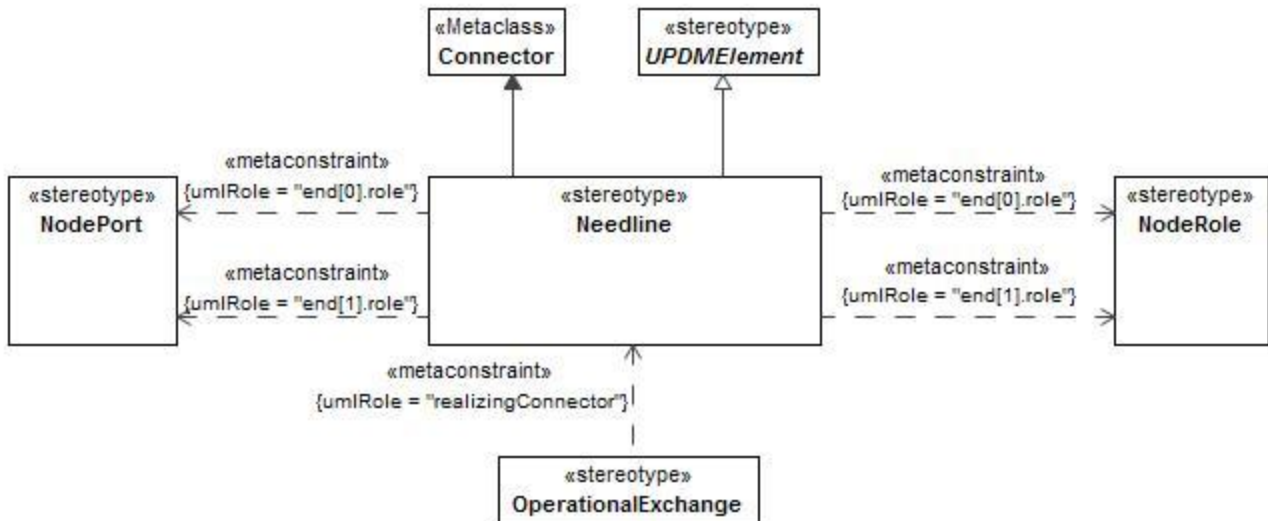
Figure 8:59 - Needline
