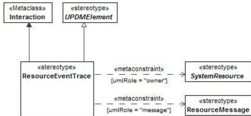
Figure 8:117 - ResourceEventTrace
