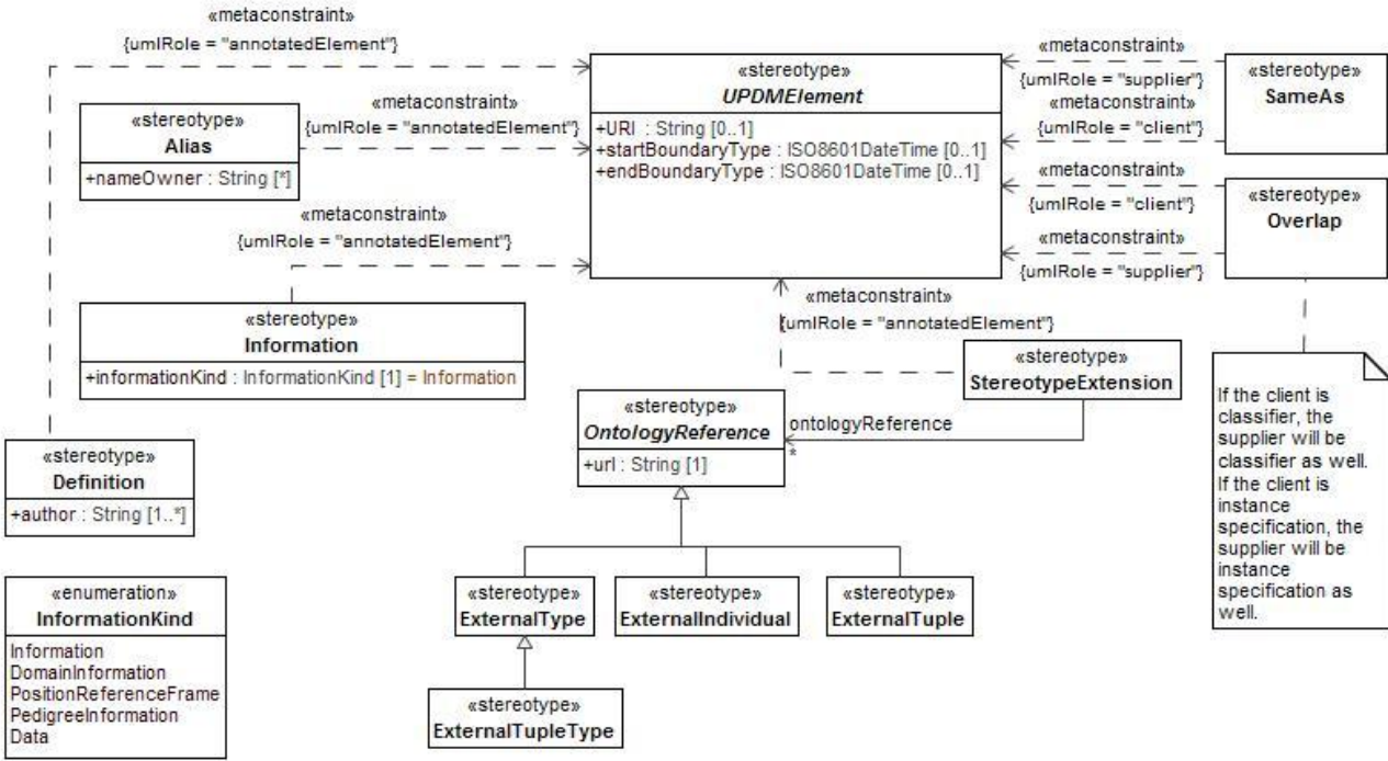
Figure B:5 - AV-2
