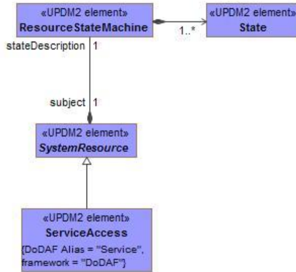
Figure A:32 - SV-10b/SvcV-10b DMM
