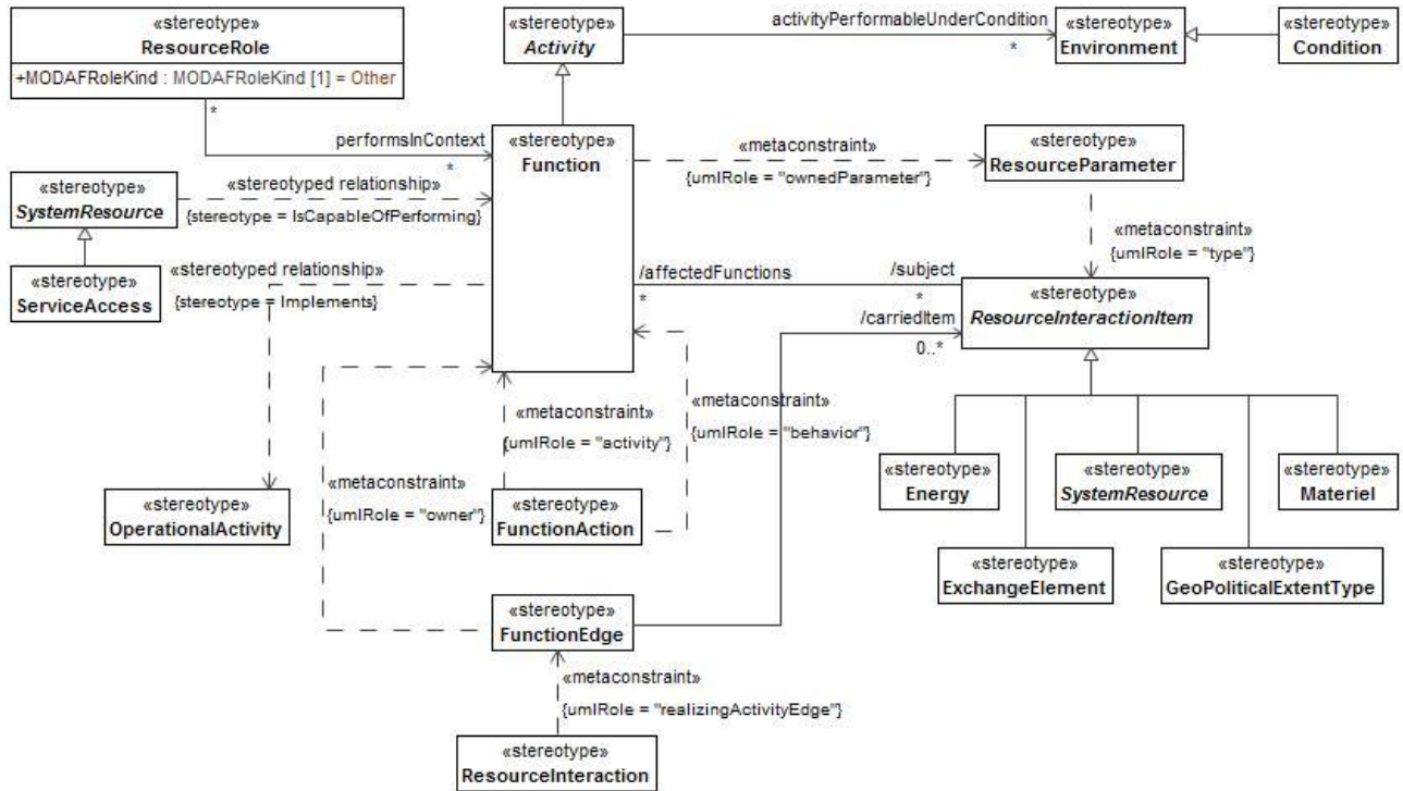
Figure B:40 - SV-4/SvcV-4
