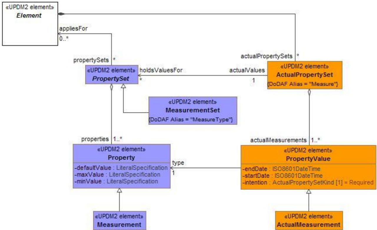
Figure A:41 - SV-7/SvcV-7 - DMM
