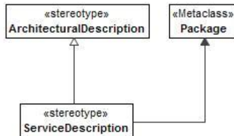
Figure 8:171 - ServiceDescription
