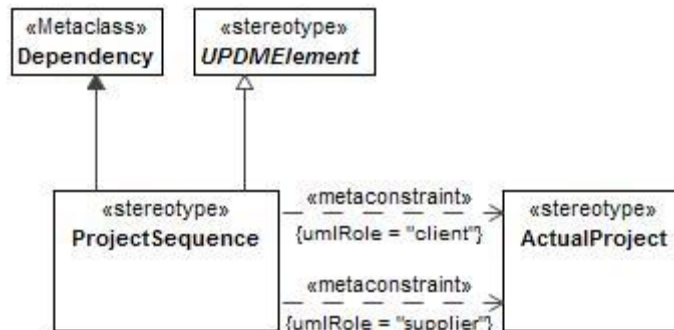
Figure 8:187 - ProjectSequence
