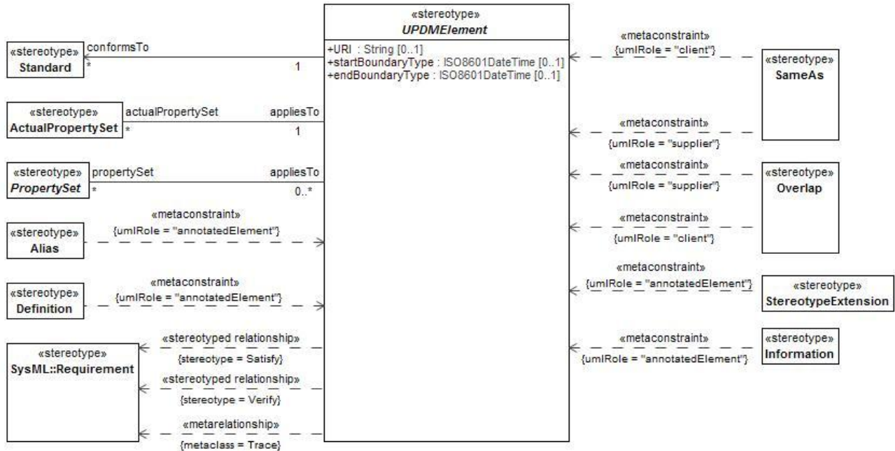
Figure 8:8 - UPDMElement
