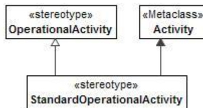
Figure 8:203 - StandardOperationalActivity
