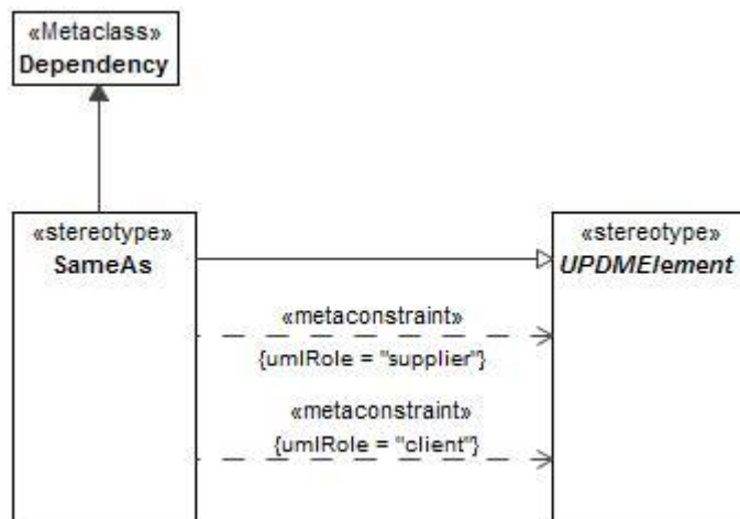
Figure 8:198 - SameAs
