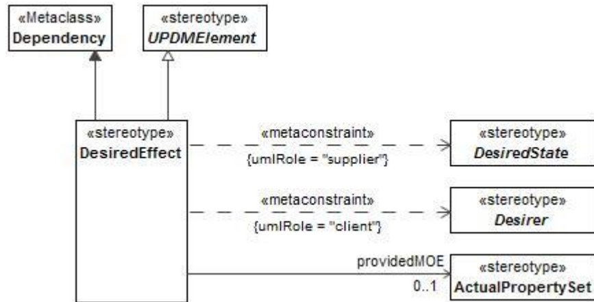
Figure 8:174 - DesiredEffect
