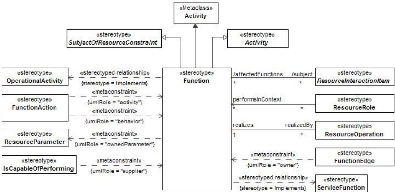
Figure 8:114 - Function
