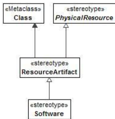
Figure 8:132 - ResourceArtifact
