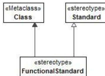
Figure 8:177 - FunctionalStandard
