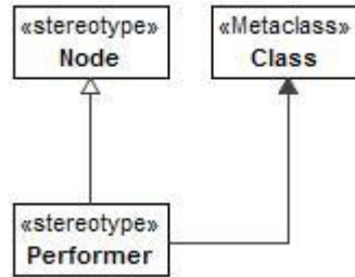
Figure 8:164 - Performer
