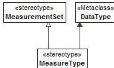
Figure 8:163 - MeasureType
