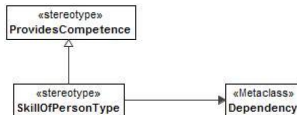
Figure 8:169 - SkillOfPersonType
