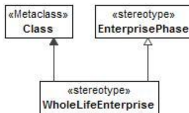
Figure 8:212 - WholeLifeEnterprise
