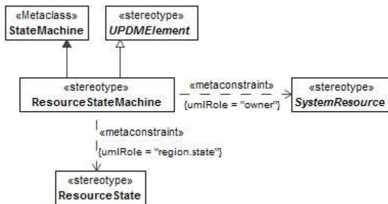
Figure 8:122 - ResourceStateMachine
