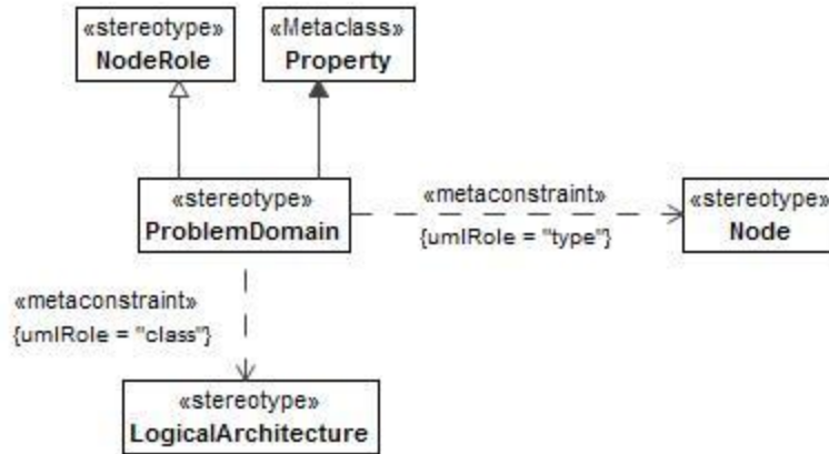
Figure 8:206 - ProblemDomain
