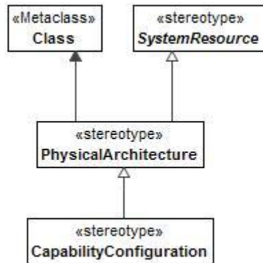
Figure 8:130 - PhysicalArchitecture
