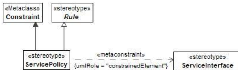
Figure 8:100 - ServicePolicy
