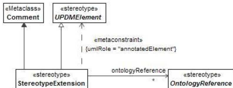
Figure 8:199 - StereotypeExtension
