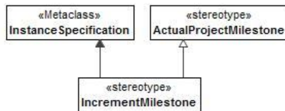
Figure 8:182 - IncrementMilestone
