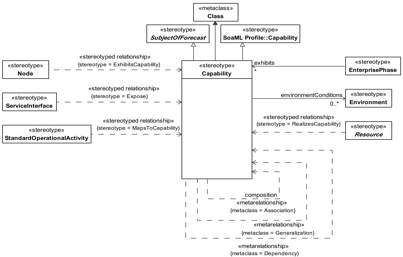
Figure 8.113 - Elements related to the Capability stereotype
