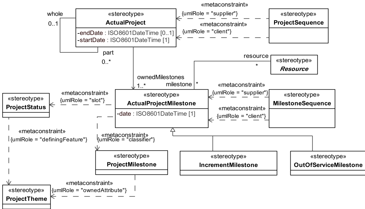
Figure 8.215 - Elements related to the AcV-2 product
