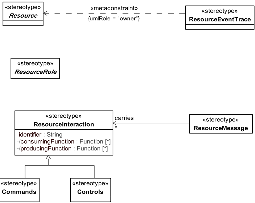
Figure 8.129 - Elements related to the SV-10c product
