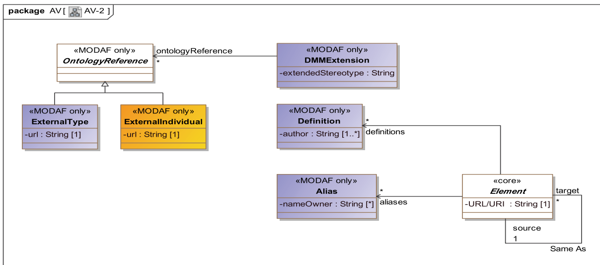
Figure A.4 - AV-2
