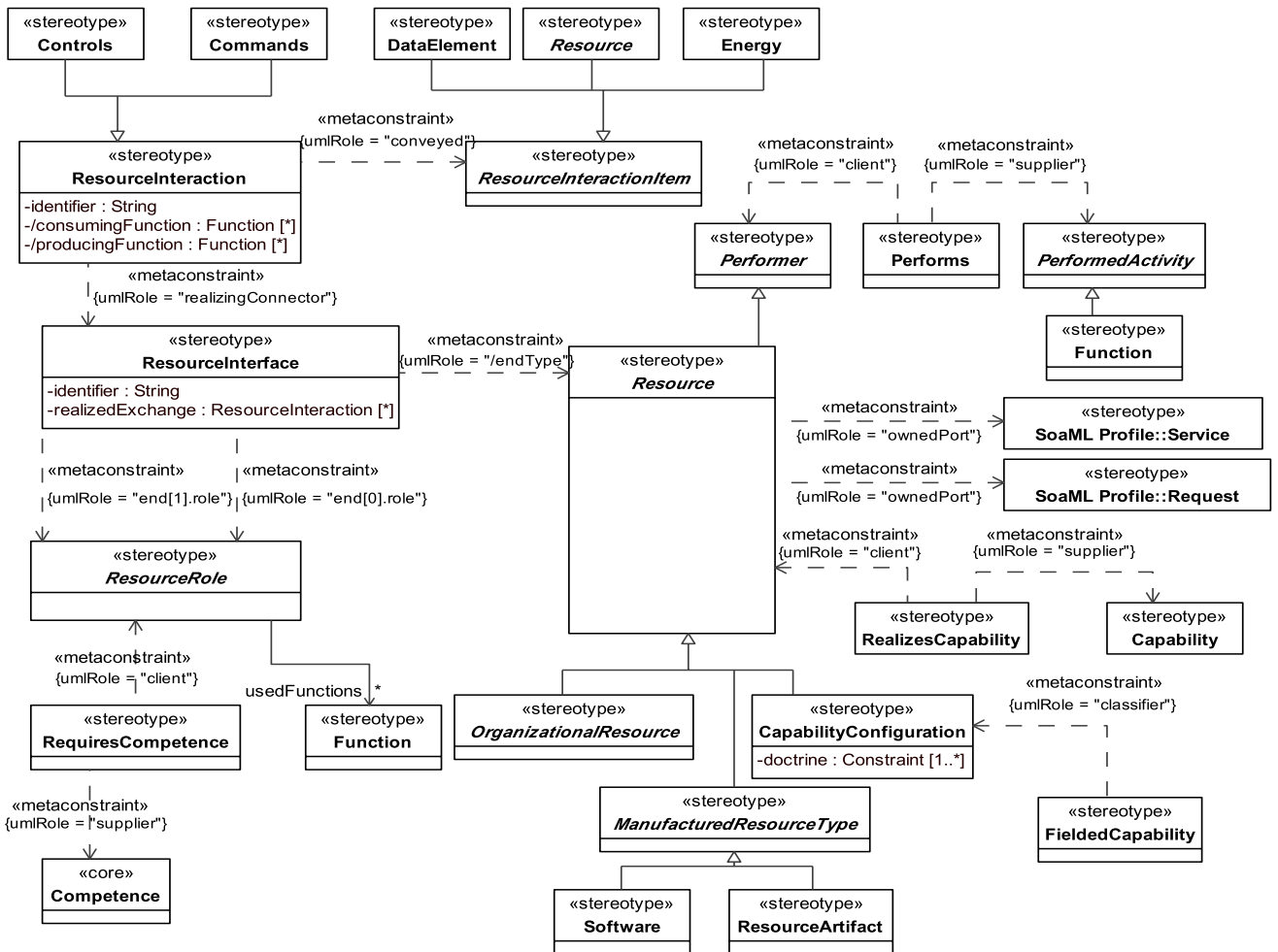
Figure 8.125 - Elements related to the SV-1 product
