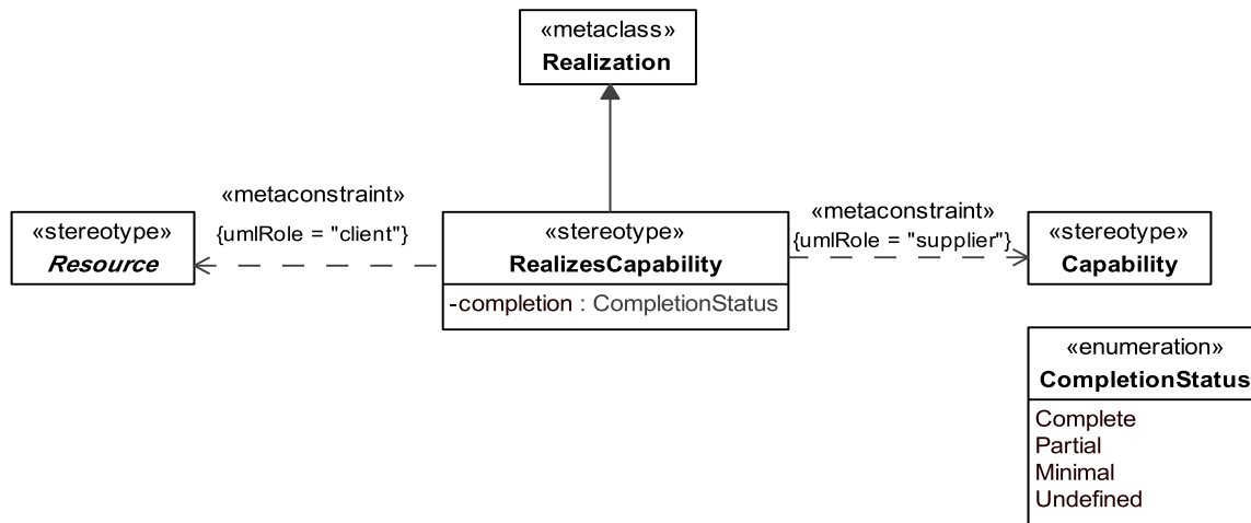
Figure 8.119 - Elements related to the RealizesCapability stereotype
