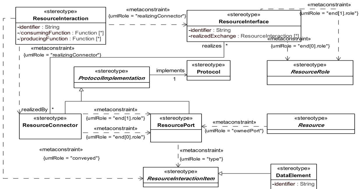
Figure 8.132 - Elements related to the SV-2 product
