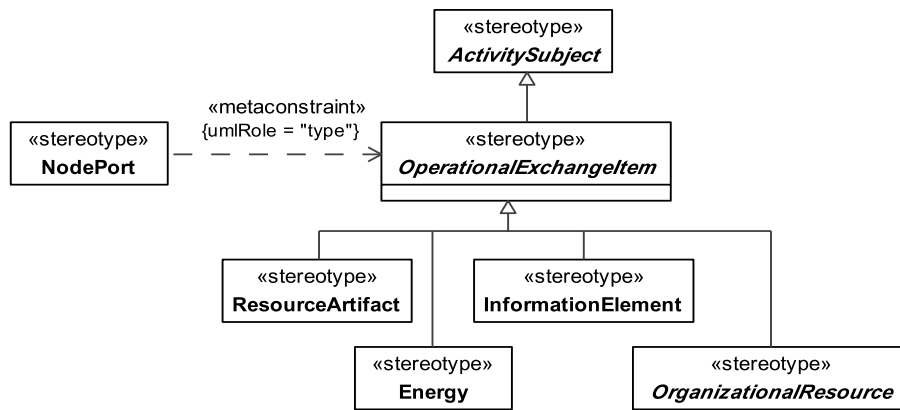
Figure 8.52 - Elements related to the abstract OperationalExchangeItem stereotype
