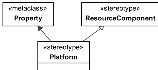
Figure 8.166 - Elements related to the Platform stereotype
