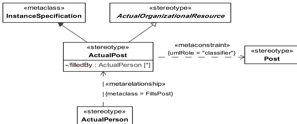
Figure 8.73 - Elements related to the ActualPost stereotype
