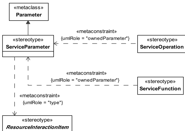
Figure 8.99 - Elements related to the ServiceParameter stereotype
