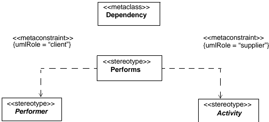
Figure 7.4 - Performs Hierarchy
