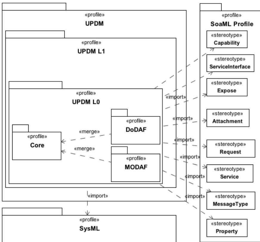
Figure 8.1 - UPDM Profile
