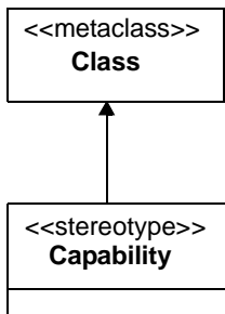
Figure 7.6 - Capabilities Generalization
