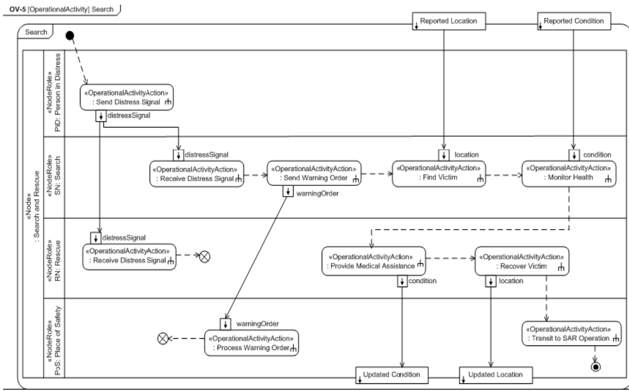
Figure C.19 - Alternate OV-5
