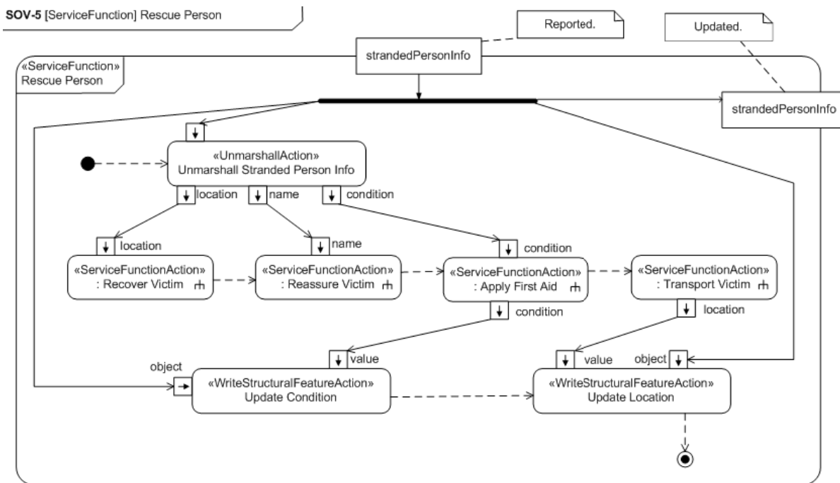
Figure C.26 - SOV-5
