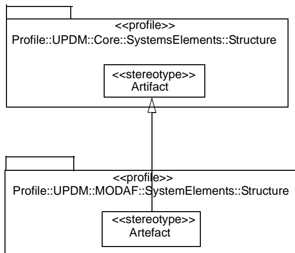
Figure 7.10 - Aliases
