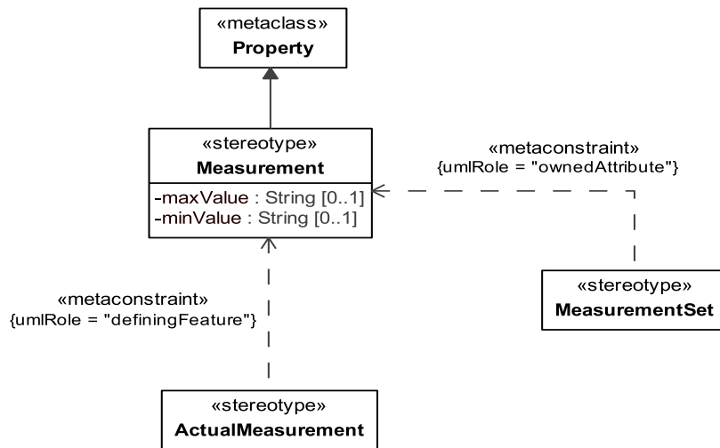
Figure 8.23 - Elements related to the Measurement stereotype
