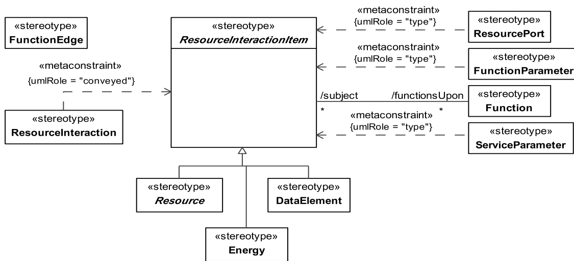
Figure 8.151 - Elements related to the abstract ResourceInteractionItem stereotype
