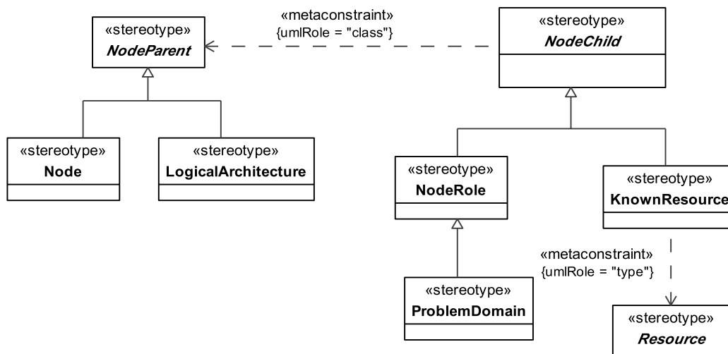
Figure 8.34 - Elements related to the OV-2 Nodes stereotype
