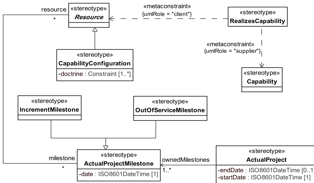
Figure 8.259 - Elements related to the StV-3 stereotype
