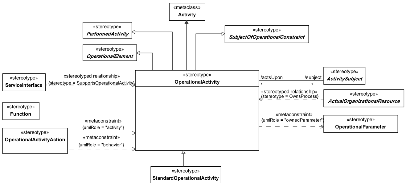
Figure 8.43 - Elements related to the OperationalActivity stereotype
