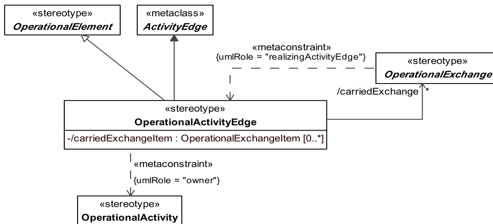
Figure 8.45 - Elements related to the OperationalActivityEdge stereotype
