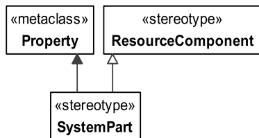
Figure 8.213 - Elements relating to the SystemPart Stereotype
