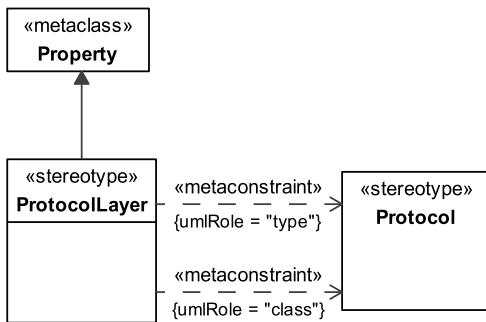
Figure 8.185 - Elements related to the ProtocolLayer stereotype
