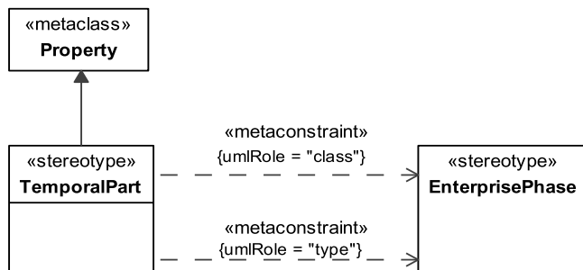
Figure 8.122 - Elements related to the TemporalPart stereotype
