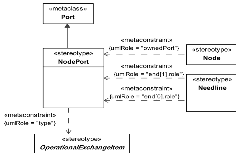
Figure 8.65 - Elements related to the NodePort stereotype
