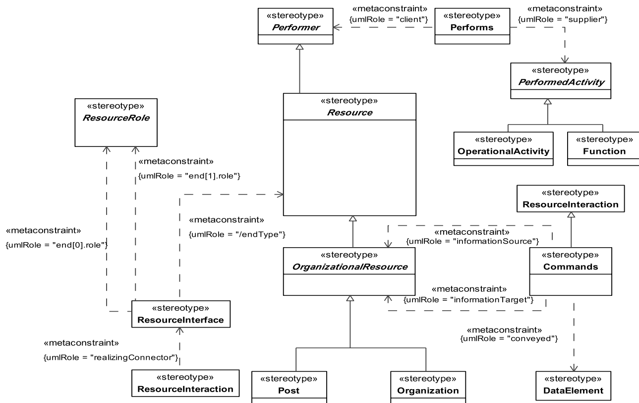
Figure 8.196 - Elements related to the OV-4 Typical product
