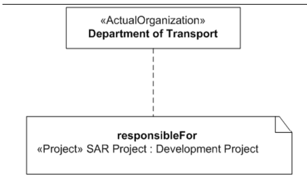
Figure C.32 - AcV-1
