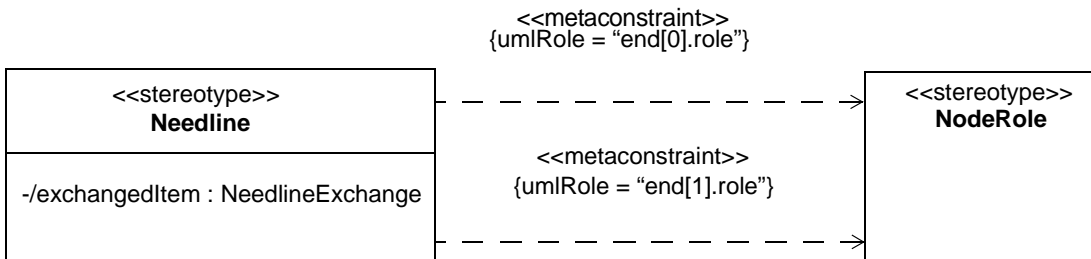
Figure 7.5 - Connector Extension
