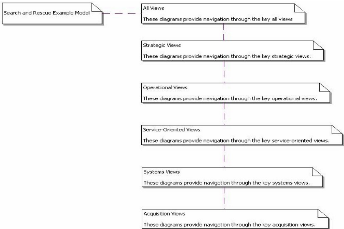
Figure C.1- Diagram Flow
