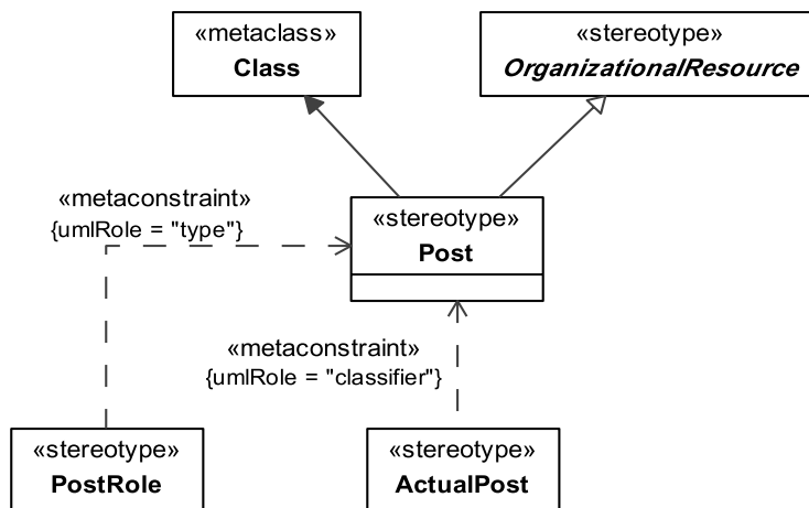
Figure 8.83 - Elements related to the Post stereotype
