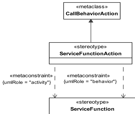
Figure 8.95 - Elements related to the ServiceFunctionAction stereotype
