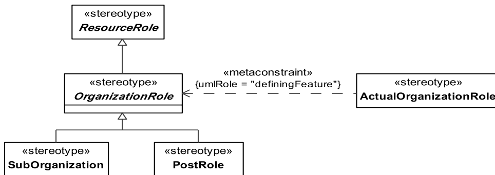
Figure 8.81 - Elements related to the abstract OrganizationRole stereotype
