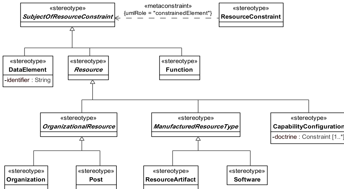
Figure 8.127 - Elements related to the SV-10a product
