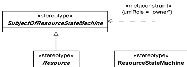
Figure 8.145 - Elements related to the abstract SubjectOfResourceStateMachine stereotype
