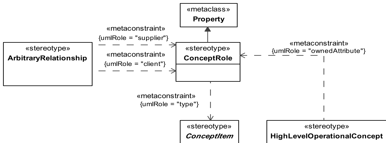
Figure 8.58 - Elements related to the abstract ConceptRole stereotype
