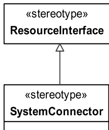
Figure 8.211 - Elements related to the SystemConnector stereotype
