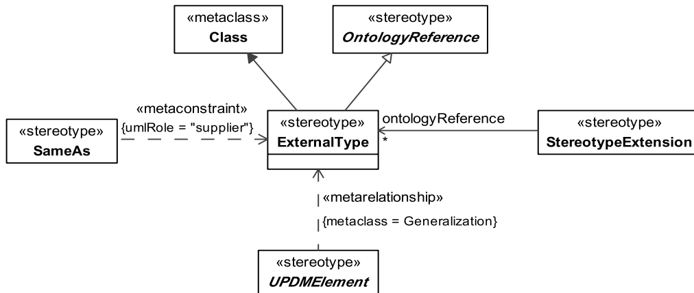
Figure 8.231 - Elements related to the ExternalType stereotype
