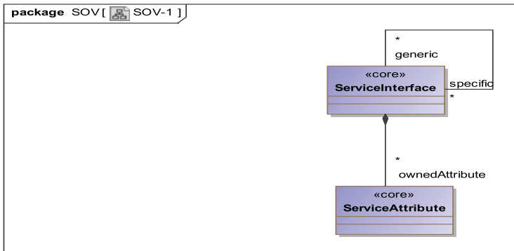
Figure A.24 - SOV-1
