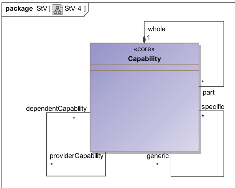
Figure A.34 - StV-4
