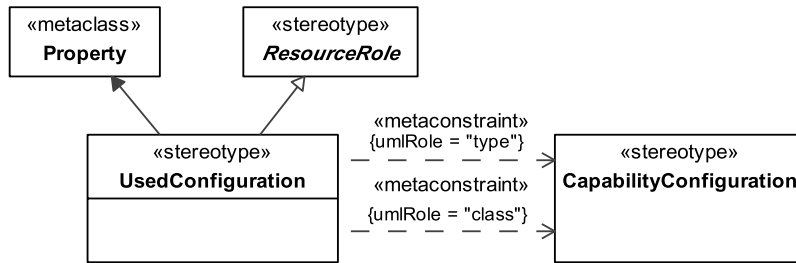
Figure 8.177 - Elements related to the UsedConfiguration stereotype
