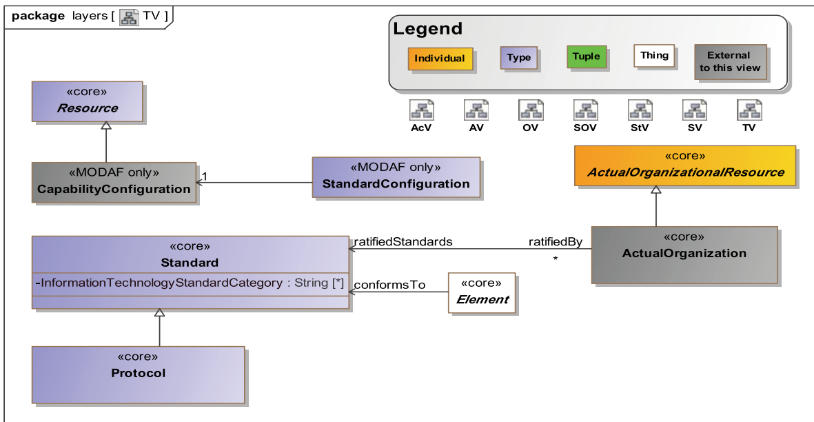
Figure A.12 - TV
