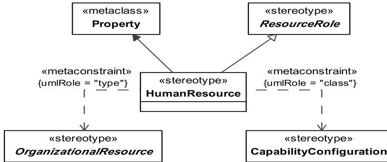
Figure 8.163 - Elements related to the HumanResource stereotype
