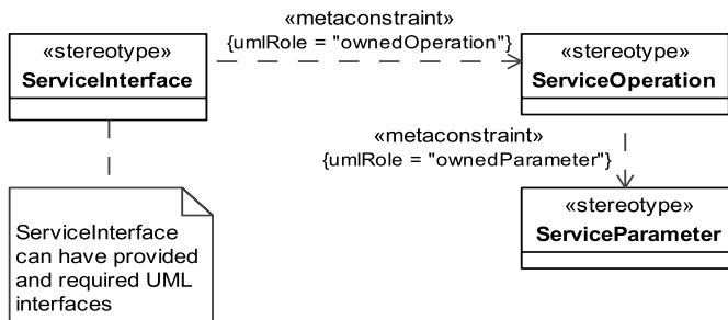
Figure 8.88 - Elements related to the SOV-2 product
