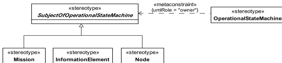
Figure 8.47 - Elements related to the abstract SubjectOfOperationalStateMachine stereotype
