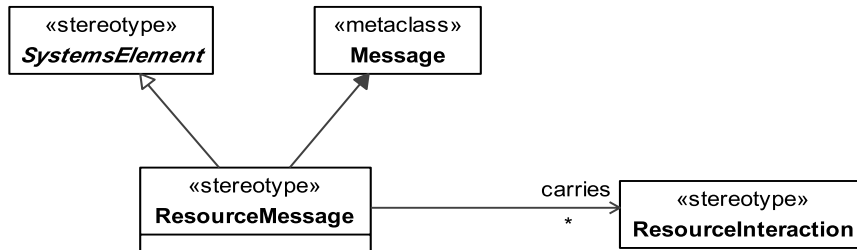
Figure 8.154 - Elements related to the ResourceMessage stereotype
