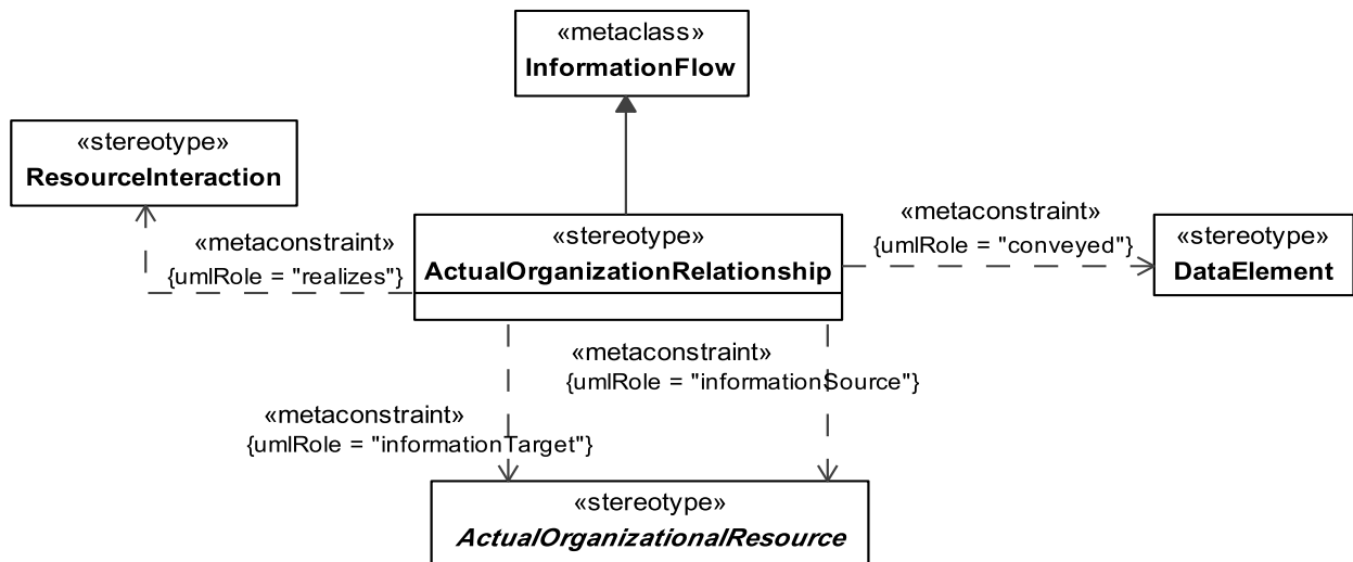
Figure 8.72 - Elements related to the ActualOrganizationRelationship stereotype
