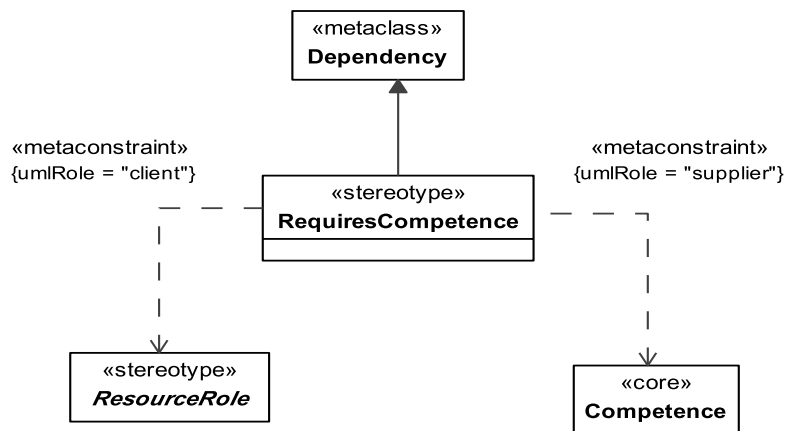
Figure 8.85 - Elements related to the RequiresCompetence stereotype
