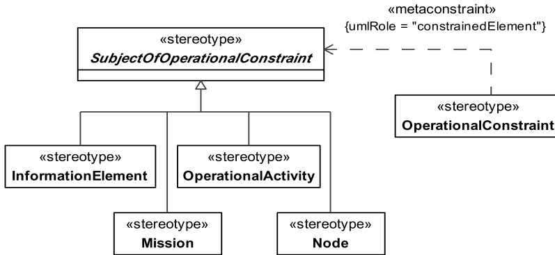
Figure 8.68 - Elements related to the abstract SubjectOfOperationalConstraint stereotype
