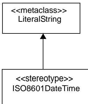
Figure 8.31 - Elements related to the ISO8601DateTime stereotype
