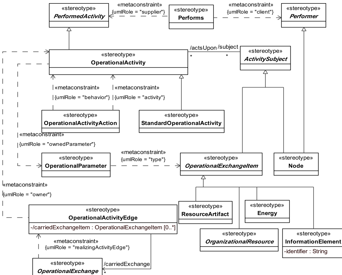
Figure 8.241 - Elements related to the OV-5 stereotype
