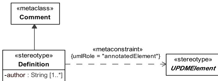
Figure 8.229 - Elements related to the Definition stereotype
