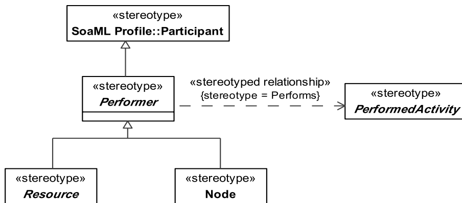
Figure 8.11 - Elements related to the abstract Performer stereotype
