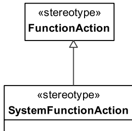
Figure 8.207 - Elements related to the SystemFunctionAction stereotype
