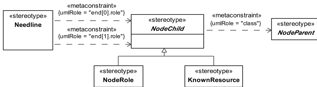
Figure 8.63 - Elements related to the abstract NodeChild stereotype
