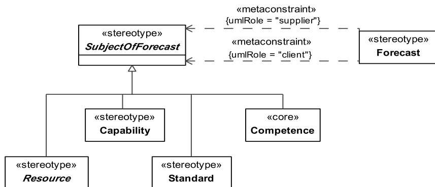
Figure 8.173 - Elements related to the abstract SubjectOfForecast stereotype
