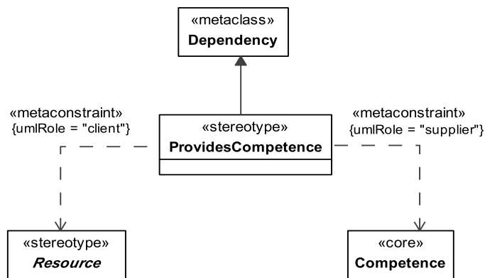
Figure 8.84 - Elements related to the ProvidesCompetence stereotype
