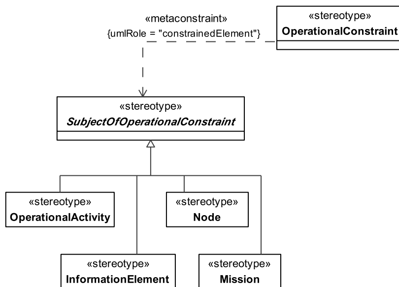
Figure 8.198 - Elements related to the OV-6a product
