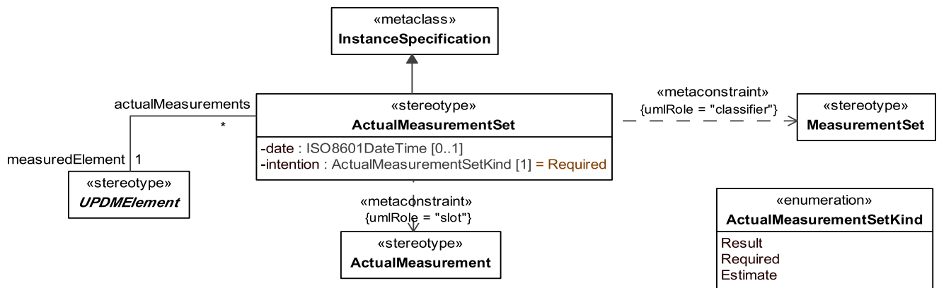
Figure 8.22 - Elements related to the ActualMeasurementSet stereotype
