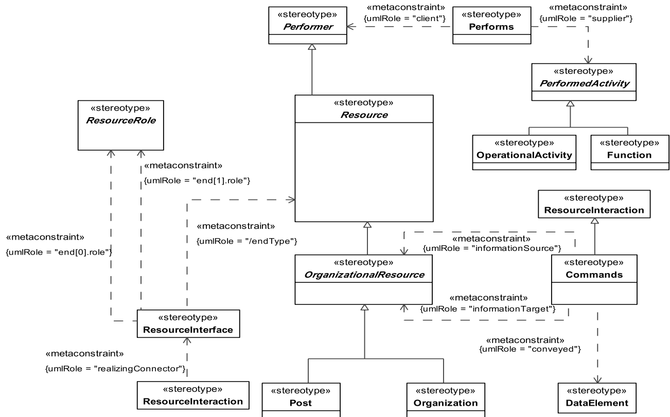
Figure 8.240 - Elements related to the OV-4 Typical stereotype
