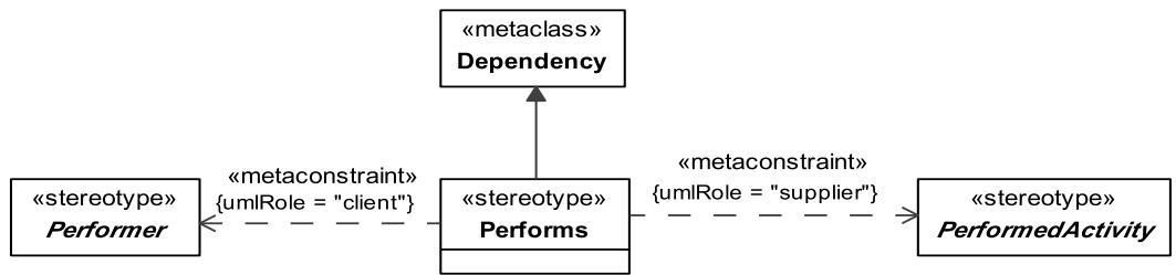
Figure 8.12 - Elements related to the Performs stereotype
