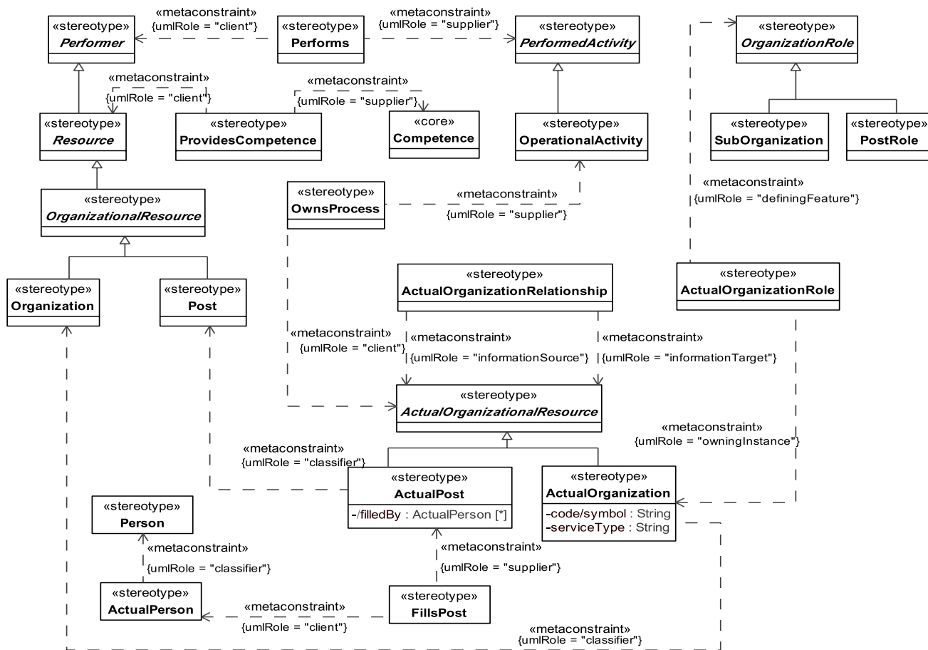
Figure 8.239 - Elements related to the OV-4 Actual stereotype
