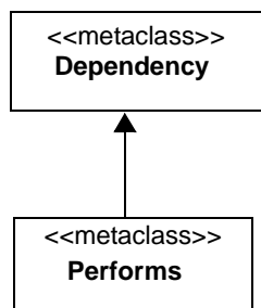
Figure 7.3 - Performs Stereotype
