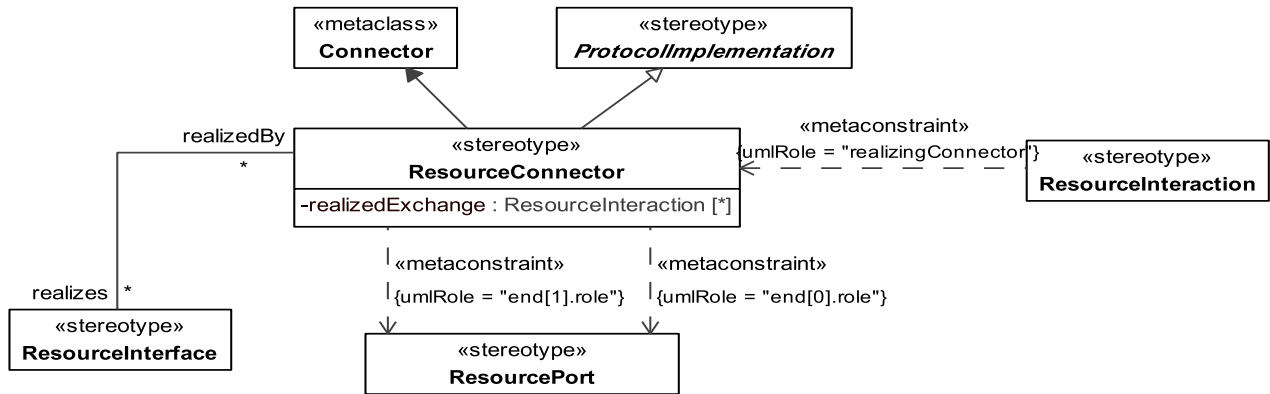
Figure 8.155 - Elements related to the ResourceConnector stereotype
