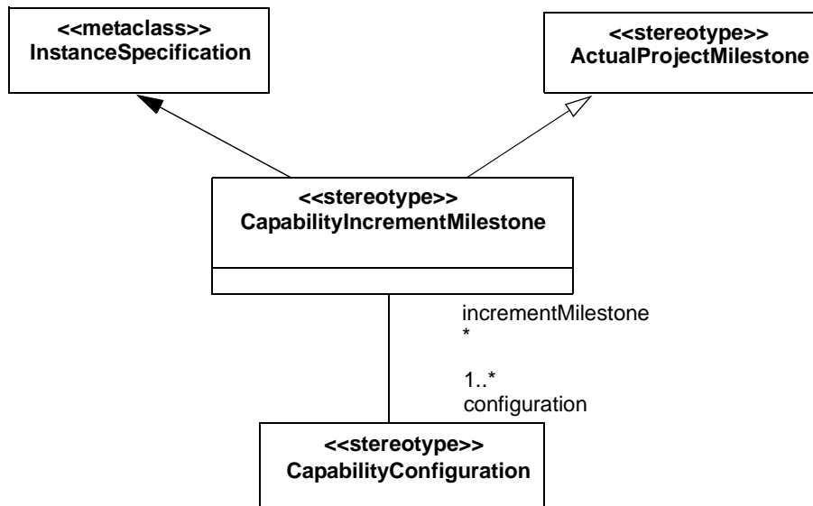
Figure 8.216 - Elements related to the CapabilityIncrementMilestone stereotype
