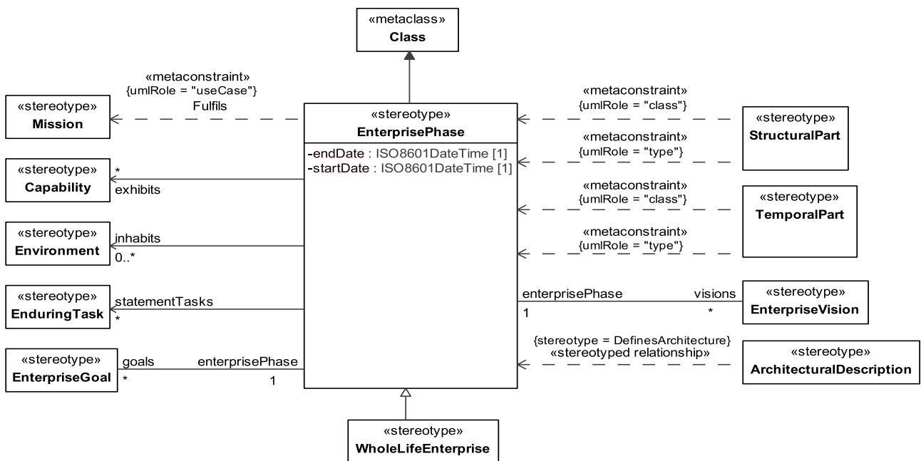
Figure 8.28 - Elements related to the DefinesArchitecture stereotype
