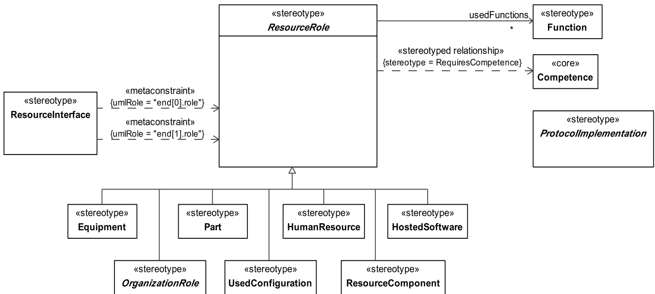
Figure 8.170 - Elements related to the abstract ResourceRole stereotype
