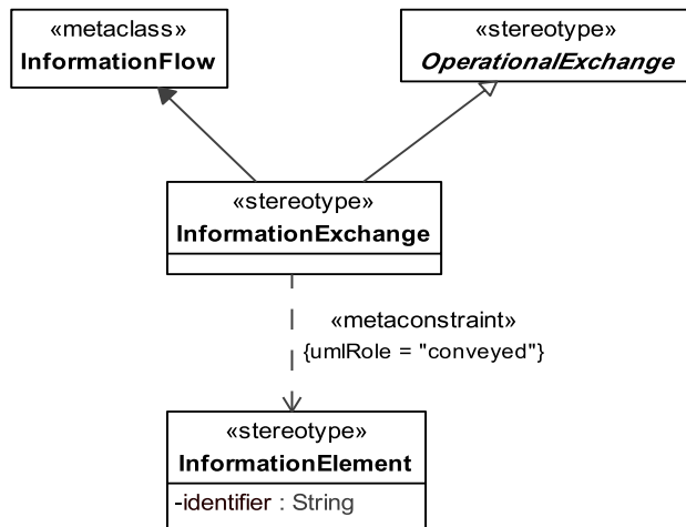
Figure 8.50 - Elements related to the InformationExchange stereotype
