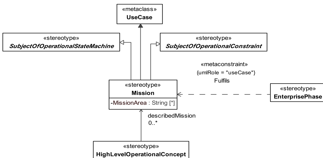
Figure 8.205 - Elements related to the Mission stereotype
