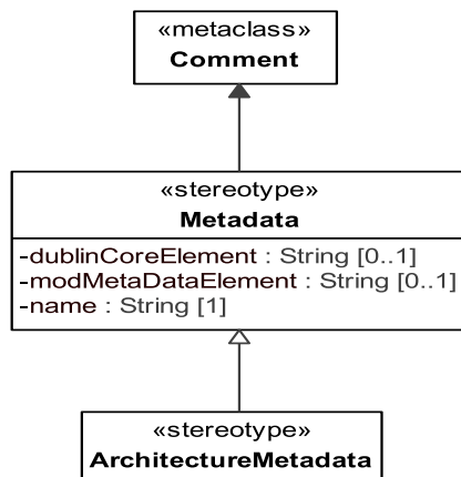
Figure 8.29 - Elements related to the Metadata stereotype
