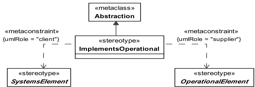
Figure 8.13 - Elements related to the ImplementsOperational stereotype
