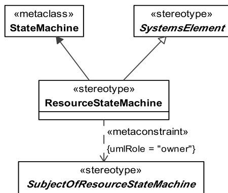
Figure 8.144 - Elements related to the ResourceStateMachine stereotype
