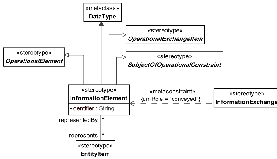
Figure 8.48 - Elements related to the InformationElement stereotype
