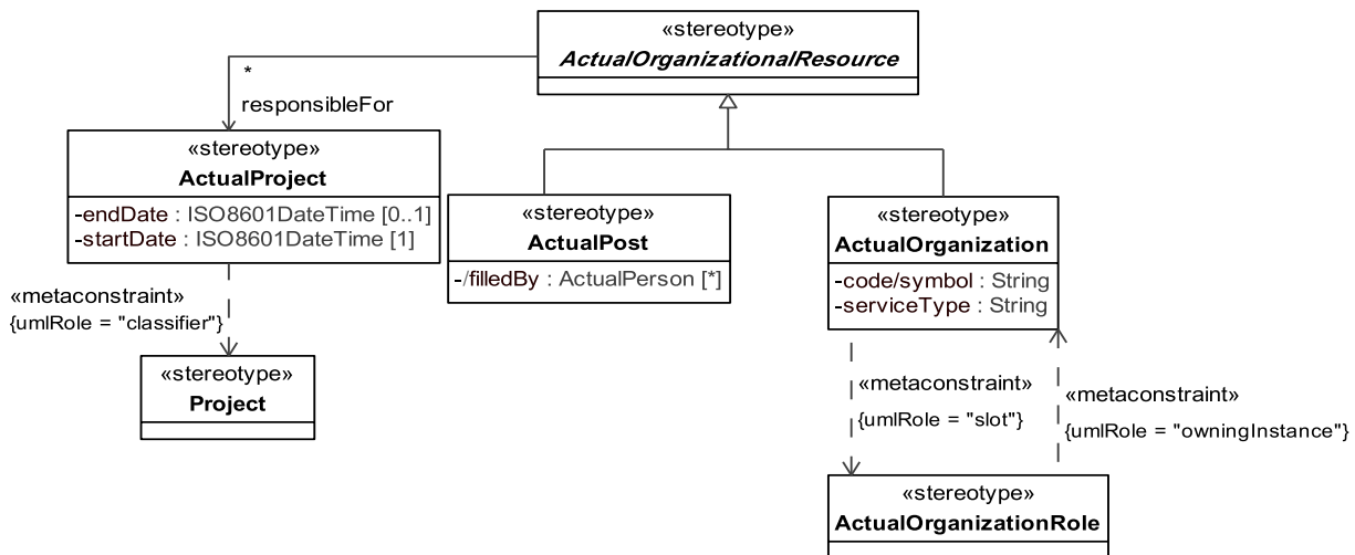
Figure 8.214 - Elements related to the AcV-1 product
