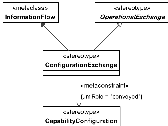
Figure 8.253 - Elements related to the ConfigurationExchange stereotype
