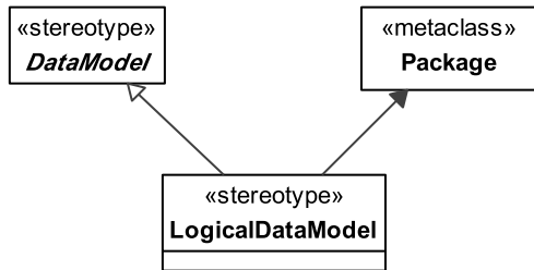
Figure 8.248 - Elements related to the LogicalDataModel stereotype
