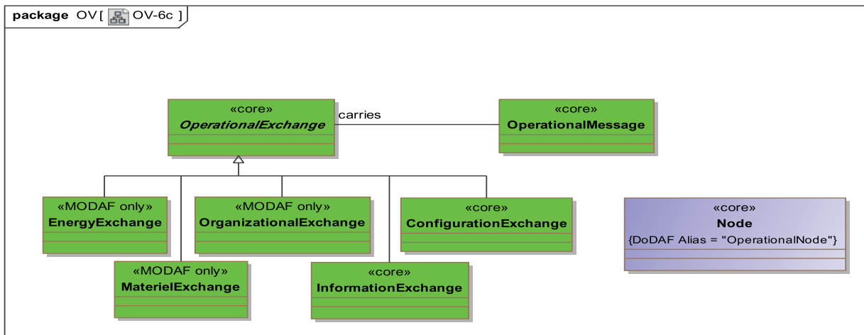
Figure A.21 - OV-6c
