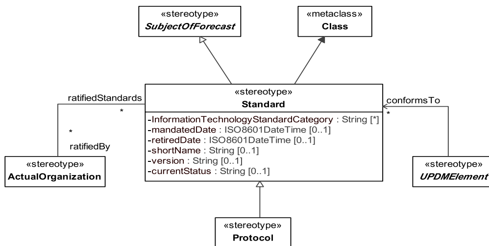
Figure 8.181 - Elements related to the Standard stereotype
