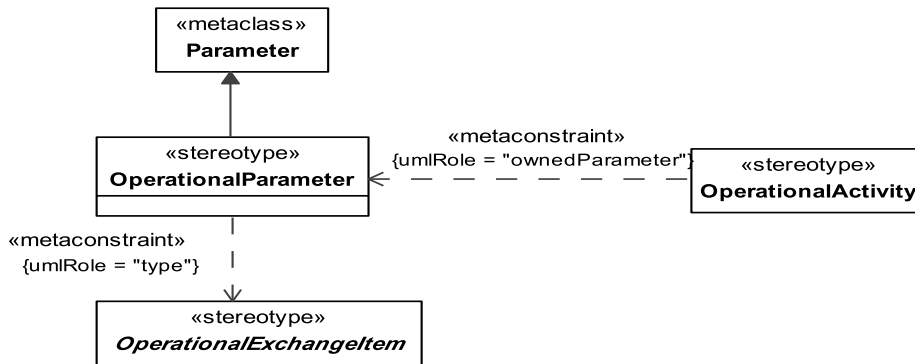
Figure 8.46 - Elements related to the OperationalParameter stereotype
