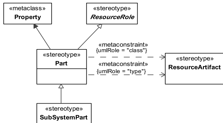
Figure 8.165 - Elements related to the Part stereotype
