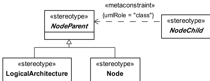
Figure 8.64 - Elements related to the abstract NodeParent stereotype
