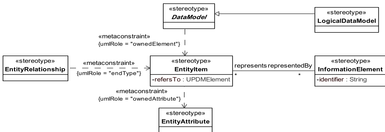
Figure 8.42 - Elements related to the OV-7 product
