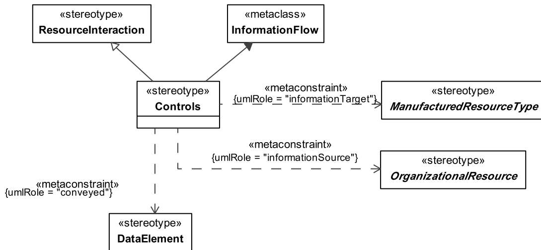
Figure 8.249 - Elements related to the Controls stereotype
