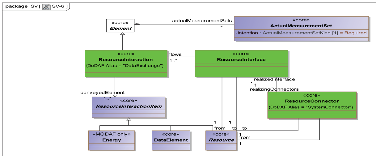
Figure A.48 - SV-6
