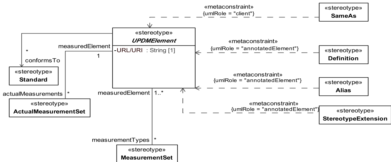
Figure 8.9 - Elements related to the abstract UPDMElement stereotype
