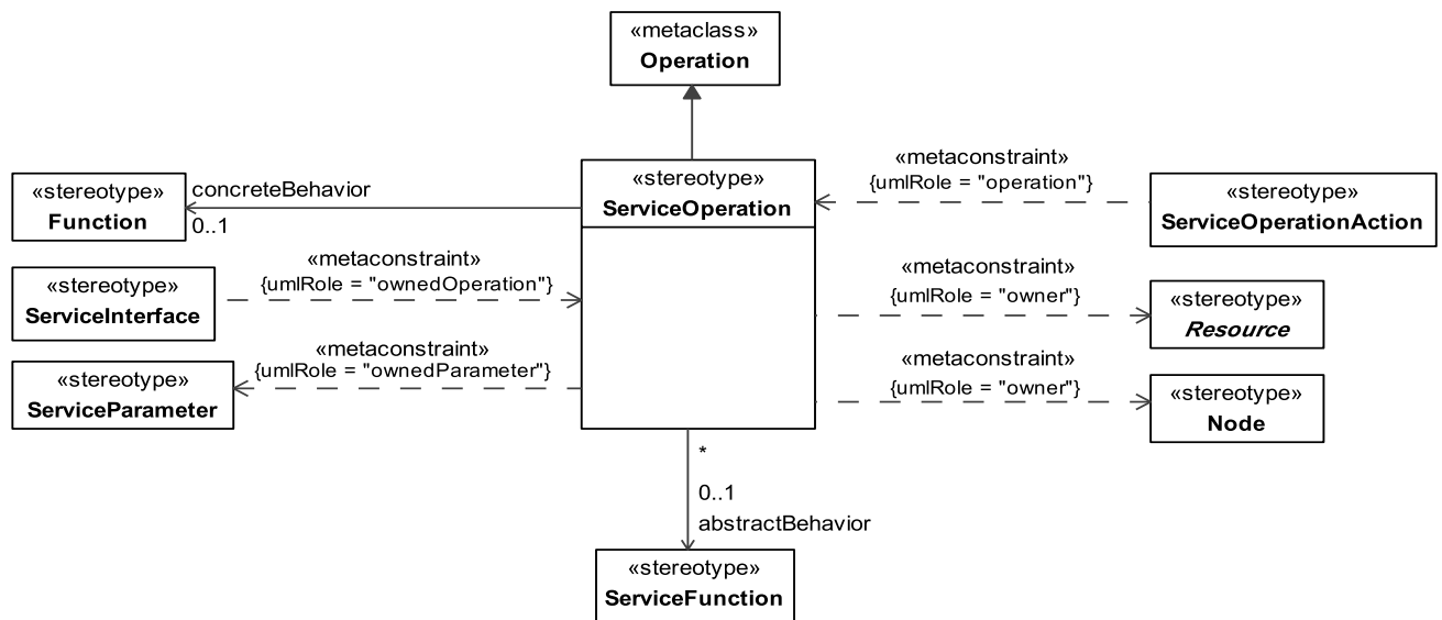
Figure 8.97 - Elements related to the ServiceOperation stereotype
