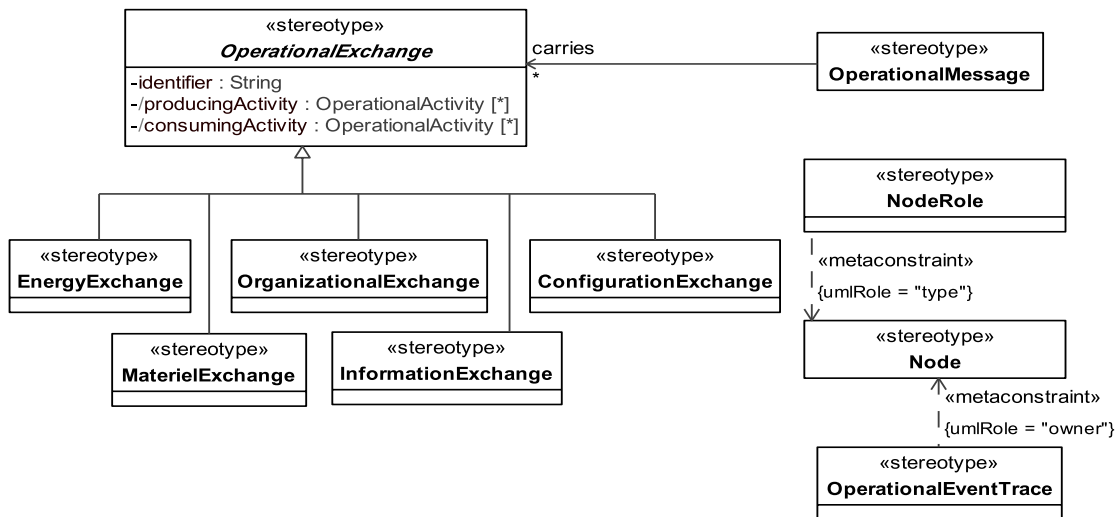
Figure 8.200 - Elements related to the OV-6c product
