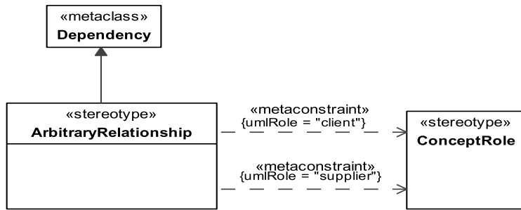
Figure 8.53 - Elements related to the ArbitraryRelationshipConnector stereotype
