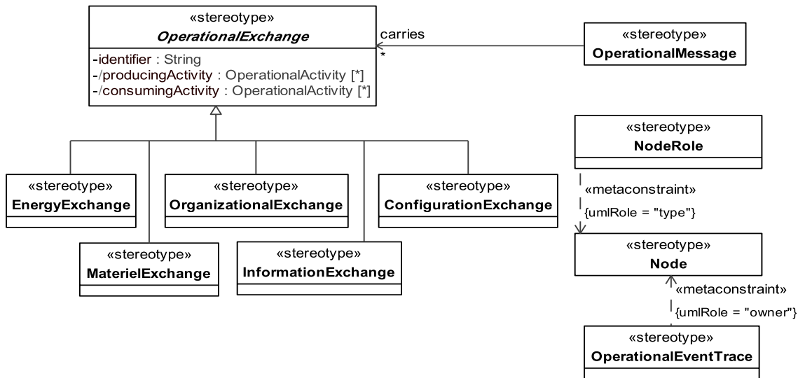
Figure 8.41 - Elements related to the OV-6c product
