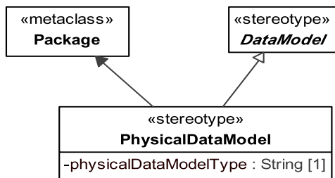
Figure 8.148 - Elements related to the PhysicalDataModel stereotype
