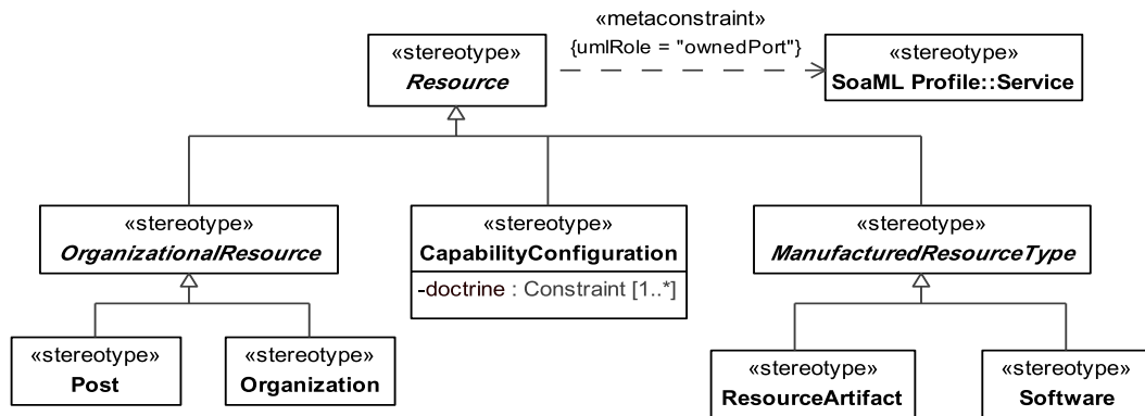
Figure 8.131 - Elements related to the SV-12 product
