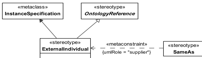
Figure 8.230 - Elements related to the ExternalIndividual stereotype
