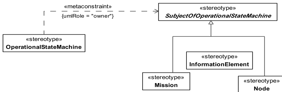
Figure 8.243 - Elements related to the OV-6b stereotype
