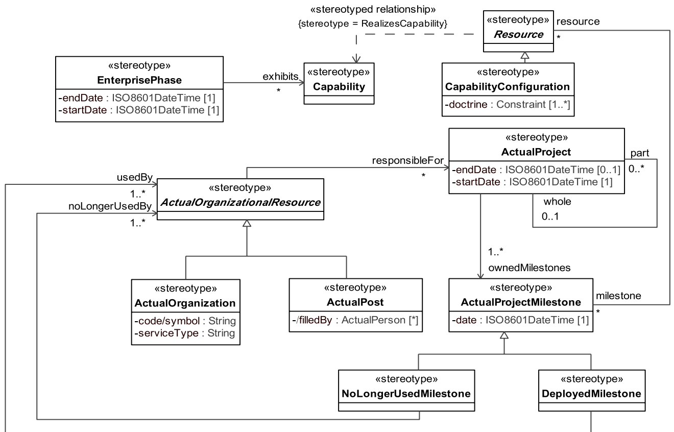
Figure 8.111 - Elements related to the StV-5 product
