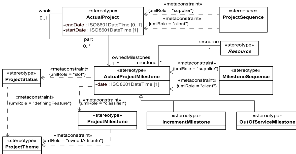
Figure 8.3 - Elements related to the AcV-2 Product
