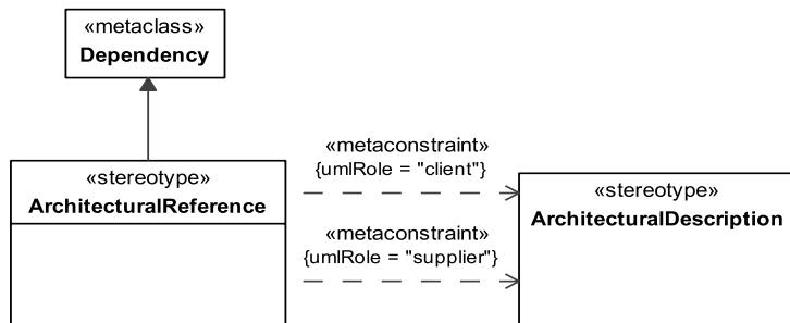
Figure 8.26 - Elements related to the ArchitecturalReference stereotype
