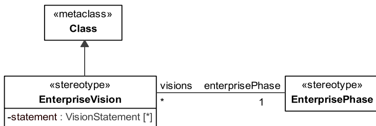
Figure 8.117 - Elements related to the EnterpriseVision stereotype
