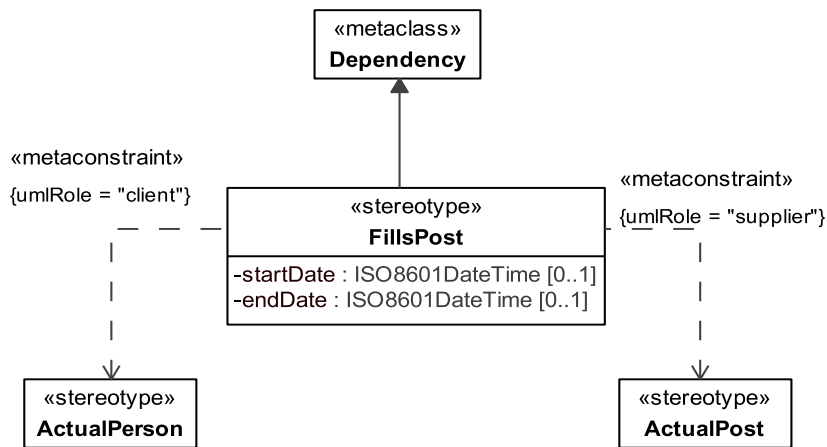
Figure 8.79 - Elements related to the FillsPost stereotype
