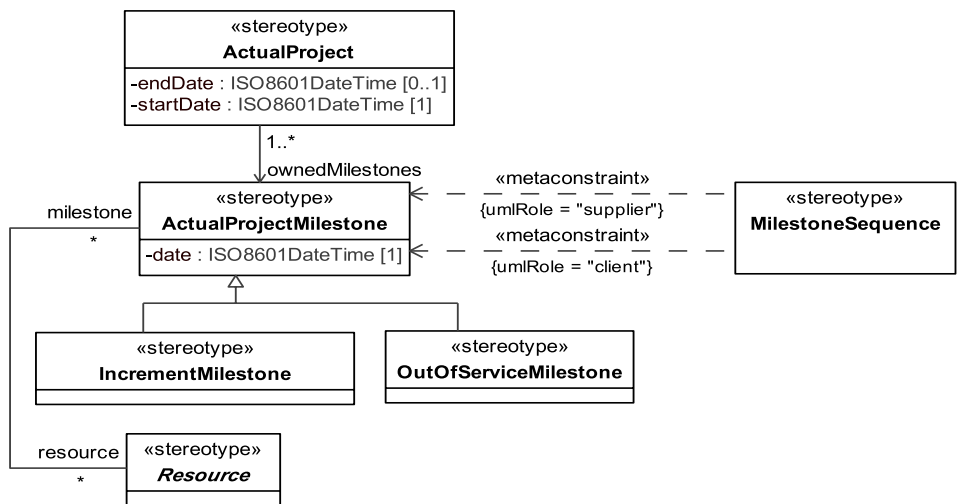
Figure 8.138 - Elements related to the SV-8 product
