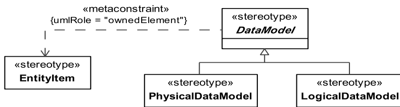
Figure 8.147 - Elements related to the abstract DataModel stereotype
