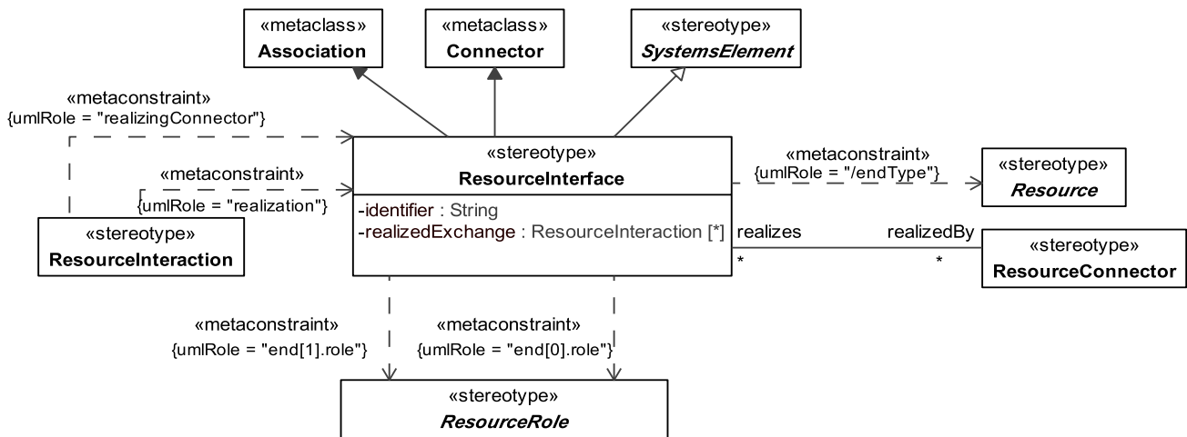
Figure 8.168 - Elements related to the ResourceInterface stereotype
