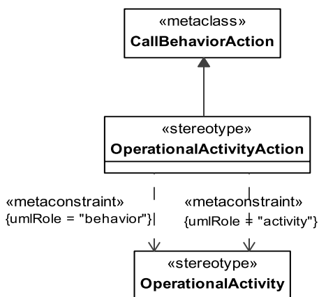
Figure 8.44 - Elements related to the OperationalActivityAction stereotype
