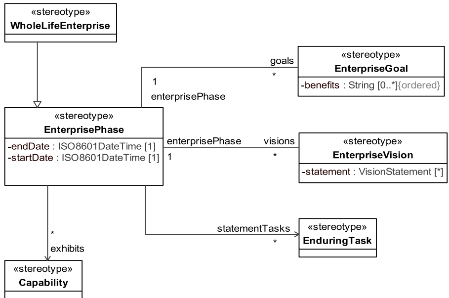
Figure 8.107 - Elements related to the StV-1 product
