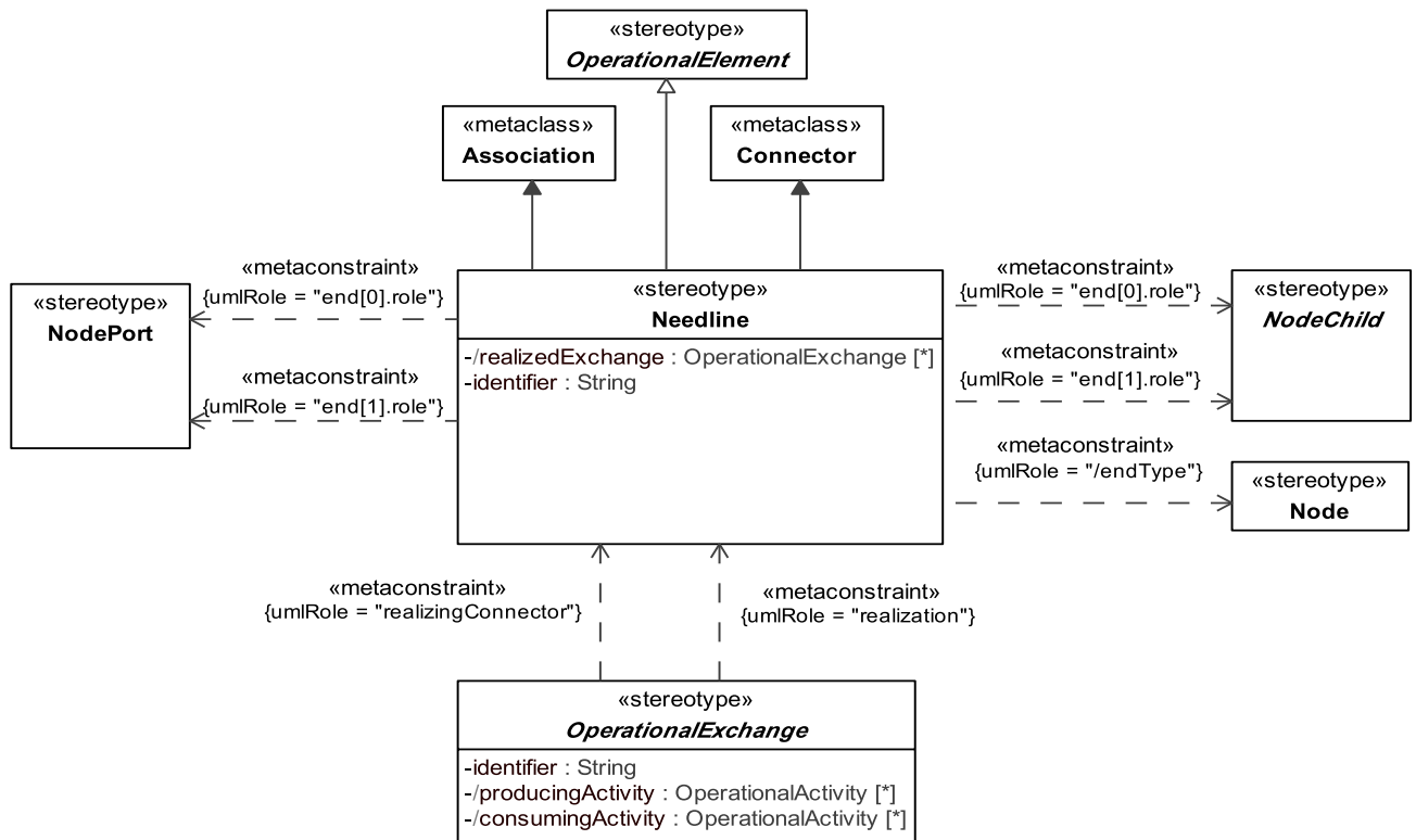
Figure 8.61 - Elements related to the Needline stereotype
