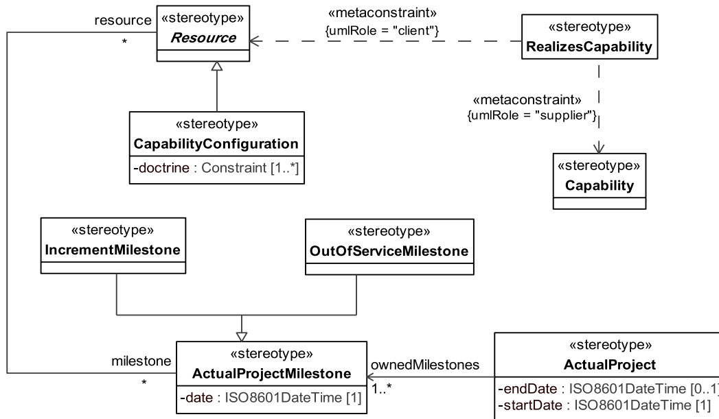
Figure 8.109 - Elements related to the StV-3 product
