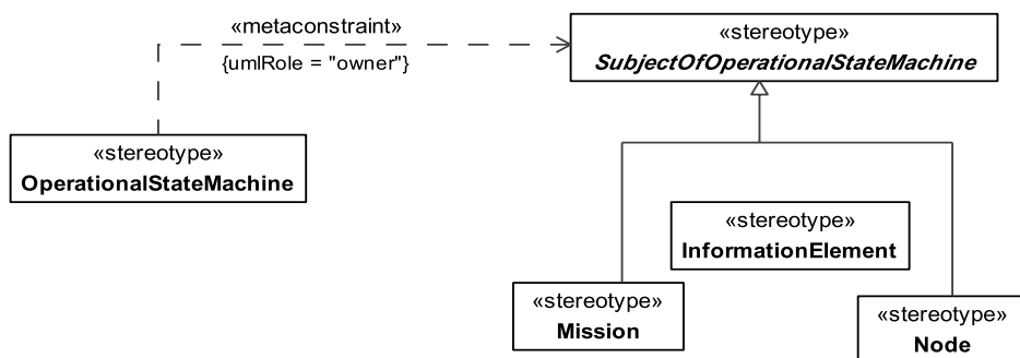
Figure 8.199 - Elements related to the OV-6b product
