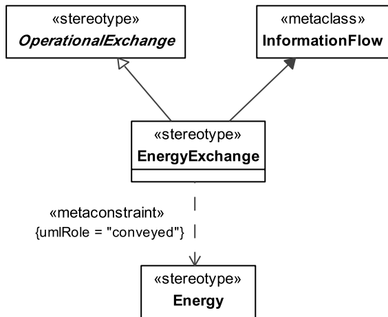
Figure 8.250 - Elements related to the EnergyExchange stereotype
