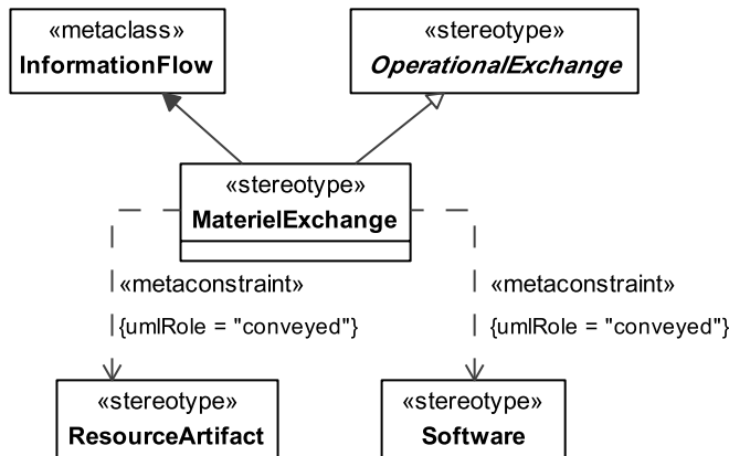
Figure 8.251 - Elements related to the MaterielExchange stereotype
