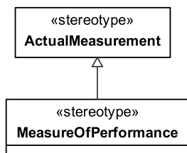
Figure 8.189 - Elements related to the MeasureOfPerformance stereotype
