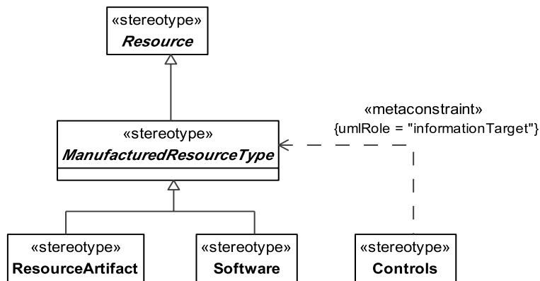
Figure 8.164 - Elements related to the abstract ManufacturedResourceType stereotype
