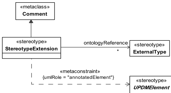
Figure 8.234 - Elements related to the StereotypeExtension stereotype
