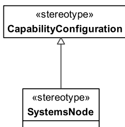
Figure 8.176 - Elements related to the SystemsNode stereotype
