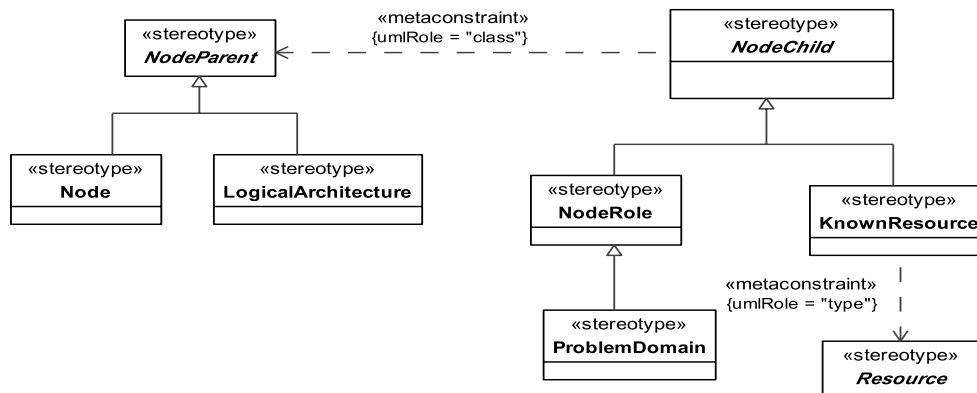
Figure 8.237 - Elements related to the OV-2 Nodes stereotype
