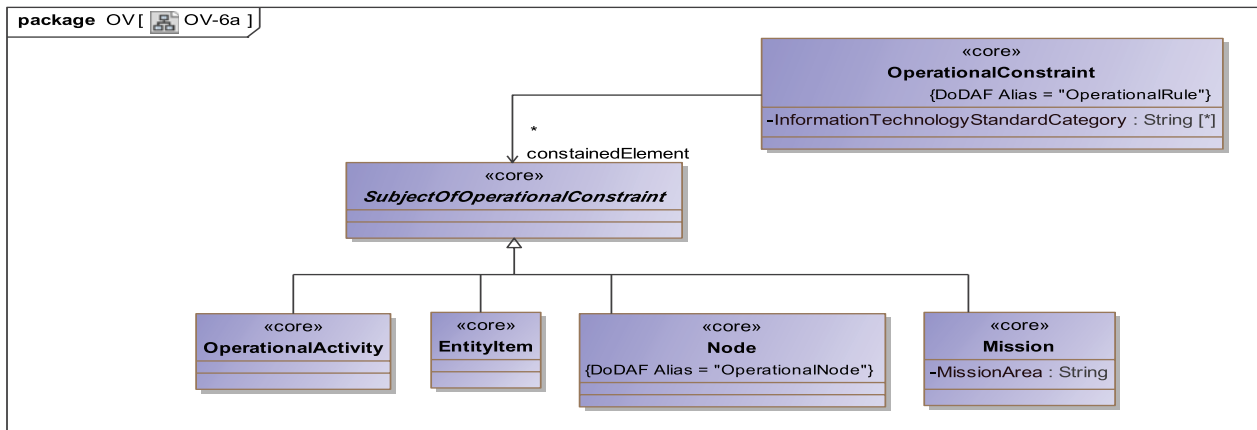
Figure A.19 - OV-6a
