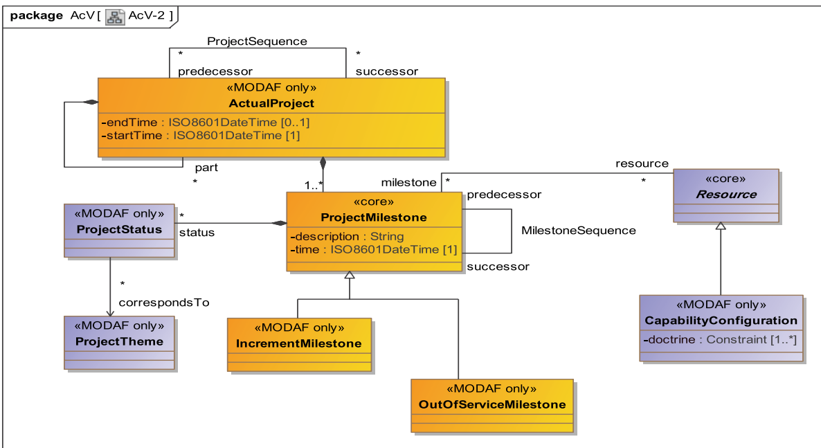
Figure A.2 - AcV-2
