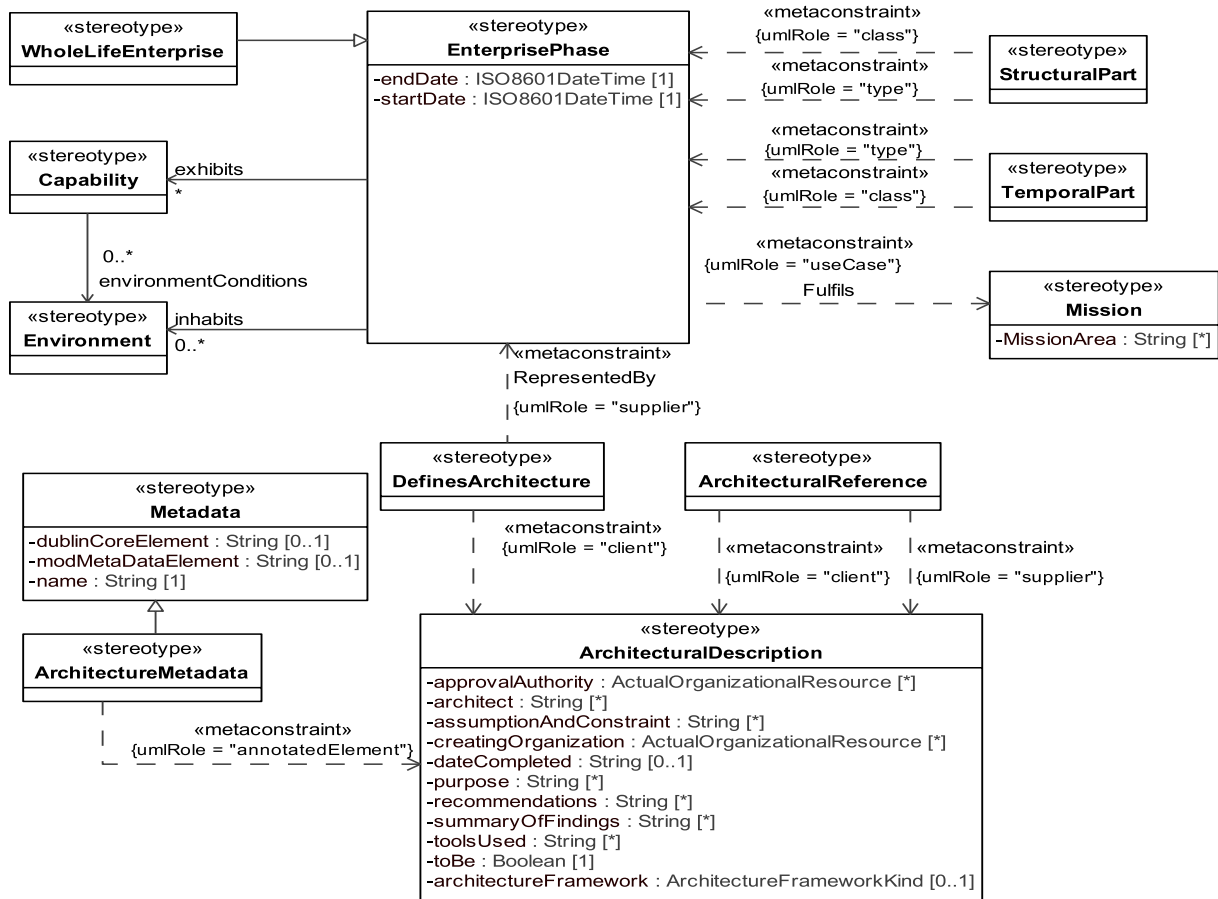
Figure 8.6 - Elements related to the AV-1 Product
