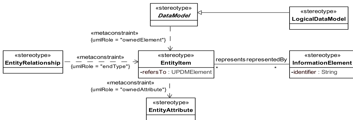
Figure 8.245 - Elements related to the OV-7 stereotype
