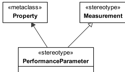
Figure 8.190 - Elements related to the PerformanceParameter stereotype
