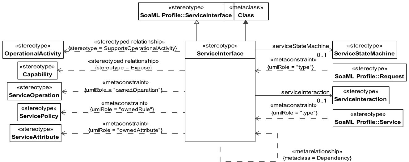
Figure 8.104 - Elements related to the ServiceInterface stereotype
