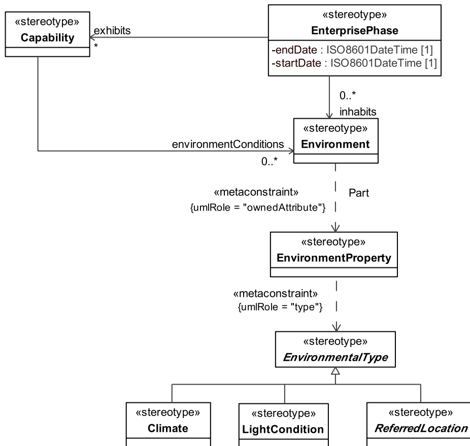
Figure 8.258 - Elements related to the StV-2 stereotype
