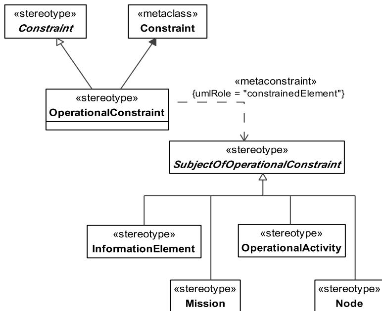
Figure 8.67 - Elements related to the OperationalConstraint stereotype
