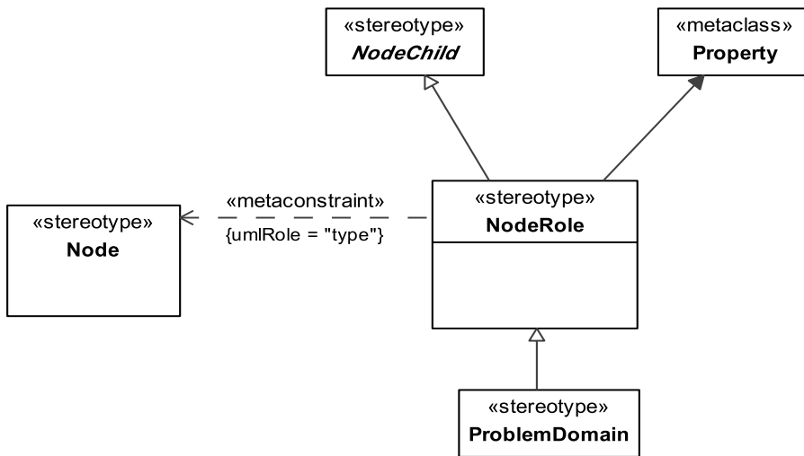
Figure 8.66 - Elements related to the NodeRole stereotype
