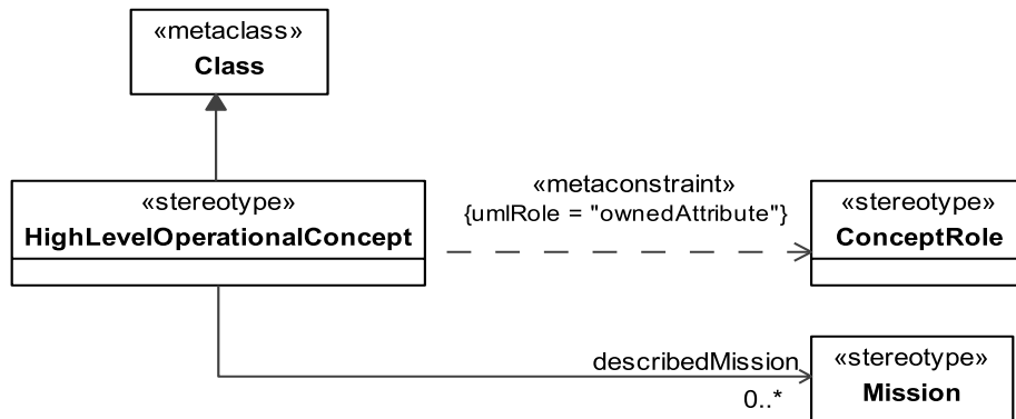
Figure 8.57 - Elements related to the HighLevelOperationalConcept stereotype
