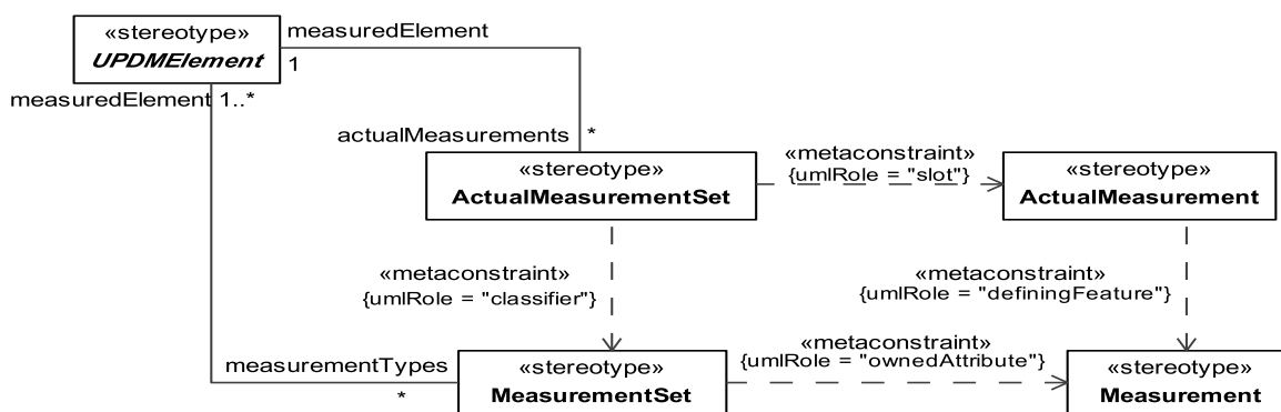
Figure 8.188 - Elements related to the AV-3 product
