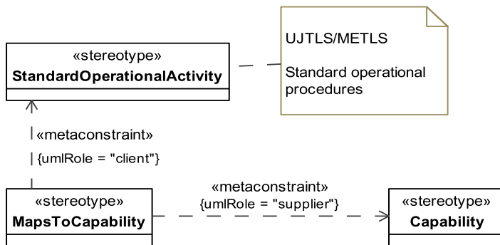
Figure 8.112 - Elements related to the StV-6 product
