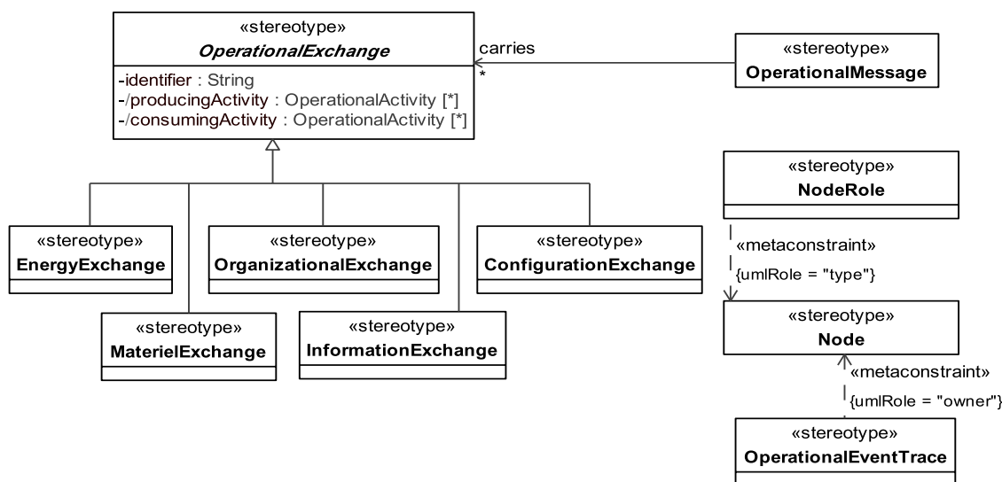
Figure 8.244 - Elements related to the OV-6c stereotype
