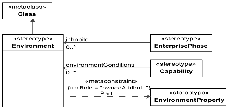
Figure 8.16 - Elements related to the Environment stereotype
