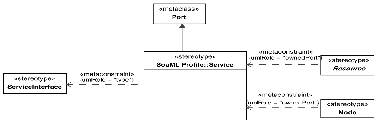
Figure 8.102 - Elements related to the Service stereotype
