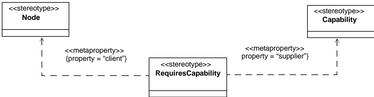
Figure 7.8 - UML Dependency metaclass
