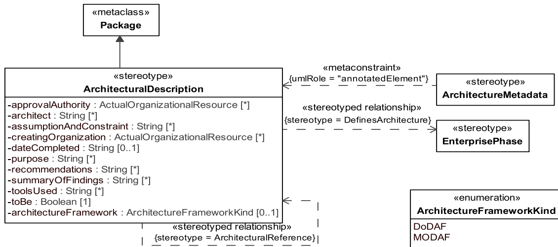
Figure 8.25 - Elements related to the ArchitecturalDescription stereotype
