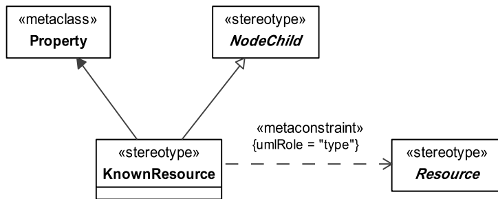
Figure 8.59 - Elements related to the KnownResource stereotype
