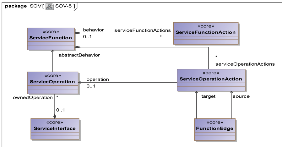
Figure A.30 - SOV-5
