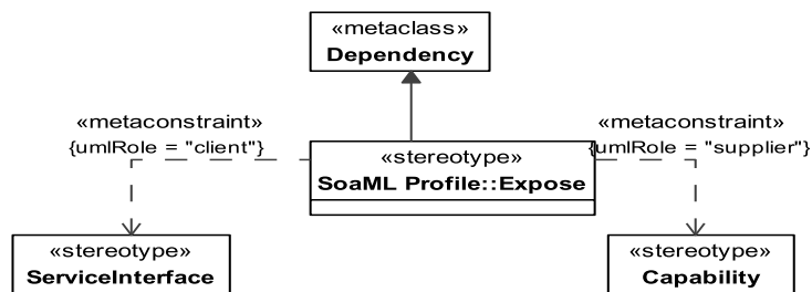
Figure 8.124 - Elements related to the Expose stereotype
