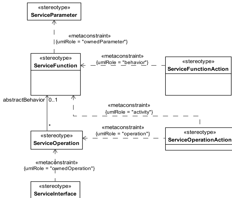
Figure 8.93 - Elements related to the SOV-5 product
