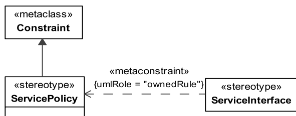
Figure 8.105 - Elements related to the ServicePolicy stereotype
