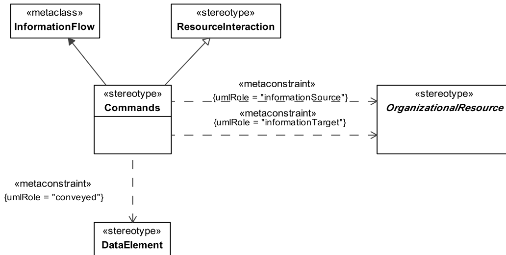
Figure 8.49 - Elements related to the Commands stereotype
