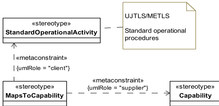
Figure 8.261 - Elements related to the StV-6 stereotype
