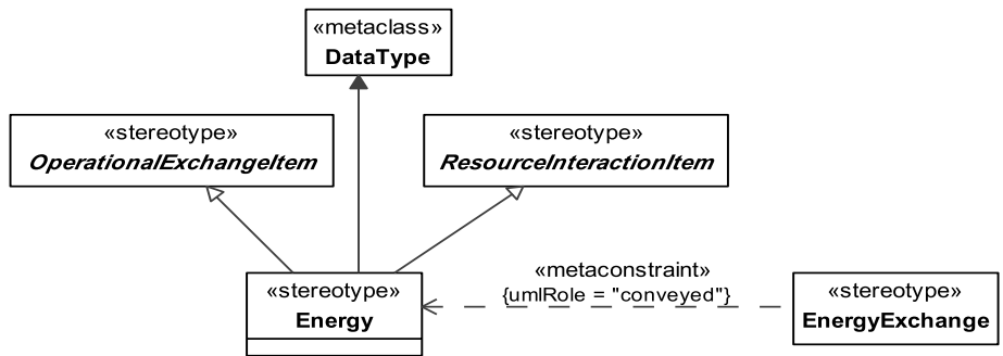
Figure 8.254 - Elements related to the Energy stereotype
