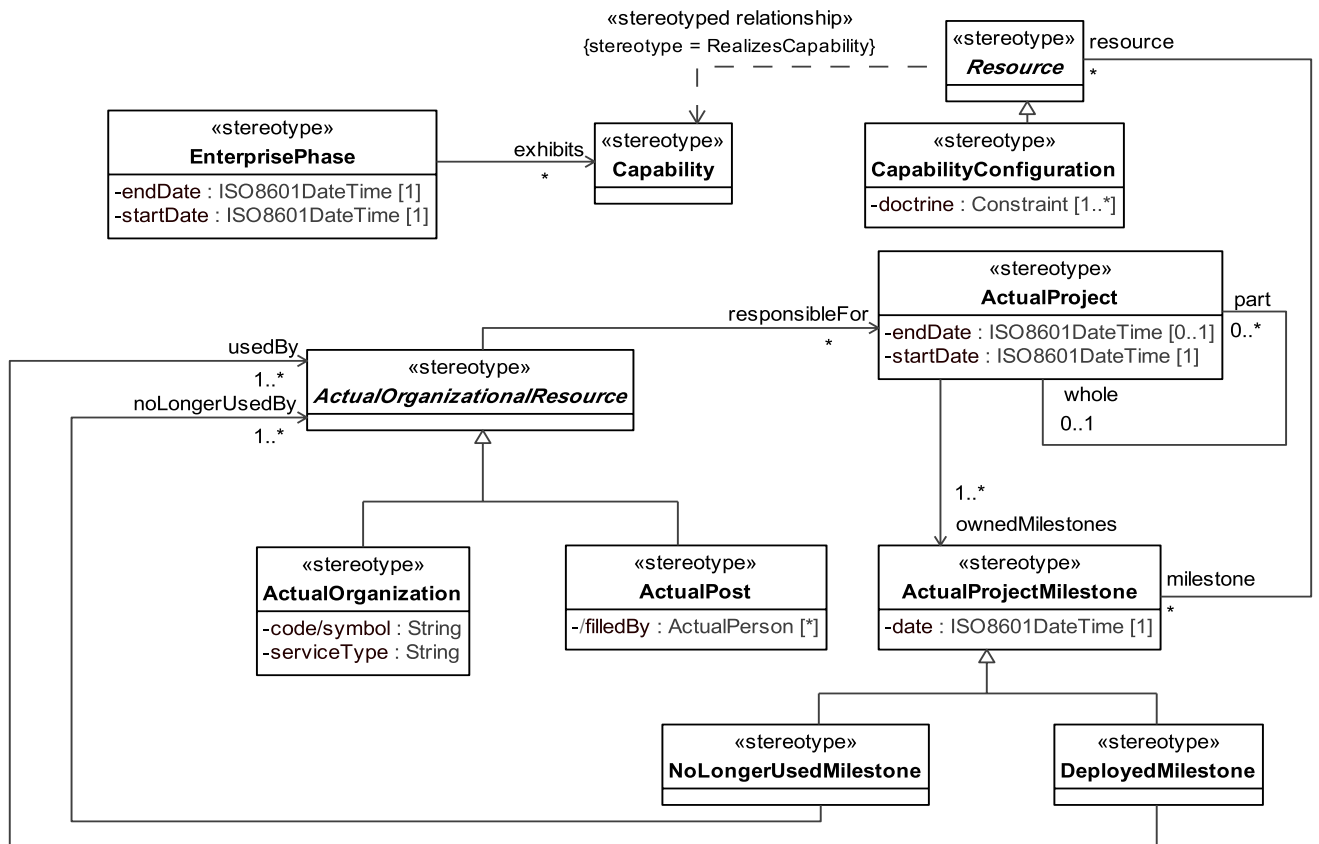
Figure 8.260 - Elements related to the StV-5 stereotype
