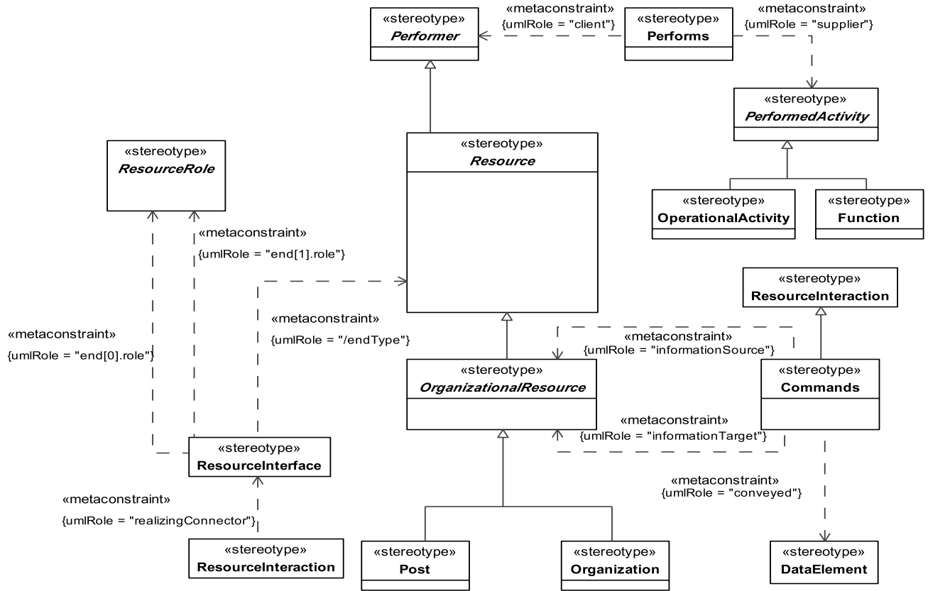
Figure 8.37 - Elements related to the OV-4 Typical product
