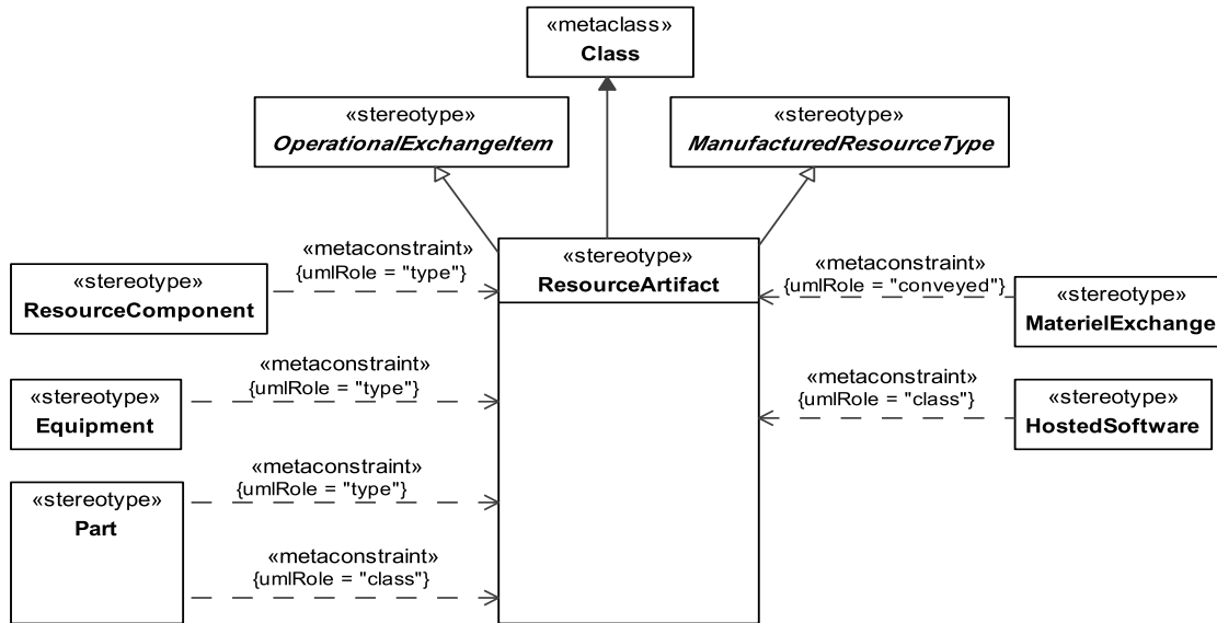
Figure 8.156 - Elements related to the ResourceArtifact stereotype
