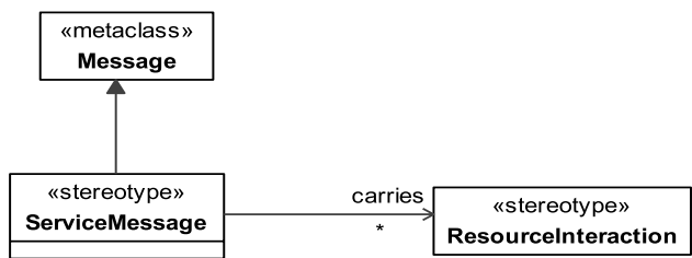
Figure 8.153 - Elements related to the ServiceMessage stereotype
