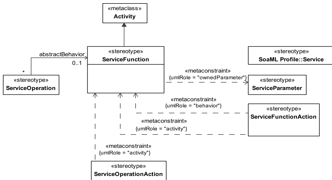
Figure 8.94 - Elements related to the ServiceFunction stereotype
