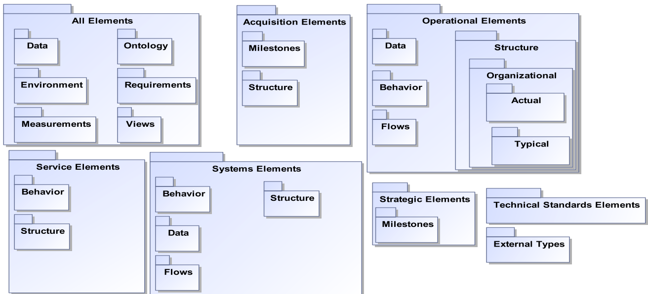
Figure A.23 - Package Structure
