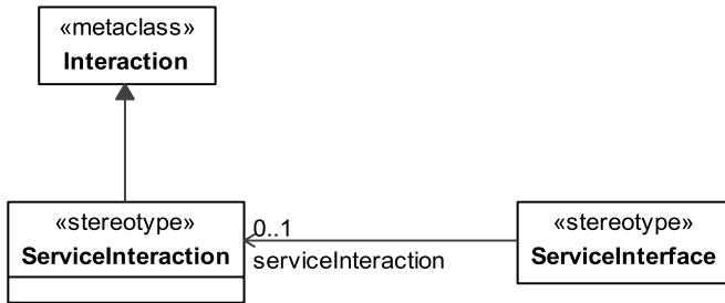
Figure 8.96 - Elements related to the ServiceInteraction stereotype
