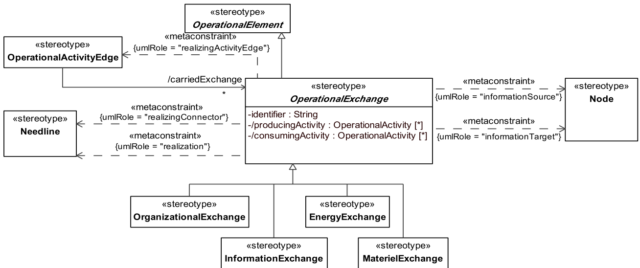
Figure 8.51 - Elements related to the abstract OperationalExchange stereotype
