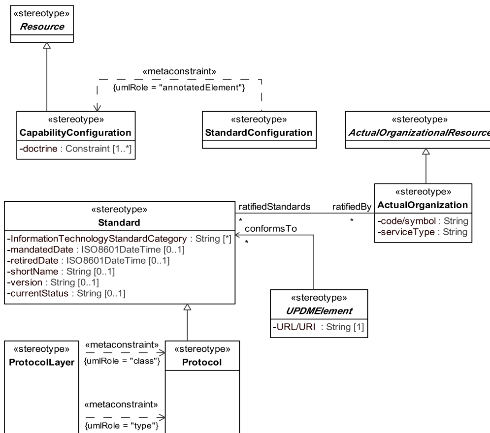
Figure 8.178 - Elements related to the TV-1&2&3 products
