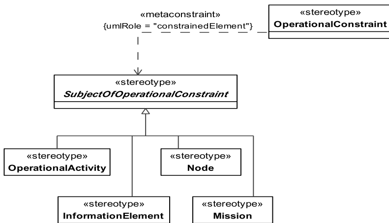
Figure 8.39 - Elements related to the OV-6a product
