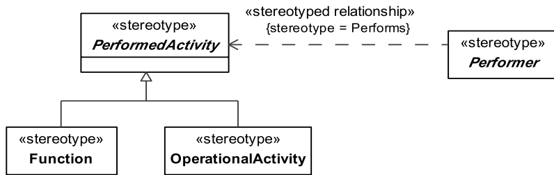
Figure 8.10 - Elements related to the abstract Activity stereotype
