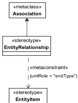
Figure 8.183 - Elements related to the EntityRelationship stereotype
