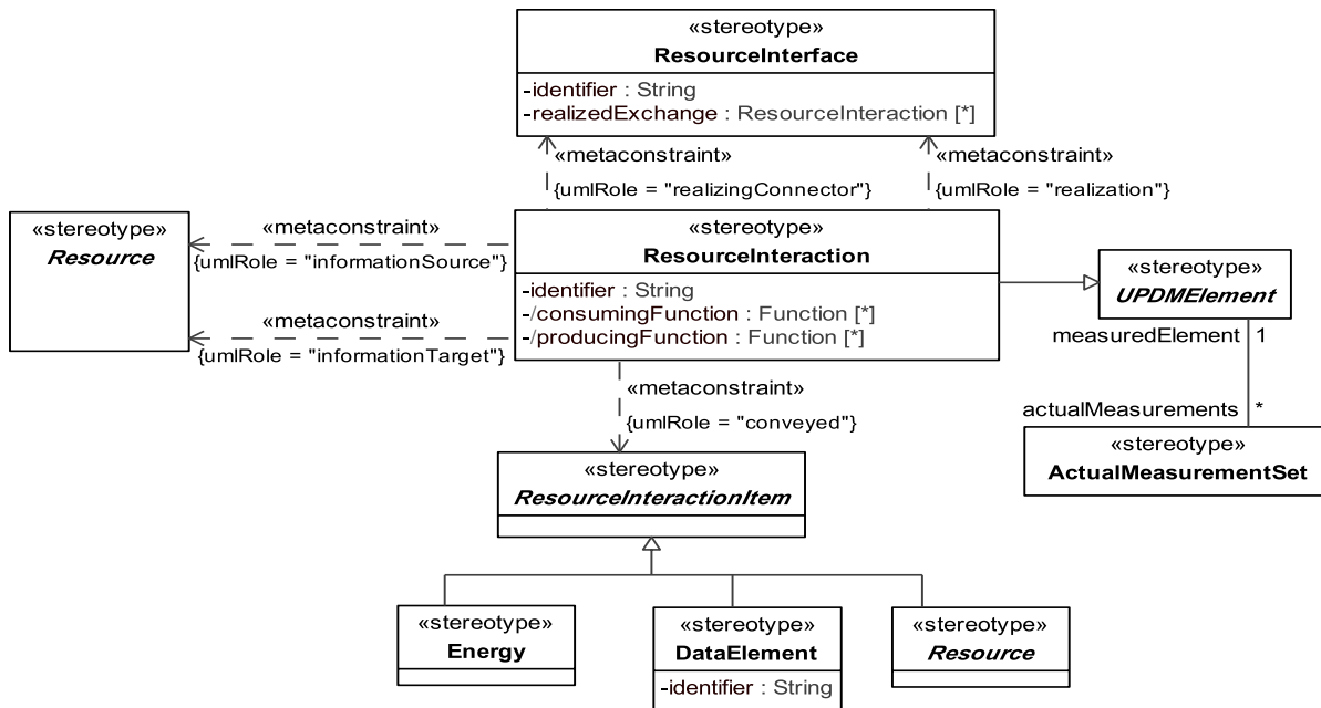
Figure 8.136 - Elements related to the SV-6 product
