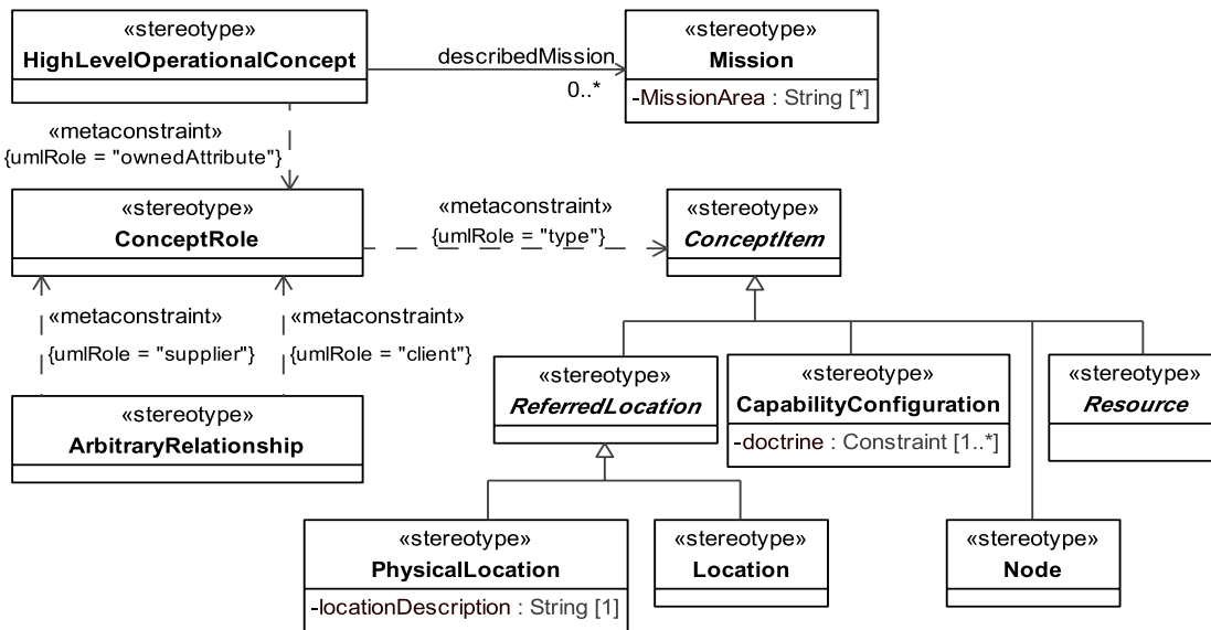
Figure 8.235 - Elements related to the OV-1 stereotype
