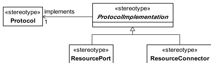
Figure 8.180 - Elements related to the abstract ProtocolImplementation stereotype
