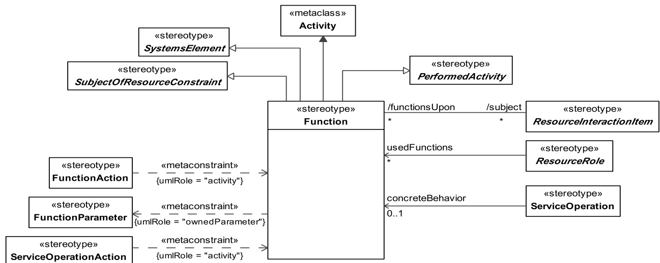
Figure 8.140 - Elements related to the Function stereotype
