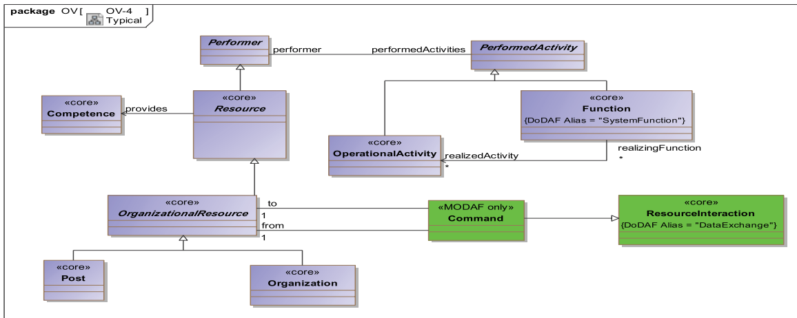
Figure A.17 - OV-4 Typical
