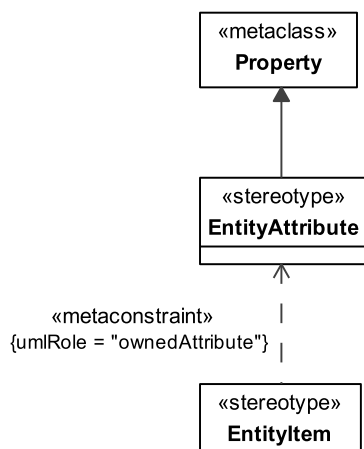
Figure 8.184 - Elements related to the EntityAttribute stereotype
