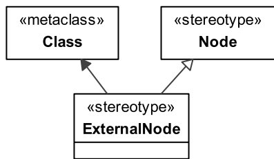
Figure 8.204 - Elements related to the ExternalNode stereotype
