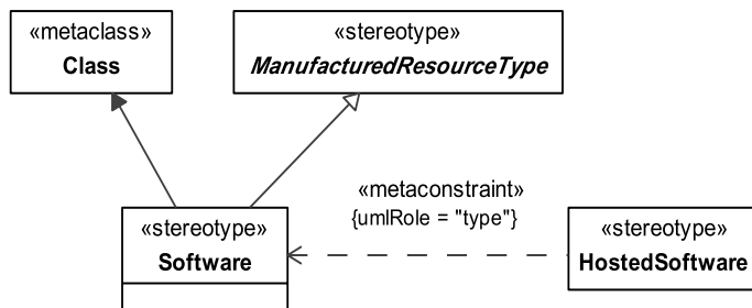
Figure 8.172 - Elements related to the Software stereotype
