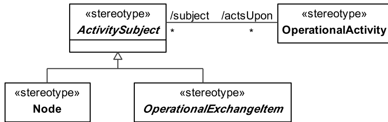
Figure 8.246 - Elements related to the abstract ActivitySubject stereotype
