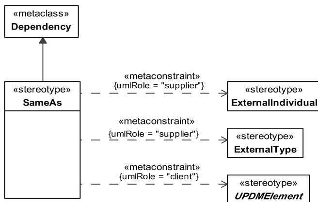
Figure 8.233 - Elements related to the SameAs stereotype
