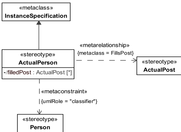
Figure 8.77 - Elements related to the ActualPerson stereotype
