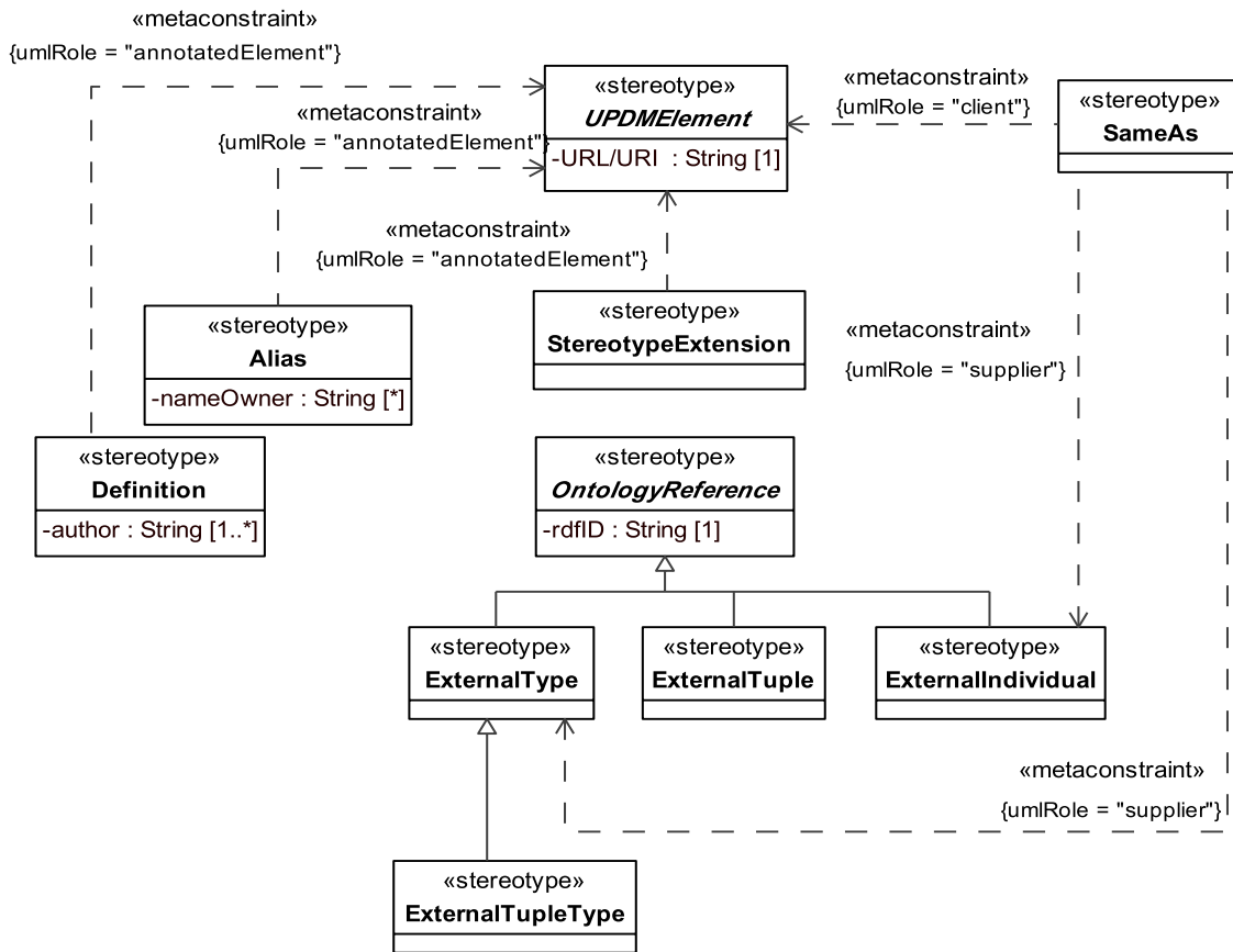
Figure 8.187 - Elements related to the AV-2 product
