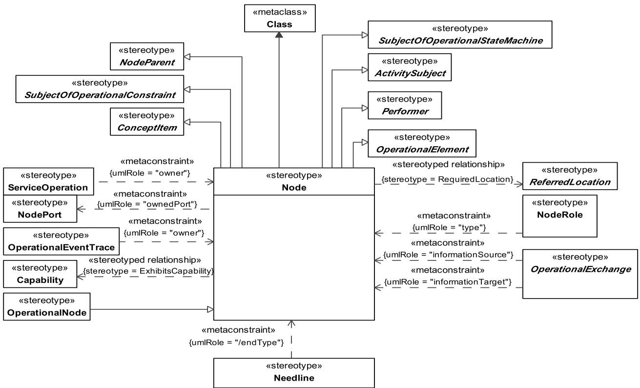
Figure 8.62 - Elements related to the Node stereotype
