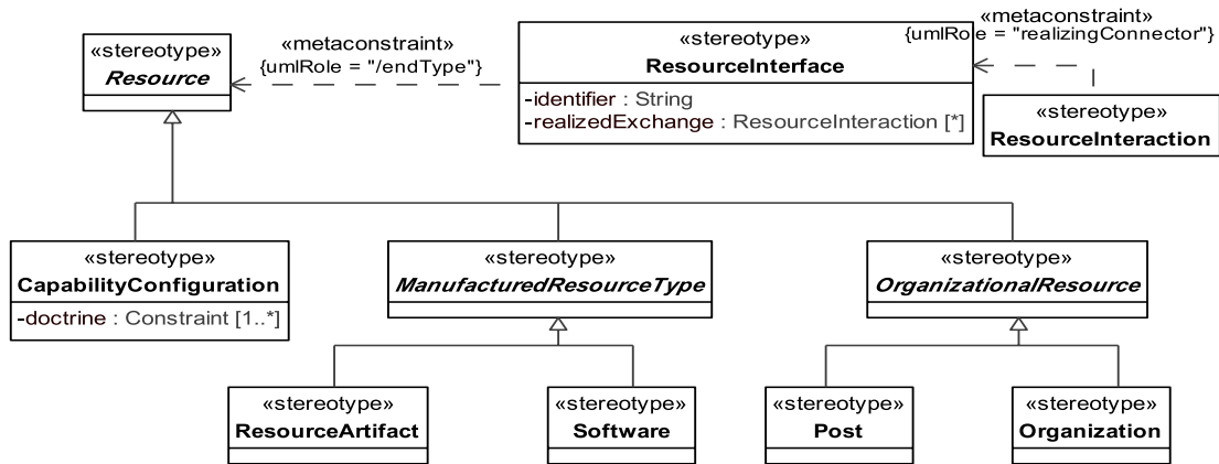
Figure 8.133 - Elements related to the SV-3 product
