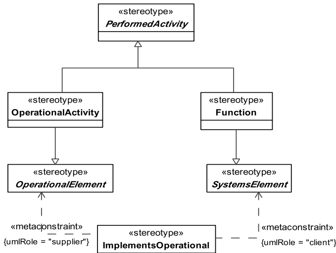
Figure 8.135 - Elements related to the SV-5 product
