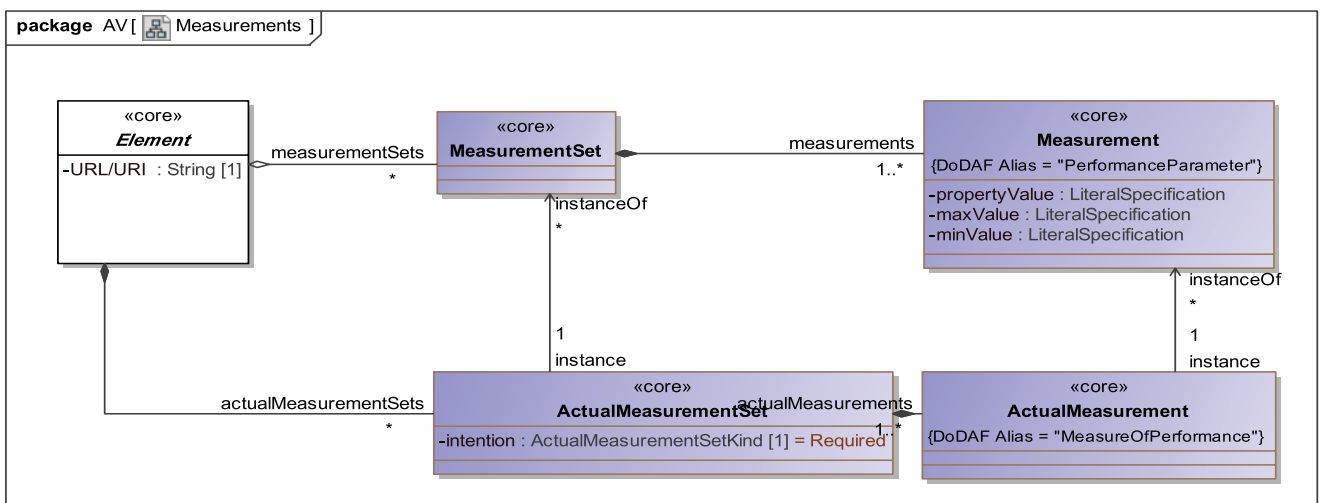
Figure A.5 - AV-3 Measurements
