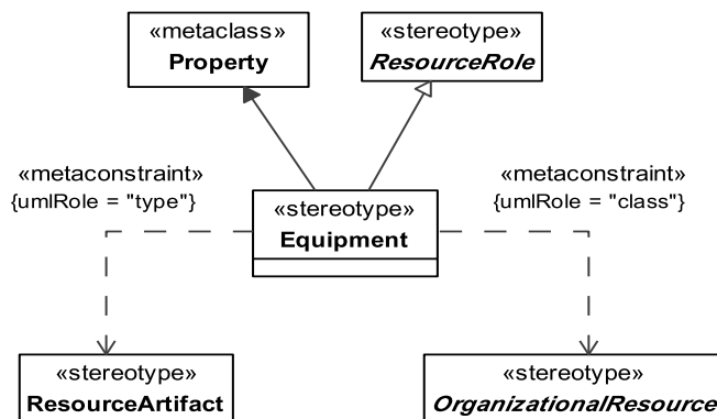
Figure 8.159 - Elements related to the Equipment stereotype
