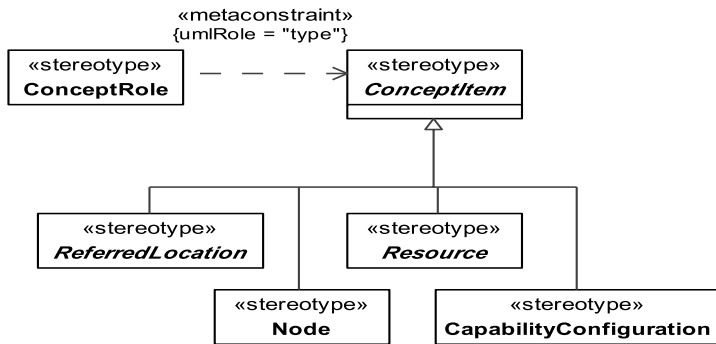
Figure 8.56 - Elements related to the abstract ConceptItem stereotype
