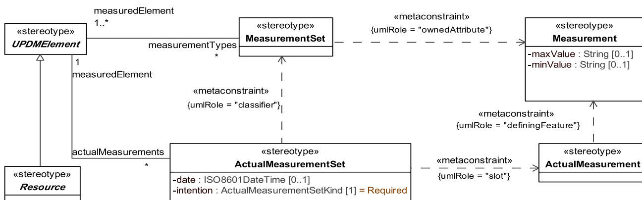
Figure 8.137 - Elements related to the SV-7 product
