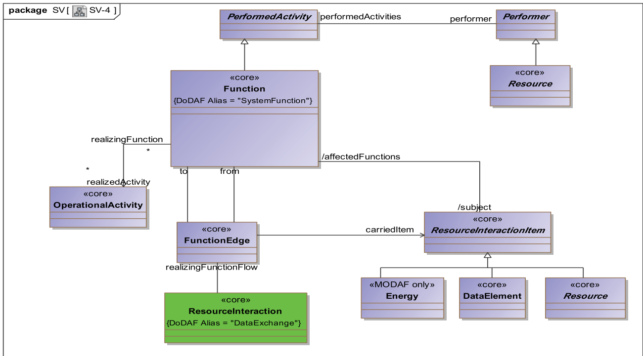
Figure A.46 - SV-4
