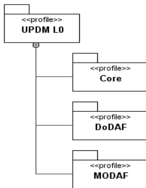
Figure 7.1 - Top Level Profile Structure
