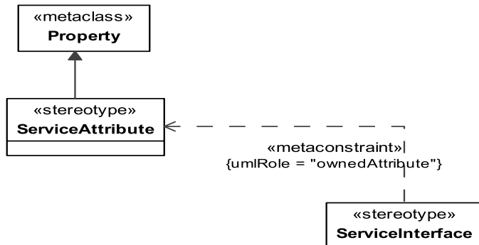
Figure 8.103 - Elements related to the ServiceAttribute stereotype
