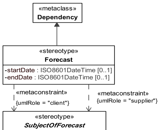
Figure 8.161 - Elements related to the Forecast stereotype
