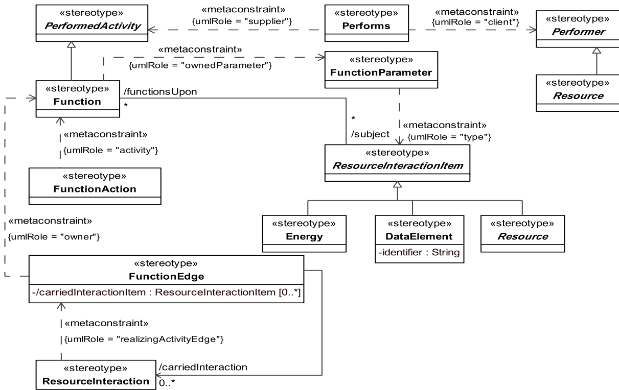
Figure 8.134 - Elements related to the SV-4 product
