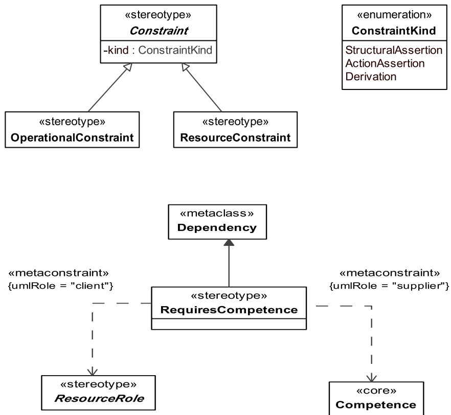
Figure 8.86 - Elements related to the abstract Constraint stereotype
