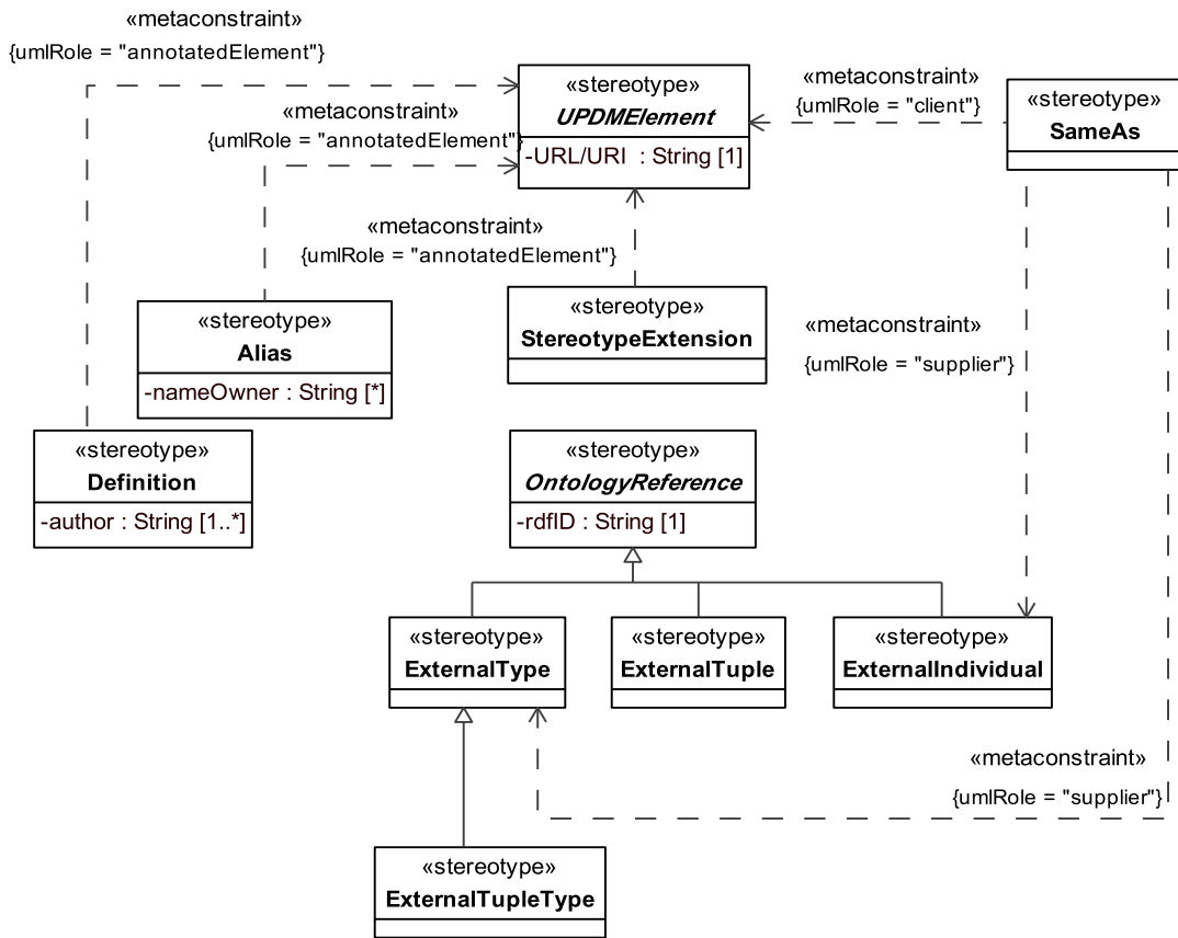
Figure 8.226 - Elements related to the AV-2 product
