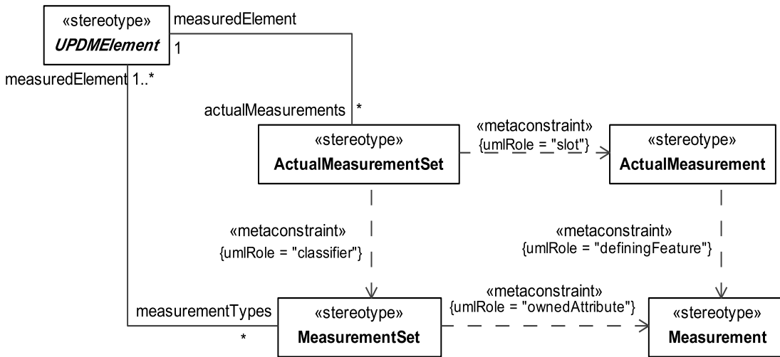
Figure 8.8 - Elements related to the AV-3 product
