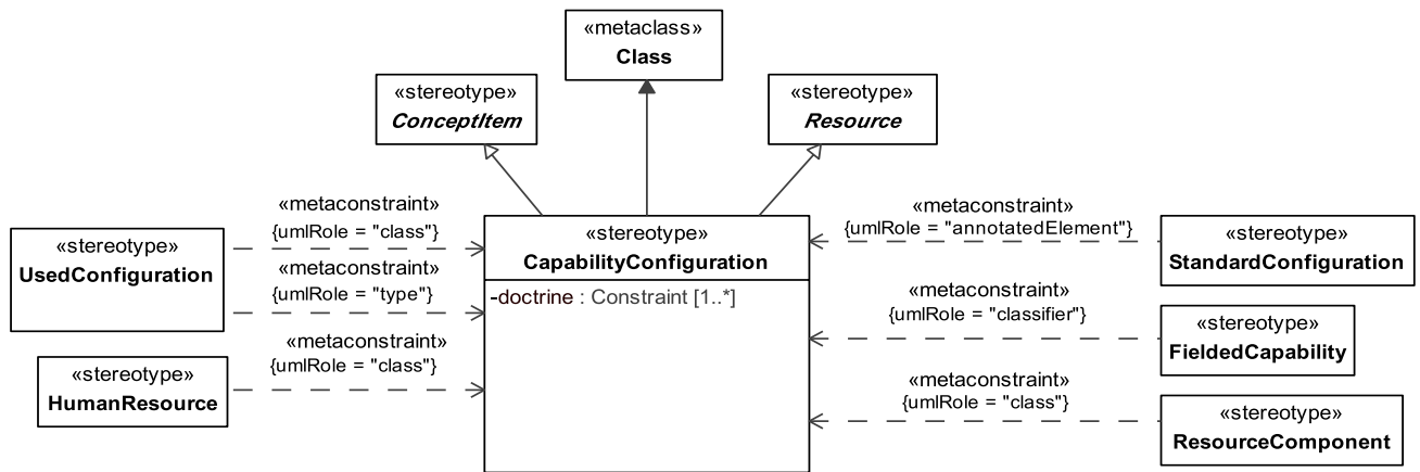
Figure 8.157 - Elements related to the CapabilityConfiguration stereotype
