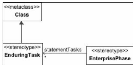
Figure 8.263 - Elements related to the EnduringTask stereotype
