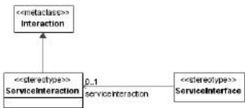
Figure 8.96 - Elements related to the ServiceInteraction stereotype
