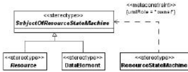
Figure 8.145 - Elements related to the abstract SubjectOfResourceStateMachine stereotype
