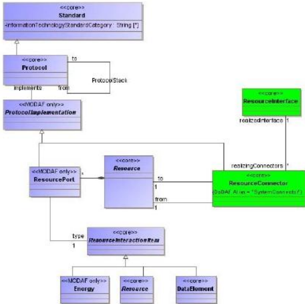
Figure A.44 - SV-2
