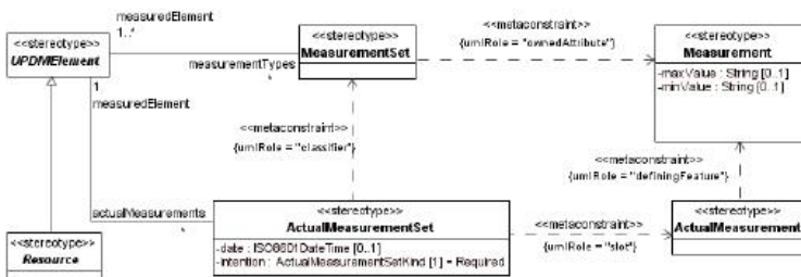
Figure 8.137 - Elements related to the SV-7 product
