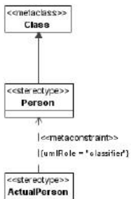
Figure 8.78 - Elements related to the Person stereotype
