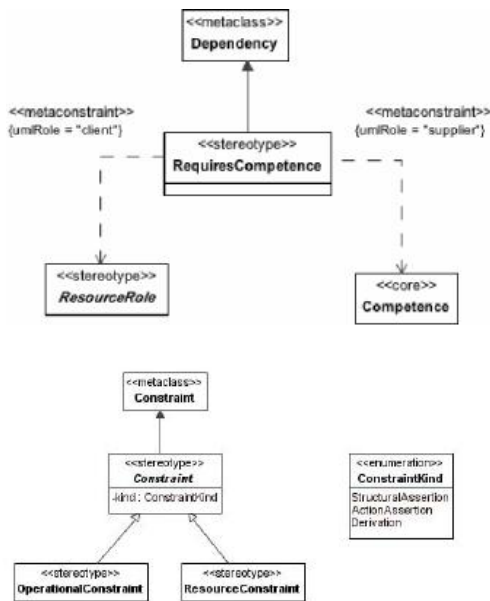
Figure 8.86 - Elements related to the abstract Constraint stereotype
