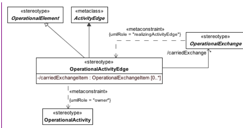
Figure 8.45 Elements related to the OperationalActivityEdge Stereotype.
