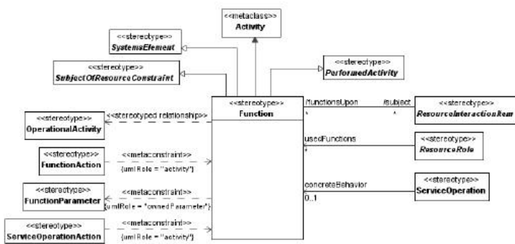
Figure 8.140 - Elements related to the Function stereotype
