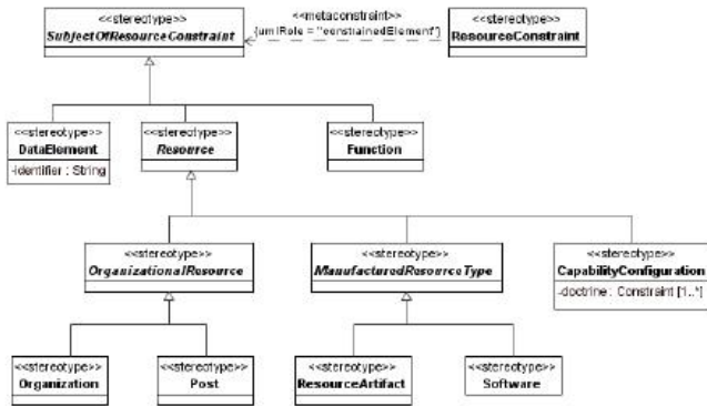
Figure 8.127 - Elements related to the SV-10a product
