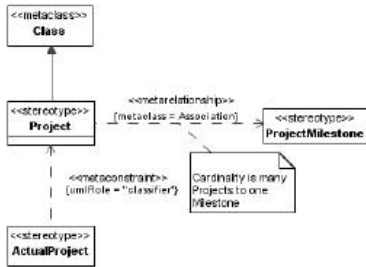
Figure 8.222 - Elements related to the Project stereotype
