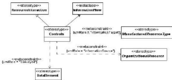
Figure 8.248 - Elements related to the Controls stereotype
