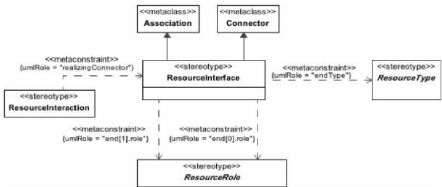
Figure 8.168 - Elements related to the ResourceInterface stereotype
