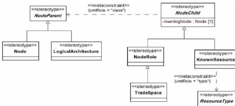
Figure 8.34 - Elements related to the OV-2 Nodes stereotype
