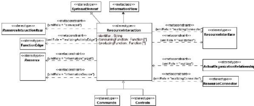
Figure 8.150 - Elements related to the ResourceInteraction stereotype
