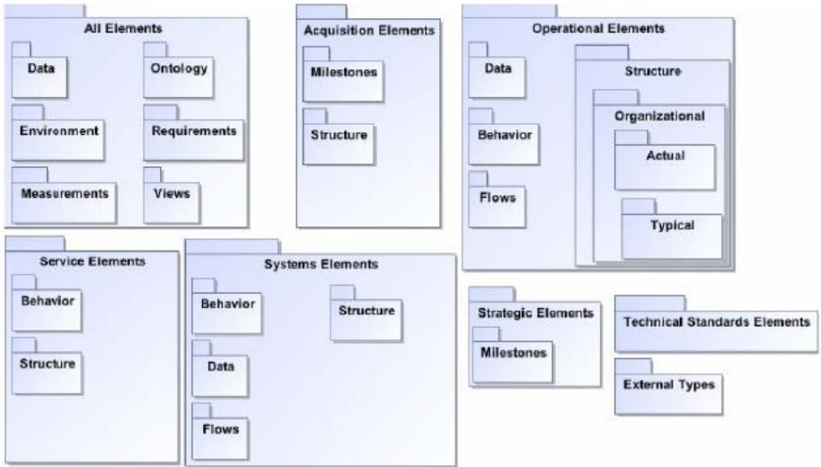
Figure A.23 - Package Structure
