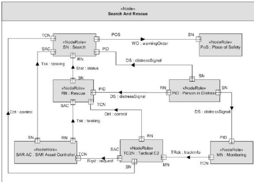
Figure C.15 - Alternate OV-2 with SysML Flow Ports
