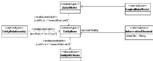
Figure 8.42 - Elements related to the OV-7 product
