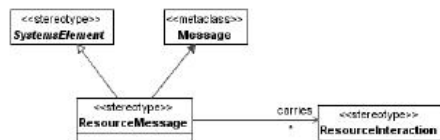
Figure 8.154 - Elements related to the ResourceMessage stereotype
