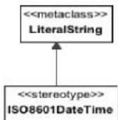
Figure 8.31 - Elements related to the ISO8601DateTime stereotype
