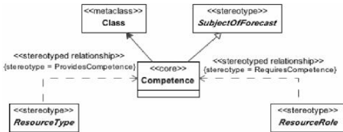
Figure 8.55 - Elements related to the Competence stereotype
