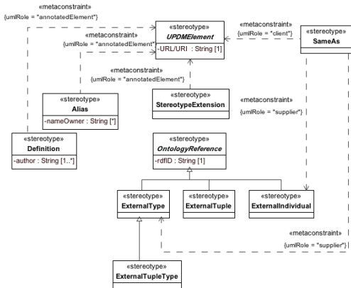
Figure 8.7 - Elements related to the AV-2 Product
