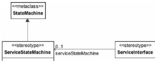
Figure 8.100 - Elements related to the ServiceStateMachine stereotype
