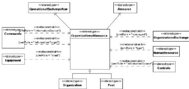
Figure 8.80 - Elements related to the abstract OrganizationalResource stereotype
