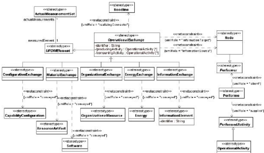
Figure 8.35 - Elements related to the OV-3 product
