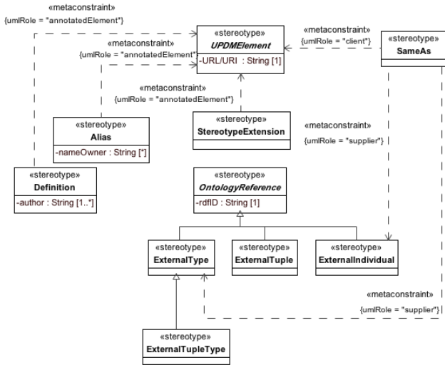
Figure 8.225 - Elements related to the AV-2 productstereotype
