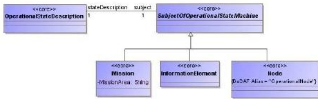
Figure A.20 - OV-6b
