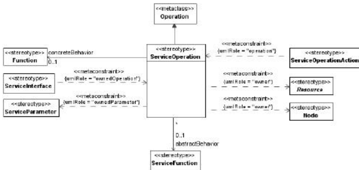
Figure 8.97 - Elements related to the ServiceOperation stereotype
