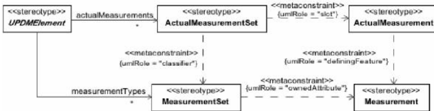
Figure 8.188 - Elements related to the AV-3 productstereotype
