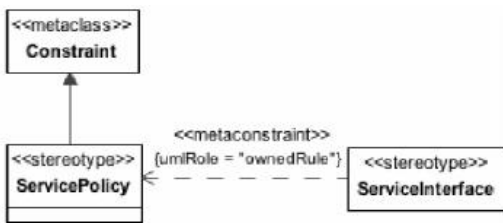
Figure 8.105 - Elements related to the ServicePolicy stereotype
