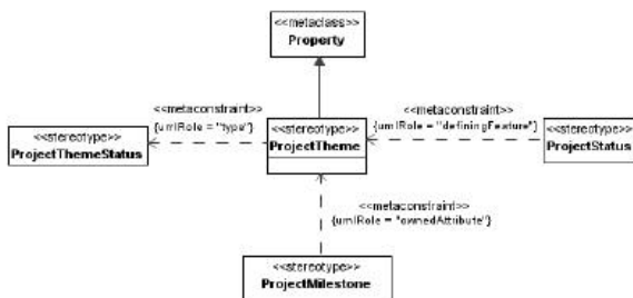
Figure 8.221 - Elements related to the ProjectTheme stereotype
