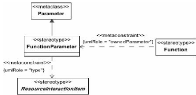
Figure 8.143 - Elements related to the FunctionParameter stereotype
