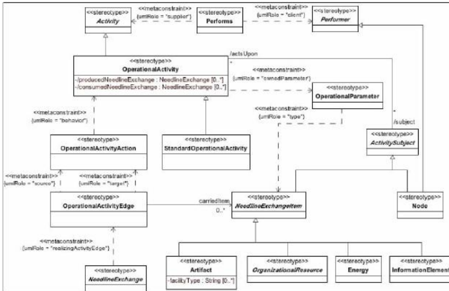
Figure 8.240 - Elements related to the OV-5 productstereotype
