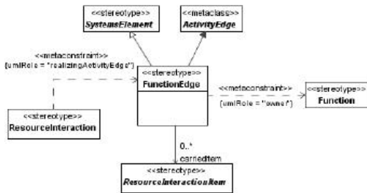
Figure 8.142 – Elements related to the FunctionEdge stereotype
