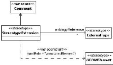
Figure 8.233 - Elements related to the StereotypeExtension stereotype
