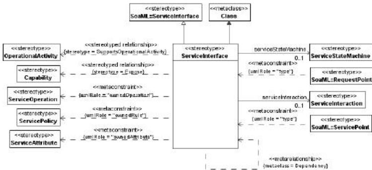
Figure 8.104 - Elements related to the ServiceInterface stereotype
