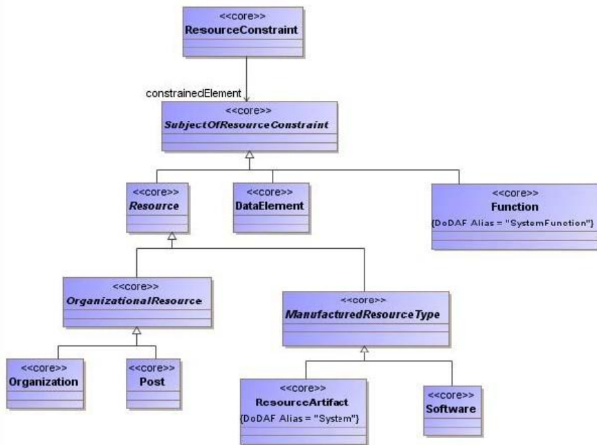
Figure A.39 - SV-10a
