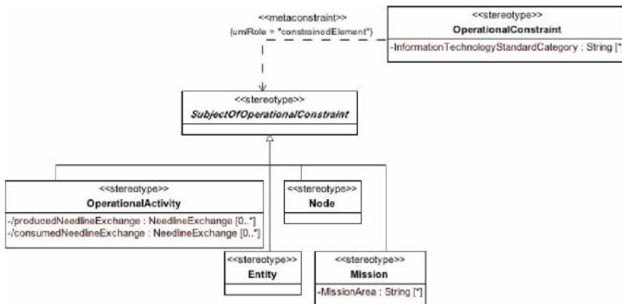
Figure 8.198 - Elements related to the OV-6a productstereotype
