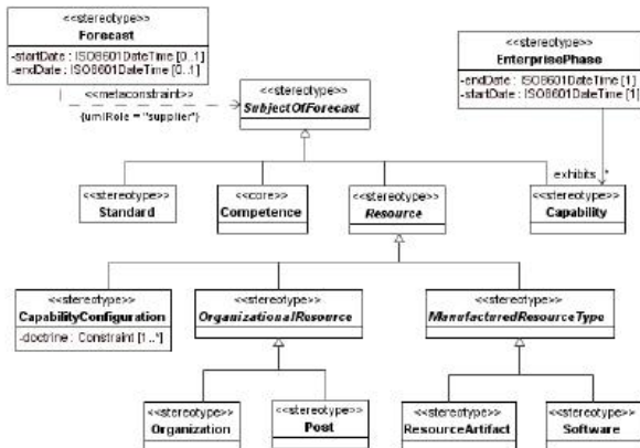
Figure 8.139 - Elements related to the SV-9 product
