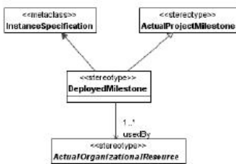
Figure 8.261 - Elements related to the ConfigurationDeployed stereotype
