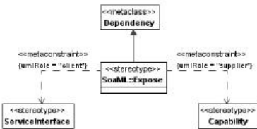
Figure 8.124 - Elements related to the Expose stereotype
