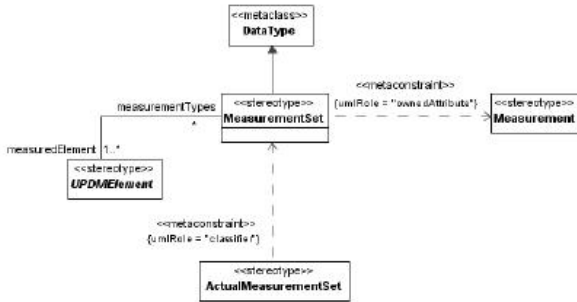
Figure 8.24 - Elements related to the MeasurementSet stereotype
