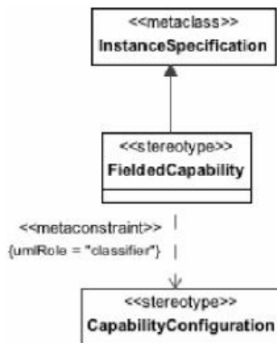
Figure 8.160 - Elements related to the FieldedCapability stereotype
