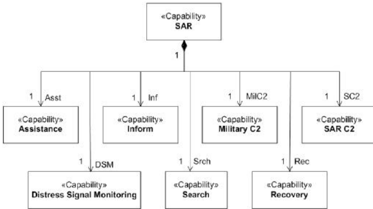
Figure C.8 – StV-4 Alternative View
