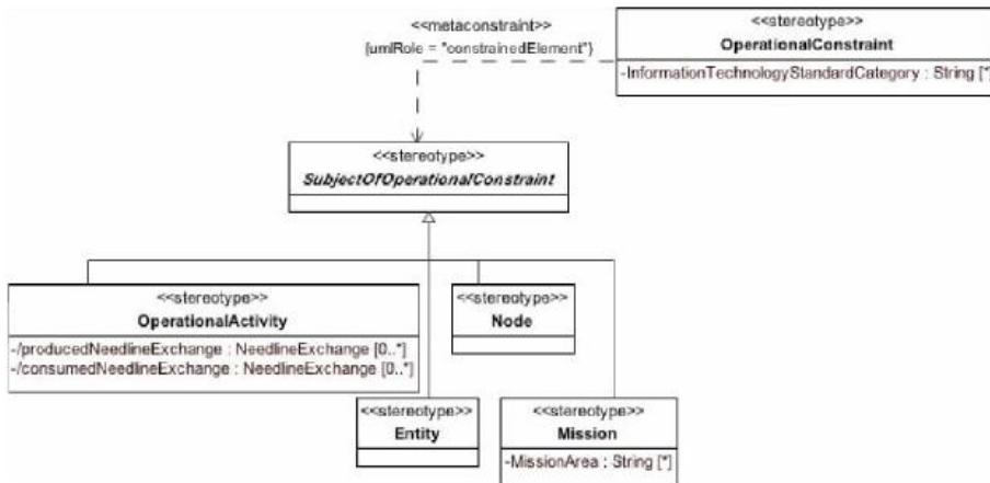
Figure 8.241 - Elements related to the OV-6a productstereotype
