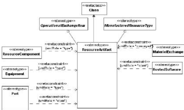
Figure 8.156 - Elements related to the ResourceArtifact stereotype
