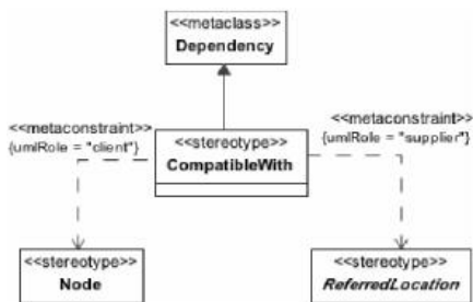
Figure 8.54 - Elements related to the CompatibleWith stereotype
