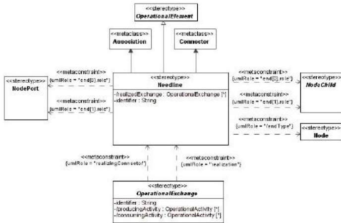
Figure 8.61 - Elements related to the Needline stereotype
