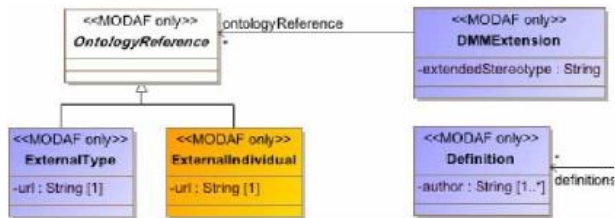
Figure A.4 - AV-2
