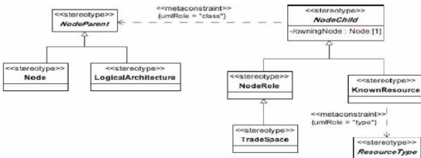
Figure 8.236 - Elements related to the OV-2 Nodes productstereotype
