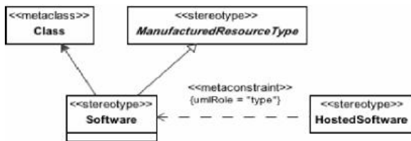
Figure 8.172 - Elements related to the Software stereotype
