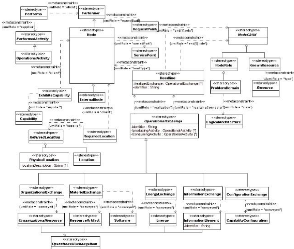
Figure 8.33 - Elements related to the OV-2 product
