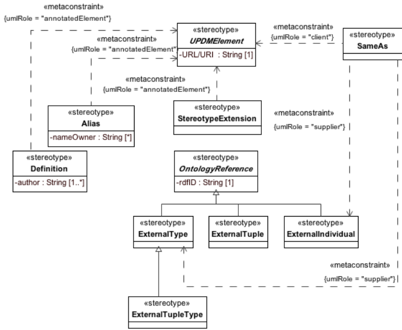
Figure 8.187 - Elements related to the AV-2 productstereotype
