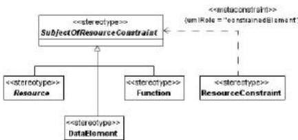
Figure 8.174 - Elements related to the abstract SubjectOfResourceConstraint stereotype
