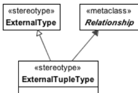
Figure 8.233b Elements related to the ExternalTupleType stereotype.
