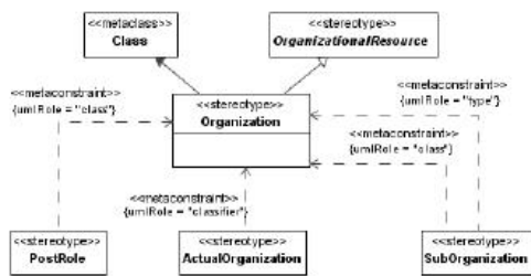
Figure 8.82 - Elements related to the Organization stereotype
