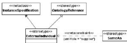
Figure 8.229 - Elements related to the ExternalIndividual stereotype
