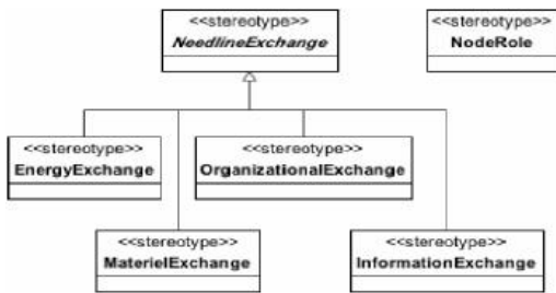
Figure 8.200 - Elements related to the OV-6c productstereotype
