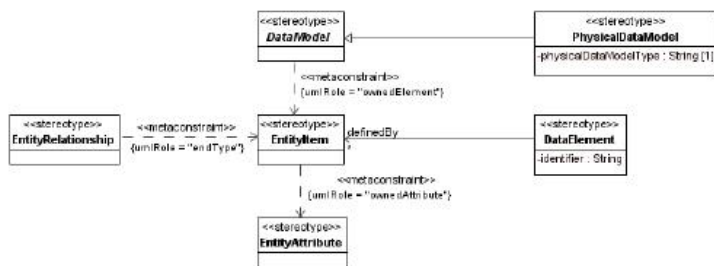
Figure 8.130 - Elements related to the SV-11 product
