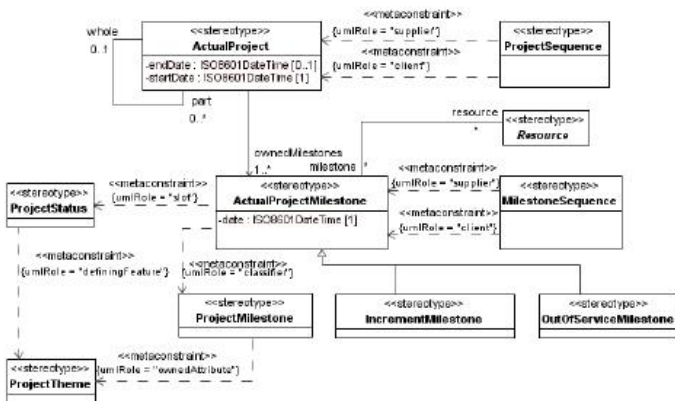
Figure 8.3 - Elements related to the AcV-2 Product
