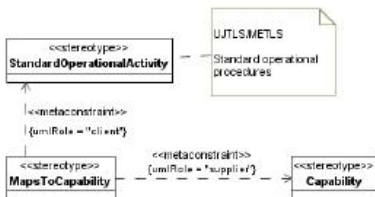
Figure 8.112 - Elements related to the StV-6 stereotype product
