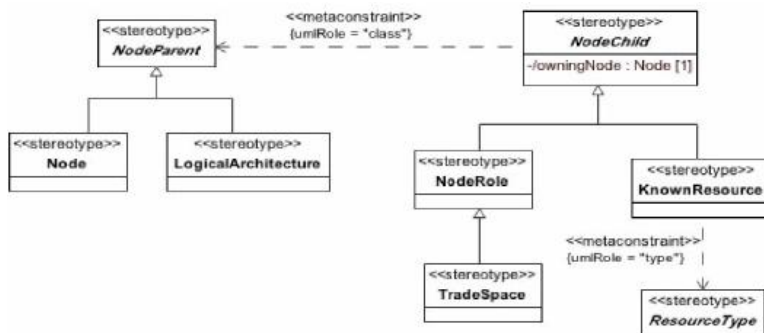
Figure 8.193 - Elements related to the OV-2 Nodes productstereotype
