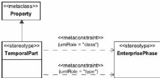
Figure 8.122 - Elements related to the TemporalPart stereotype
