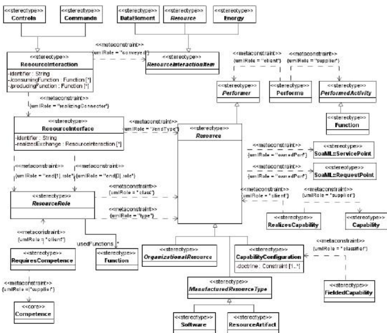
Figure 8.125 - Elements related to the SV-1 product
