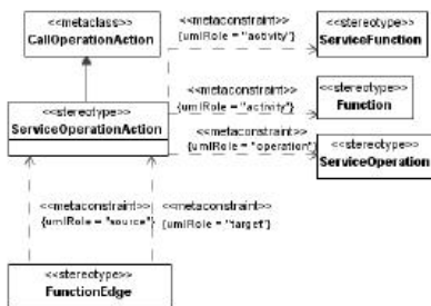
Figure 8.98 - Elements related to the ServiceOperationAction stereotype
