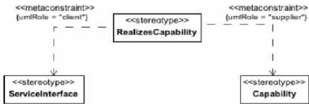
Figure 8.89 - Elements related to the SOV-3 stereotype product
