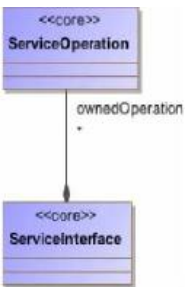
Figure A.25 - SOV-2
