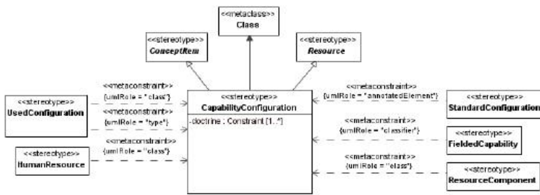
Figure 8.157 - Elements related to the CapabilityConfiguration stereotype
