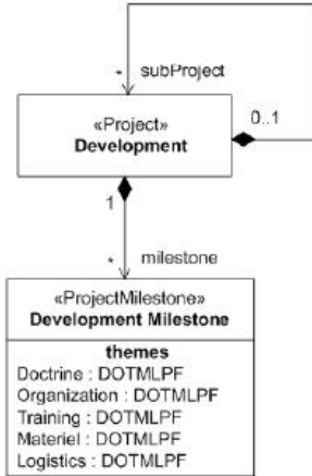
Figure C.33 - AcV-1 Class Diagram
