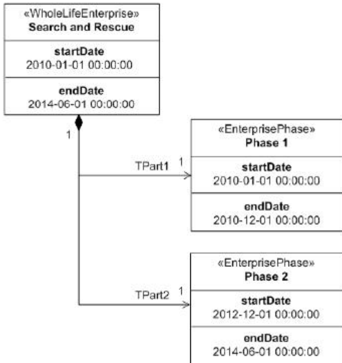
Figure C.2 - AV-1
