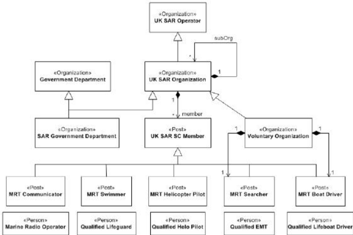
Figure C.16 - OV-4 Typical
