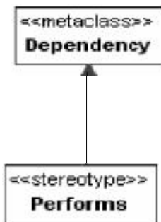
Figure 7.3 - Performs Stereotype
