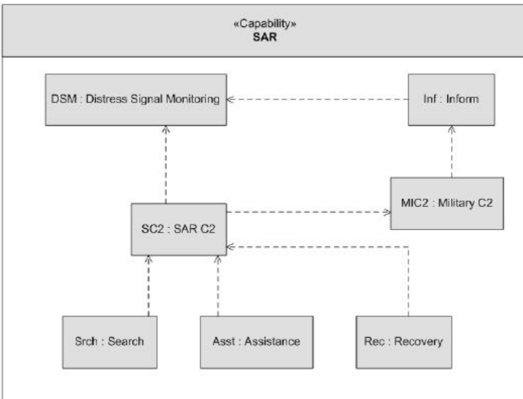
Figure C.7 - StV-4
