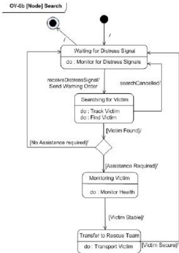
Figure C.20 - OV-6b
