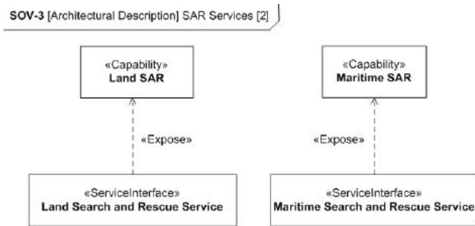
Figure C.24 - SOV-3
