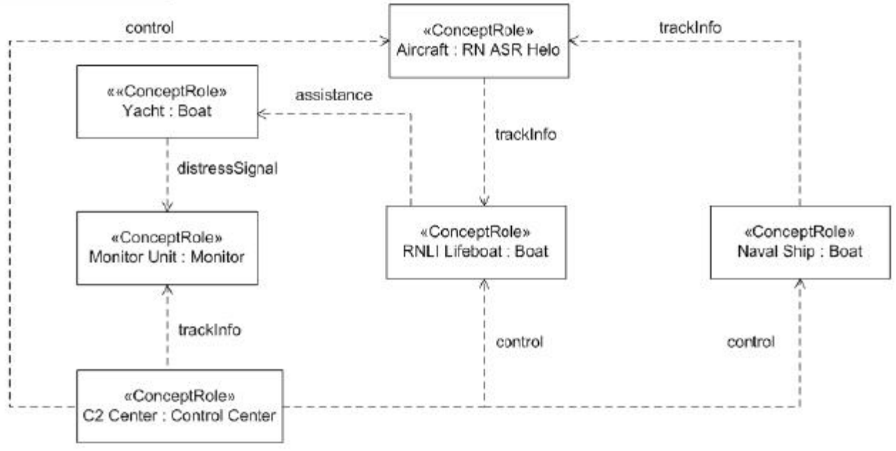
Figure C.11 - OV-1
