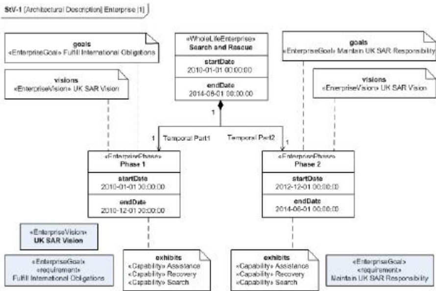
Figure C.5 - StV-1
