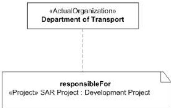
Figure C.32 - AcV-1
