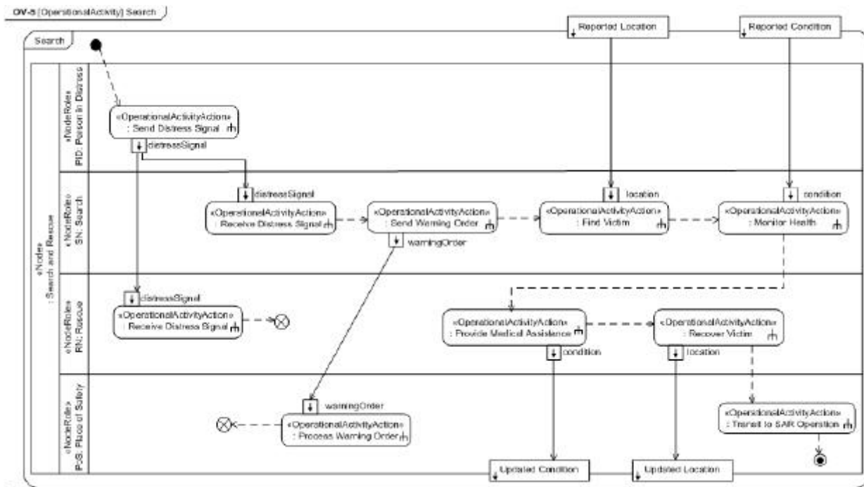
Figure C.19 - Alternate OV-5
