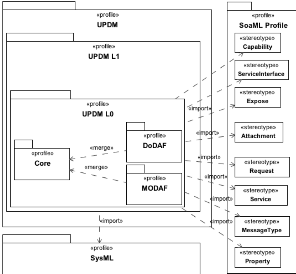
Figure 8.1 - UPDM Profile
