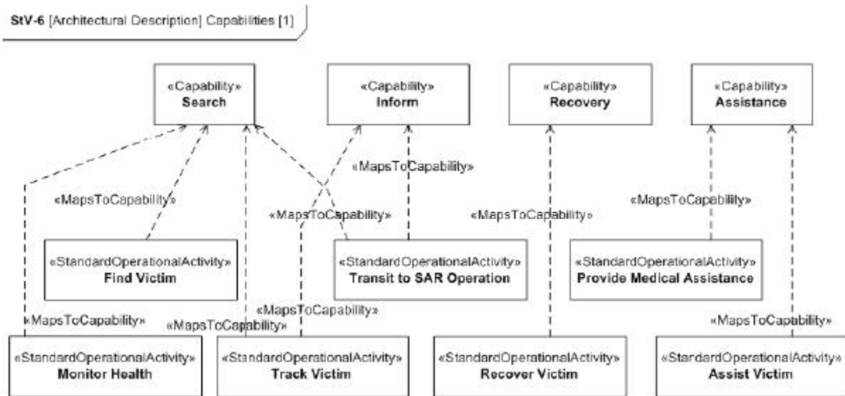
Figure C.10 - StV-6
