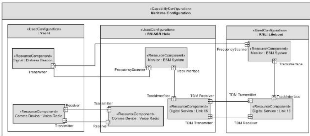
Figure C.28 - SV-2
