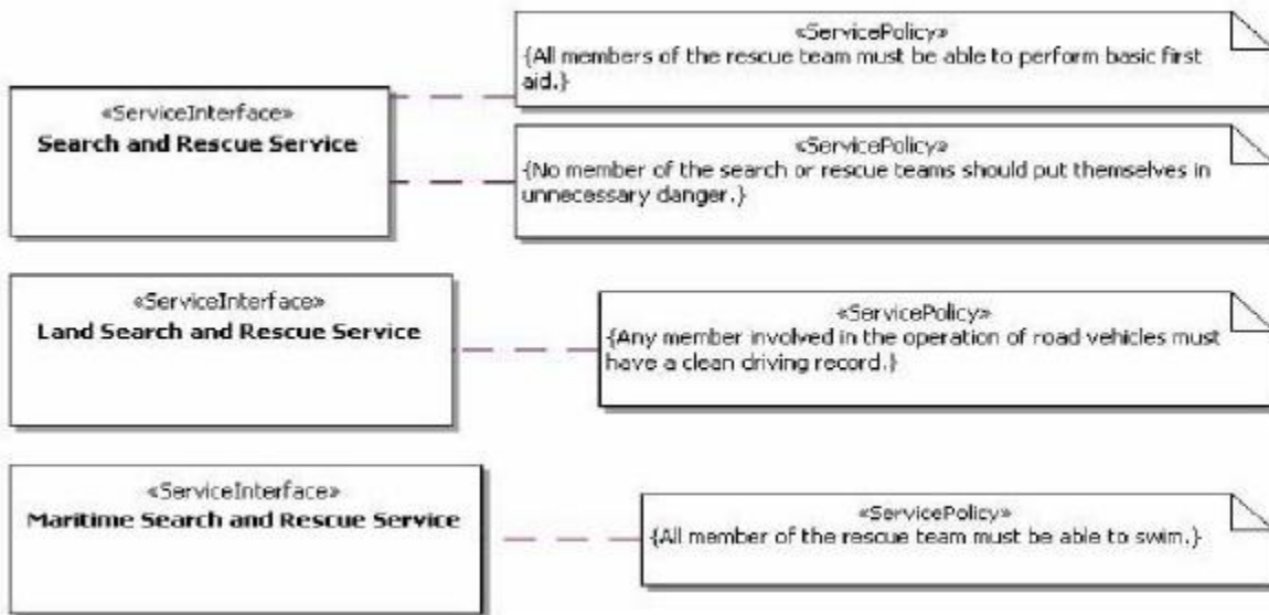
Figure C.25 - SOV-4
