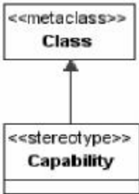
Figure 7.6 - Capabilities Generalization
