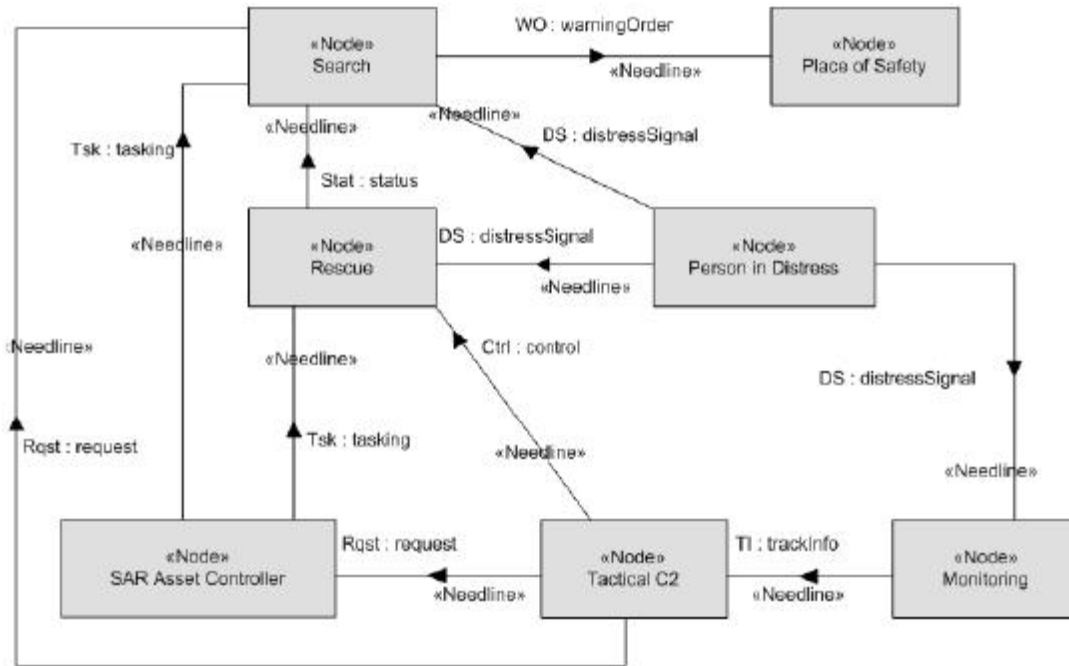
Figure C.13 - OV-2
