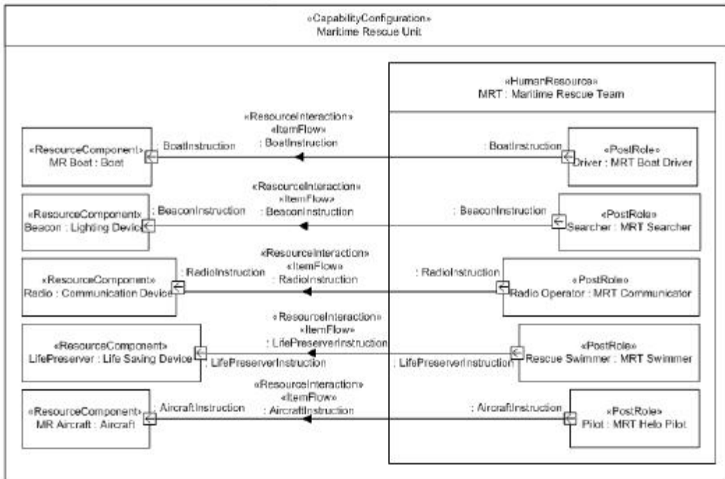
Figure C.27 - SV-1
