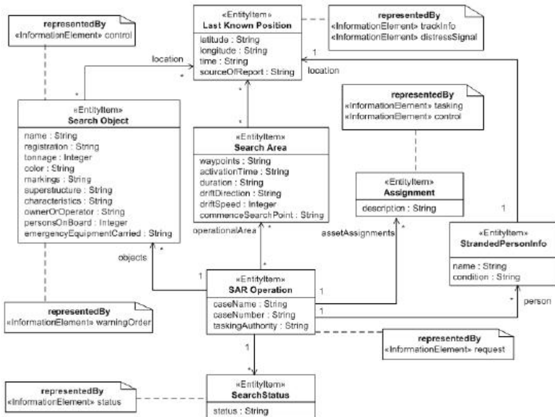
Figure C.21 - OV-7
