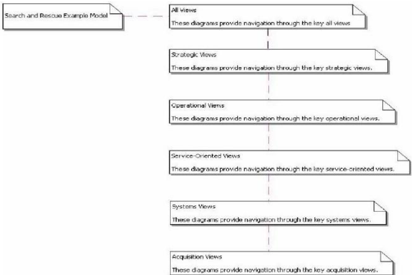
Figure C.1- Diagram Flow
