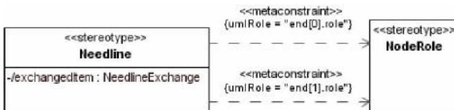
Figure 7.5 - Connector Extension
