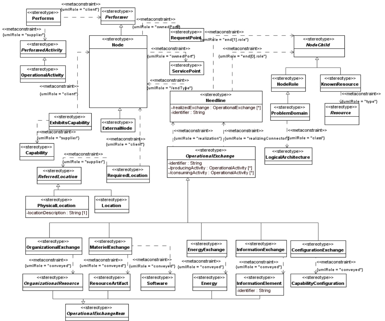
Figure 8.33 - Elements related to the OV-2 product
