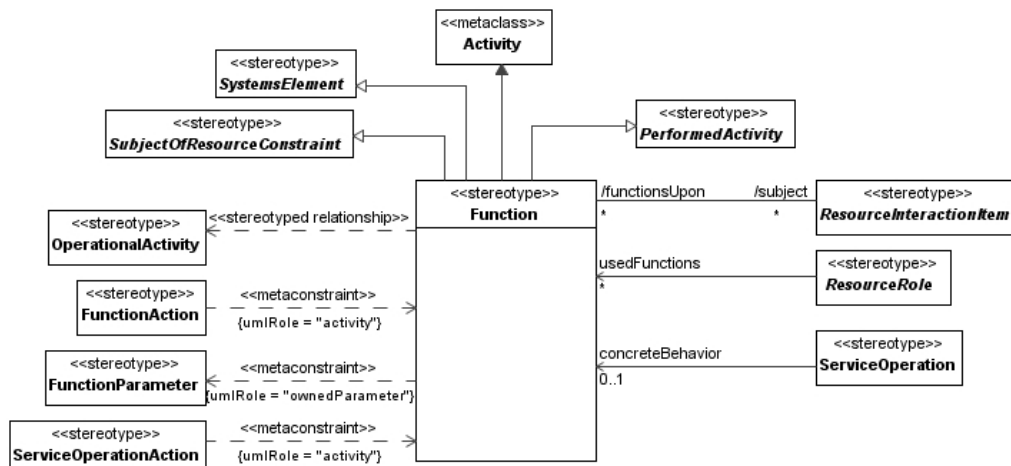
Figure 8.140 - Elements related to the Function stereotype
