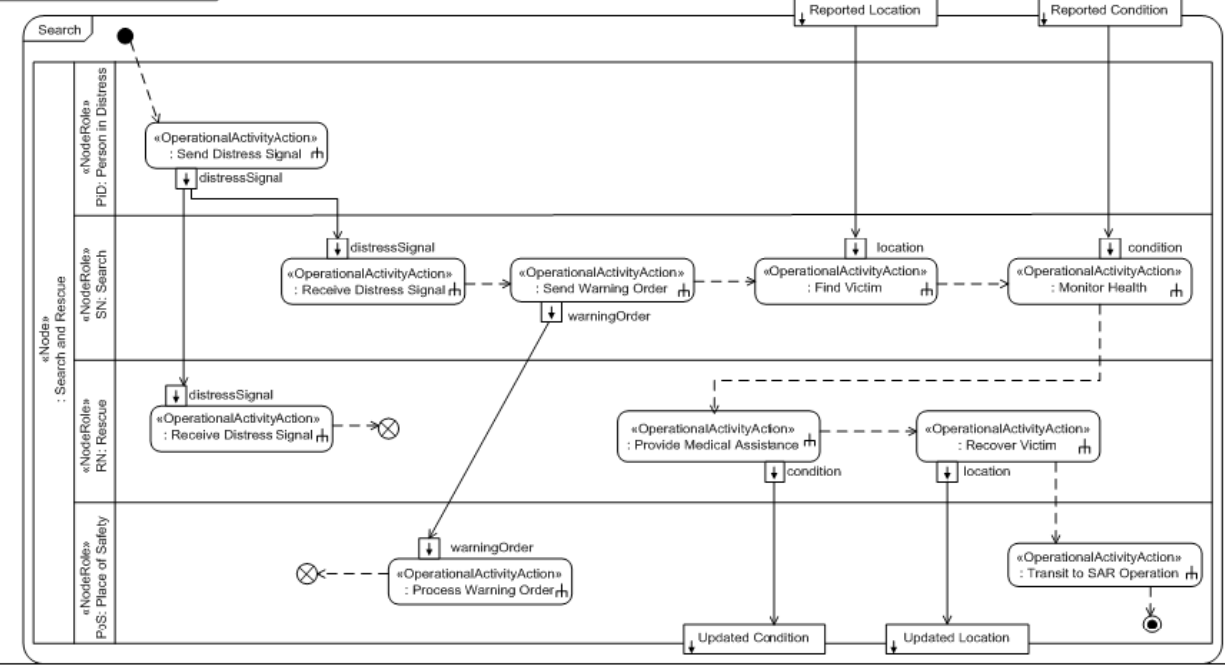
Figure C.19 - Alternate OV-5
