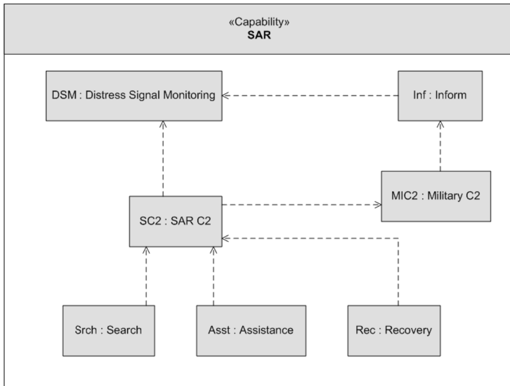
Figure C.7 - StV-4
