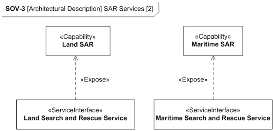
Figure C.24 - SOV-3
