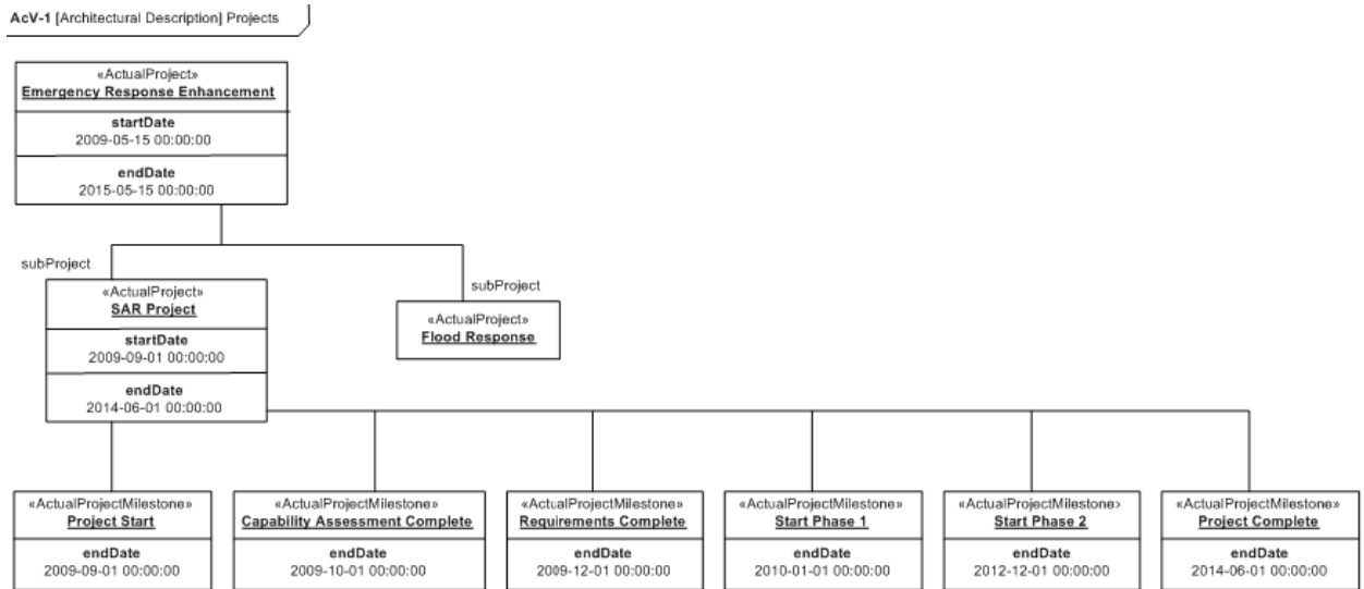
Figure C.34 - AcV-1 Typical
