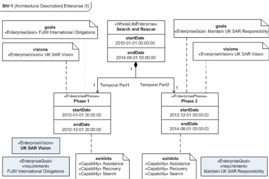
Figure C.5 - StV-1
