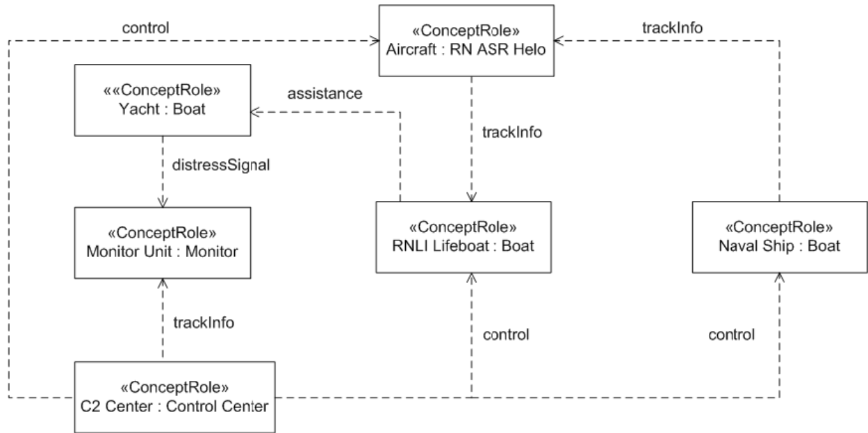
Figure C.11 - OV-1
