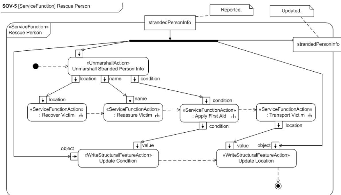
Figure C.26 - SOV-5
