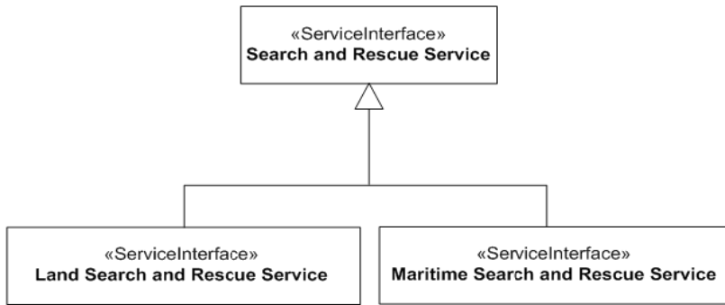
Figure C.22 - SOV-1
