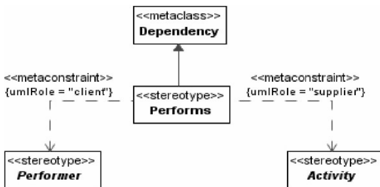
Figure 7.4 - Performs Hierarchy
