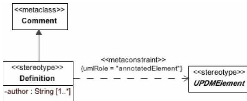
Figure 8.228 - Elements related to the Definition stereotype
