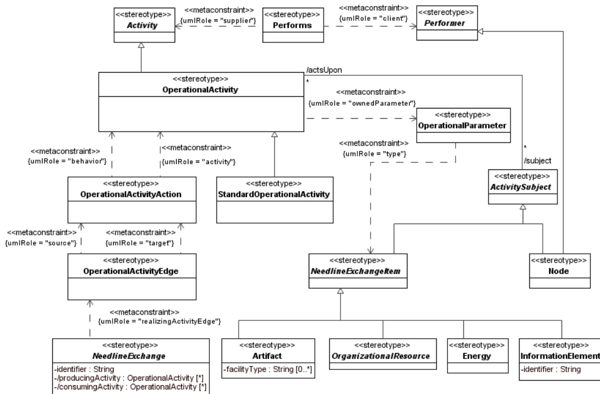
Figure 8.197 - Elements related to the OV-5 stereotype
