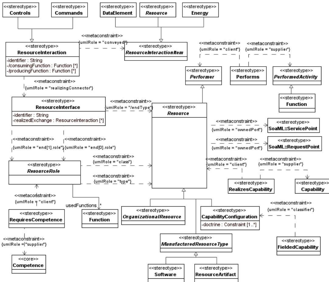
Figure 8.125 - Elements related to the SV-1 product
