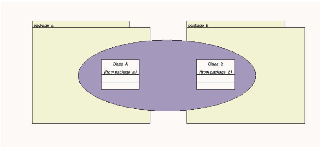
Figure 8 : - An ellipse contained within two paths in the tree of DiagramElements
