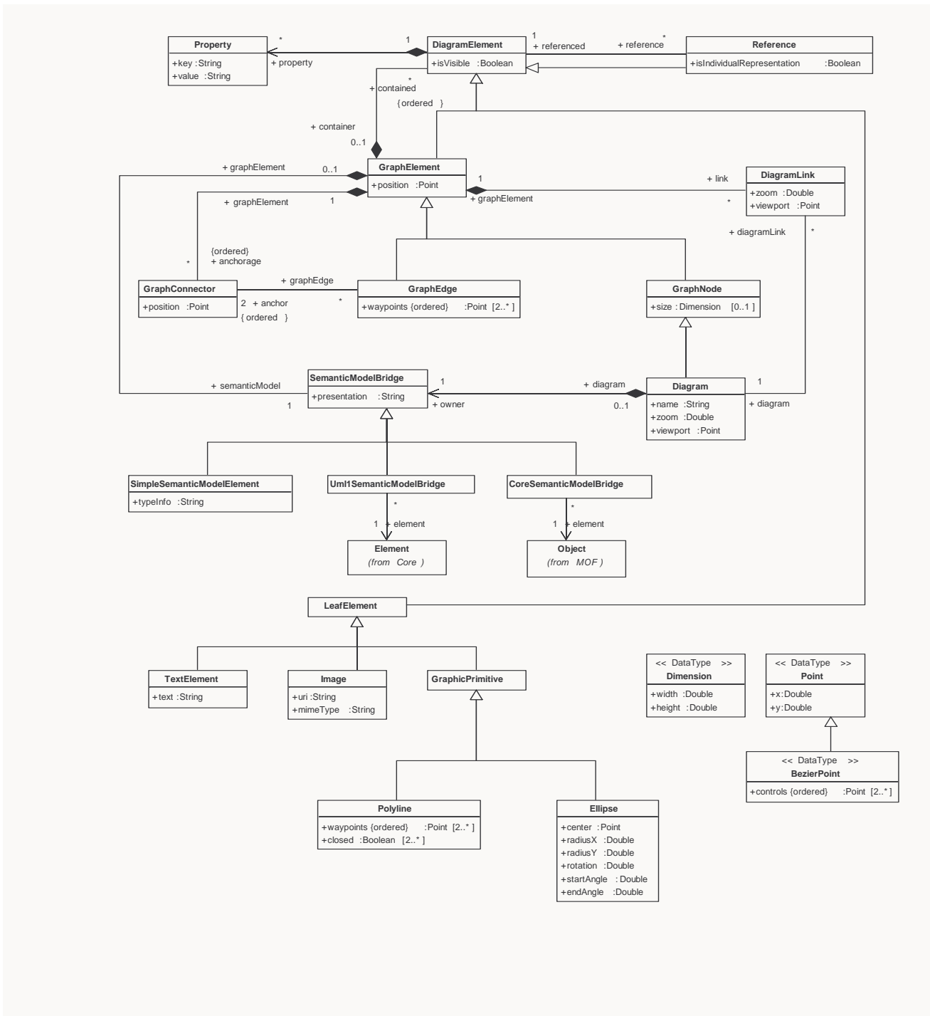
Figure 3 - Diagram Interchange Metamodel
