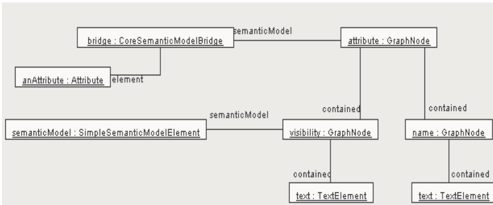
Figure 6 - Example of a TextElement
