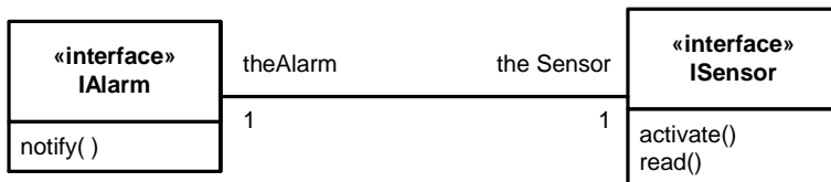
Figure 7.58 - Alarm is the required interface for any classifier implementing ISensor; conversely, ISensor is the required interface for any classifier implementing IAAlarm.
