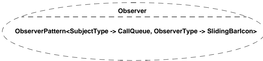
Figure 17.19 - Bound Collaboration
