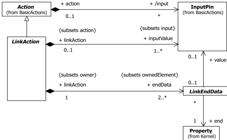
Figure 11.8 - Link identification
