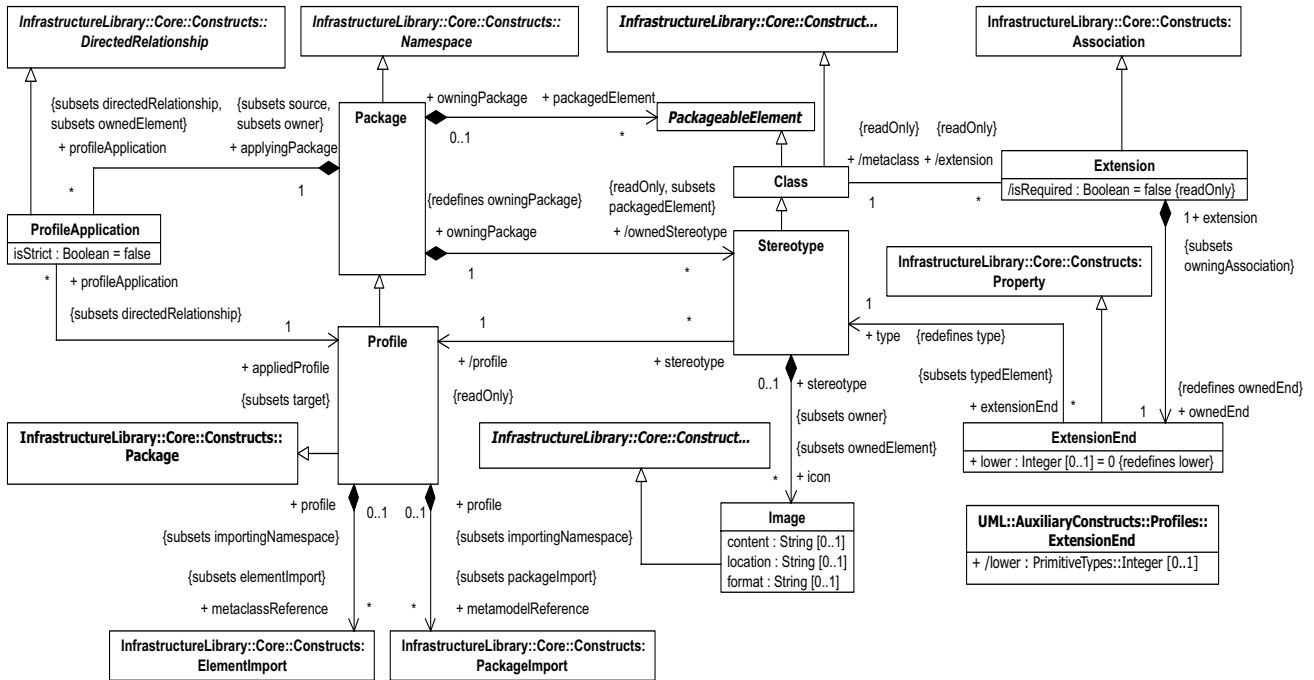
Figure 18.2 - The elements defined in the Profiles package
