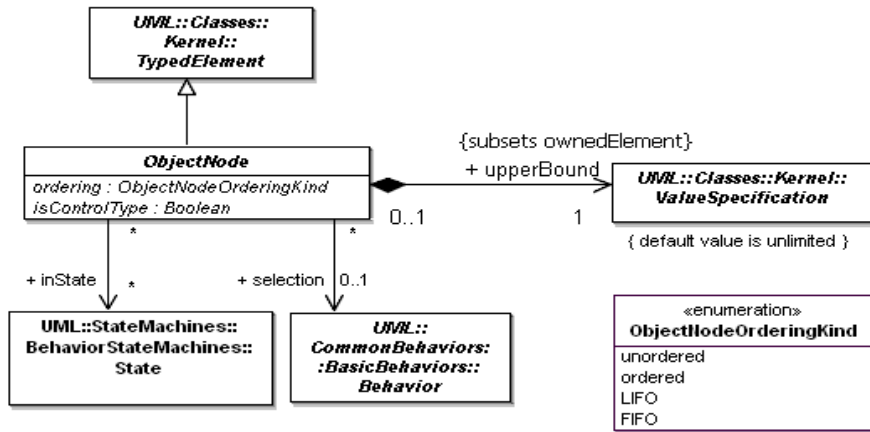
Figure 12.15 - Object nodes (CompleteActivities)
