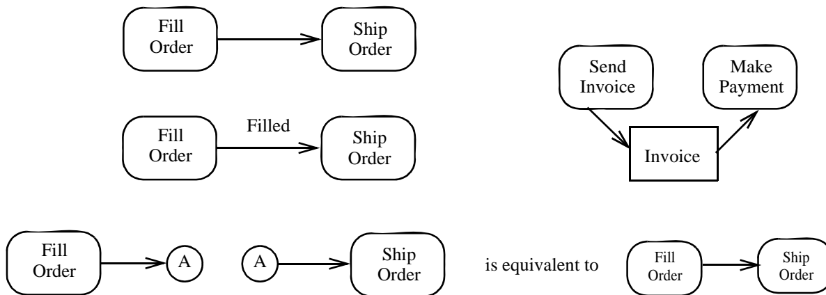
Figure 12.42 - Activity edge examples
