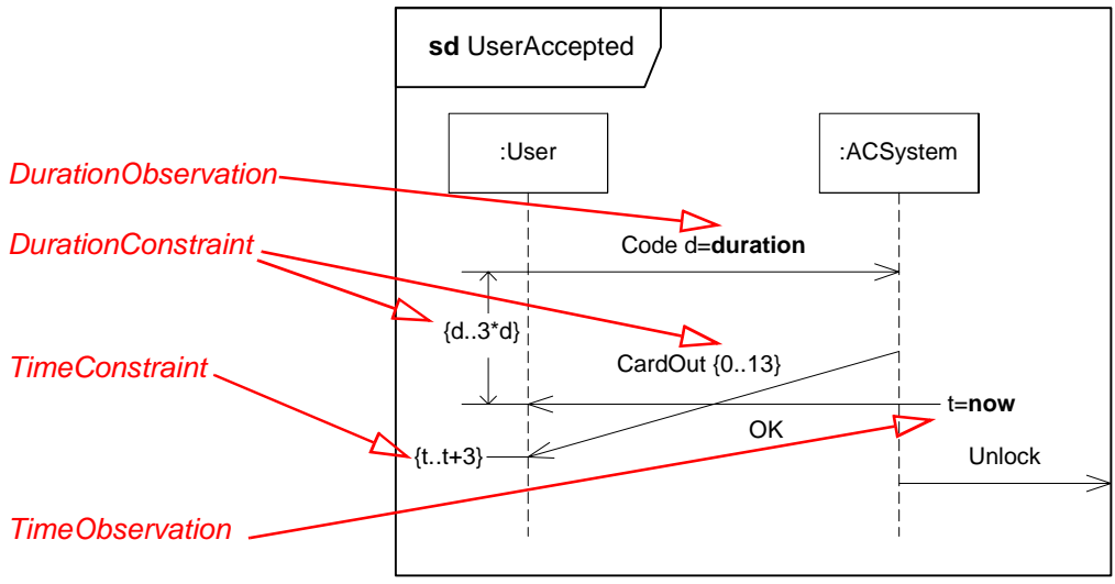
Figure 14.26 - Sequence Diagram with time and timing concepts
