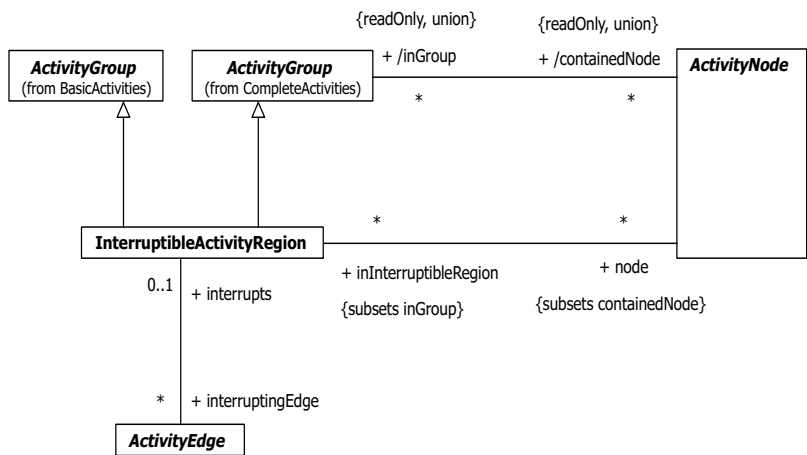
Figure 12.20 - Interruptible regions
