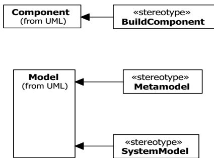
Figure C.1 - StandardProfileL3
