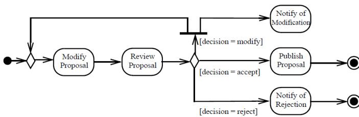
Figure 15.44 ActivityFinalNode example
