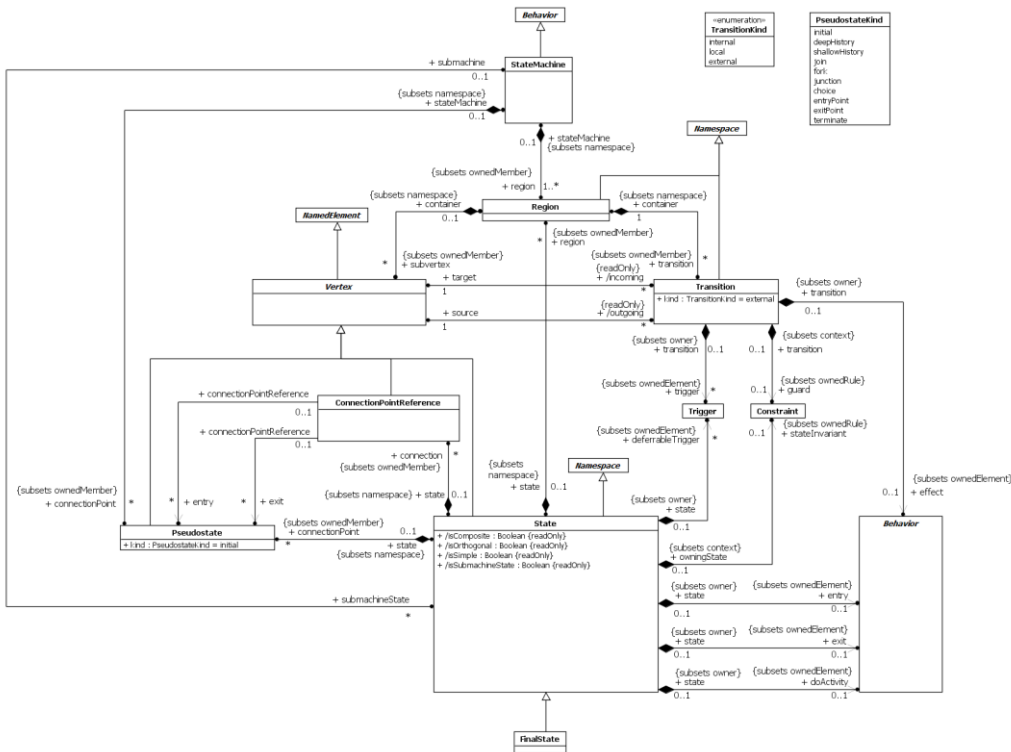
Figure 14.1 Behavior StateMachines
