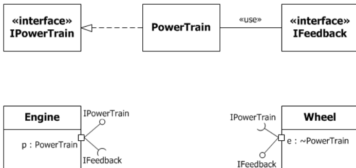
Figure 11.11 Port notation
