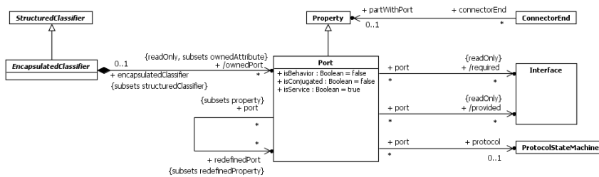
Figure 11.10 Encapsulated Classifiers
