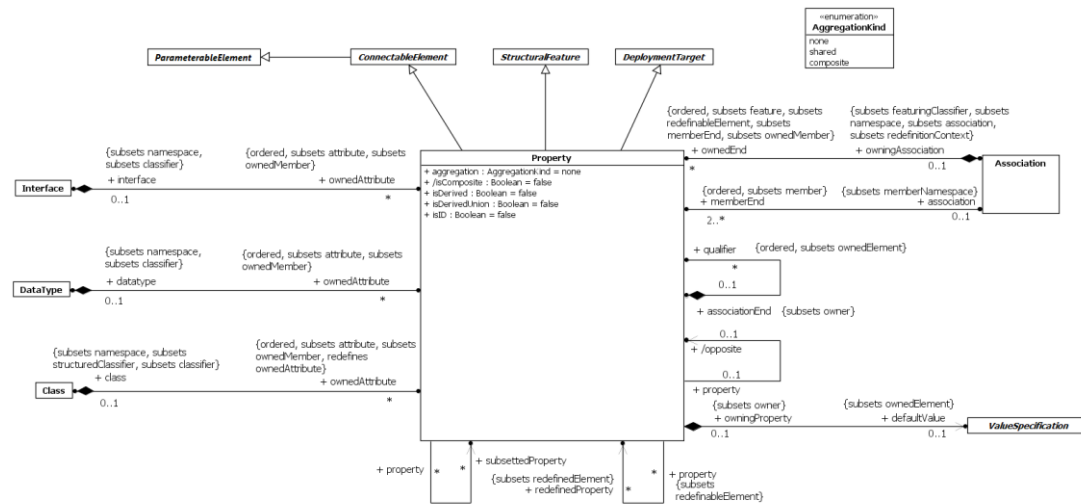
Figure 9.10 Properties
