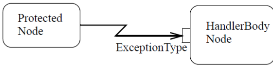
Figure 15.62 ExceptionHandler notation
