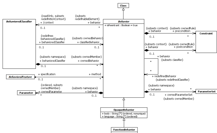
Figure 13.1 Behaviors
