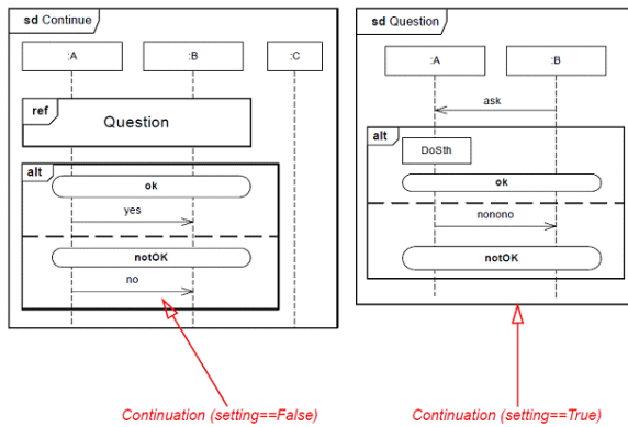
Figure 17.15 Continuation
