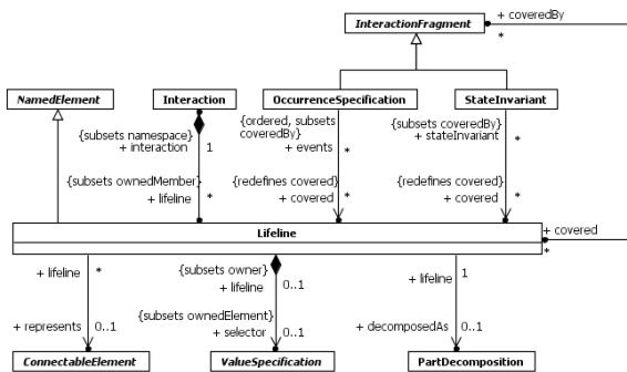
Figure 17.6 Lifelines
