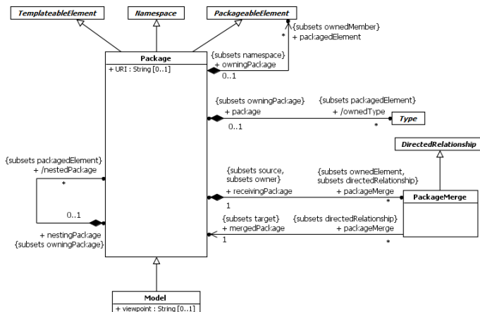
Figure 12.1 Packages
