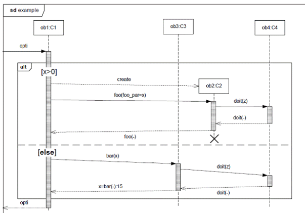
Figure 17.14 CombinedFragment
