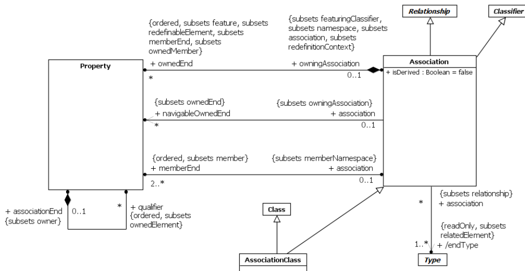
Figure 11.25 Associations
