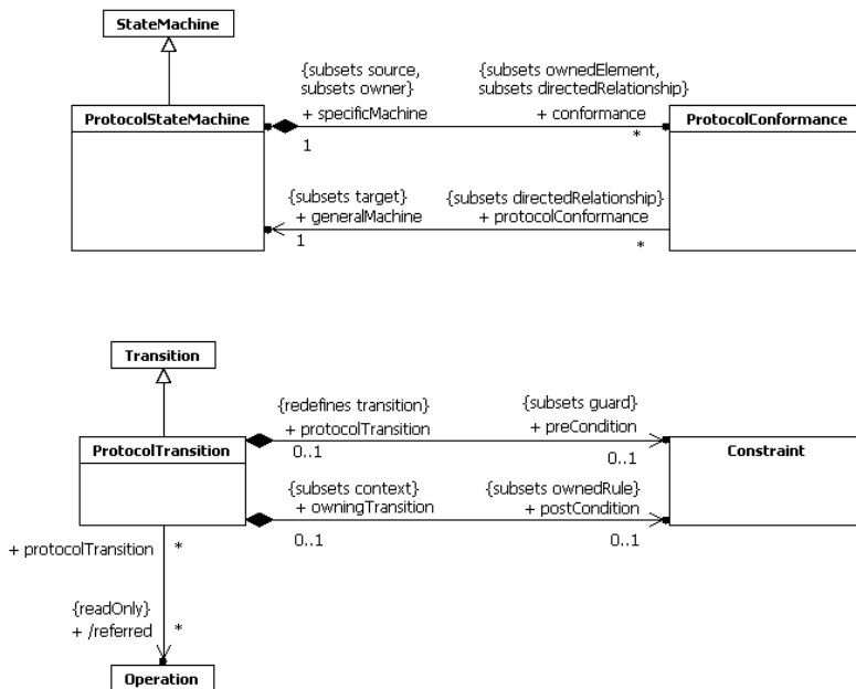
Figure 14.41 ProtocolStateMachines
