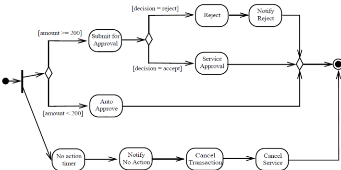
Figure 15.43 ActivityFinalNode example
