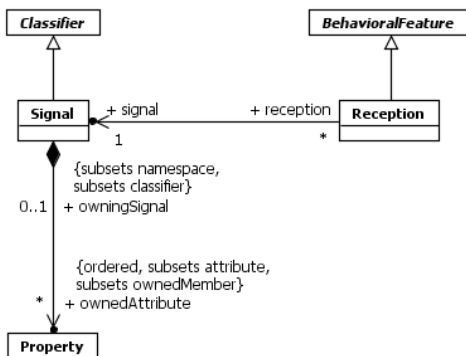
Figure 10.5 Signals
