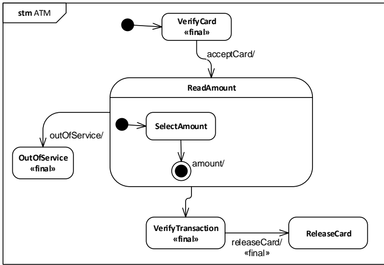
Figure 14.38 A general StateMachine
