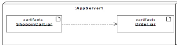
Figure 19.16 Deployed component Artifacts on a Node.
