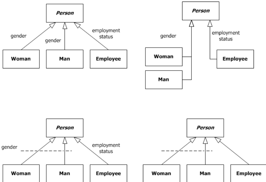
Figure 9.22 GeneralizationSet notation options
