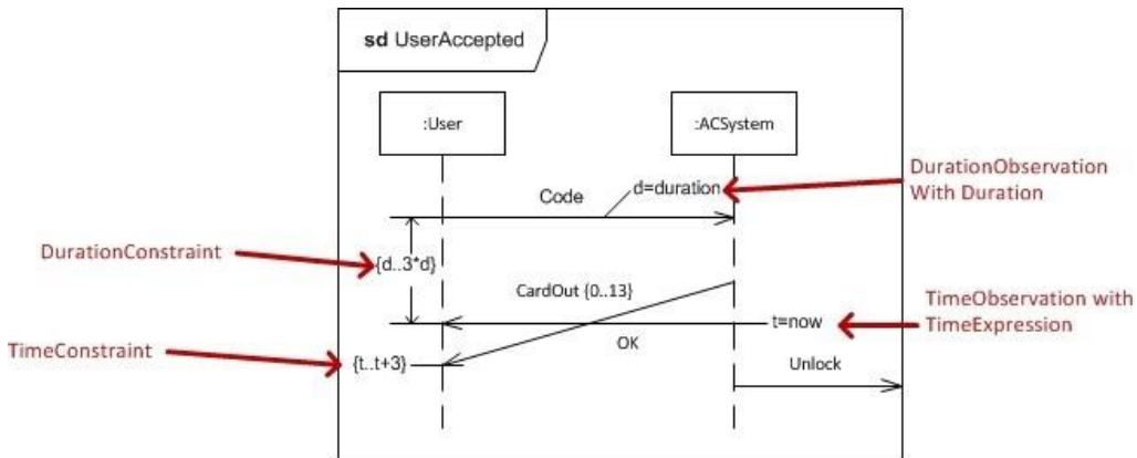
Figure 8.5 Example of DurationConstraints and TimeConstraints
