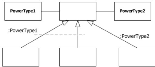
Figure 9.21 Power type notation with dashed line style
