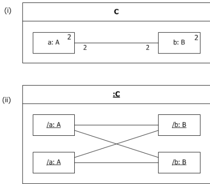
Figure 11.6 "Star" Connector pattern
