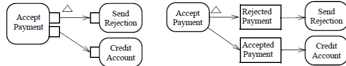
Figure 16.27 Exception Pin examples
