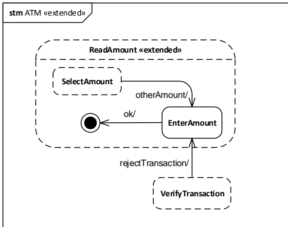
Figure 14.39 An extended StateMachine
