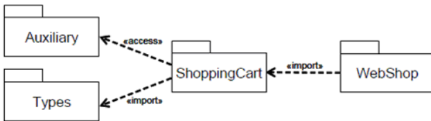
Figure 7.9 Examples of public and private package imports
