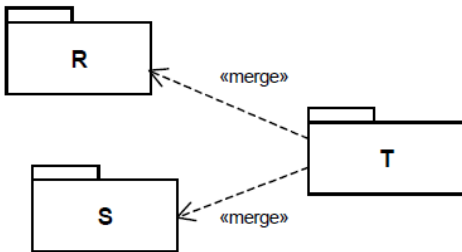
Figure 12.8 Introducing Additional Package Merges
