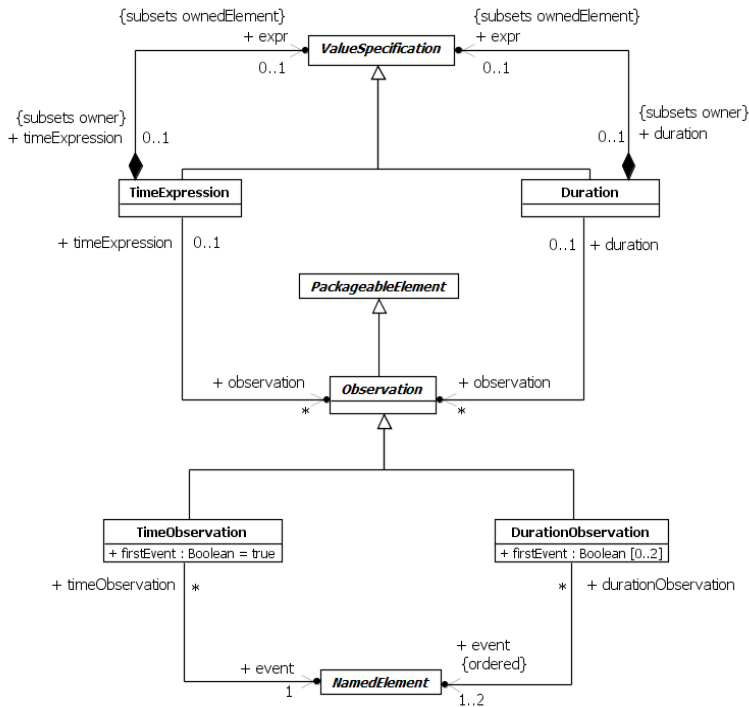
Figure 8.3 Time and Duration
