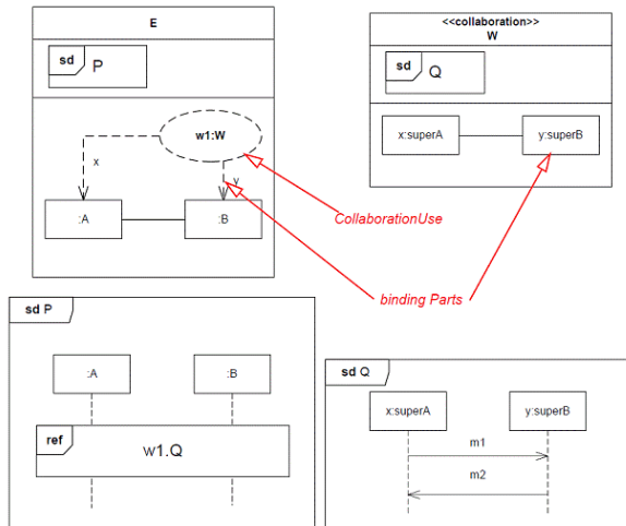
Figure 17.24 Describing Collaborations and their binding
