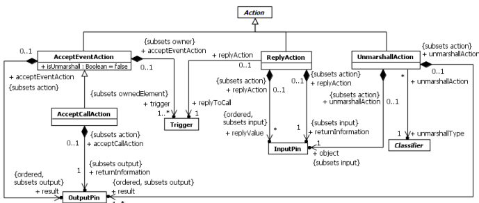
Figure 16.39 Accept Event Actions
