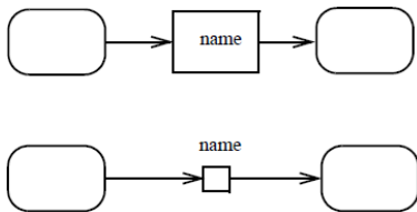
Figure 16.6 Standalone Pin notations
