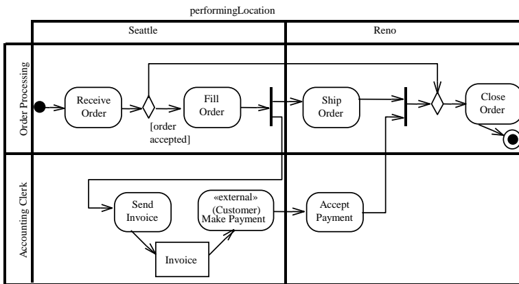
Figure 15.72 ActivityPartitions using multidimensional swimlane notation
