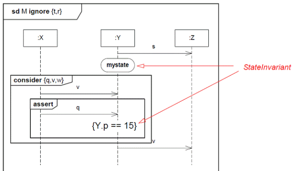
Figure 17.17 Ignore, consider, assert with StateInvariants
