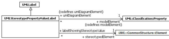
Figure B.7 Stereotype Application Labels
