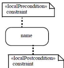
Figure 16.3 Local pre- and post-conditions
