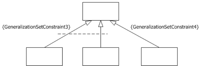
Figure 9.19 GeneralizationSet constraint notation with dashed line style
