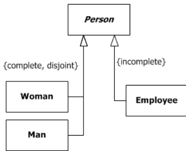
Figure 9.23 GeneralizationSets and constraints
