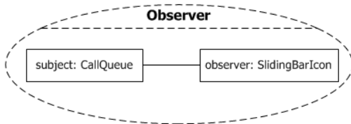
Figure 11.50 The internal structure of the Observer Collaboration
