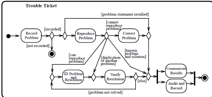
Figure 15.24 Trouble ticket workflow example
