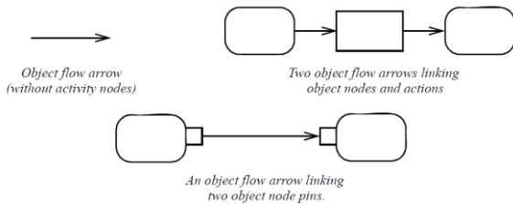
Figure 15.9 ObjectFlow notations
