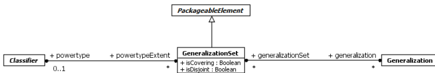
Figure 9.14 Generalization Sets
