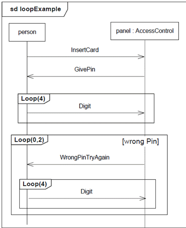
Figure 17.13 - Loop CombinedFragment
