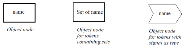
Figure 15.49 ObjectNode notations
