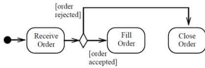
Figure 15.40 DecisionNode example
