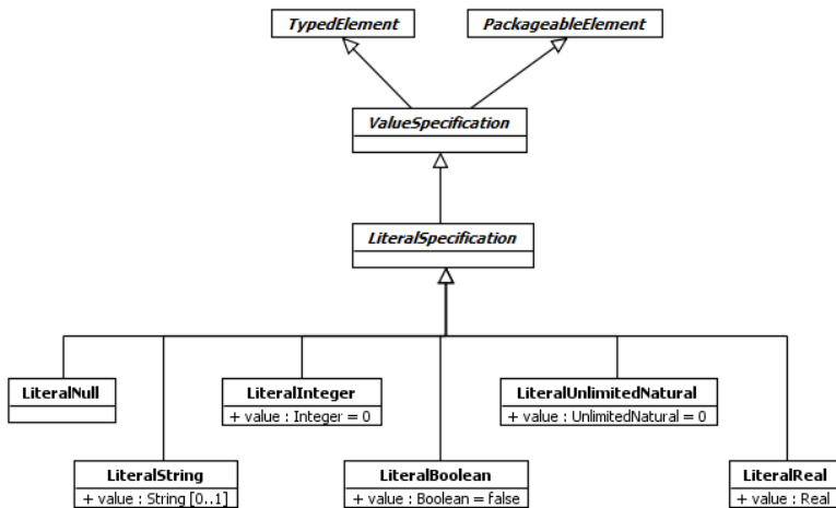
Figure 8.1 Literals
