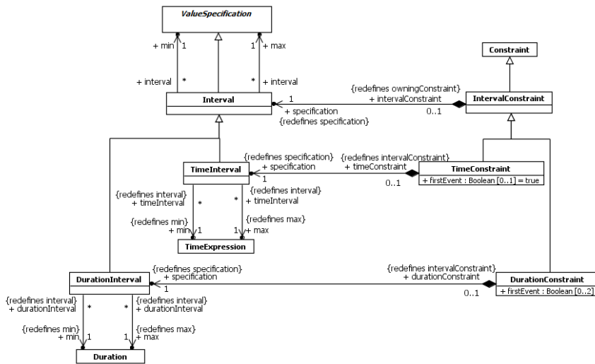
Figure 8.4 Intervals
