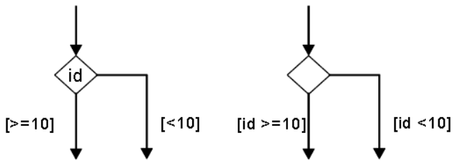
Figure 14.25 choice Pseudostates
