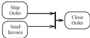
Figure 15.37 JoinNode example
