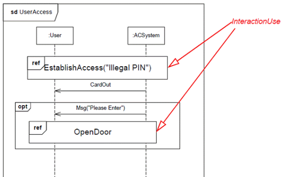
Figure 17.19 InteractionUse
