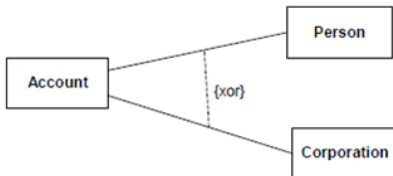
Figure 7.16 {xor} constraint
