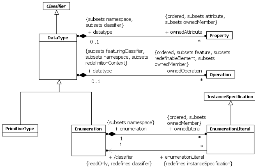
Figure 10.1 DataTypes
