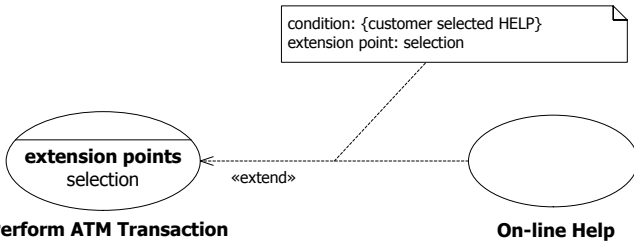
Figure 18.3 Example Extend
