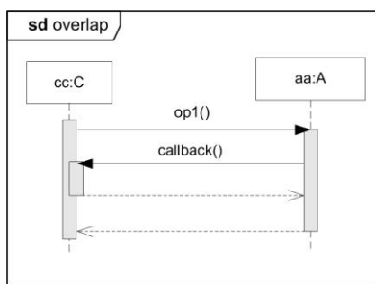
Figure 17.2 Overlapping ExecutionSpecifications
