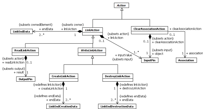
Figure 16.34 Link Actions
