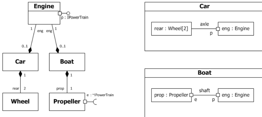
Figure 11.14 Port examples
