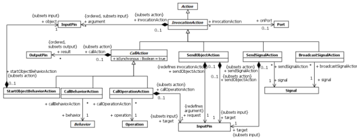
Figure 16.13 Invocation Actions
