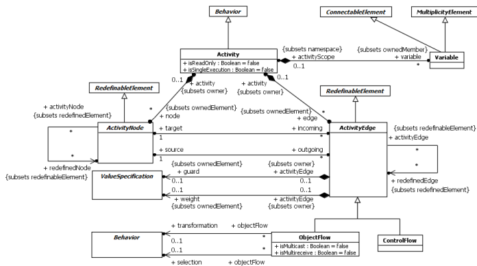
Figure 15.1 Activities
