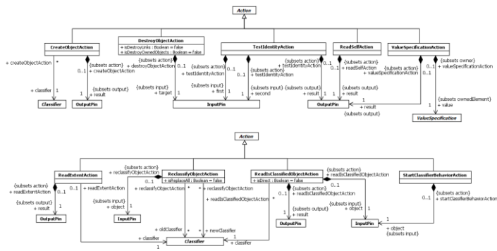
Figure 16.30 Object Actions
