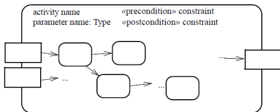
Figure 15.2 Activity notation
