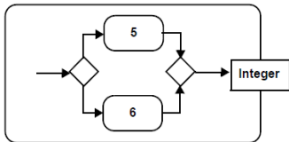
Figure 16.32 ValueSpecificationActions
