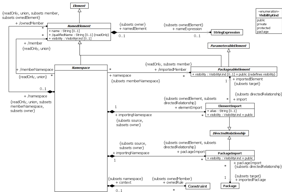
Figure 7.5 Namespaces
