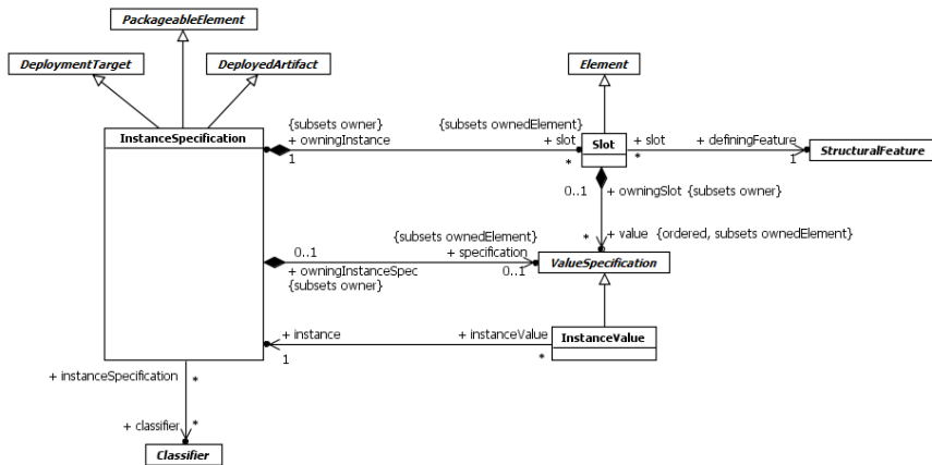
Figure 9.27 Instances
