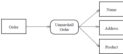
Figure 16.44 UnmarshallAction
