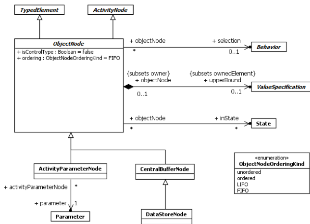
Figure 15.48 Object Nodes
