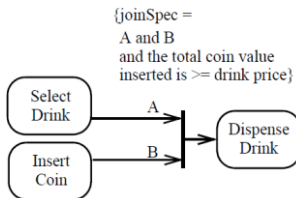
Figure 15.38 joinSpec example
