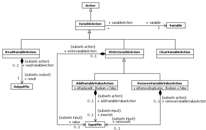
Figure 16.37 Variable Actions
