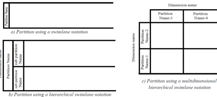
Figure 15.66 ActivityPartition notations
