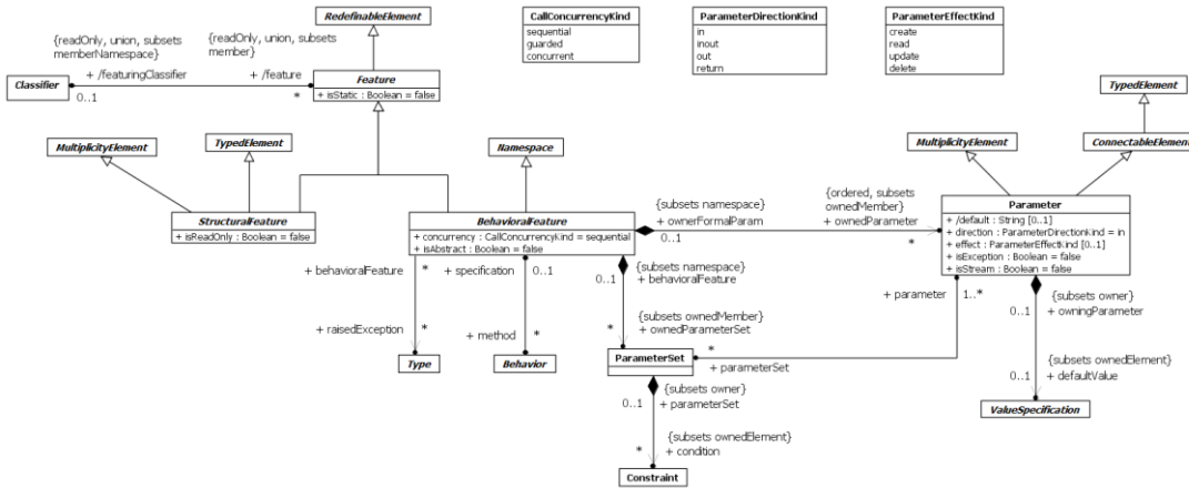
Figure 9.9 Features
