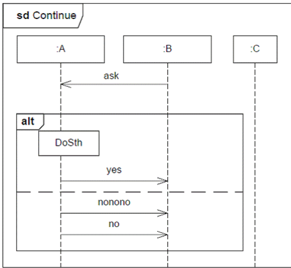
Figure 17.16 Continuation interpretation
