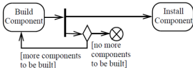
Figure 15.45 FlowFinalNode example
