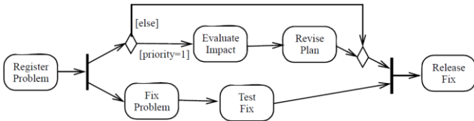
Figure 15.20 Equivalent model
