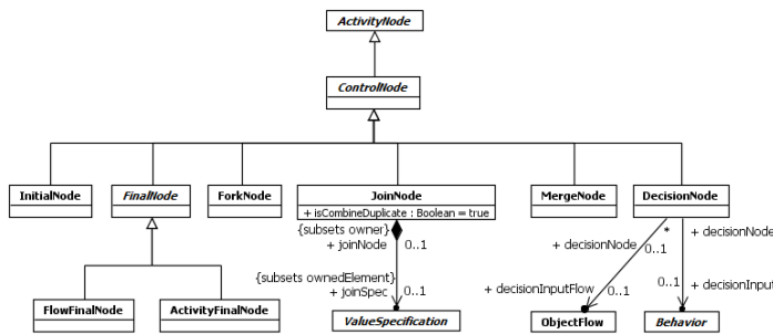
Figure 15.26 Control Nodes
