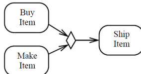
Figure 15.39 MergeNode example
