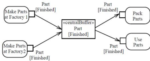
Figure 15.58 CentralBufferNode example
