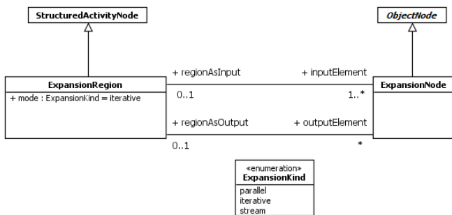
Figure 16.47 Expansion Regions
