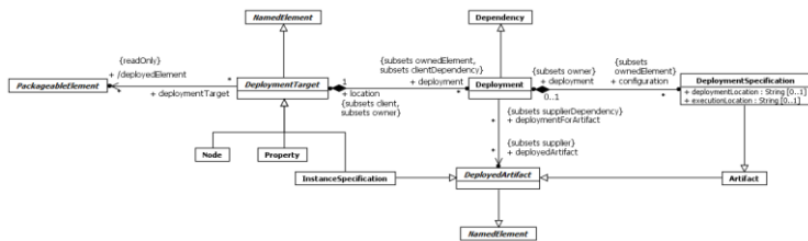
Figure 19.1 Deployments
