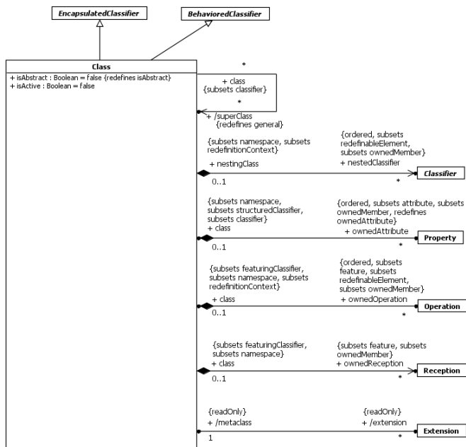
Figure 11.15 Classes
