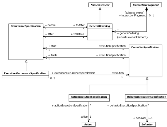
Figure 17.9 Occurrences
