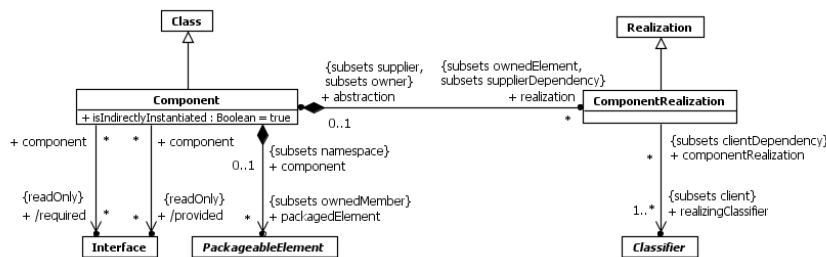
Figure 11.38 Components
