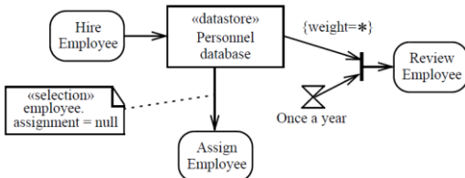
Figure 15.59 DataStoreNode example
