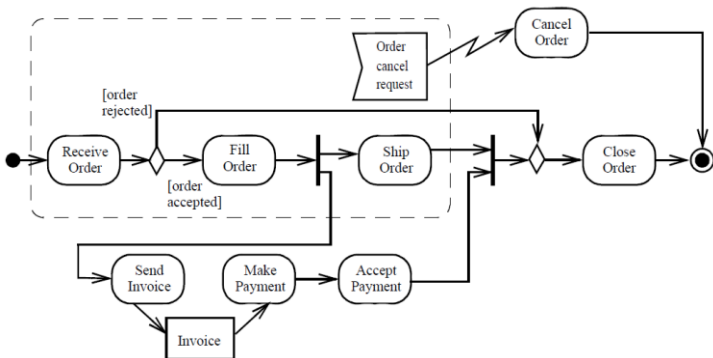
Figure 15.73 InterruptibleActivityRegion example
