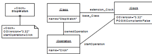
Figure 12.29 Showing Values of Stereotypes and a Simple Instance Specification
