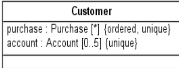
Figure 7.11 Multiplicity within a textual specification
