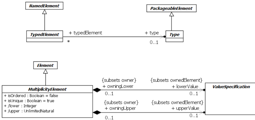
Figure 7.10 Abstract syntax of types and multiplicity elements
