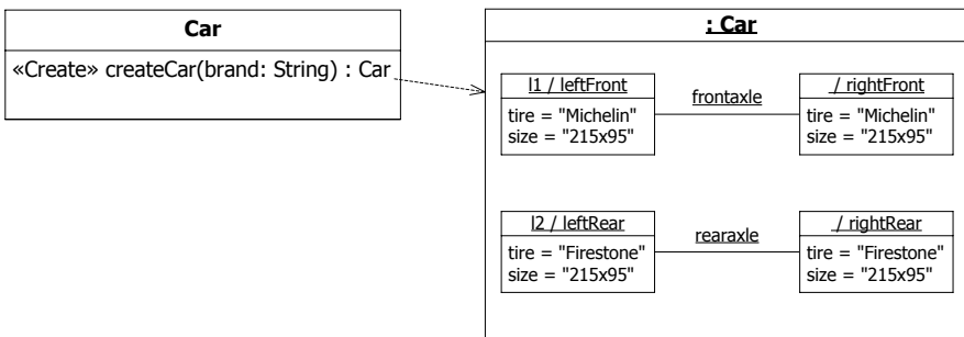
Figure 11.23 A constructor for the Car Class
