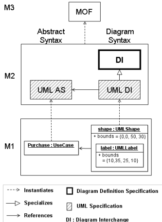
Figure B.2 UML Diagram Interchange Architecture
