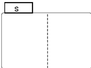
Figure 14.3 Notation for a composite State with Regions
