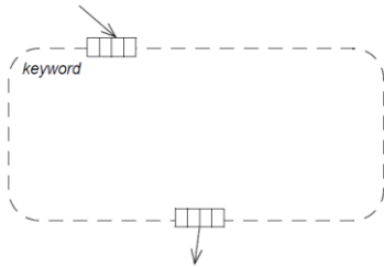
Figure 16.48 Expansion Region
