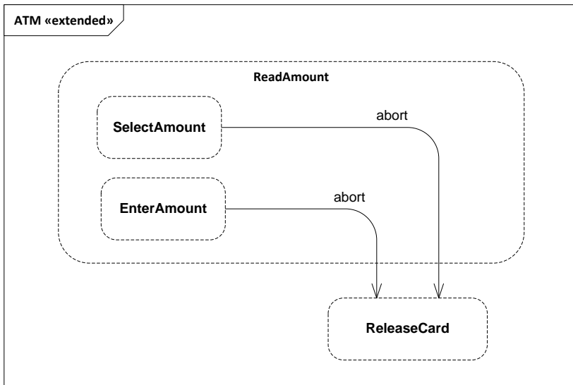
Figure 14.40 Adding Transitions
