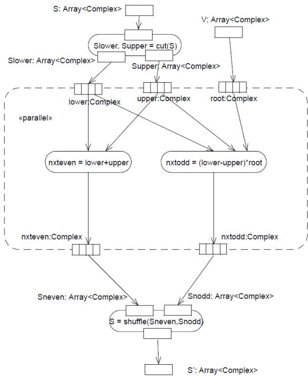
Figure 16.53 Expansion Region
