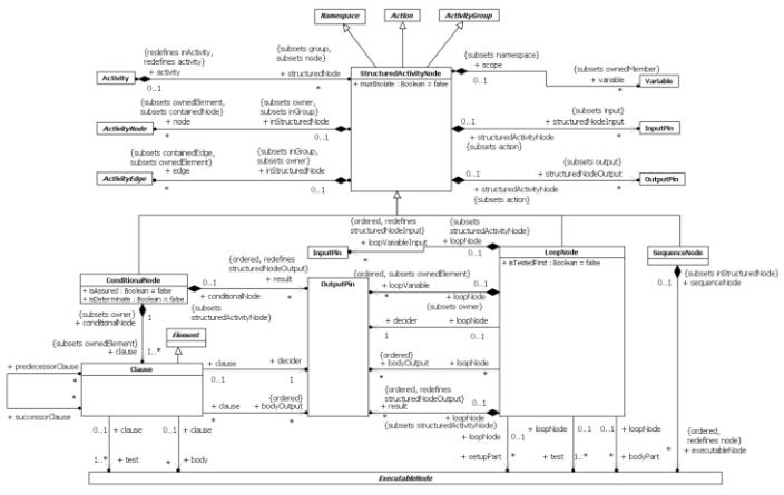
Figure 16.45 Structured Actions
