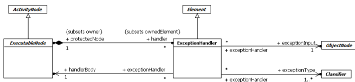
Figure 15.60 Executable Nodes
