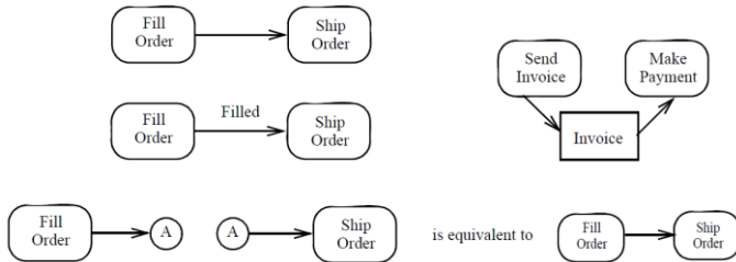
Figure 15.13 ActivityEdge examples
