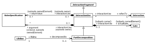
Figure 17.18 InteractionUses
