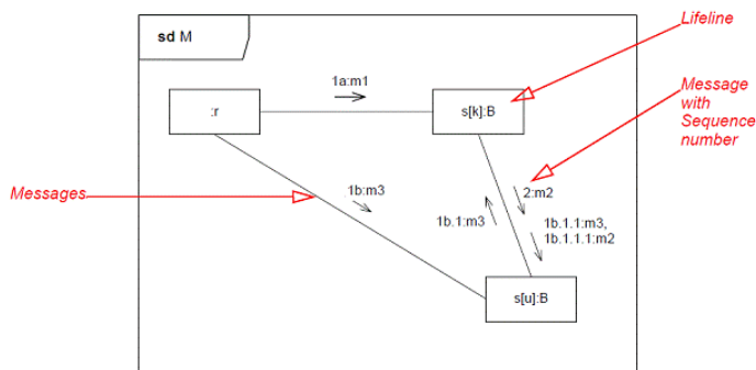
Figure 17.26 Communication diagram
