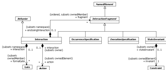
Figure 17.1 Interactions
