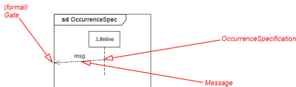
Figure 17.4 OccurrenceSpecification
