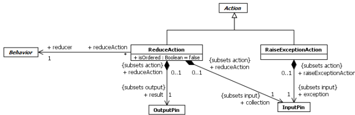
Figure 16.56 Other Actions
