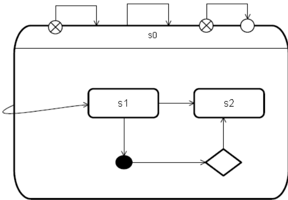
Figure 14.35 External Transitions
