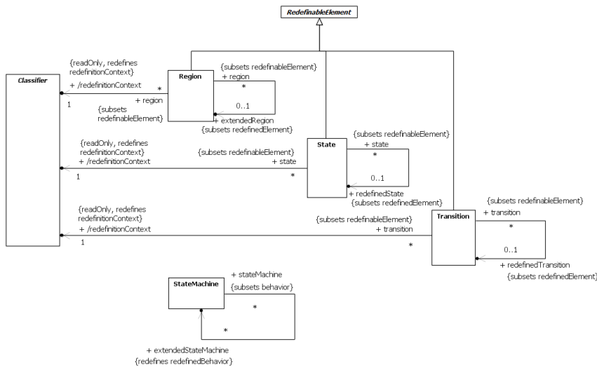
Figure 14.37 StateMachine redefinition
