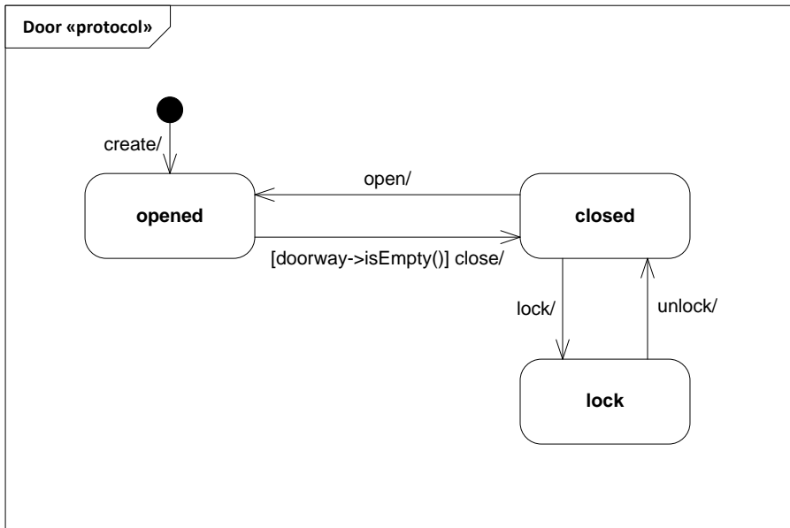
Figure 14.44 ProtocolStateMachine example
