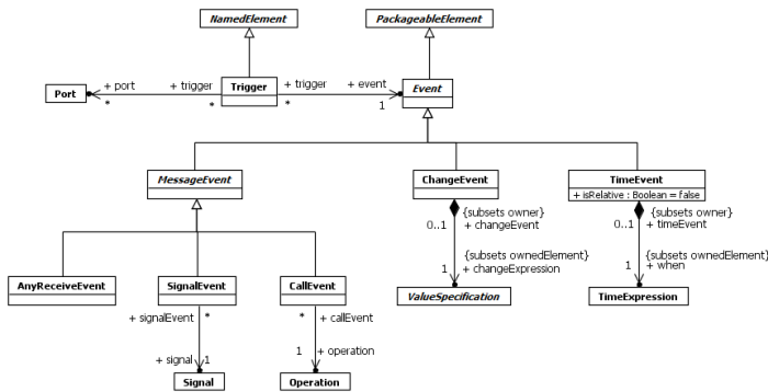
Figure 13.2 Events
