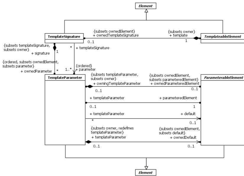
Figure 7.3 Templates
