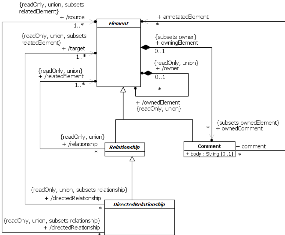
Figure 7.1 Root
