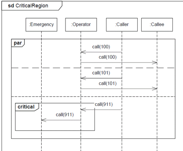
Figure 17.12 Critical Region
