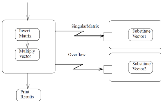
Figure 15.64 ExceptionHandler example
