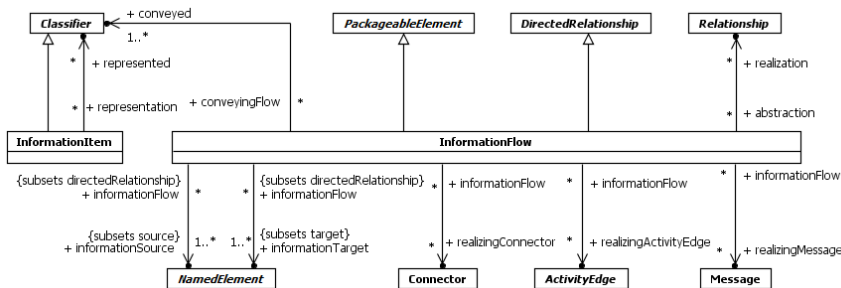
Figure 20.1 Information Flows
