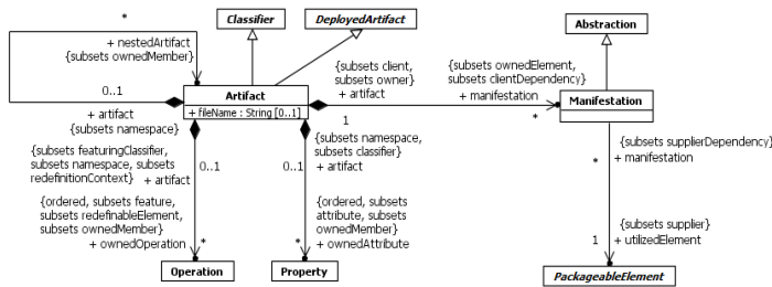
Figure 19.8 Artifacts
