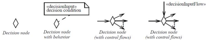
Figure 15.33 DecisionNode notation
