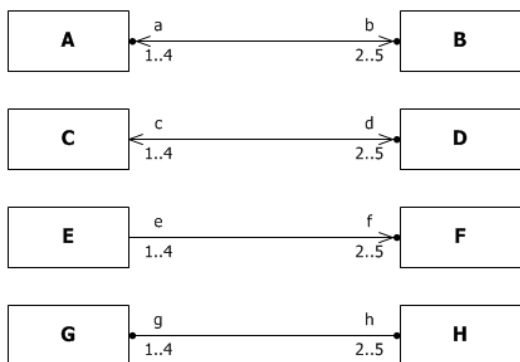
Figure 11.30 Examples of class-owned ends
