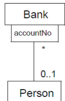
Figure . Qualified associations¶
