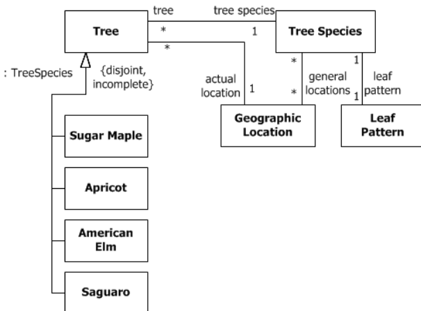
Figure 9.24 Power type example
