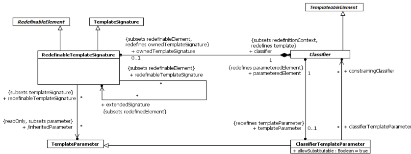
Figure 9.4 Classifier Templates
