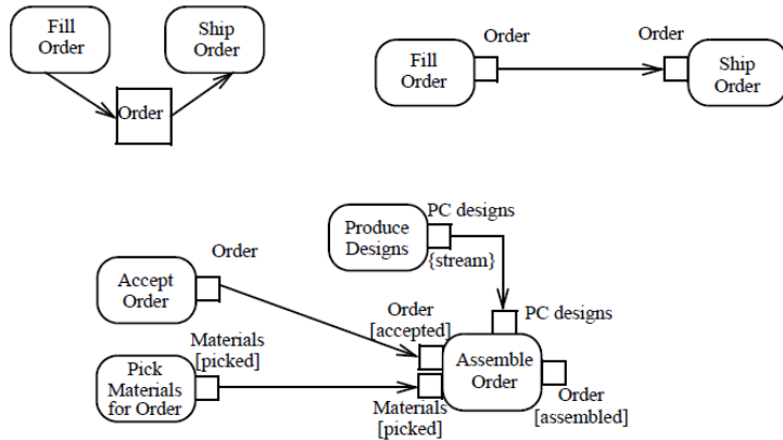
Figure 16.10 Pin examples
