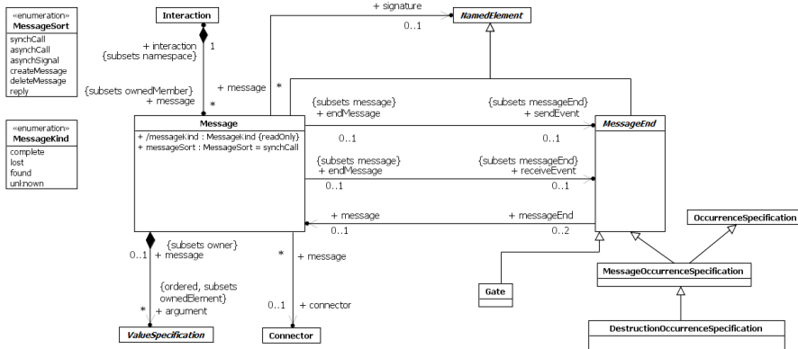
Figure 17.7. Messages
