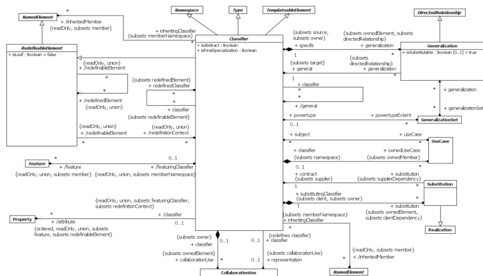
Figure 9.1 Classifiers
