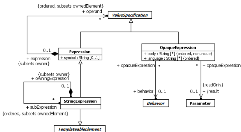
Figure 8.2 Expressions
