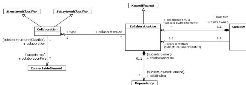
Figure 11.49 Collaborations
