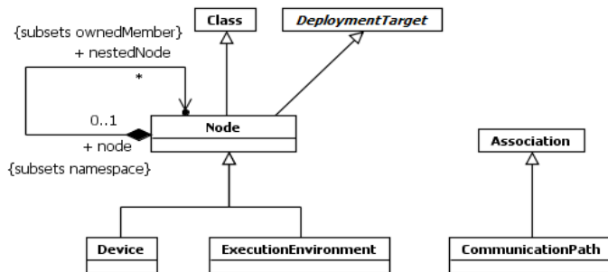
Figure 19.11 Nodes
