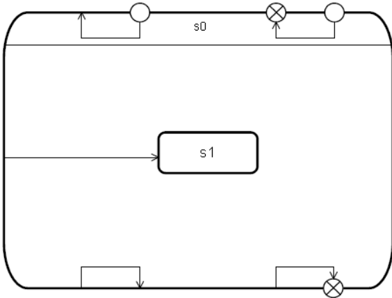
Figure 14.34 Local Transitions
