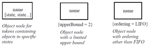
Figure 15.50 ObjectNode annotations
