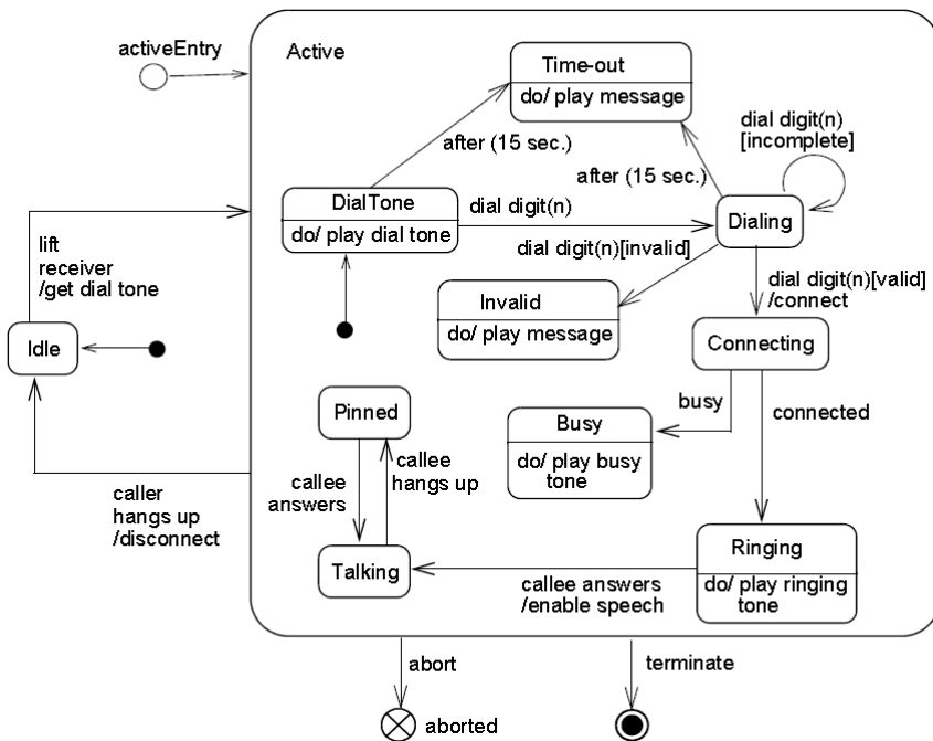
Figure 14.36 StateMachine diagram representing a telephone
