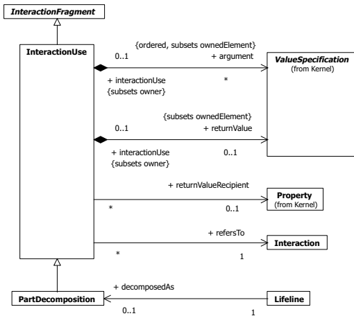
Figure 14.8 - InteractionUses
