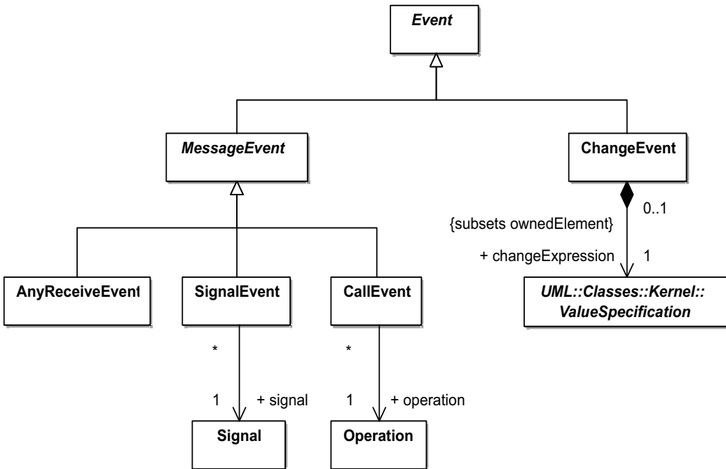
Figure 13.12 - Events
