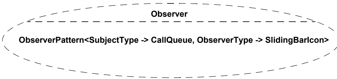
Figure 17.19 - Bound Collaboration
