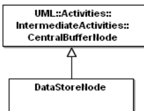
Figure 12.17 - Data stores
