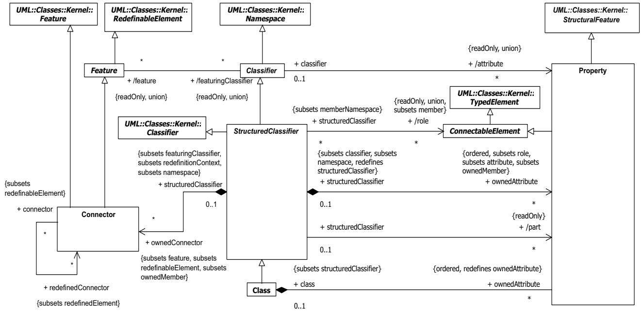
Package InternalStructures Figure 9.2 - Structured classifier
