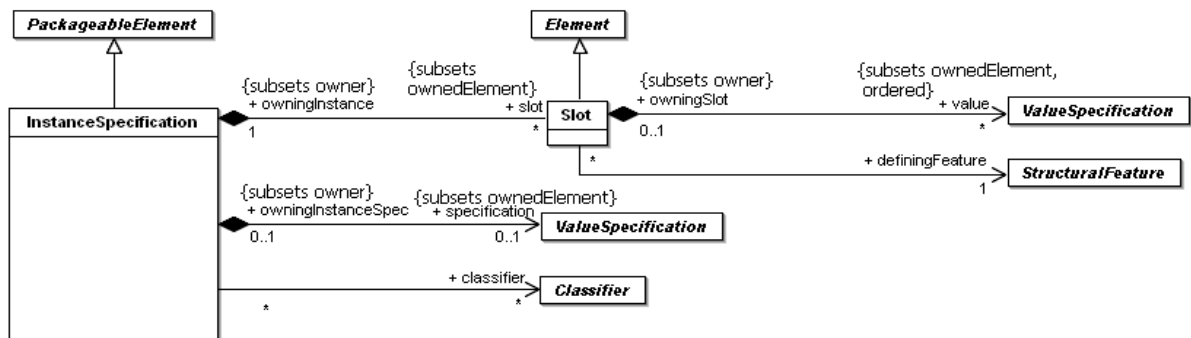
Figure 7.8 - Instances diagram of the Kernel package
