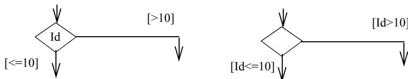
Figure 15.26 - Alternative Notation for Choice Pseudostate
