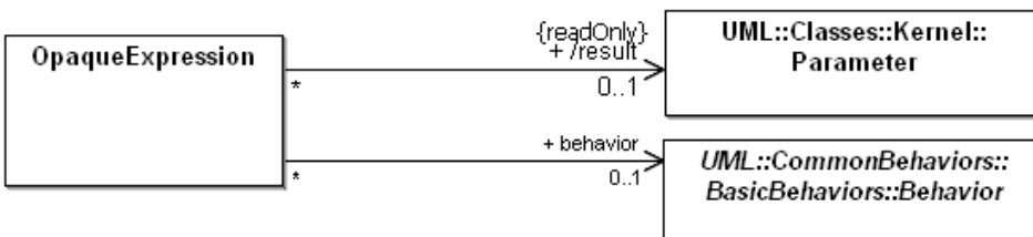
Figure 13.7 - Expression
