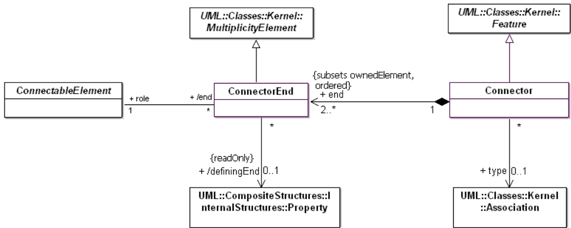
Figure 9.3 - Connectors
