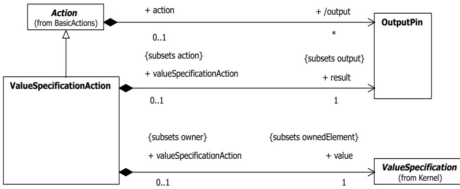
Figure 11.11 - Miscellaneous actions
