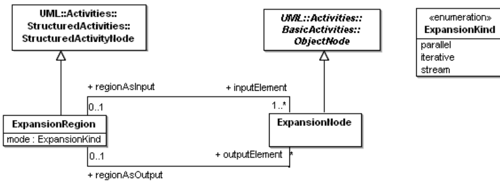
Figure 12.24 - Expansion regions
