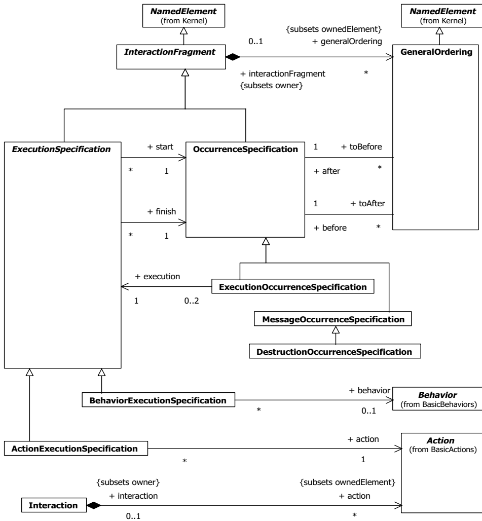
Figure 14.5 - Occurrences
