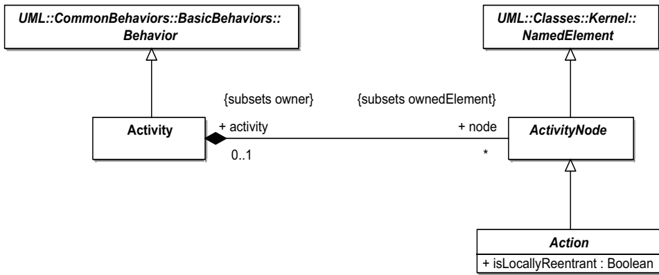
Figure 12.2 - Fundamental nodes
