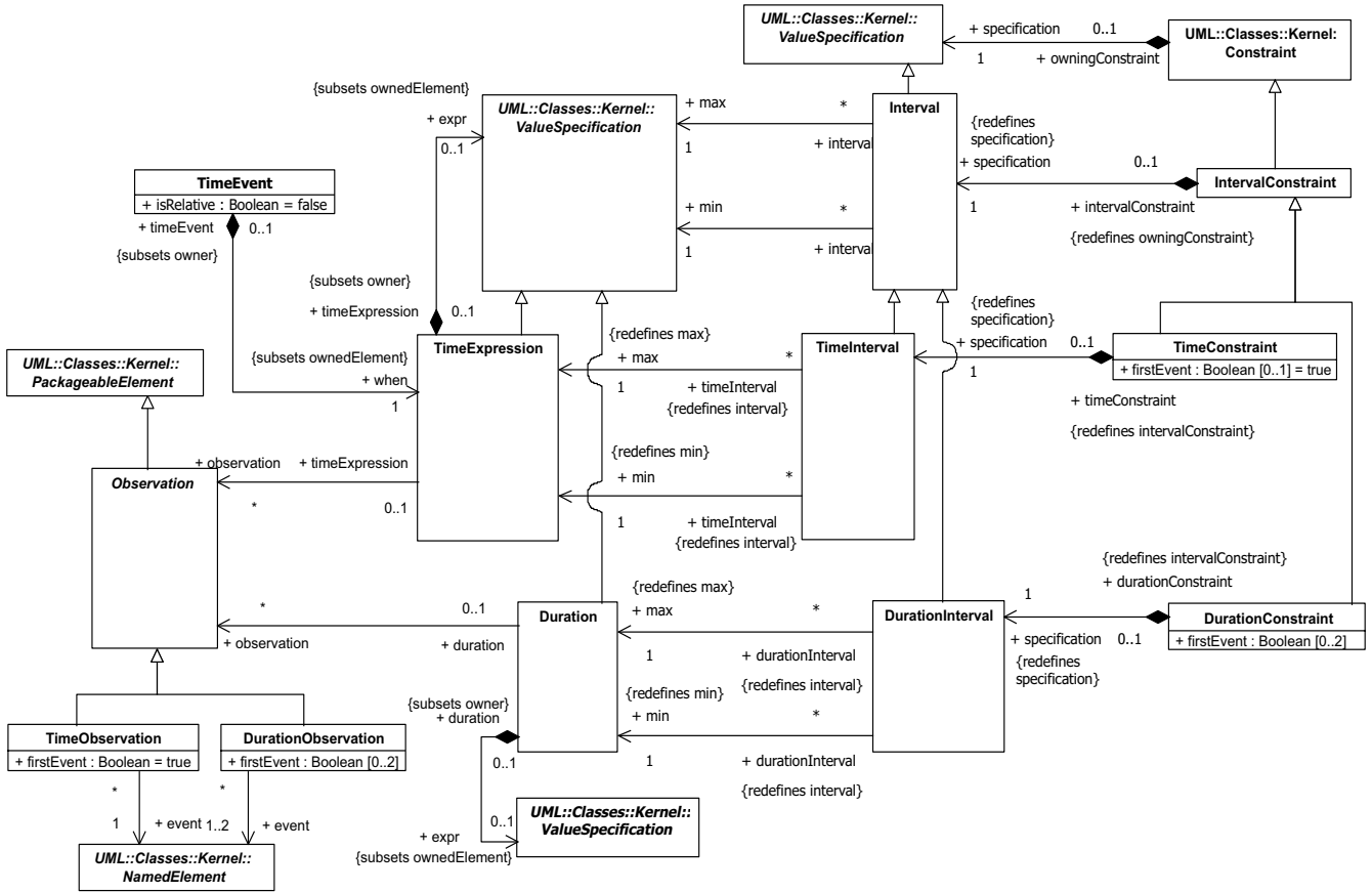
Figure 13.13 - SimpleTime
