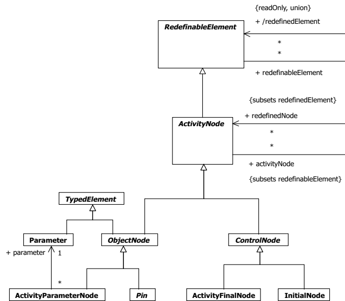
Figure 12.4 - Nodes (BasicActivities)
