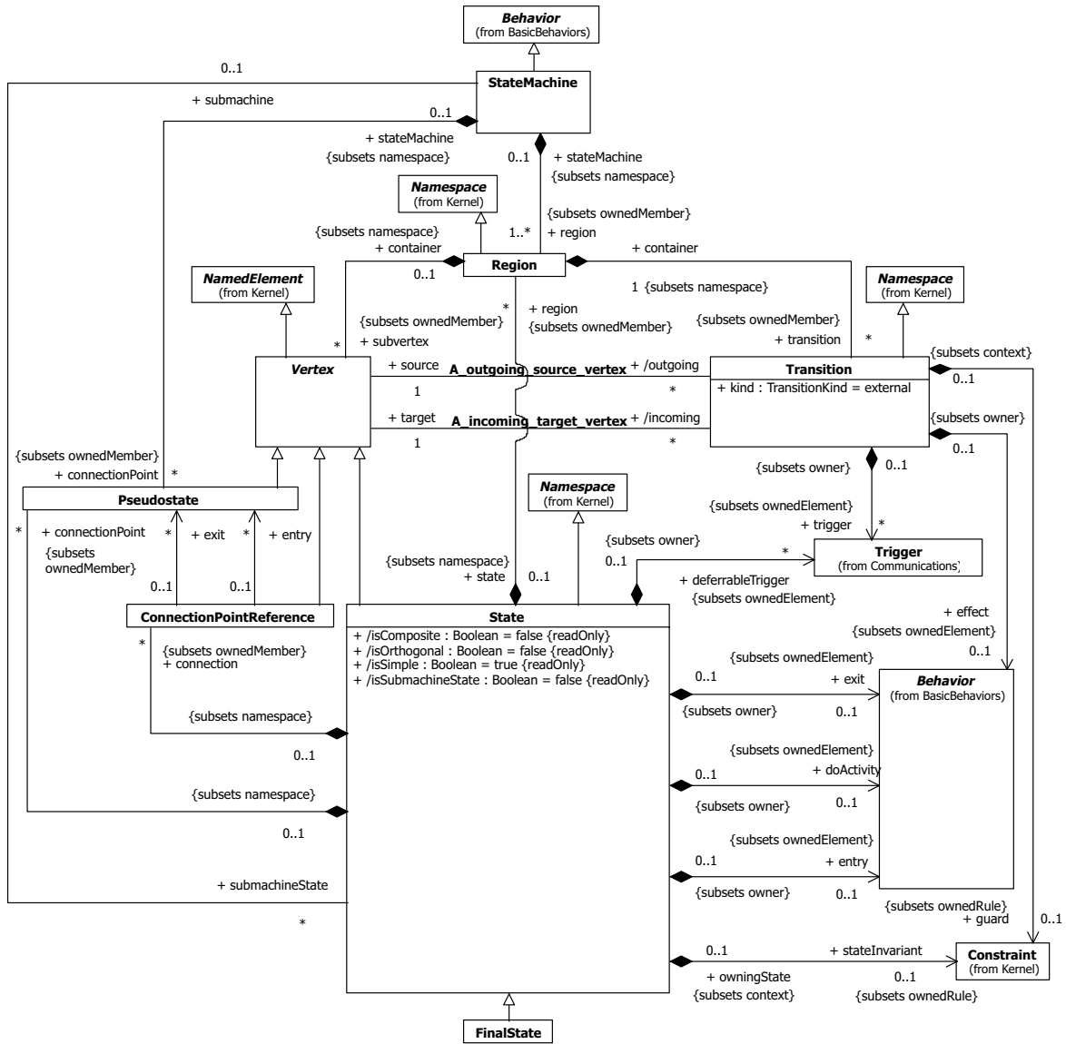
Figure 15.2 - State Machines
