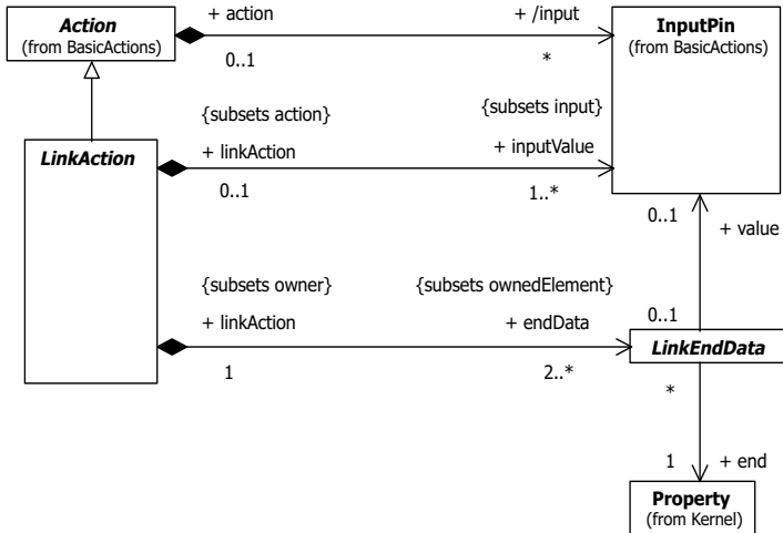
Figure 11.8 - Link identification
