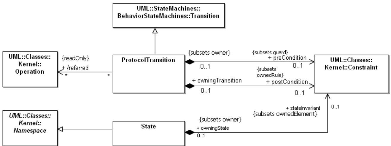
Figure 15.6 - Constraints
