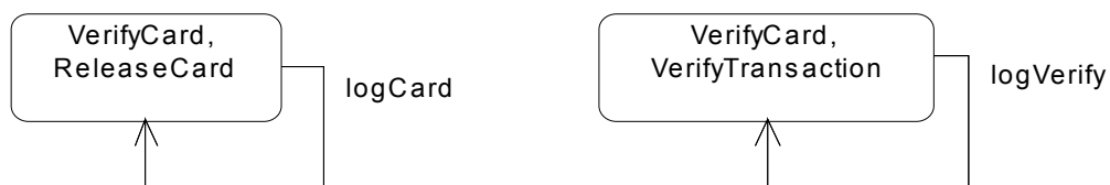
Figure 15.28 - State Lists
