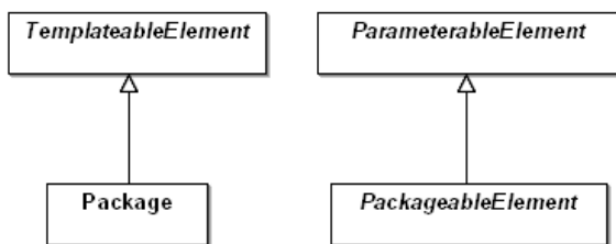
Figure 17.20 - Package templates
