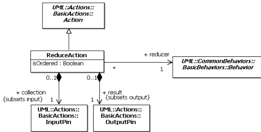
Figure 11.17 - ReduceAction (CompleteActions)
