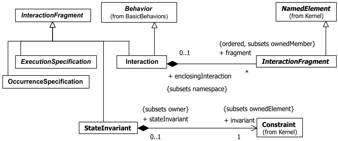
Figure 14.2 - Interactions
