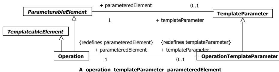
Figure 17.24 - Operation templates and parameters
