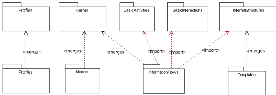
Figure 17.1 - Dependencies between packages described in this clause
