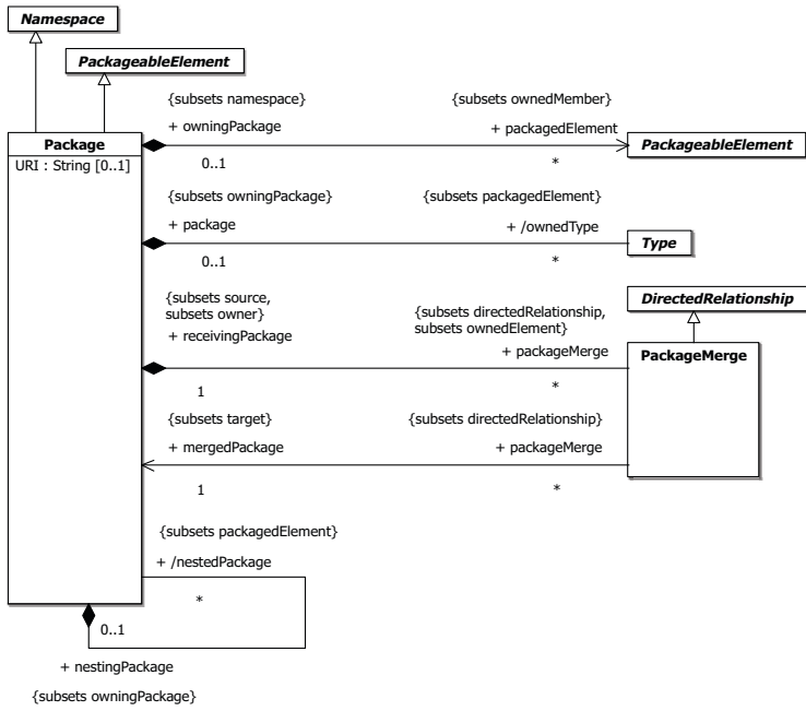
Figure 7.14 - The Packages diagram of the Kernel package
