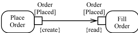
Figure 12.131 Pin example with effects
