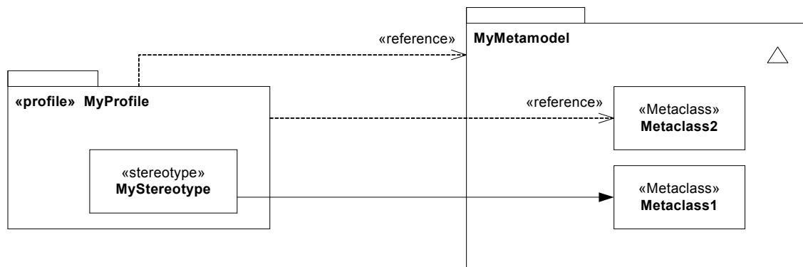
Figure 18.8 - Specification of an accessible metaclass
