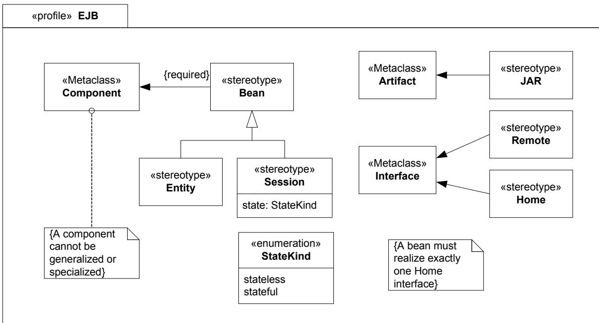
Figure 18.10 - Defining a simple EJB profile
