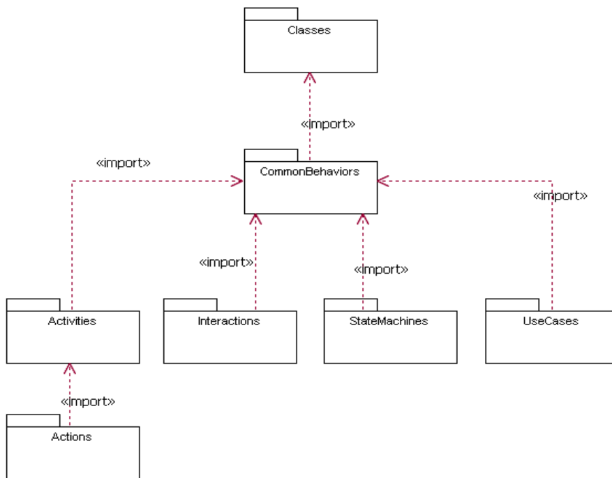
Part II, Figure 1 - UML packages that support behavioral modeling
