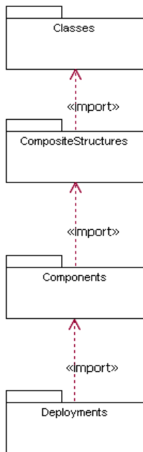
Part I, Figure 1 - UML packages that support structural modeling
