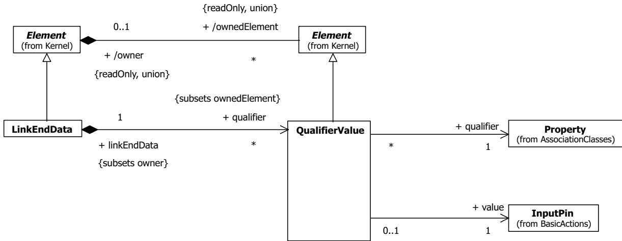
Figure 11.14 - Link identification (CompleteActions)
