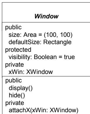
Figure 7.29 - Class notation: attributes and
