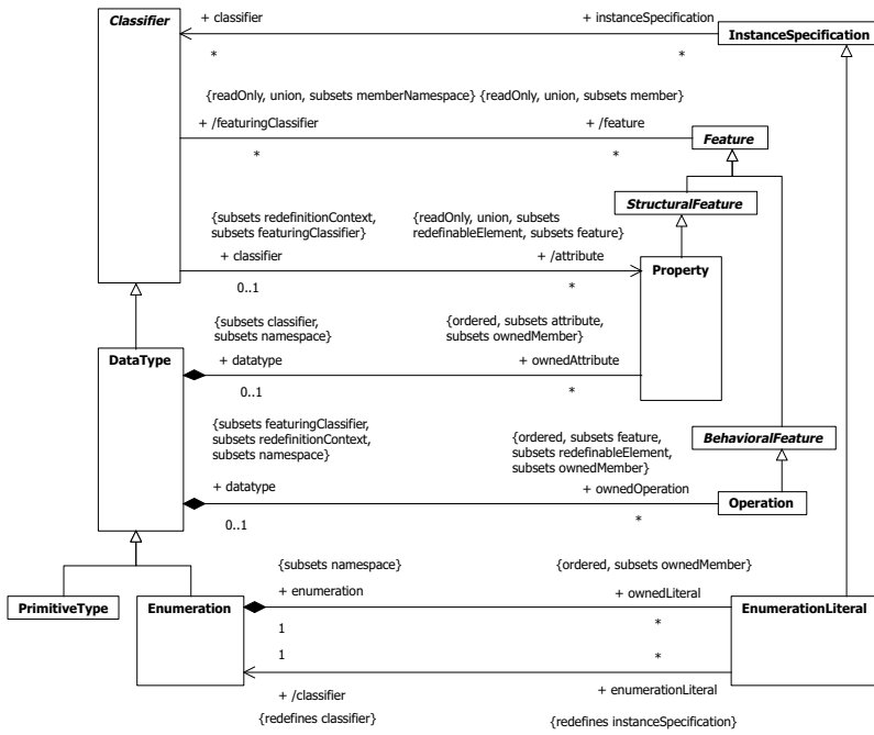
Figure 7.13 - DataTypes diagram of the Kernel package
