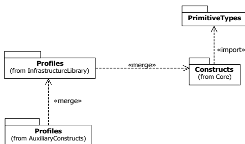
Figure 18.1 - Dependencies between packages described in this clause
