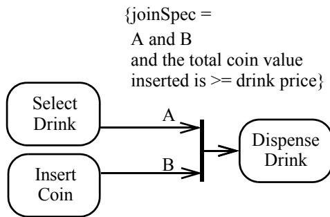
Figure 12.104 - Join node example
