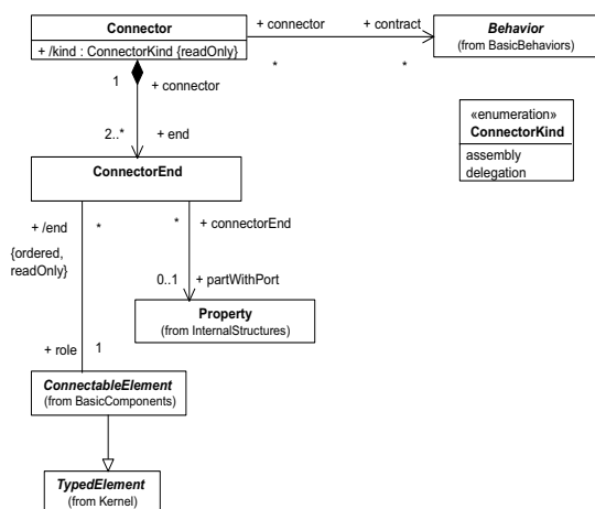
Figure 8.3 - The metaclasses that define the component wiring constructs
