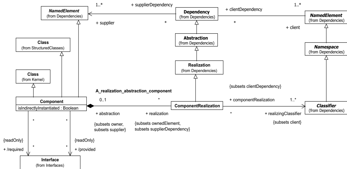
Figure 8.2 - The metaclasses that define the basic Component construct
