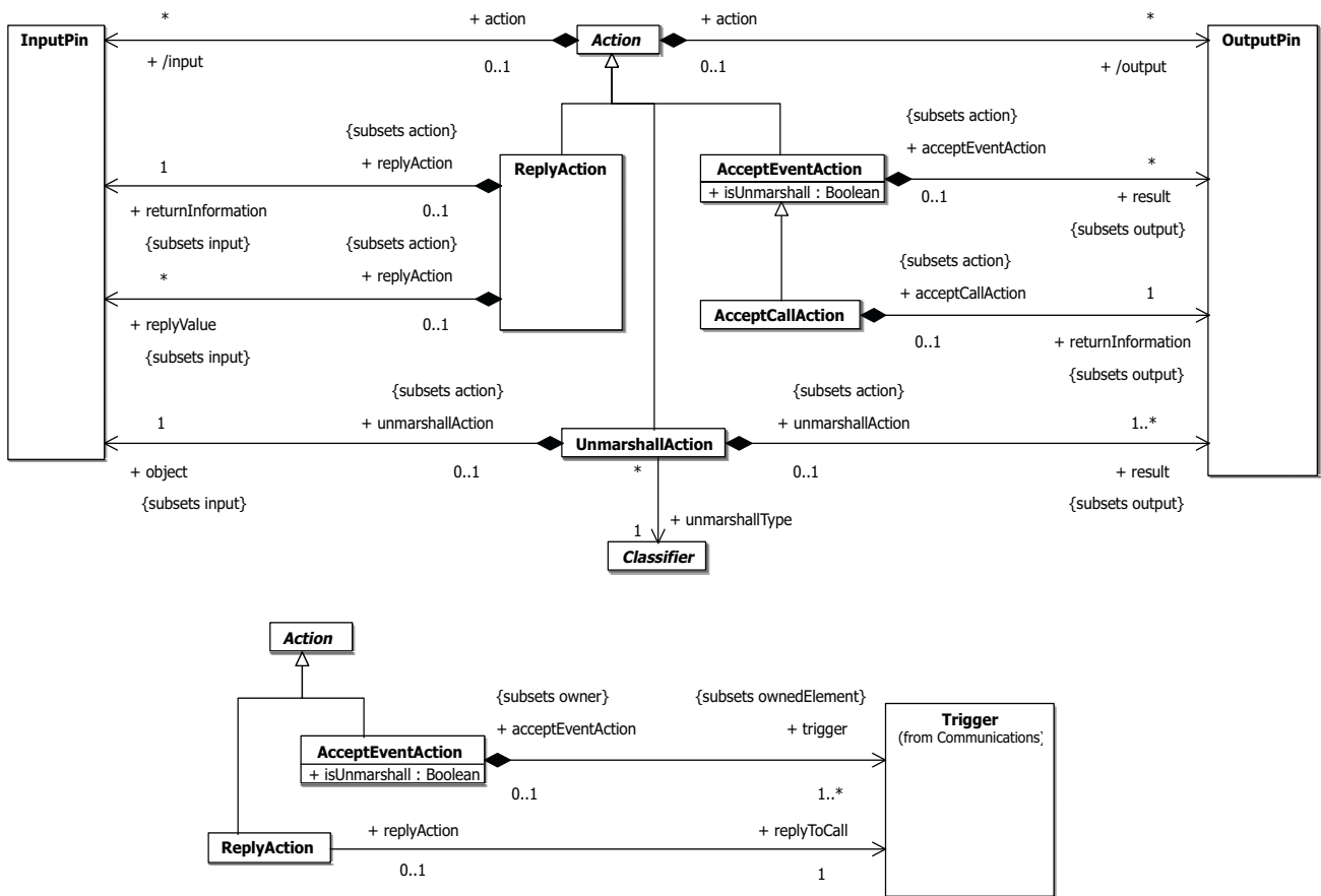
Figure 11.12 - Accept event actions
