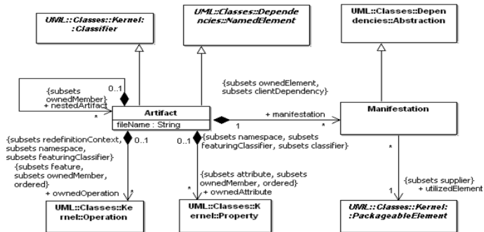
Figure 10.2 - The elements defined in the Artifacts package
