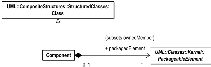
Figure 8.4 - The packaging capabilities of Components
