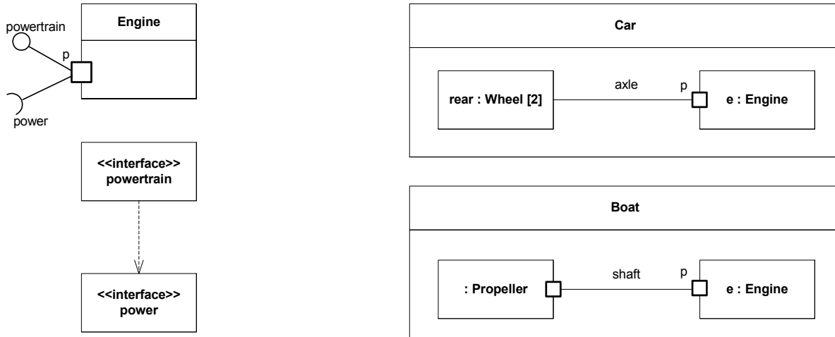
Figure 9.19 - Port examples
