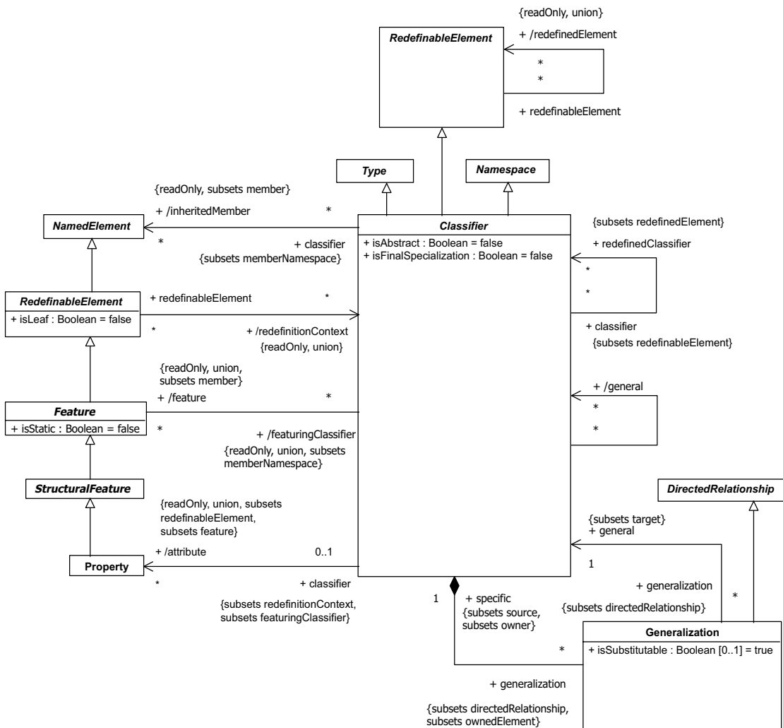
Figure 7.9 - Classifiers diagram of the Kernel package
