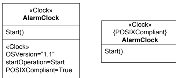
Figure 18.20 - Other notational forms for depicting stereotype values
