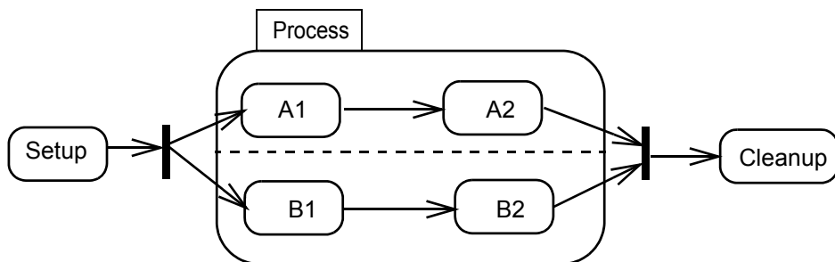
Figure 15.25 - Fork and Join
