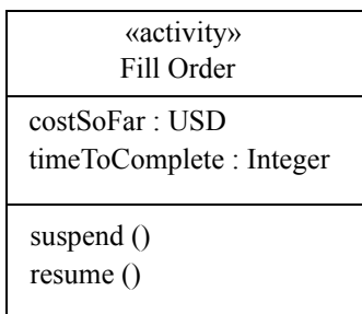
Figure 12.38 - Activity class with attributes and operations
