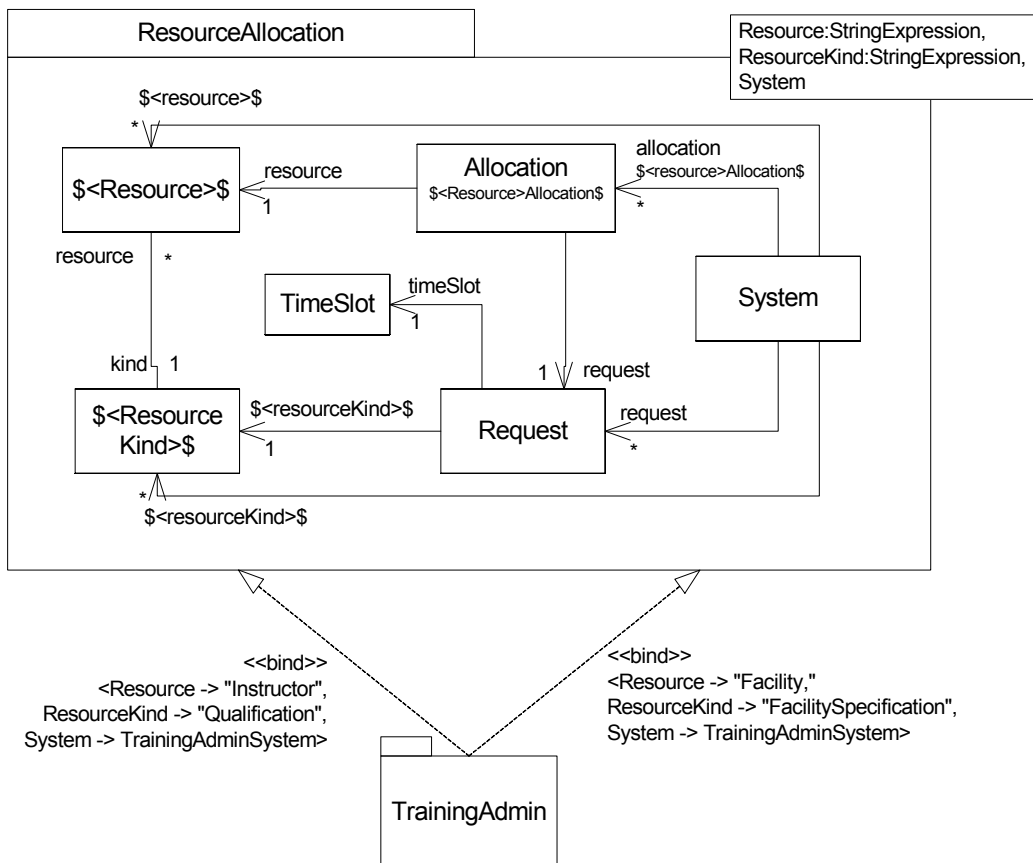
Figure 17.23 - Template Package with string parameters
