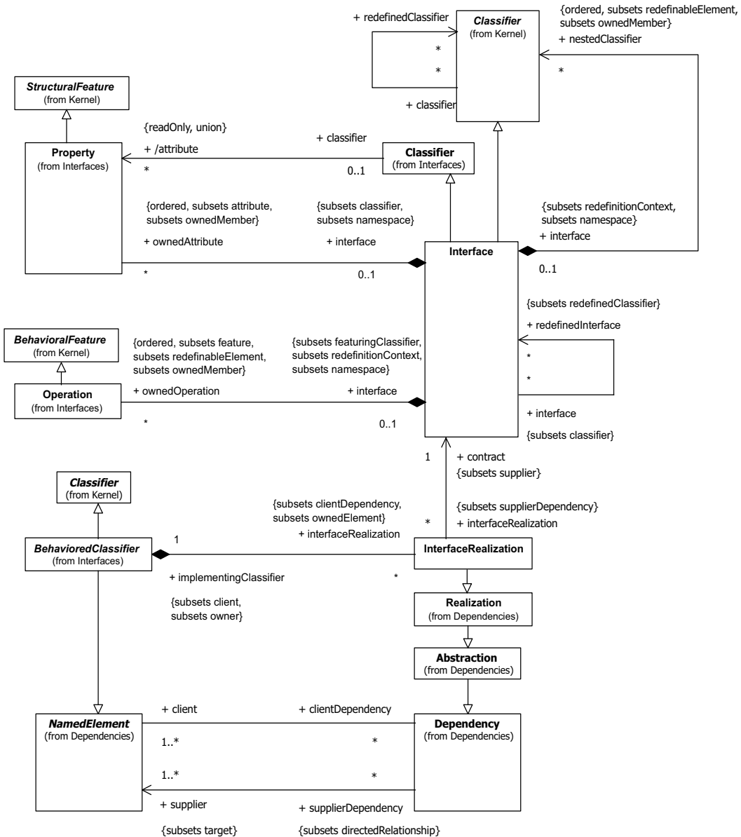
Figure 7.16 - Contents of Interfaces package
