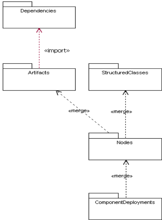
Figure 10.1 - Dependencies between packages described in this clause
