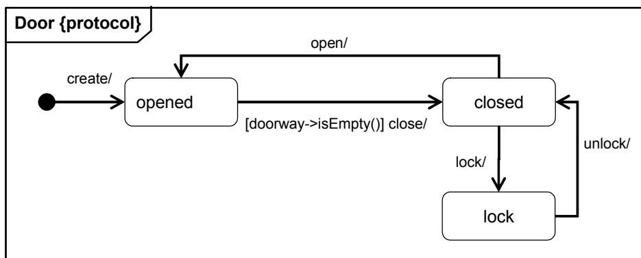
Figure 15.12 - Protocol state machine
