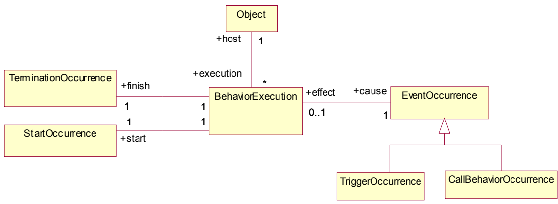
Figure 13.2 - Invocation Domain Model
