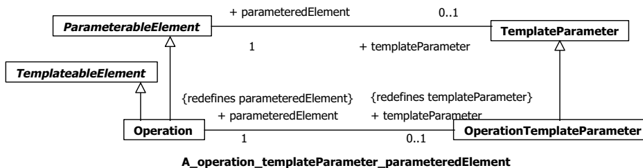
Figure 17.24 - Operation templates and parameters
