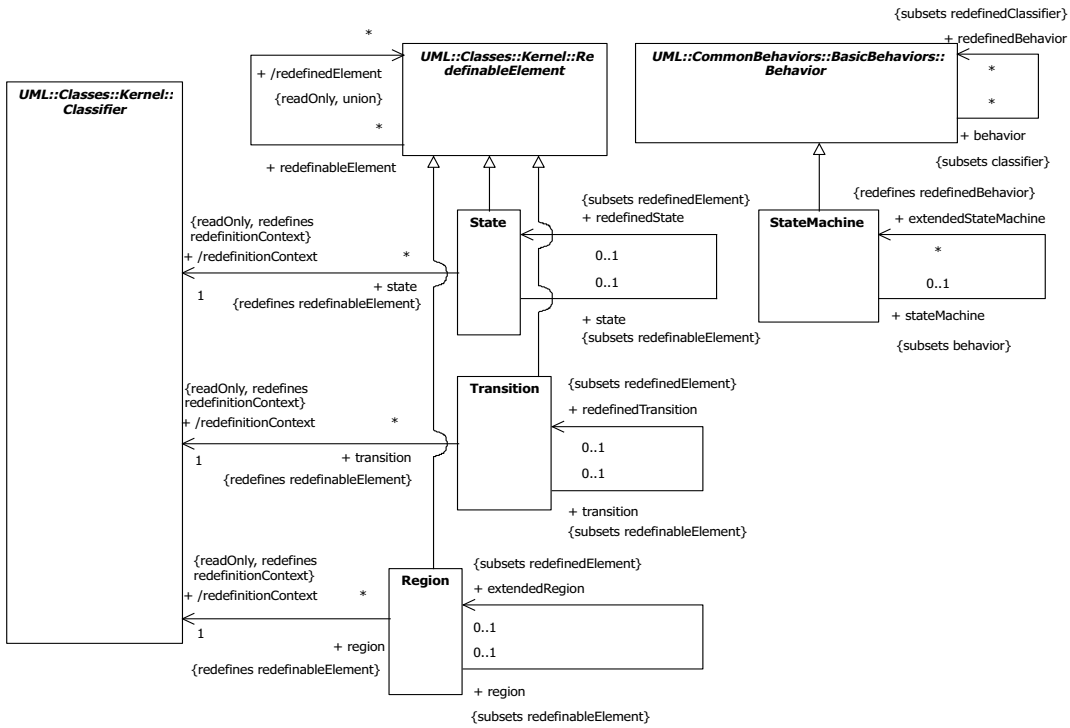
Figure 15.3 - State Machine Redefinitions
