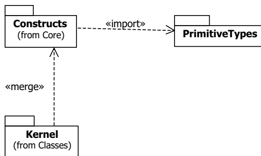
Figure 7.1 - InfrastructureLibrary packages that are merged by Kernel (all dependencies in the picture represent package merges)
