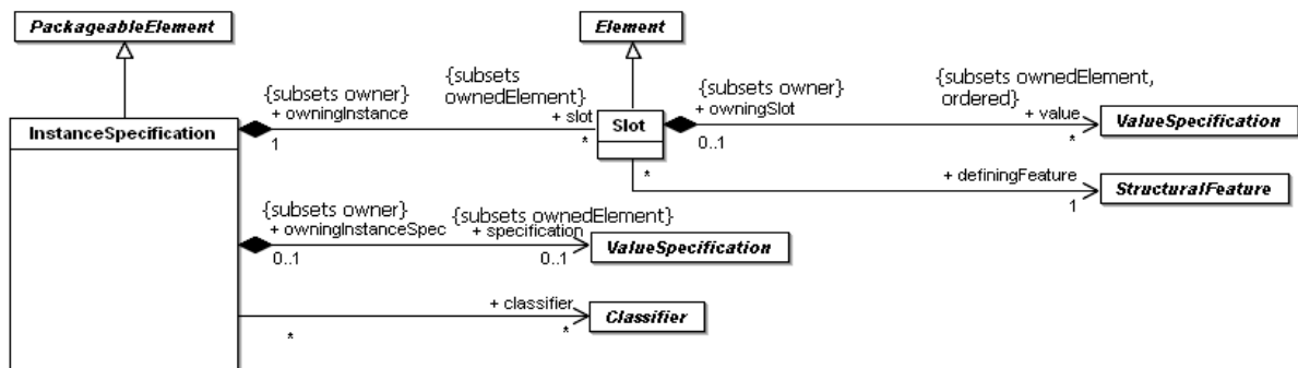
Figure 7.8 - Instances diagram of the Kernel package
