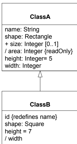
Figure 7.30 - Examples of attributes
