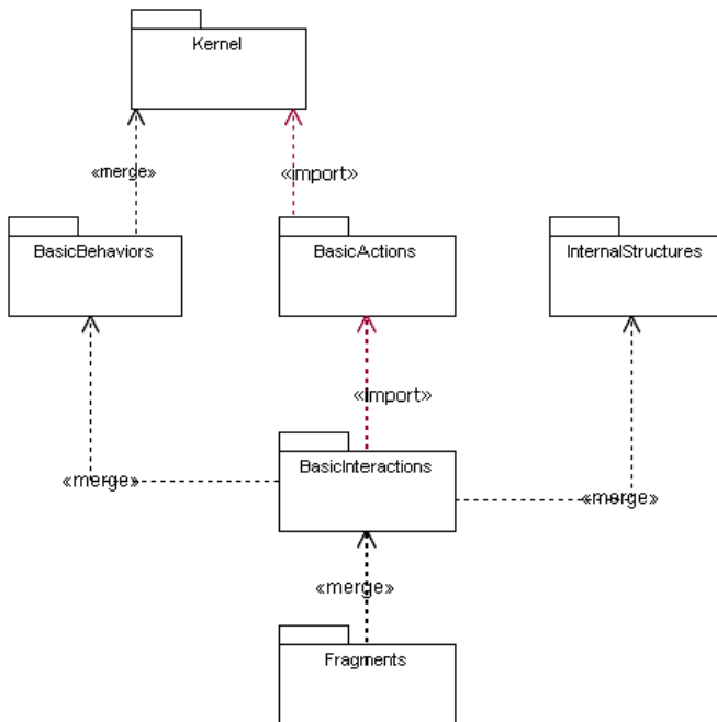
Figure 14.1 - Dependencies of the Interactions packages
