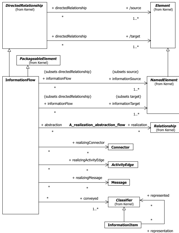
Figure 17.2 - The contents of the InformationFlows package
