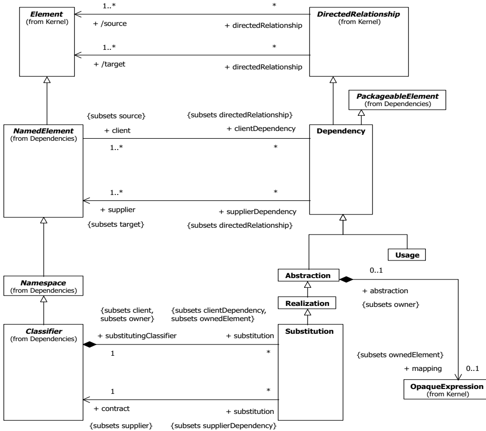
Figure 7.15 - Contents of Dependencies package
