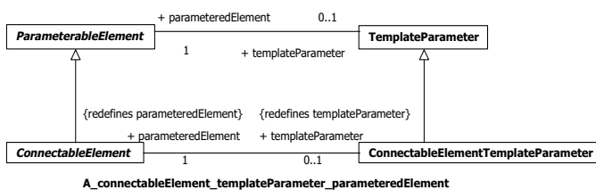
Figure 17.25 - Connectable element template parameters
