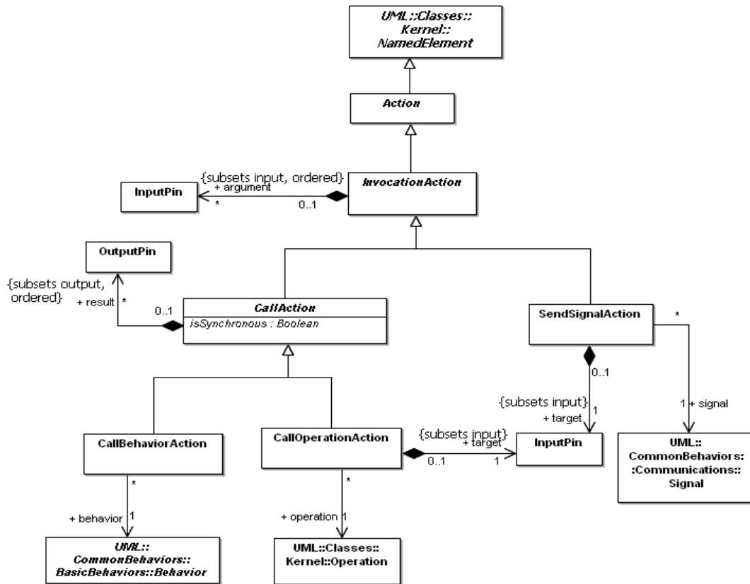
Figure 11.4 - Basic invocation actions
