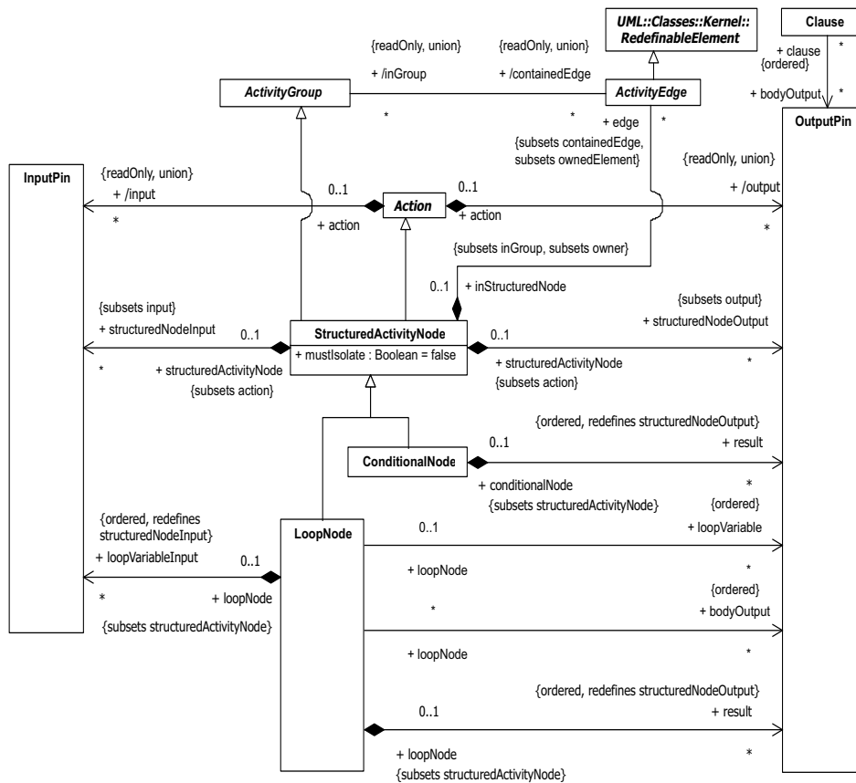
Figure 12.22 - Structured nodes (CompleteStructuredActivities)
