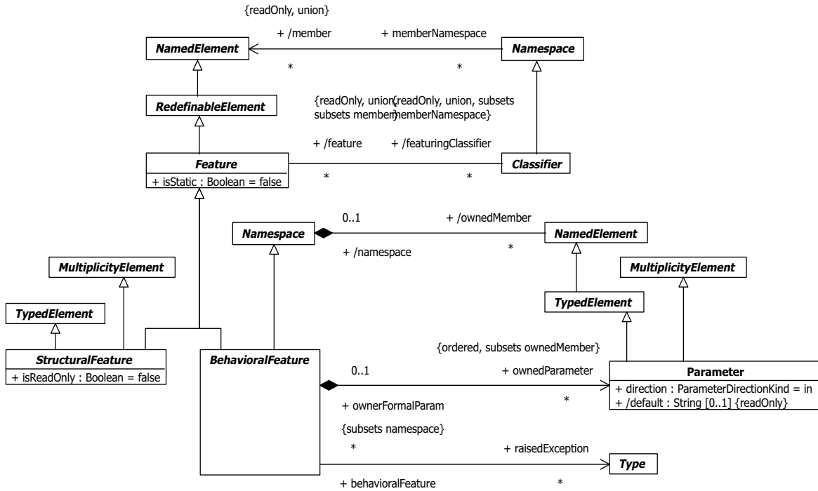
Figure 7.10 - Features diagram of the Kernel package
