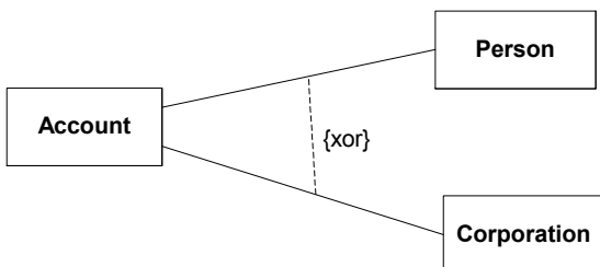
Figure 9.15 - {xor} constraint
