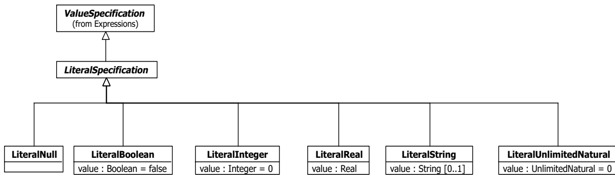
Figure 9.30 - The elements defined in the Literals package
