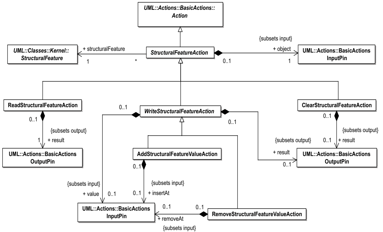
Figure 11.7 - Structural Feature Actions
