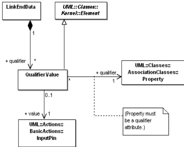
Figure 11.14 - Link identification (CompleteActions)
