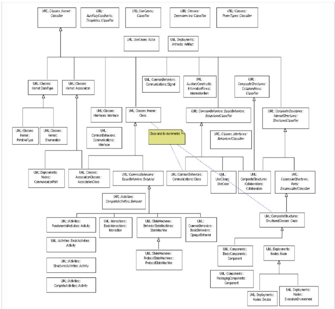
Figure F.1 - Classifier hierarchy for UML 2.0 Superstructure
