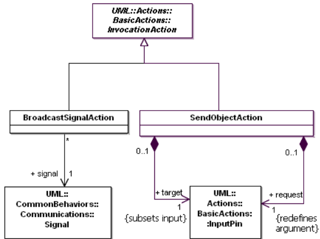
Figure 11.5 - Intermediate invocation actions
