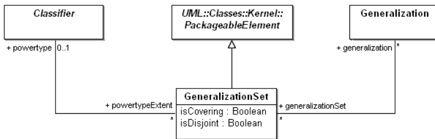
Figure 7.18 - Contents of PowerTypes package
