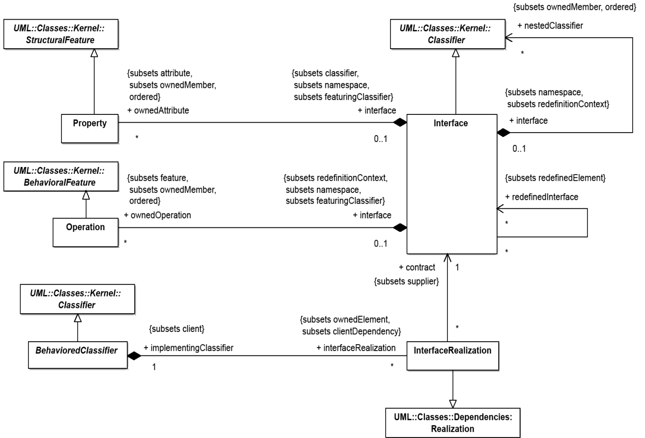
Figure 7.16 - Contents of Interfaces package
