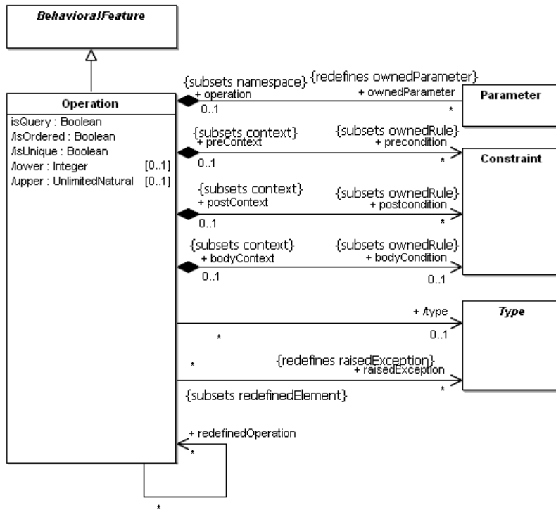
Figure 7.11 - Operations diagram of the Kernel package
