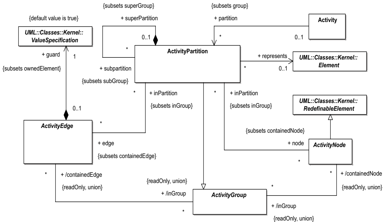
Figure 12.10 - Partitions
