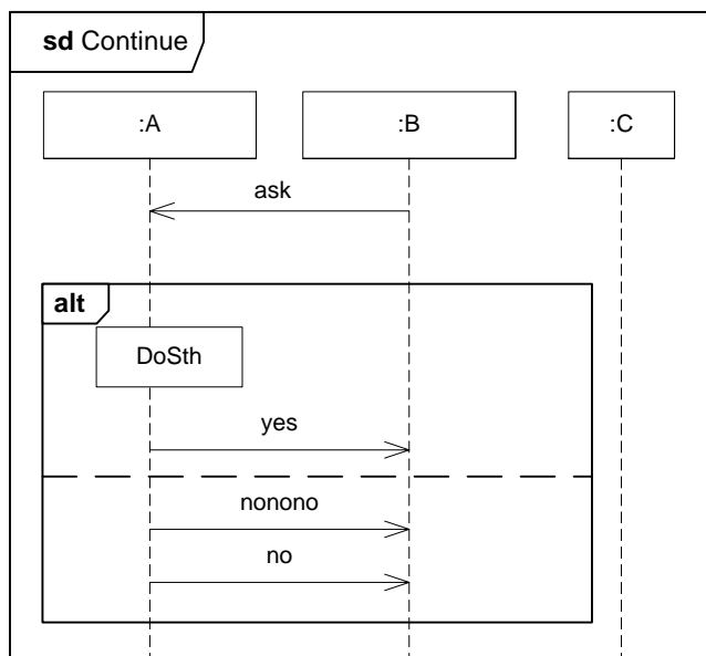
Figure 14.14 - Continuation interpretation
