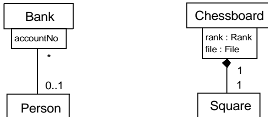
Figure 7.72 - Qualified associations
