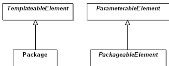
Figure 17.25 - Package templates
