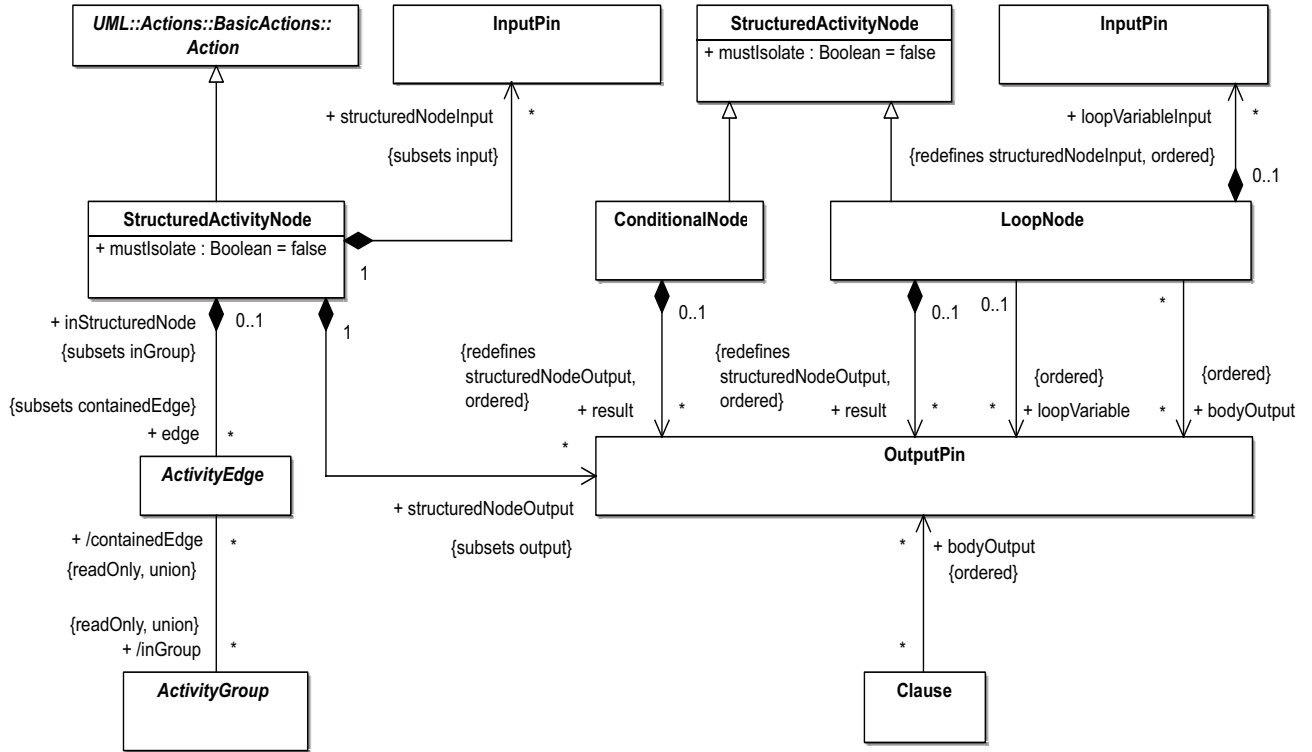
Figure 12.22 - Structured nodes (CompleteStructuredActivities)
