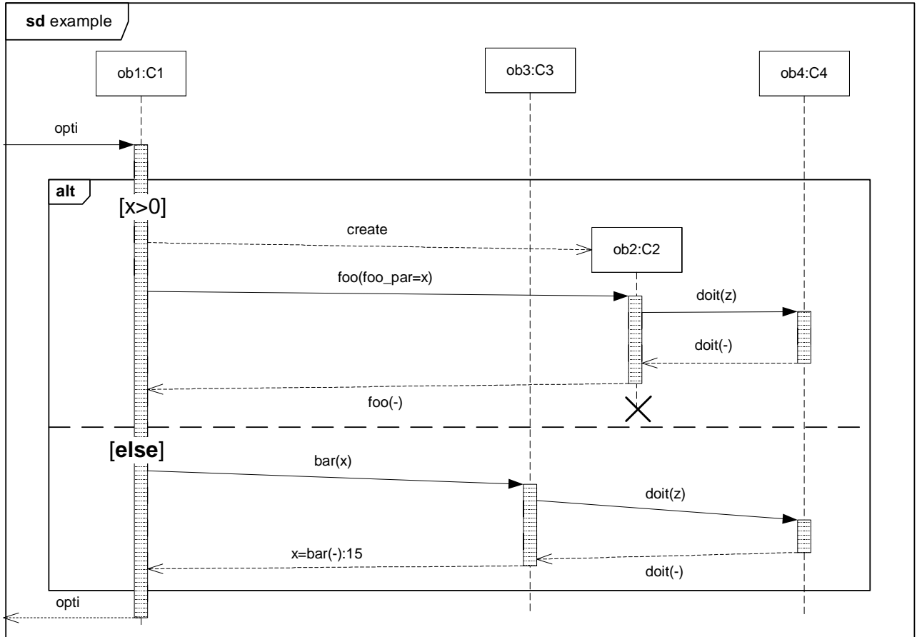
Figure 14.12 - CombinedFragment
