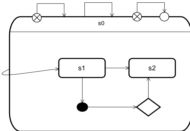
Figure 15.48 - External Transitions
