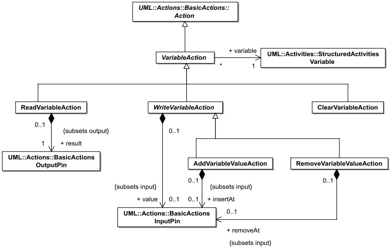
Figure 11.18 - Variable actions
