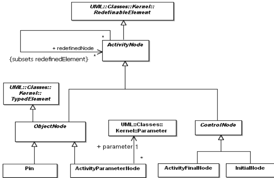
Figure 12.4 - Nodes (BasicActivities)
