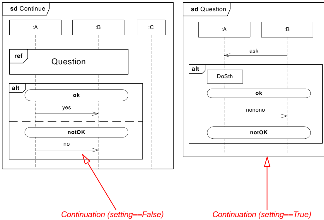
Figure 14.13 - Continuation
