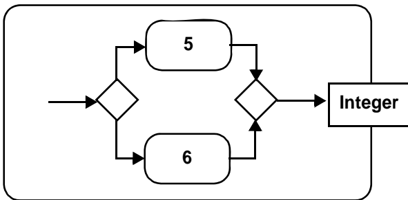
Figure 12.136 - Example ValueSpecificationAction
