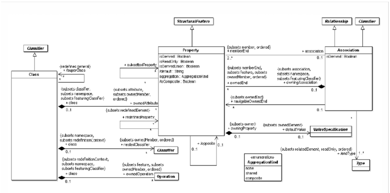
Figure 7.12 - Classes diagram of the Kernel package
