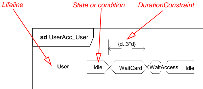
Figure 14.31 - Compact Lifeline with States
