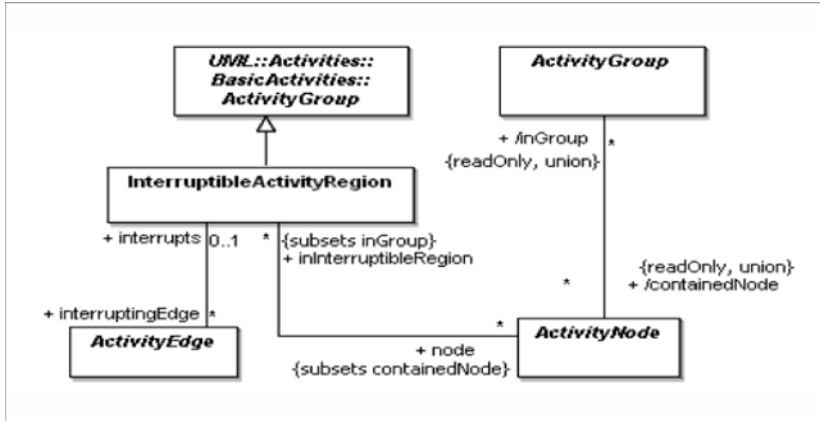
Figure 12.20 - Interruptible regions
