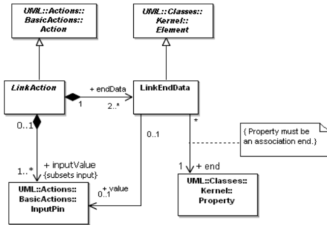
Figure 11.8 - Link identification
