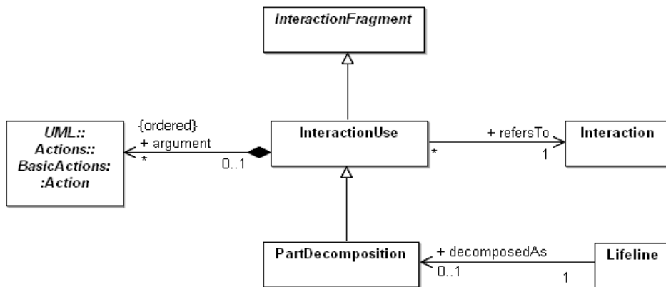
Figure 14.9 - InteractionUses
