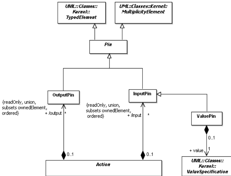
Figure 11.3 - Basic pins
