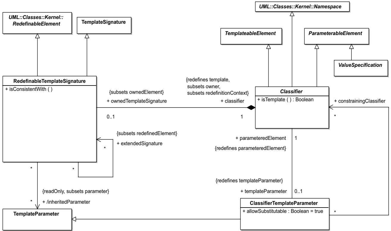
Figure 17.18 - Classifier templates
