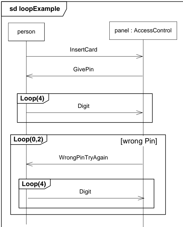
Figure 14.11 - Loop CombinedFragment
