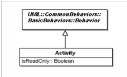
Figure 12.7 - Elements
