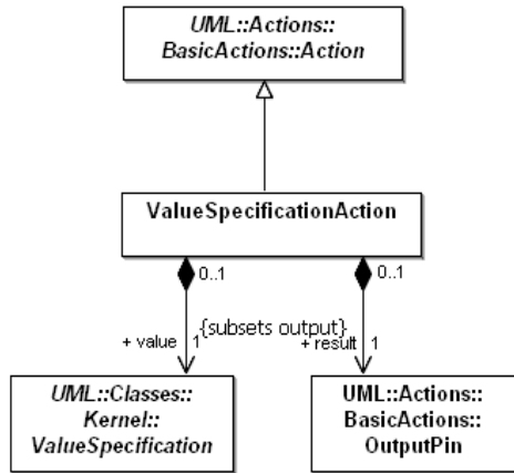
Figure 11.11 - Miscellaneous actions
