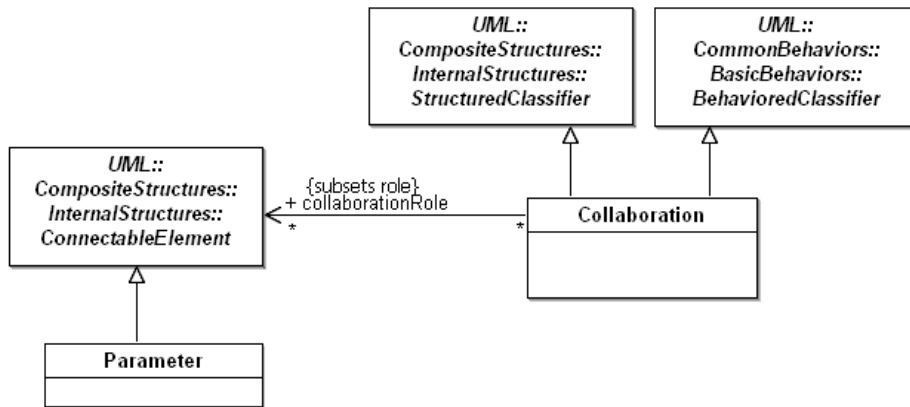
Figure 9.6 - Collaboration
