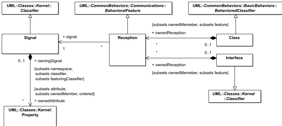
Figure 13.9 - Reception
