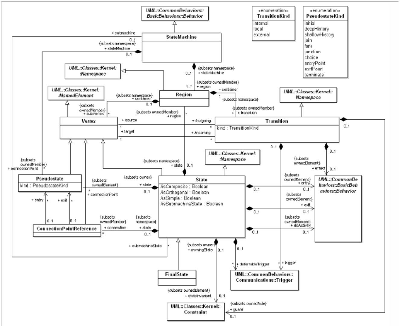
Figure 15.2 - State Machines
