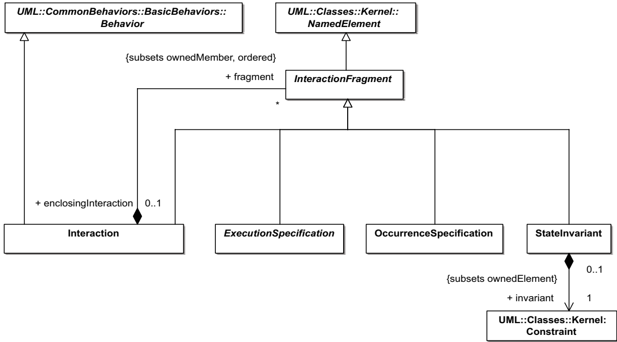
Figure 14.3 - Interactions
