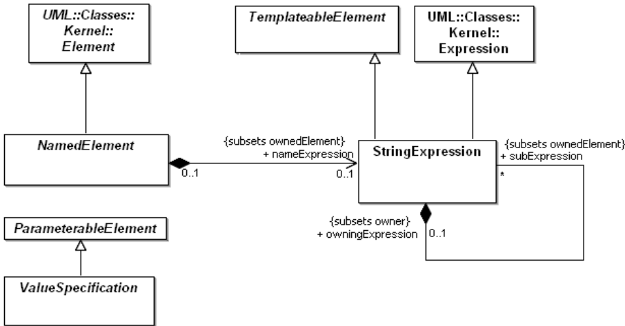
Figure 17.27 - Name expression
