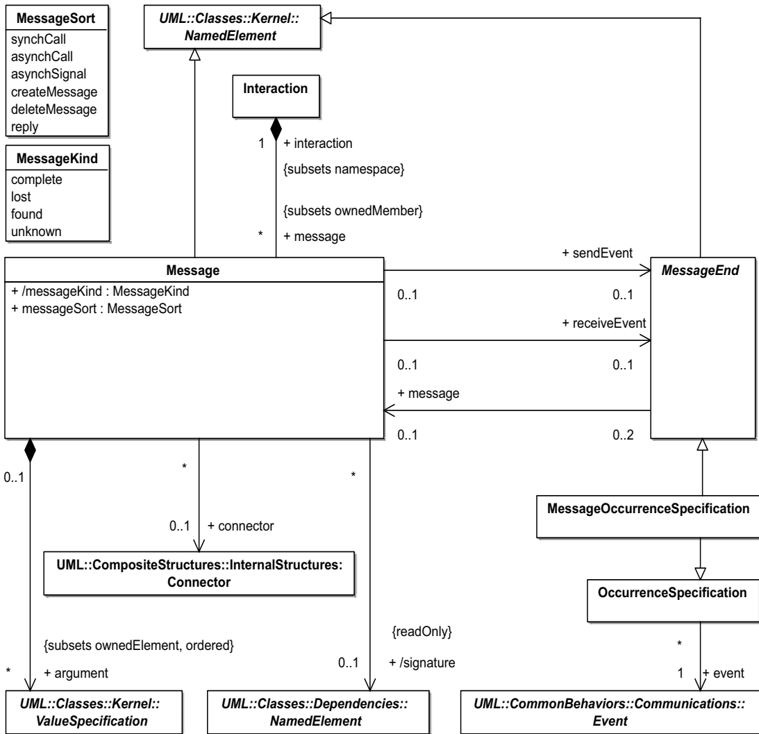
Figure 14.5 - Messages
