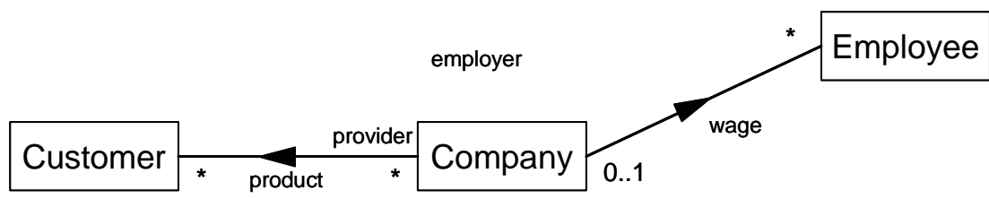
Figure 17.7 - Information Items attached to associations
