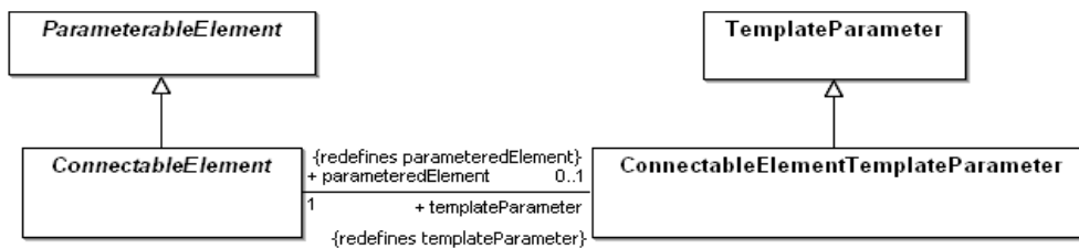
Figure 17.30 - Connectable element template parameters
