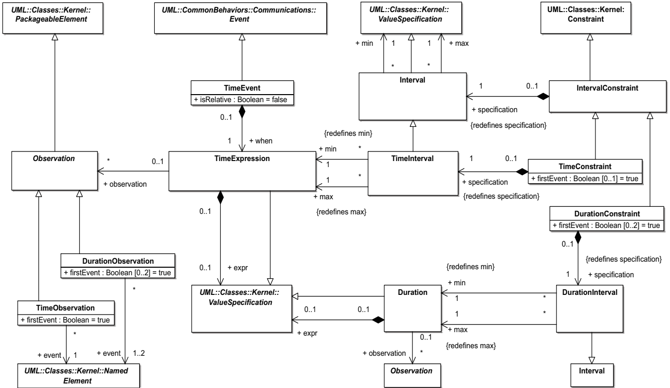
Figure 13.13 - SimpleTime
