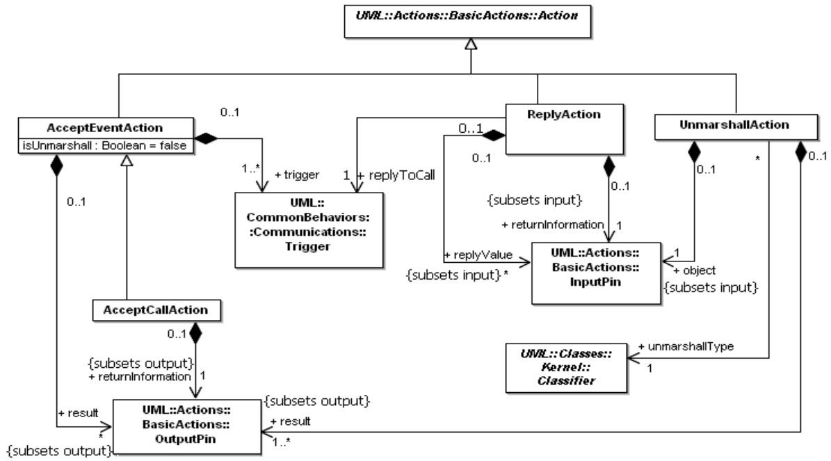
Figure 11.12 - Accept event actions
