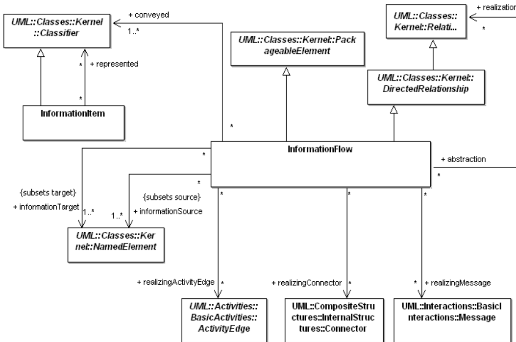
Figure 17.2 - The contents of the InformationFlows package
