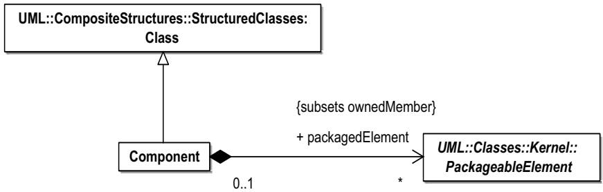
Figure 8.4 - The packaging capabilities of Components
