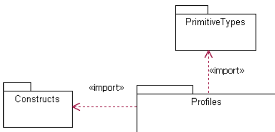
Figure 18.1 - Dependencies between packages described in this clause
