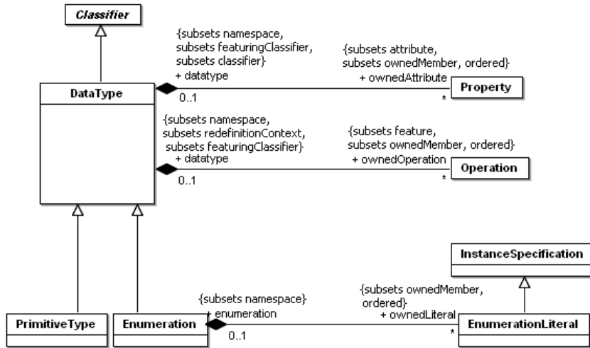
Figure 7.13 - DataTypes diagram of the Kernel package
