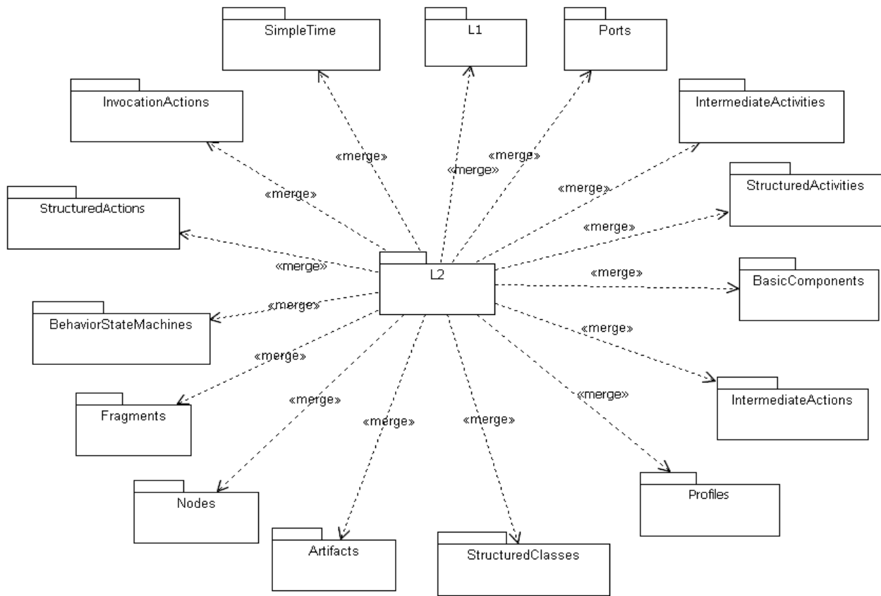
Figure 2.3 - Level 2 top-level package merges
