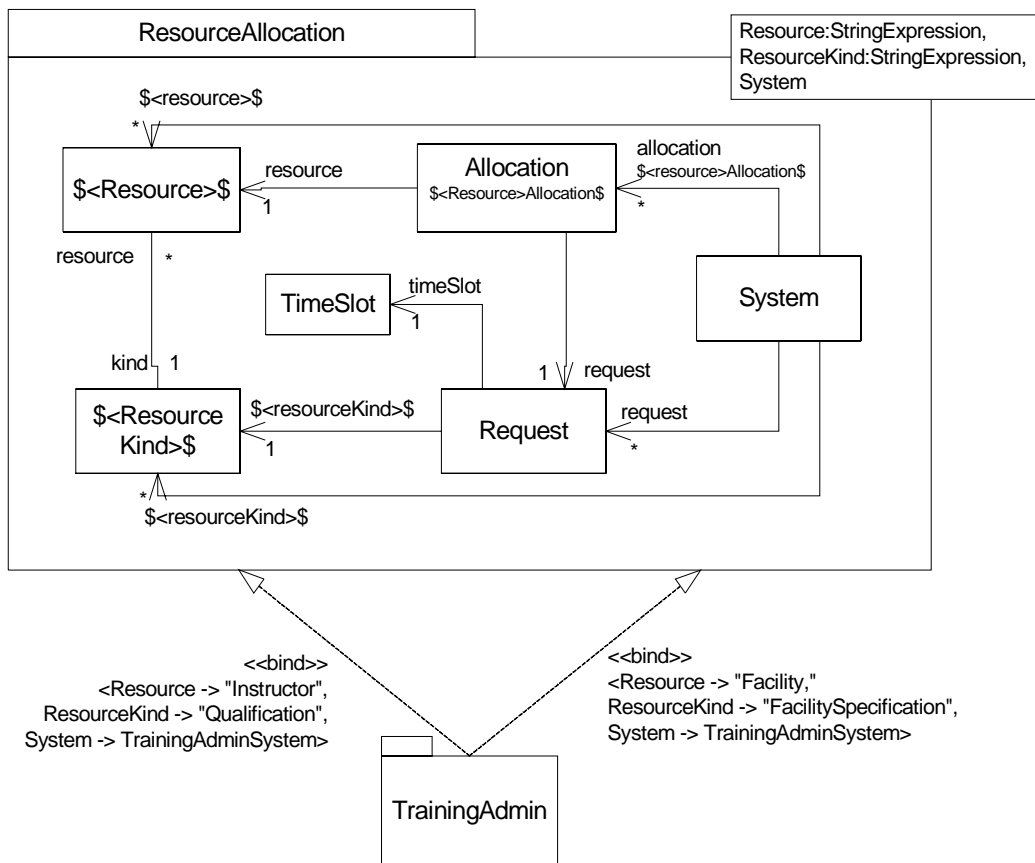
Figure 17.28 - Template Package with string parameters
