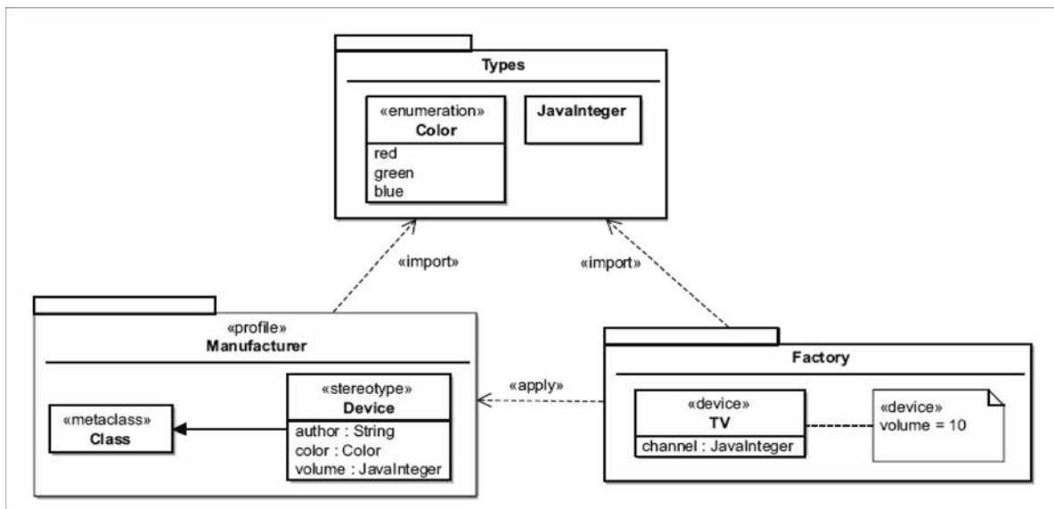
Figure 13.11 - Importing a package from a profile
