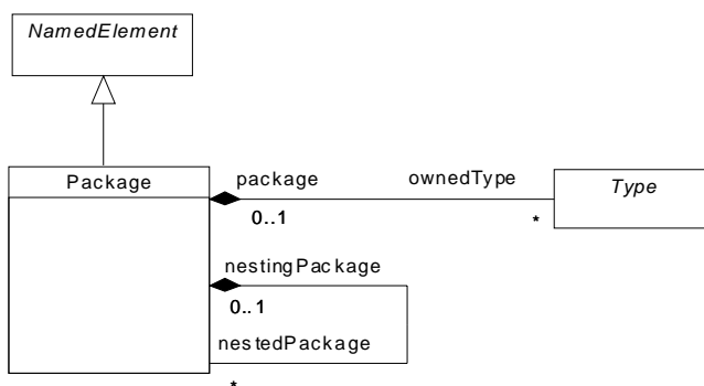
Figure 10.5 - The classes defined in the Packages diagram
