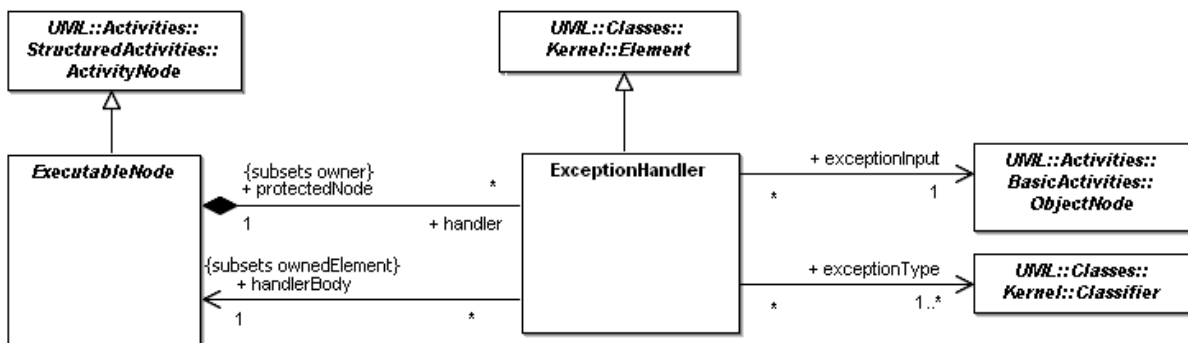
Figure 12.23 - Exceptions
