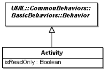
Figure 12.7 - Elements
