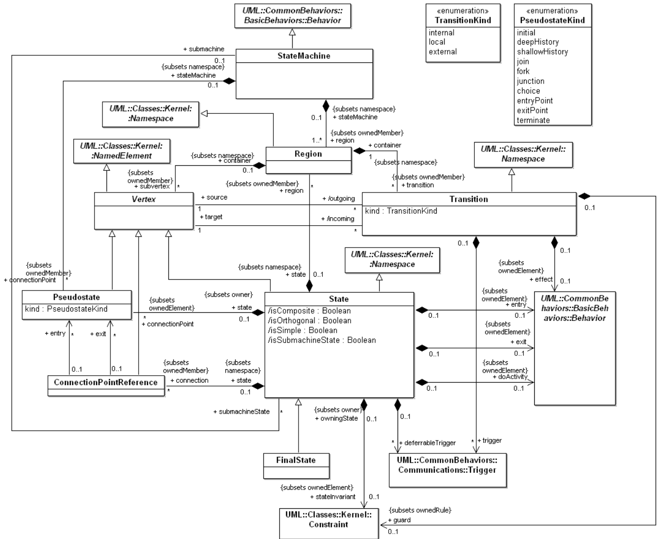
Figure 15.2 - State Machines
