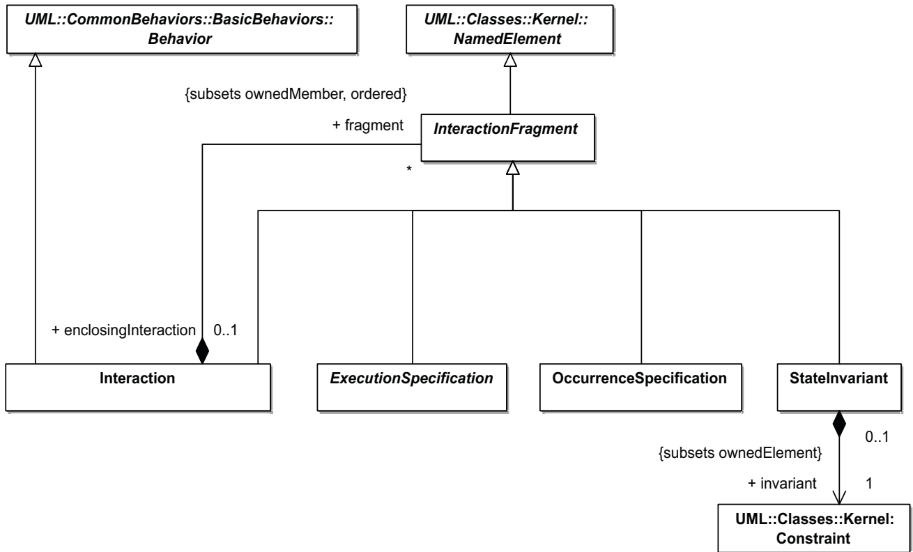
Figure 14.3 - Interactions
