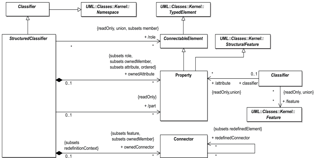
Figure 9.2 - Structured classifier
