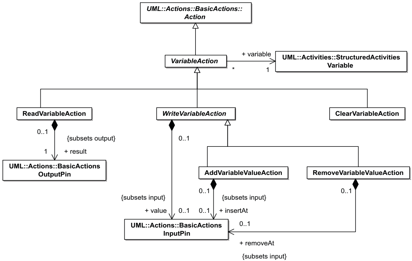
Figure 11.18 - Variable actions
