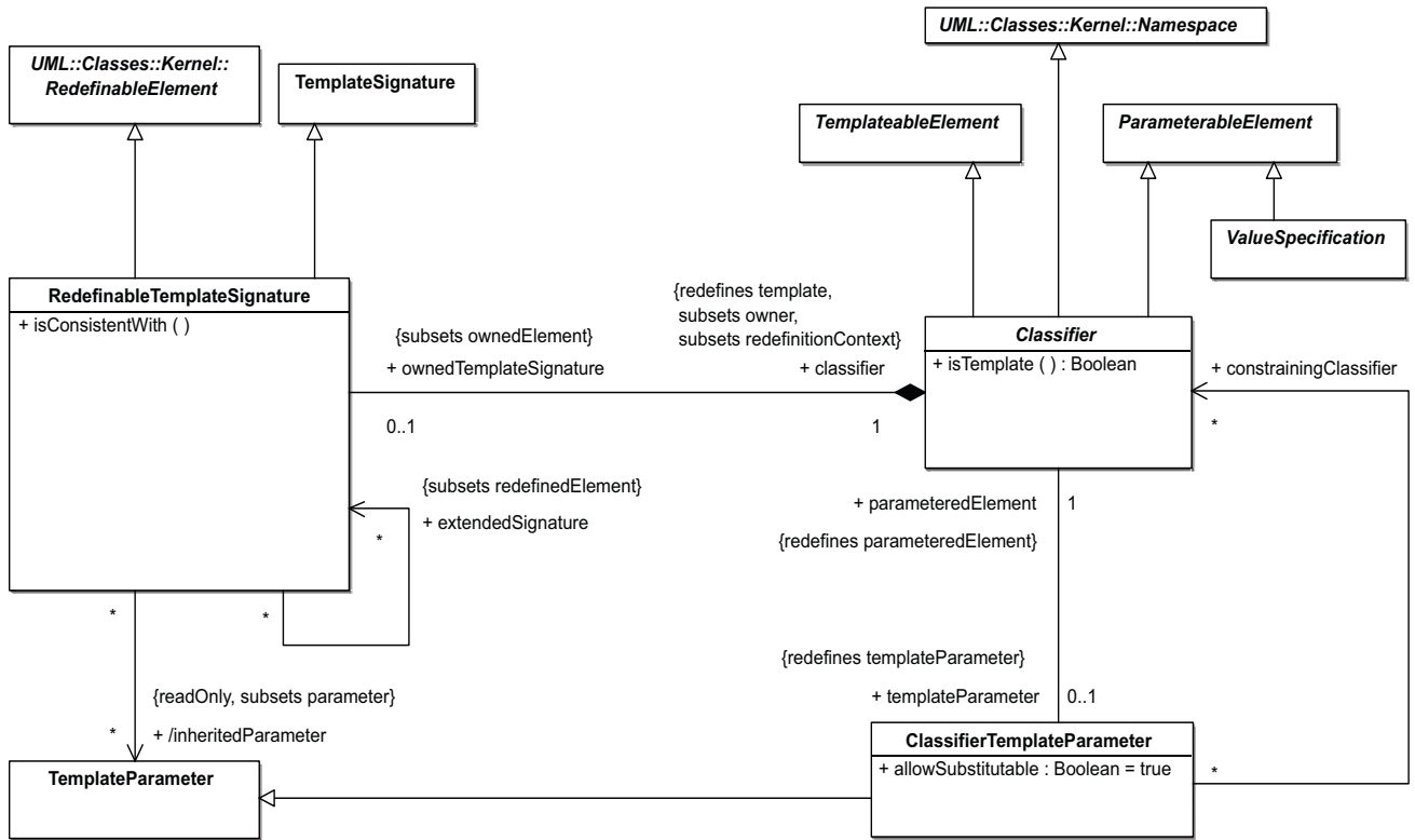
Figure 17.18 - Classifier templates
