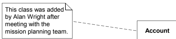
Figure 7.32 - Comment notation
