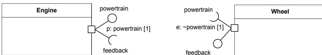
Figure 9.16 - Port notation
