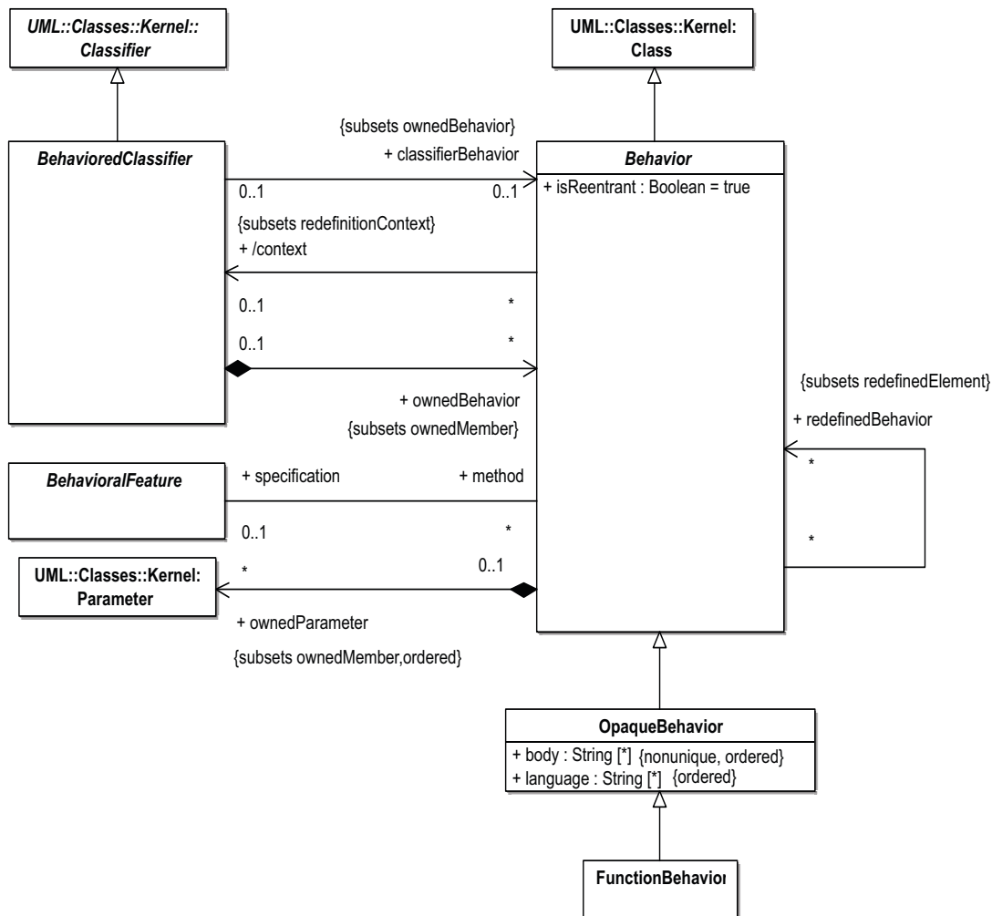
Figure 13.6 - Common Behavior
