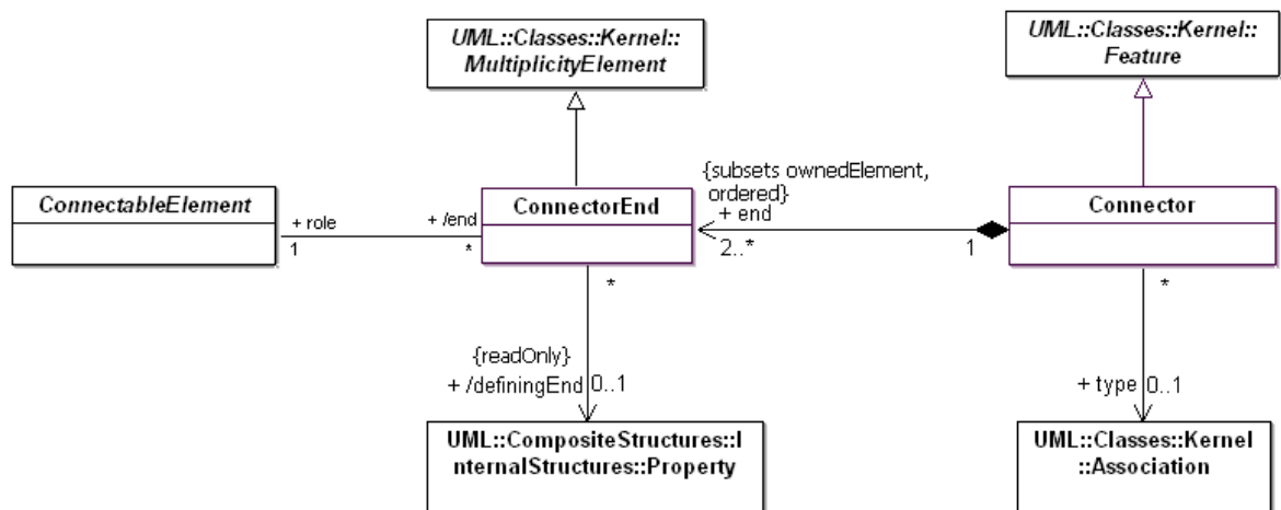
Figure 9.3 - Connectors
