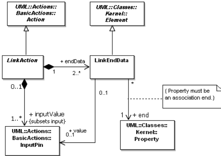
Figure 11.8 - Link identification
