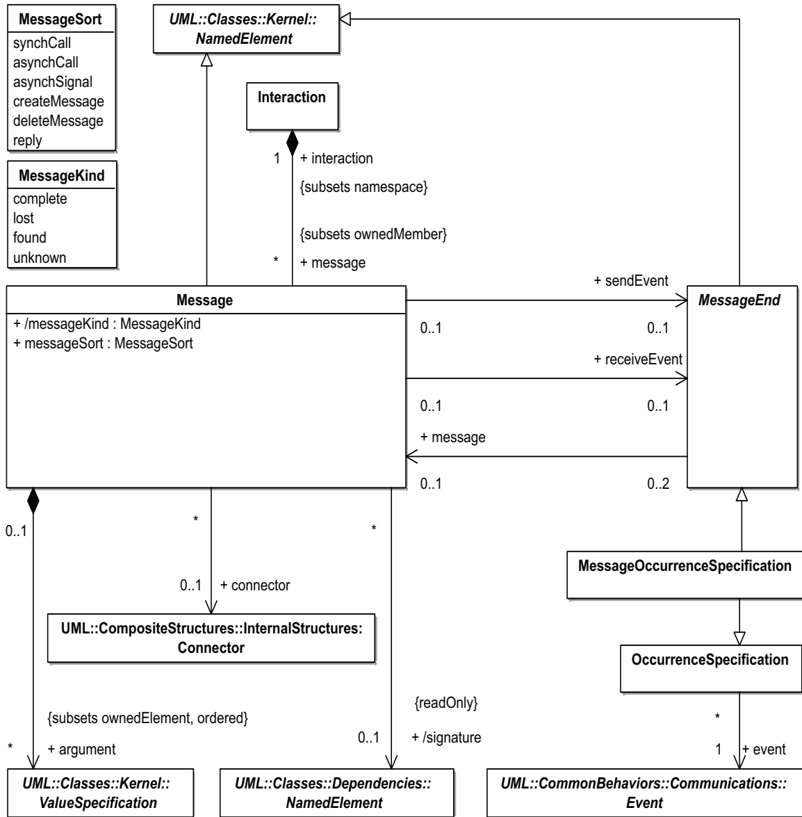
Figure 14.5 - Messages
