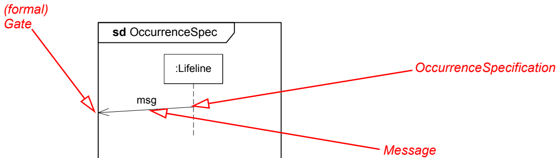
Figure 14.20 - OccurrenceSpecification
