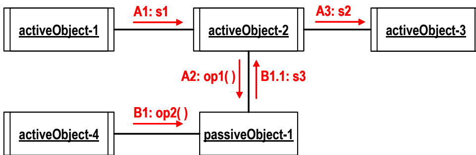
Figure 6.2 - Example illustrating the basic causality model of UML
