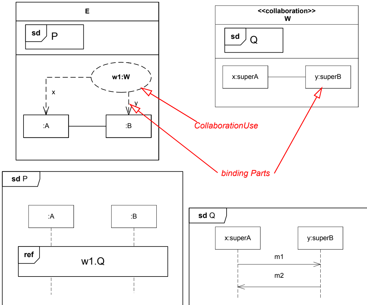
Figure 14.26 - Describing collaborations and their binding
