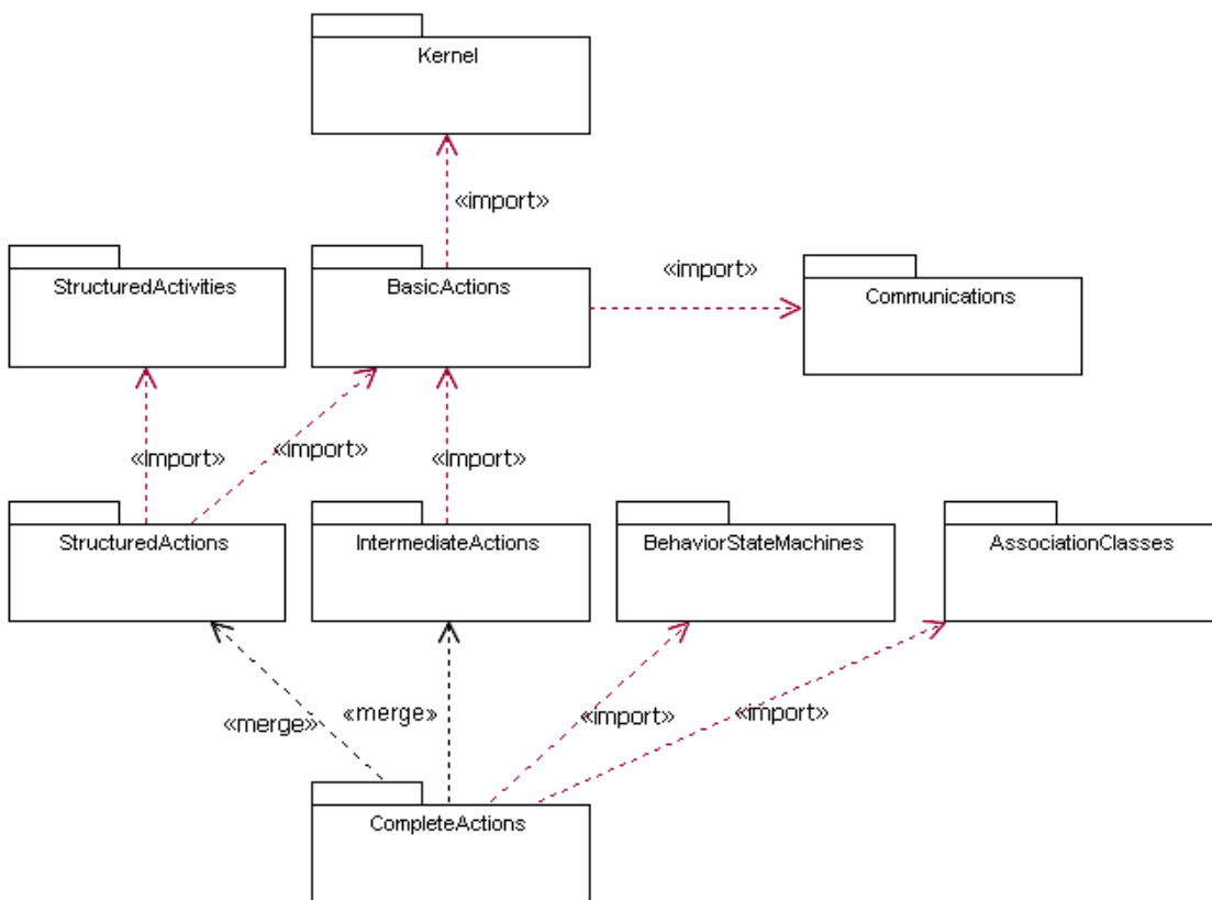
Figure 11.1 - Dependencies of the Action packages
