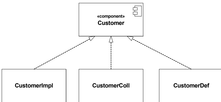
Figure 8.10 - A representation of the realization of a complex component
