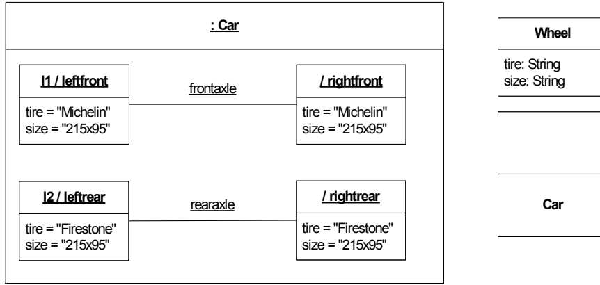
Figure 9.26 - An instance of the Car class
