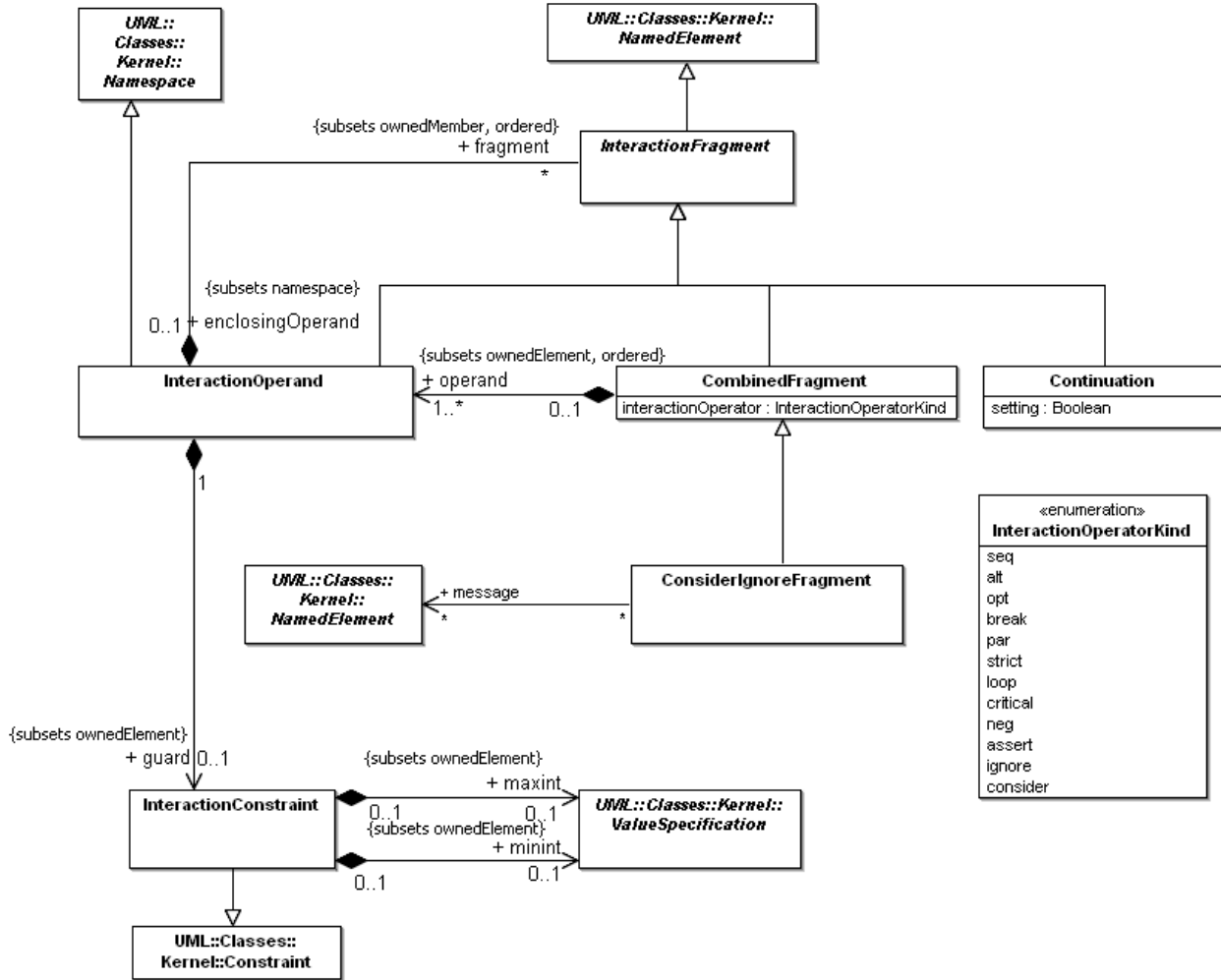
Figure 14.7 - CombinedFragments
