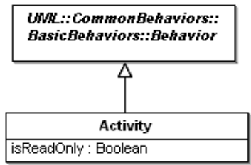
Figure 12.7 - Elements
