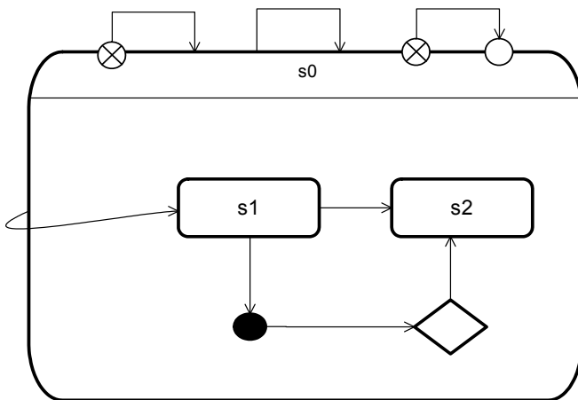
Figure 15.48 - External Transitions
