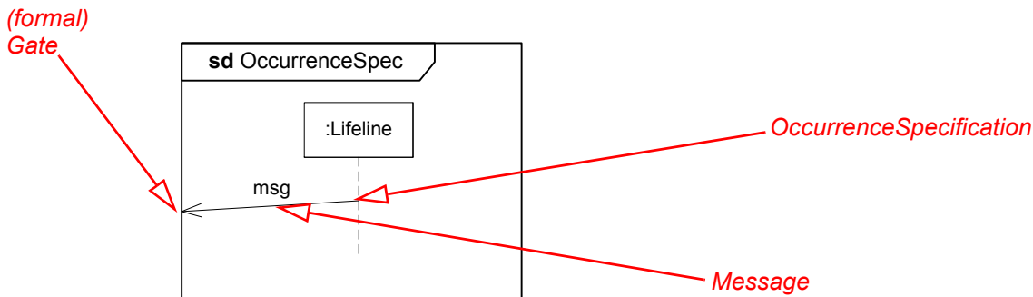
Figure 14.20 - OccurrenceSpecification
