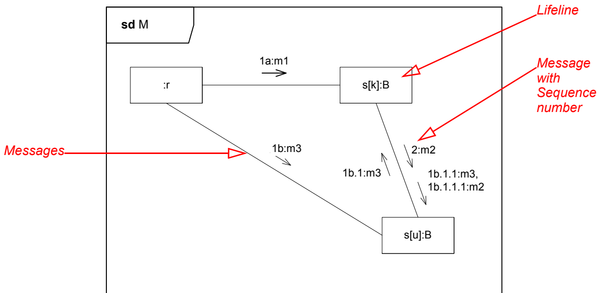
Figure 14.28 - Communication diagram
