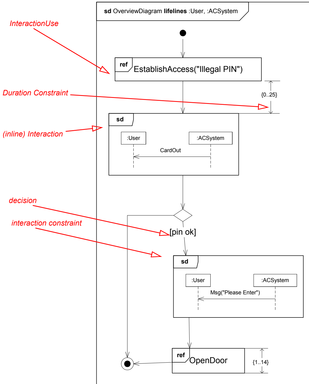
Figure 14.29 - Interaction Overview Diagram representing a High Level Interaction diagram
