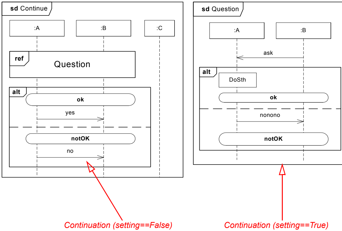
Figure 14.13 - Continuation
