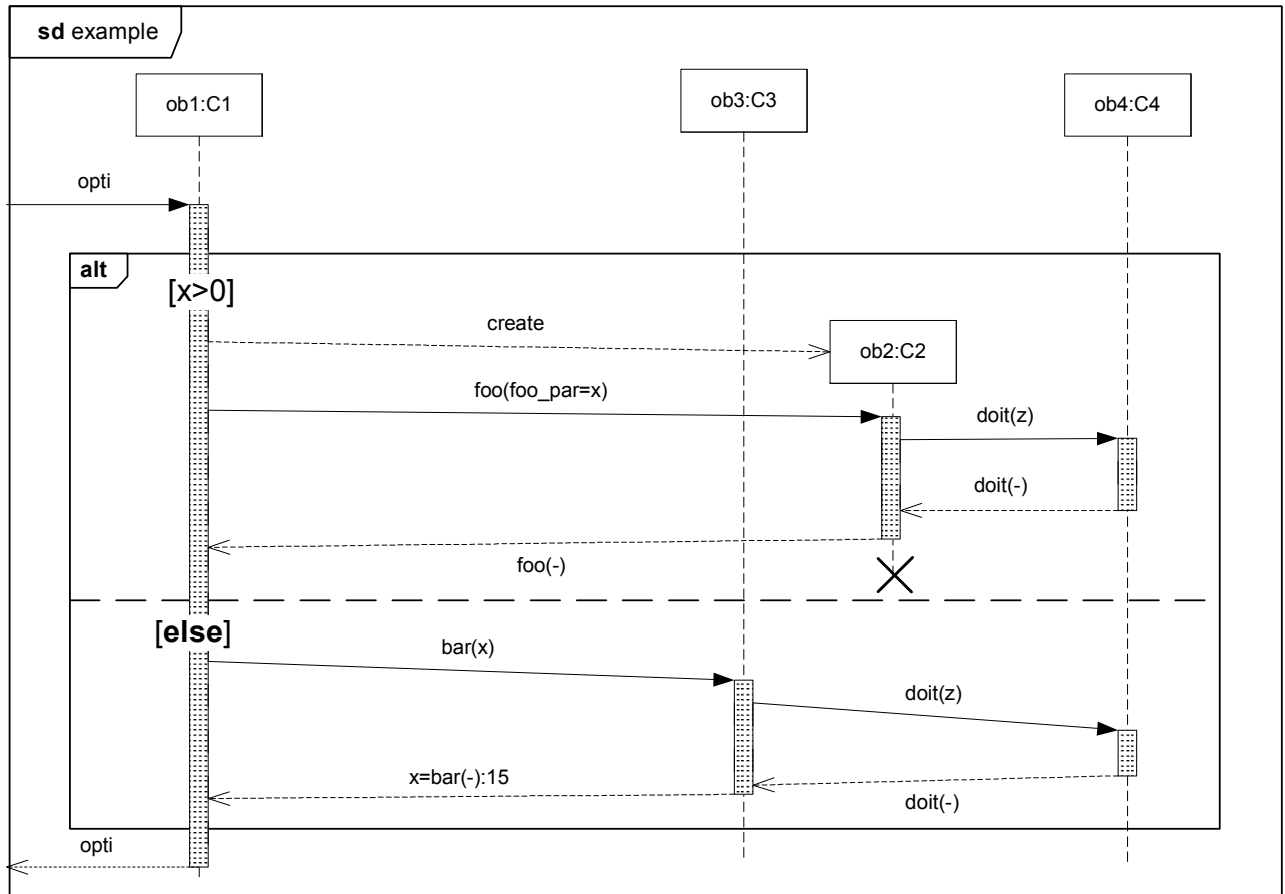
Figure 14.12 - CombinedFragment
