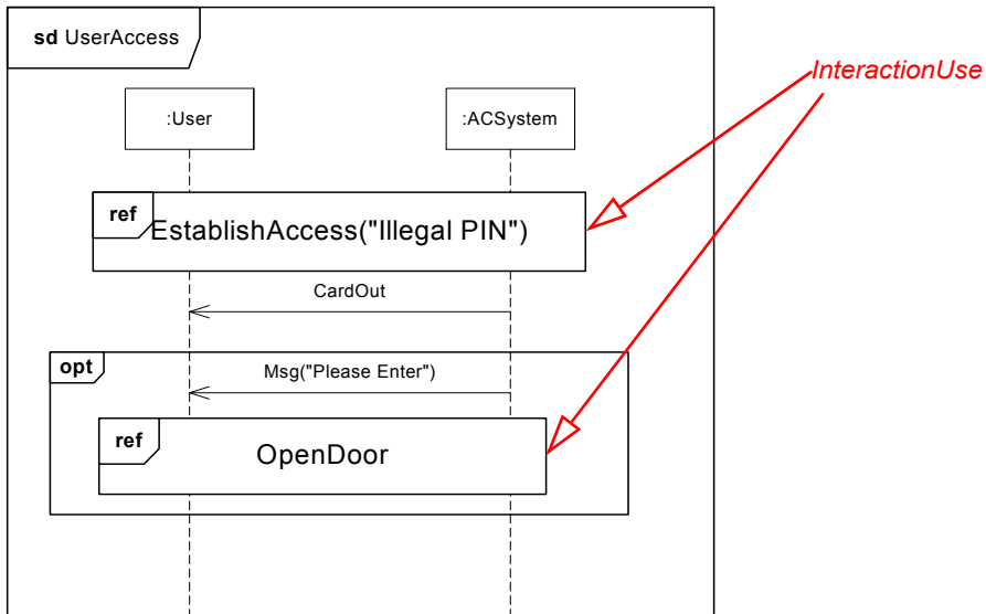
Figure 14.18 - InteractionUse
