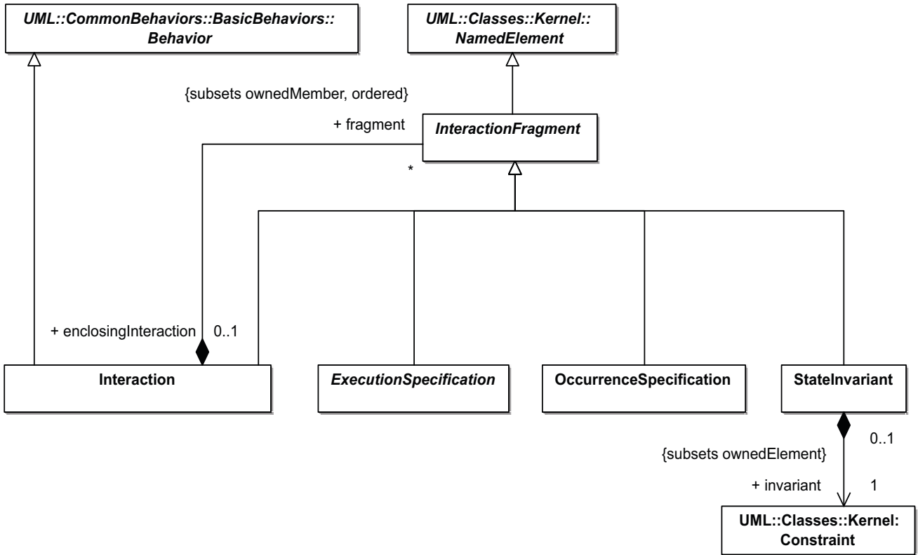
Figure 14.3 - Interactions
