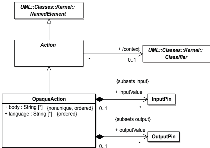
Figure 11.2 - Basic actions
