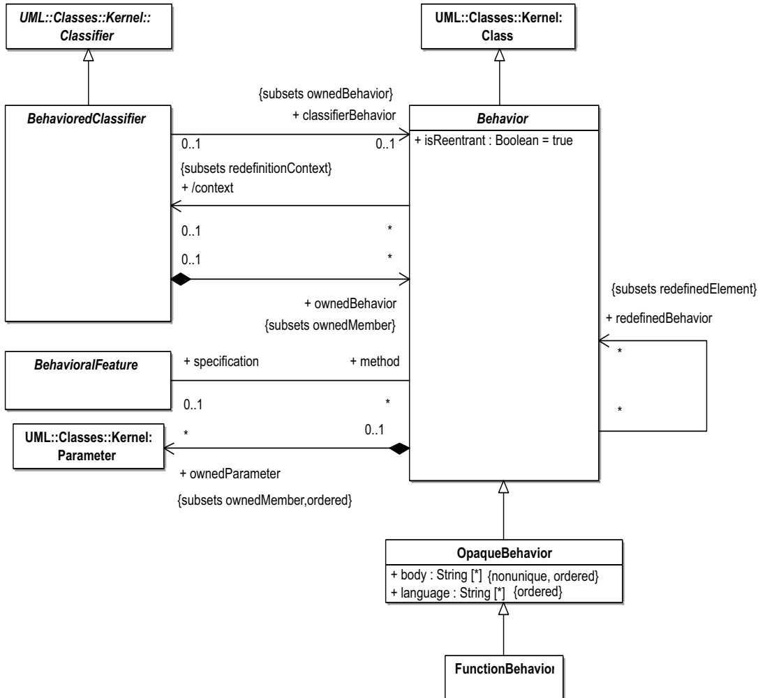
Figure 13.6 - Common Behavior
