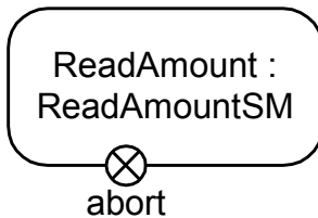
Figure 15.8 - Exit Point
