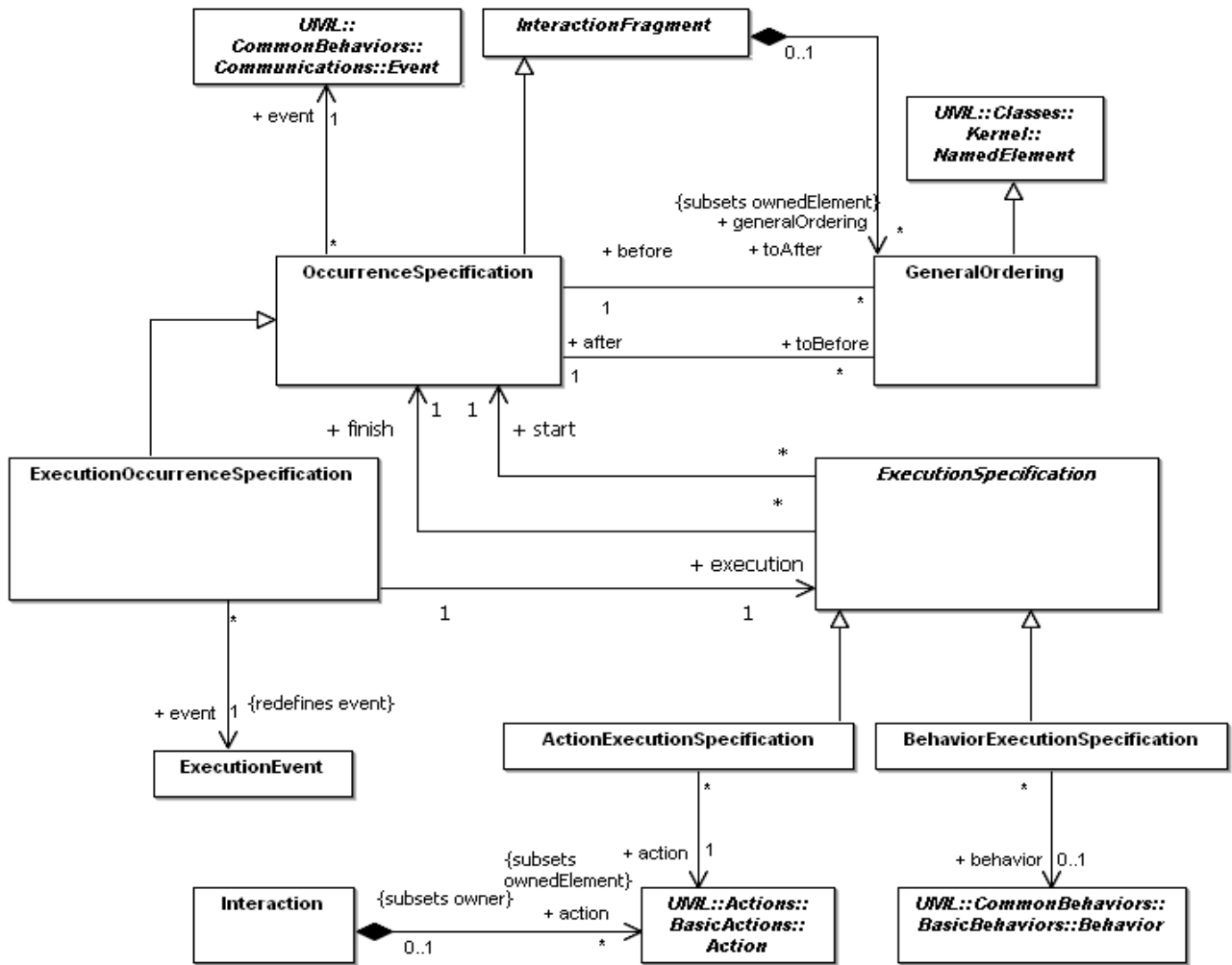
Figure 14.6 - Occurrences
