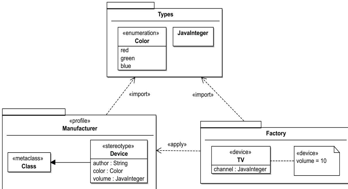
Figure 18.11 - Importing a package from a profile
