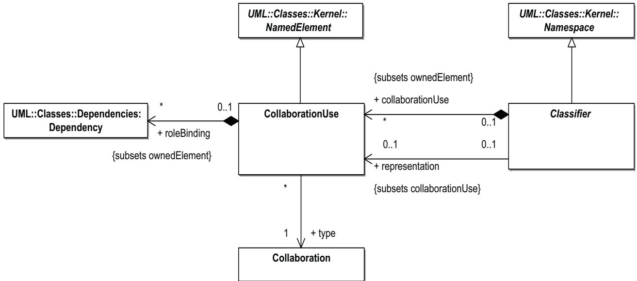
Figure 9.7 - Collaboration.use and role binding
