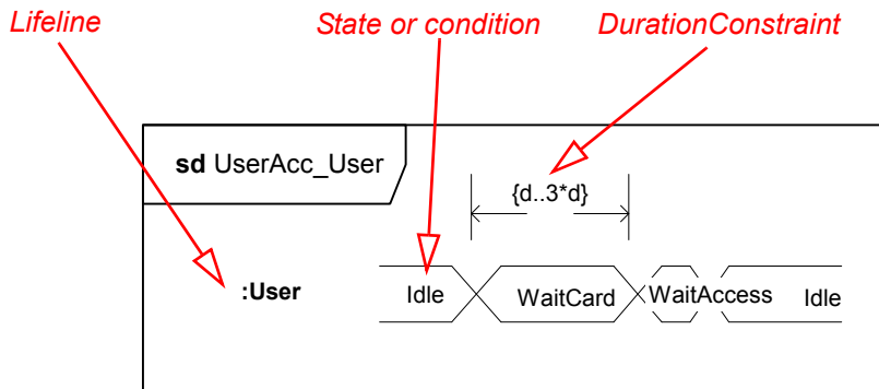
Figure 14.31 - Compact Lifeline with States
