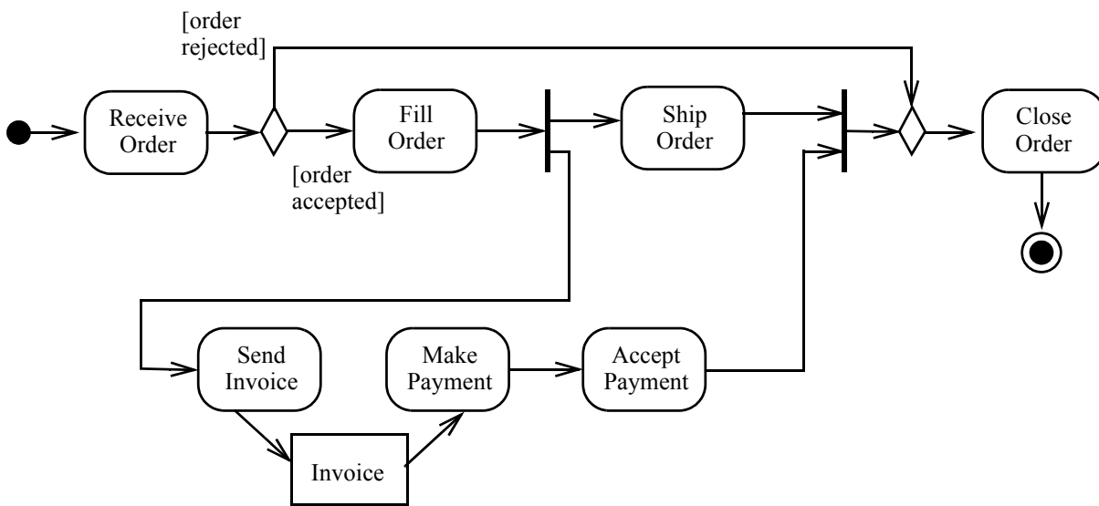
Figure 12.51 - Activity node example (where the arrowed lines are only the non-activity node symbols)
