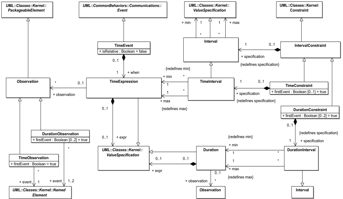
SimpleTime Figure 13.13 - SimpleTime
