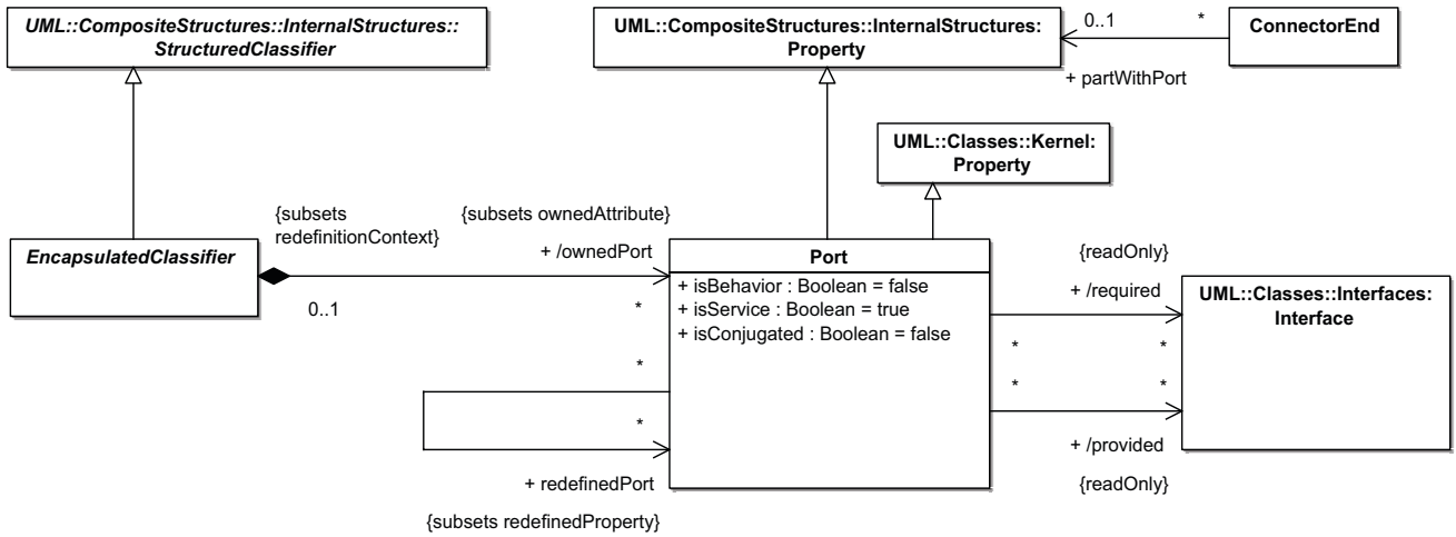
Figure 9.4 - The Port metaclass
