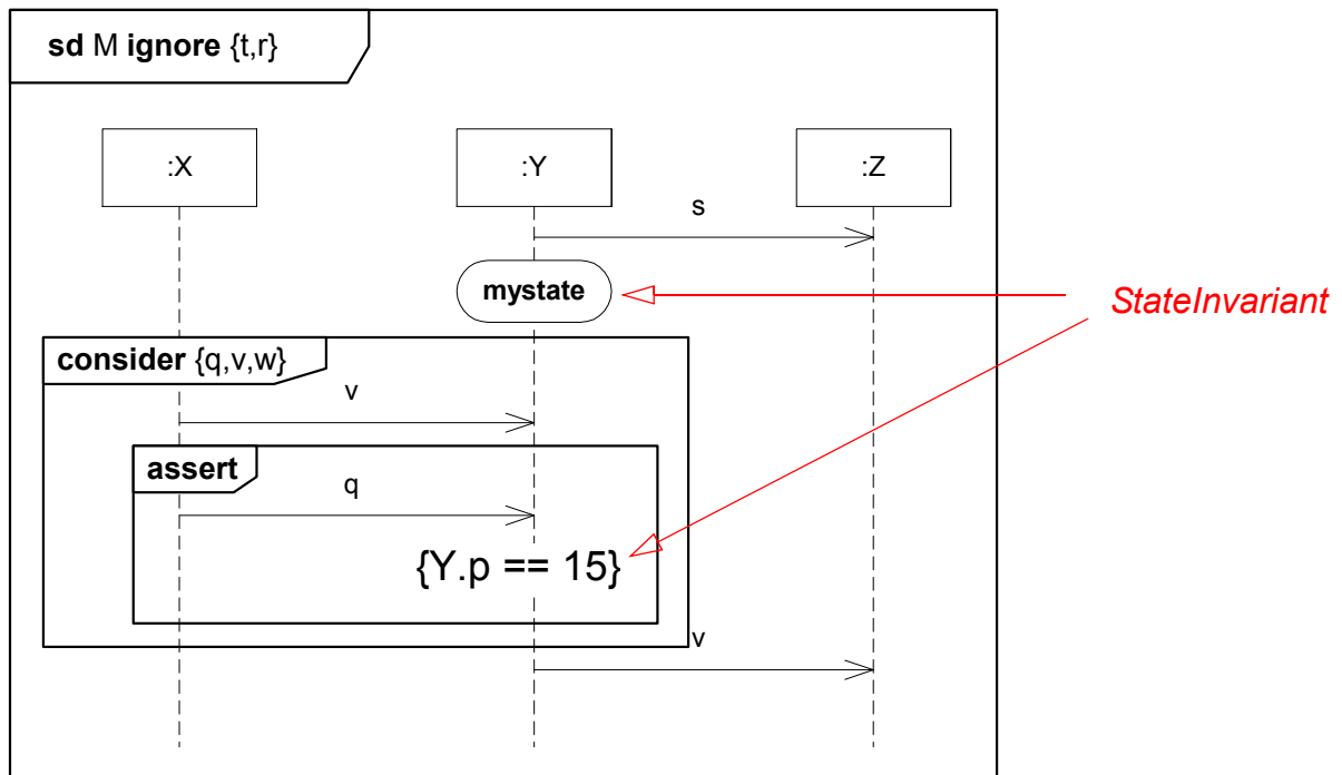
Figure 14.25 - Ignore, Consider, assert with State Invariants
