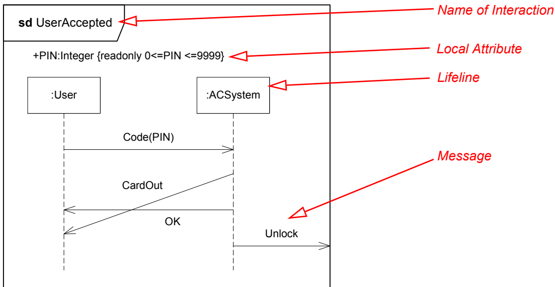
Figure 14.17 - An example of an Interaction in the form of a Sequence Diagram
