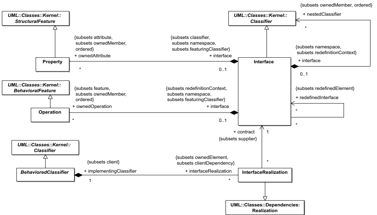
Figure 7.16 - Contents of Interfaces package
