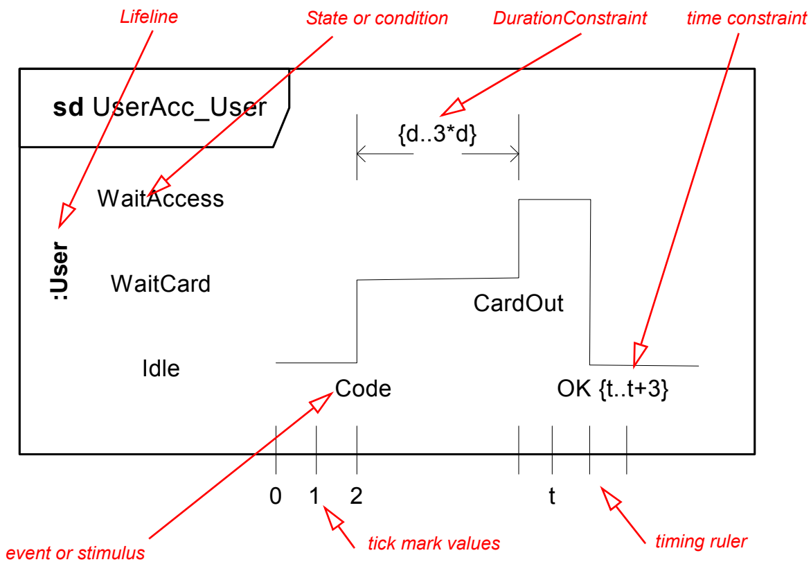
Figure 14.30 - A Lifeline for a discrete object
