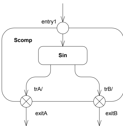
Figure 15.21 - Entry and exit points on composite states
