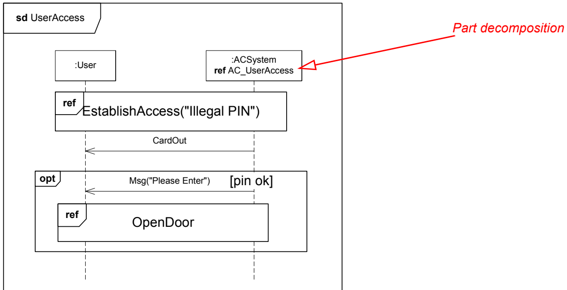
Figure 14.21 - Part Decomposition - the decomposed part
