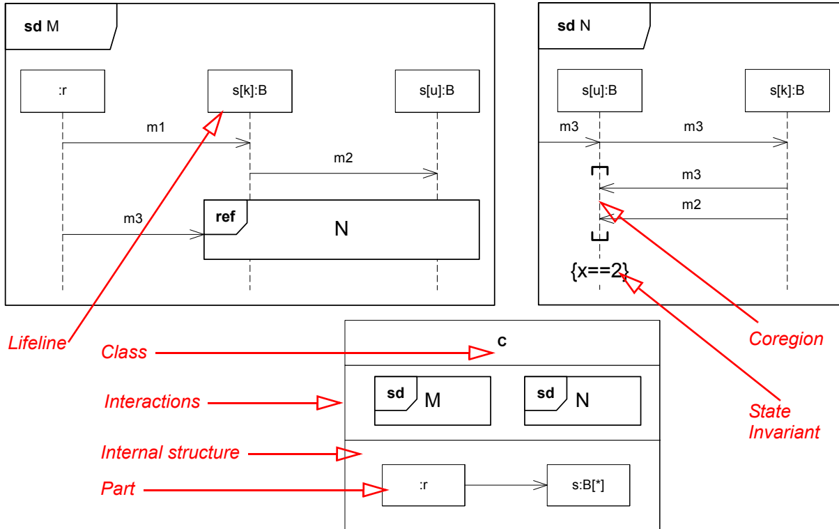
Figure 14.23 - Sequence Diagrams where two Lifelines refer to the same set of Parts (and Internal Structure)
