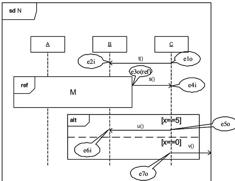
Figure E.6 - Sequence diagram enhanced with identification of the Event occurrences
