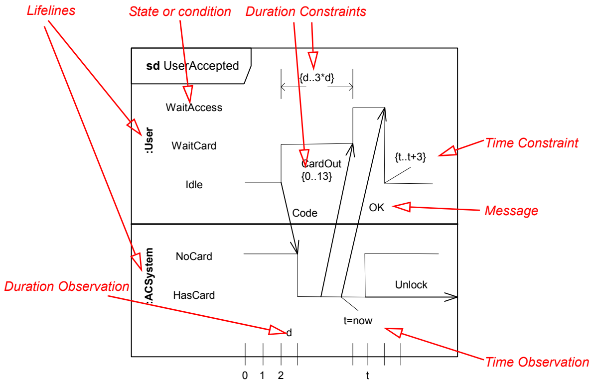
Figure 14.32 - Timing Diagram with more than one Lifeline and with Messages
