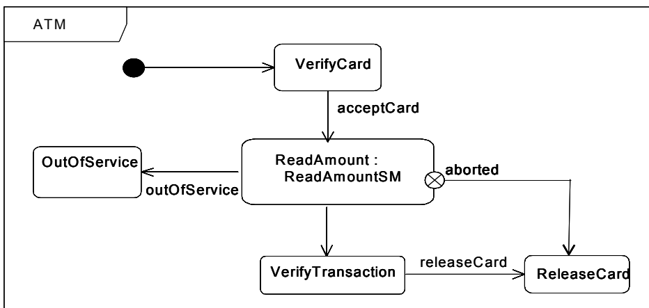
Figure 15.50 - SubmachineState with usage of exit point
