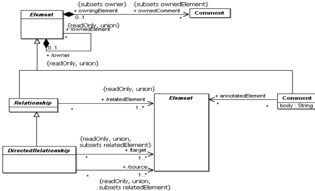
Figure 7.3 - Root diagram of the Kernel package
