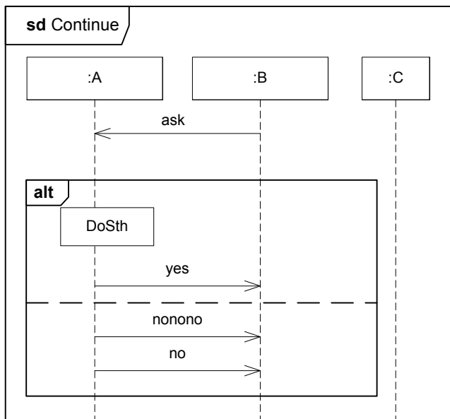
Figure 14.14 - Continuation interpretation
