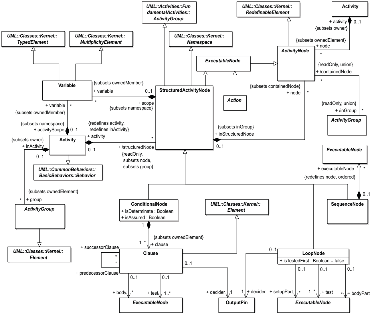
Figure 12.21 - Structured nodes
