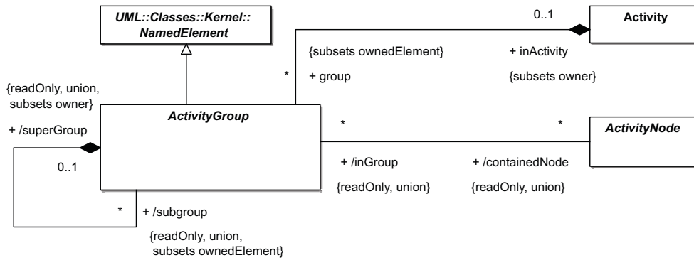
Figure 12.3 - Fundamental groups
