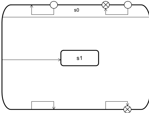
Figure 15.47 - Local Transitions
