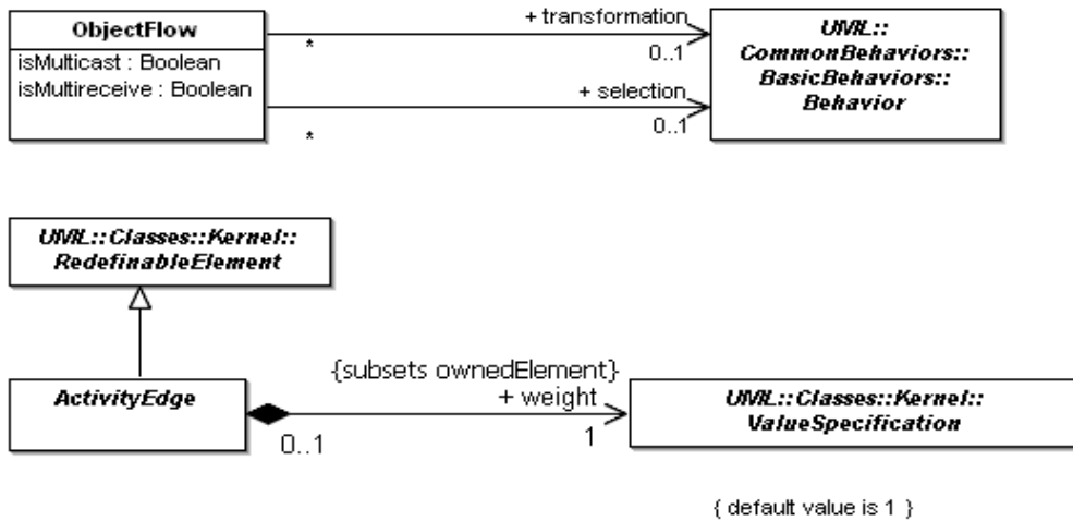
Figure 12.14 - Flows (CompleteActivities)
