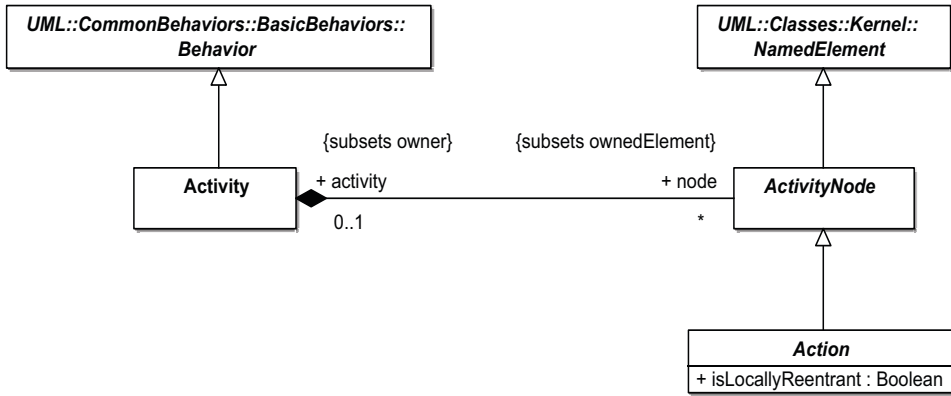
Figure 12.2 - Fundamental nodes
