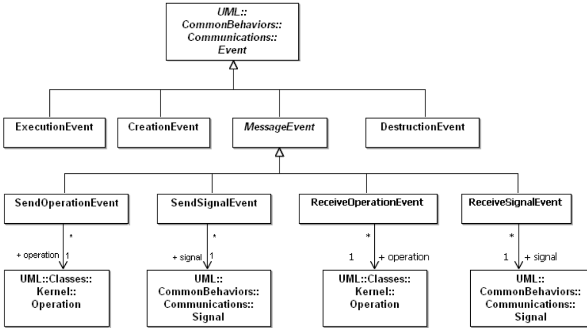
Figure 14.2 Events
