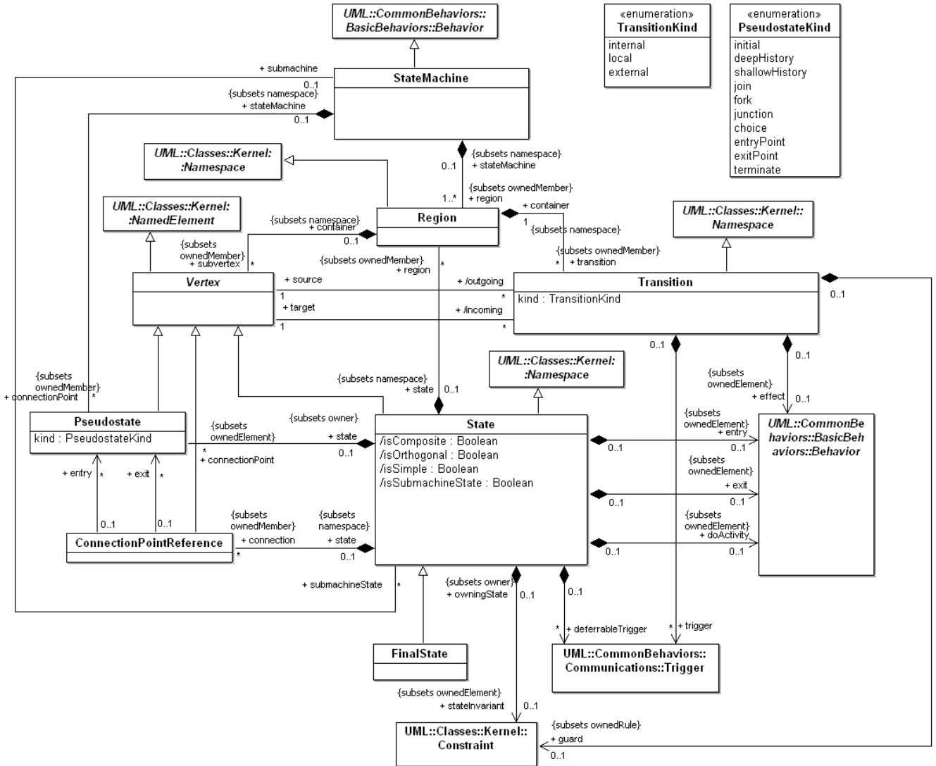
Figure 15.2 - State Machines
