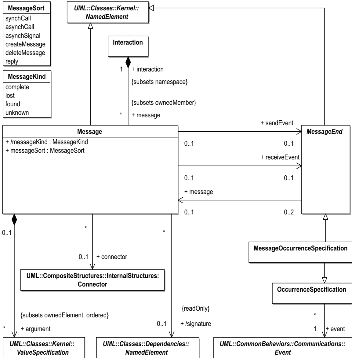
Figure 14.5 - Messages
