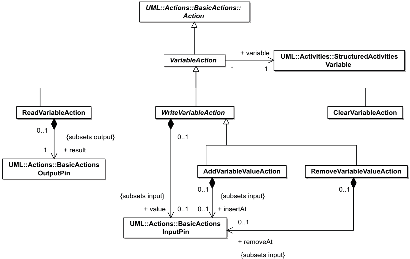
Figure 11.18 - Variable actions
