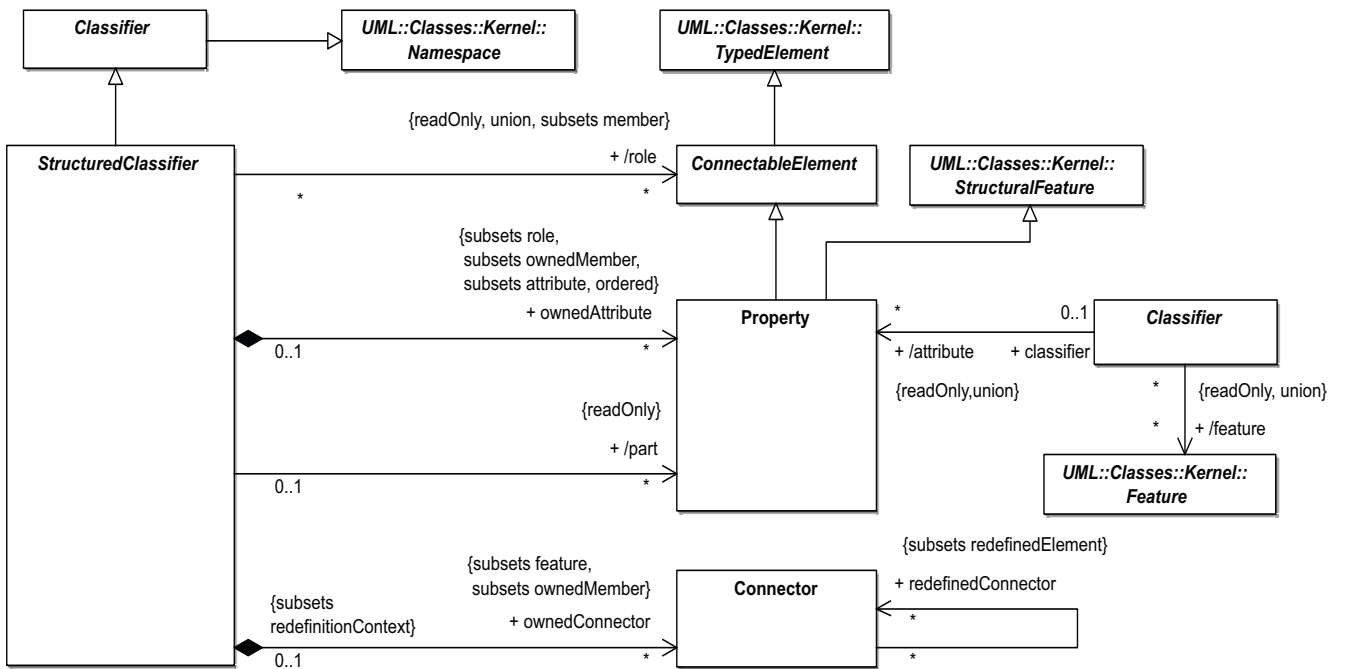
Figure 9.2 - Structured classifier
