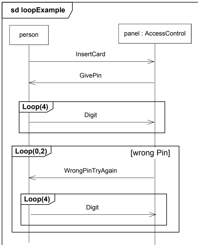
Figure 14.11 - Loop CombinedFragment
