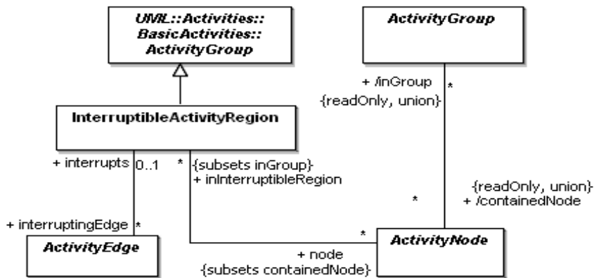
Figure 12.20 - Interruptible regions
