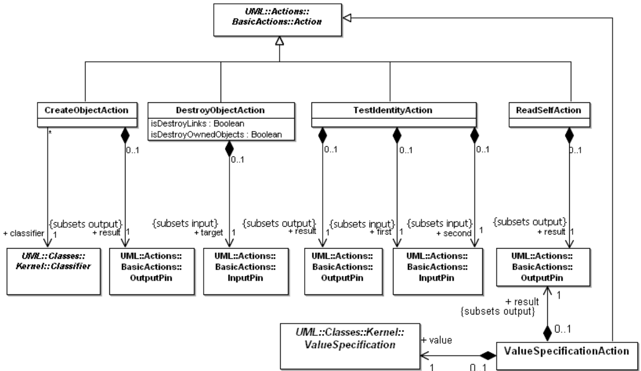
Figure 11.6 - Object actions
