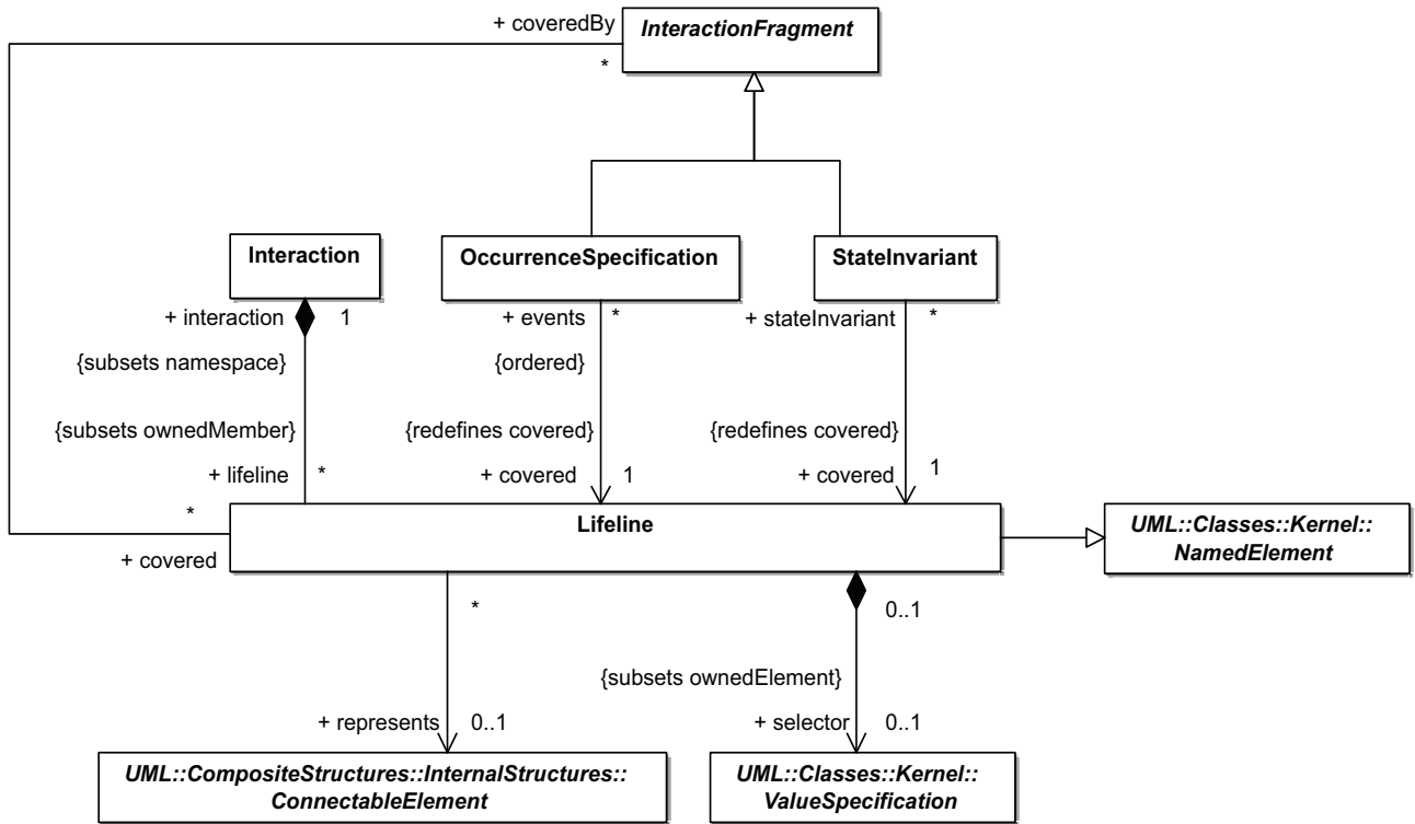
Figure 14.4 - Lifelines
