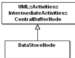
Figure 12.17 - Data stores
