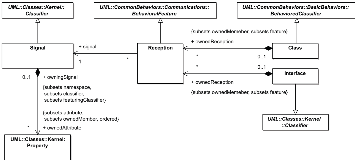
Figure 13.9 - Reception
