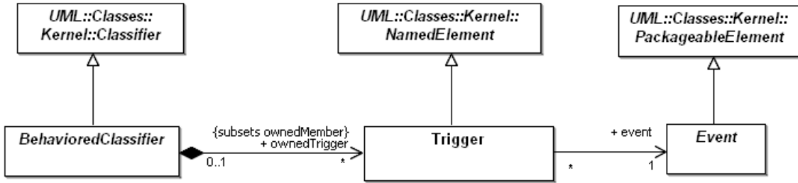
Figure 13.11 - Triggers
