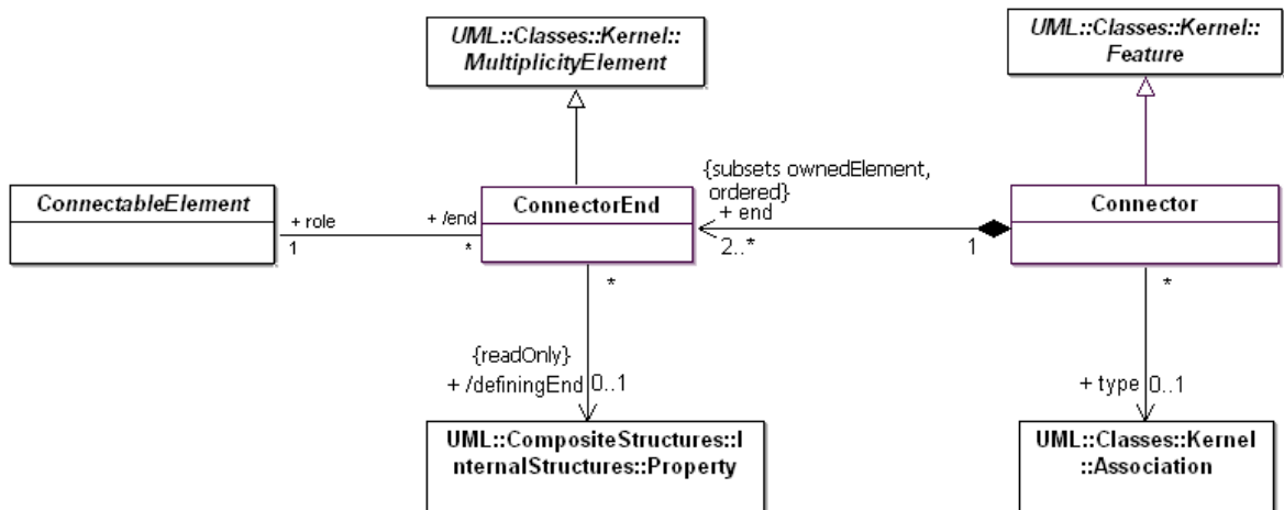
Figure 9.3 - Connectors
