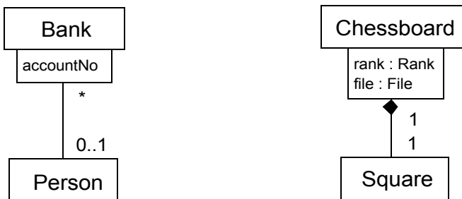
Figure 7.72 - Qualified associations
