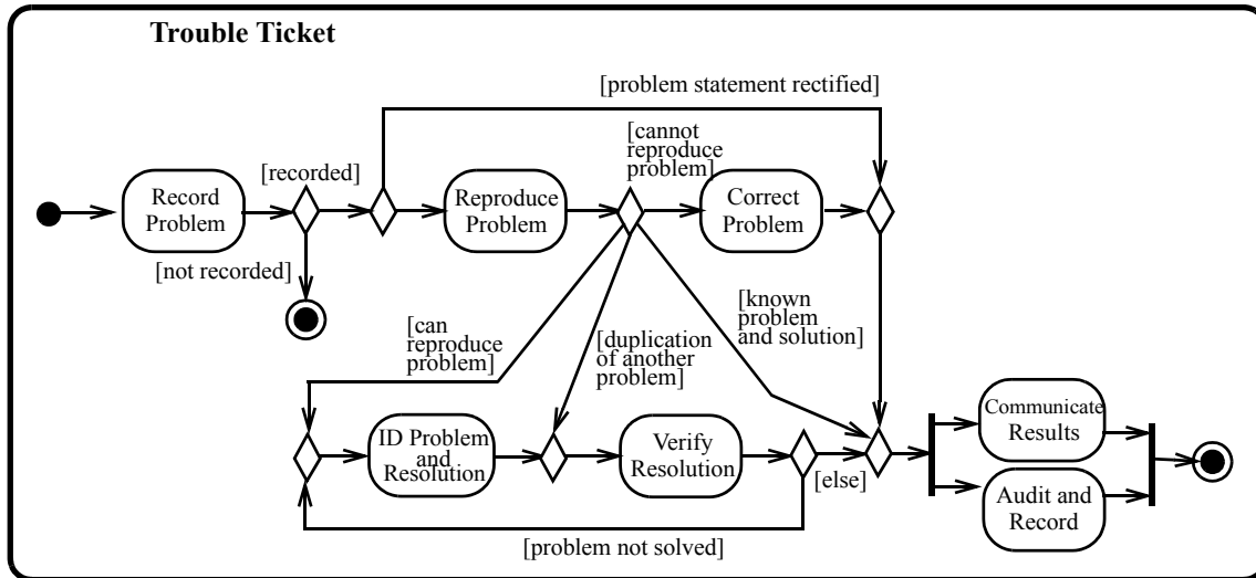
Figure 12.37 - Workflow example
