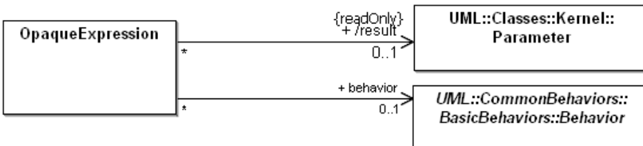
Figure 13.7 - Expression
