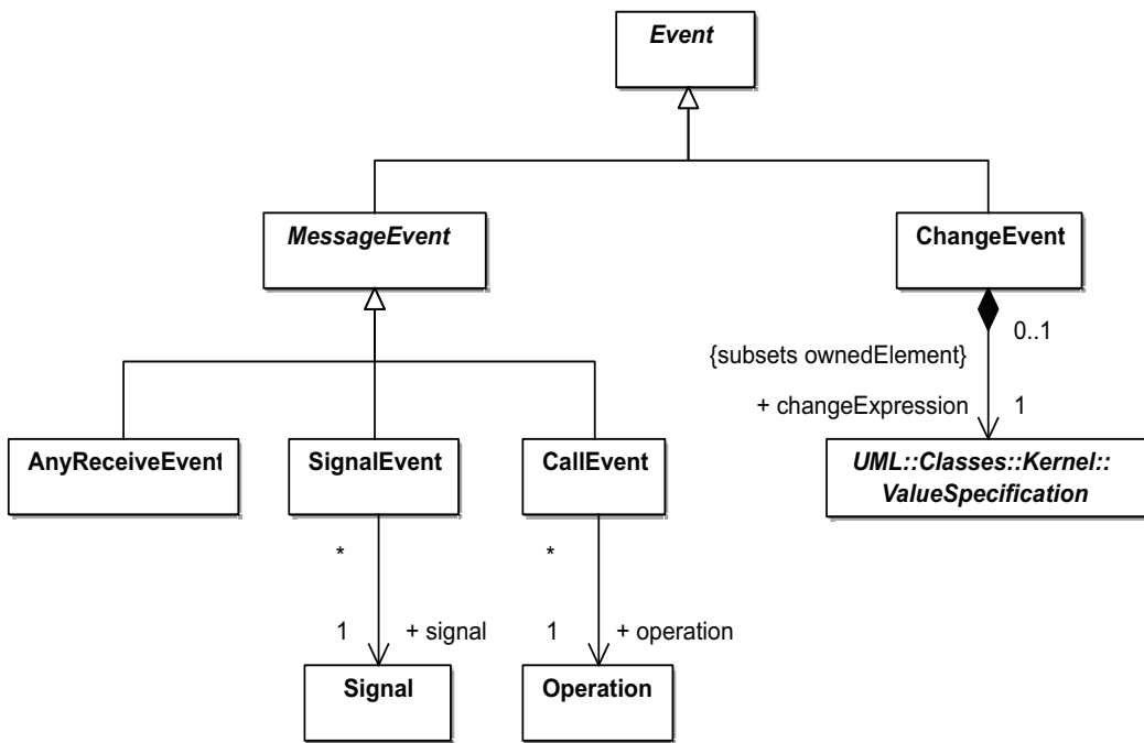
Figure 13.12 - Events
