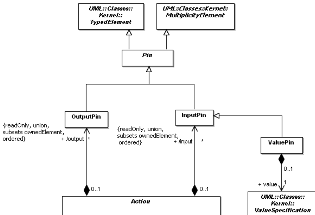
Figure 11.3 - Basic pins
