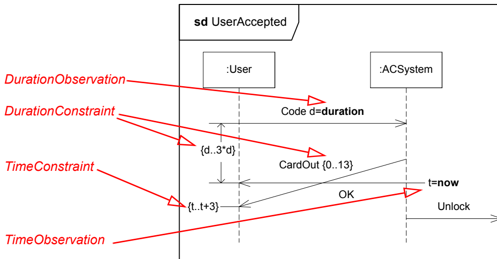
Figure 14.27 - Sequence Diagram with time and timing concepts
