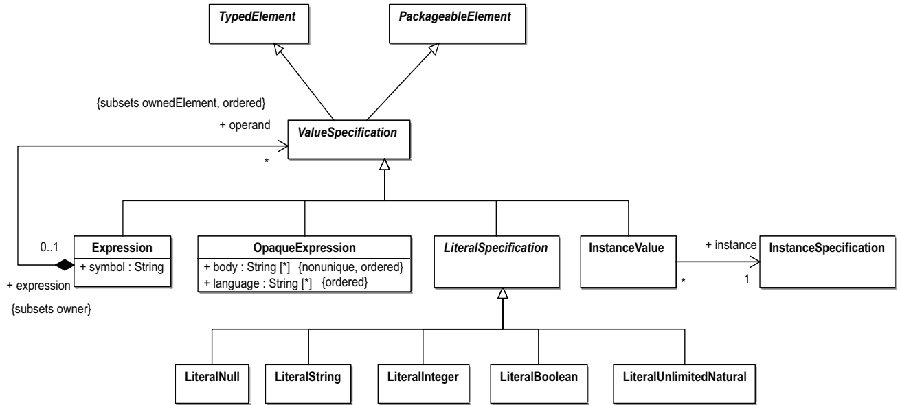
Figure 7.6 - Expressions diagram of the Kernel package
