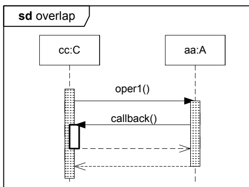
Figure 14.16 - Overlapping execution occurrences
