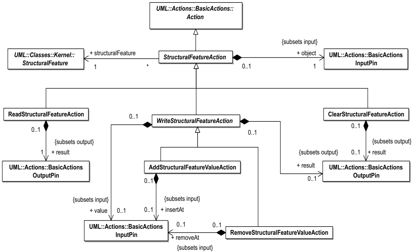
Figure 11.7 - Structural Feature Actions
