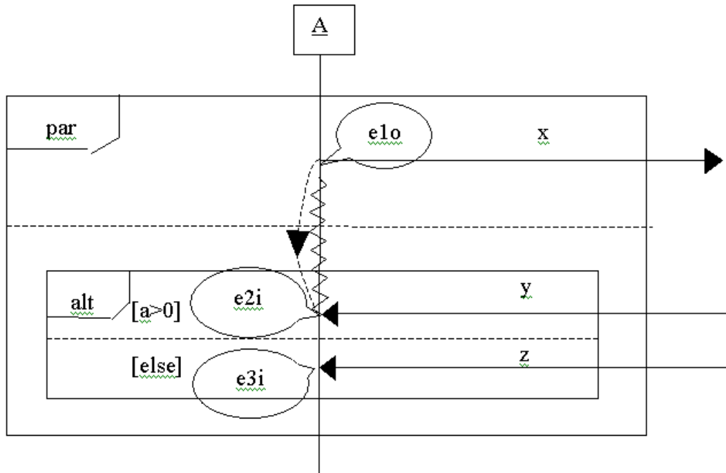
Figure E.7 - Sequence diagram with guards, parallel composition and alternatives
