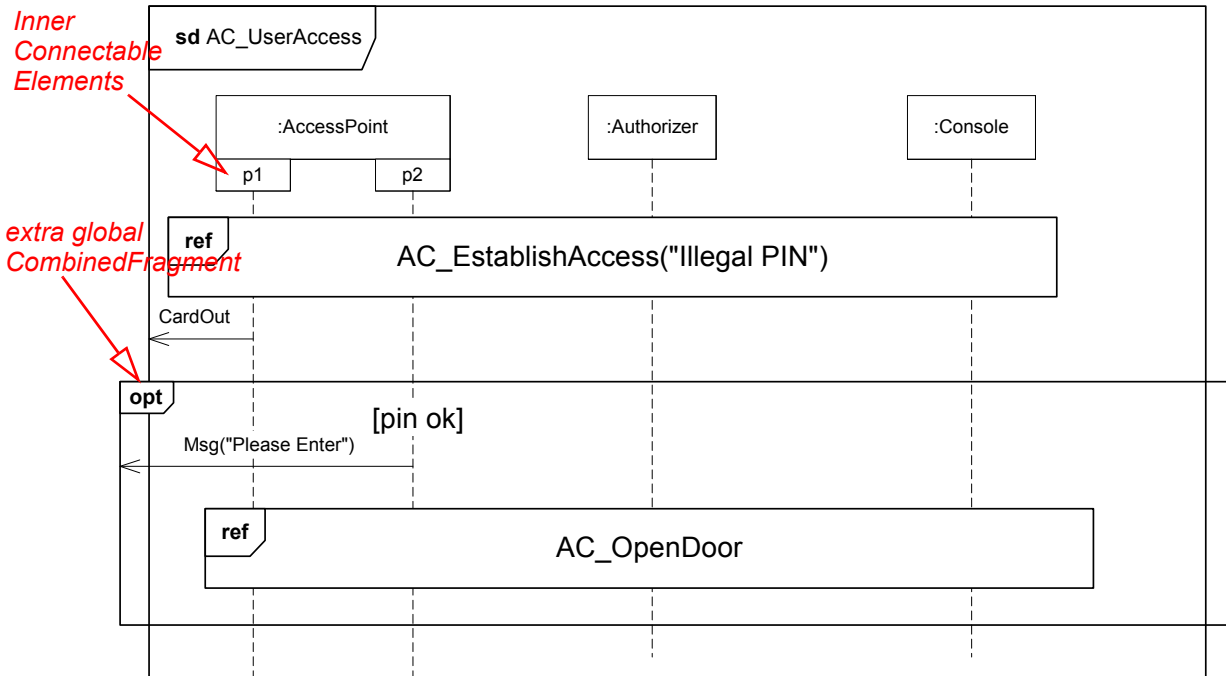
Figure 14.22 - PartDecomposition - the decomposition
