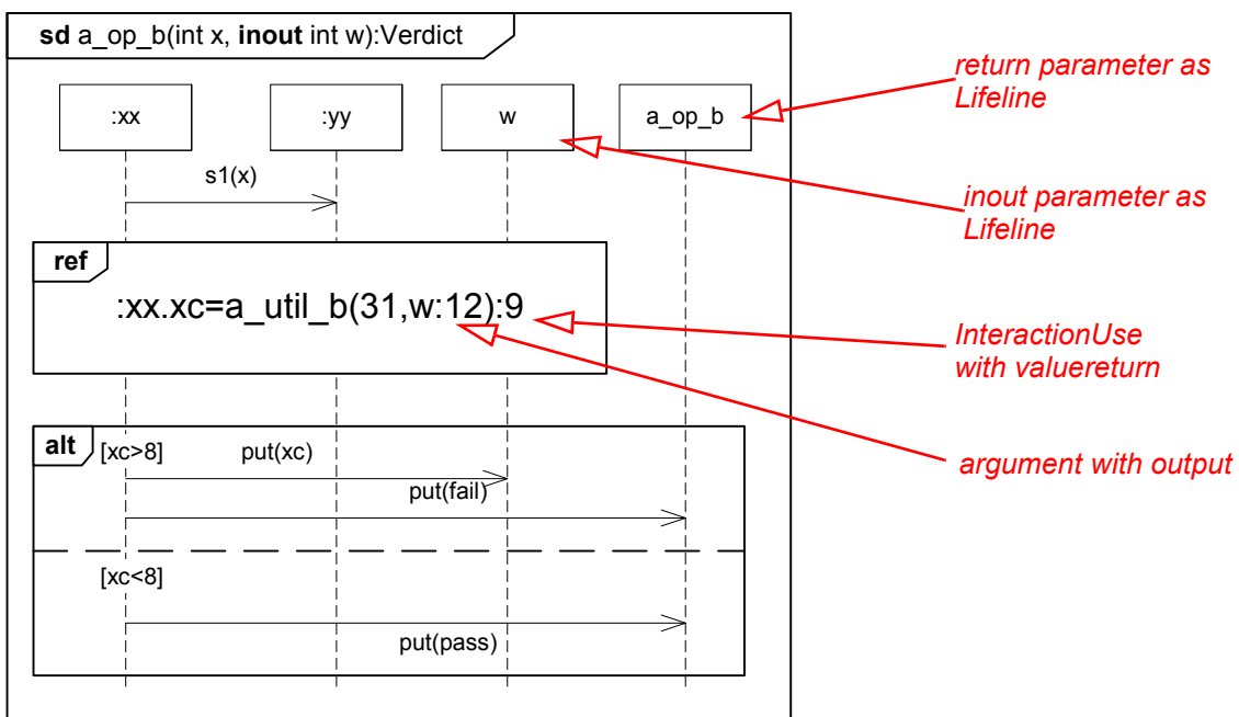
Figure 14.19 - InteractionUse with value return
