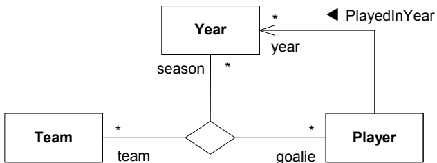
Figure 7.21 - Binary and ternary associations
