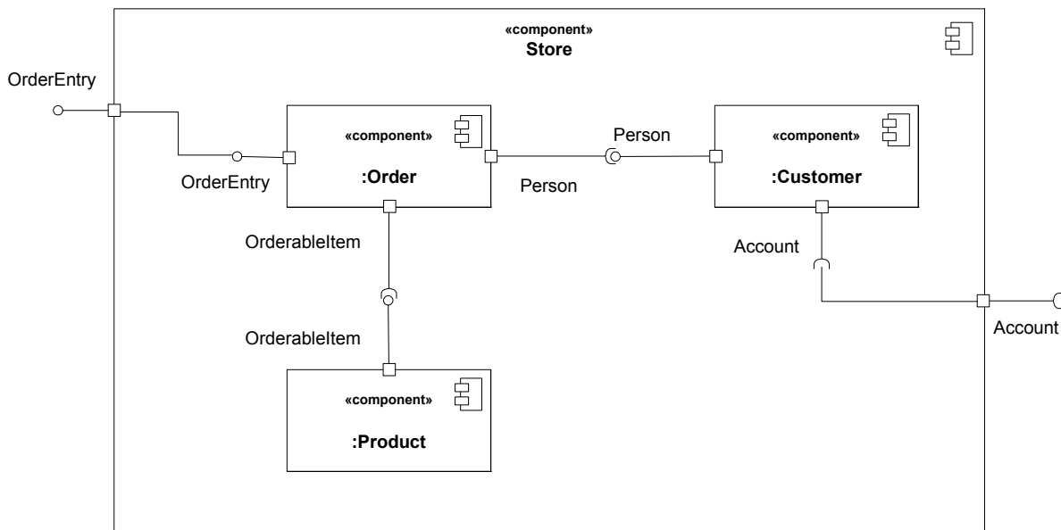
Figure 8.12 - An internal or white-box view of the internal structure of a component that contains other components
