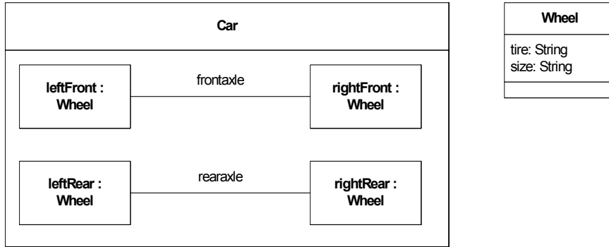
Figure 9.24 - Connectors and parts in a structure diagram
