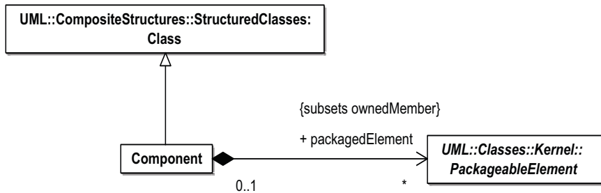
Figure 8.4 - The packaging capabilities of Components
