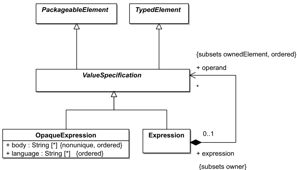
Figure 11.4 - The Expressions diagram of the Constructs package
