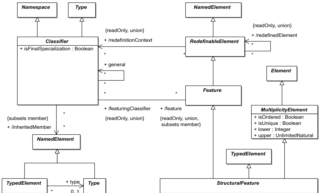
Figure 11.16 - The Classifiers diagram of the Constructs package
