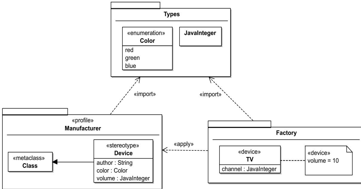
Figure 13.11 - Importing a package from a profile
