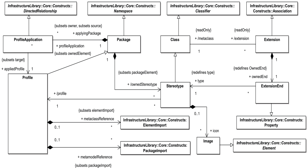
Figure 13.2 - The classes defined in the Profiles package
