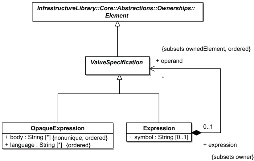
Figure 9.20 - The elements defined in the Expressions package
