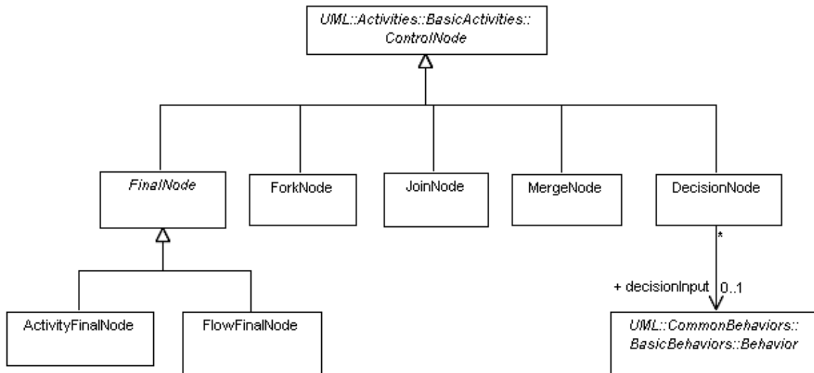
Figure 12.9 - Control nodes ( IntermediateActivities )
