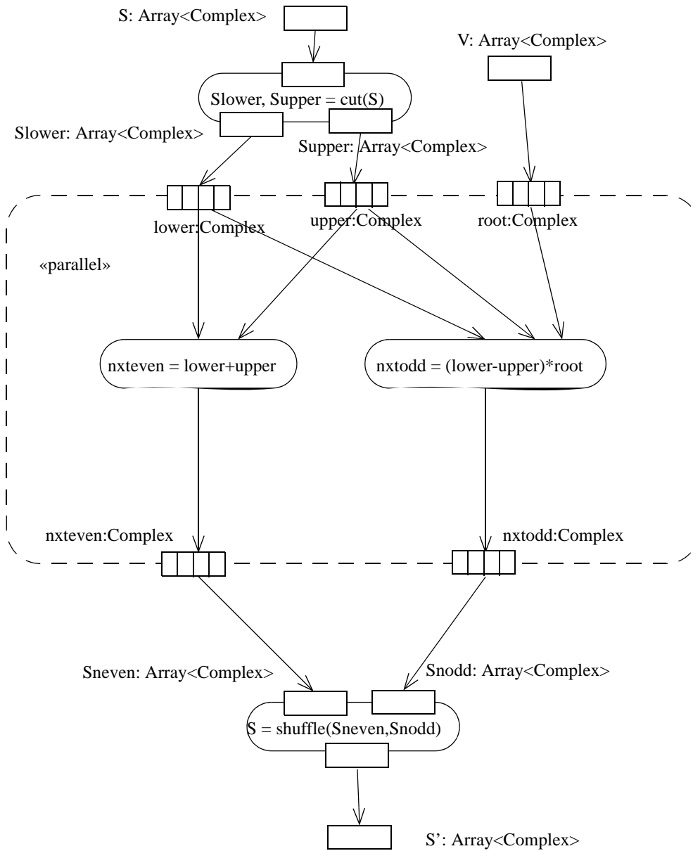
Figure 12.87 - Expansion region
