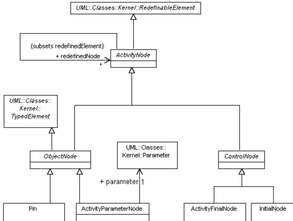
Figure 12.4 - Nodes (BasicActivities)
