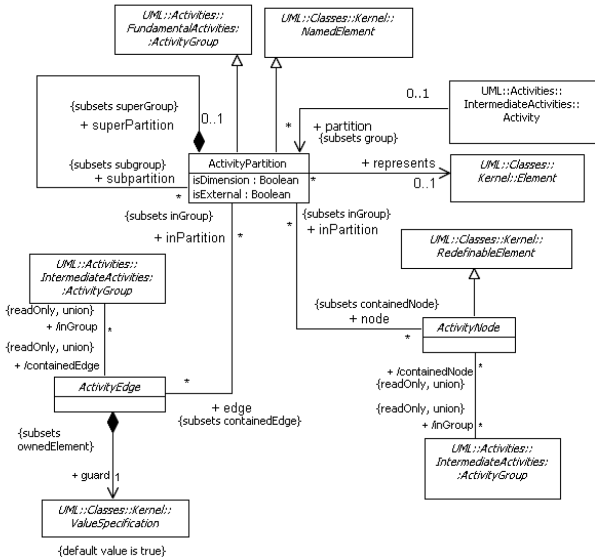
Figure 12.10 - Partitions
