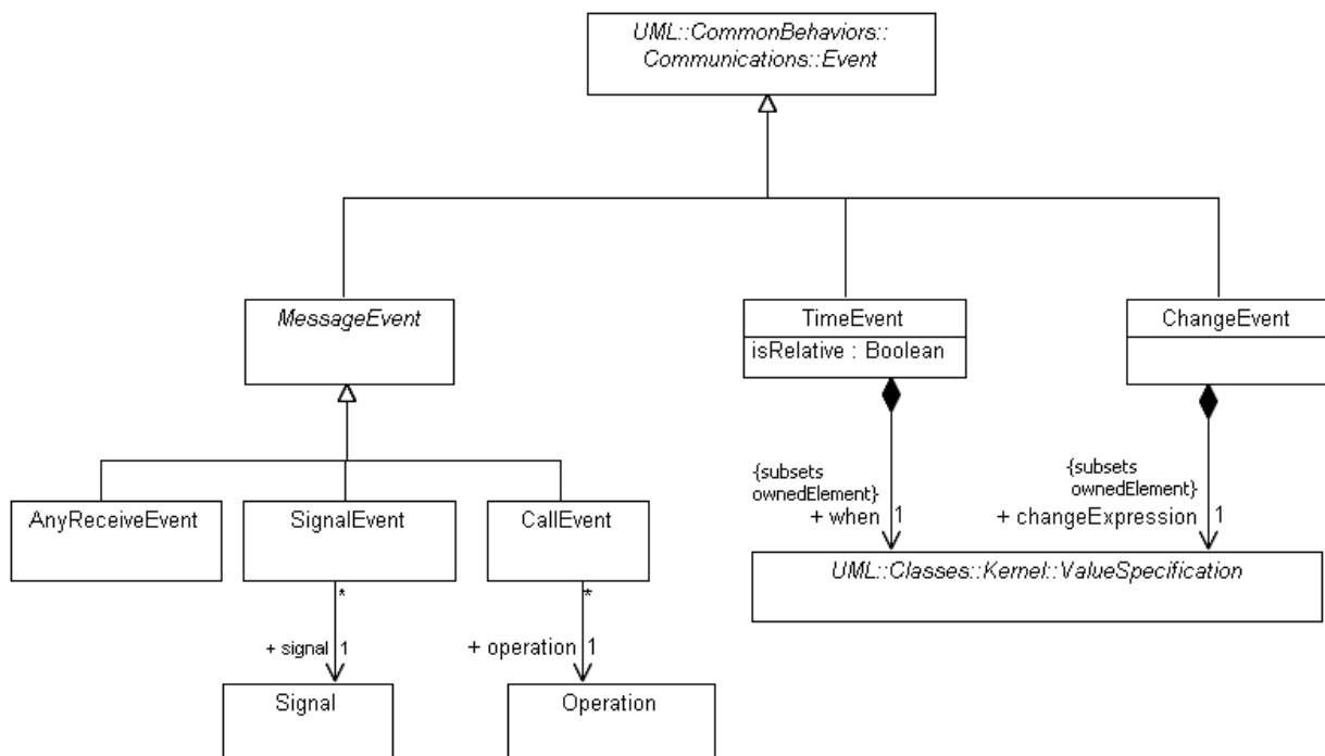
Figure 13.12 - Events
