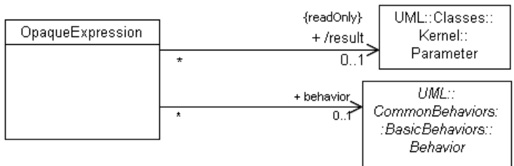
Figure 13.7 - Expression
