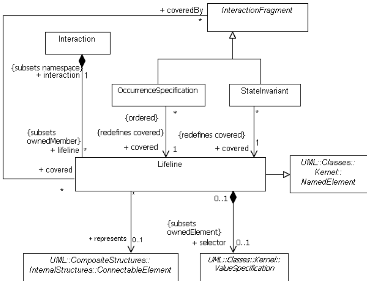
Figure 14.4 - Lifelines
