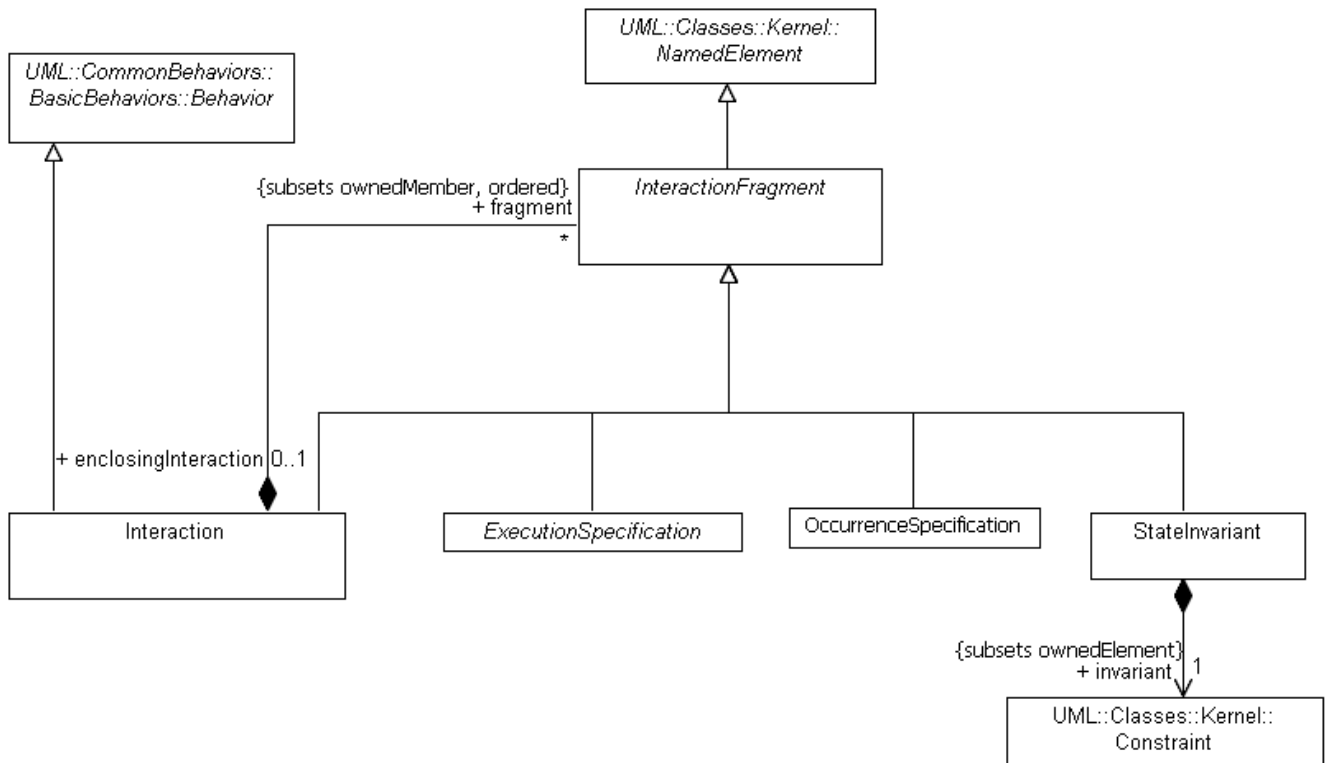
Figure 14.3 - Interactions
