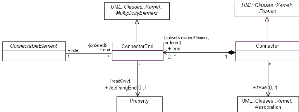
Figure 9.3 - Connectors
