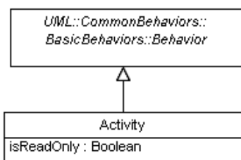
Figure 12.7 - Elements
