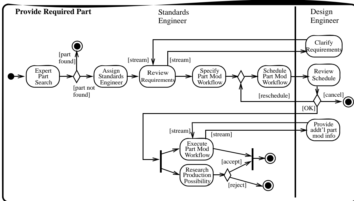
Figure 12.36 - Workflow example
