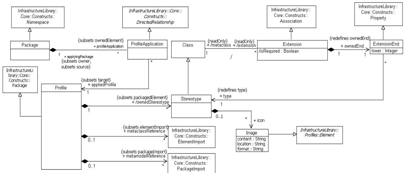
Figure 18.2 - The elements defined in the Profiles package
