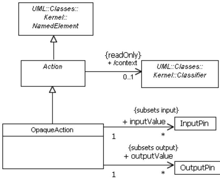
Figure 11.2 - Basic actions
