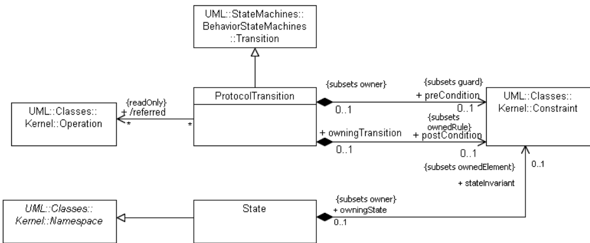
Figure 15.6 - Constraints
