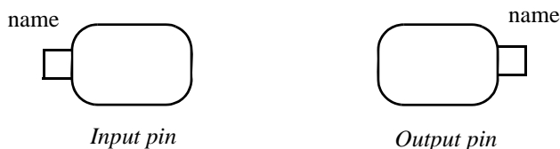
Figure 12.119 - Pin notations
