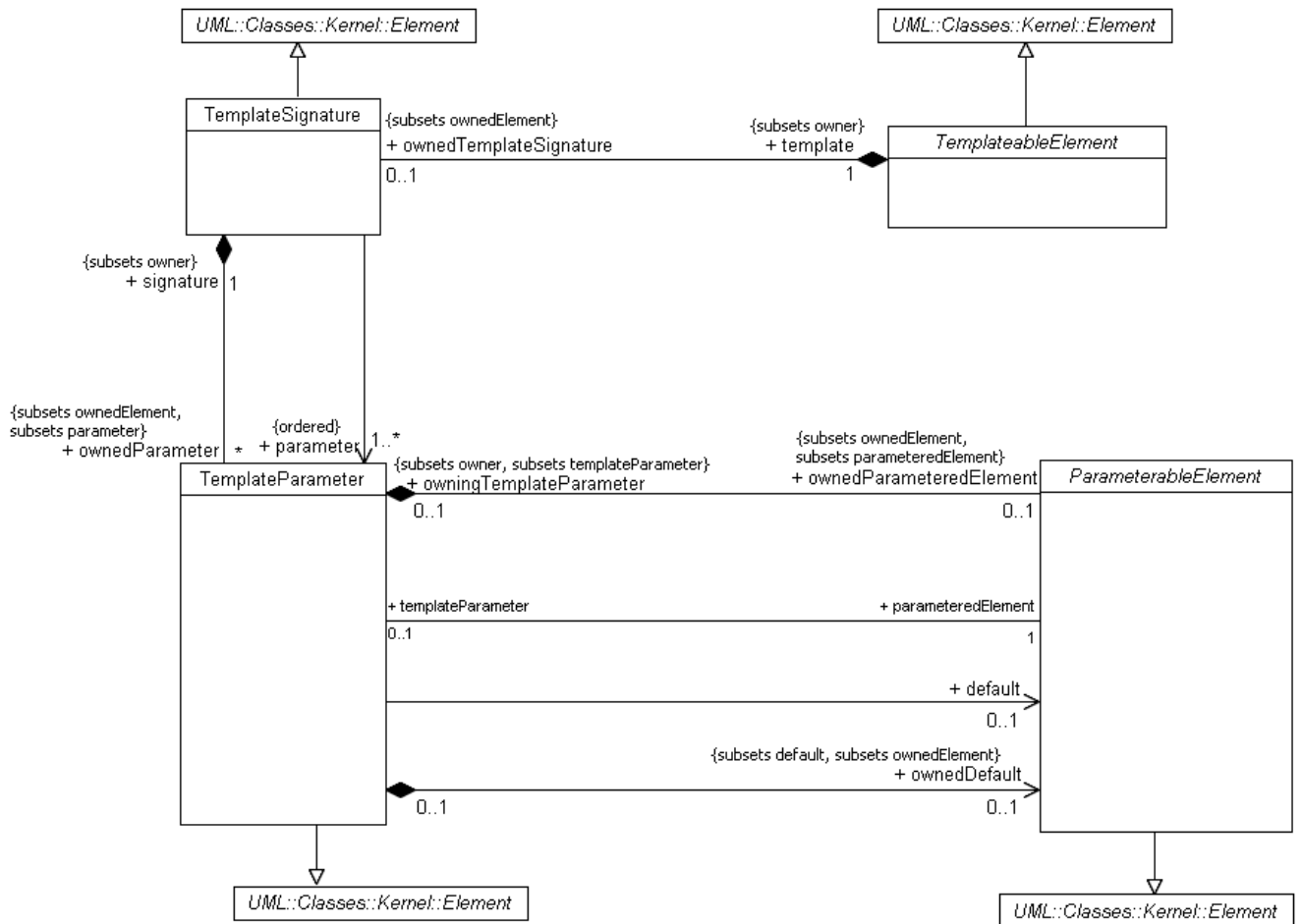
Figure 17.16 - Templates
