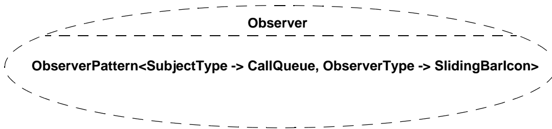
Figure 17.24 - Bound Collaboration
