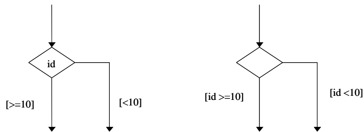
Figure 15.23 - Choice Pseudostate
