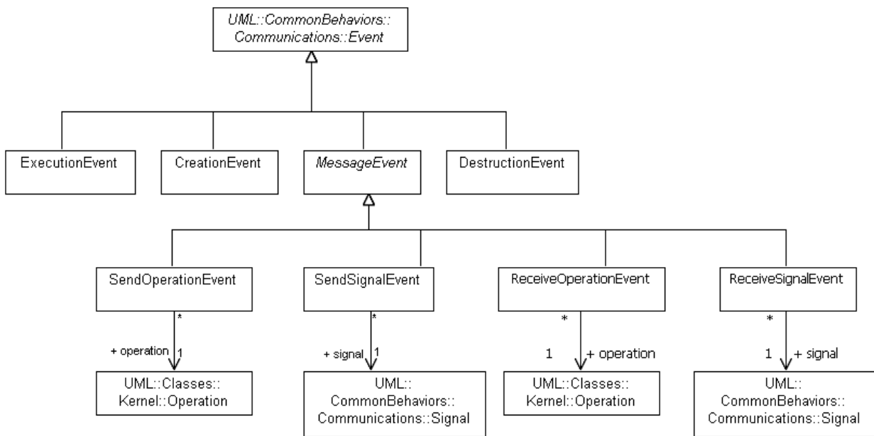
Figure 14.2 Events
