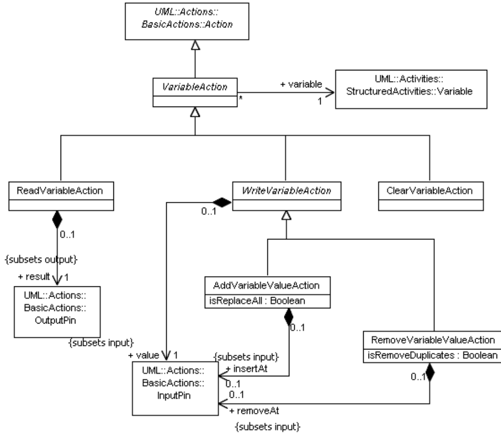
Figure 11.18 - Variable actions
