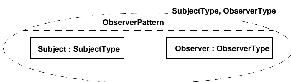
Figure 17.23 - Template Collaboration
