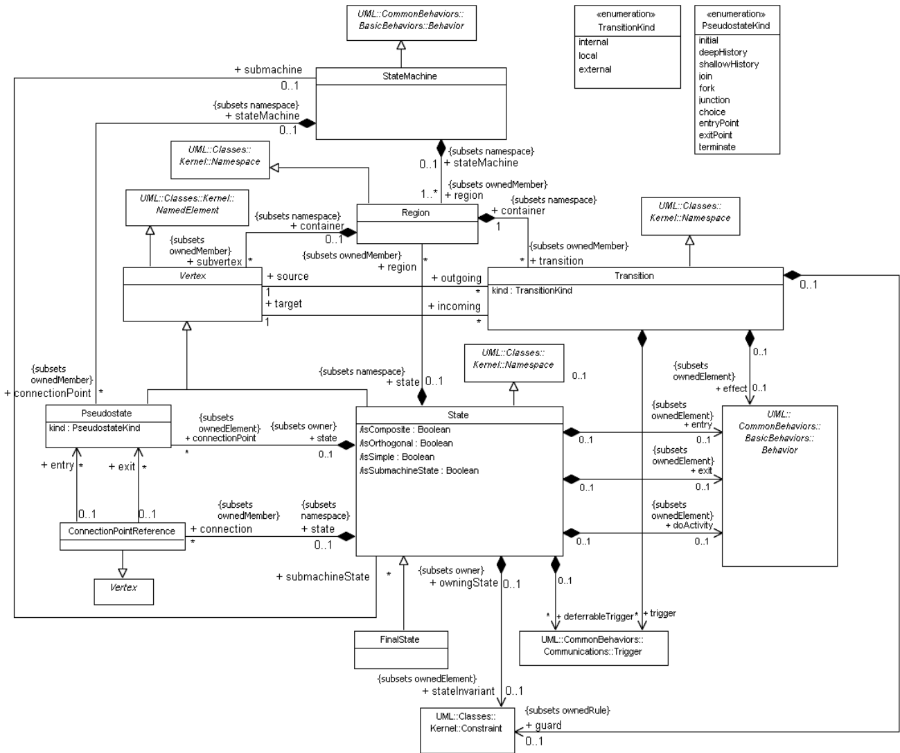
Figure 15.2 - State Machines
