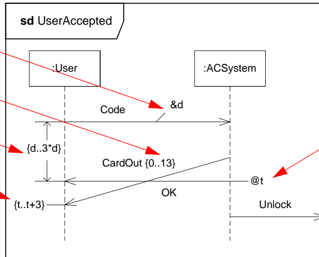
Figure 13.15 - DurationConstraint and other time-related concepts
