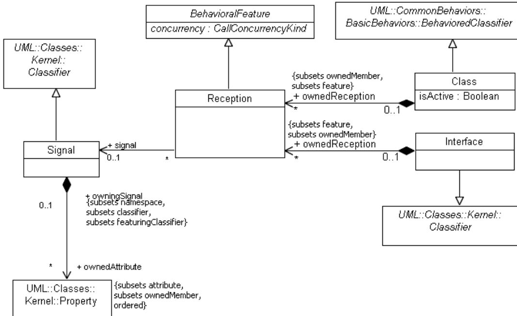
Figure 13.9 - Reception
