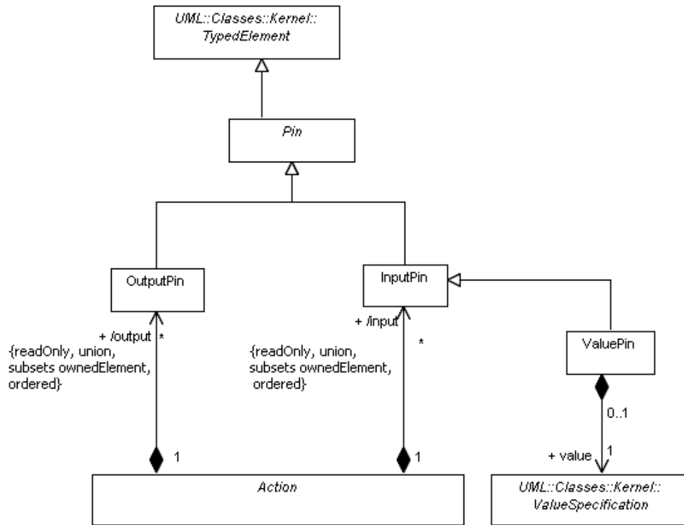
Figure 11.3 - Basic pins
