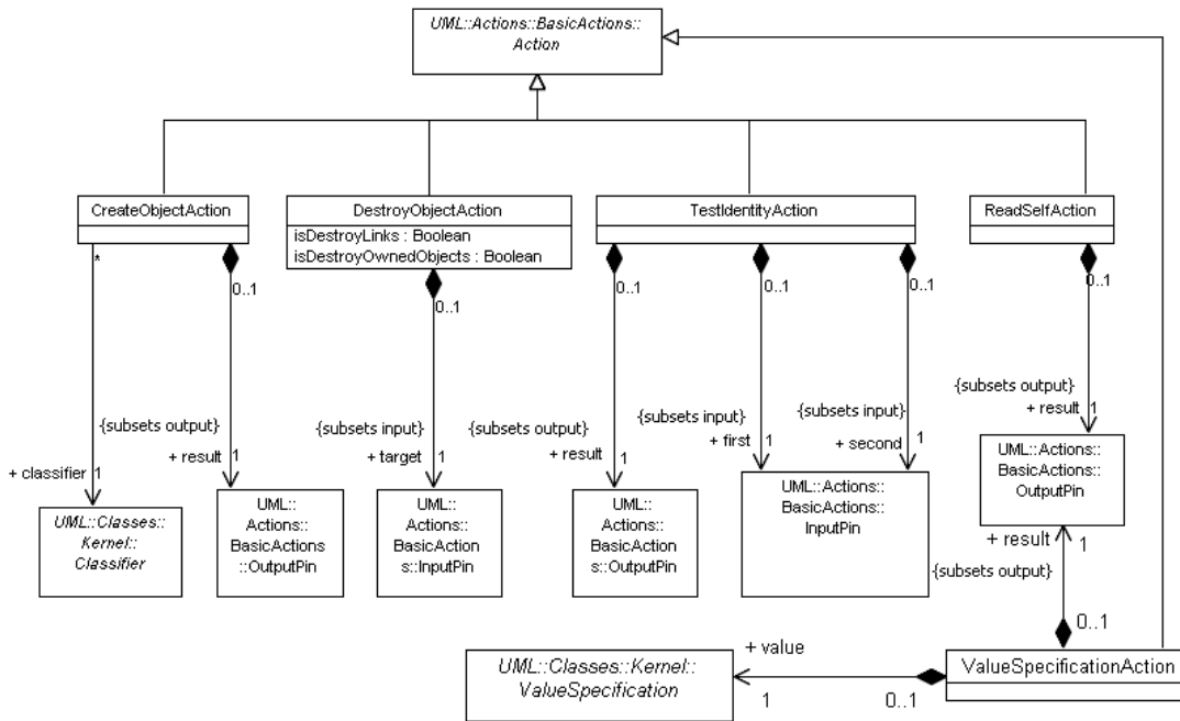
Figure 11.6 - Object actions
