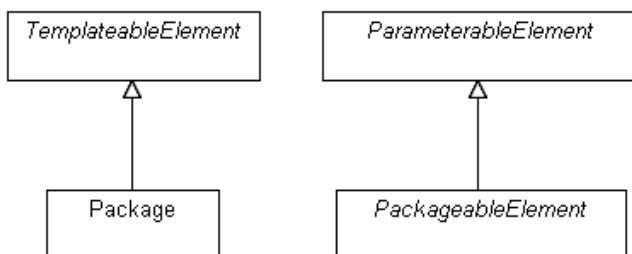
Figure 17.25 - Package templates
