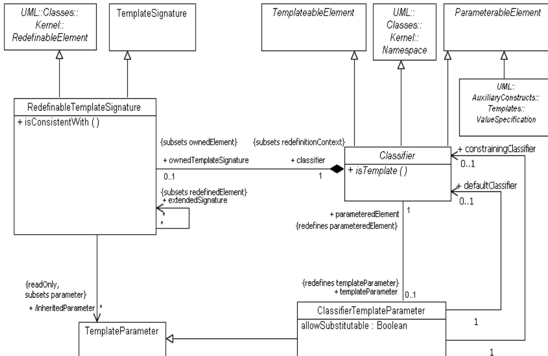
Figure 17.18 - Classifier templates
