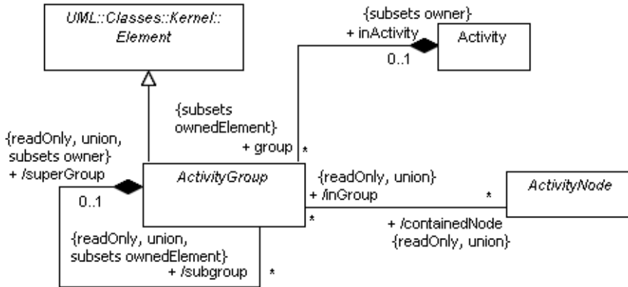
Figure 12.3 - Fundamental groups
