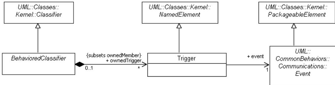
Figure 13.11 - Triggers
