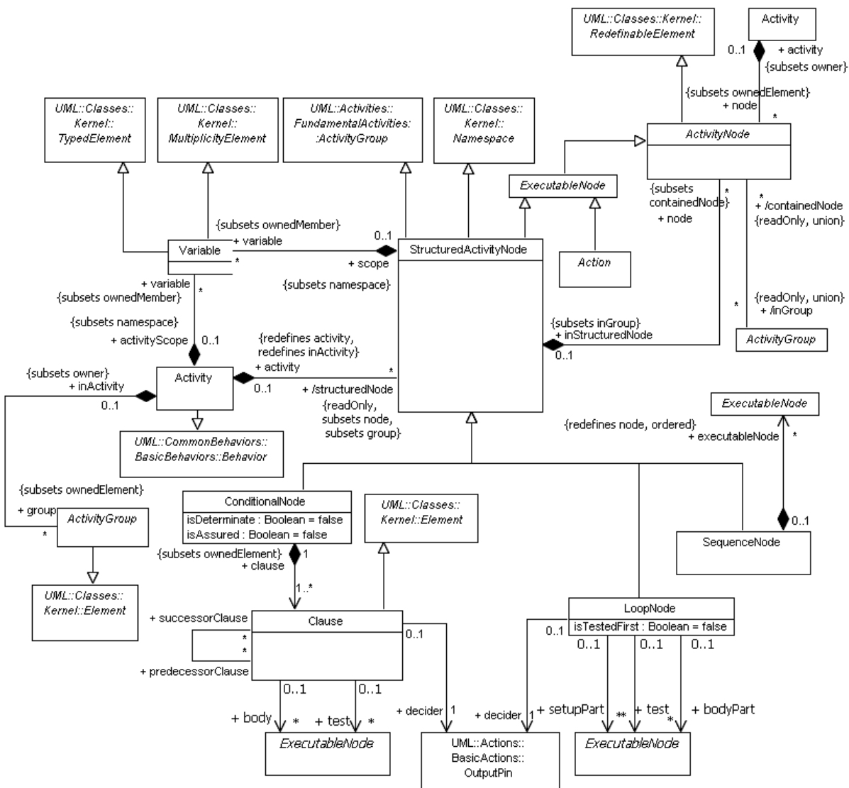
Figure 12.21 - Structured nodes
