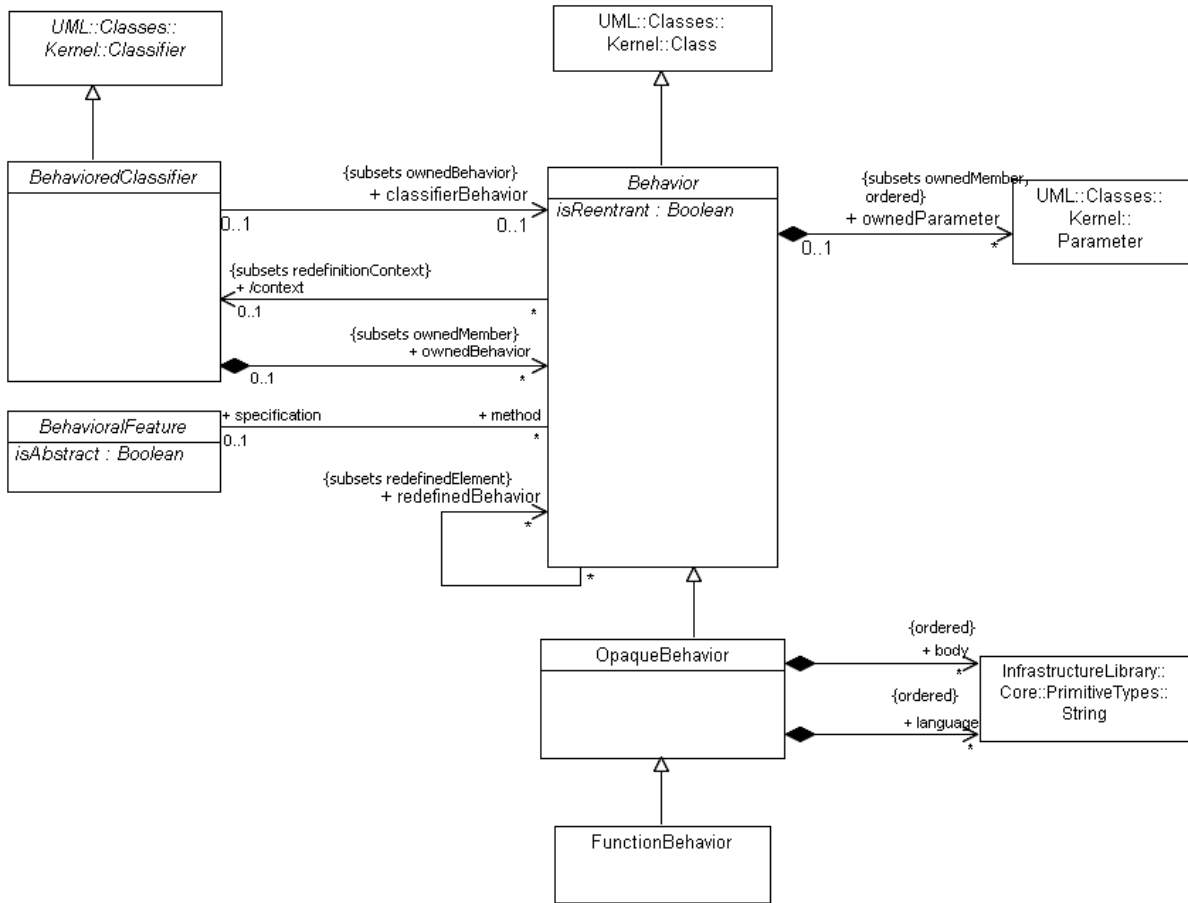
Figure 13.6 - Common Behavior
