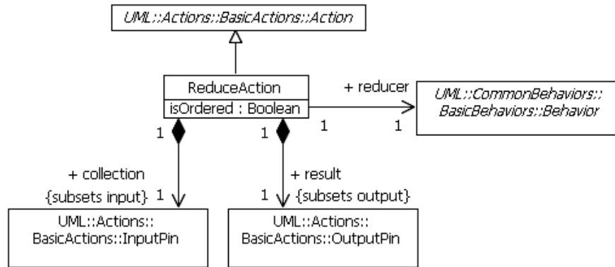
Figure 11.17 - ReduceAction (CompleteActions)
