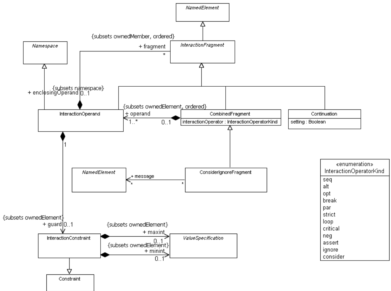
Figure 14.7 - CombinedFragments
