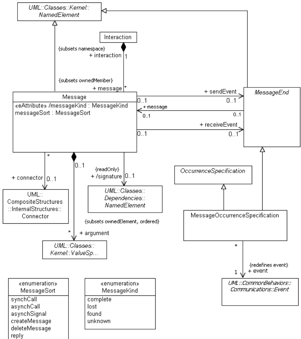
Figure 14.5 - Messages
