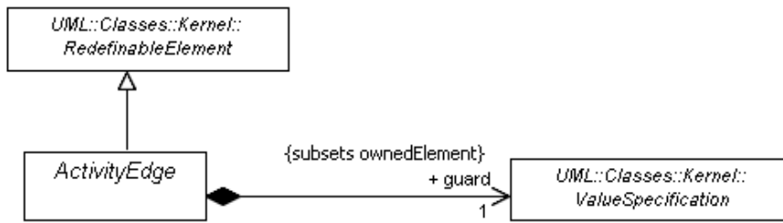
Figure 12.11 - Flows (IntermediateActivities)
