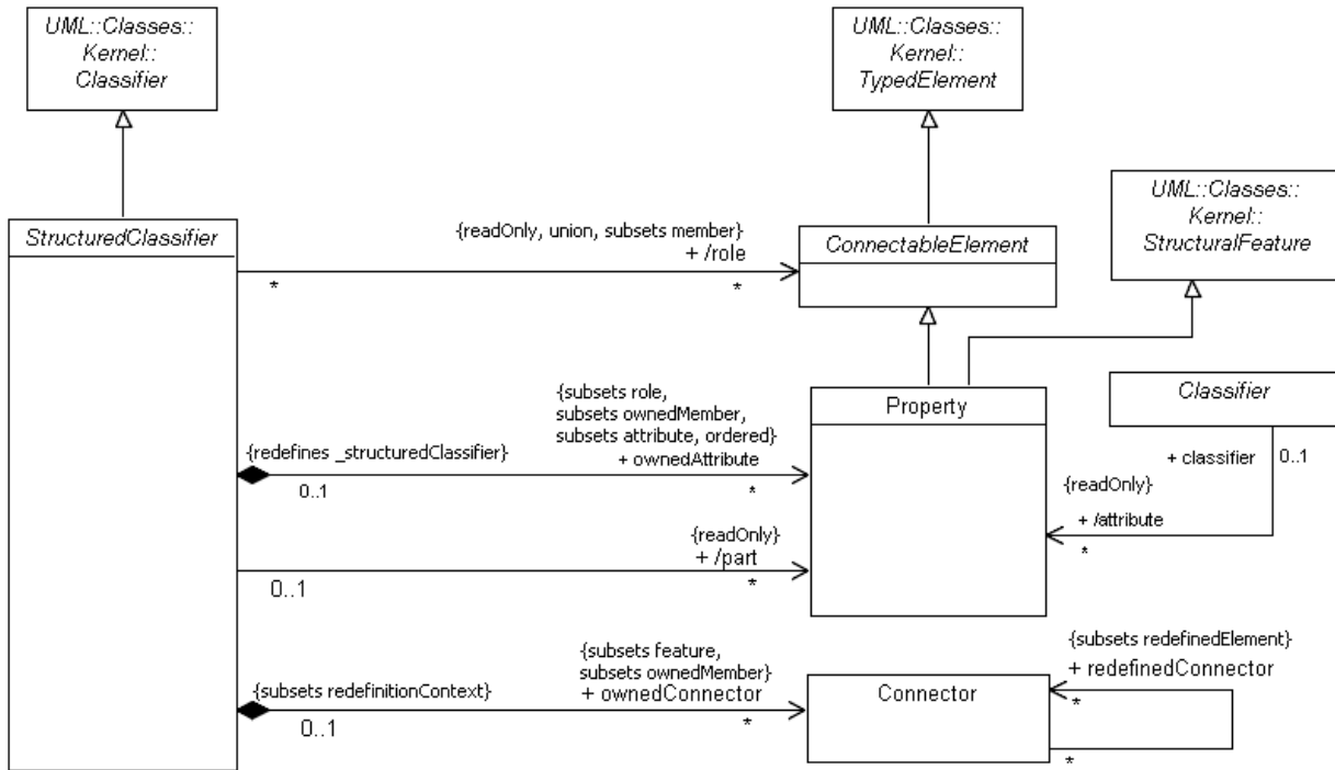
Figure 9.2 - Structured classifier
