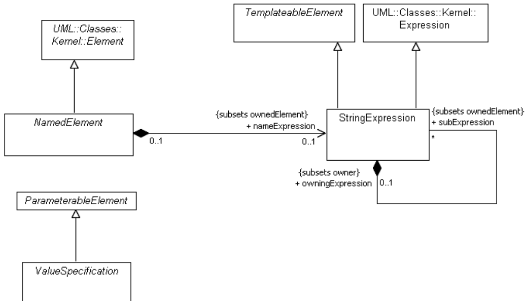
Figure 17.27 - Name expression
