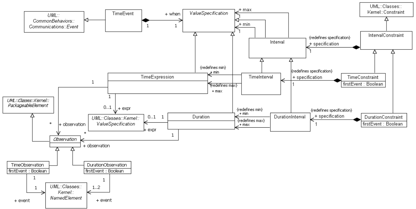
Figure 13.13 - SimpleTime
