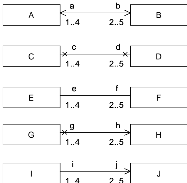
Figure 7.23 - Examples of navigable ends
