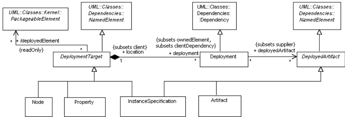
Figure 10.4 - Definition of the Deployment relationship between DeploymentTargets and DeployedArtifacts
