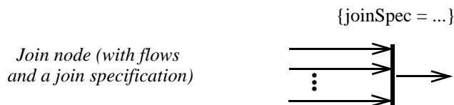
Figure 12.102 - Join node notations
