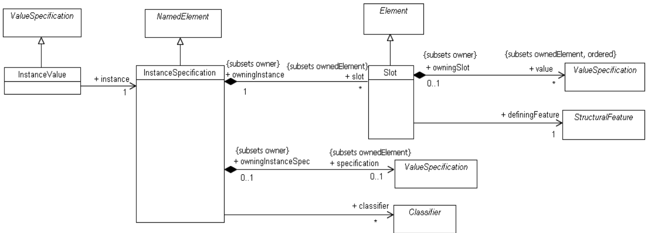
Figure 9.25 - The elements defined in the Instances package
