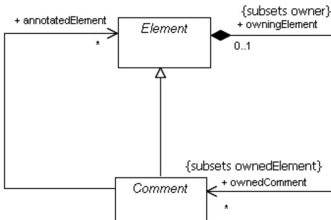
Figure 9.10 - The elements defined in the Comments package
