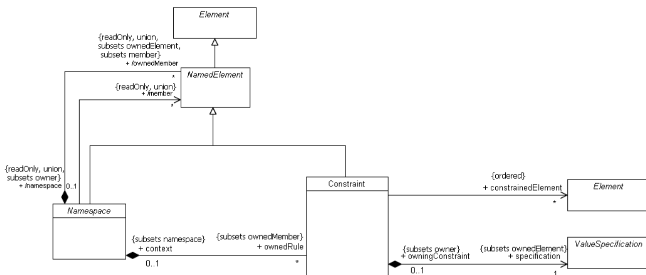
Figure 9.13 - The elements defined in the Constraints package
