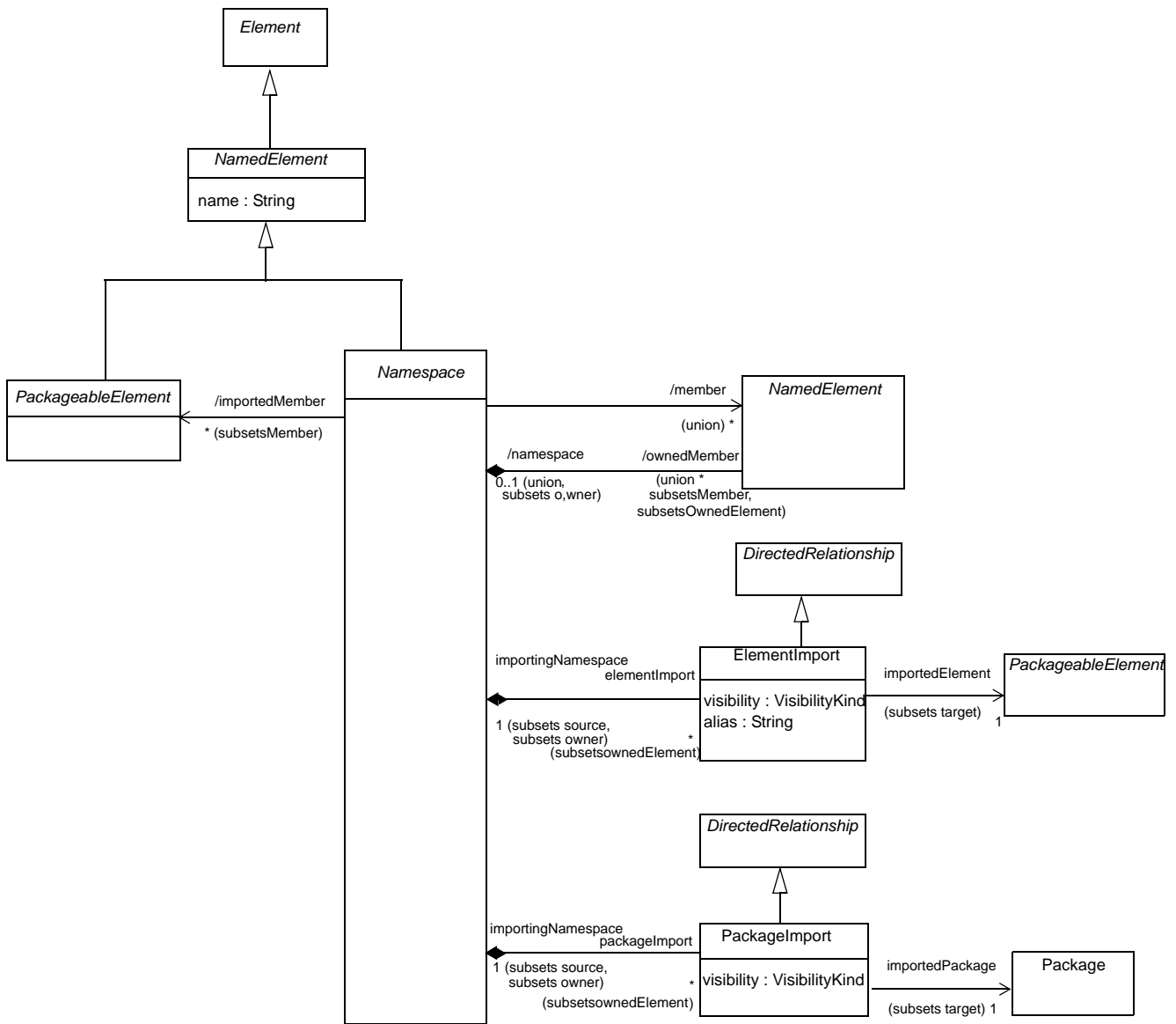
Figure 11.21 - The Namespaces diagram of the Constructs package
