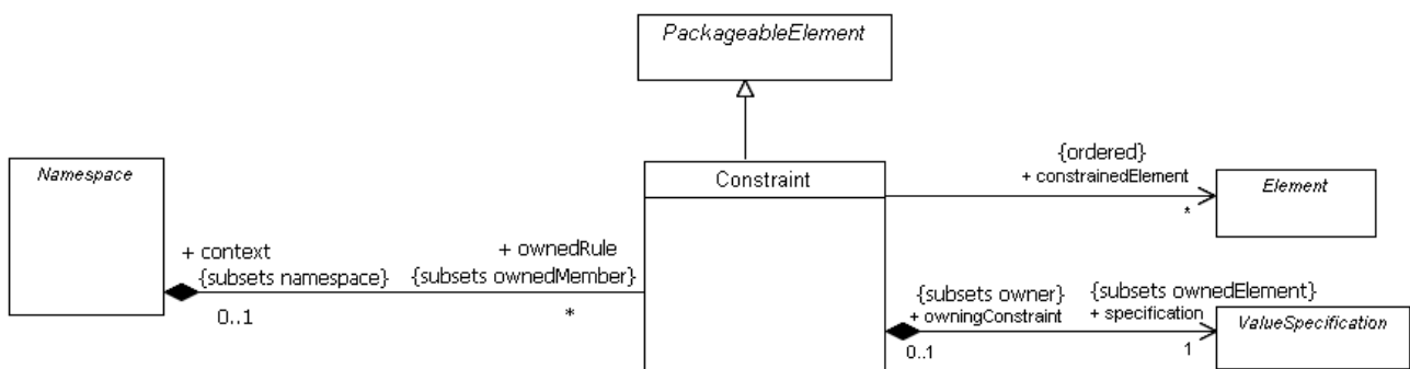
Figure 11.17 - The Classes diagram of the Constructs package
