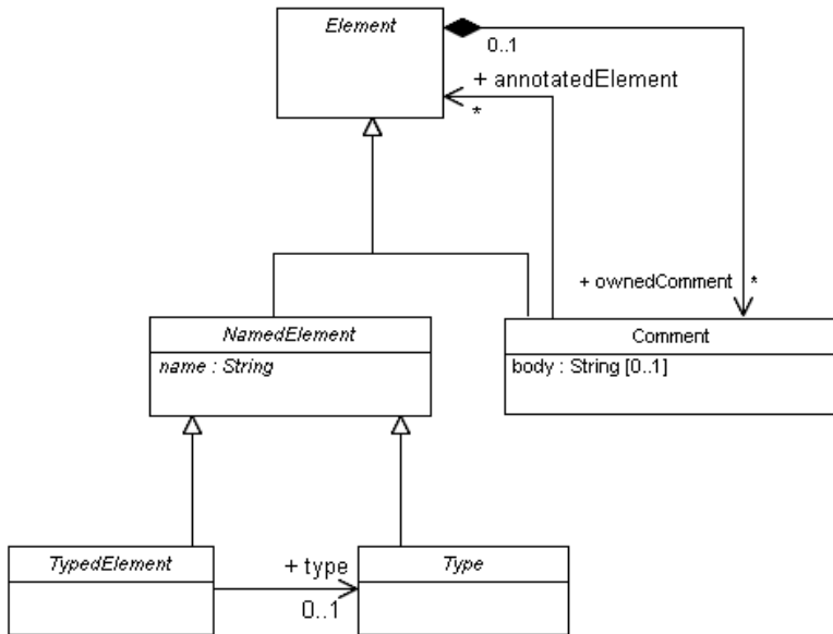
Figure 10.2 - The classes defined in the Types diagram
