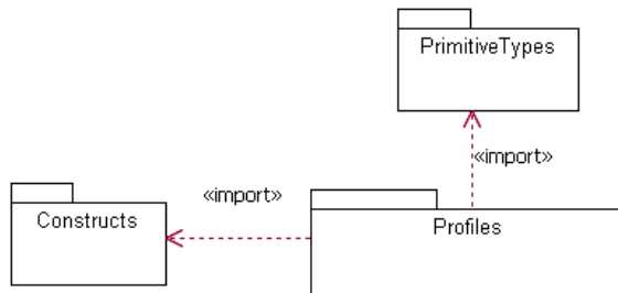
Figure 18.1 - Dependencies between packages described in this chapter
