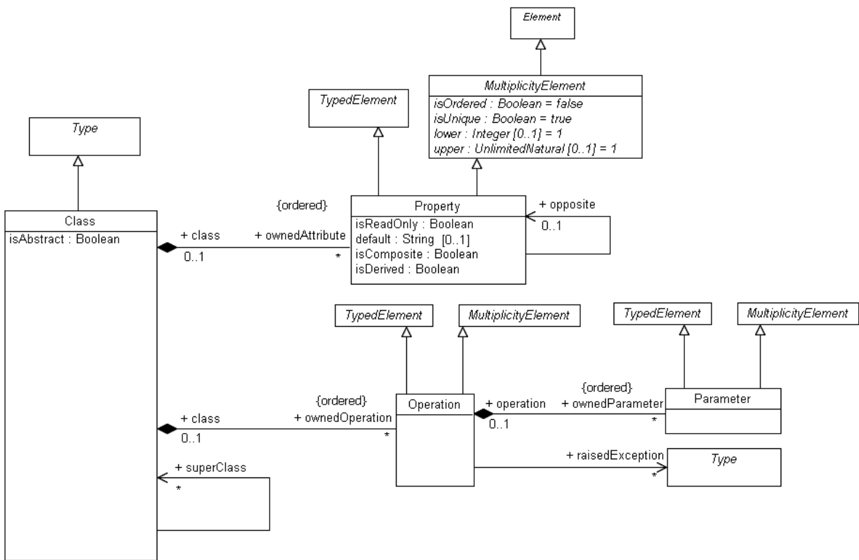
Figure 10.3 - The classes defined in the Classes diagram
