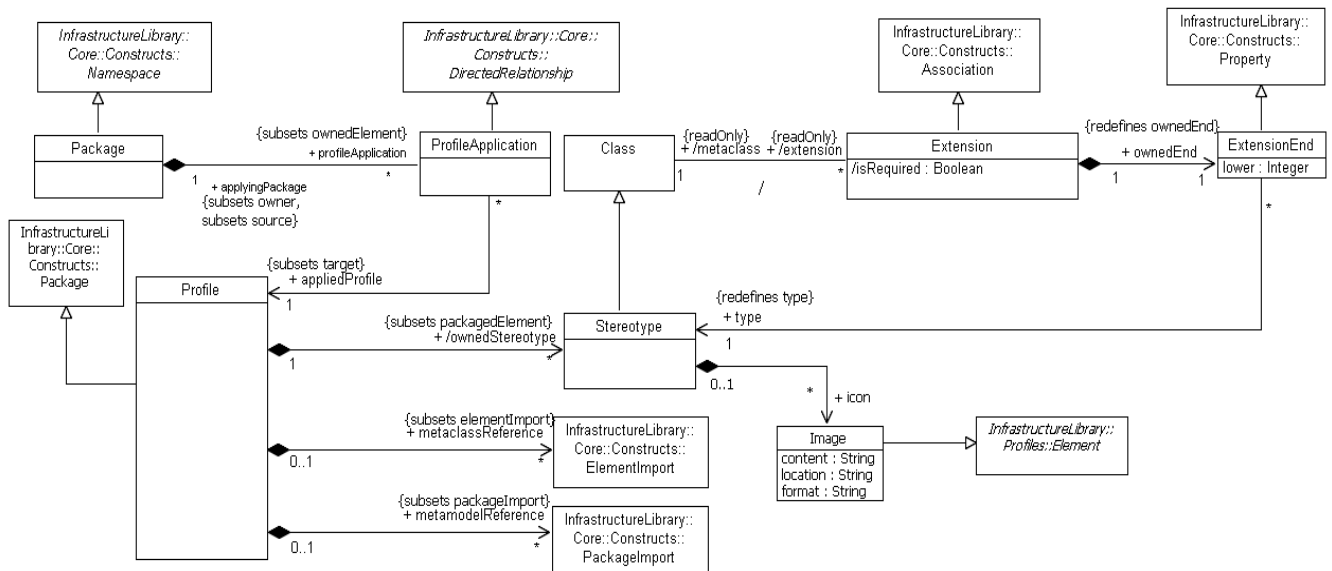
Figure 18.2 - The classes defined in the Profiles package
