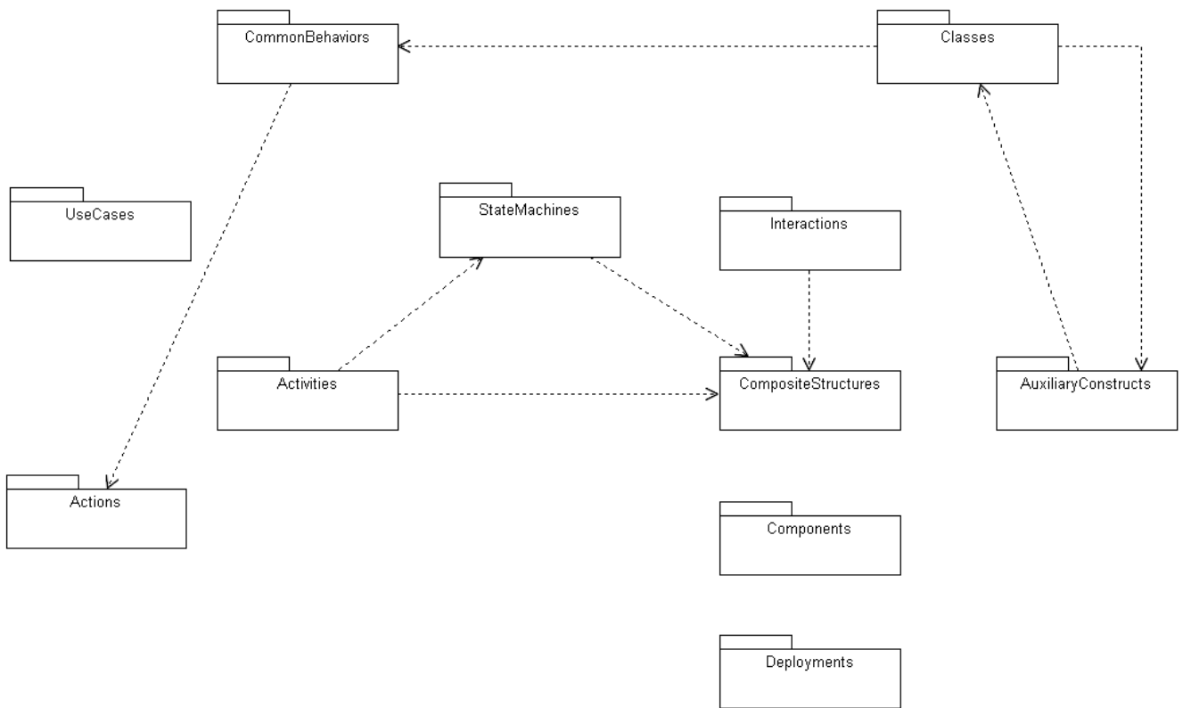
Figure 7.5 - The top-level package structure of the UML 2.1 Superstructure
