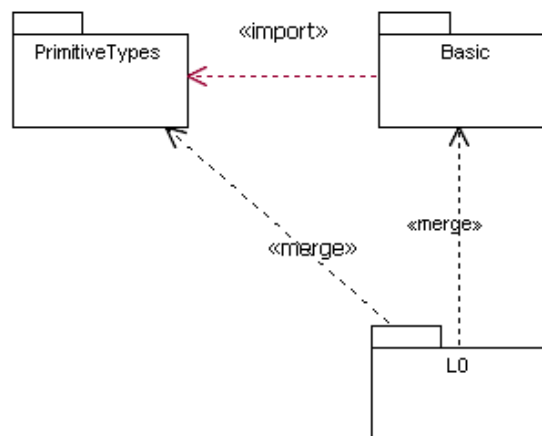
Figure 7.1 Level 0 package diagram
