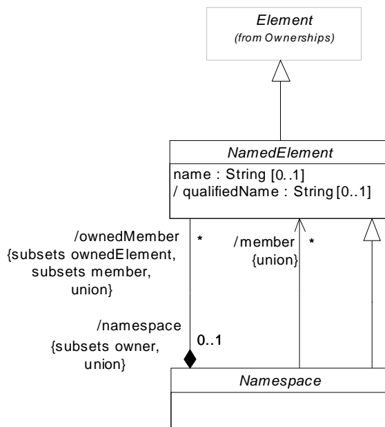
Figure 9.38 - The elements defined in the Namespaces package
