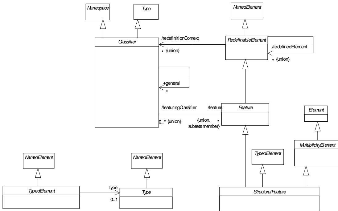
Figure 11.16 - The Classifiers diagram of the Constructs package
