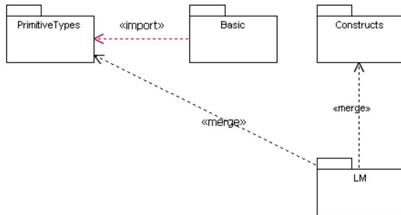
Figure 7.2 Level M package diagram
