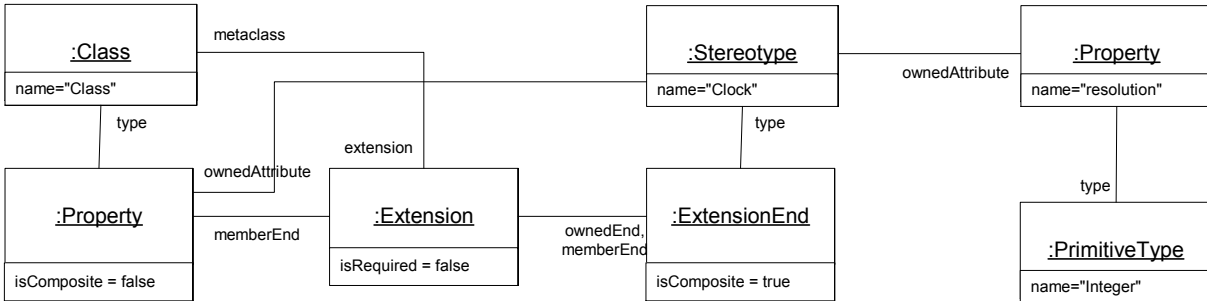
Figure 121 - An instance specification when defining a stereotype
