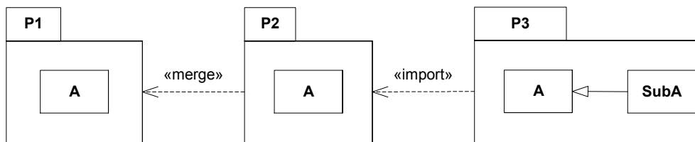
Figure 96 - Illustration of the meaning of package merge
