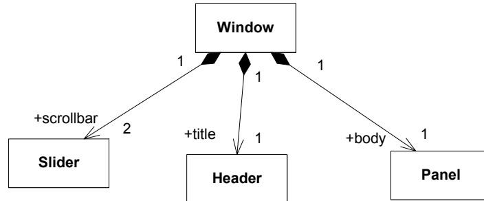
Figure 79 - Composite aggregation is depicted as a black diamond
