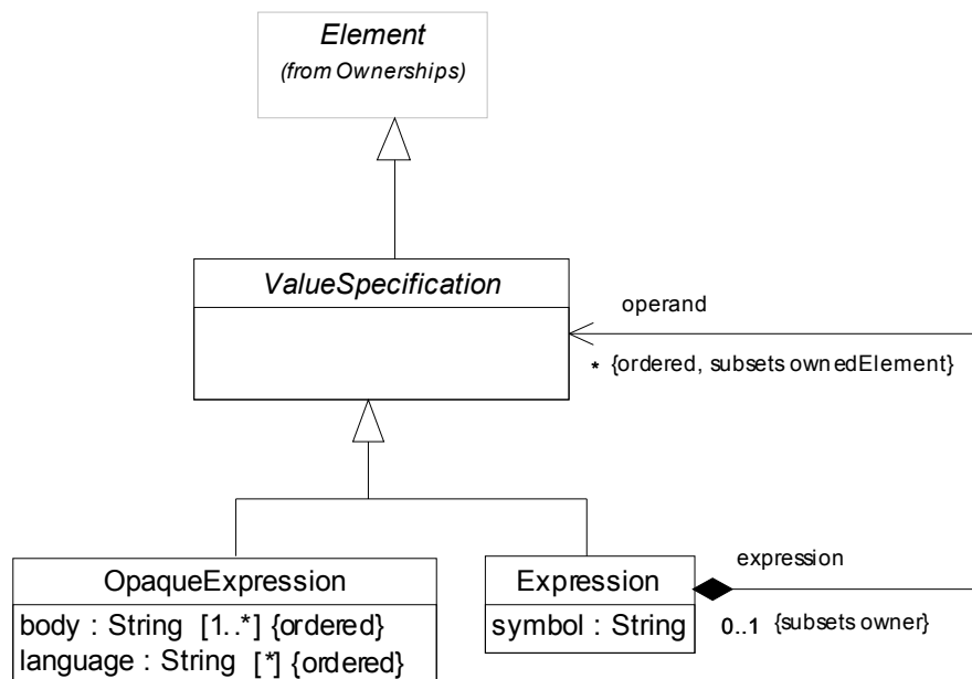
Figure 30 - The elements defined in the Expressions package
