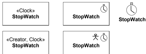
Figure 120 - Presentation options for an extended class
