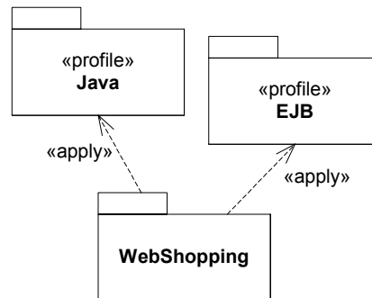
Figure 118 - Profiles applied to a package
