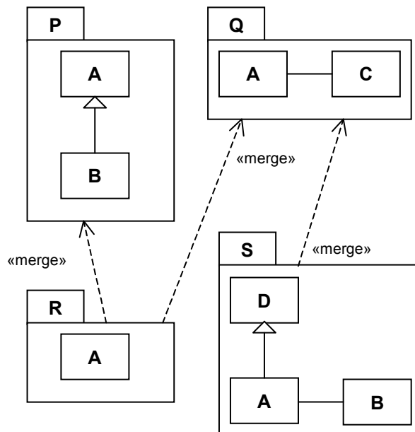
Figure 99 - Simple example of package merges
