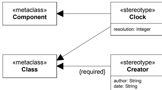
Figure 122 - Defining multiple stereotypes on multiple stereotypes
