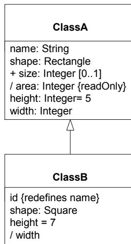
Figure 82 - Examples of attributes
