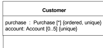
Figure 43 - Multiplicity within a textual specification
