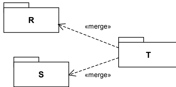
Figure 101 - Introducing additional package merges
