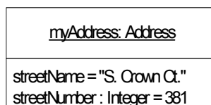
Figure 37 - Slots with values
