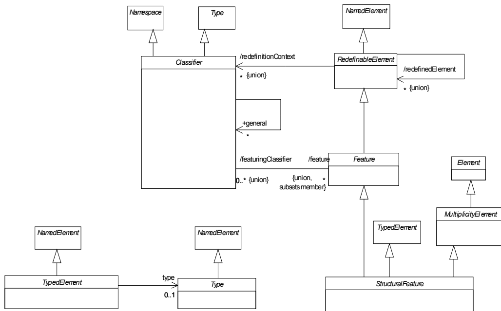
Figure 84 - The Classifiers diagram of the Constructs package
