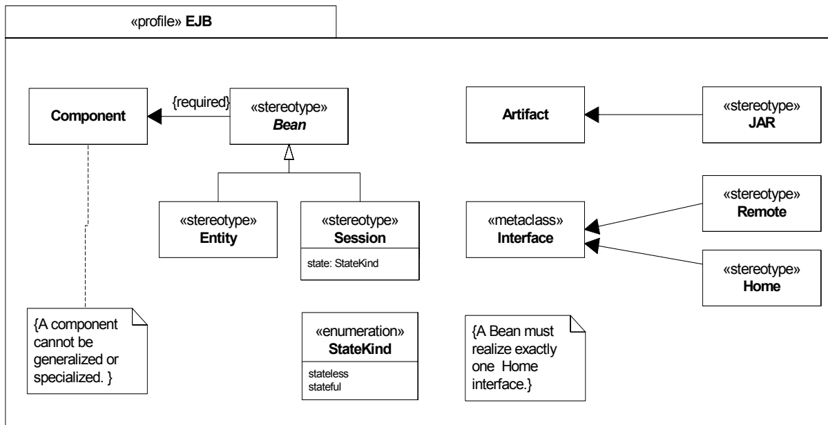
Figure 116 - Defining a simple EJB profile
