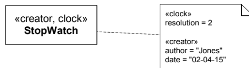
Figure 125 - Using stereotypes and showing values
