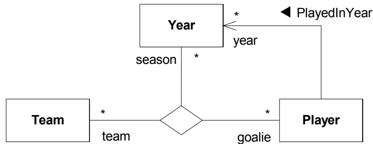
Figure 74 - Binary and ternary associations
