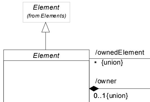
Figure 50 - The elements defined in the Ownerships package
