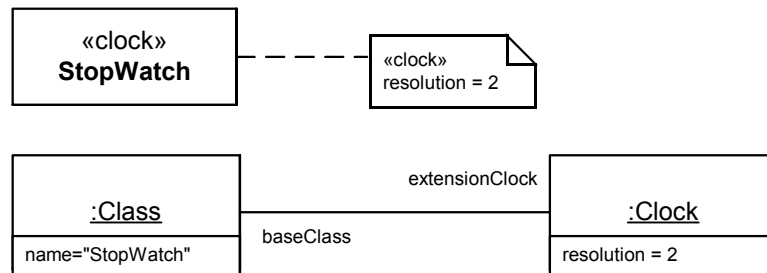
Figure 124 - Showing values of stereotypes and a simple instance specification
