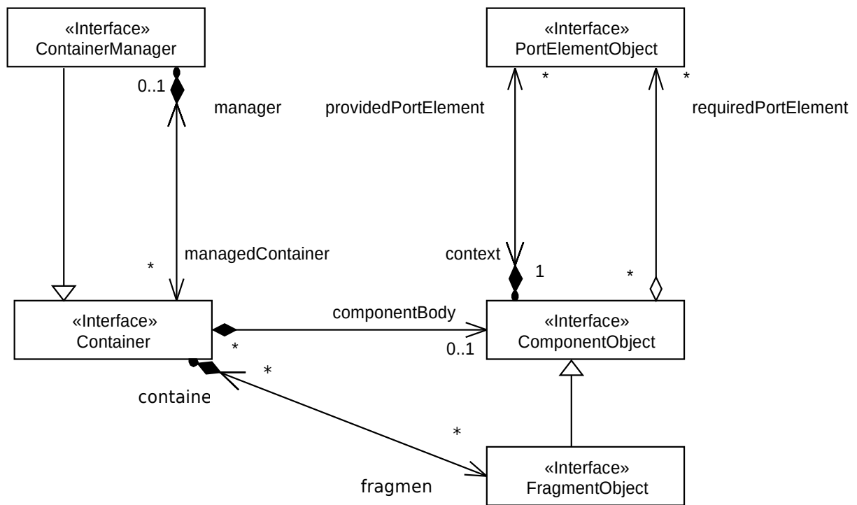
Figure 39: UCM container model
