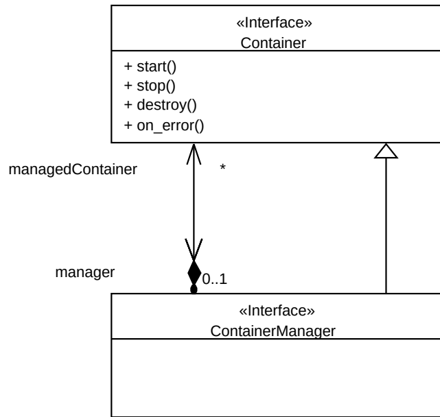
Figure 41: Container and container manager
