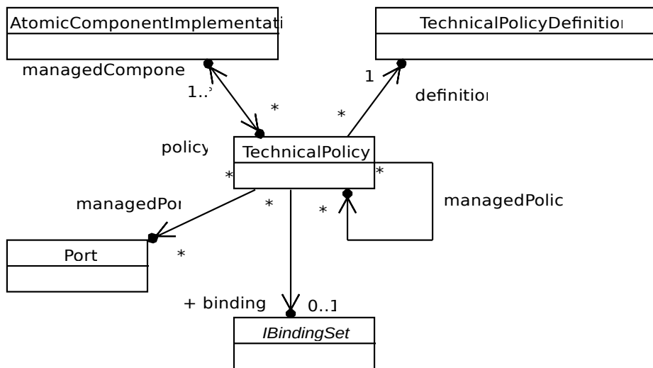
Figure 33: UCM technical policies
