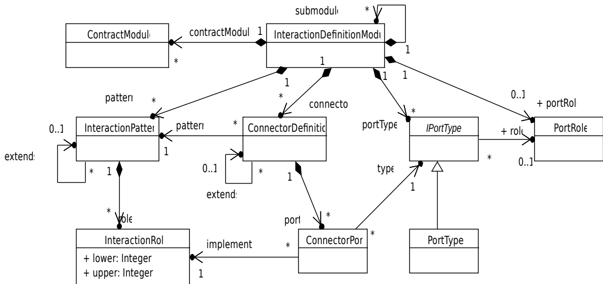
Figure 23: Main classes of the UCM interaction package
