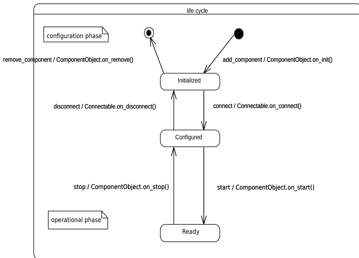
Figure 42: UCM component instance life cycle
