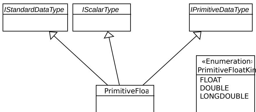
Figure 9: UCM floating point numbers
