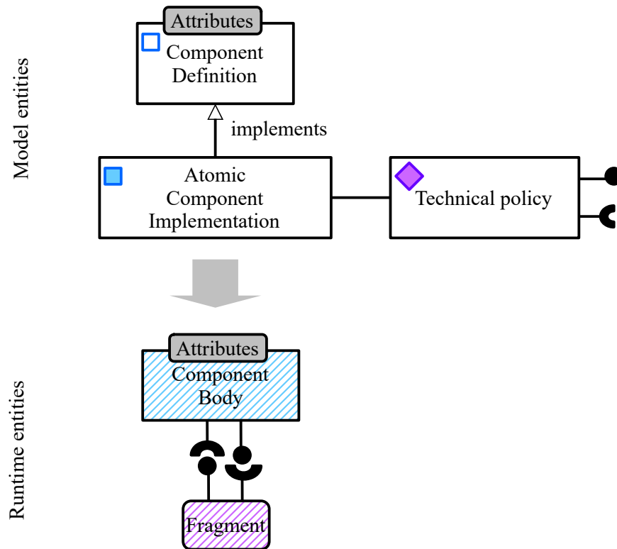
Figure 37: Technical policy fragmentation example
