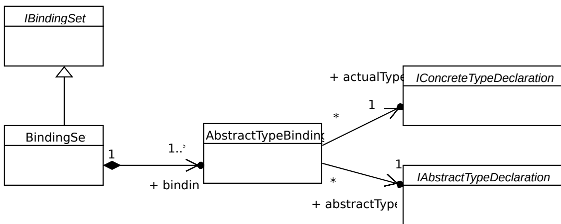
Figure 29: UCM binding sets
