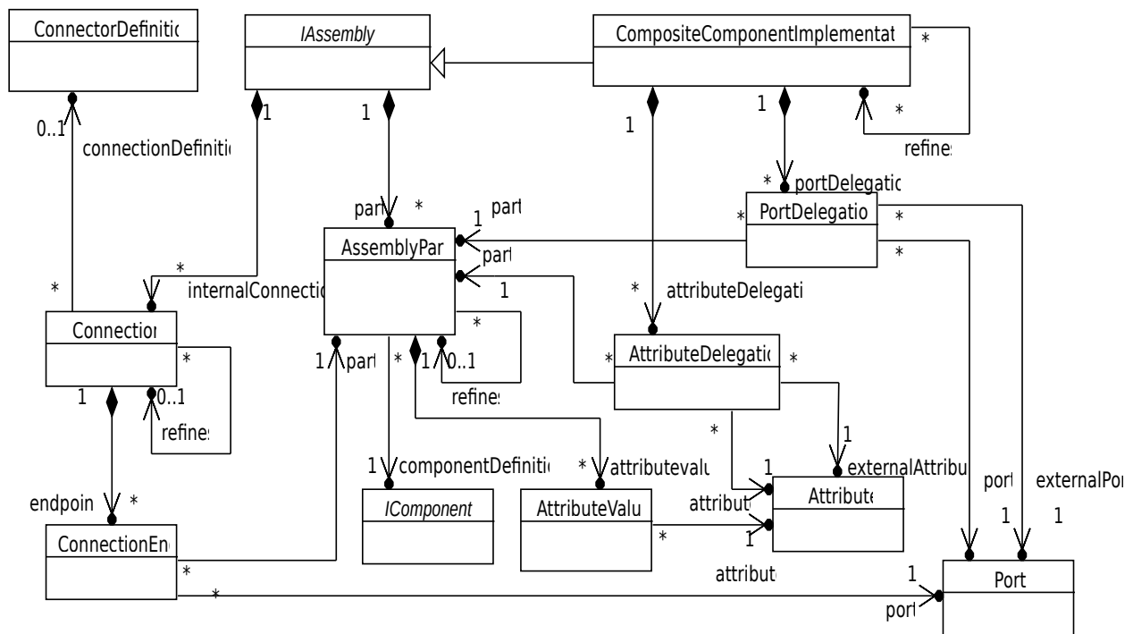
Figure 34: UCM composite component implementations
