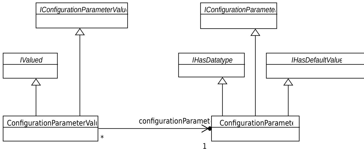
Figure 20: UCM configuration elementsparameters
