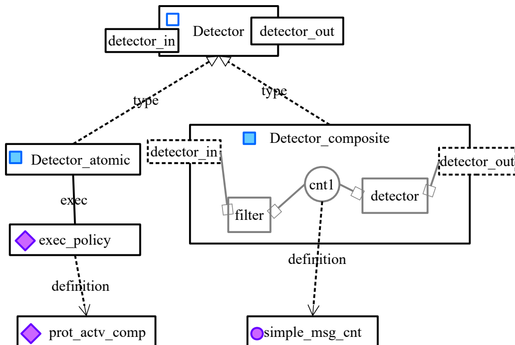
Figure 35: graphical example
