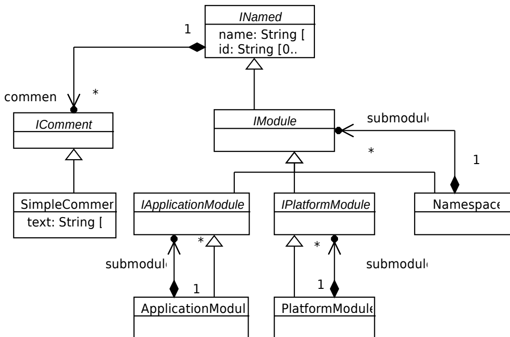
Figure 5: Base classes
