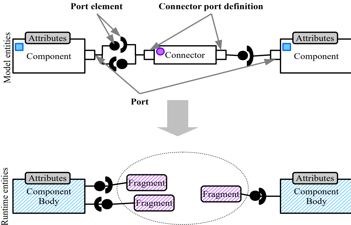
Figure 36: Connector fragmentation example
