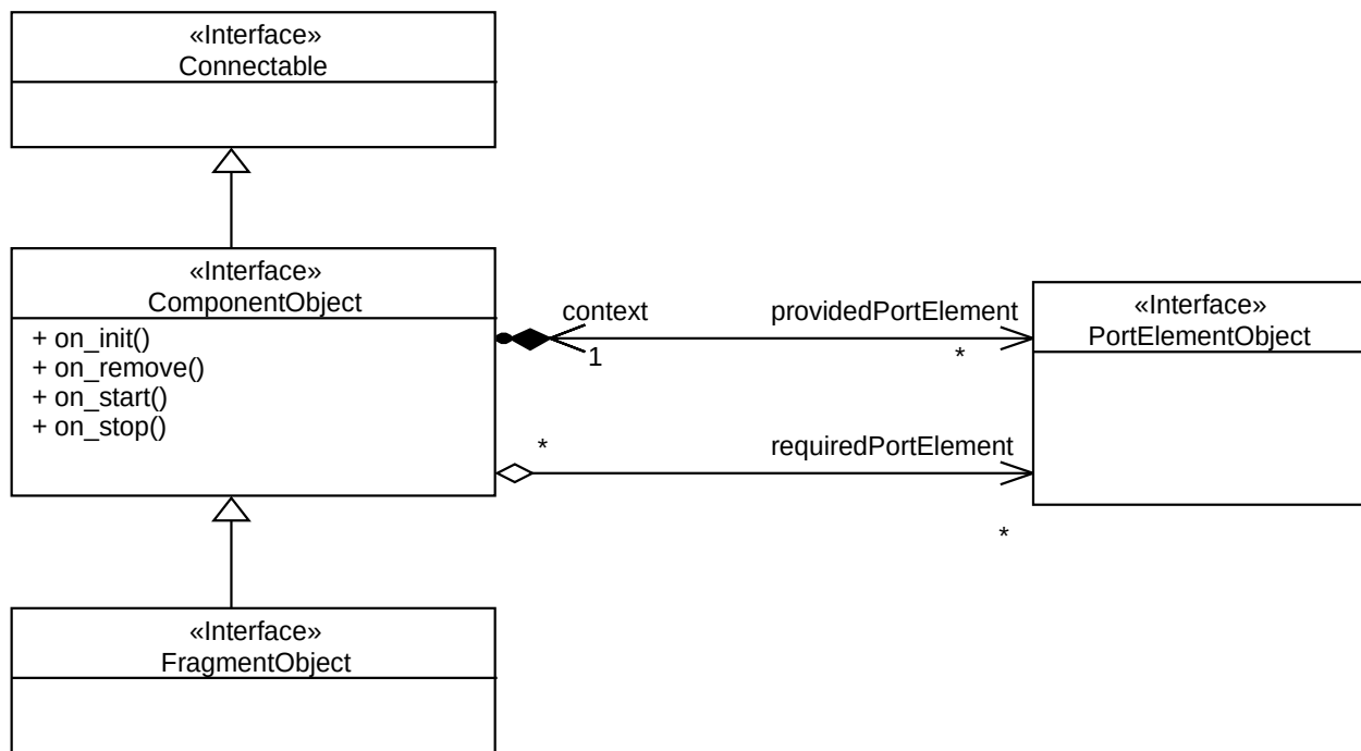
Figure 40: UCM component object interfaces
