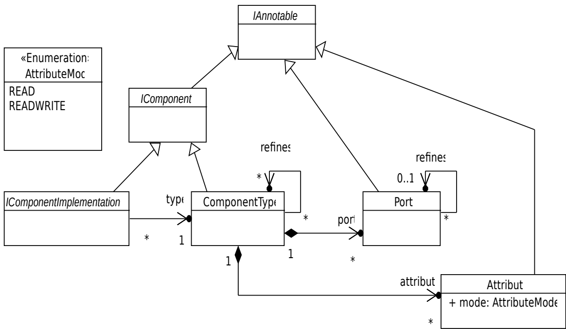
Figure 30: UCM component types
