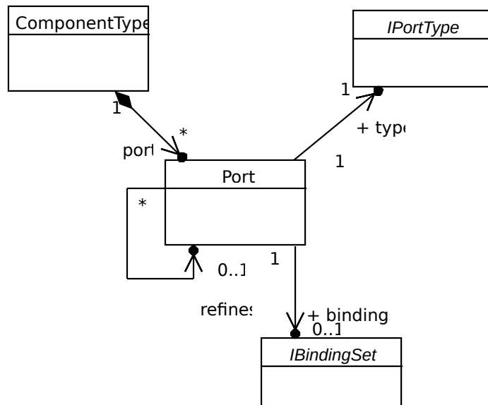
Figure 31: UCM component ports
