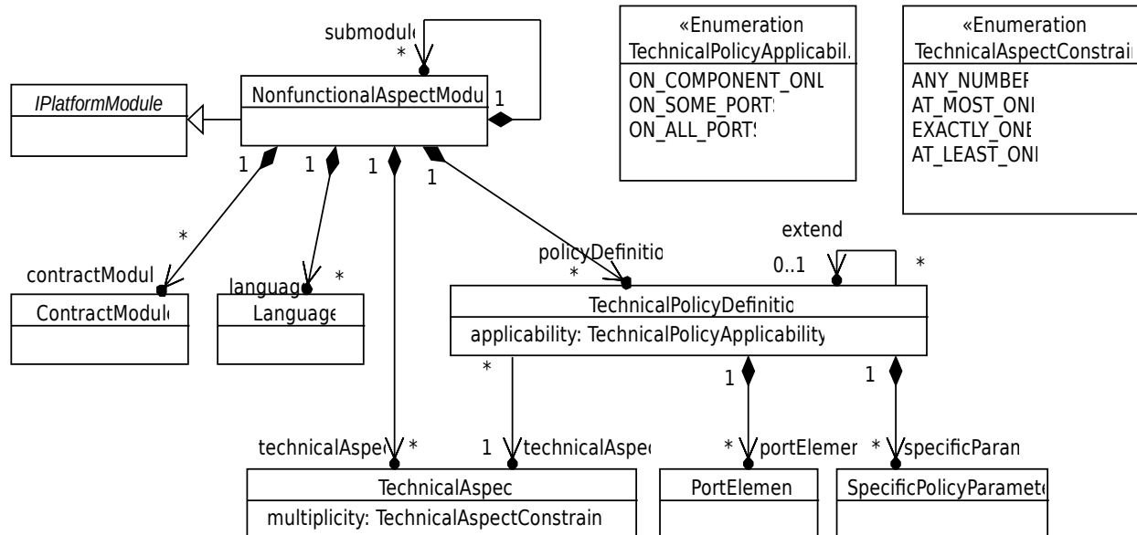
Figure 27: Main classes of UCM technical policies package
