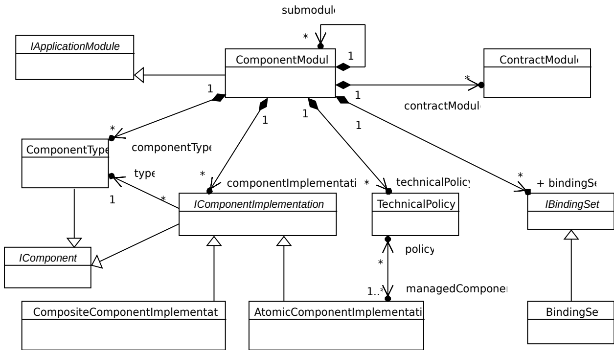
Figure 28: Main classes involved in the UCM component package
