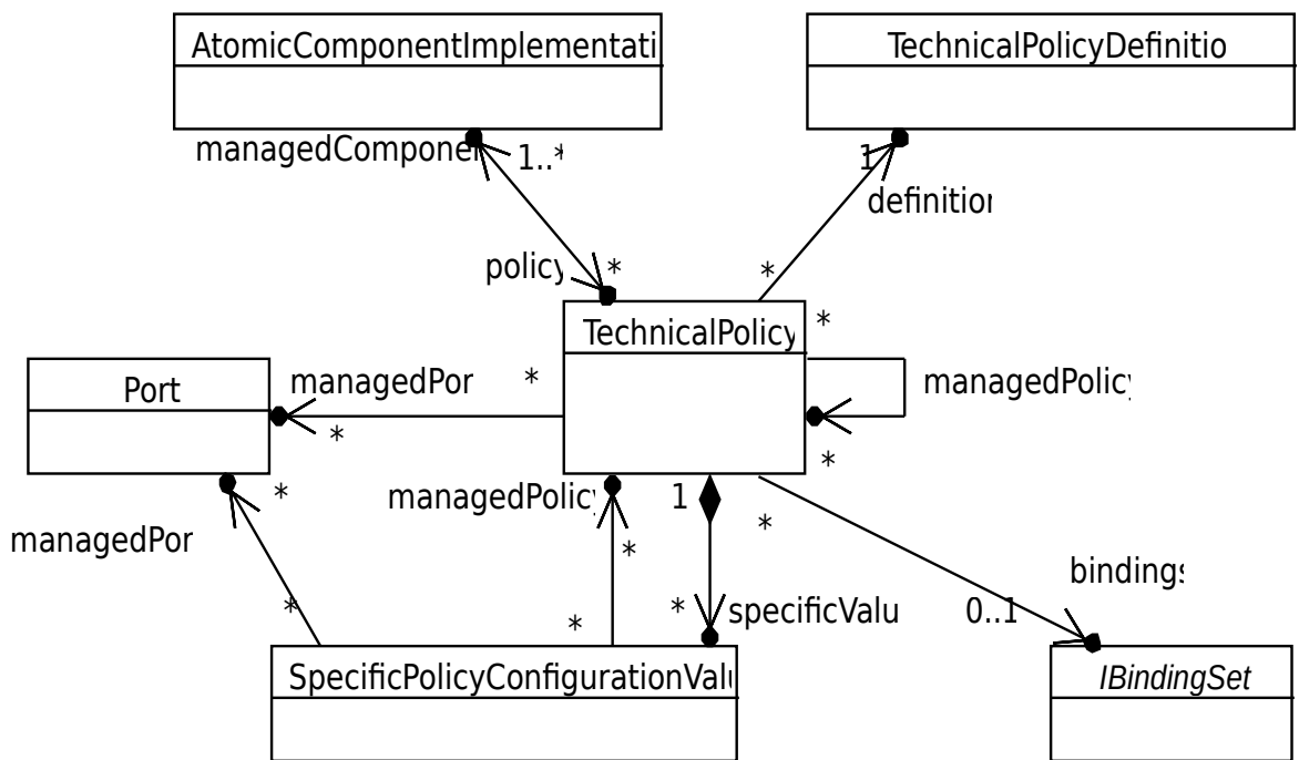
Figure 32: UCM atomic component implementations
