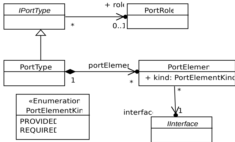
Figure 26: UCM port types
