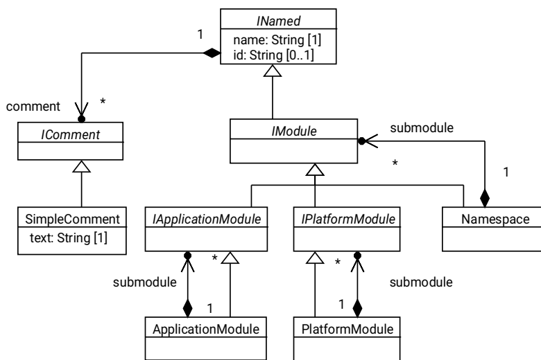
Figure 5: Base classes
