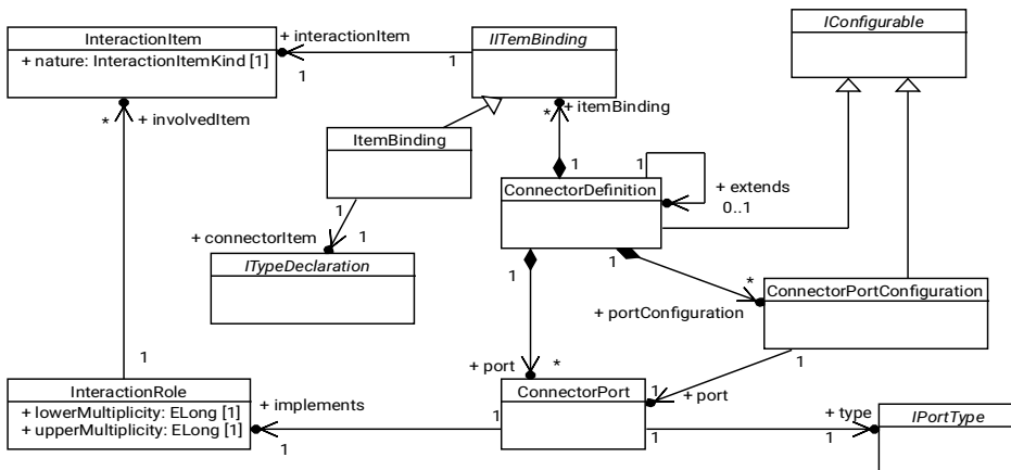
Figure 25: UCM connectors
