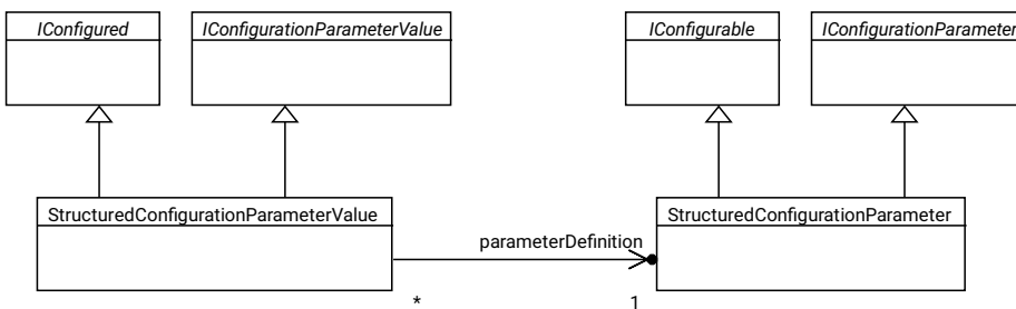
Figure 22: UCM structured configuration parameters
