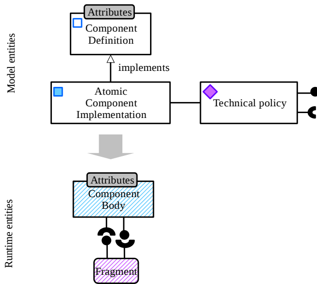
Figure 37: Technical policy fragmentation example
