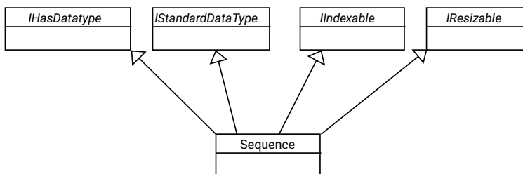
Figure 16: UCM sequence
