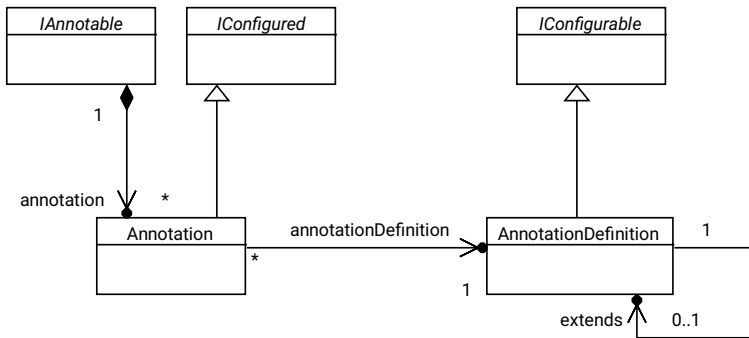
Figure 21: UCM annotations
