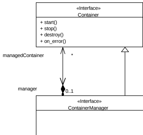
Figure 41: Container and container manager
