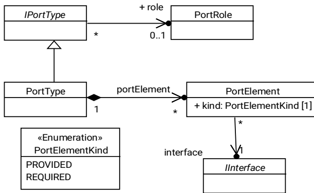
Figure 26: UCM port types
