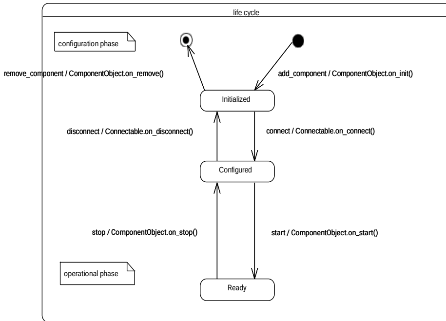
Figure 42: UCM component instance life cycle
