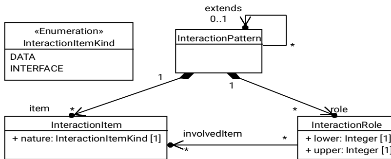
Figure 24: UCM interaction patterns
