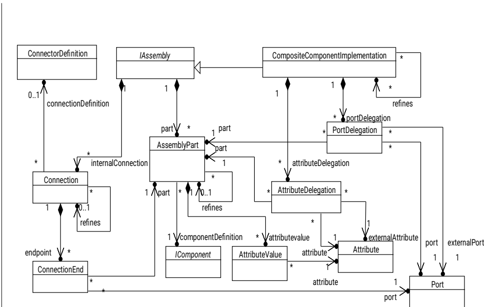
Figure 34: UCM composite component implementations
