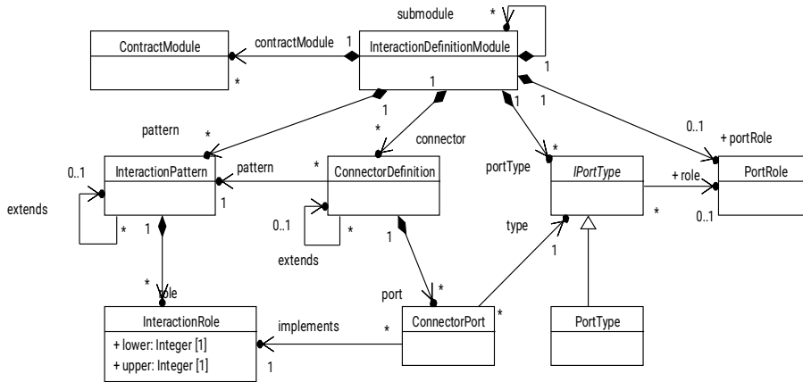
Figure 23: Main classes of the UCM interaction package
