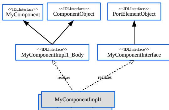
Figure 43: generated IDL interfaces
