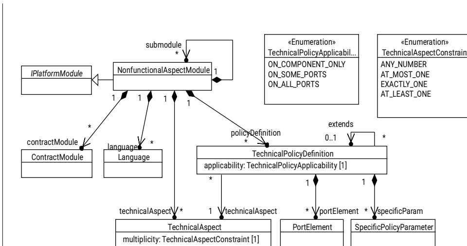
Figure 27: Main classes of UCM technical policies package
