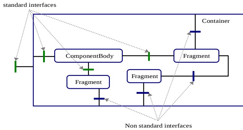
Figure 38: UCM Runtime Interfaces
