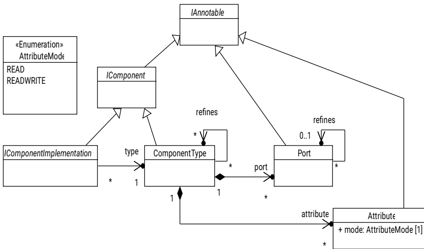
Figure 30: UCM component types
