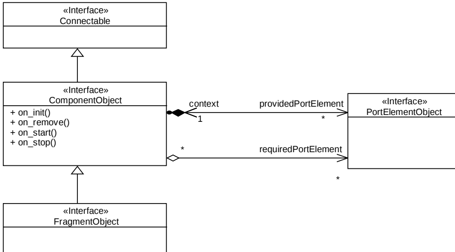
Figure 40: UCM component object interfaces
