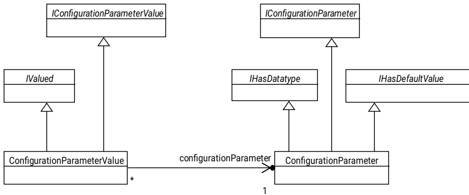
Figure 20: UCM configuration elements parameters
