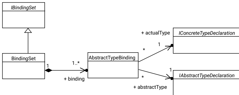
Figure 29: UCM binding sets
