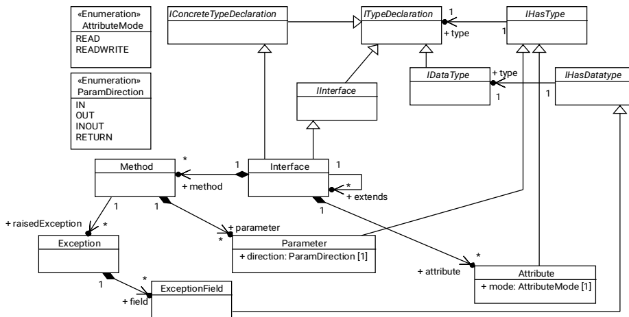
Figure 18: UCM interfaces
