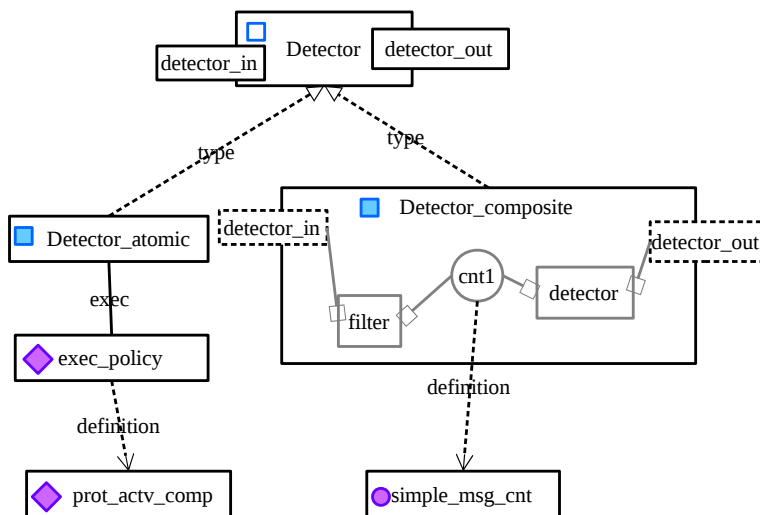
Figure 35: graphical example
