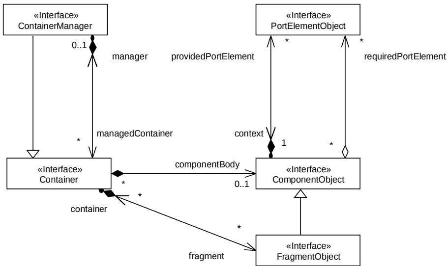
Figure 39: UCM container model
