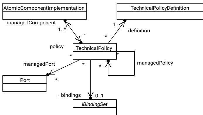
Figure 33: UCM technical policies
