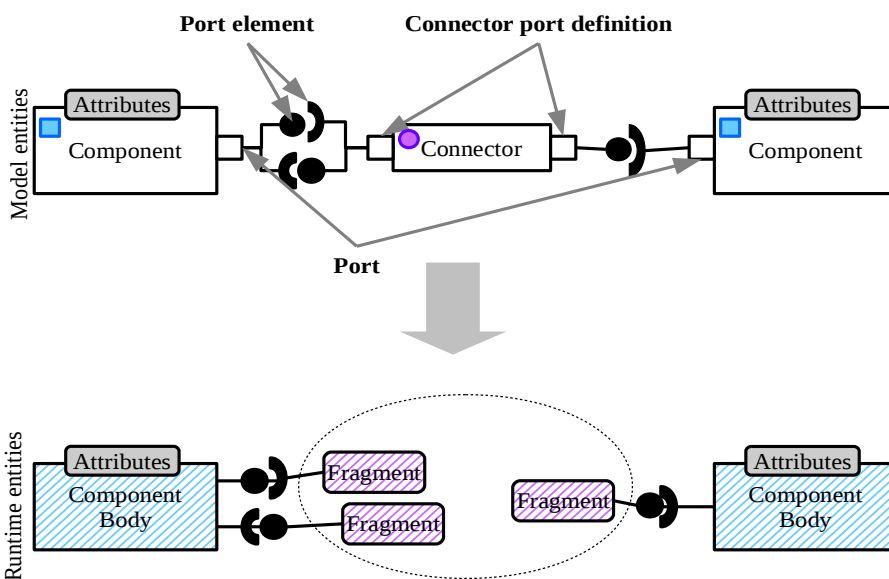
Figure 36: Connector fragmentation example
