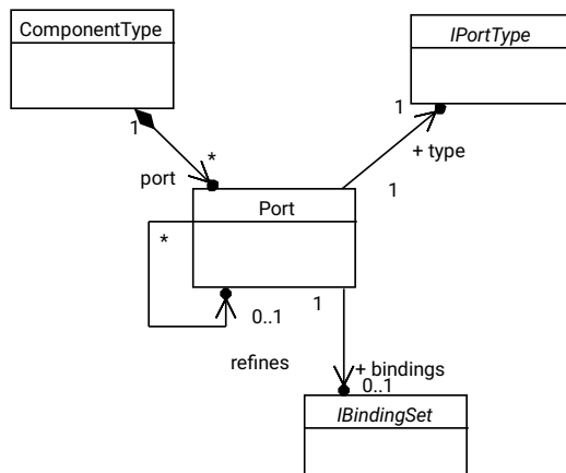
Figure 31: UCM component ports
