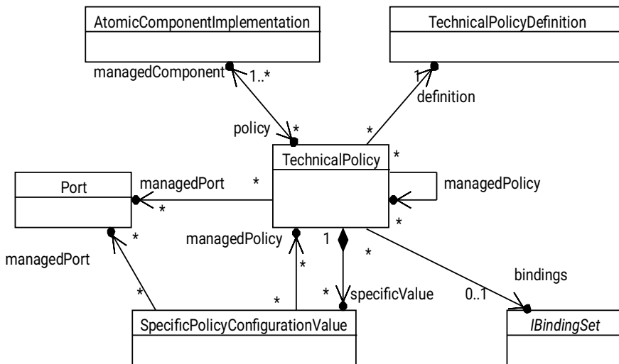
Figure 32: UCM atomic component implementations
