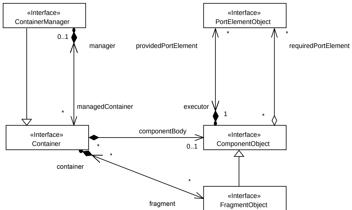
Figure 37: UCM Ccontainer Programming mModel
