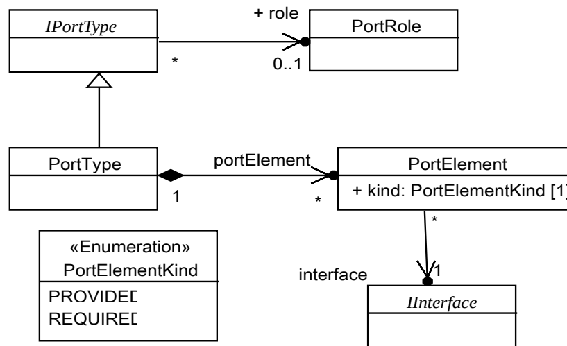
Figure 24: UCM port types
