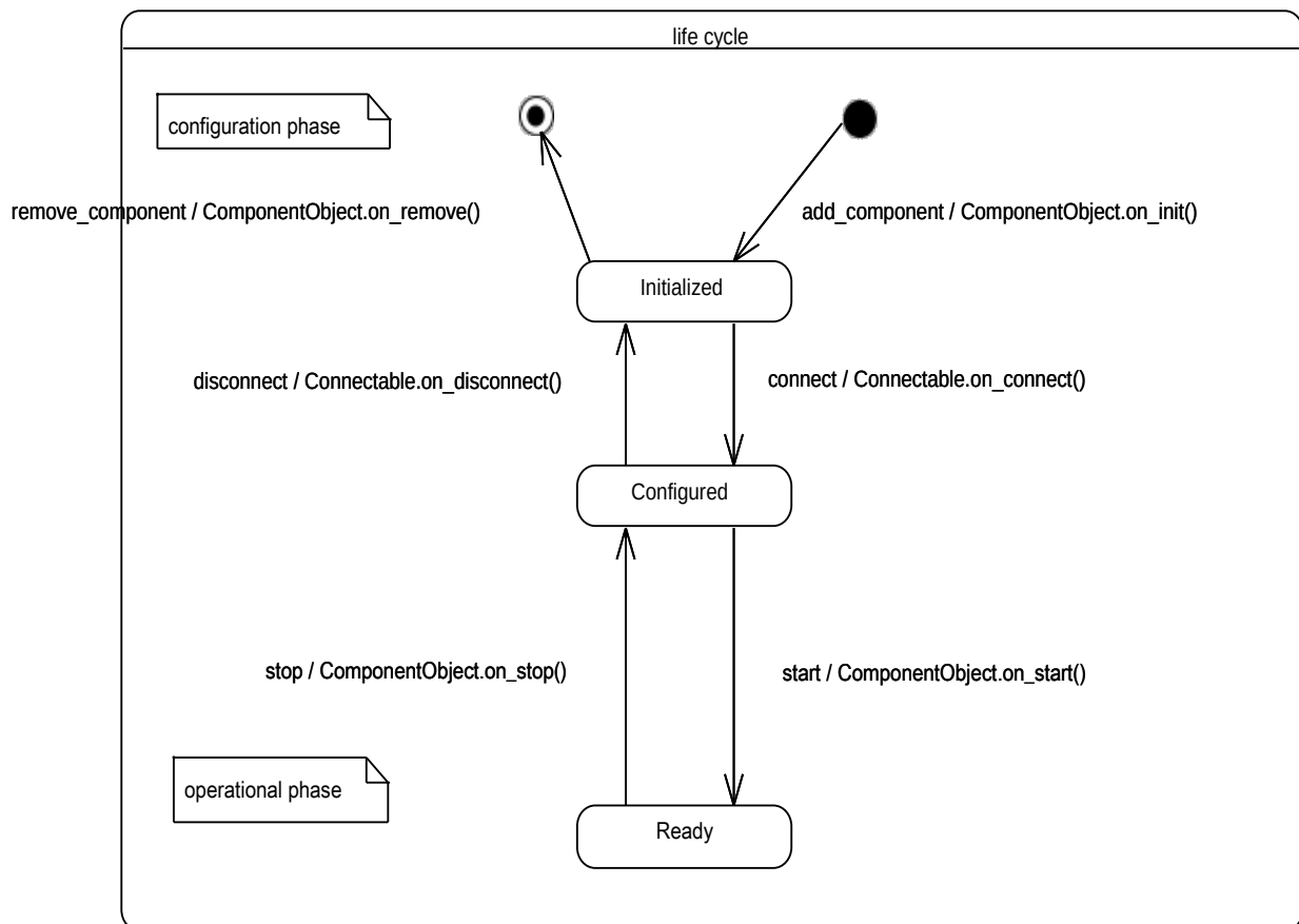
Figure 40: UCM cComponent Instance Life Cycle
