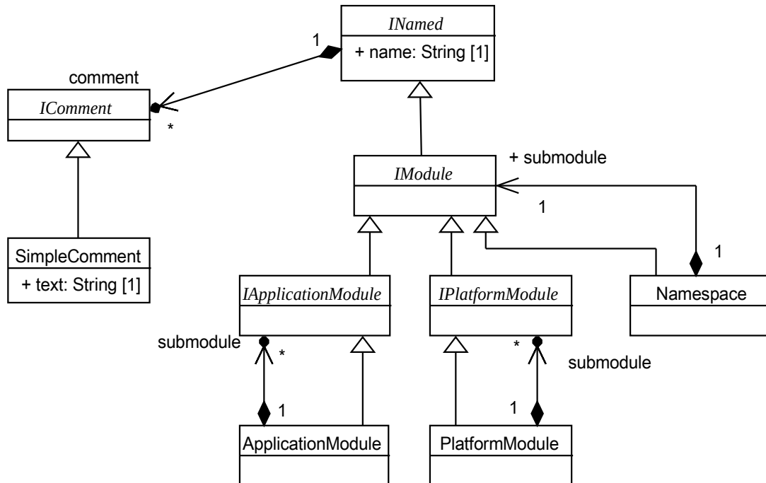
Figure 5: Base classes
