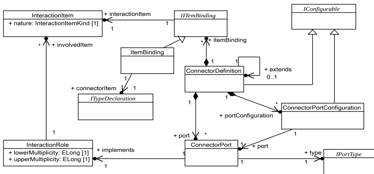
Figure 23: UCM connectors
