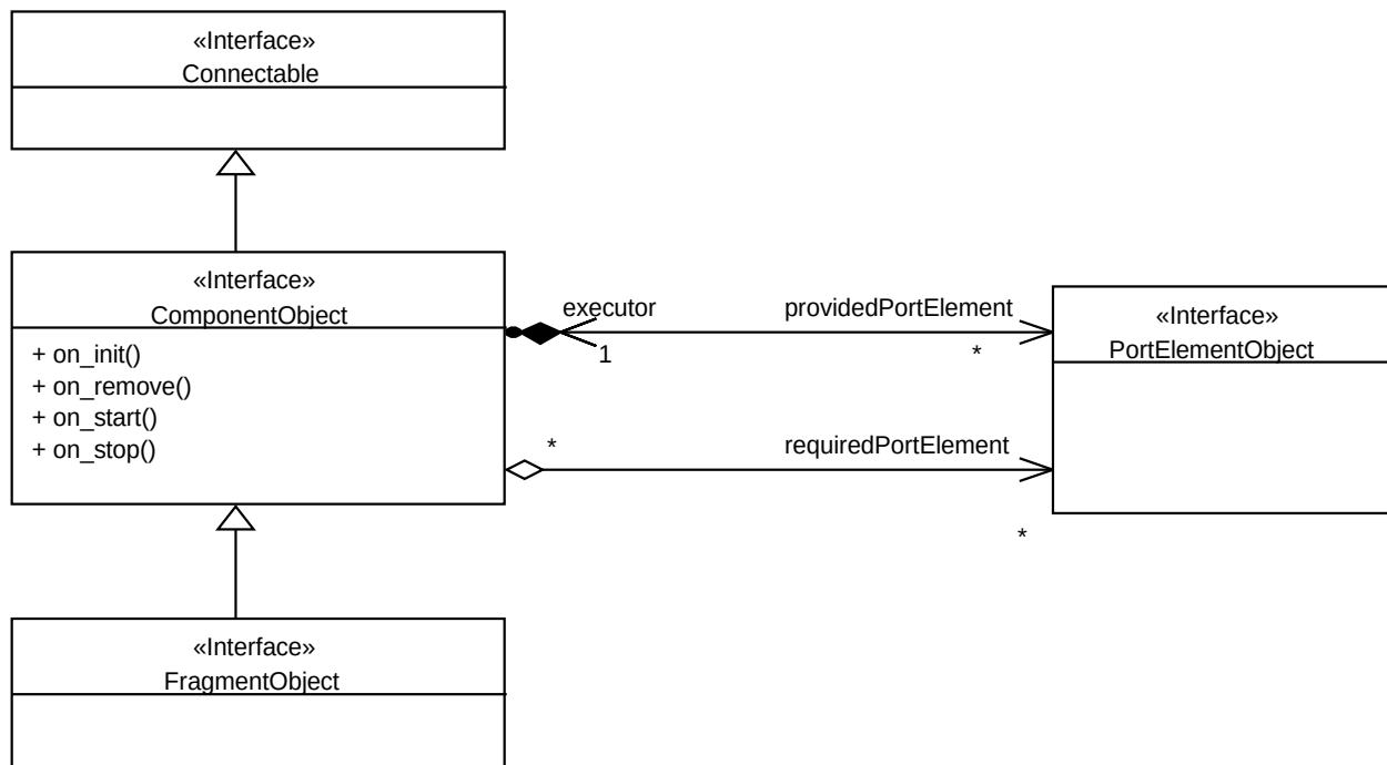
Figure 38: UCM cComponent objectBody iInterfaces
