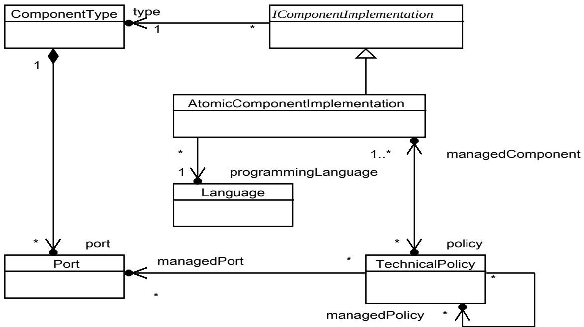
Figure 30: UCM atomic component implementations
