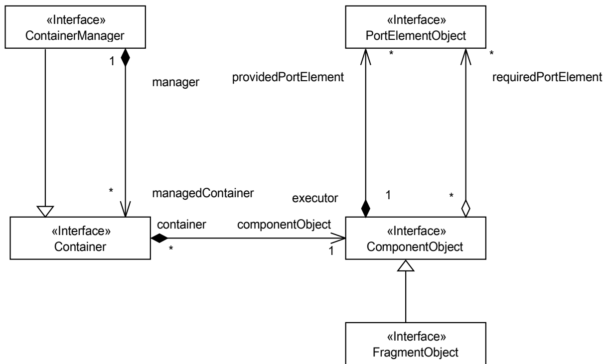
Figure 37: UCM Container Programming Model
