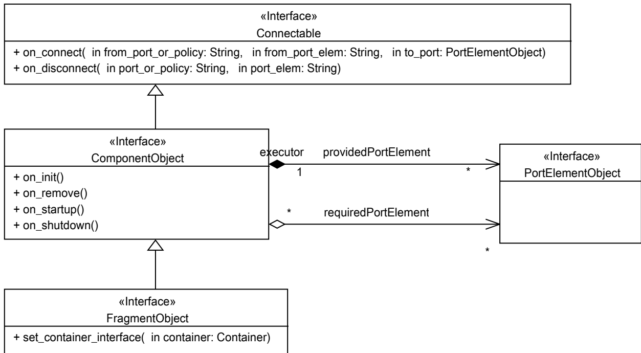
Figure 38: UCM Component Body Interfaces
