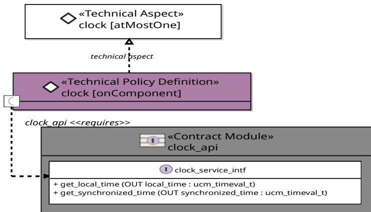
Figure 40: Standard clock service
