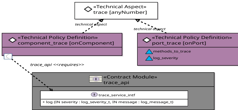
Figure 41: Standard trace service
