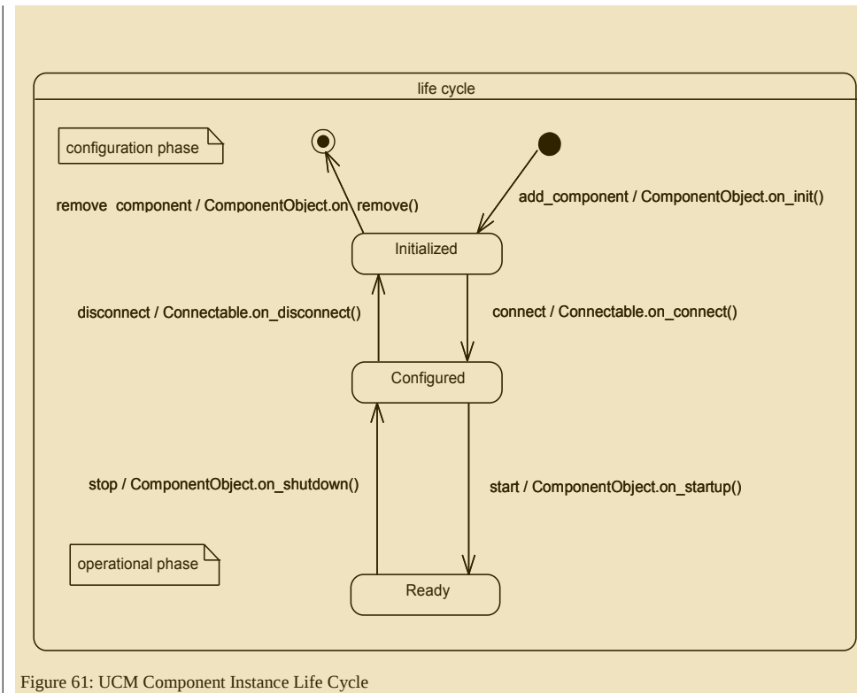
Figure 61: UCM Component Instance Life Cycle
