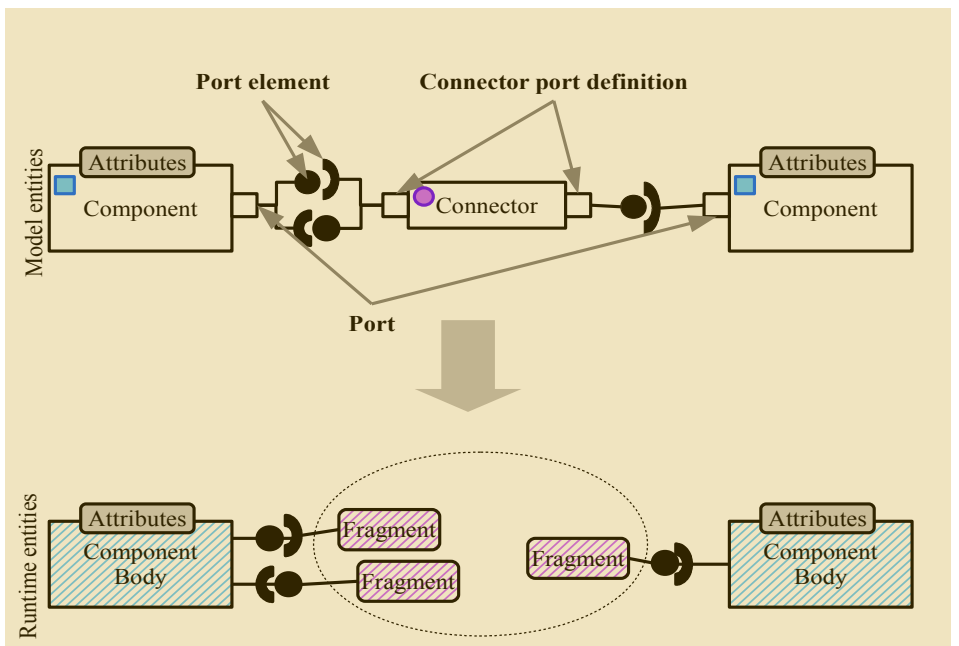
Figure 55: Connector fragmentation example
