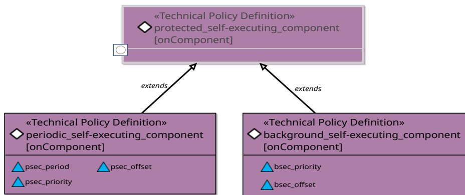
Figure 53: Extended technical policies for self-executing components
