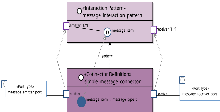
Figure 44: Message based interaction
