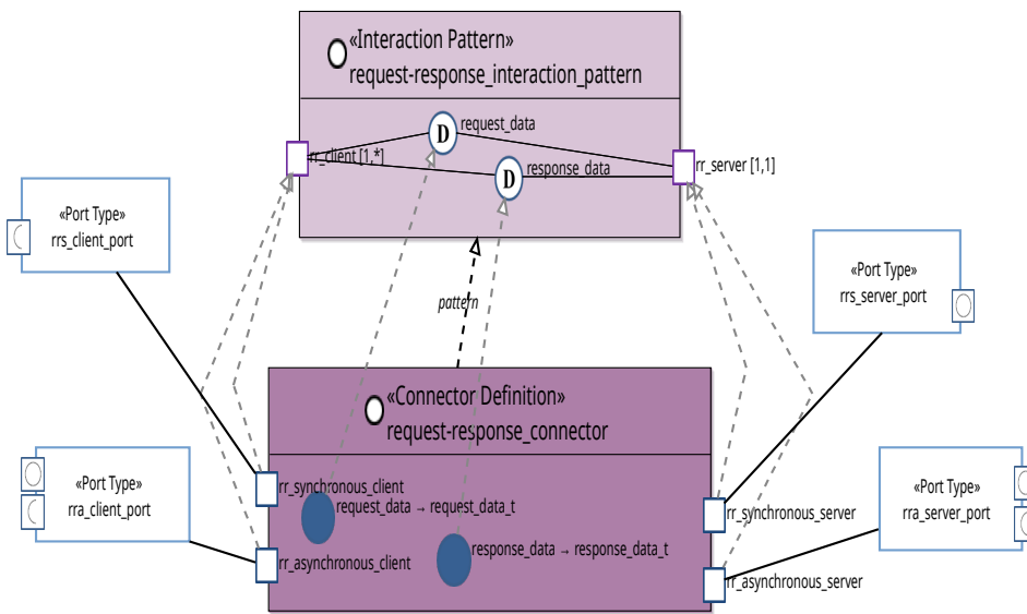
Figure 49: Request-response
