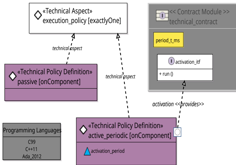
Figure 28: Example of technical policy definition
