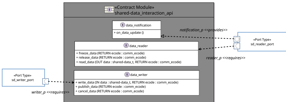
Figure 52: Port types for shared data interactions
