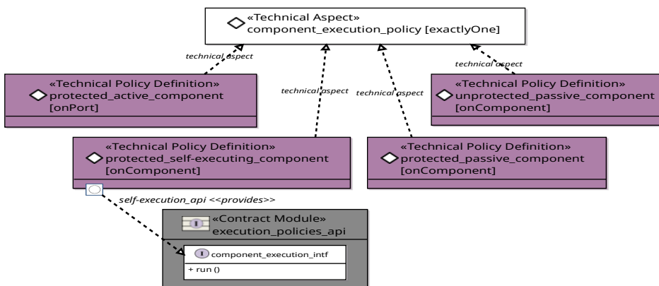
Figure 39: Standard component execution model
