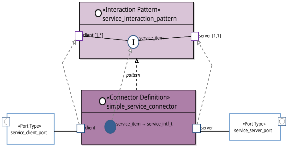
Figure 42: Service based interaction
