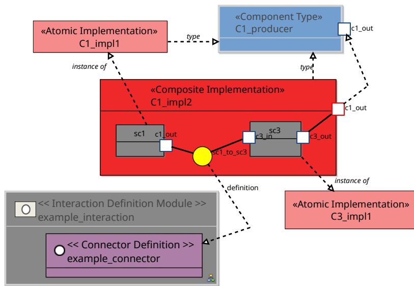
Figure 31: Example of composite component implementation
