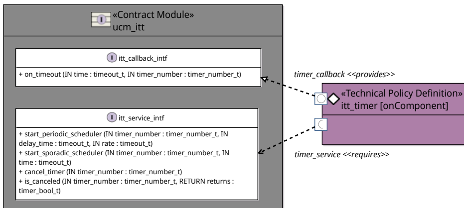
Figure 48: Technical policy for index-based programmable timers
