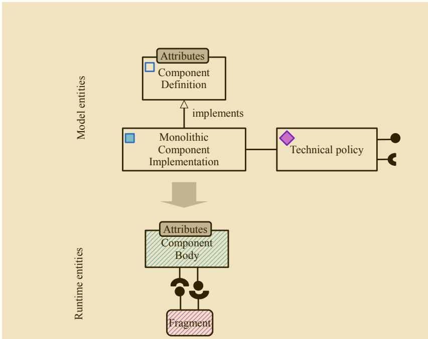
Figure 56: Technical policy fragmentation example
