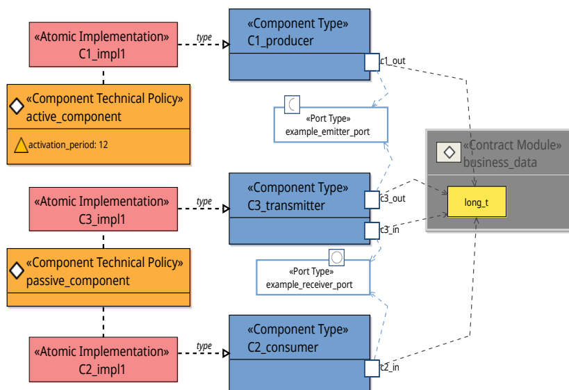
Figure 30: Example of component declarations
