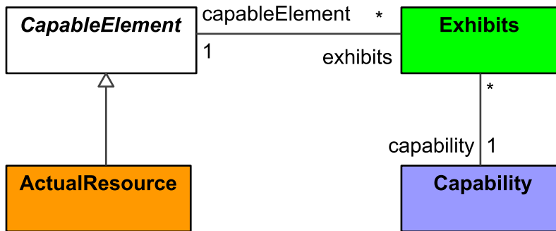
Figure 8:88 - Actual Resources Traceability
