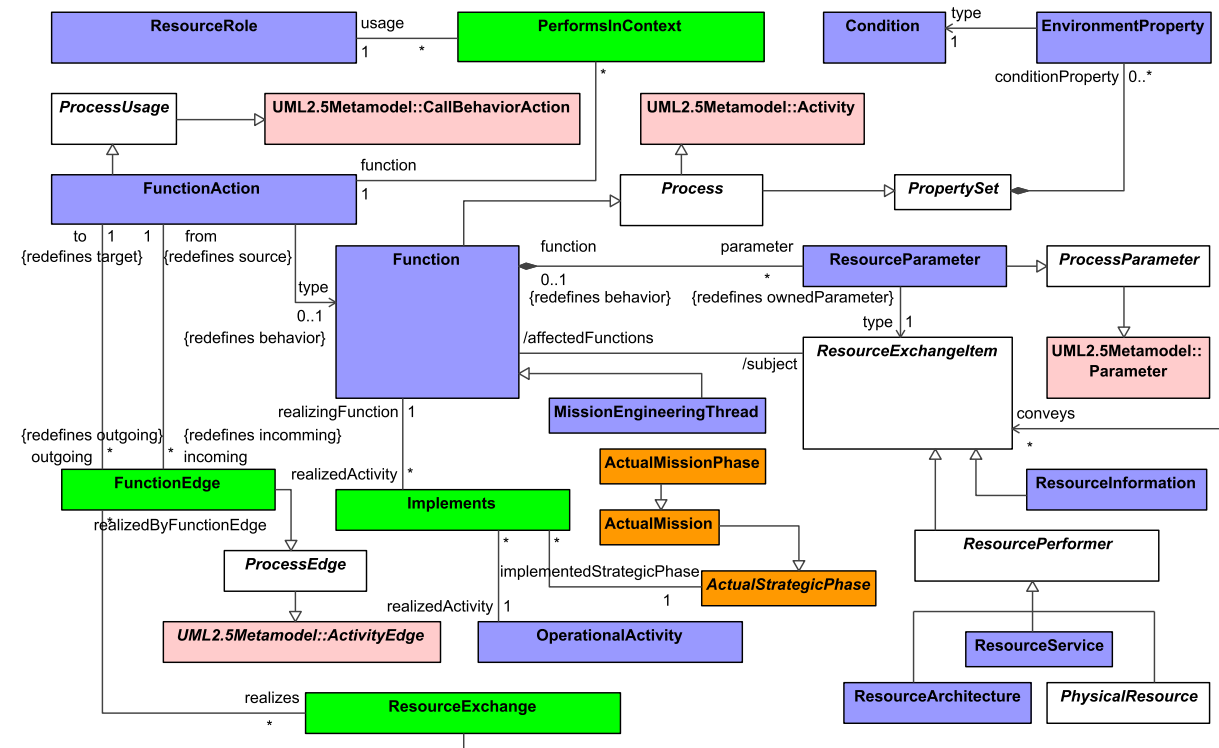
Figure 8:62 - Resources Processes: Mission Engineering Threads
