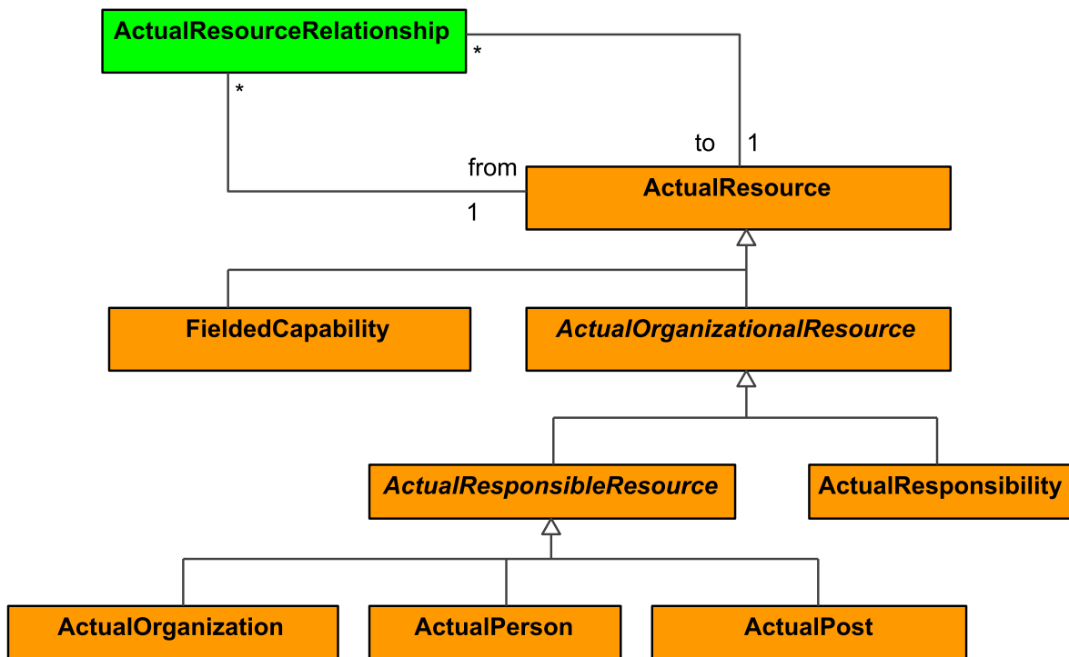
Figure 8:87 - Actual Resources Connectivity
