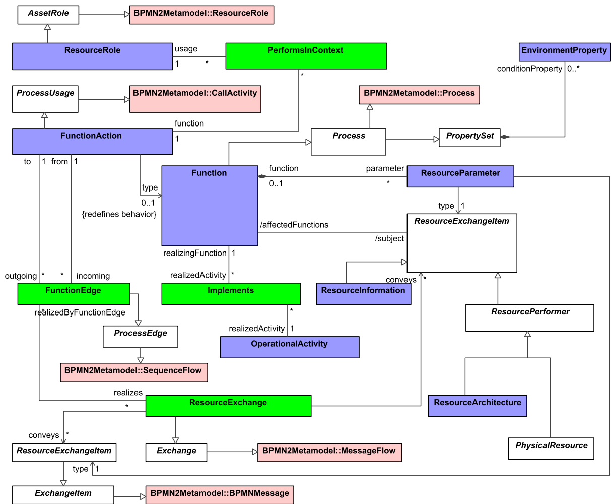
Figure 8:61 - Resources Processes BPMN Semantics
