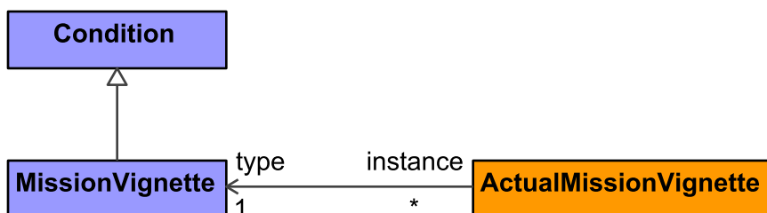
Figure 9:279 - MissionVignette
