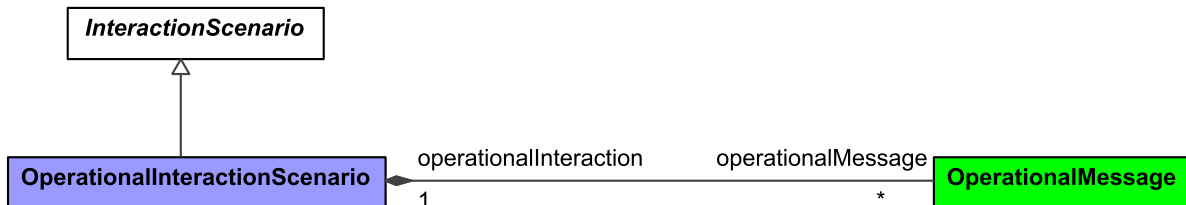
Figure 9:119 - OperationalInteractionScenario
