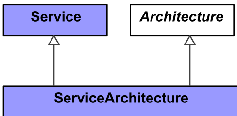
Figure 9:125 - ServiceArchitecture
