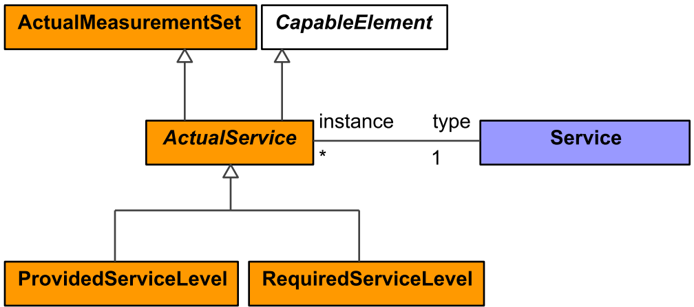
Figure 9:252 - ActualService
