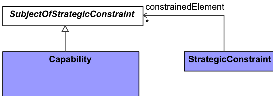
Figure 8:20 - Strategic Constraints
