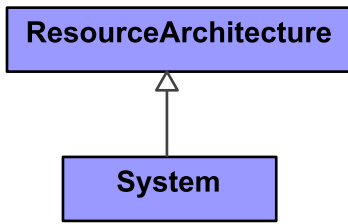
Figure 9:169 - System
