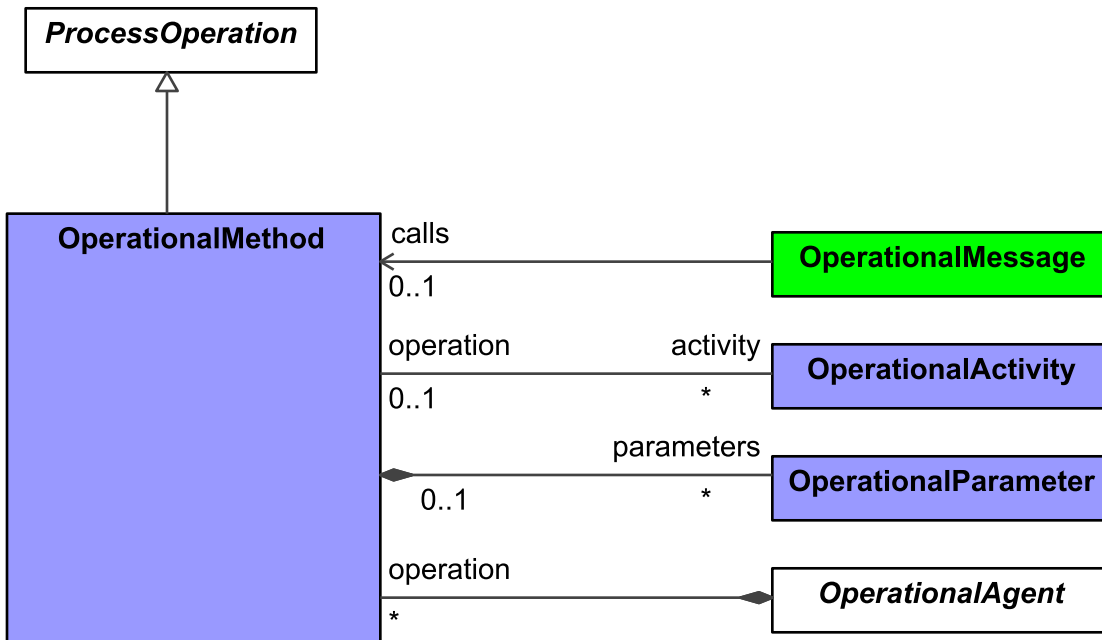
Figure 9:100 - OperationalMethod
