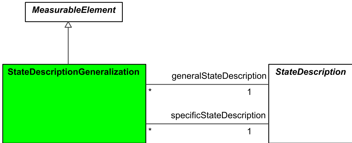
Figure 9:8 - StateDescriptionGeneralization
