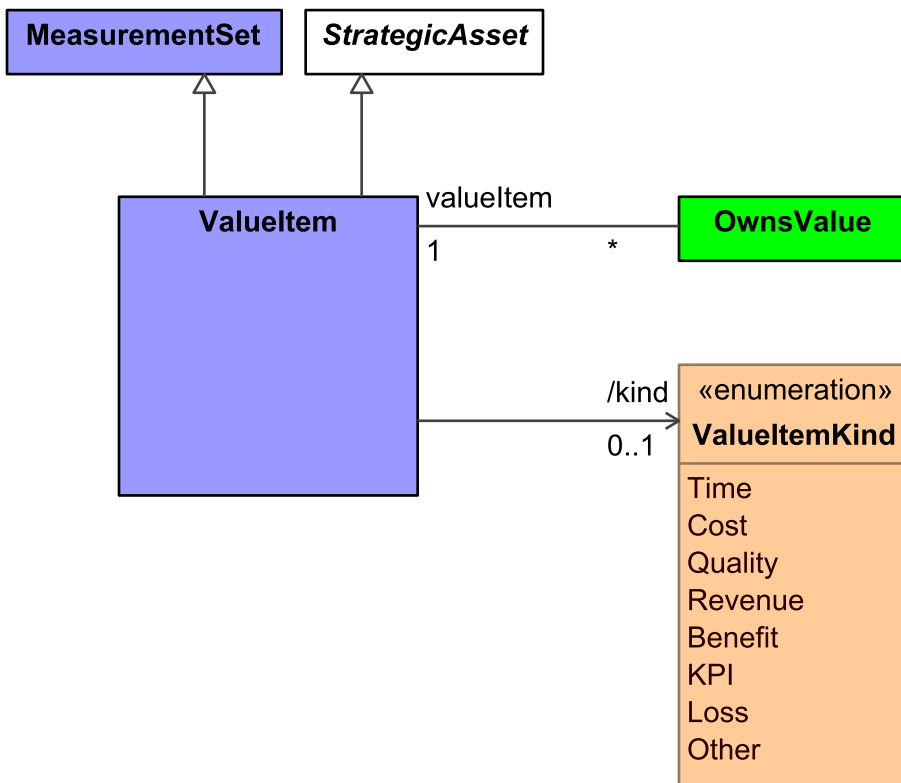
Figure 9:63 - ValueItem
