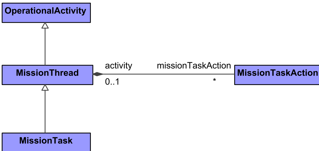
Figure 9:113 - MissionThread
