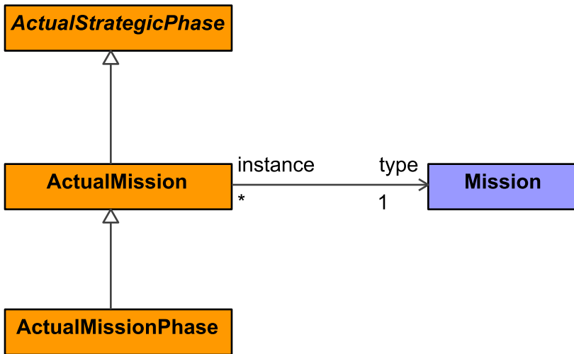
Figure 9:74 - ActualMission
