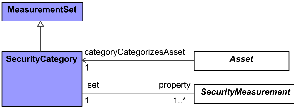
Figure 9:216 - SecurityCategory
