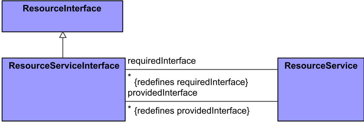
Figure 9:178 - ResourceServiceInterface
