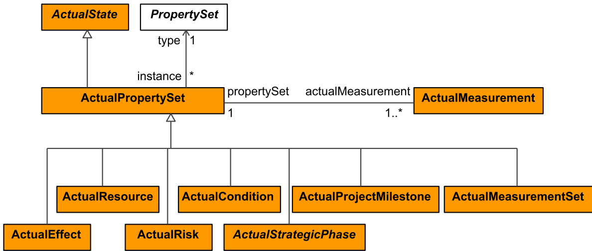
Figure 9:264 - ActualPropertySet
