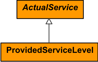
Figure 9:253 - ProvidedServiceLevel
