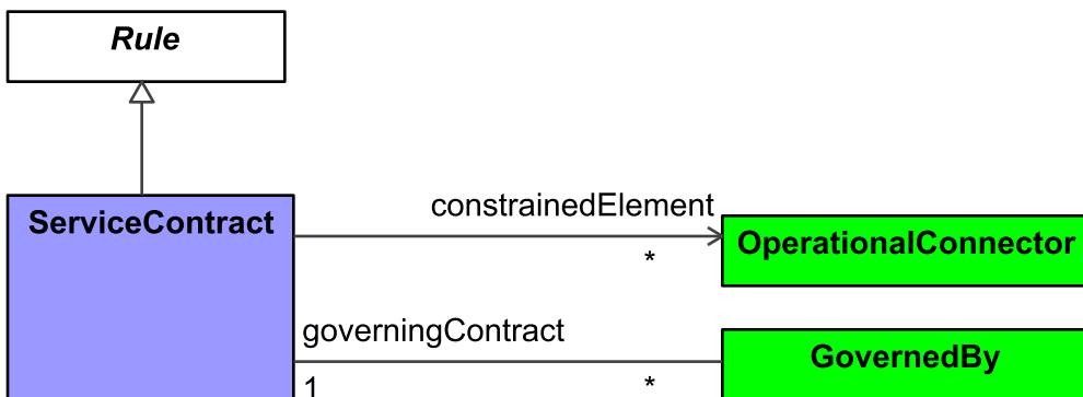
Figure 9:142 - ServiceContract
