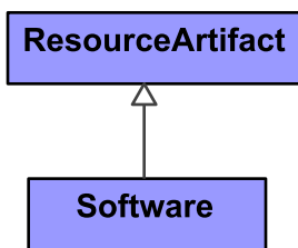
Figure 9:168 - Software
