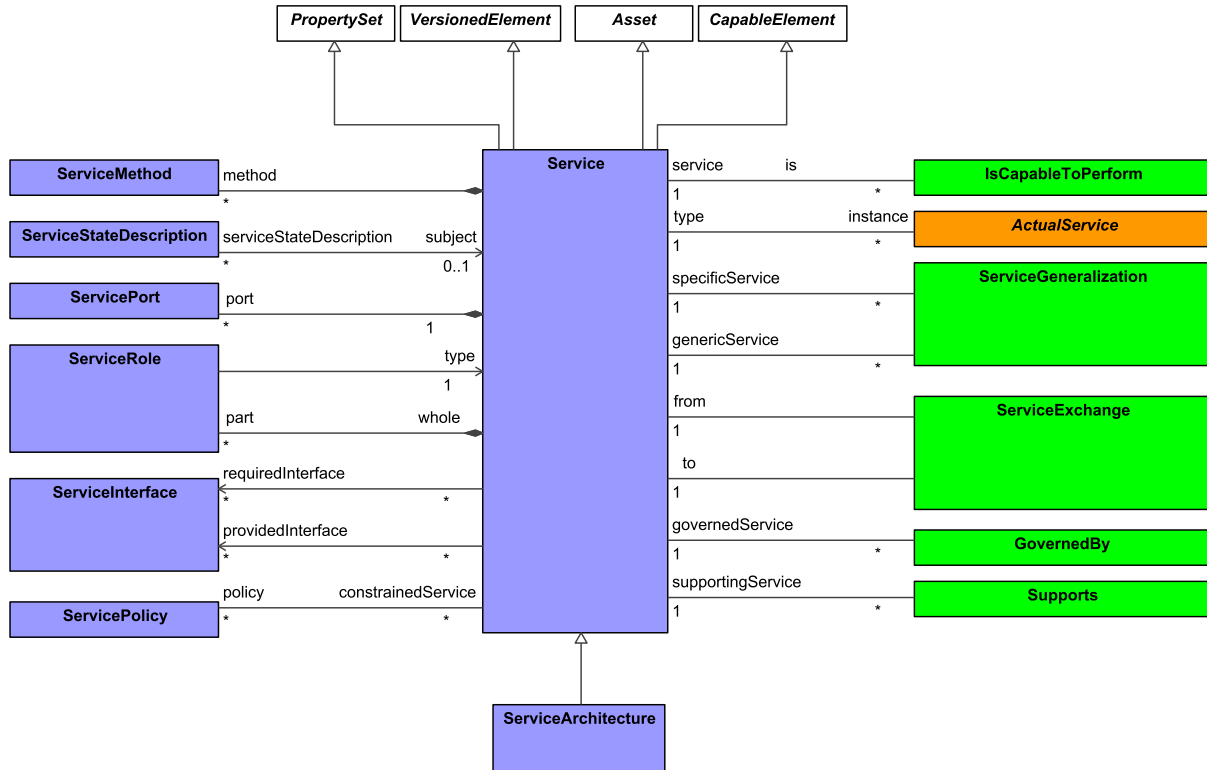
Figure 9:124 - Service
