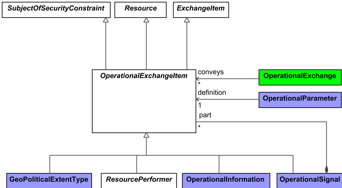
Figure 9:107 - OperationalExchangeItem
