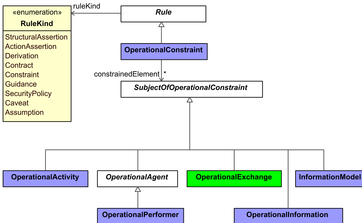
Figure 8:32 - Operational Constraints
