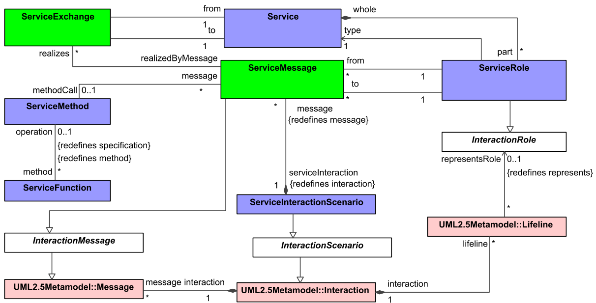
Figure 8:40 - Services Sequences
