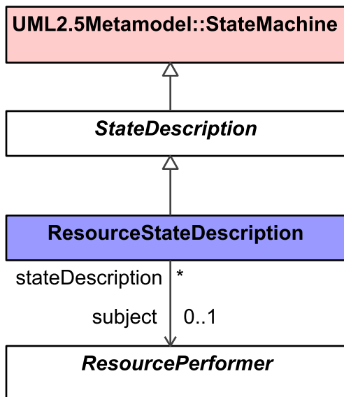
Figure 8:63 - Resources States
