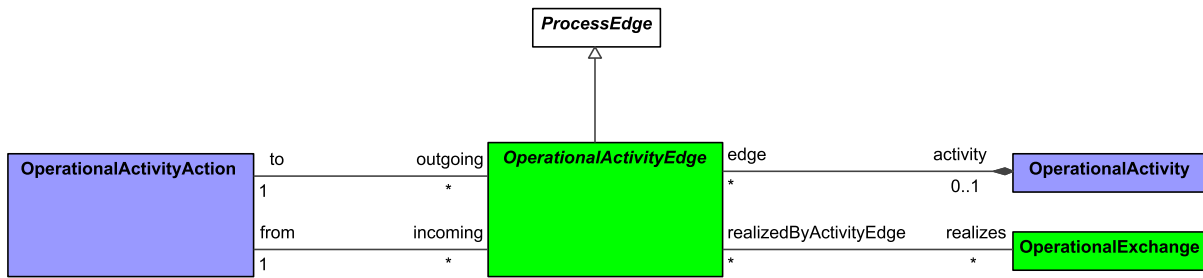
Figure 9:116 - OperationalActivityEdge
