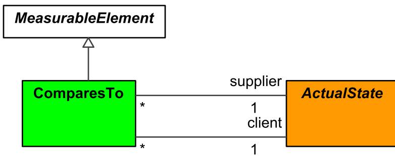
Figure 9:34 - ComparesTo
