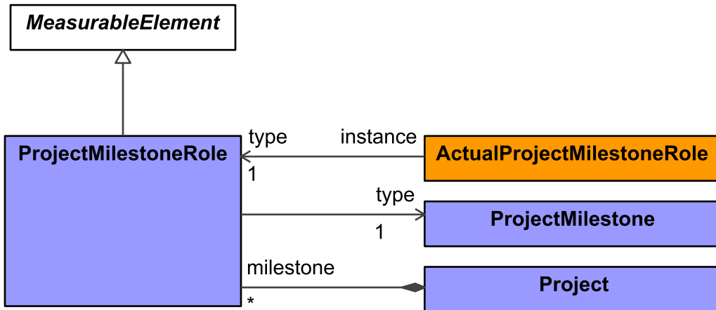
Figure 9:227 - ProjectMilestoneRole
