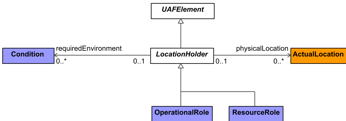
Figure 9:274 - LocationHolder
