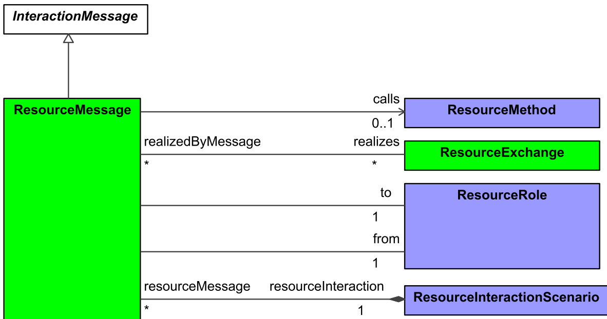
Figure 9:185 - ResourceMessage
