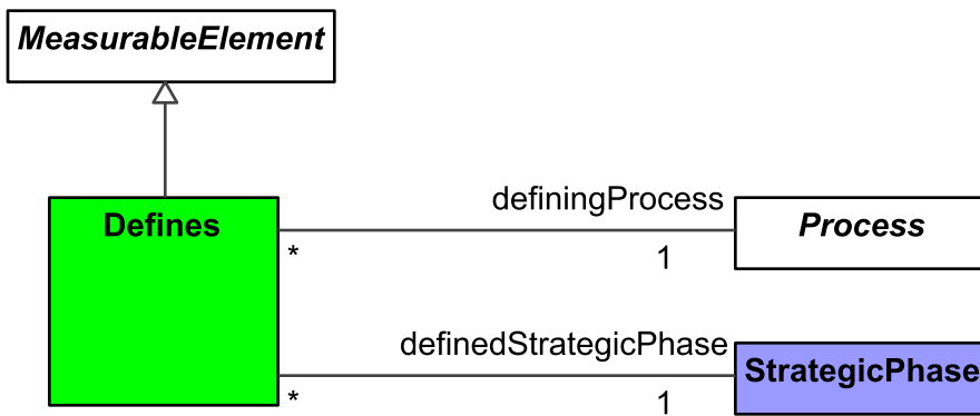
Figure 9:78 - Defines
