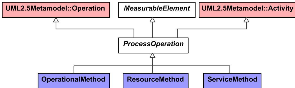
Figure 9:17 - ProcessOperation
