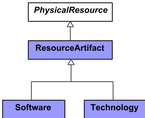
Figure 9:165 - ResourceArtifact
