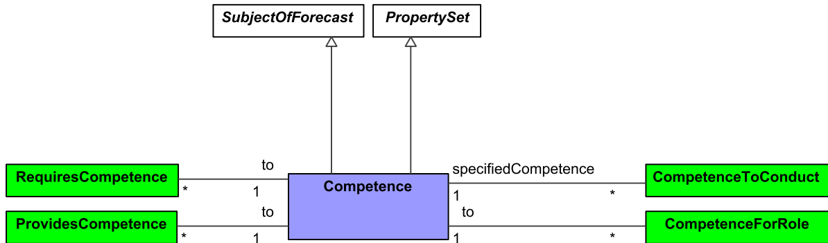
Figure 9:156 - Competence
