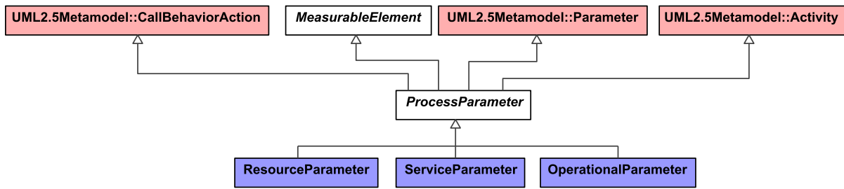
Figure 9:18 - ProcessParameter
