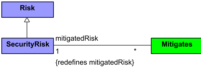
Figure 9:222 - SecurityRisk
