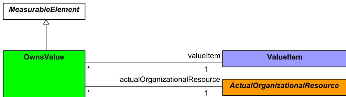
Figure 9:59 - OwnsValue
