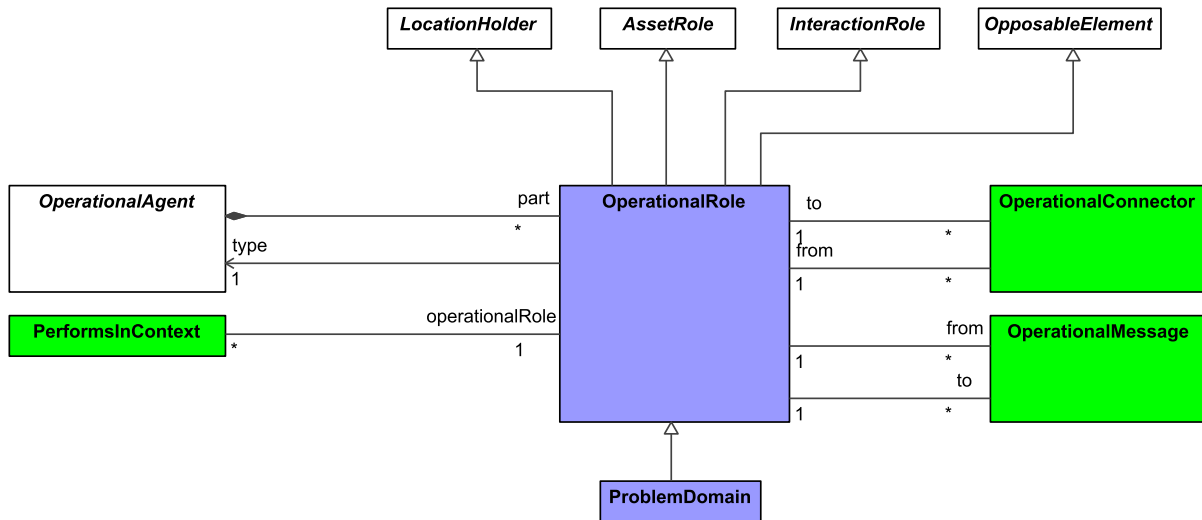
Figure 9:103 - OperationalRole
