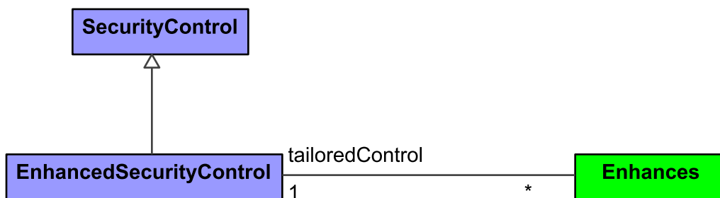
Figure 9:197 - EnhancedSecurityControl
