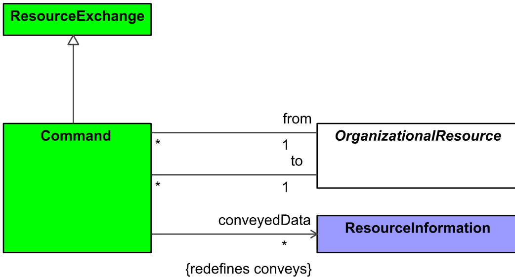
Figure 9:153 - Command
