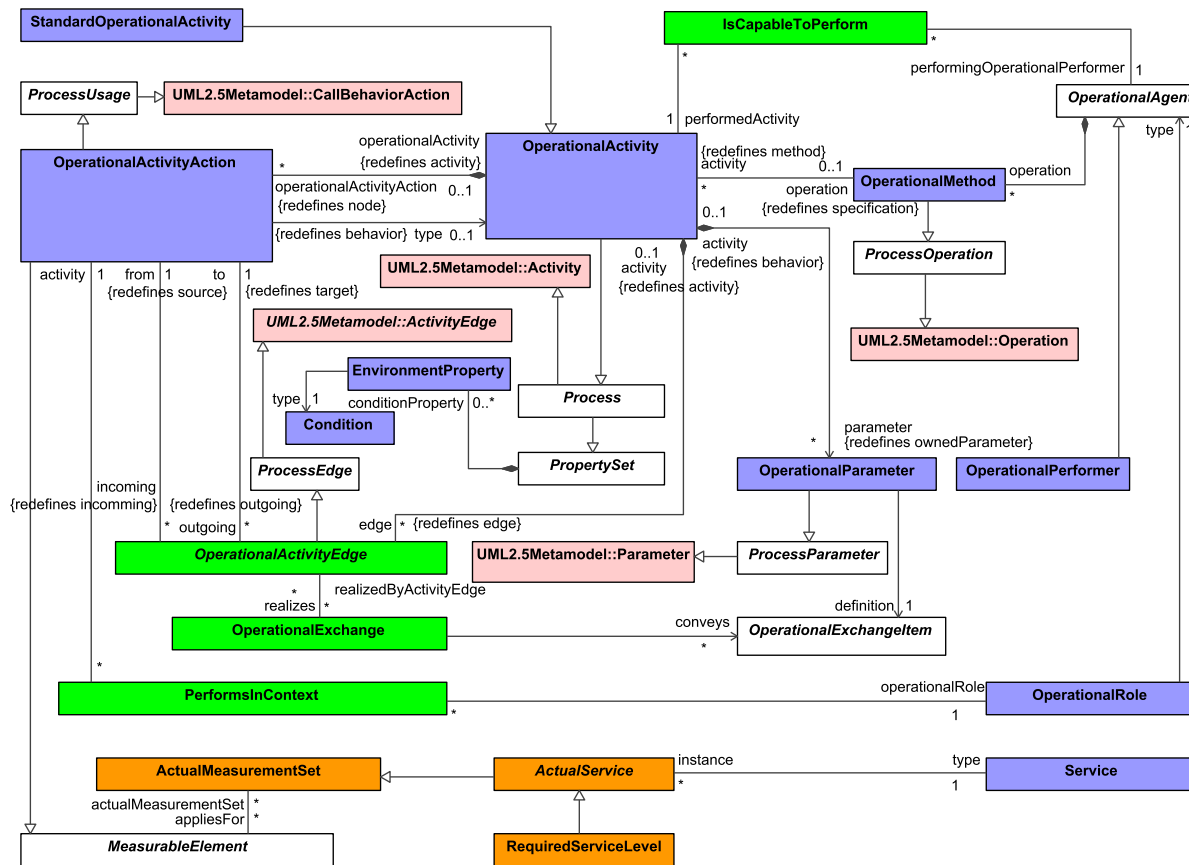
Figure 8:27 - Operational Processes
