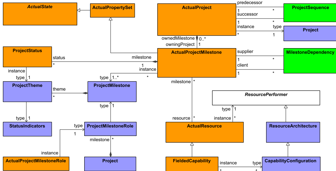
Figure 8:80 - Project Roadmap
