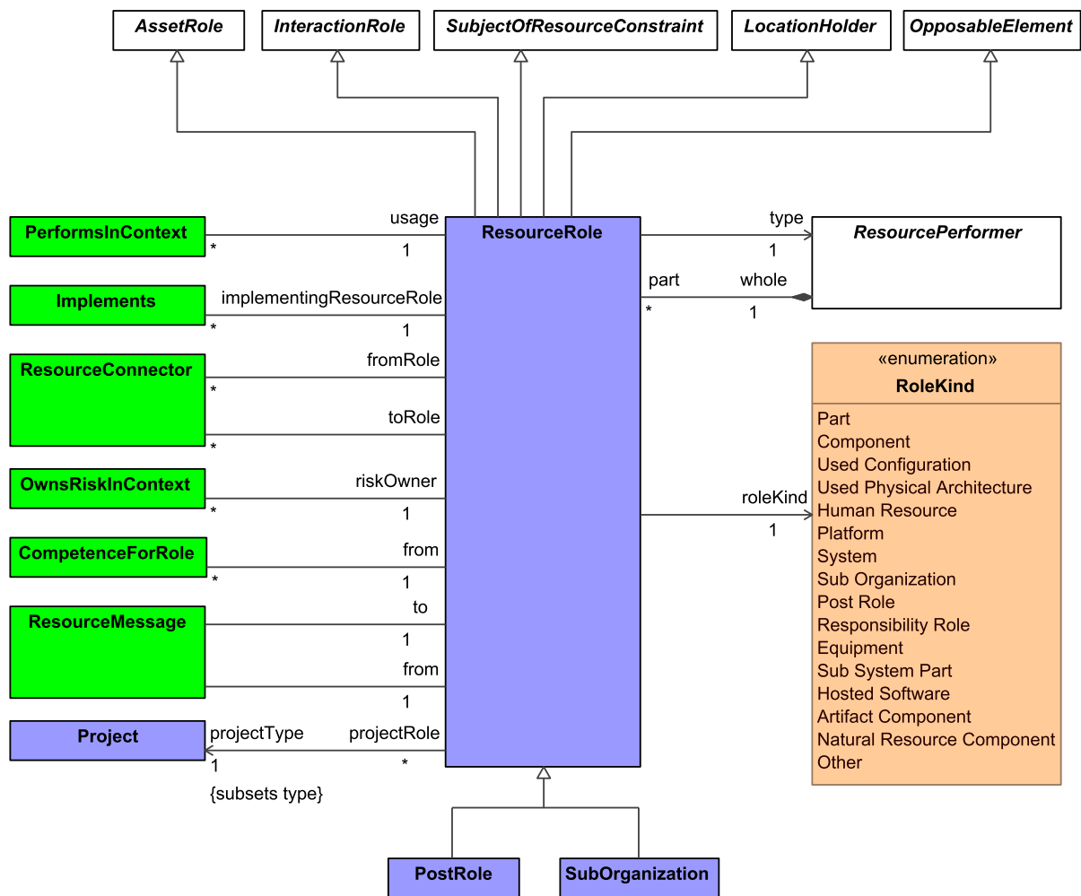
Figure 9:173 - ResourceRole
