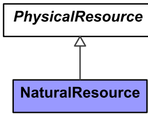
Figure 9:162 - NaturalResource
