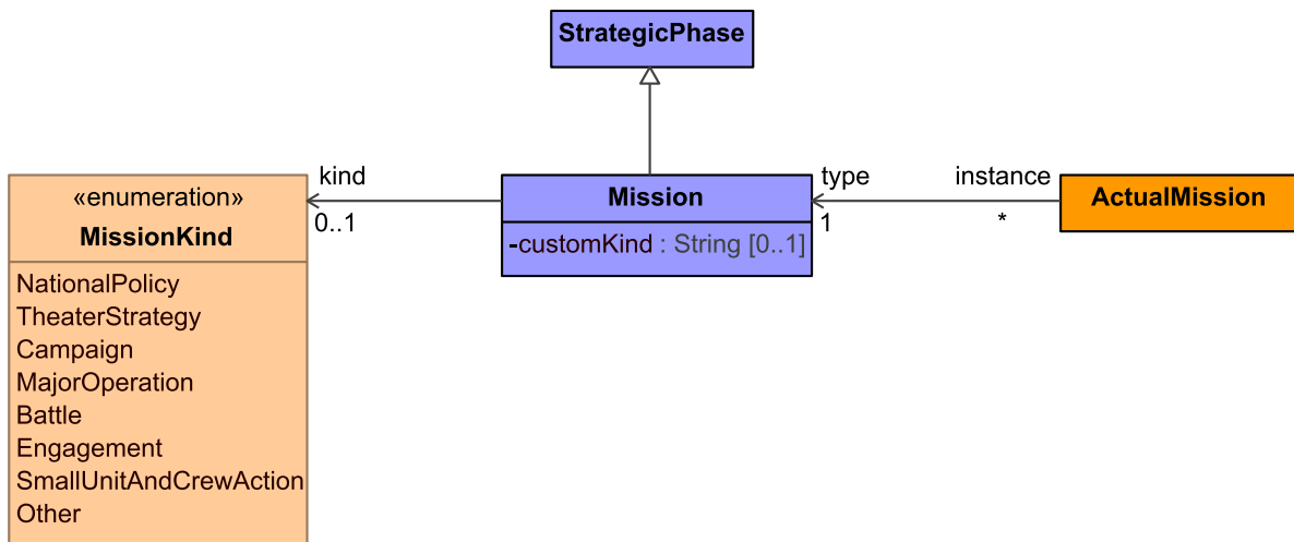
Figure 9:58 - Mission
