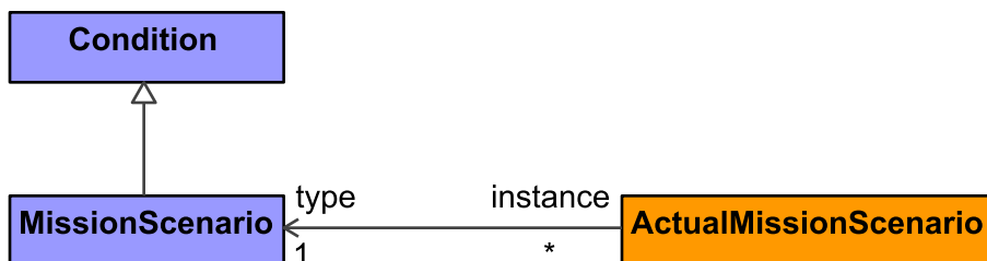
Figure 9:278 - MissionScenario
