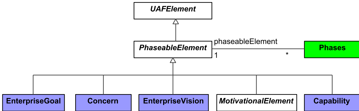
Figure 9:60 - PhaseableElement
