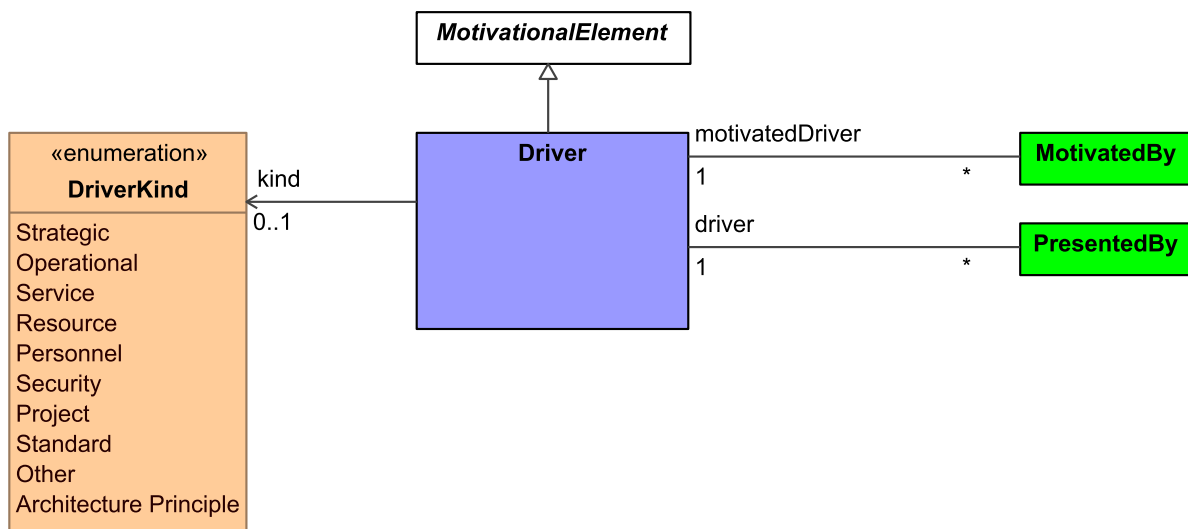
Figure 9:46 - Driver
