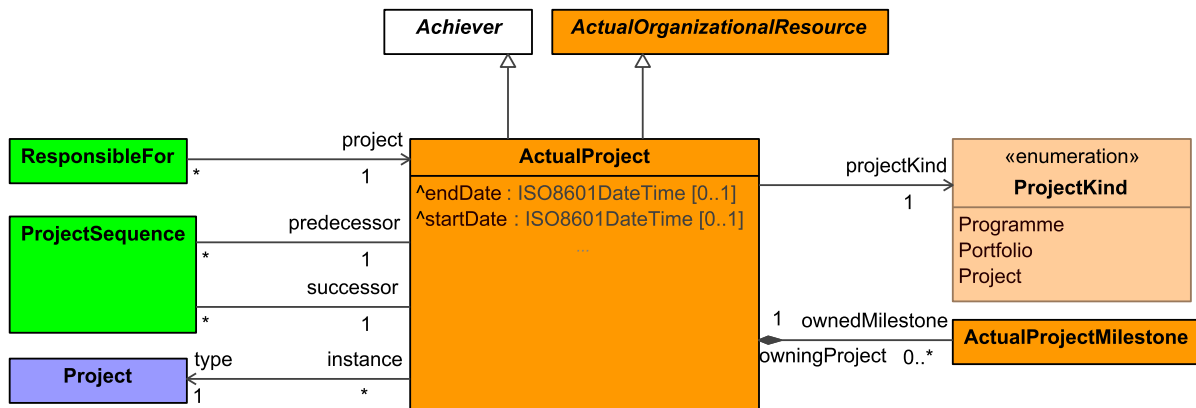
Figure 9:235 - ActualProject
