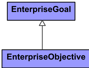
Figure 9:56 - EnterpriseObjective
