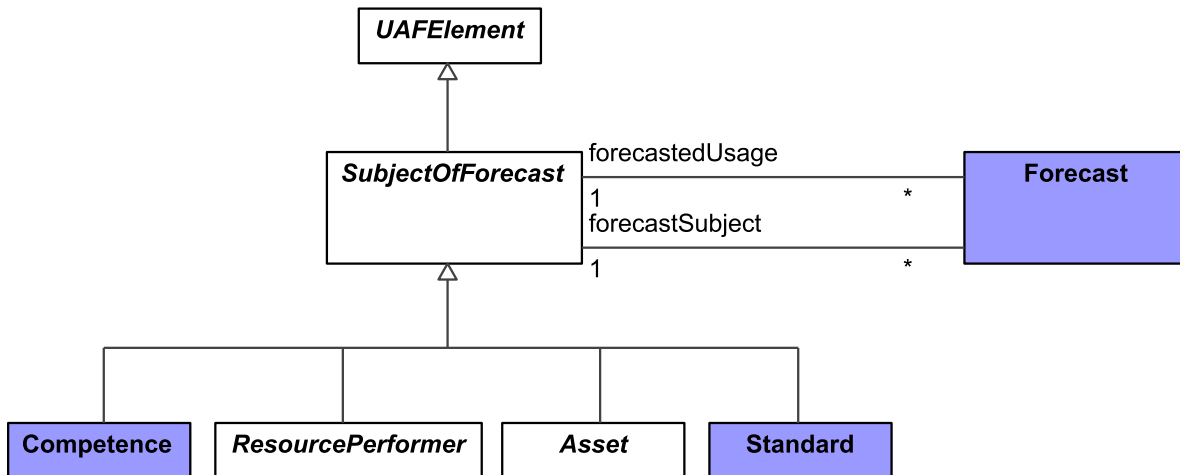
Figure 9:190 - SubjectOfForecast
