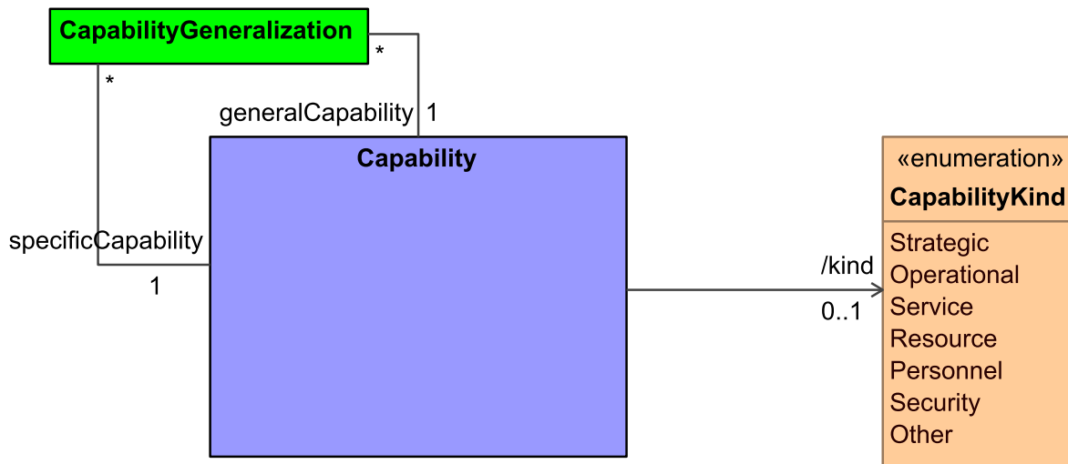
Figure 8:13 - Strategic Taxonomy
