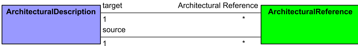
Figure 8:3 - Architecture References
