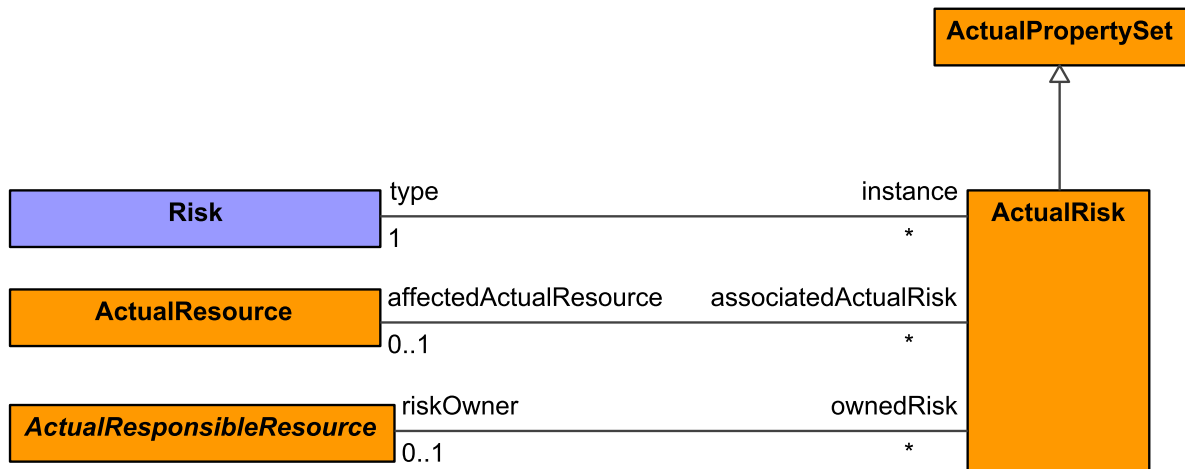
Figure 9:265 - ActualRisk
