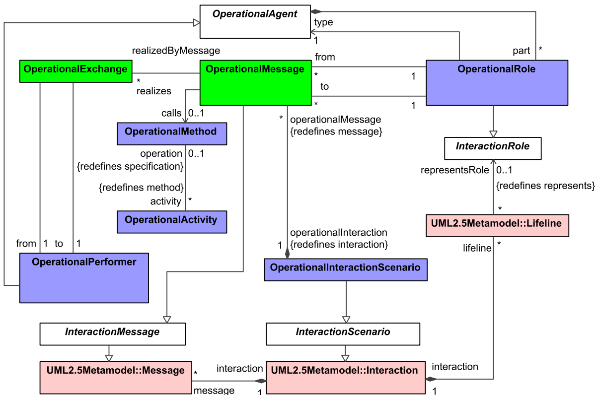
Figure 8:31 - Operational Sequences
