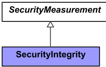
Figure 9:220 - SecurityIntegrity
