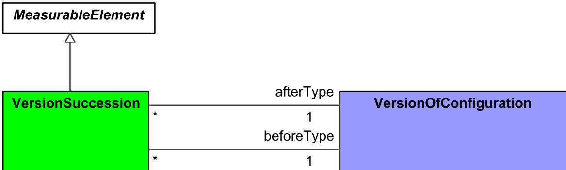
Figure 9:194 - VersionSuccession
