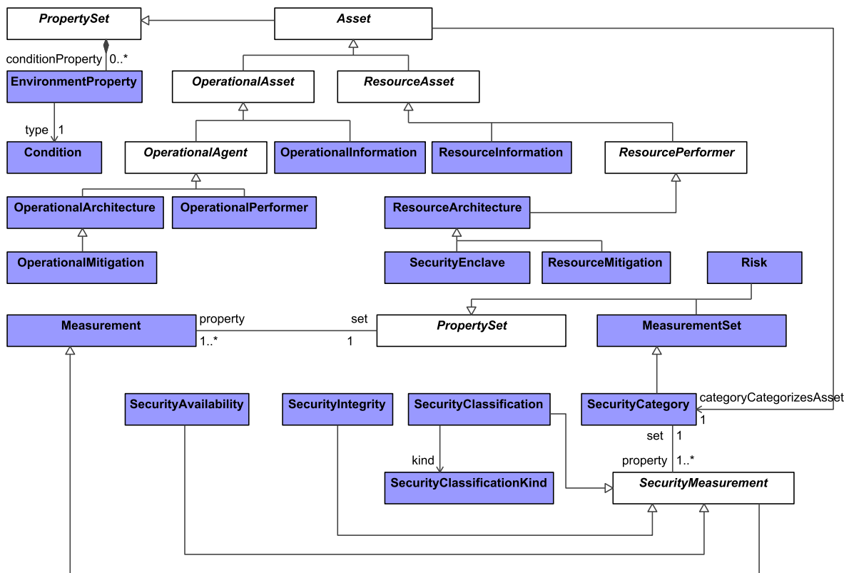
Figure 8:70 - Security Taxonomy
