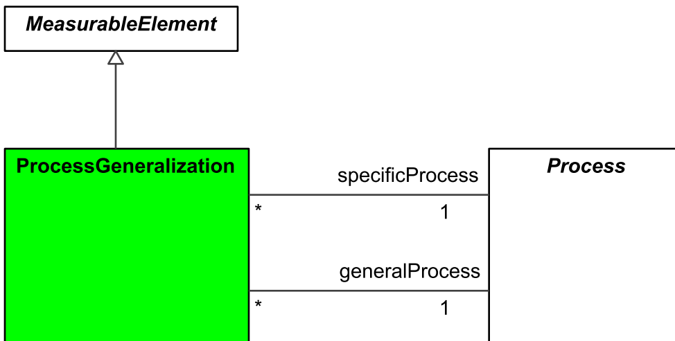
Figure 9:6 - ProcessGeneralization
