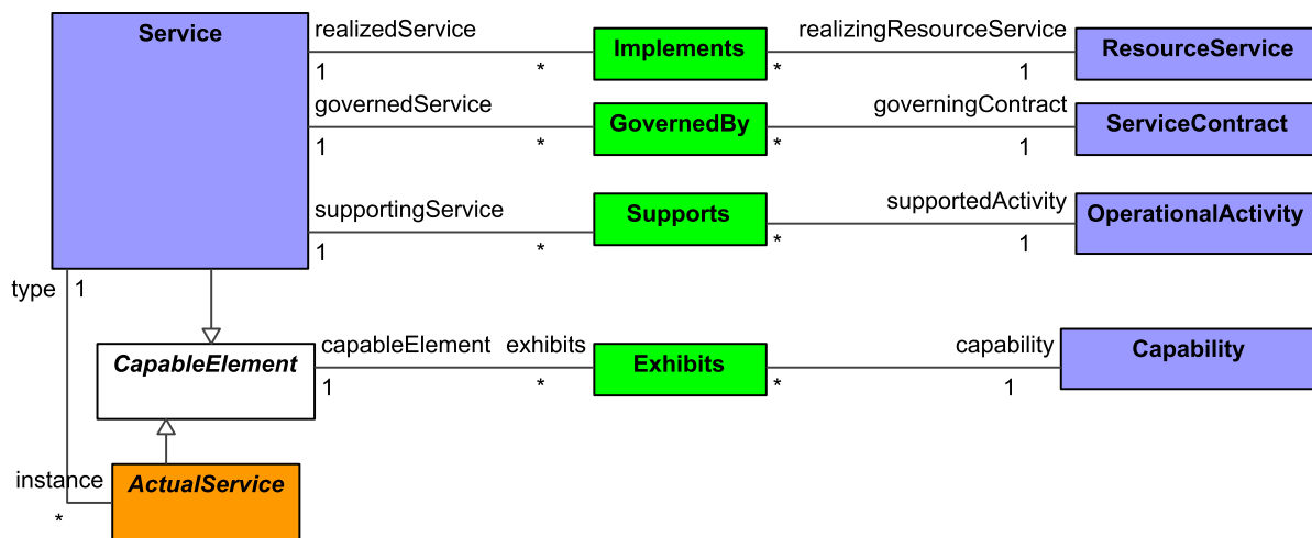
Figure 8:43 - Services Traceability
