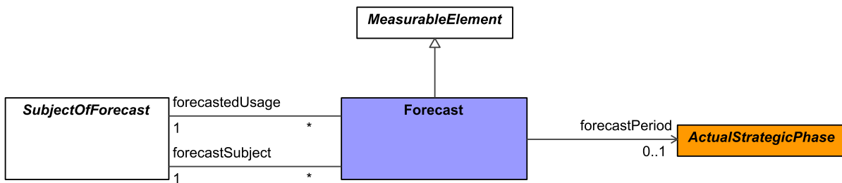
Figure 9:189 - Forecast
