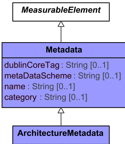
Figure 9:29 - Metadata
