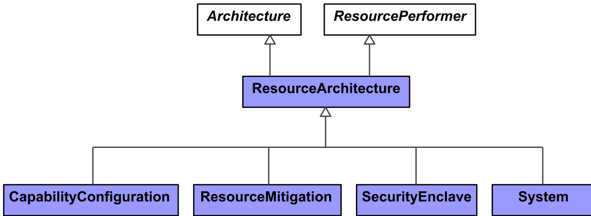
Figure 9:164 - ResourceArchitecture
