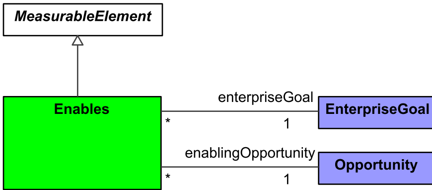
Figure 9:47 - Enables
