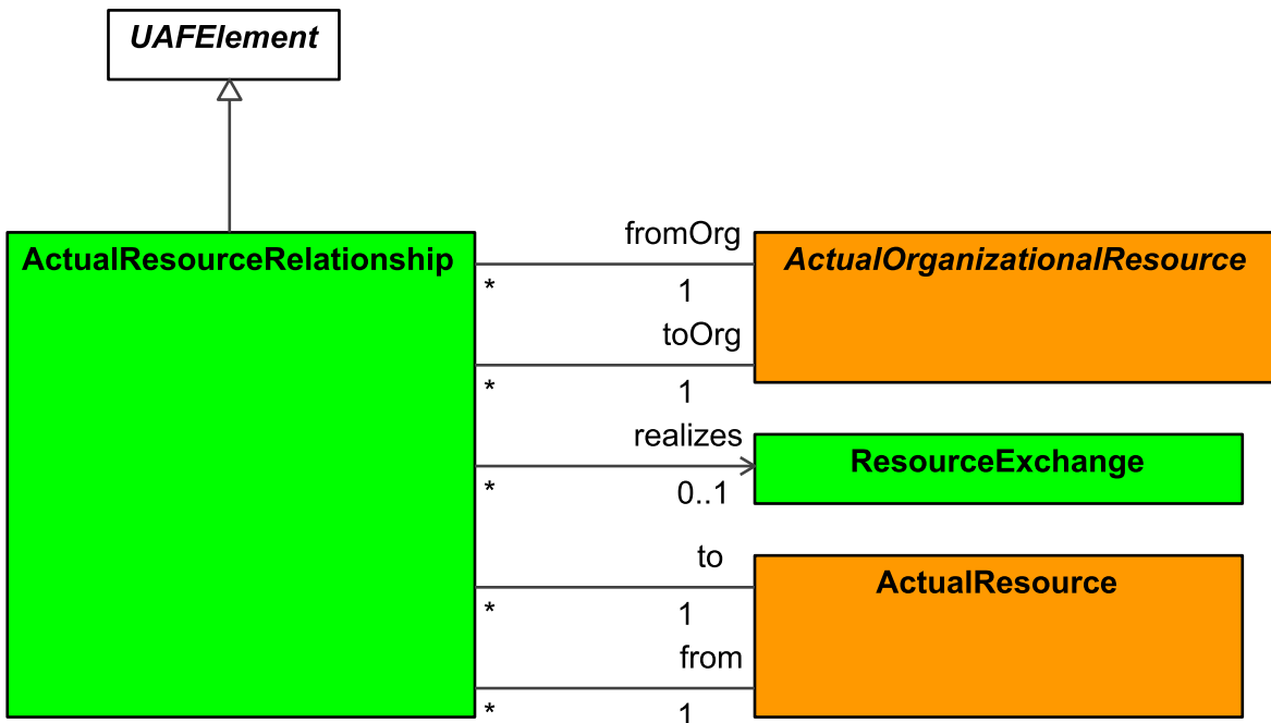
Figure 9:248 - ActualResourceRelationship
