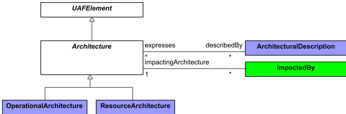
Figure 9:38 - Architecture
