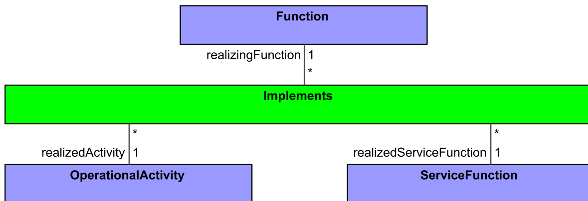
Figure 8:56 - Personnel Traceability
