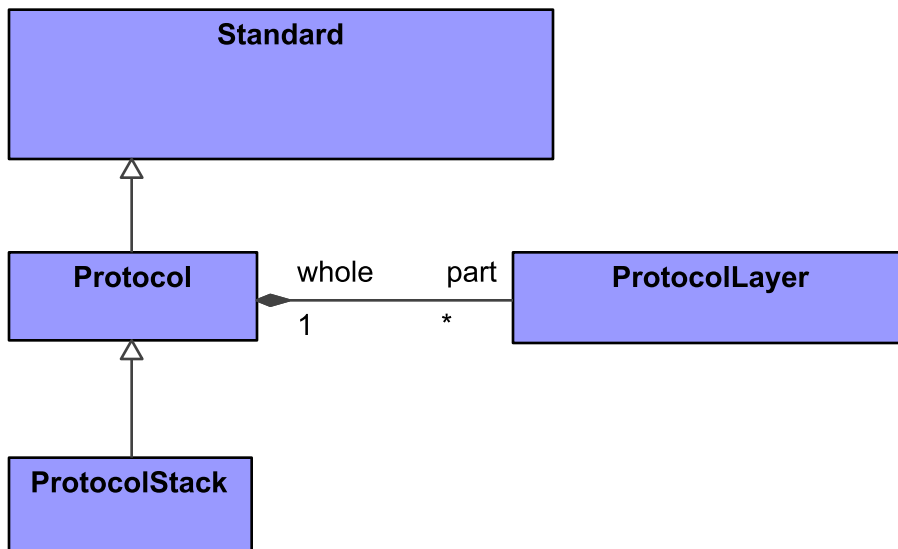
Figure 8:83 - Standards Structure
