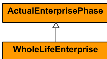
Figure 9:65 - WholeLifeEnterprise
