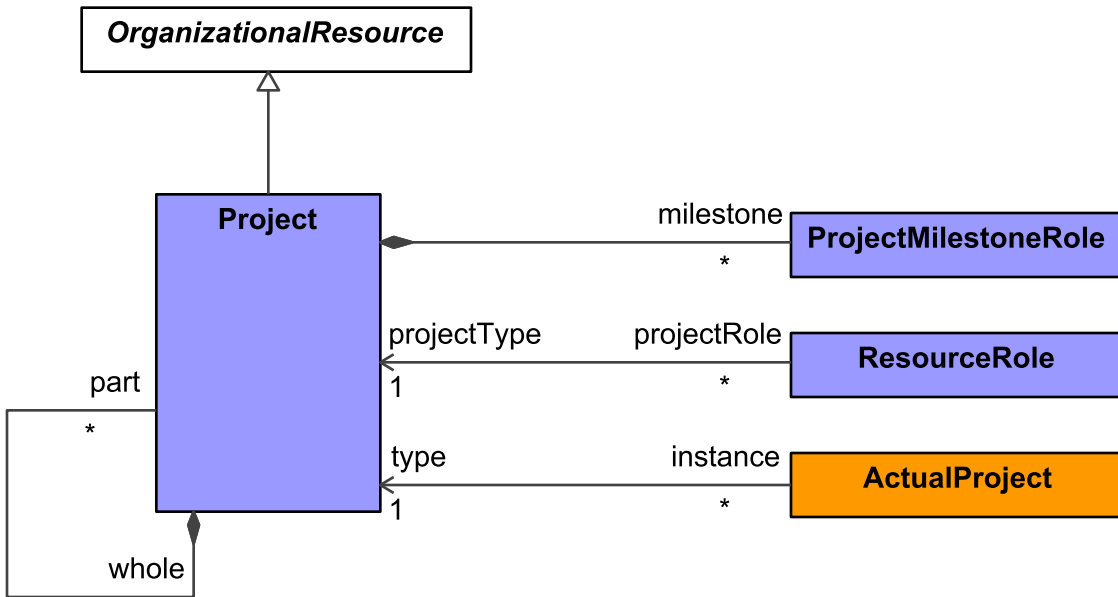
Figure 9:224 - Project
