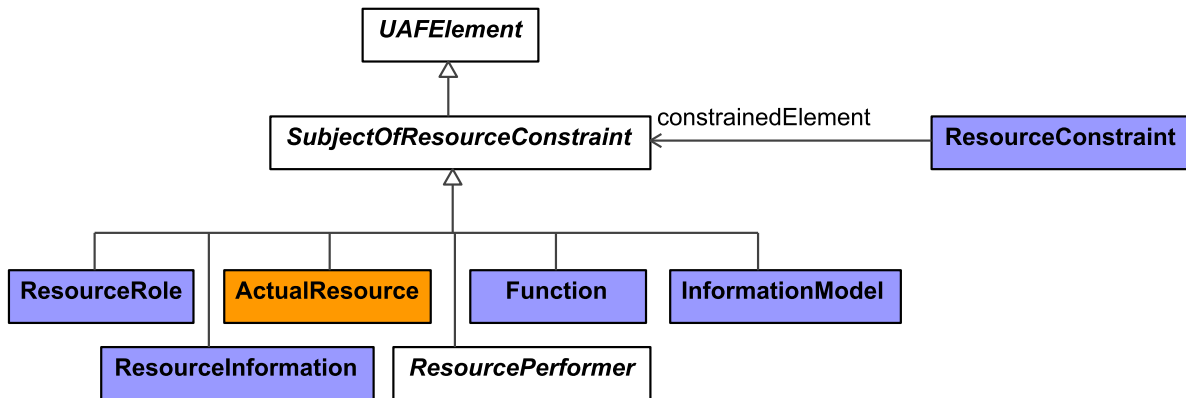
Figure 9:188 - SubjectOfResourceConstraint
