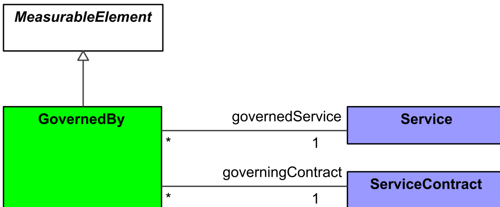
Figure 9:144 - GovernedBy
