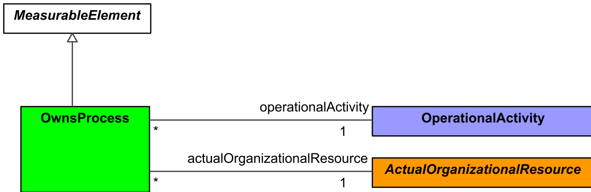
Figure 9:256 - OwnsProcess
