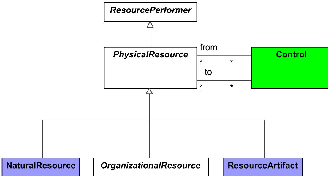
Figure 9:163 - PhysicalResource
