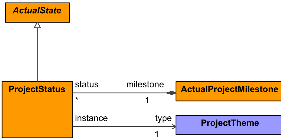
Figure 9:228 - ProjectStatus
