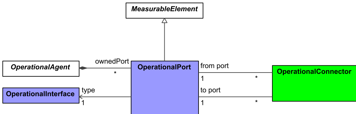
Figure 9:109 - OperationalPort
