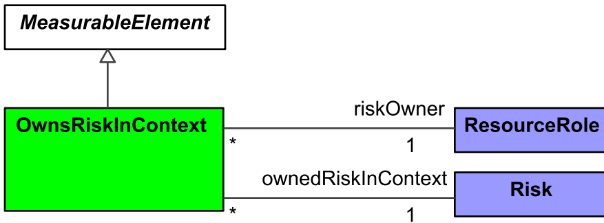
Figure 9:282 - OwnsRiskInContext
