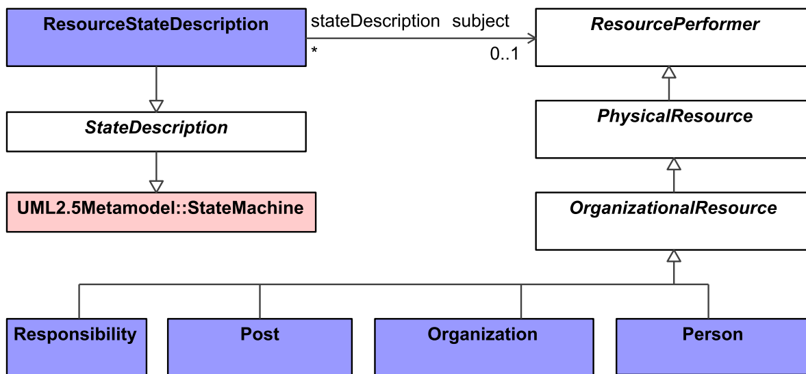
Figure 8:48 - Personnel States
