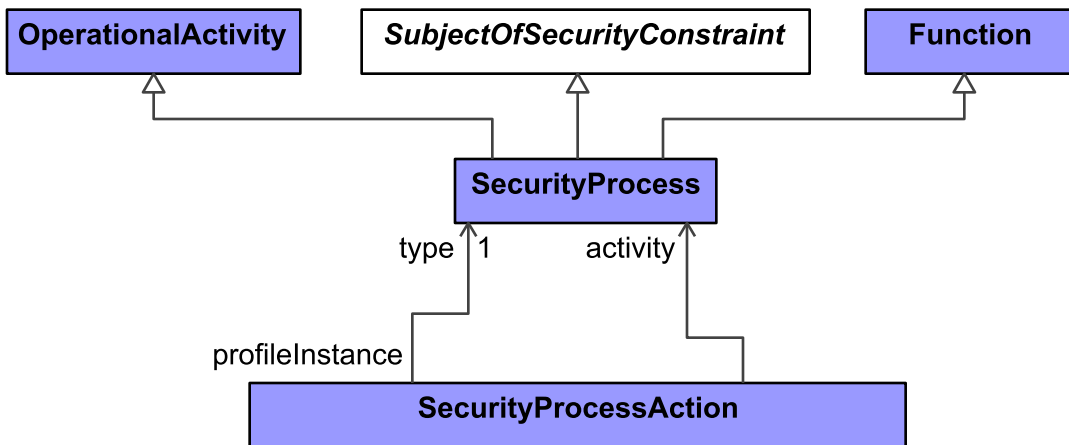
Figure 9:212 - SecurityProcess
