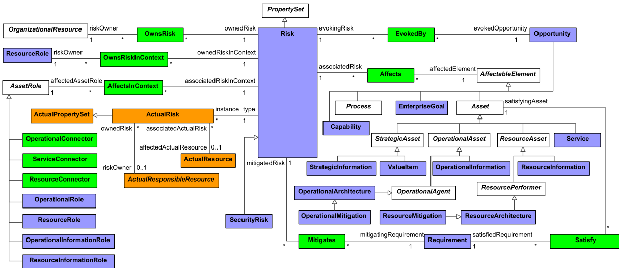
Figure 8:95 - Parameters: Risk
