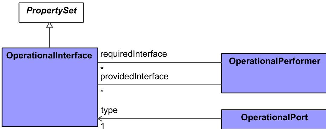
Figure 9:108 - OperationalInterface
