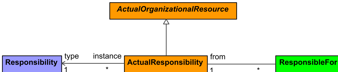
Figure 9:249 - ActualResponsibility
