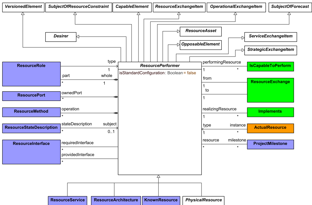
Figure 9:166 - ResourcePerformer
