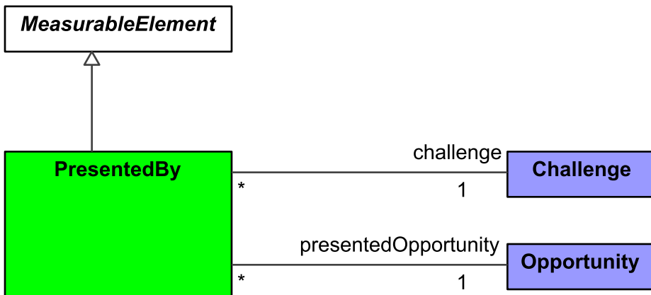
Figure 9:52 - PresentedBy
