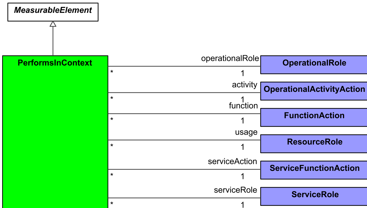
Figure 9:14 - PerformsInContext
