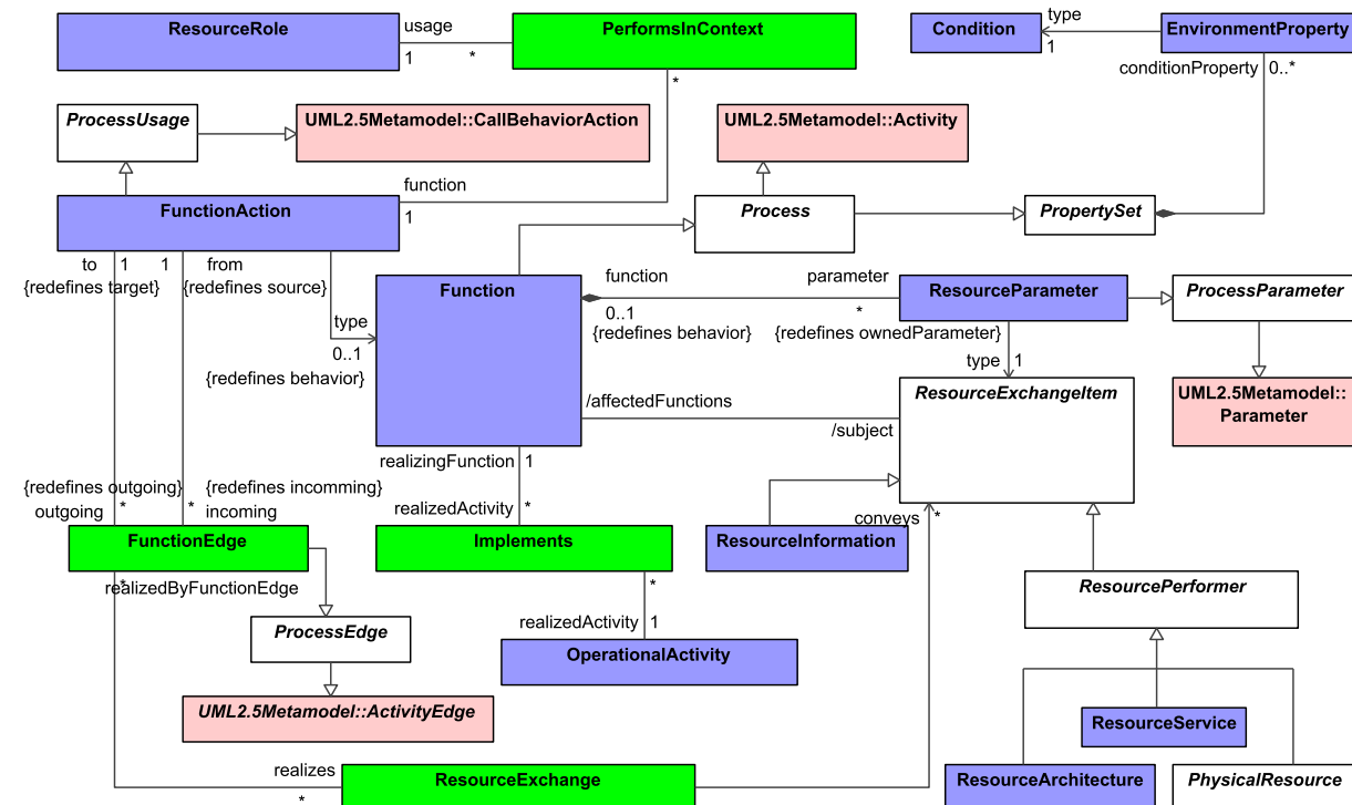
Figure 8:60 - Resources Processes
