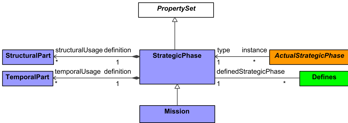
Figure 9:62 - StrategicPhase
