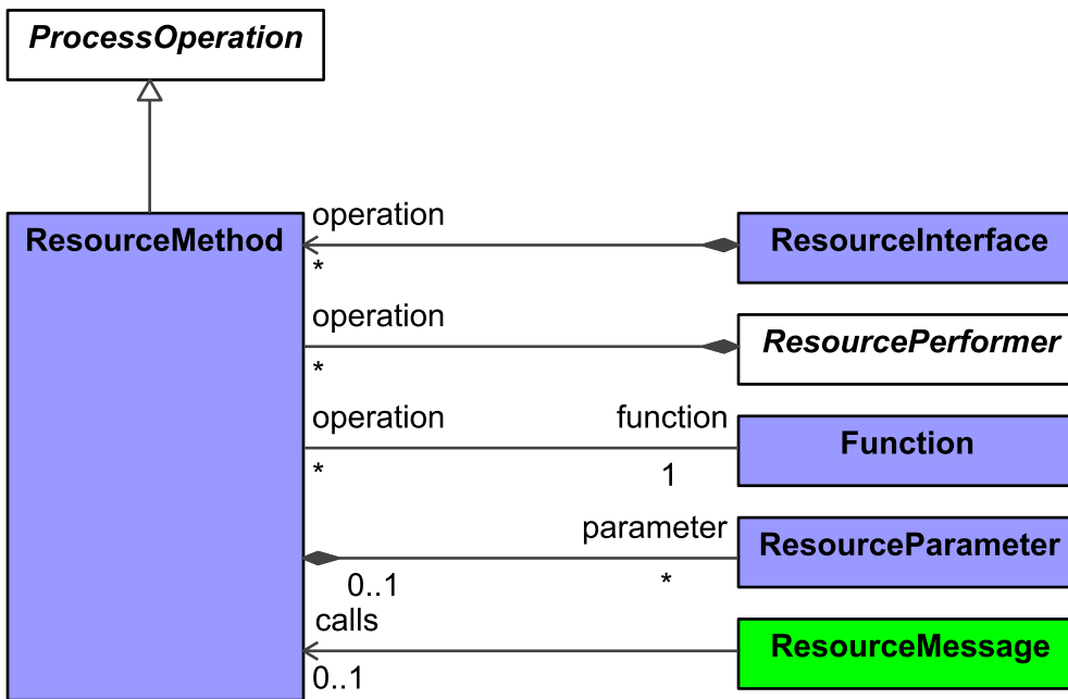
Figure 9:170 - ResourceMethod
