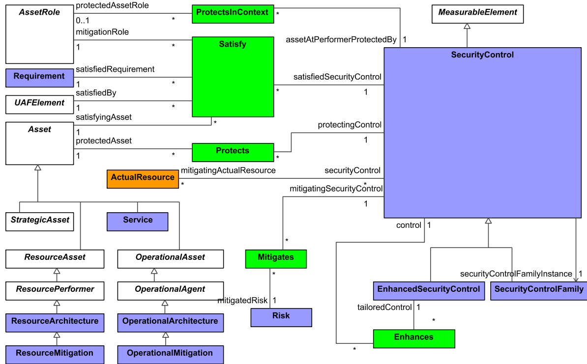
Figure 8:69 - Security Controls
