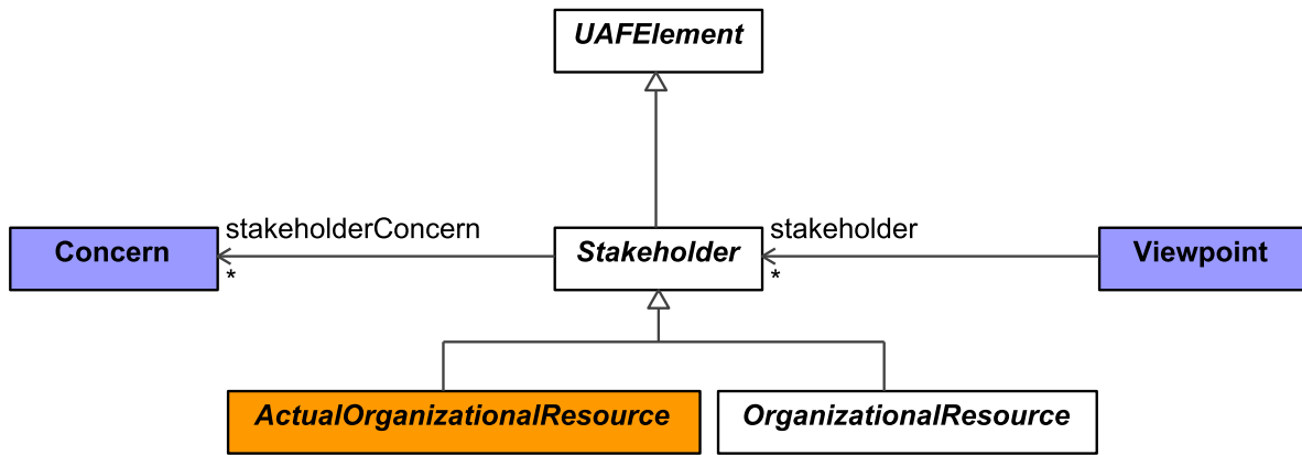
Figure 9:41 - Stakeholder
