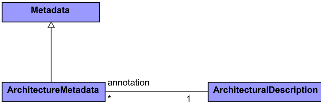
Figure 9:24 - ArchitectureMetadata
