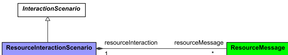
Figure 9:155 - ResourceInteractionScenario
