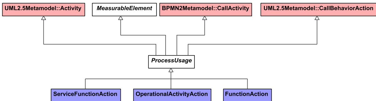
Figure 9:19 - ProcessUsage
