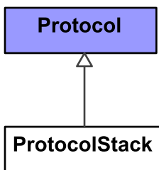
Figure 9:240 - ProtocolStack
