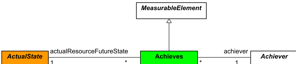
Figure 9:81 - Achieves
