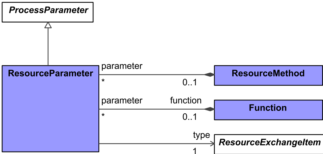
Figure 9:171 - ResourceParameter
