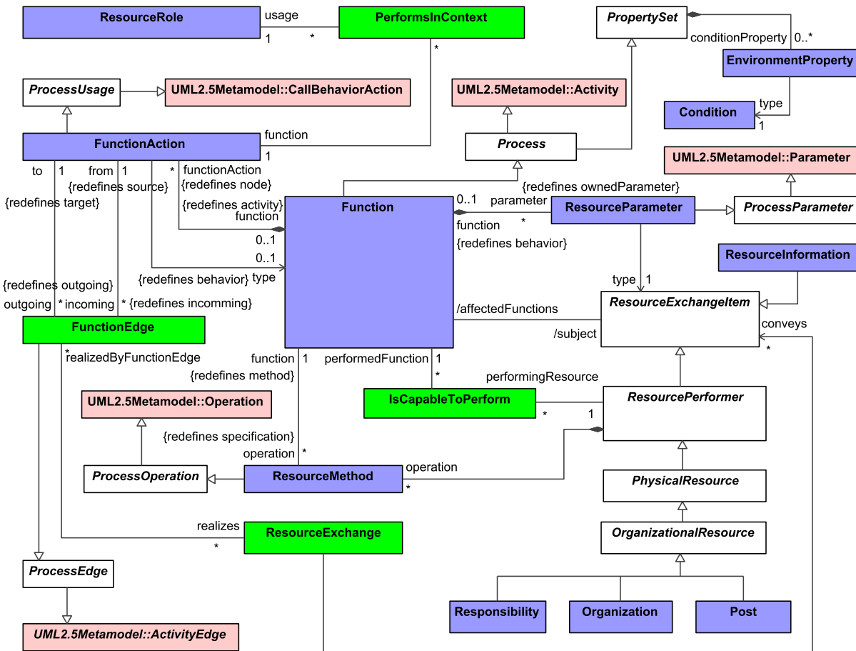
Figure 8:47 - Personnel Processes
