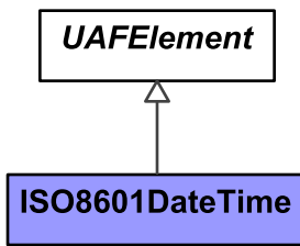
Figure 9:4 - ISO8601DateTime
