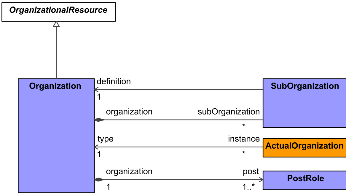
Figure 9:146 - Organization
