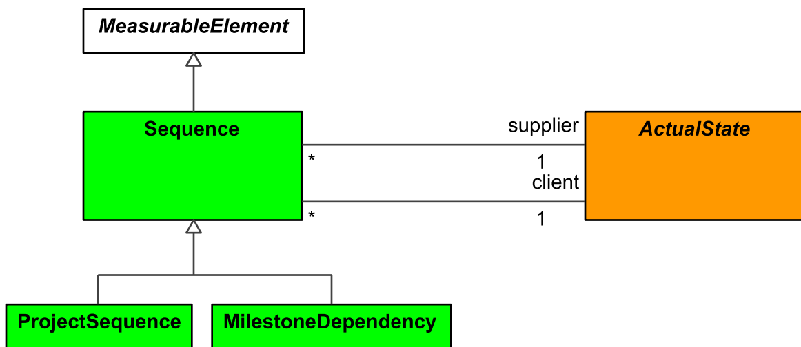
Figure 9:36 - Sequence
