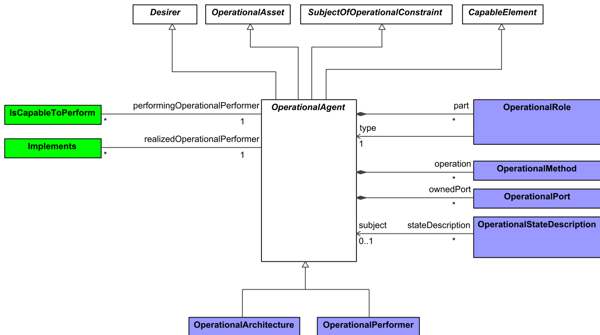
Figure 9:98 - OperationalAgent
