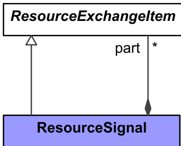
Figure 9:179 - ResourceSignal
