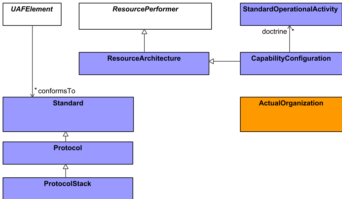
Figure 8:82 - Standards Taxonomy
