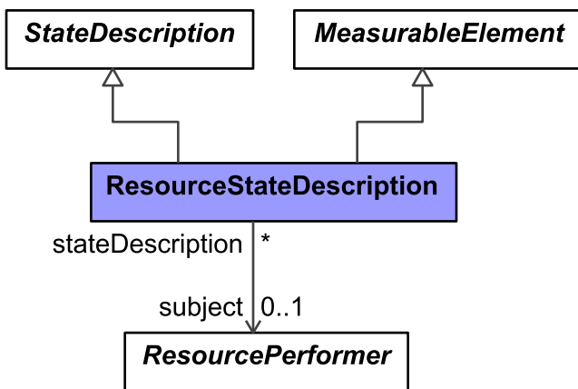
Figure 9:184 - ResourceStateDescription
