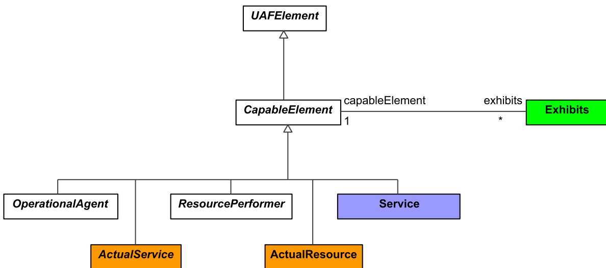
Figure 9:12 - CapableElement
