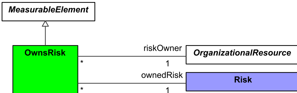
Figure 9:281 - OwnsRisk
