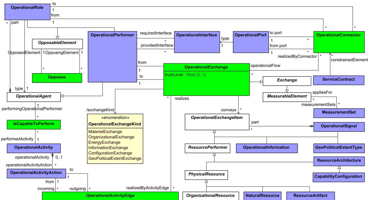
Figure 8:26 - Operational Connectivity
