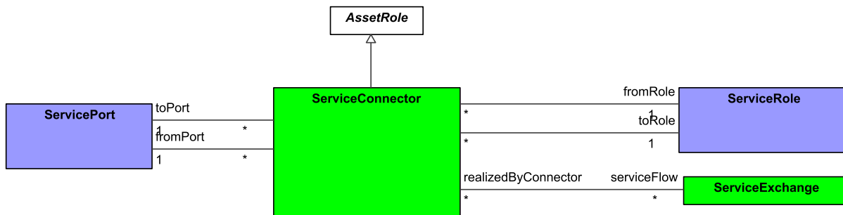
Figure 9:130 - ServiceConnector
