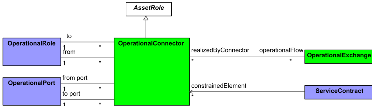
Figure 9:105 - OperationalConnector
