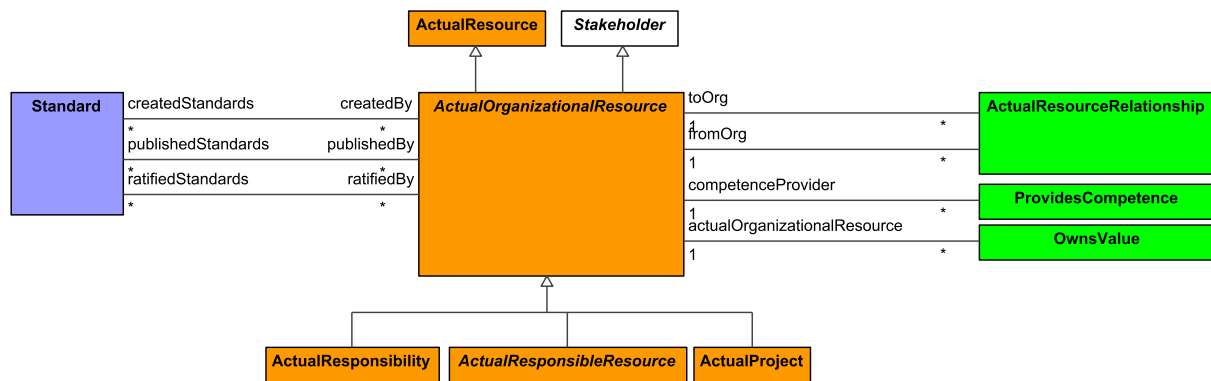
Figure 9:244 - ActualOrganizationalResource
