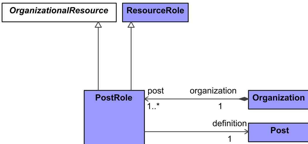
Figure 9:151 - PostRole
