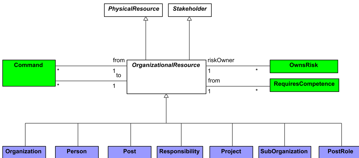
Figure 9:147 - OrganizationalResource
