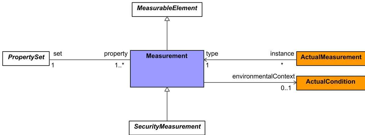
Figure 9:276 - Measurement
