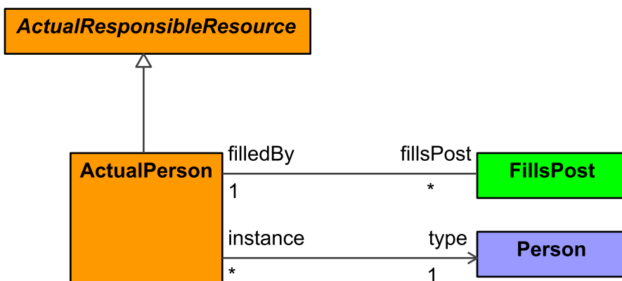
Figure 9:245 - ActualPerson
