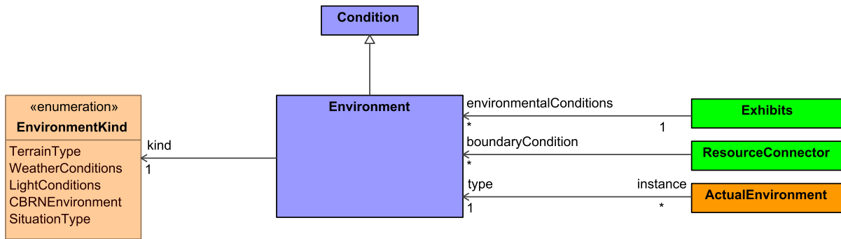
Figure 9:270 - Environment
