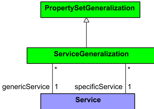
Figure 9:126 - ServiceGeneralization
