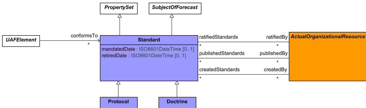
Figure 9:241 - Standard
