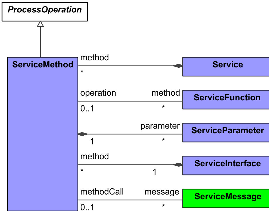
Figure 9:127 - ServiceMethod
