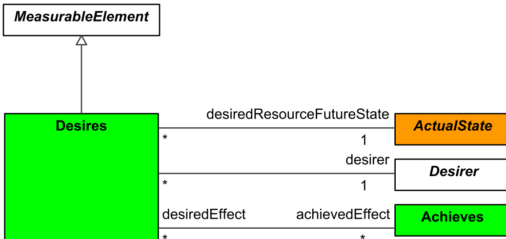
Figure 9:85 - Desires
