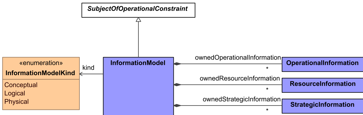
Figure 9:28 - InformationModel
