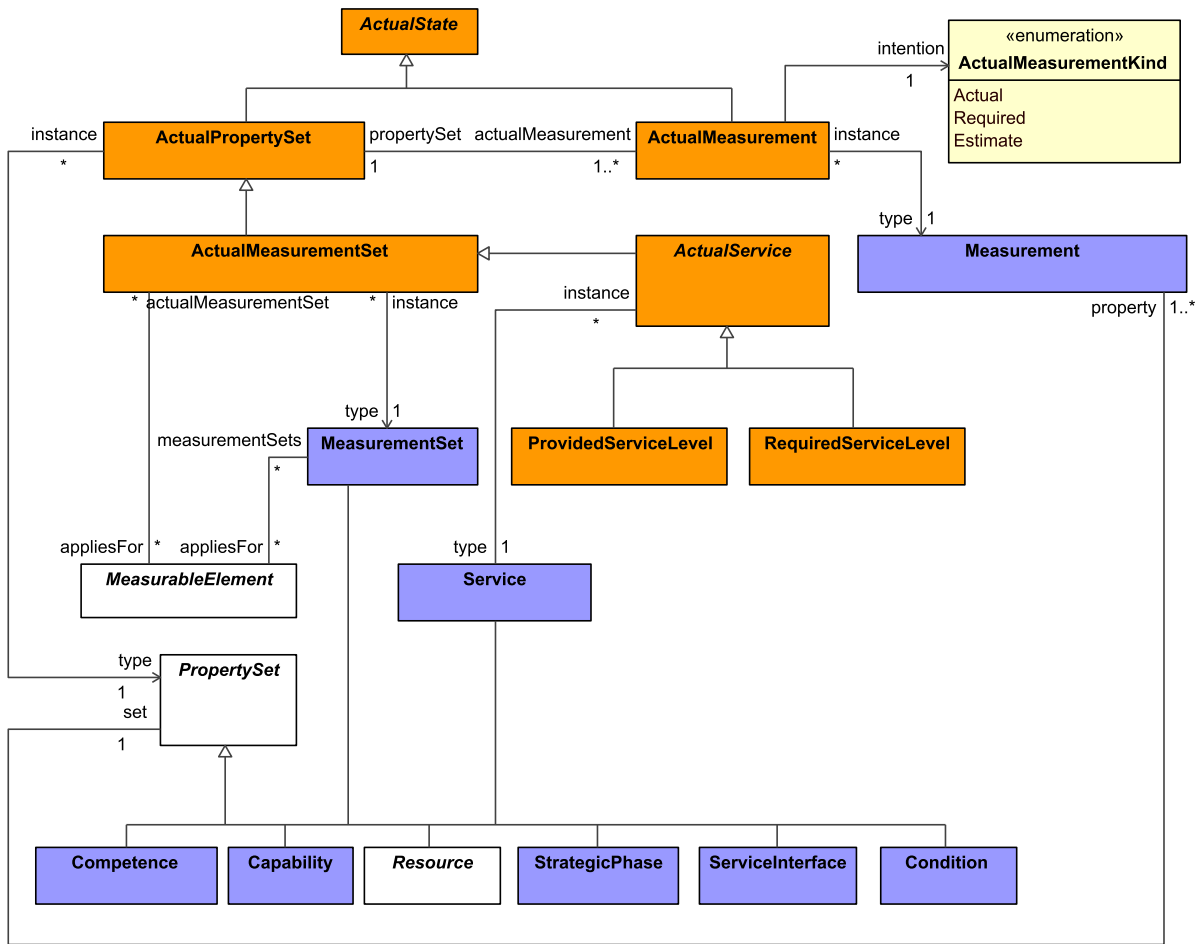
Figure 8:93 - Parameters: Measurements
