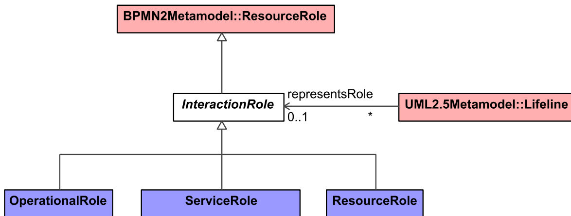
Figure 9:21 - InteractionRole
