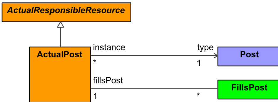
Figure 9:246 - ActualPost
