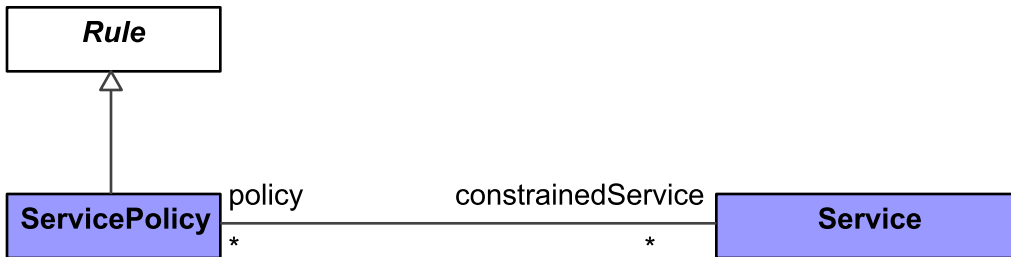
Figure 9:143 - ServicePolicy
