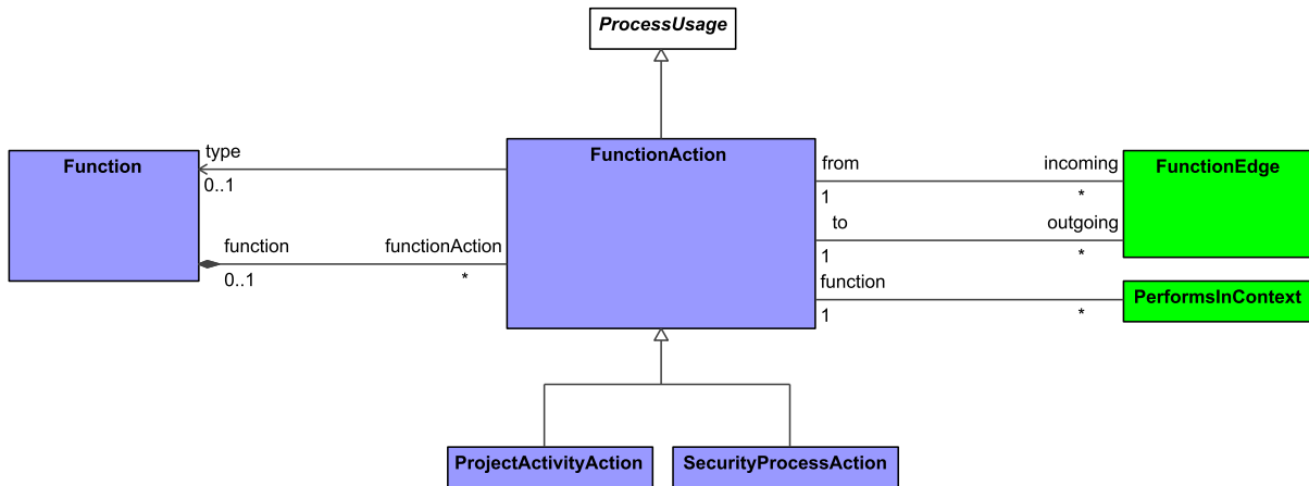
Figure 9:181 - FunctionAction
