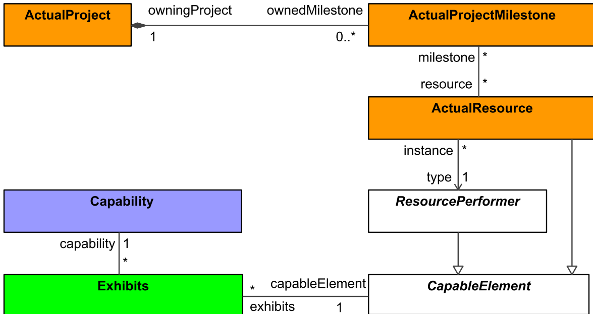
Figure 8:81 - Project Traceability
