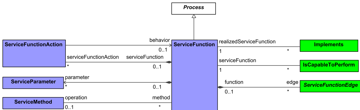
Figure 9:136 - ServiceFunction
