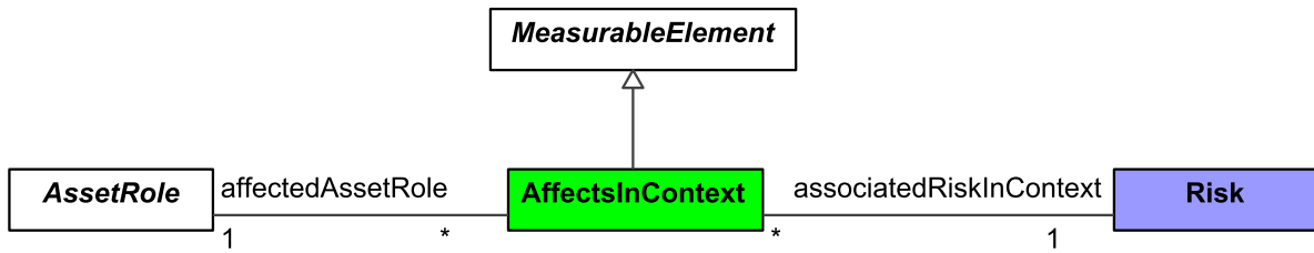
Figure 9:268 - AffectsInContext
