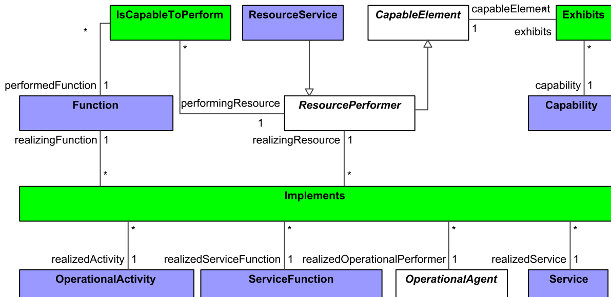
Figure 8:68 - Resources Traceability
