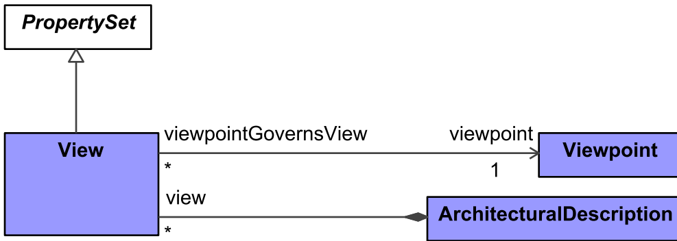
Figure 9:43 - View
