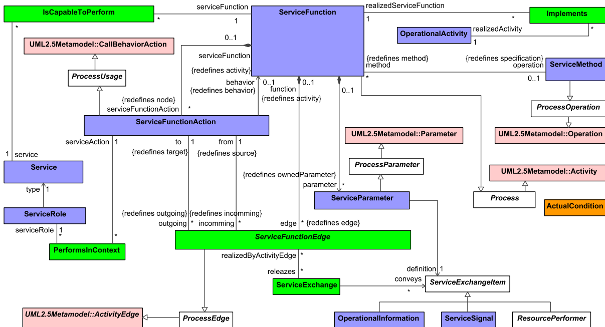
Figure 8:37 - Services Processes
