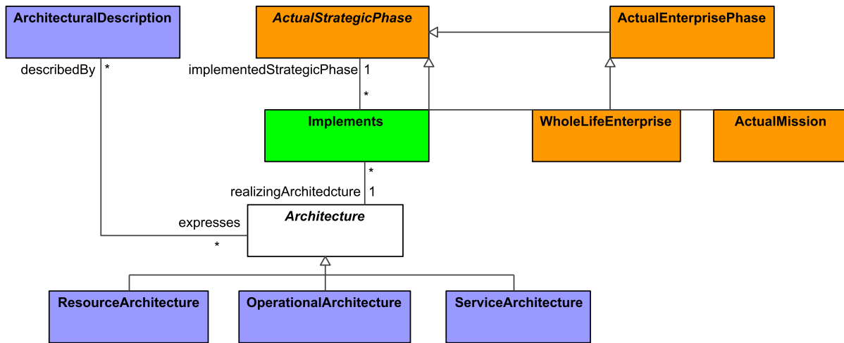
Figure 8:10 - Architecture Traceability
