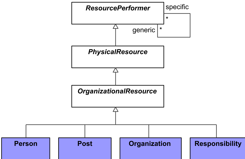
Figure 8:44 - Personnel Taxonomy
