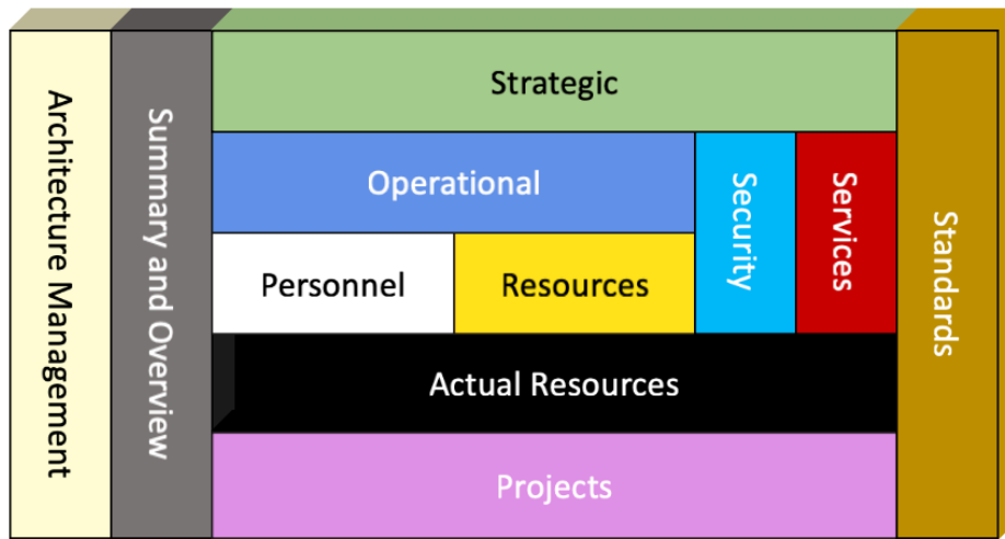
Figure 7:2 – Viewpoint Interrelationships
