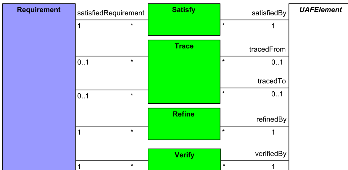
Figure 8:89 - Motivation: Requirements
