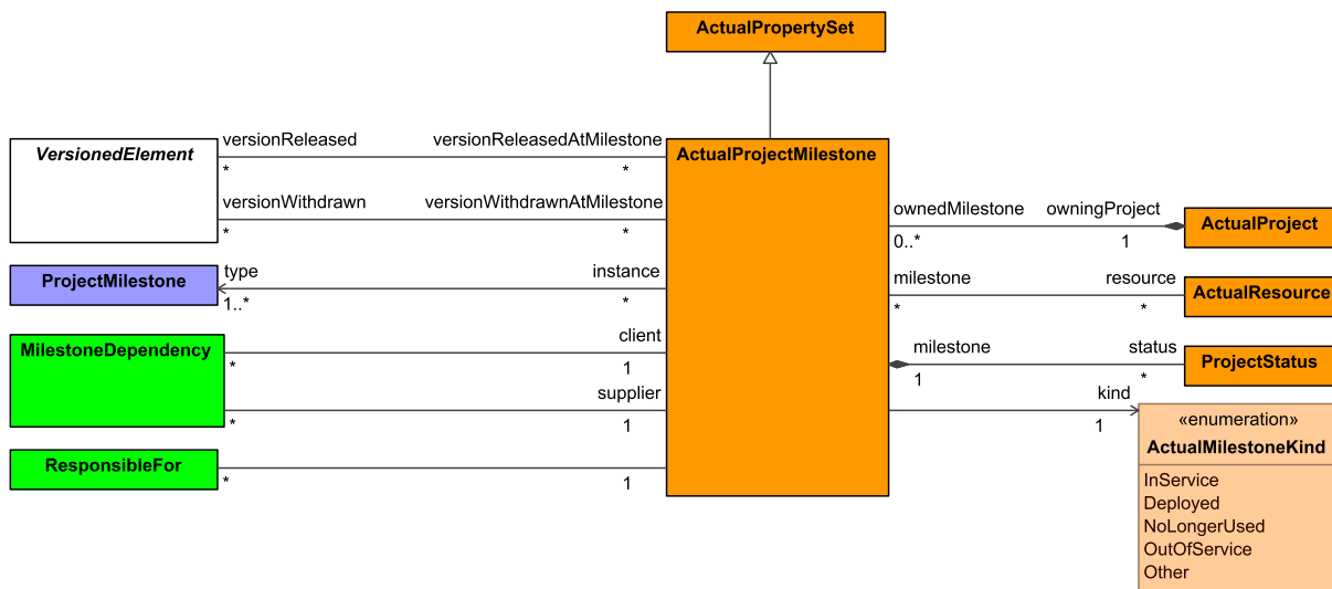
Figure 9:236 - ActualProjectMilestone
