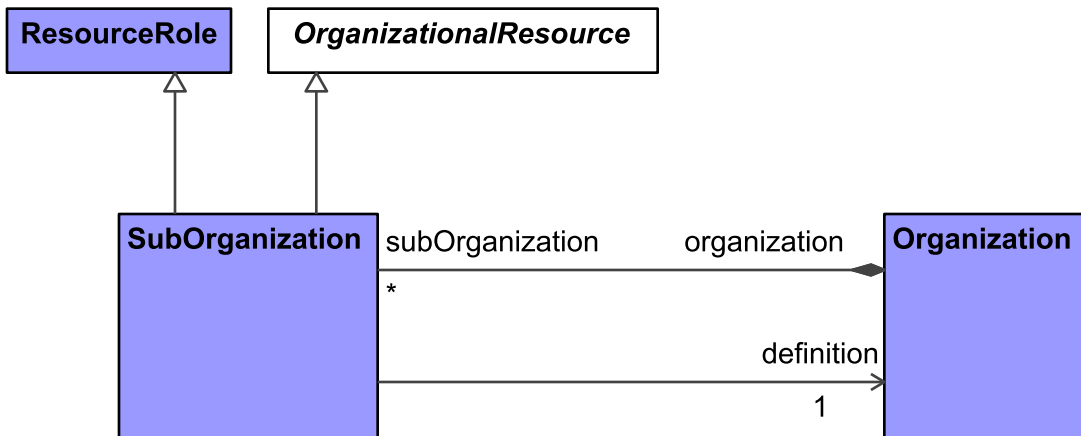
Figure 9:152 - SubOrganization
