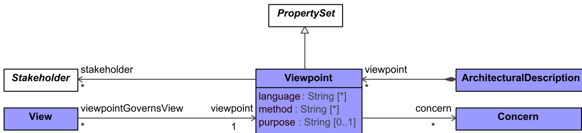
Figure 9:44 - Viewpoint
