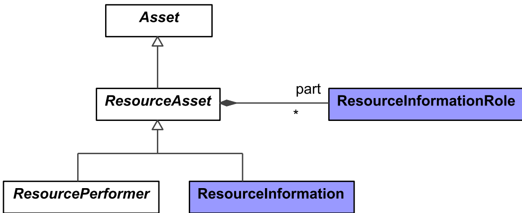
Figure 9:206 - ResourceAsset
