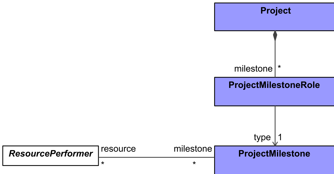
Figure 8:78 - Project Connectivity
