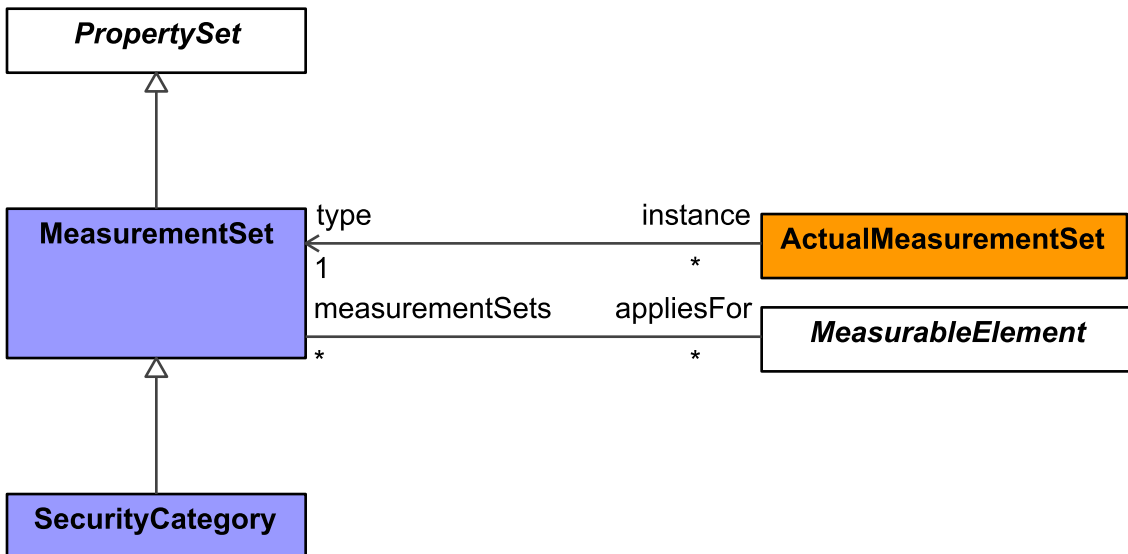
Figure 9:277 - MeasurementSet
