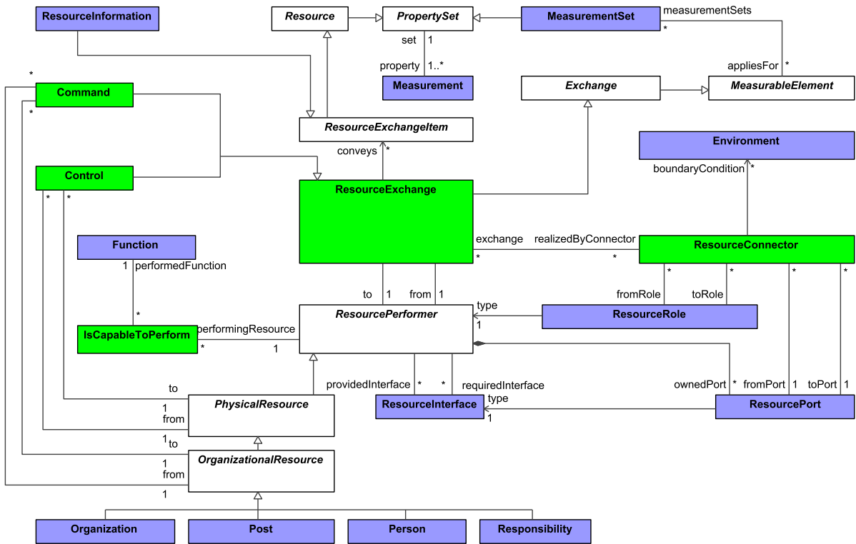
Figure 8:46 - Personnel Connectivity
