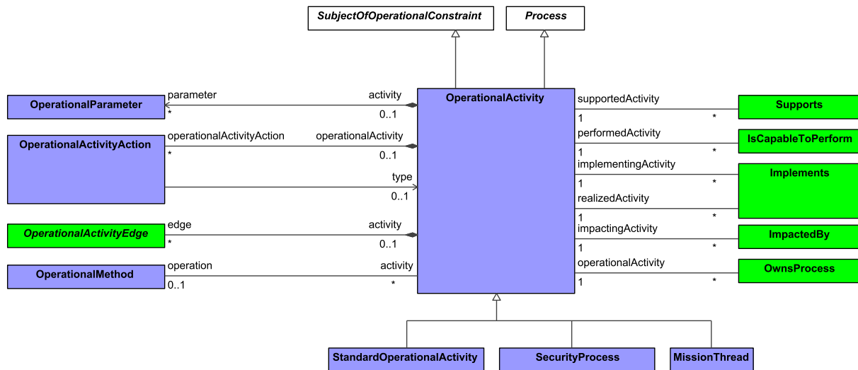
Figure 9:114 - OperationalActivity
