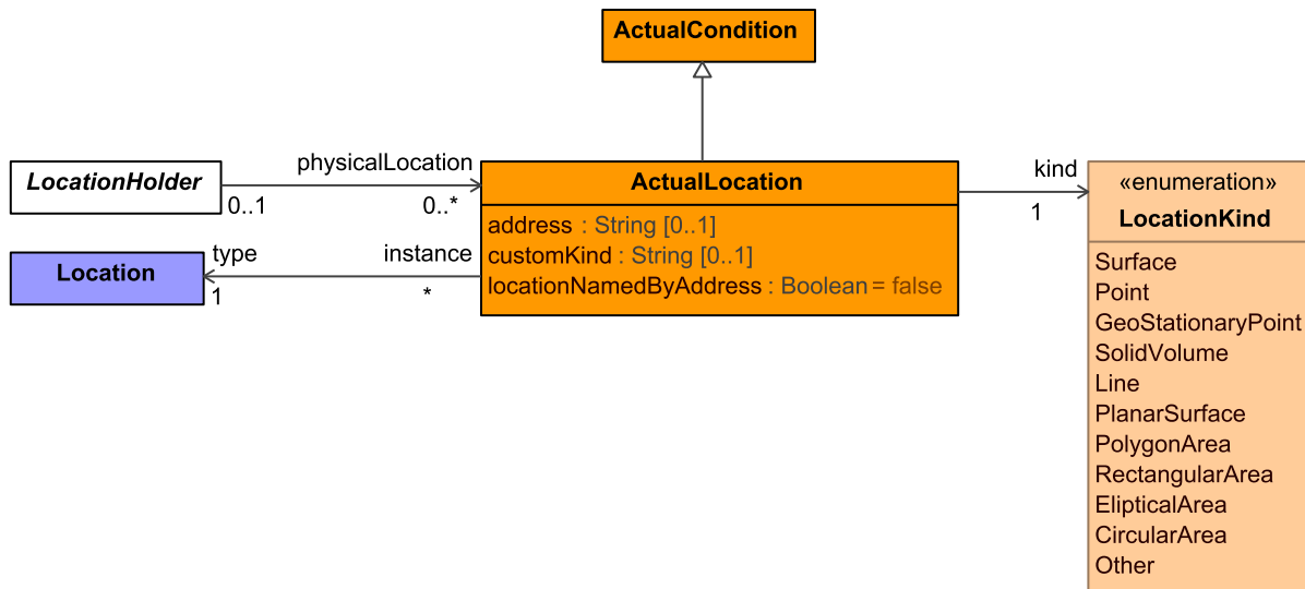
Figure 9:259 - ActualLocation
