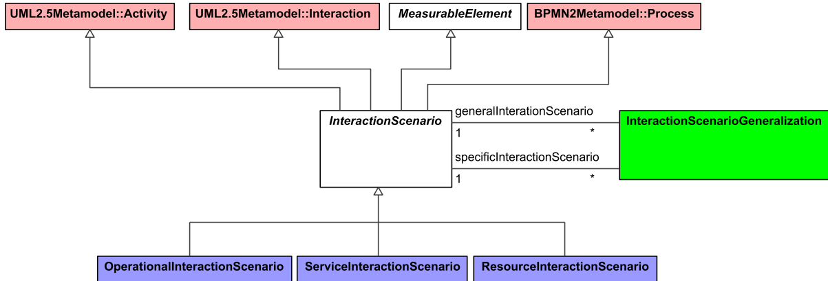
Figure 9:22 - InteractionScenario
