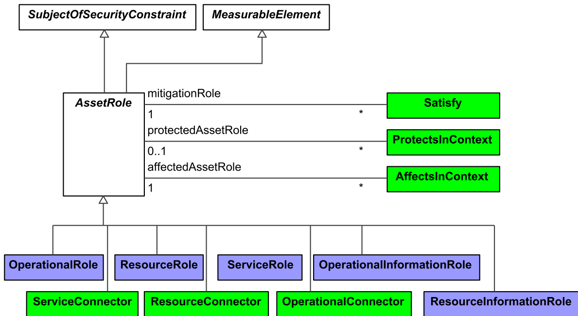
Figure 9:209 - AssetRole
