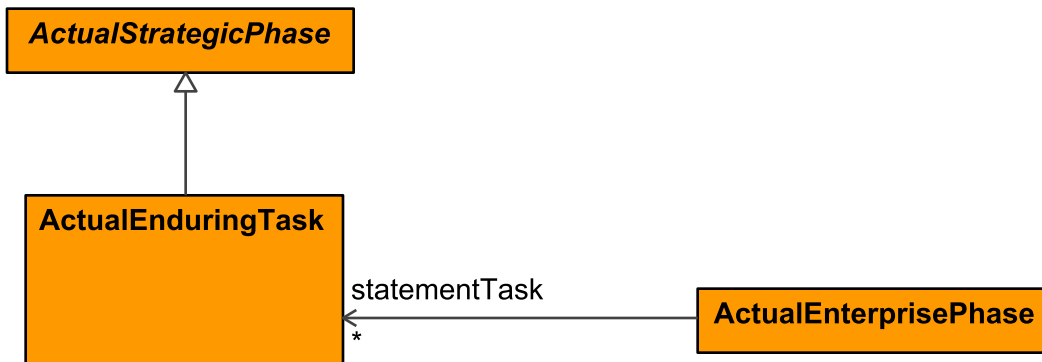
Figure 9:72 - ActualEnduringTask
