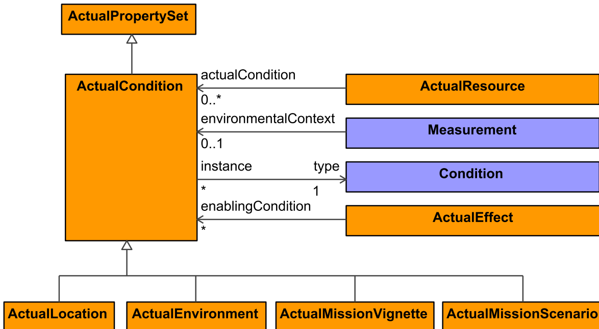
Figure 9:257 - ActualCondition
