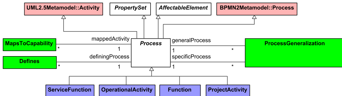
Figure 9:15 - Process
