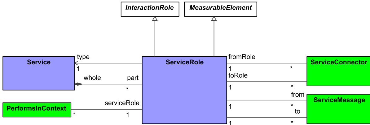
Figure 9:129 - ServiceRole
