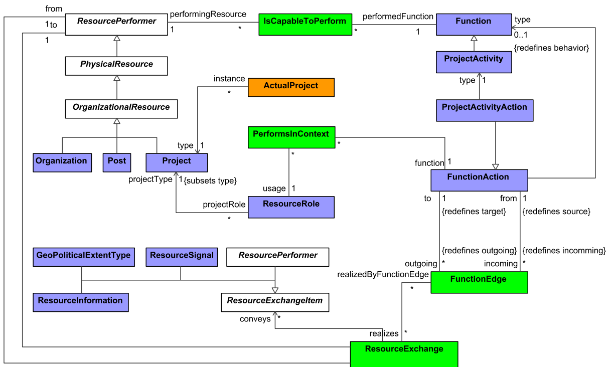
Figure 8:79 - Project Processes
