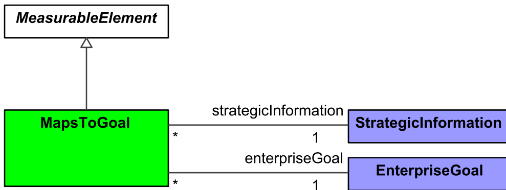
Figure 9:87 - MapsToGoal
