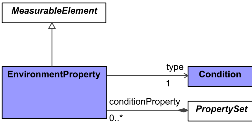
Figure 9:271 - EnvironmentProperty
