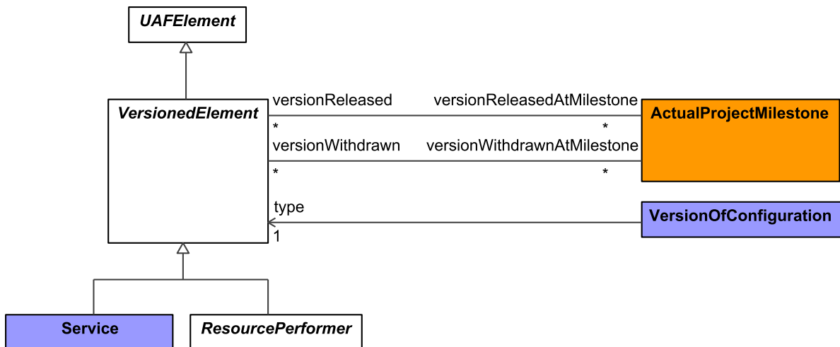
Figure 9:192 - VersionedElement
