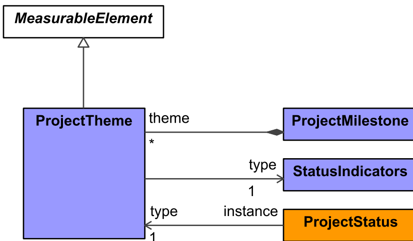
Figure 9:229 - ProjectTheme
