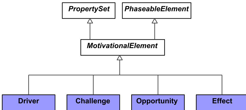
Figure 9:50 - MotivationalElement
