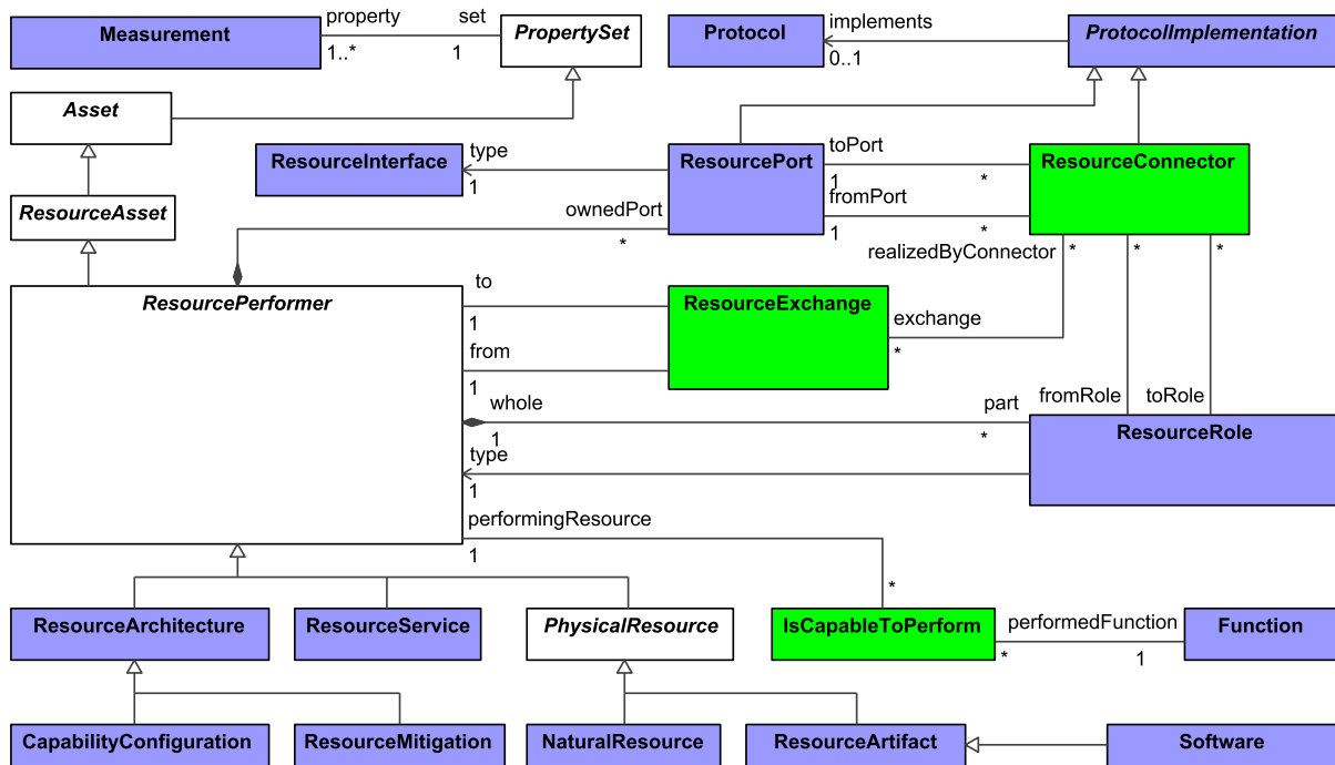
Figure 8:58 - Resources Structure
