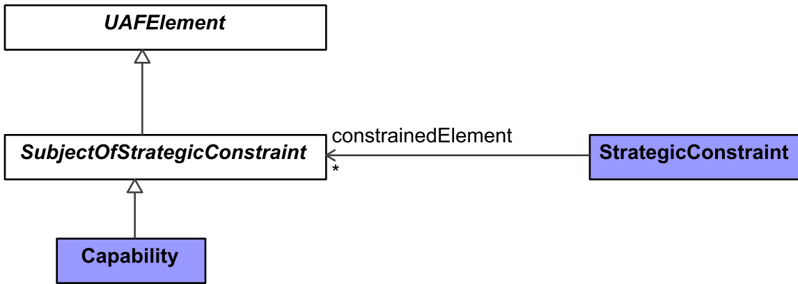
Figure 9:89 - SubjectOfStrategicConstraint
