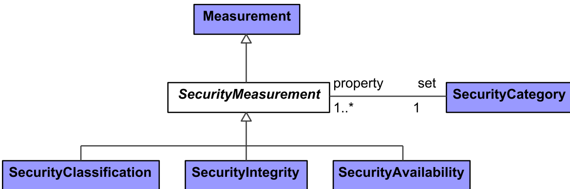
Figure 9:221 - SecurityMeasurement
