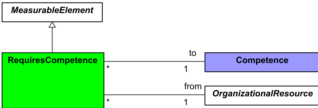
Figure 9:158 - RequiresCompetence
