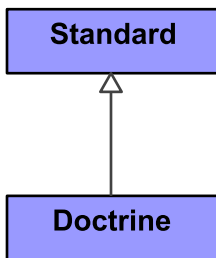
Figure 9:238 - Doctrine
