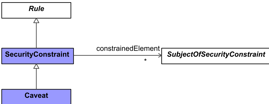
Figure 9:219 - SecurityConstraint
