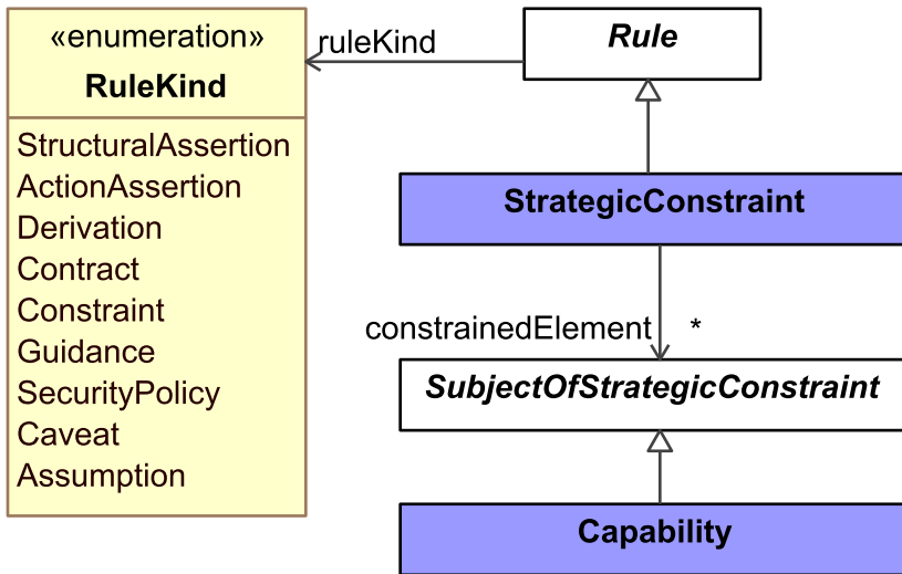
Figure 9:88 - StrategicConstraint
