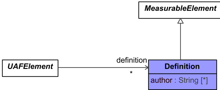
Figure 9:26 - Definition
