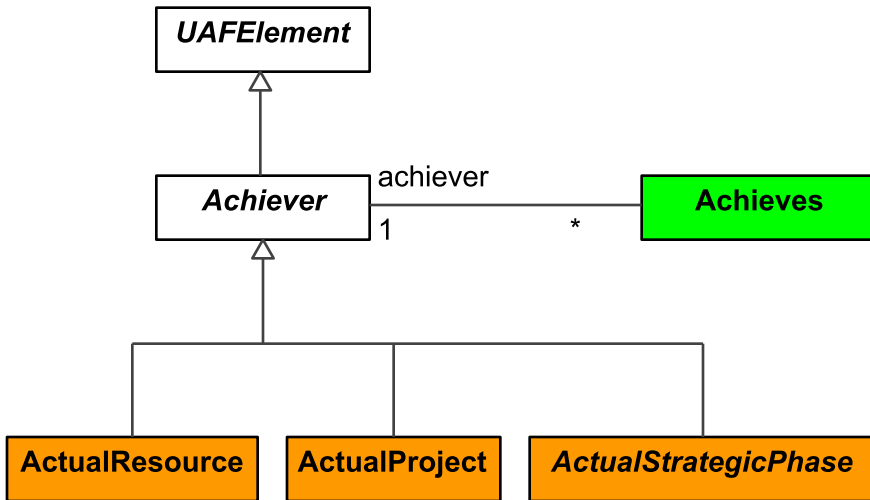
Figure 9:80 - Achiever
