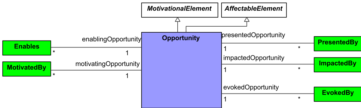
Figure 9:51 - Opportunity
