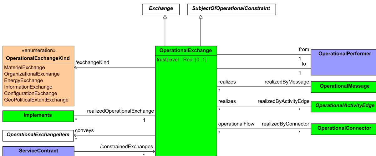
Figure 9:106 - OperationalExchange
