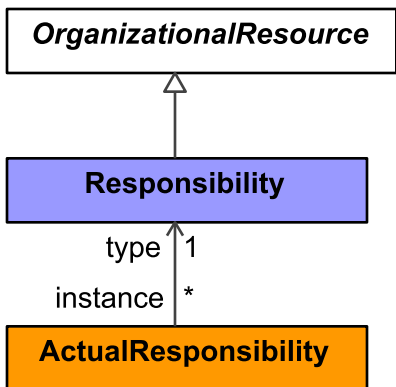
Figure 9:150 - Responsibility
