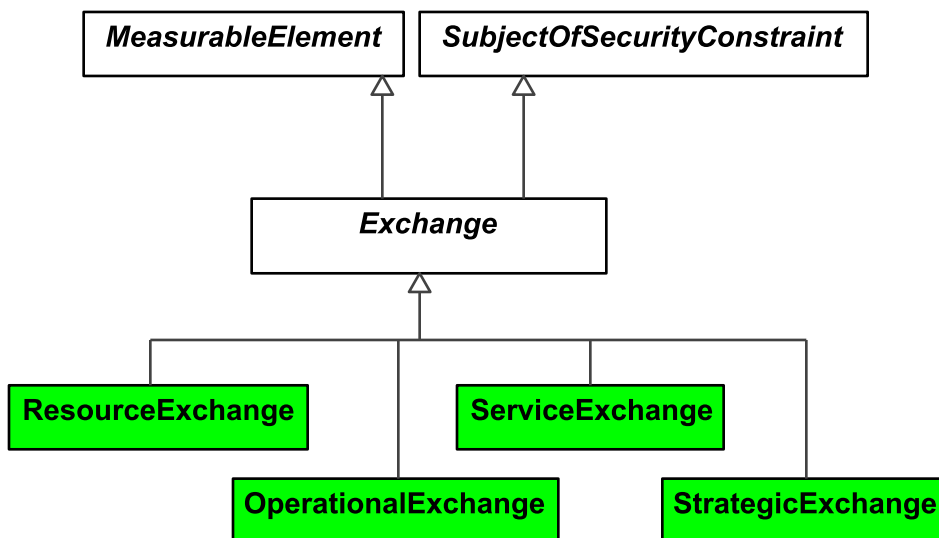
Figure 9:9 - Exchange
