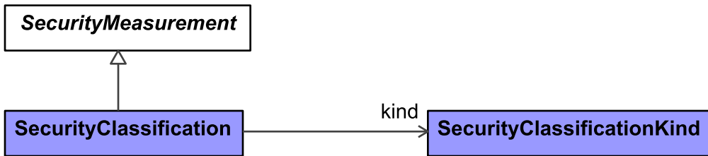
Figure 9:217 - SecurityClassification
