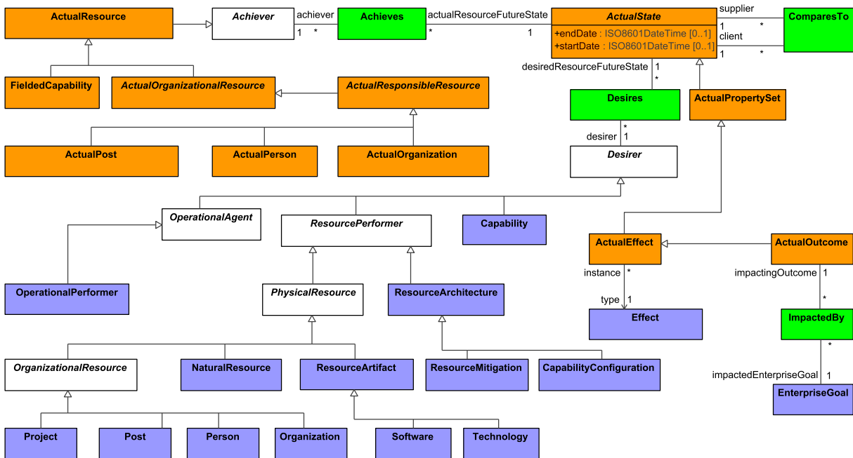
Figure 8:18 - Strategic States
