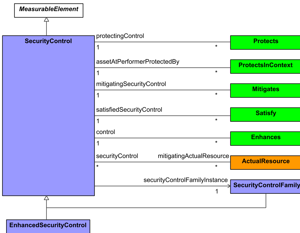
Figure 9:201 - SecurityControl
