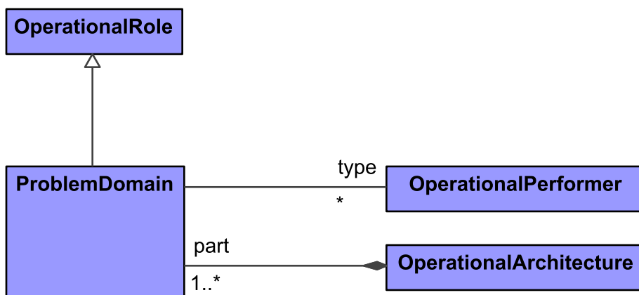
Figure 9:104 - ProblemDomain
