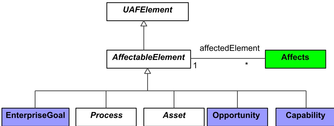
Figure 9:266 - AffectableElement
