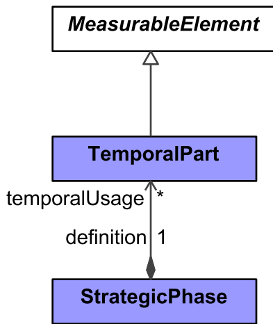
Figure 9:68 - TemporalPart
