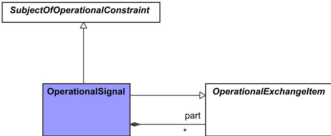
Figure 9:110 - OperationalSignal
