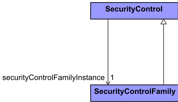
Figure 9:202 - SecurityControlFamily
