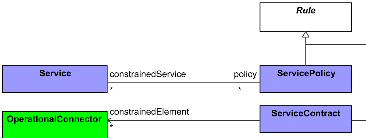
Figure 8:41 - Services Constraints
