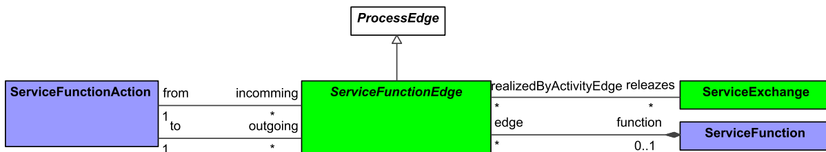
Figure 9:138 - ServiceFunctionEdge
