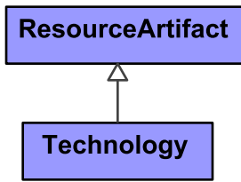
Figure 9:191 - Technology
