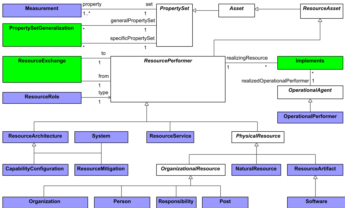
Figure 8:57 - Resources Taxonomy
