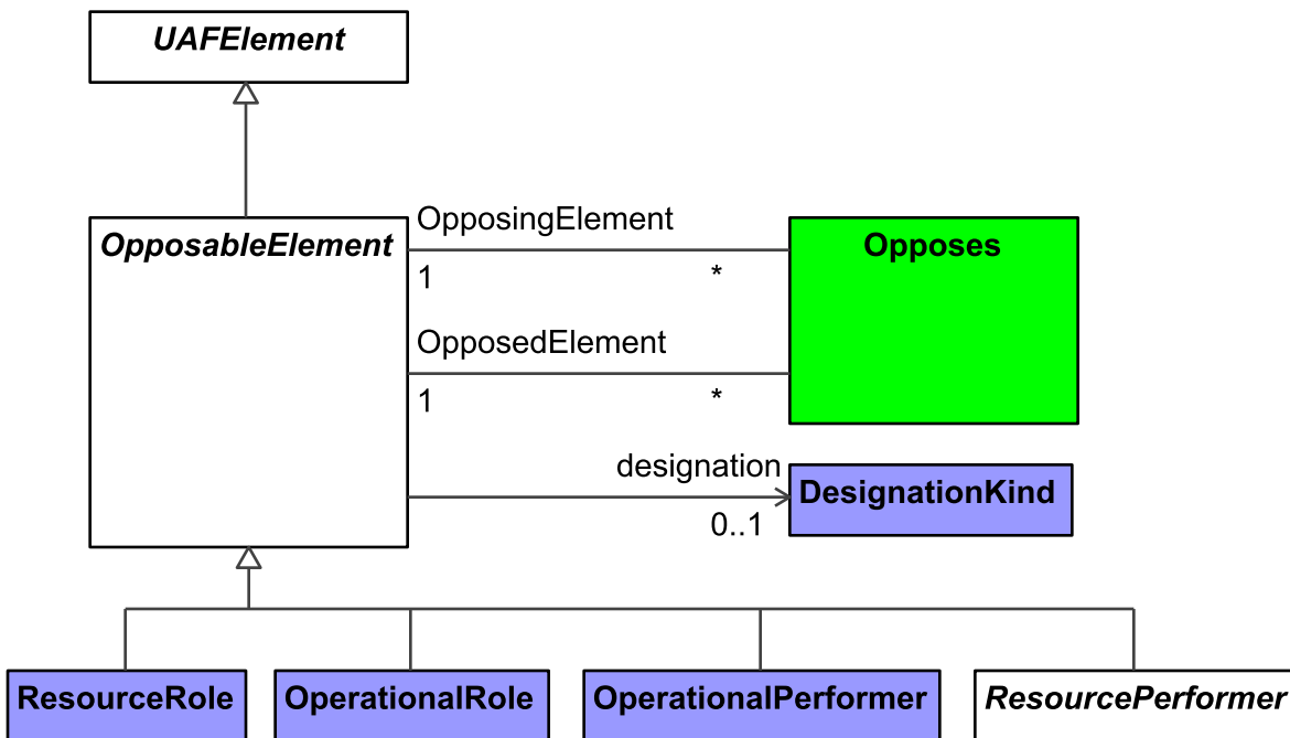
Figure 9:5 - OpposableElement
