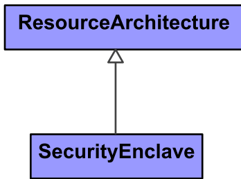
Figure 9:208 - SecurityEnclave
