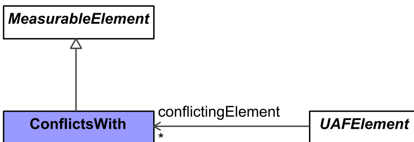
Figure 9:25 - ConflictsWith
