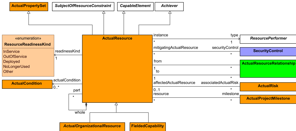
Figure 9:247 - ActualResource
