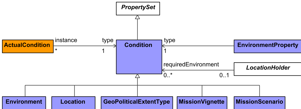
Figure 9:269 - Condition
