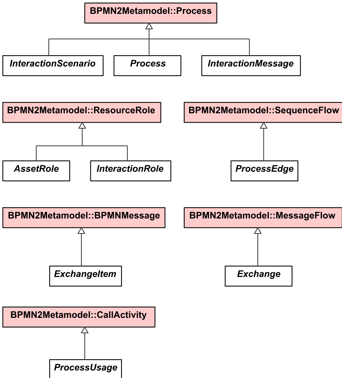
Figure 8:96 - BPMN
