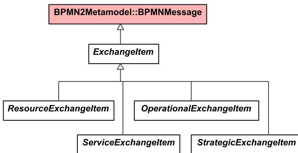
Figure 9:10 - Exchangeltem
