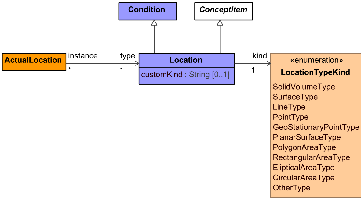
Figure 9:273 - Location
