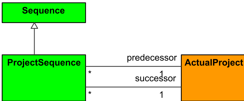
Figure 9:232 - ProjectSequence
