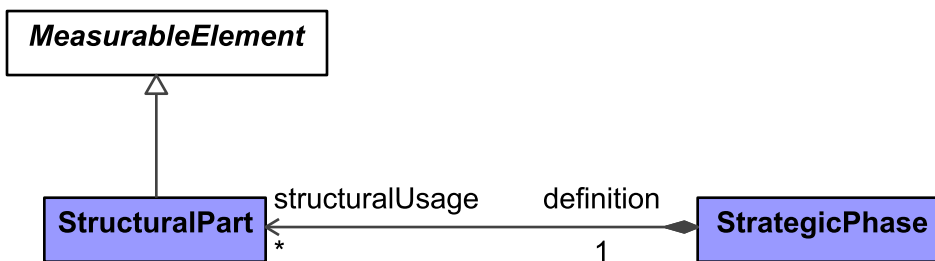
Figure 9:67 - StructuralPart
