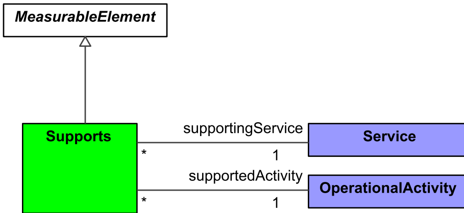
Figure 9:145 - Supports
