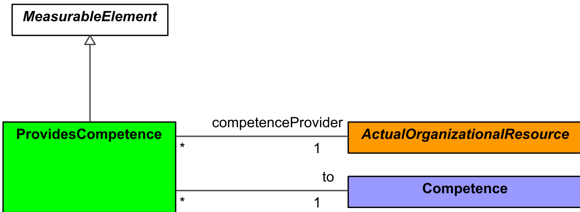
Figure 9:254 - ProvidesCompetence
