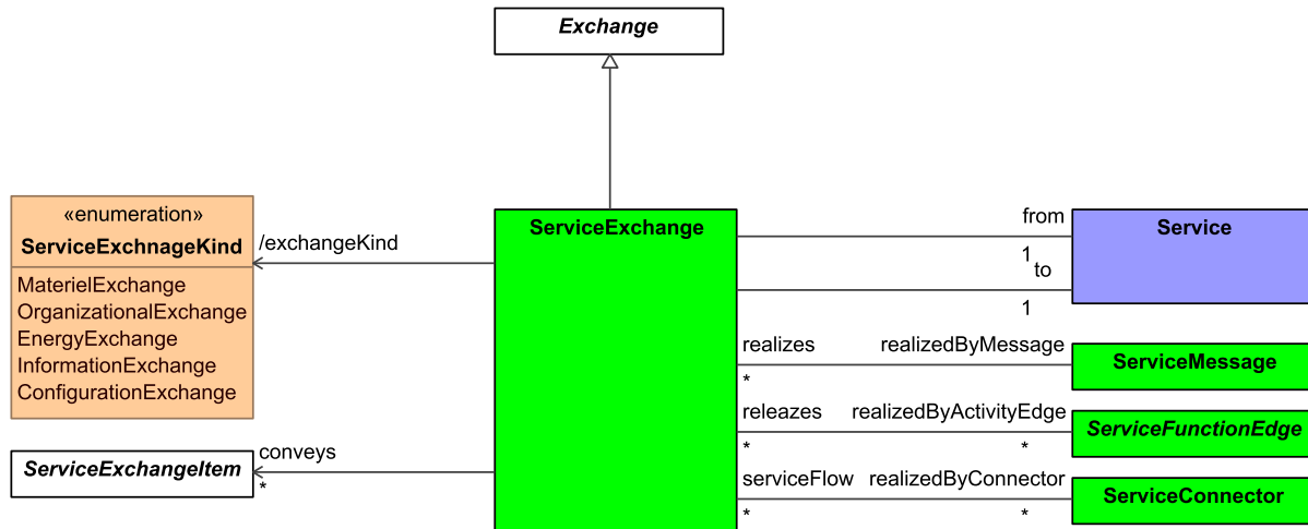
Figure 9:131 - ServiceExchange
