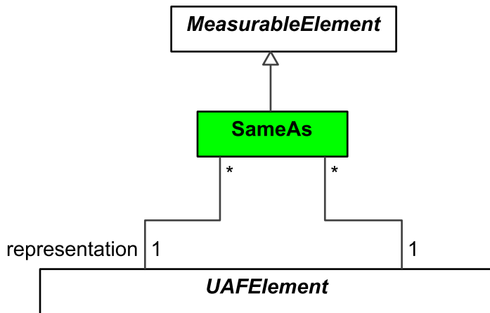
Figure 9:31 - SameAs
