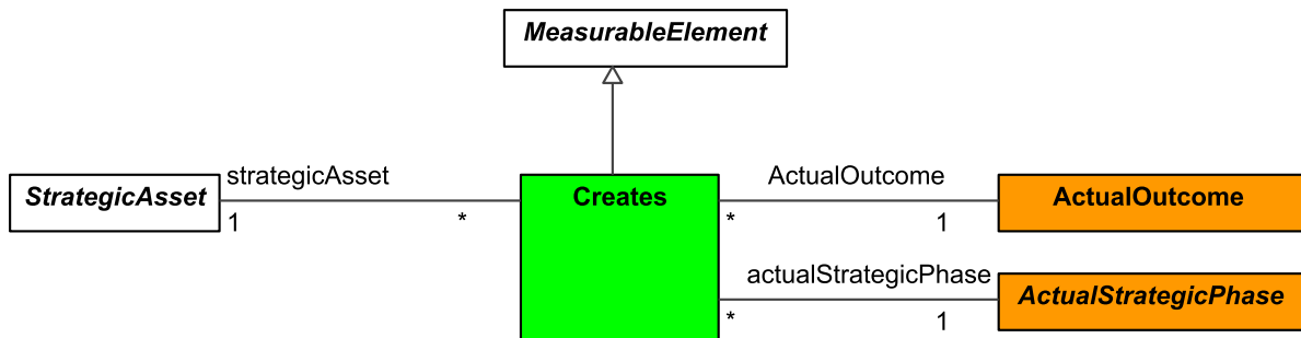
Figure 9:77 - Creates
