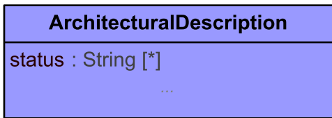
Figure 8:5 - Architecture Status
