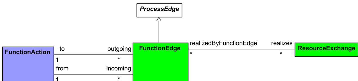
Figure 9:182 - FunctionEdge
