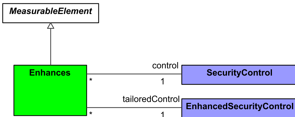
Figure 9:198 - Enhances
