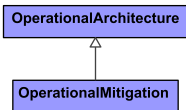
Figure 9:205 - OperationalMitigation
