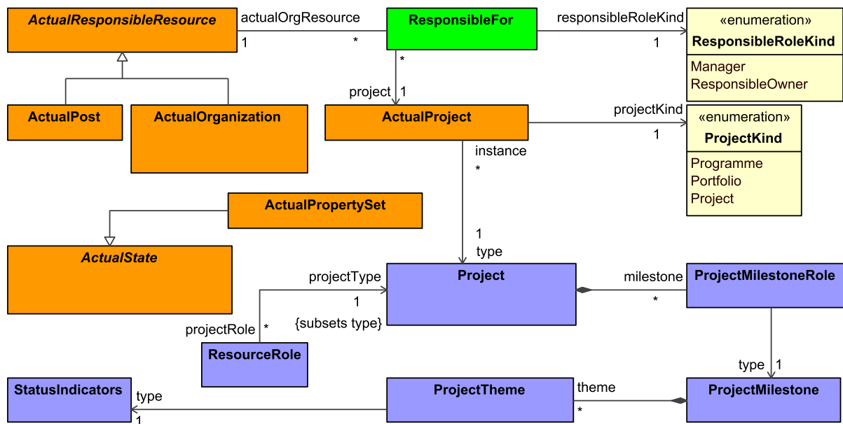
Figure 8:77 - Project Structure
