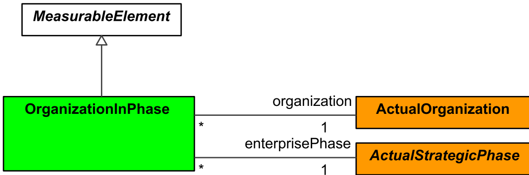
Figure 9:93 - OrganizationInPhase
