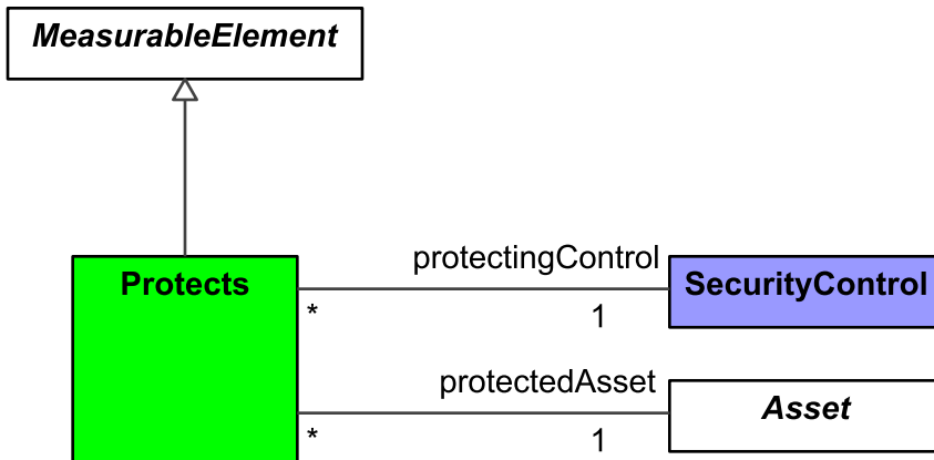
Figure 9:199 - Protects
