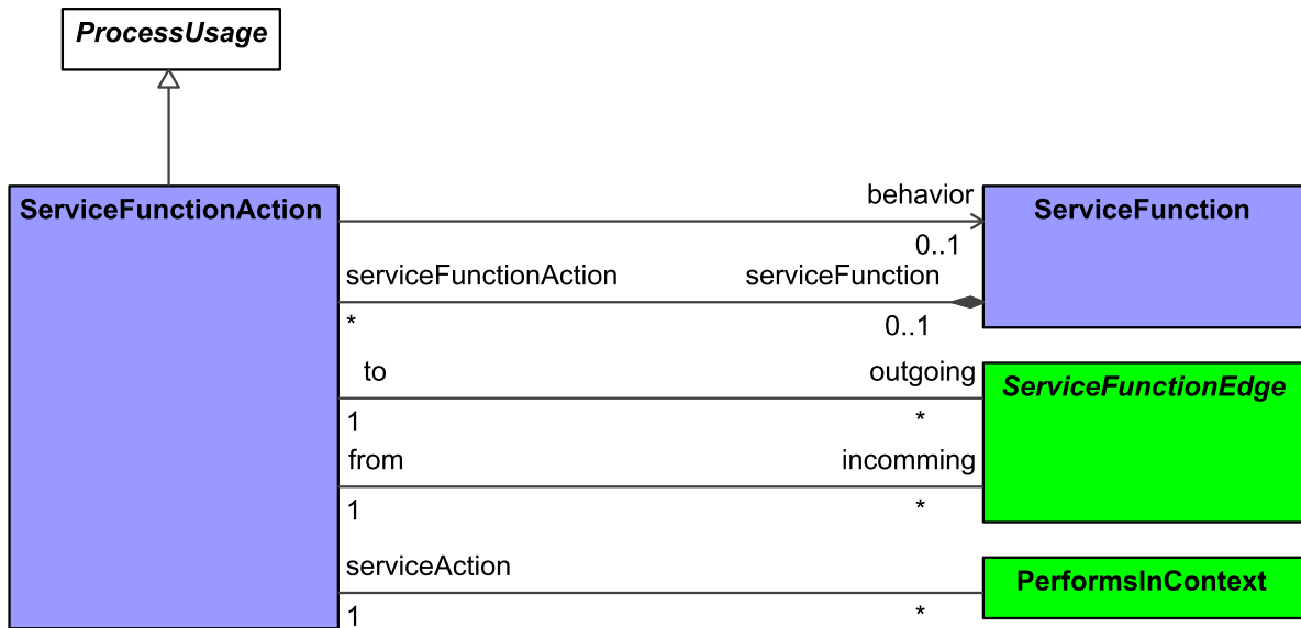
Figure 9:137 - ServiceFunctionAction
