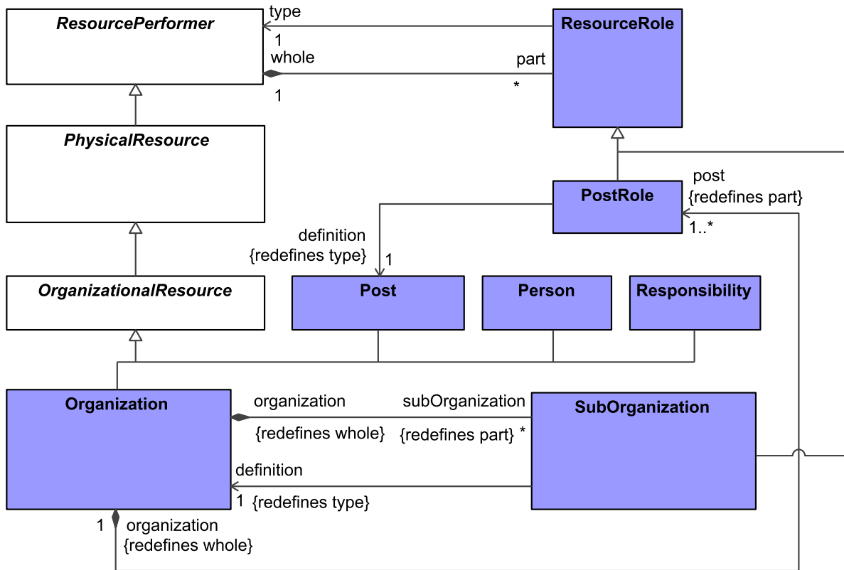
Figure 8:45 - Personnel Structure
