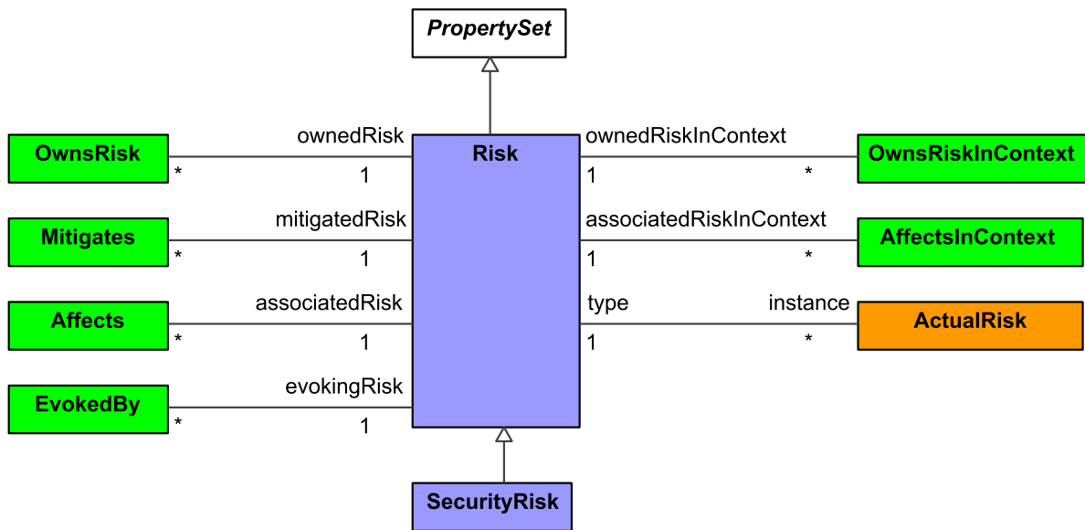
Figure 9:284 - Risk
