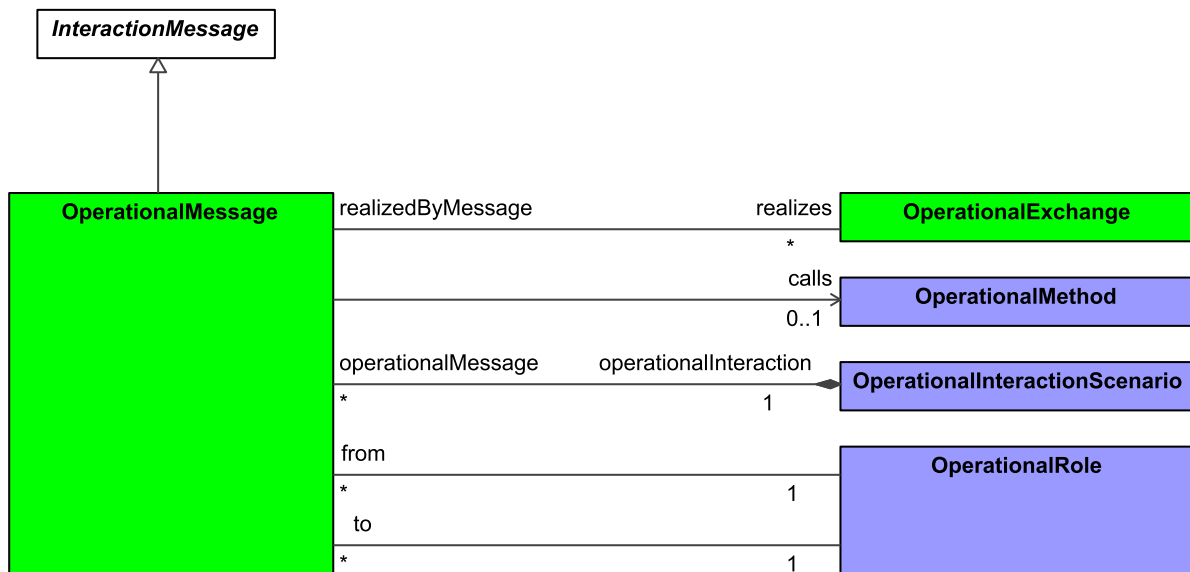
Figure 9:120 - OperationalMessage
