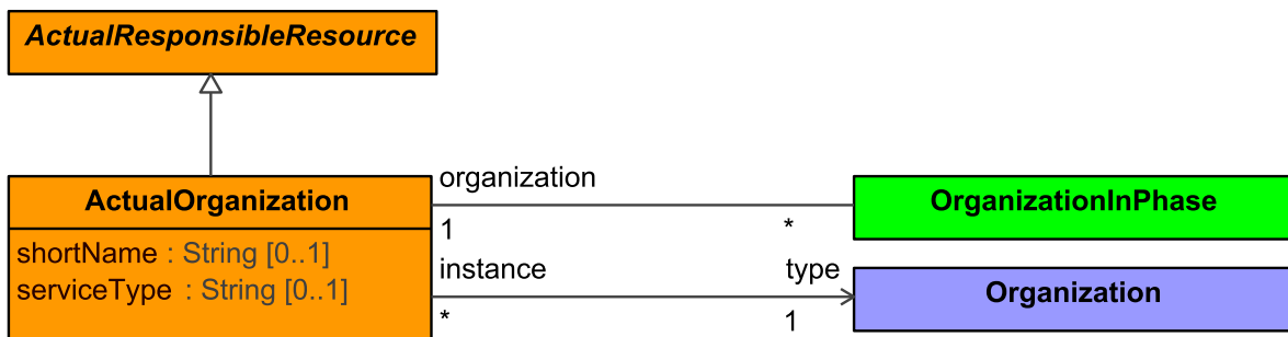
Figure 9:243 - ActualOrganization
