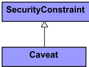
Figure 9:214 - Caveat
