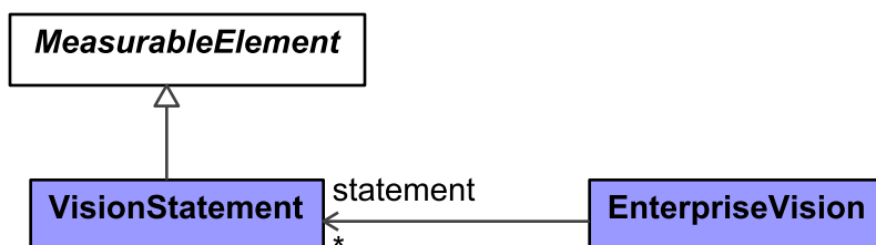
Figure 9:64 - VisionStatement
