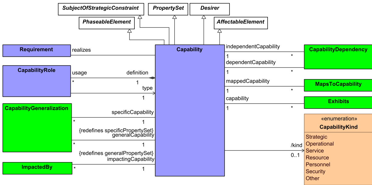
Figure 9:53 - Capability
