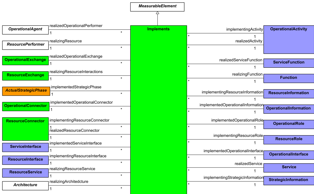
Figure 9:35 - Implements
