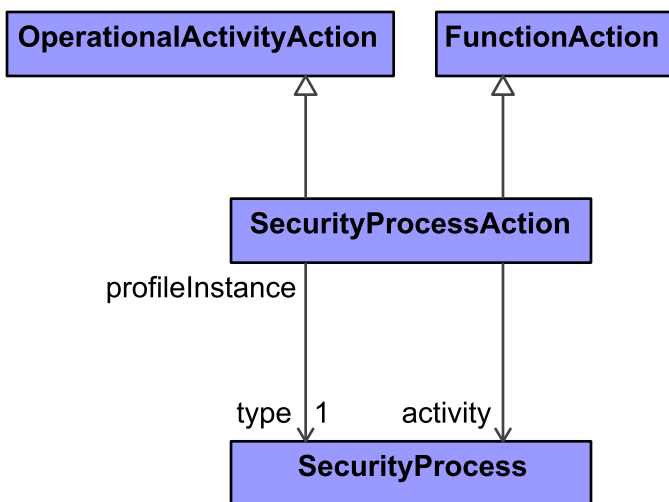
Figure 9:213 - SecurityProcessAction
