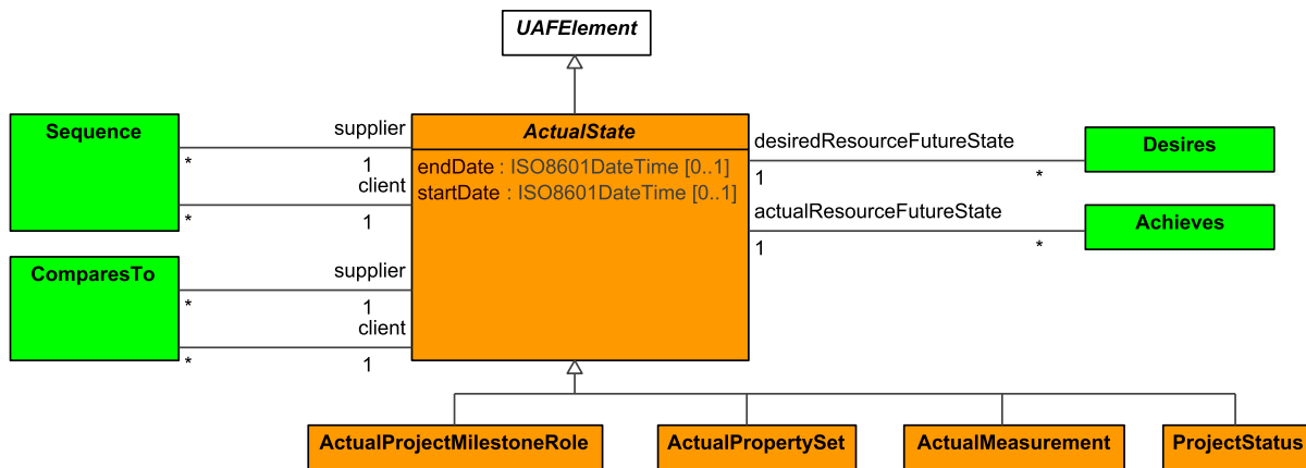
Figure 9:1 - ActualState
