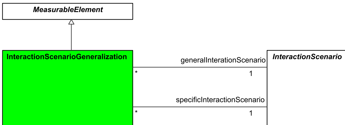
Figure 9:3 - InteractionScenarioGeneralization
