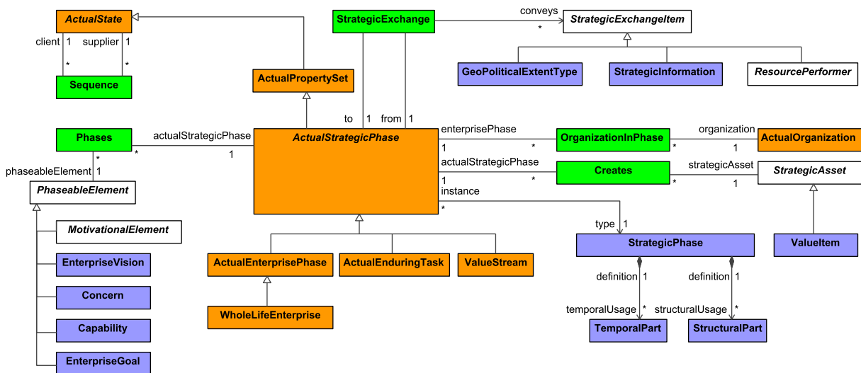
Figure 8:16 - Strategic Processes
