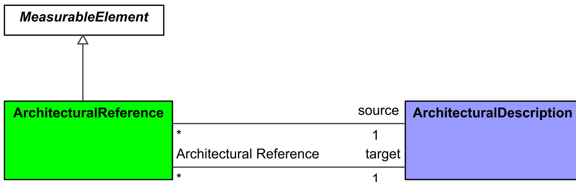
Figure 9:33 - ArchitecturalReference
