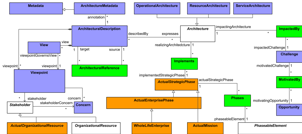
Figure 8:11 - Summary & Overview
