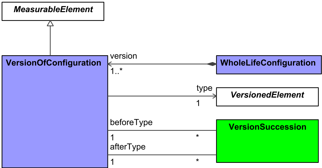
Figure 9:193 - VersionOfConfiguration
