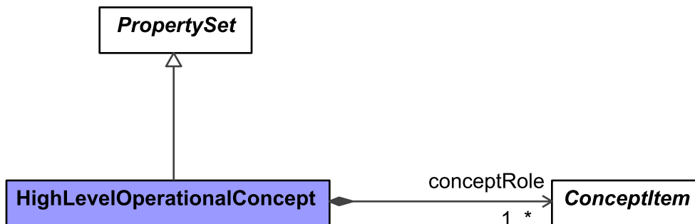
Figure 9:96 - HighLevelOperationalConcept
