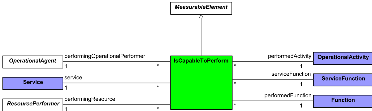
Figure 9:13 - IsCapableToPerform
