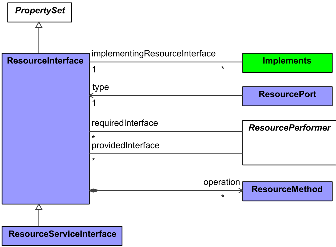
Figure 9:177 - ResourceInterface
