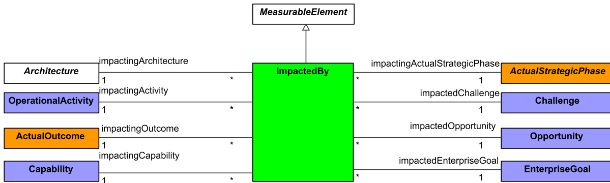
Figure 9:48 - ImpactedBy
