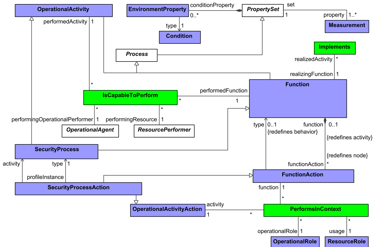
Figure 8:73 - Security Processes
