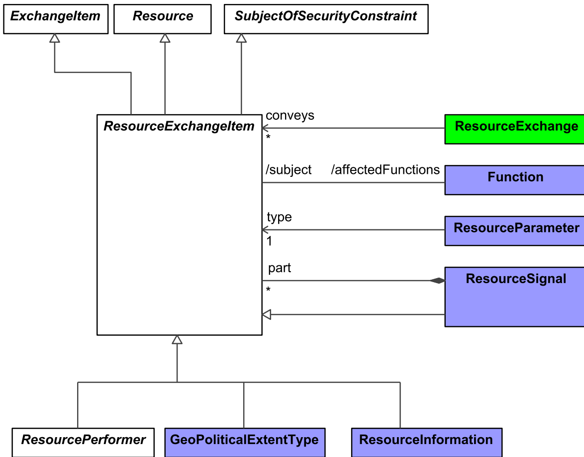
Figure 9:176 - ResourceExchangeItem
