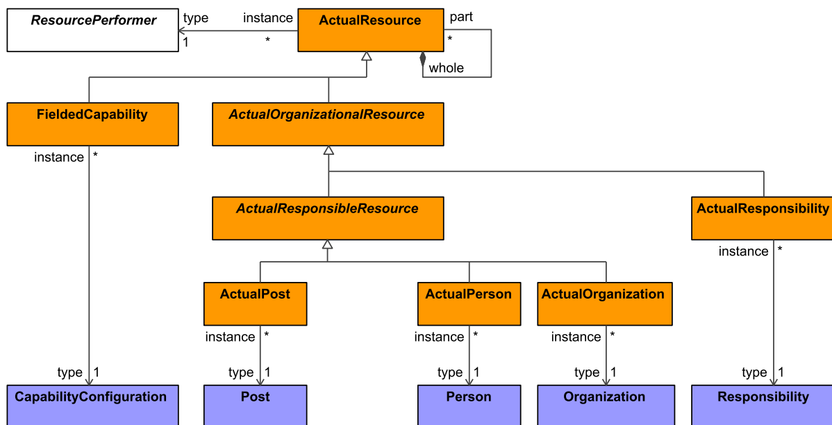
Figure 8:86 - Actual Resources Structure
