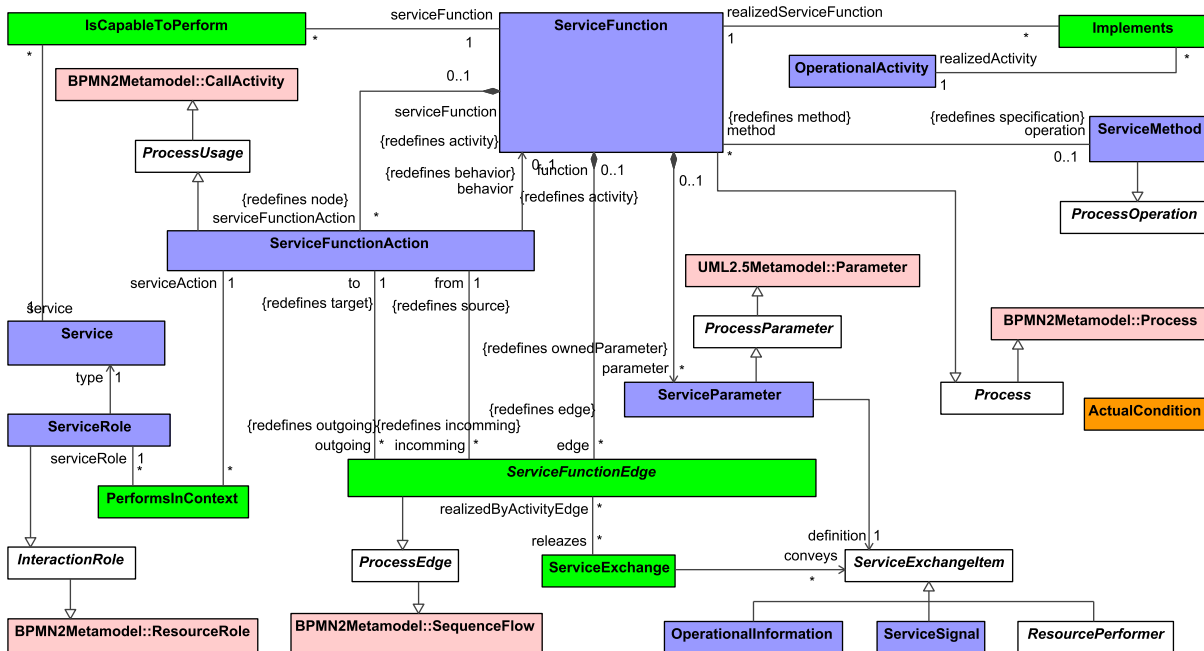
Figure 8:38 - Services Processes BPMN Semantics
