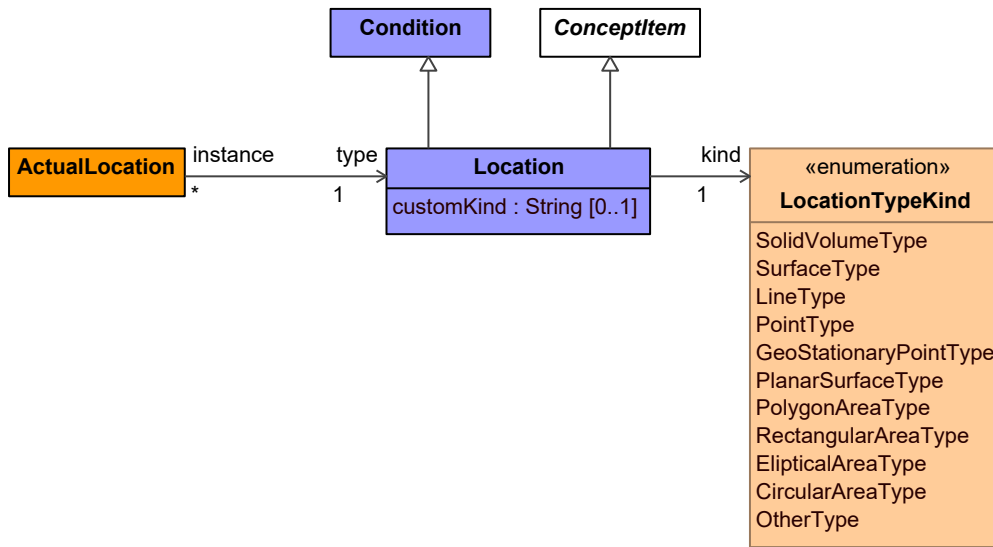
Figure 9:355 - Location
