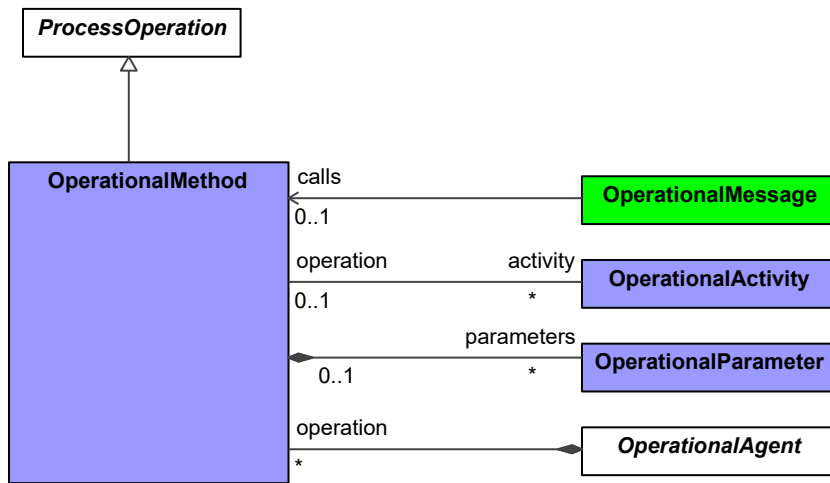
Figure 9:189 - OperationalMethod
