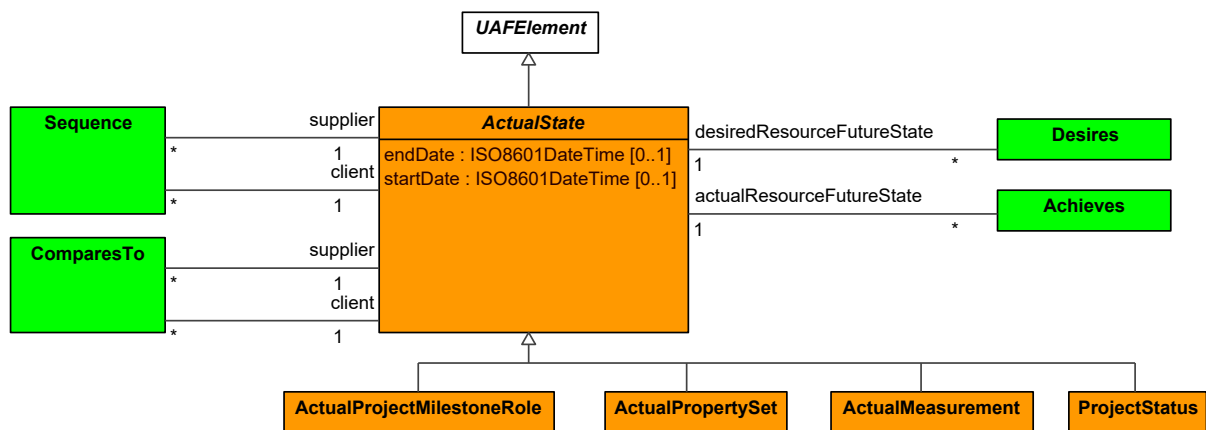
Figure 9:95 - ActualState
