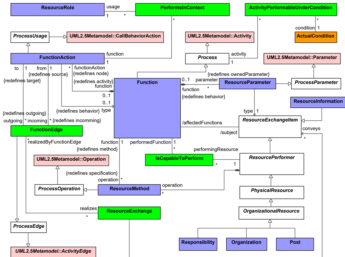
Figure 8:45 - Personnel Processes
