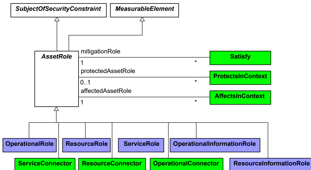
Figure 9:294 - AssetRole
