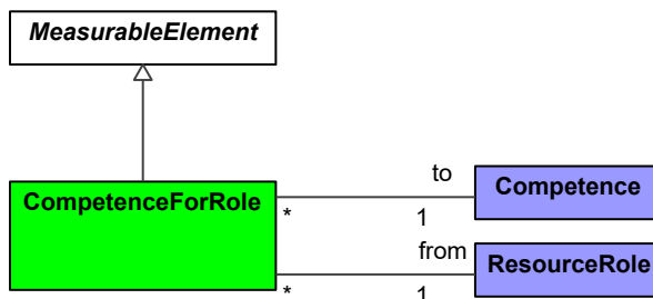
Figure 9:243 - CompetenceForRole
