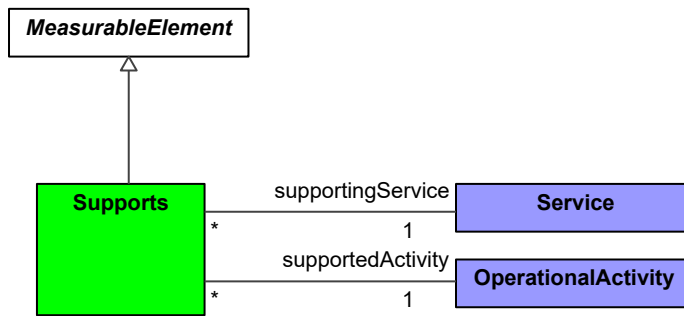
Figure 9:231 - Supports
