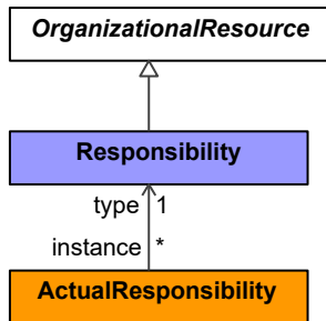
Figure 9:236 - Responsibility
