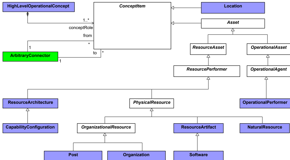
Figure 8:23 - Operational Taxonomy
