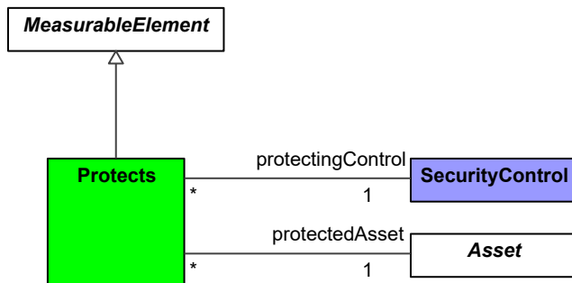
Figure 9:284 - Protects
