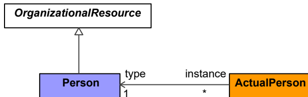
Figure 9:234 - Person
