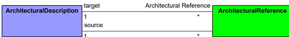
Figure 8:3 - Architecture References
