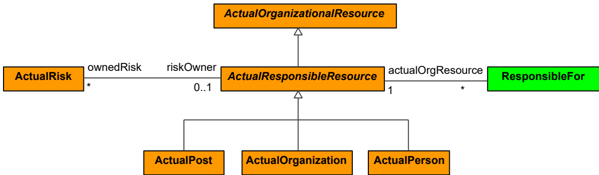
Figure 9:334 - ActualResponsibleResource
