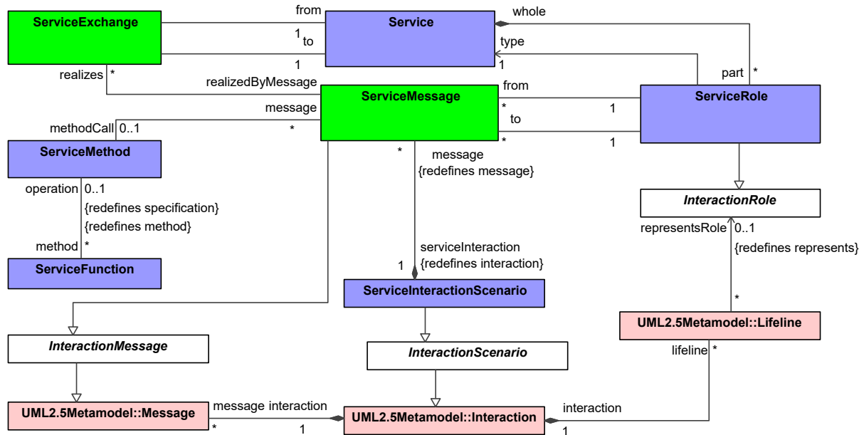
Figure 8:38 - Services Sequences
