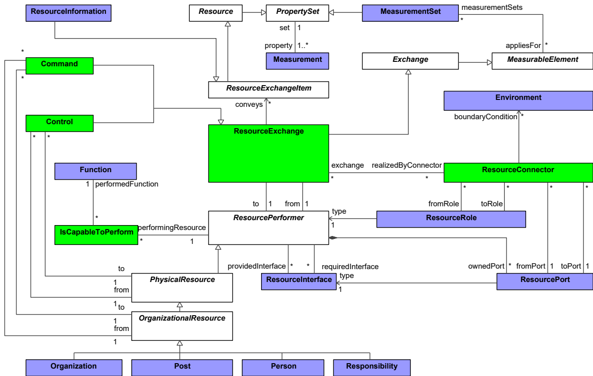
Figure 8:44 - Personnel Connectivity
