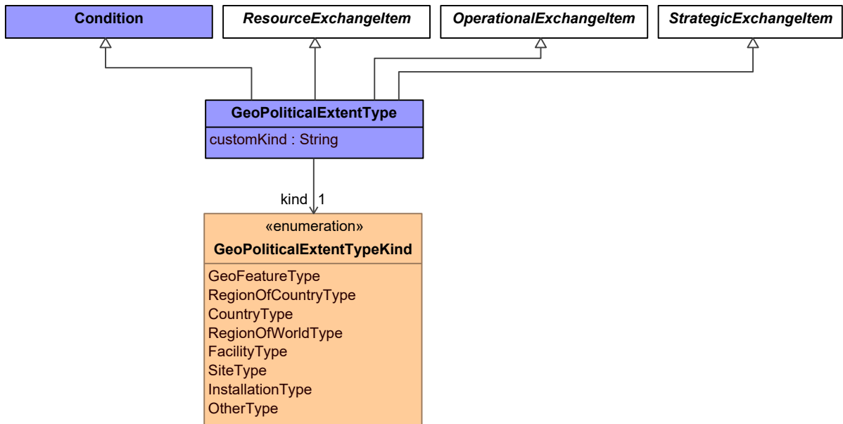
Figure 9:354 - GeoPoliticalExtentType
