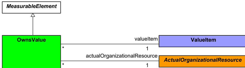
Figure 9:150 - OwnsValue
