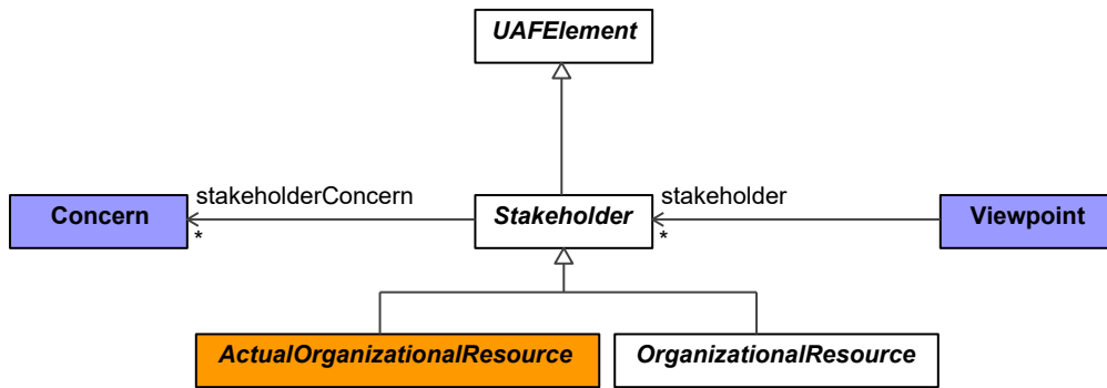
Figure 9:133 - Stakeholder
