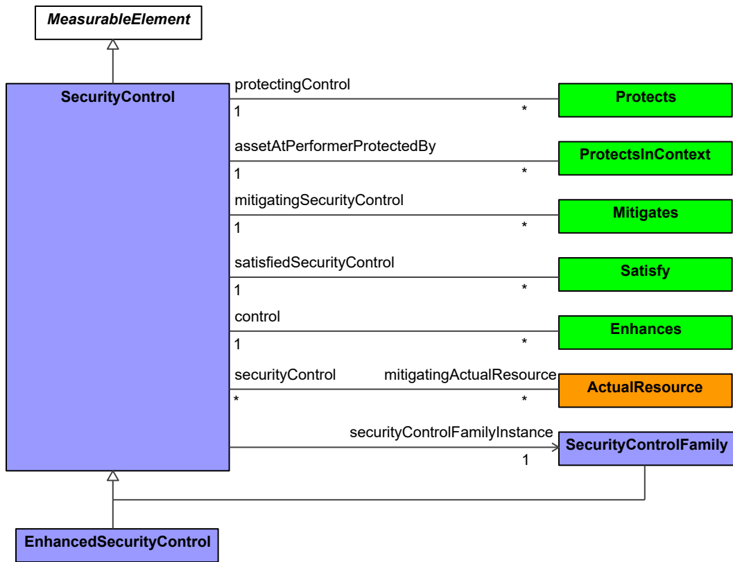
Figure 9:286 - SecurityControl
