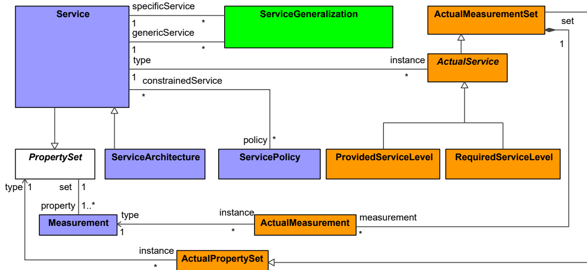
Figure 8:32 - Services Taxonomy
