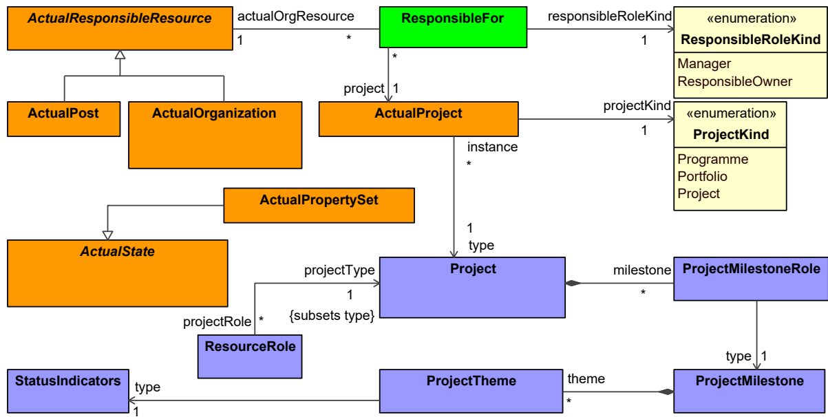
Figure 8:74 - Project Structure
