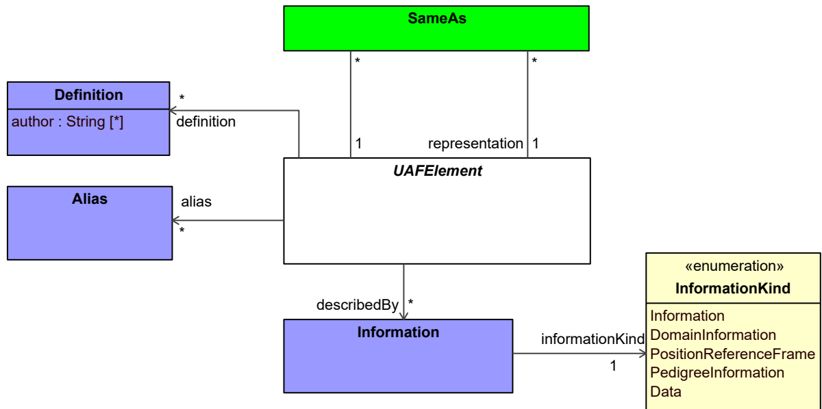
Figure 8:6 - Dictionary Elements
