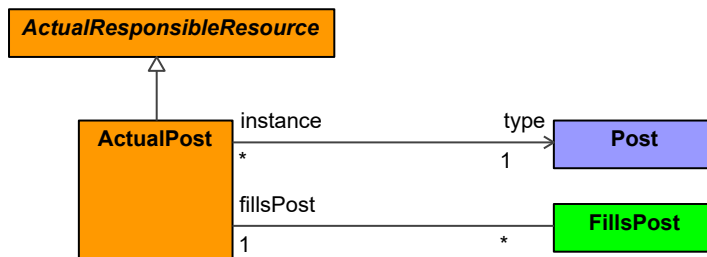
Figure 9:330 - ActualPost
