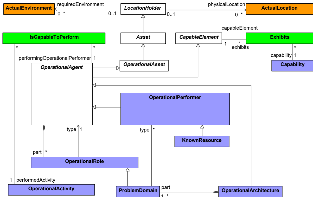
Figure 8:24 - Operational Structure
