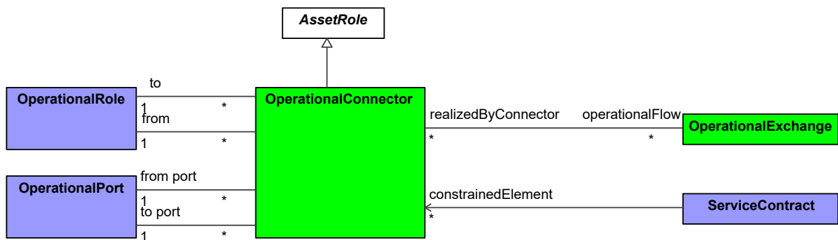
Figure 9:194 - OperationalConnector
