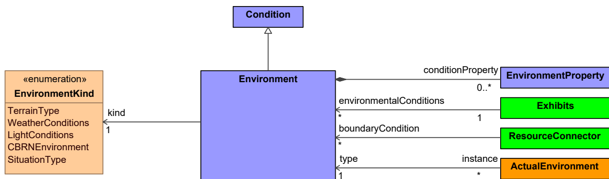
Figure 9:352 - Environment
