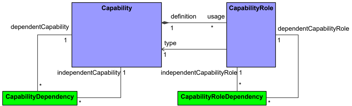
Figure 8:15 - Strategic Connectivity
