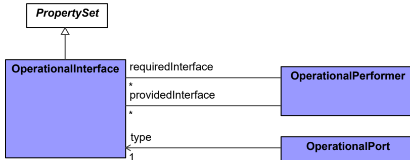
Figure 9:197 - OperationalInterface
