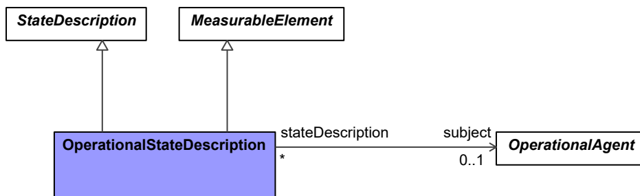
Figure 9:204 - OperationalStateDescription
