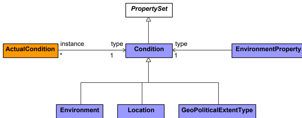
Figure 9:351 - Condition
