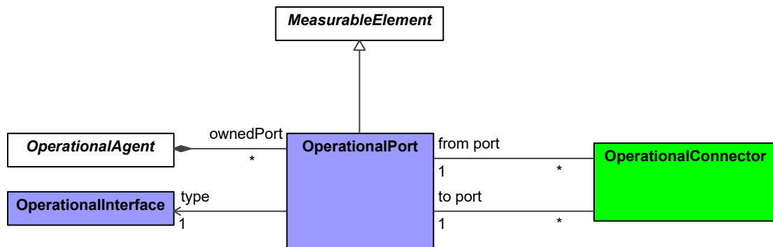
Figure 9:198 - OperationalPort
