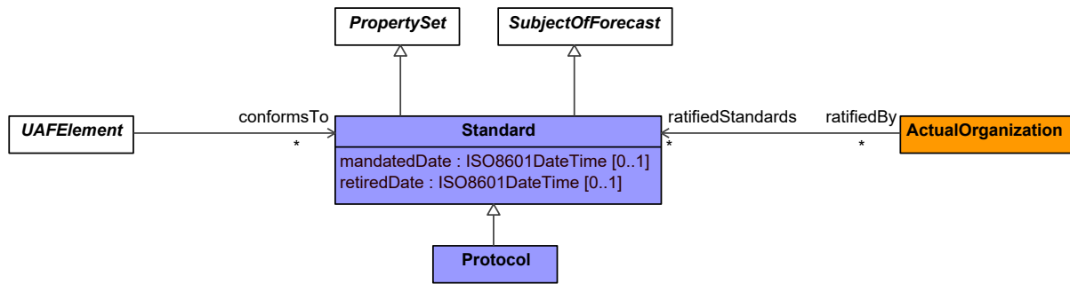
Figure 9:325 - Standard
