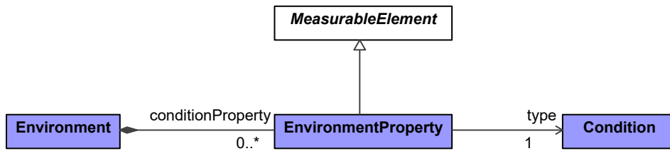
Figure 9:353 - EnvironmentProperty
