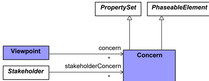
Figure 9:131 - Concern
