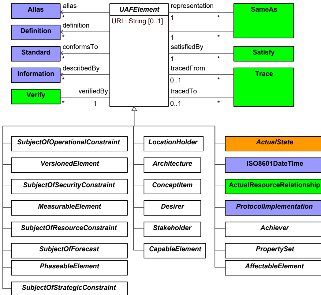
Figure 9:134 - UAFElement
