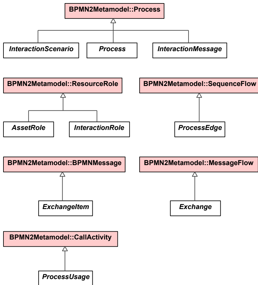
Figure 8:92 - BPMN
