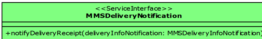
Figure 8.10—Definition of MMSDeliveryNotification client interface
