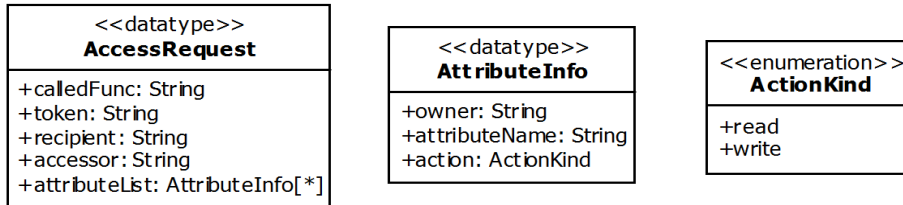
Figure 8.28 - Specific data types for the Privacy Resource Manager Interface
