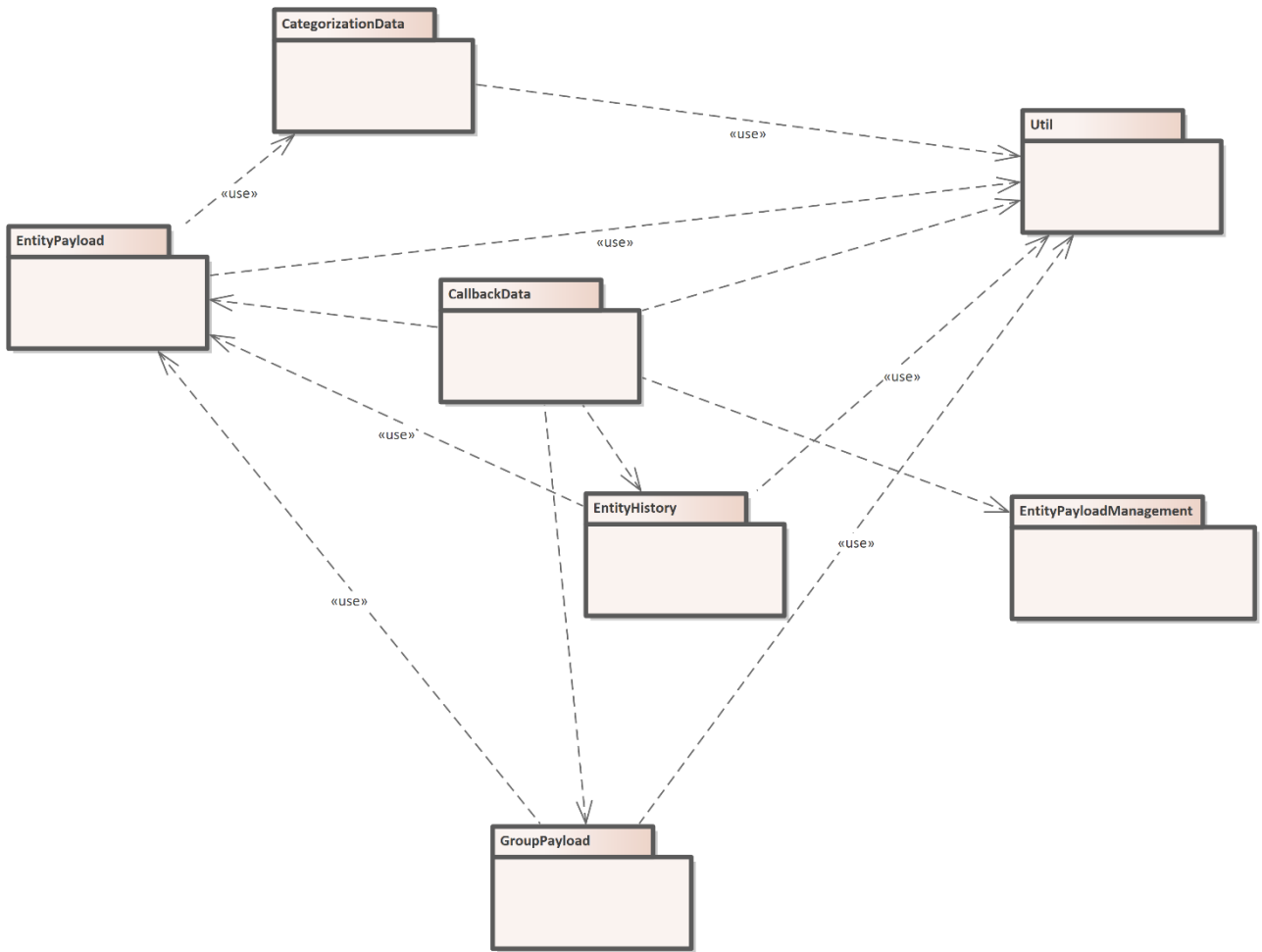
Figure 7-1: DataPayload (Class diagram)
