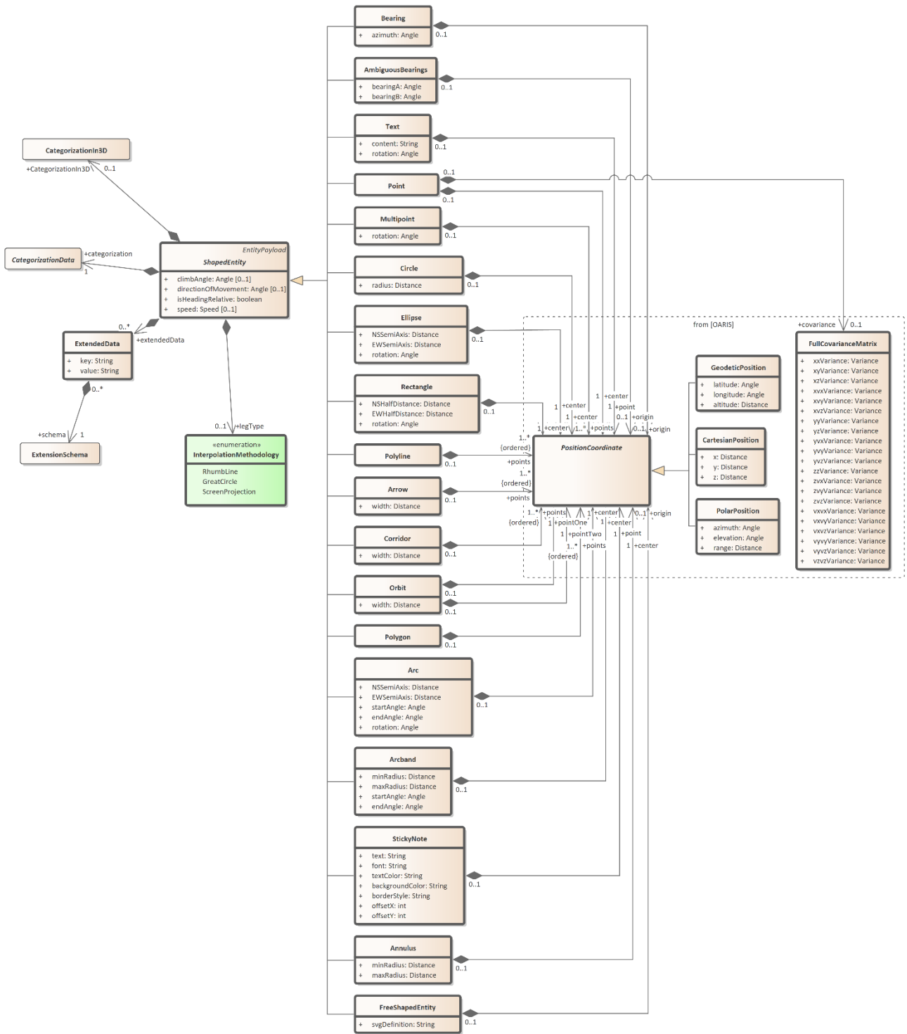
Figure 7-5: EntityPayload - 2 of 2 (Class diagram)
