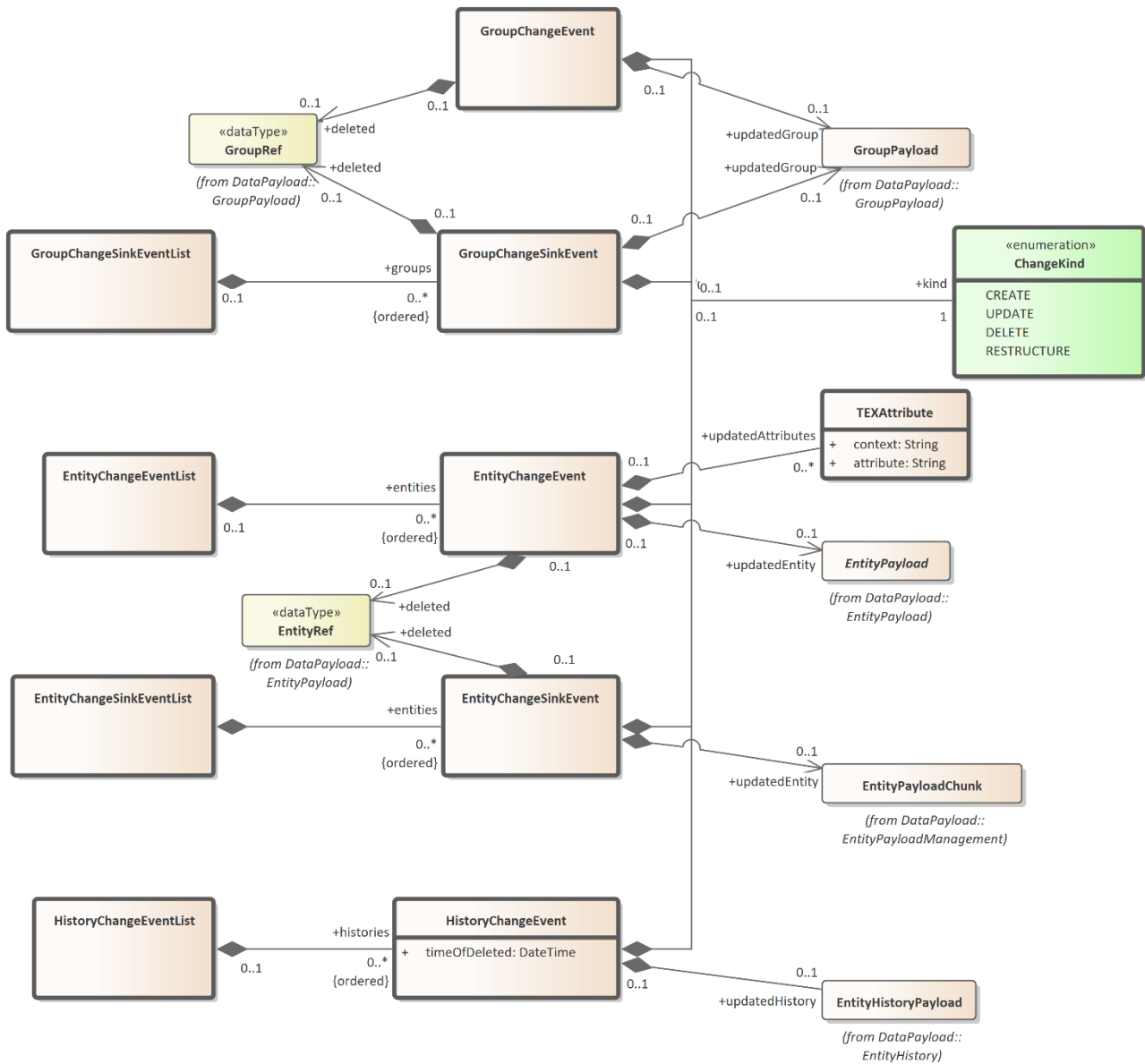
Figure 7-8: CallbackData (Class diagram)
