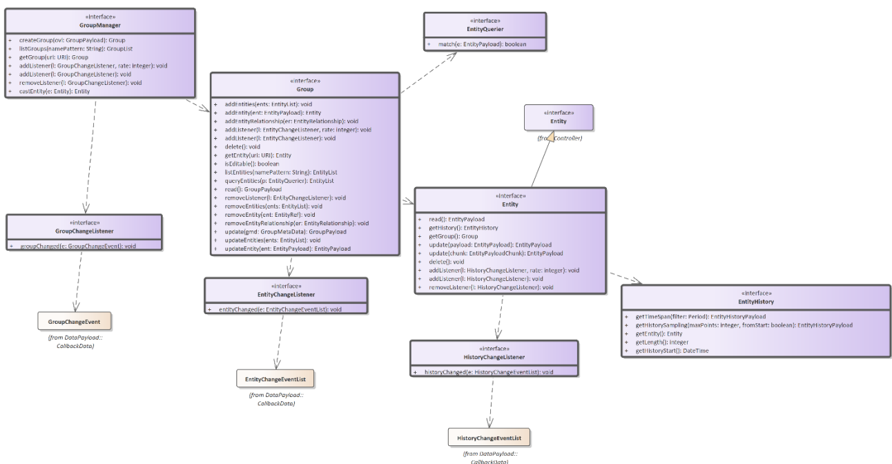
Figure 8-1: DataInterface (Class diagram)
