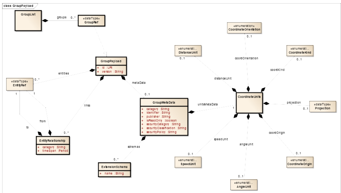
Figure 7-3: GroupPayload (Class diagram)
