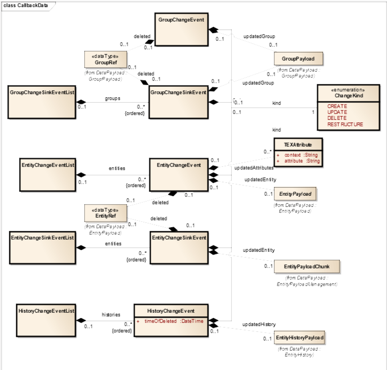
Figure 7-8: CallbackData (Class diagram)
