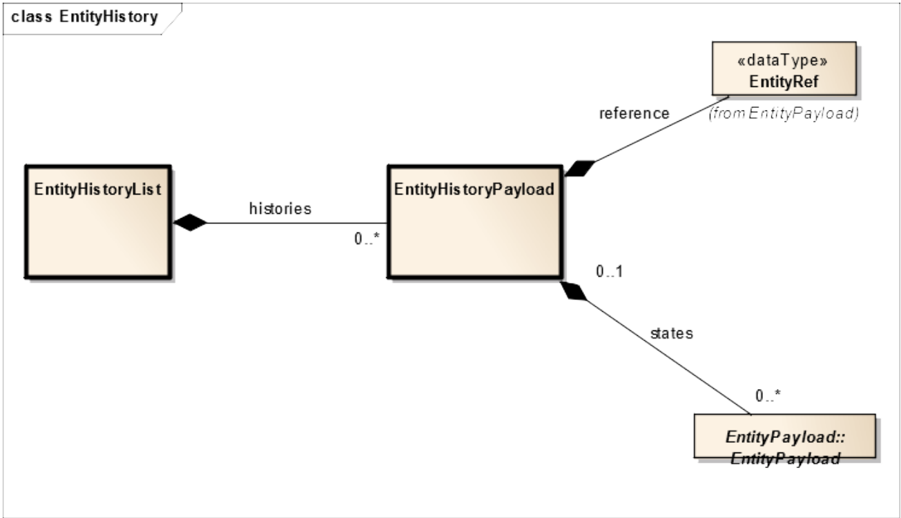
Figure 7-7: EntityHistory (Class diagram)
