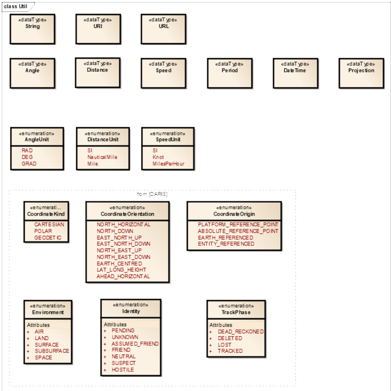
Figure 7-2: Util (Class diagram)
