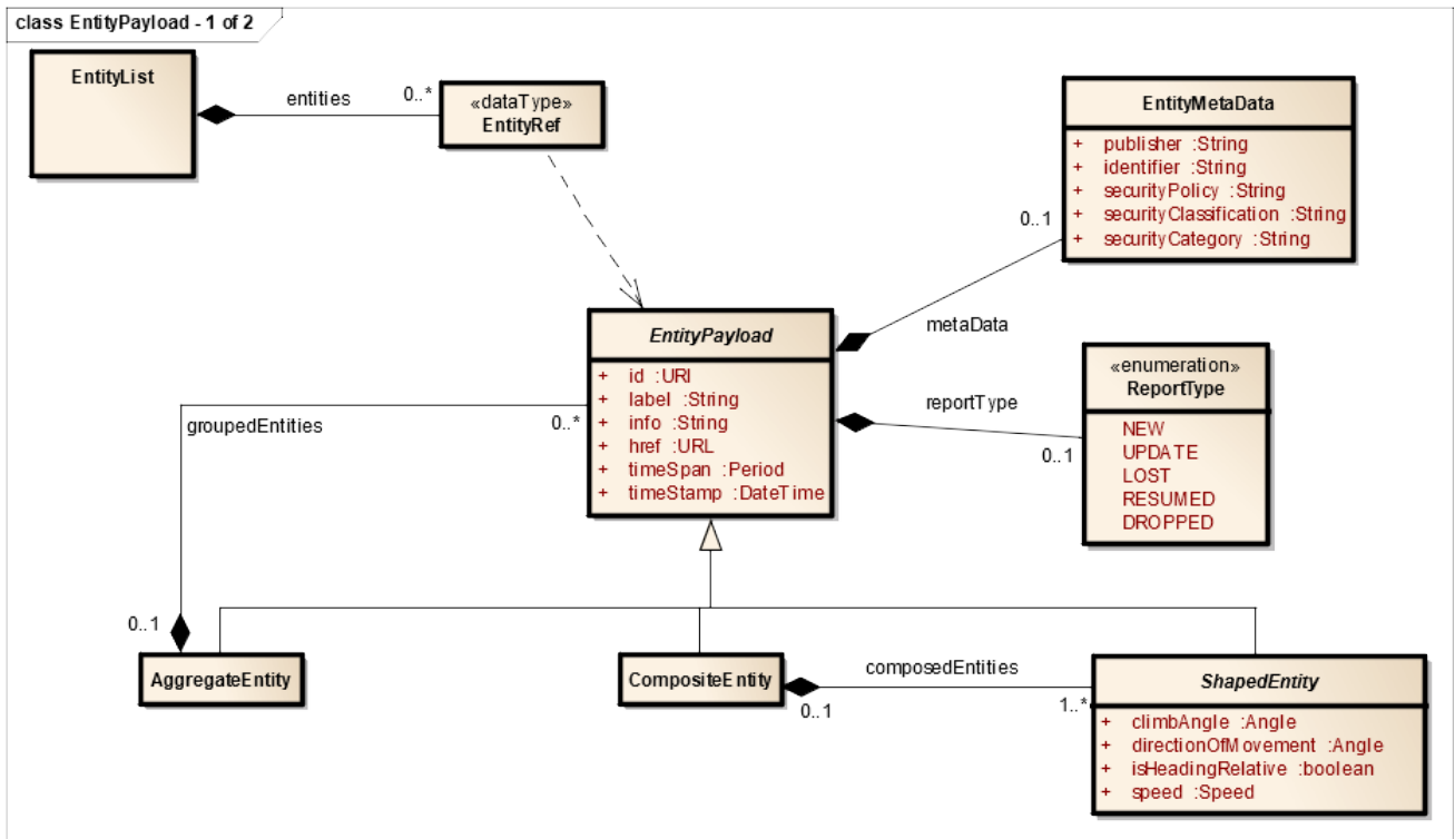
Figure 7-4: EntityPayload - 1 of 2 (Class diagram)
