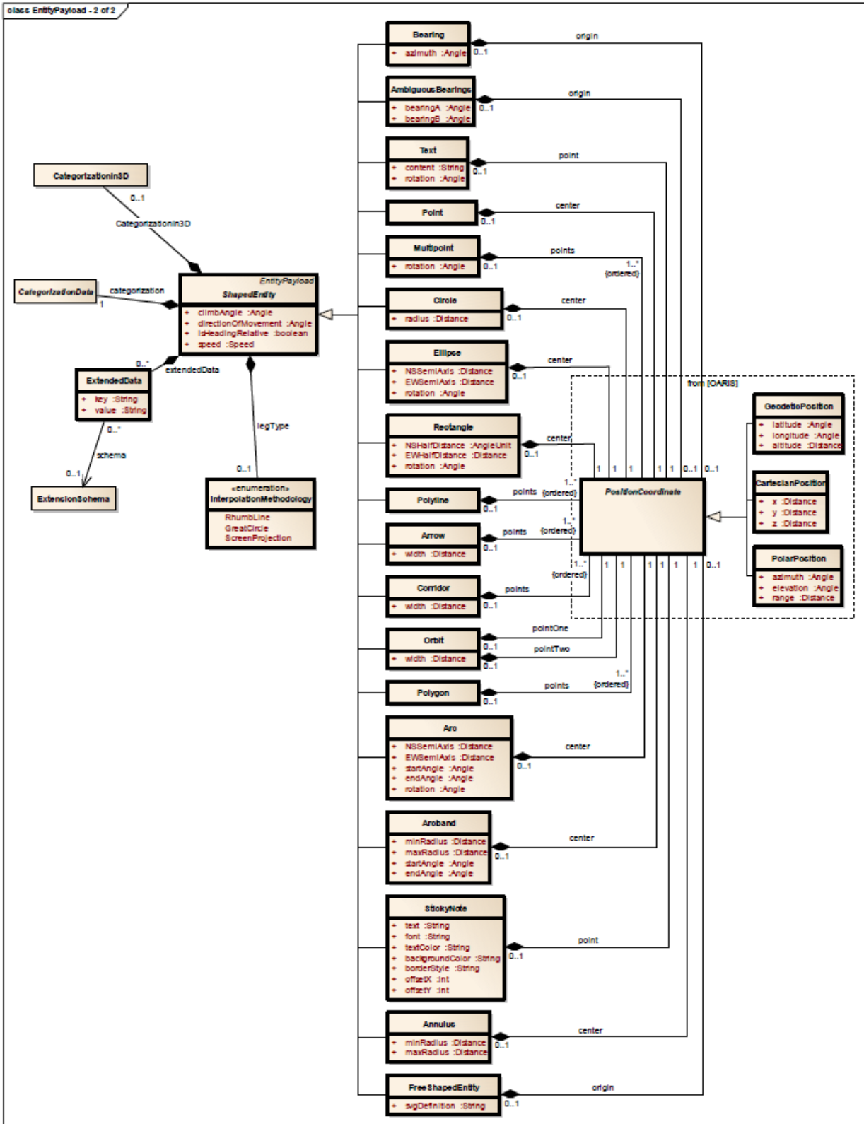
Figure 7-5: EntityPayload - 2 of 2 (Class diagram)
