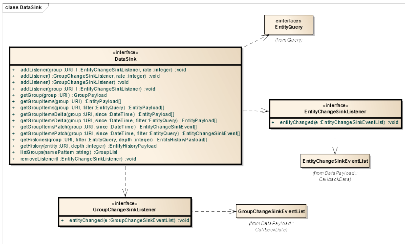
Figure 9-1: DataSink (Class diagram)
