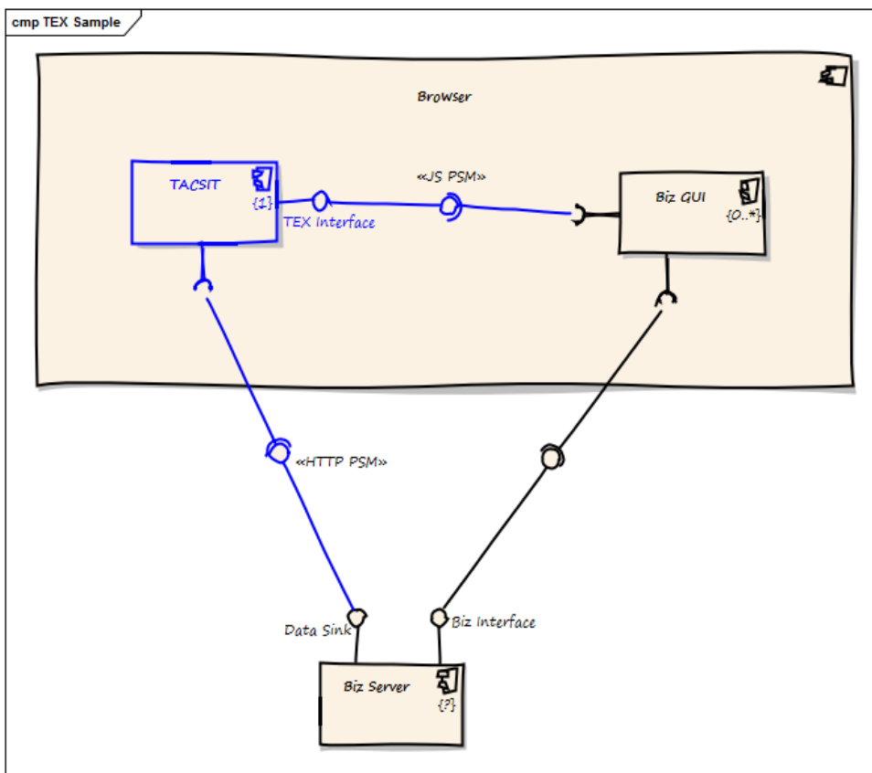
Figure 5.5 – Example of use of a web-based TACSIT system (non-normative)
