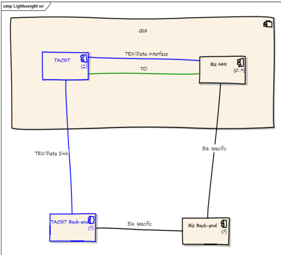
Figure 5.4 – Distributed With TACSIT back-end Architecture Pattern (non-normative)
