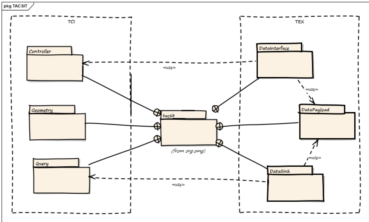
Figure 5.6 – Enhancement to TACSIT TCI by TACSIT TEX
