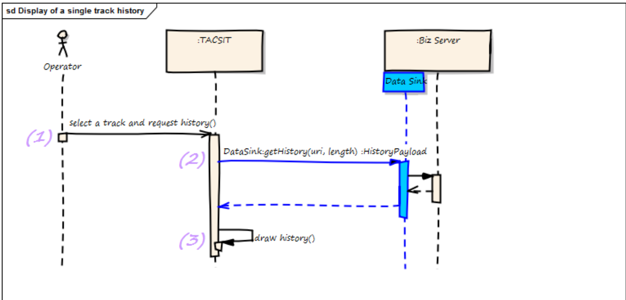
Figure 5.10 – The 'Display of a Single Track/BSO History' Use pattern
