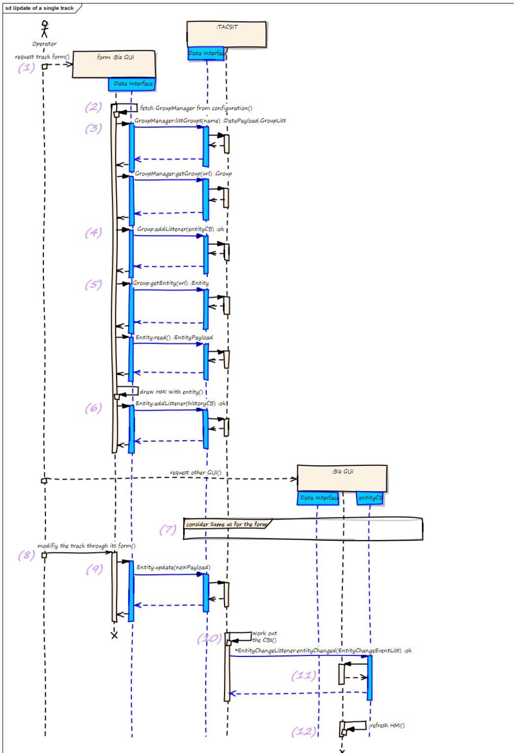
Figure 5.8 – The 'Update of a Single Track/BSO' Use pattern
