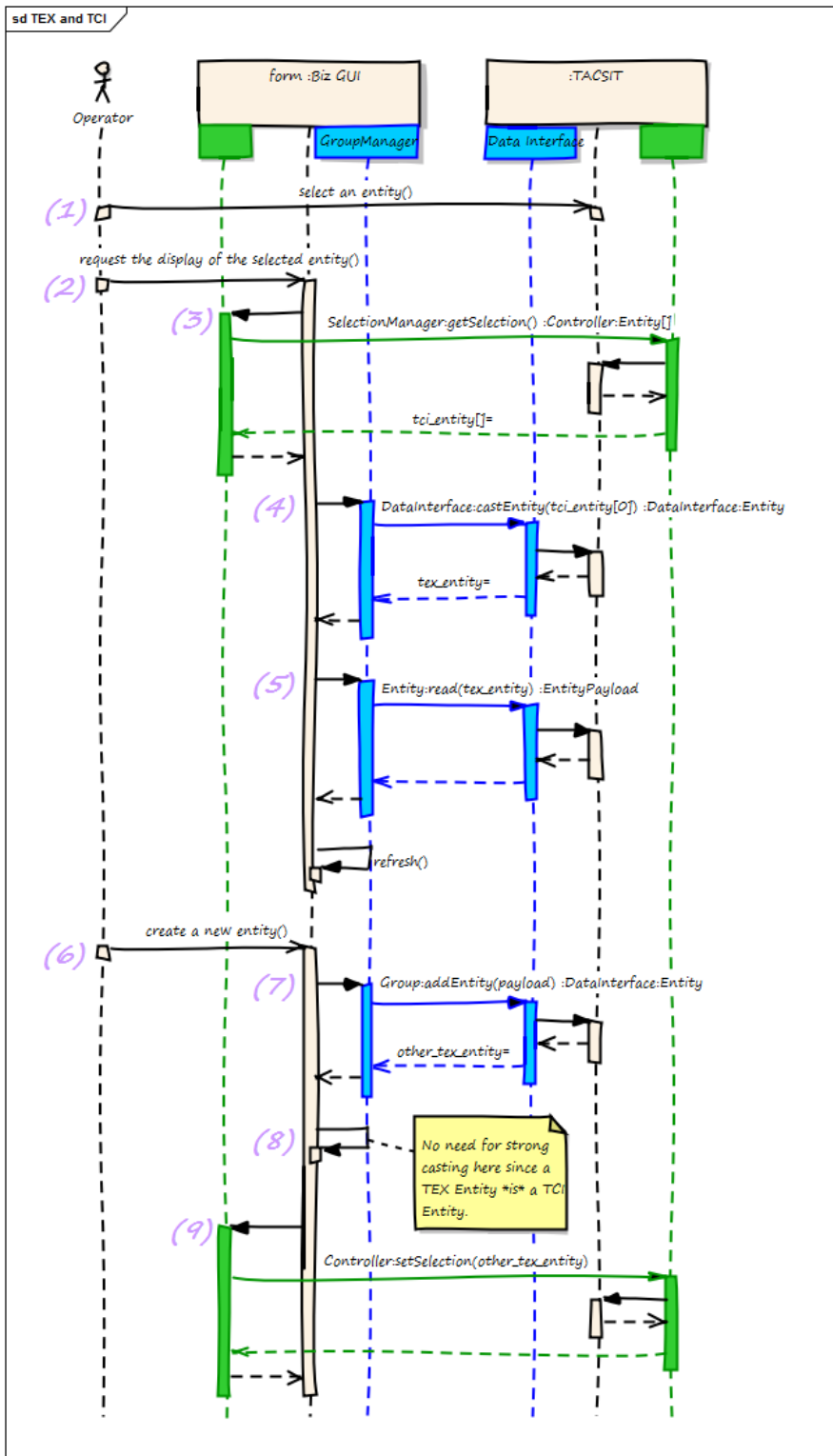
Figure 5.11 – The 'TEX and TCI' Use pattern
