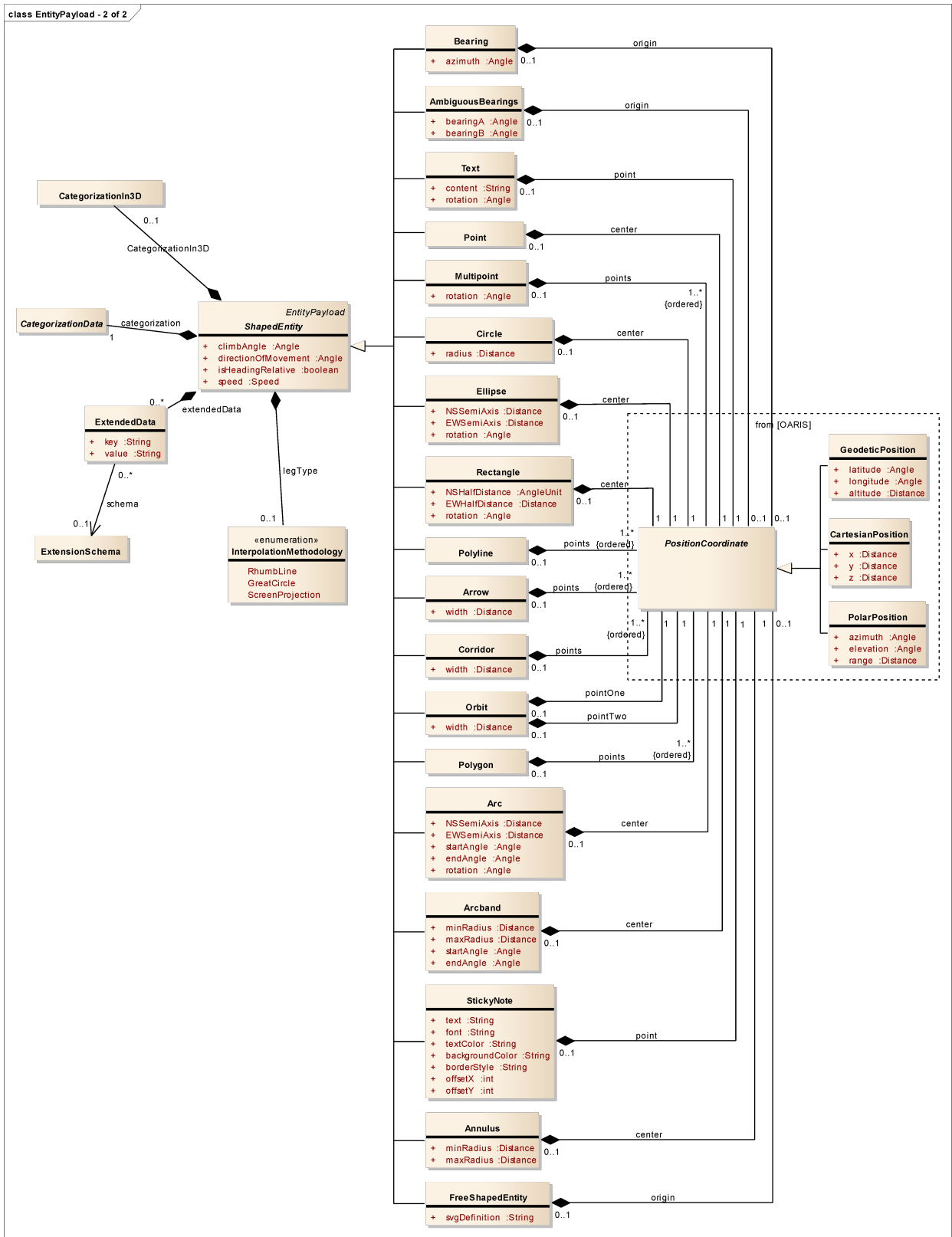
Figure 6.5 - EntityPayload - 2 of 2 (Class diagram)
