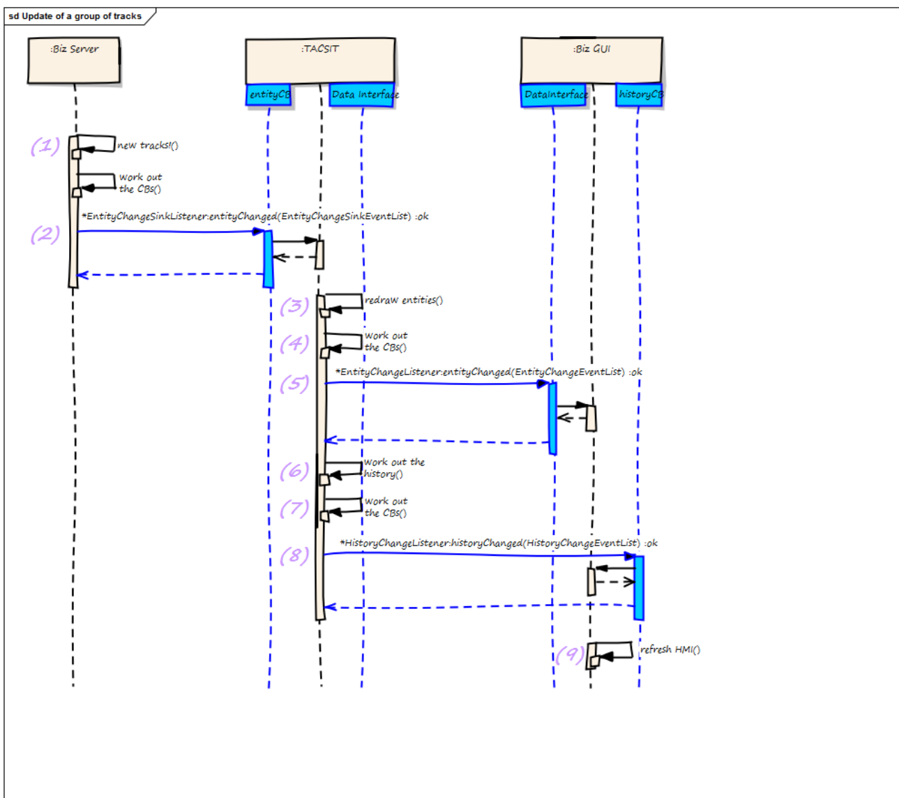
Figure 5.9 – The 'Update of a Group of Tracks/BSOs' Use pattern
