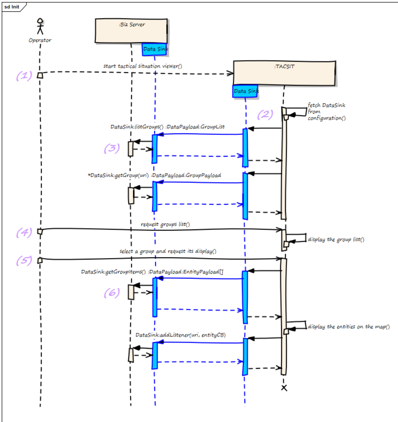
Figure 5.7 – The 'Initialization' Use pattern
