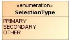
Figure 7.19 - SelectionType
