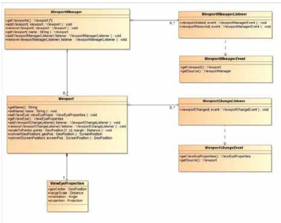
Figure 7.3 - Viewport Interfaces
