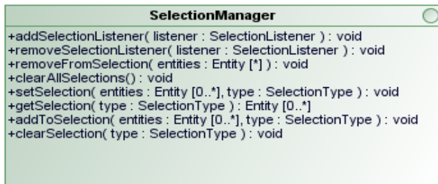
Figure 7.9 - SelectionManager
