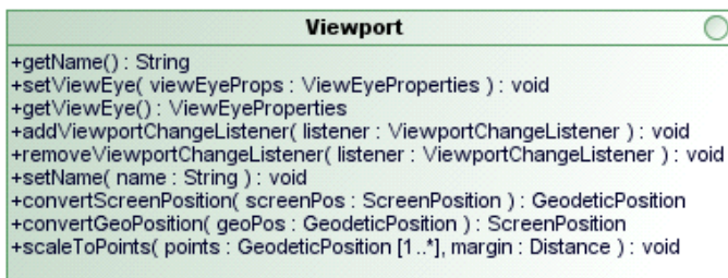
Figure 7.12 - Viewport
