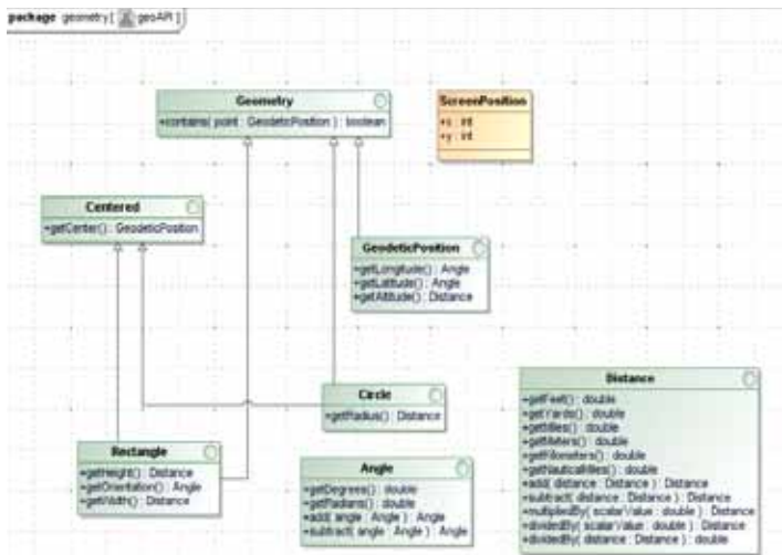
Figure 7.27 - Query Interfaces
