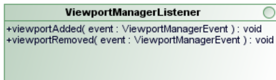
Figure 7.17 - ViewportManagerListener
