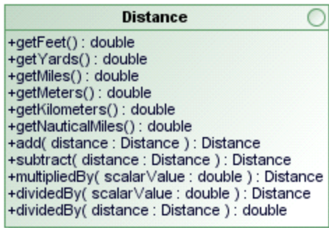
Figure 7.35 - Distance
