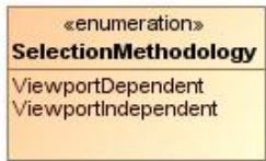
Figure 7.18 - SelectionMethodology
