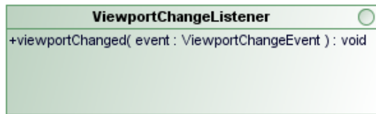
Figure 7.14 - ViewportChangeListener
