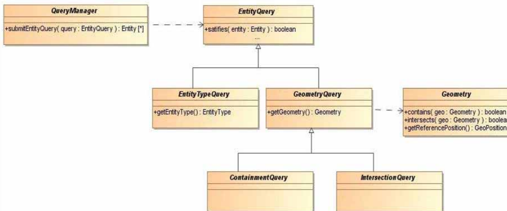
Figure 7.20 - Query Interfaces
