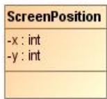
Figure 7.30 - ScreenPosition
