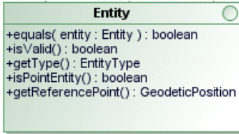
Figure 7.4 - Entity
