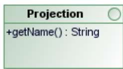
Figure 7.6 - Projection
