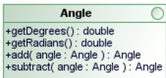
Figure 7.34 - Angle
