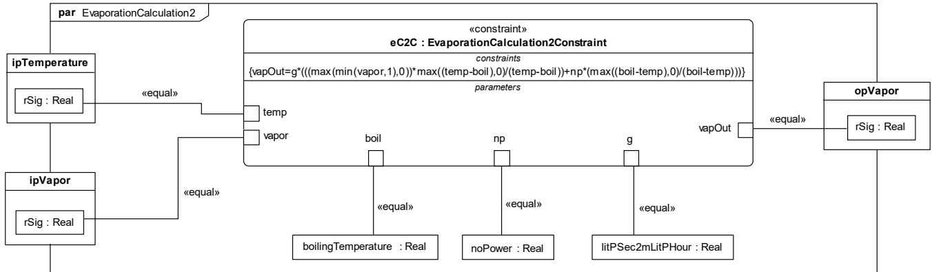
Figure 91: Parametric diagram applying the second evaporation calculation constraint
