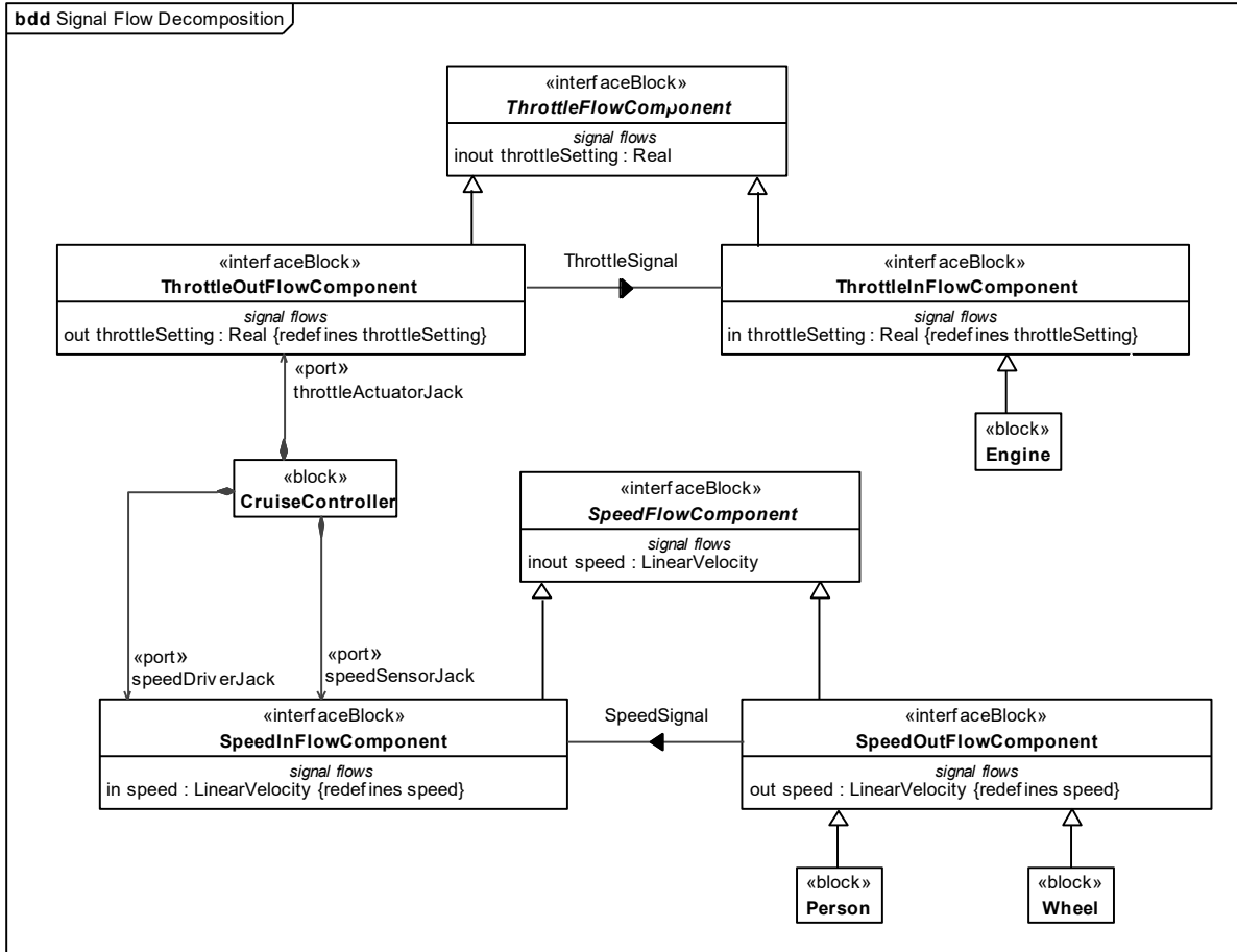
Figure 110: Signal flow interactions blocks, ports, & component properties
