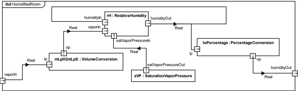
Figure 66: Internal structure of the humidified room
