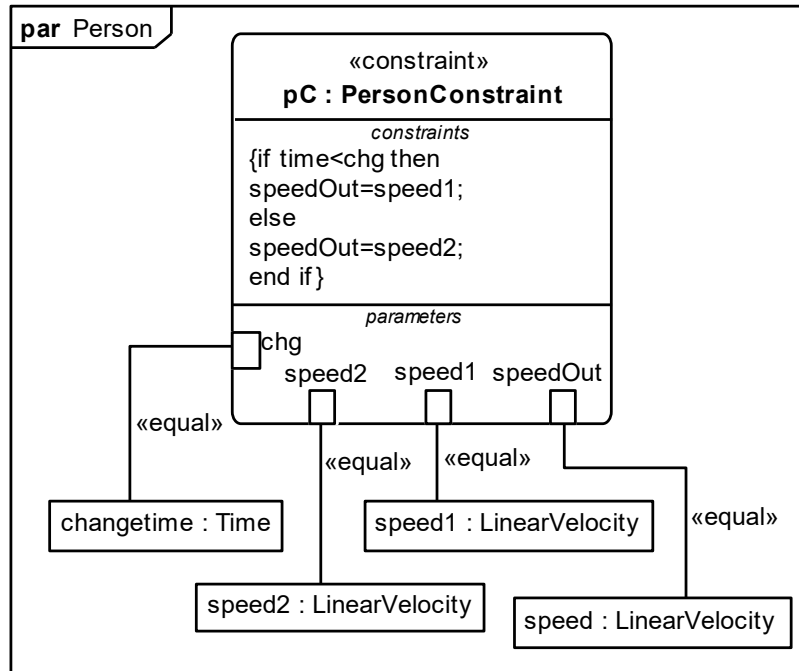
Figure 119: Parametric diagram applying the person constraint
