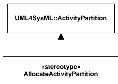
Figure 15.2 - Abstract syntax expression for AllocatedActivityPartition
