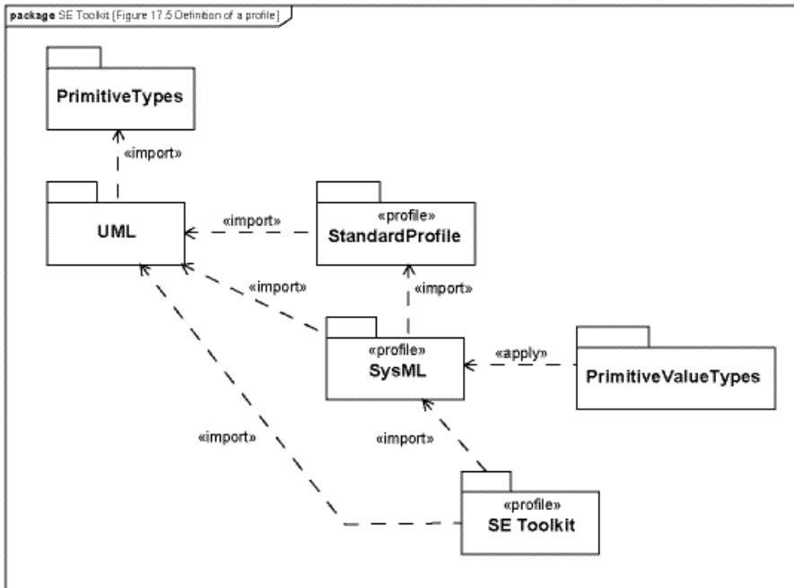
Figure 17.5 - Definition of a profile
