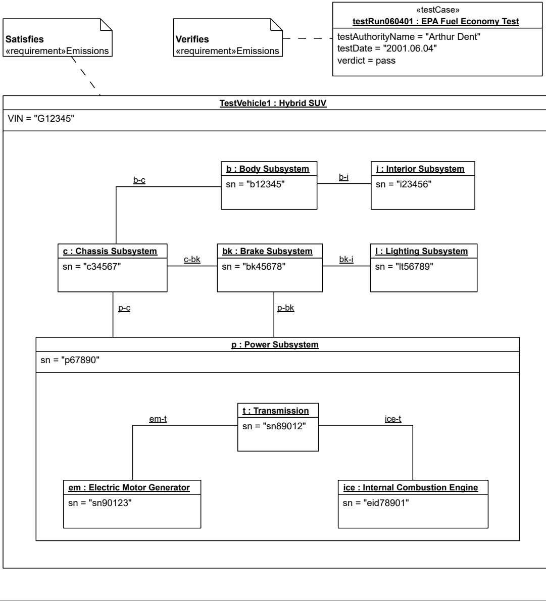
Figure D.41. Test Results
