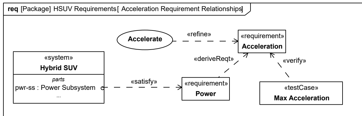
Figure D.13. Acceleration Requirement Relationships
