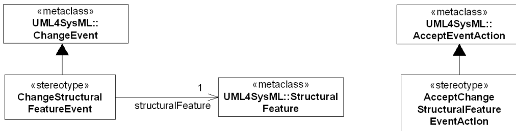
Figure 9.3 - Stereotypes for Property Value Change Events
