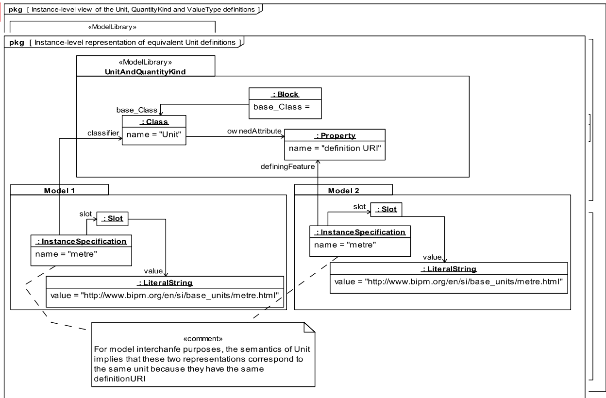
Figure 8.21 - Instance-level representation of equivalent Unit definitions
