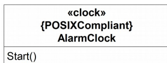
Figure 17.2 - Using a stereotype
