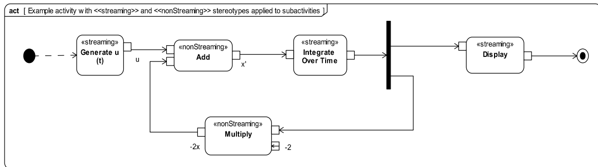
Figure E.2: Example activity with «streaming» and «nonStreaming» stereotypes applied to subactivities
