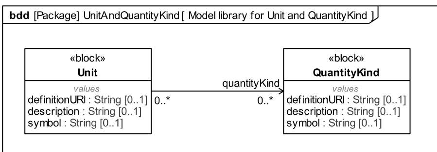
Figure 8.11: Model library for Unit and QuantityKind
