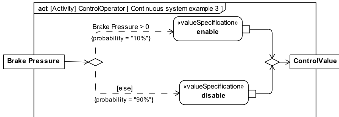
Figure 11.12 - Continuous system example 3
