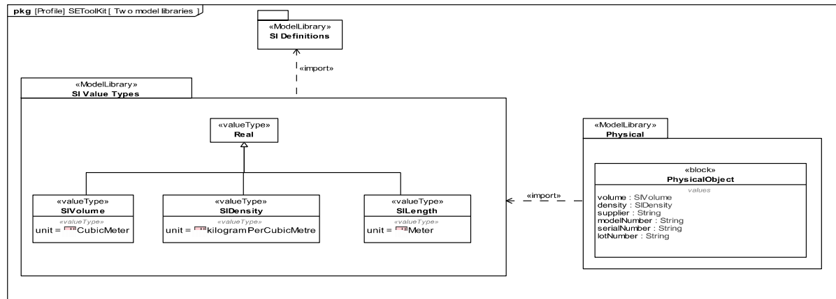
Figure 17.7 - Two model libraries
