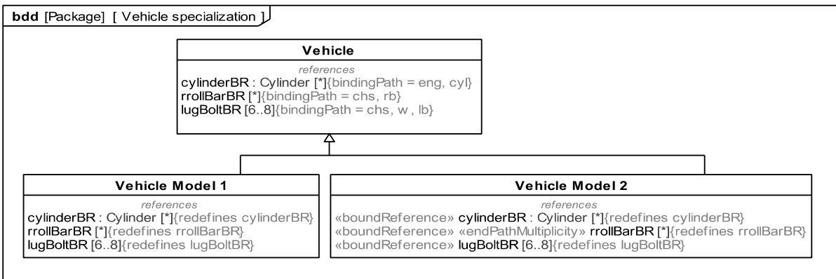
Figure 8.17: Vehicle specialization
