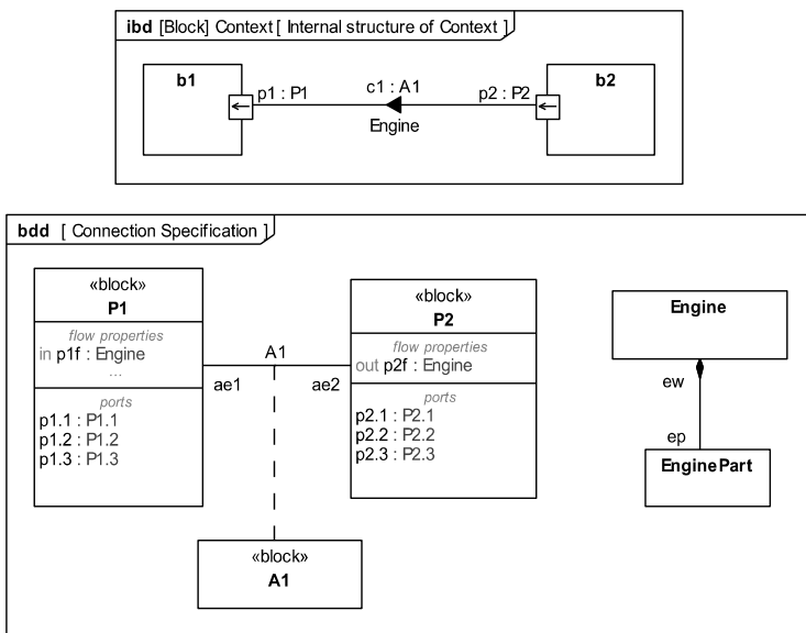
Figure 9.17 - Usage example of item flow decomposition
