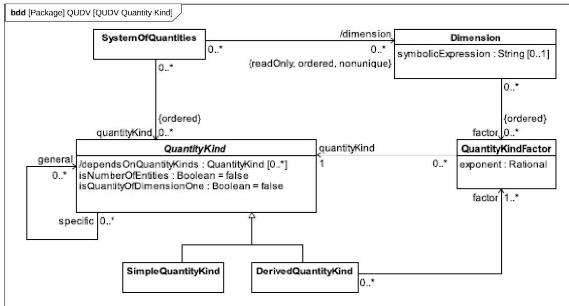
Figure E.7: QUDV QuantityKinds Diagram
