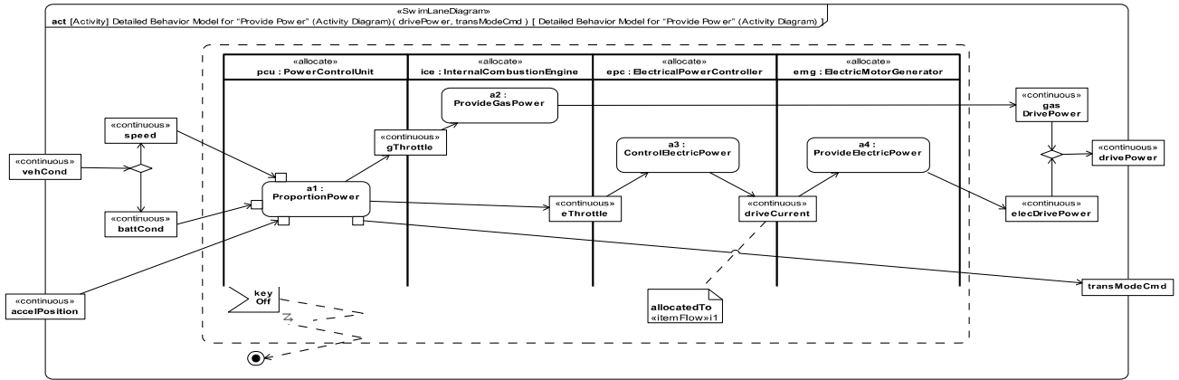
Figure D.38: Detailed Behavior Model for "Provide Power" (Activity Diagram) Note hierarchical consistency with Figure D.36.
