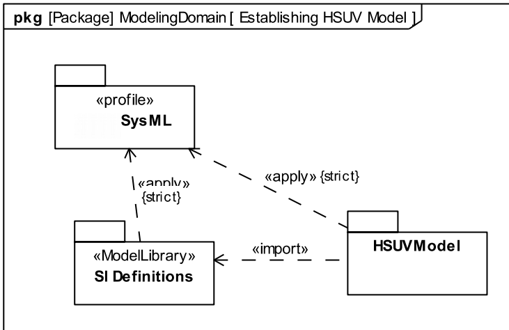
Figure 17.8 - A model with applied profile and imported model library
