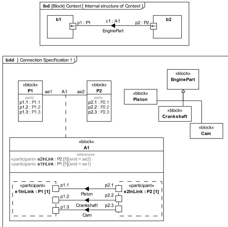
Figure 9.16 - Usage example of item flow decomposition
