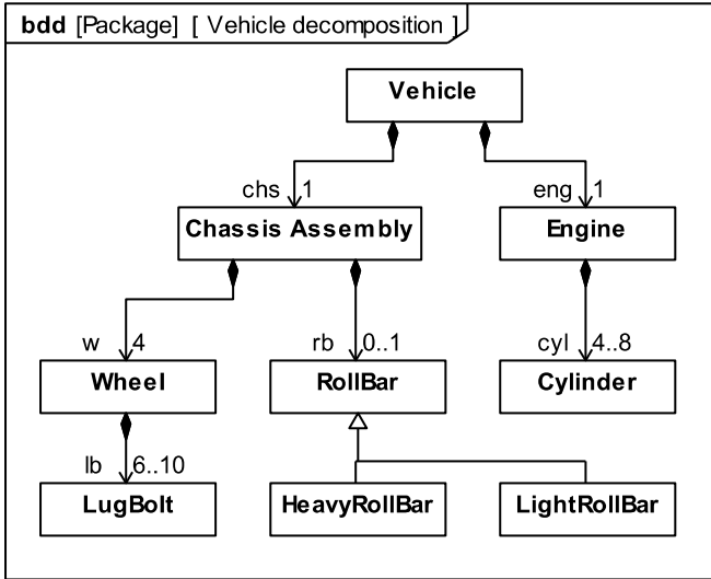
Figure 8.15: Vehicle Decomposition
