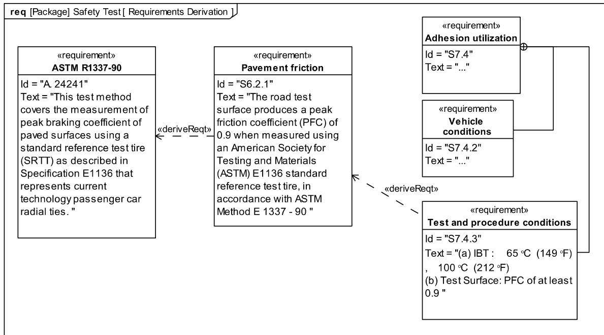
Figure 16.2 - Requirements Derivation
