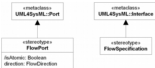
Figure C.1: Deprecated Stereotypes
