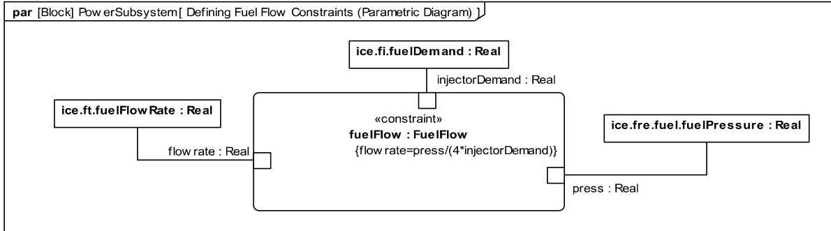
Figure D.24: Defining Fuel Flow Constraints (Parametric Diagram)
