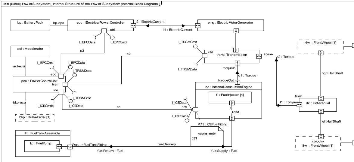
Figure D.19: Internal Structure of the Power Subsystem (Internal Block Diagram)
